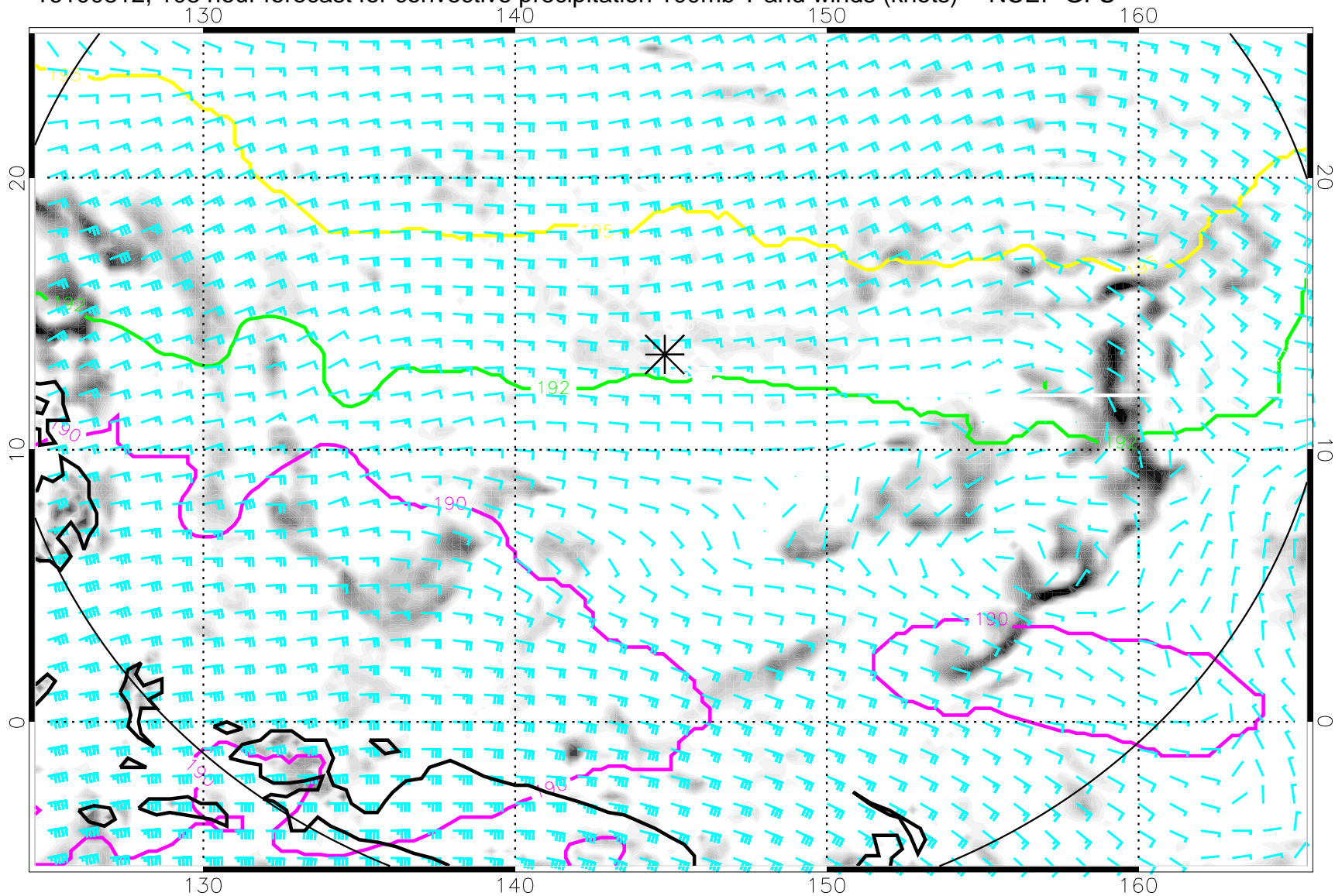
16100812, 108 hour forecast for convective precipitation 100mb T and winds (knots) -- NCEP GFS
