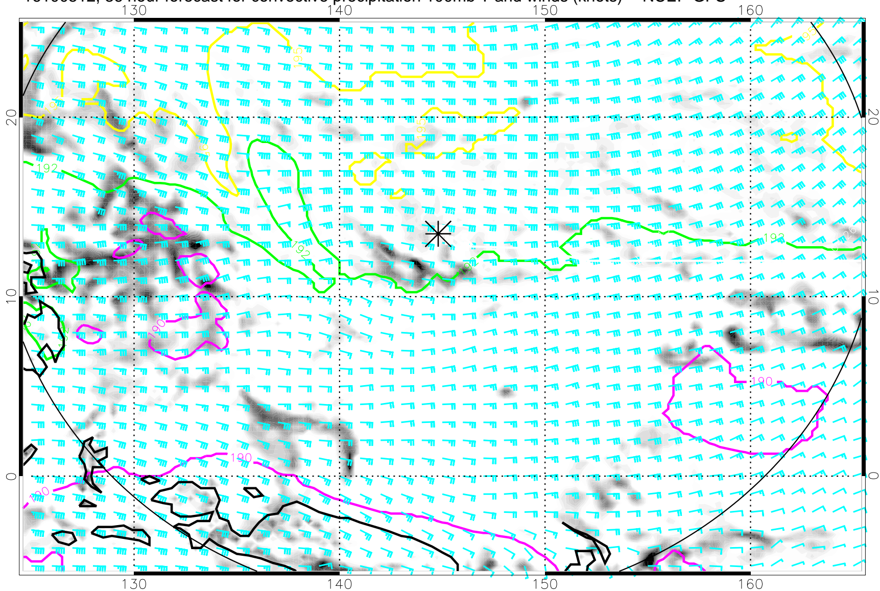
16100512, 36 hour forecast for convective precipitation 100mb T and winds (knots) -- NCEP GFS
