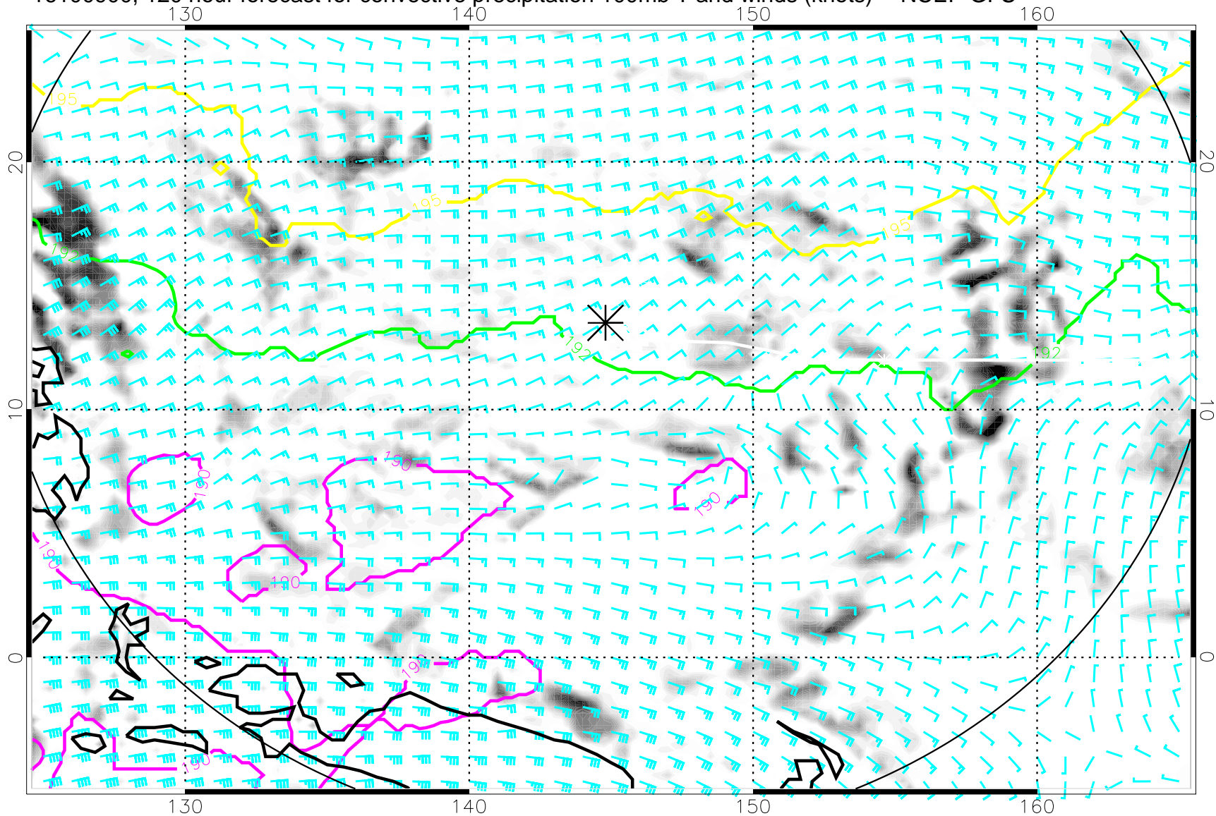
16100900, 120 hour forecast for convective precipitation 100mb T and winds (knots) -- NCEP GFS
