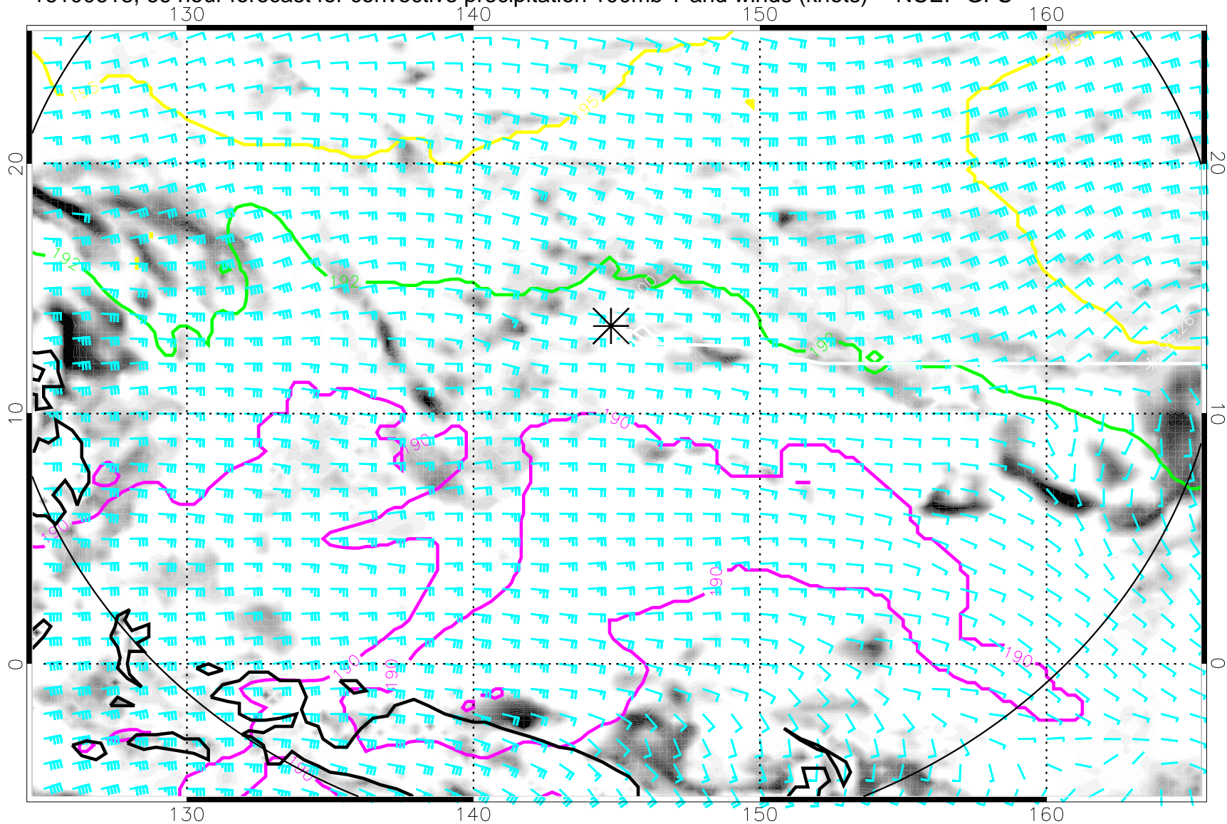
16100618, 66 hour forecast for convective precipitation 100mb T and winds (knots) -- NCEP GFS
