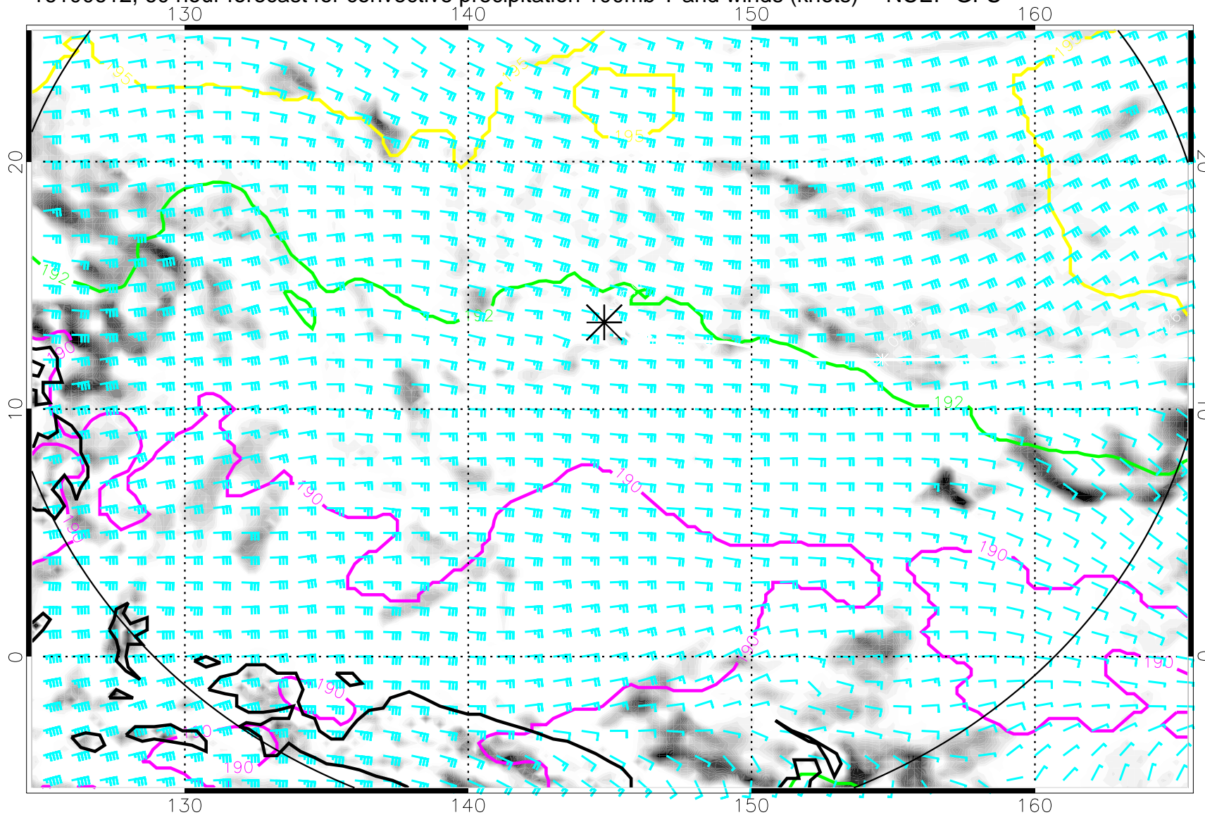
16100612, 60 hour forecast for convective precipitation 100mb T and winds (knots) -- NCEP GFS
