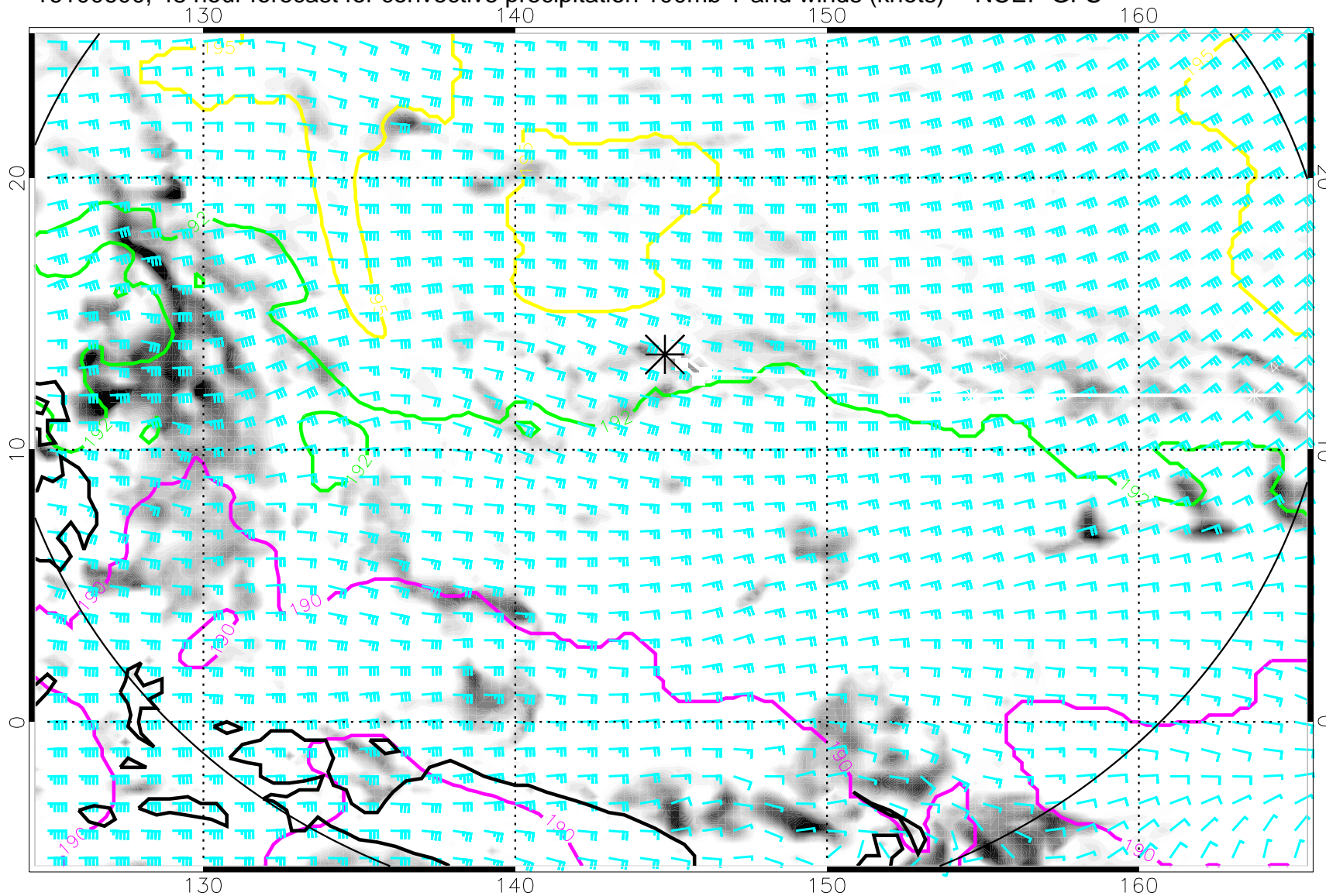
16100600, 48 hour forecast for convective precipitation 100mb T and winds (knots) -- NCEP GFS
