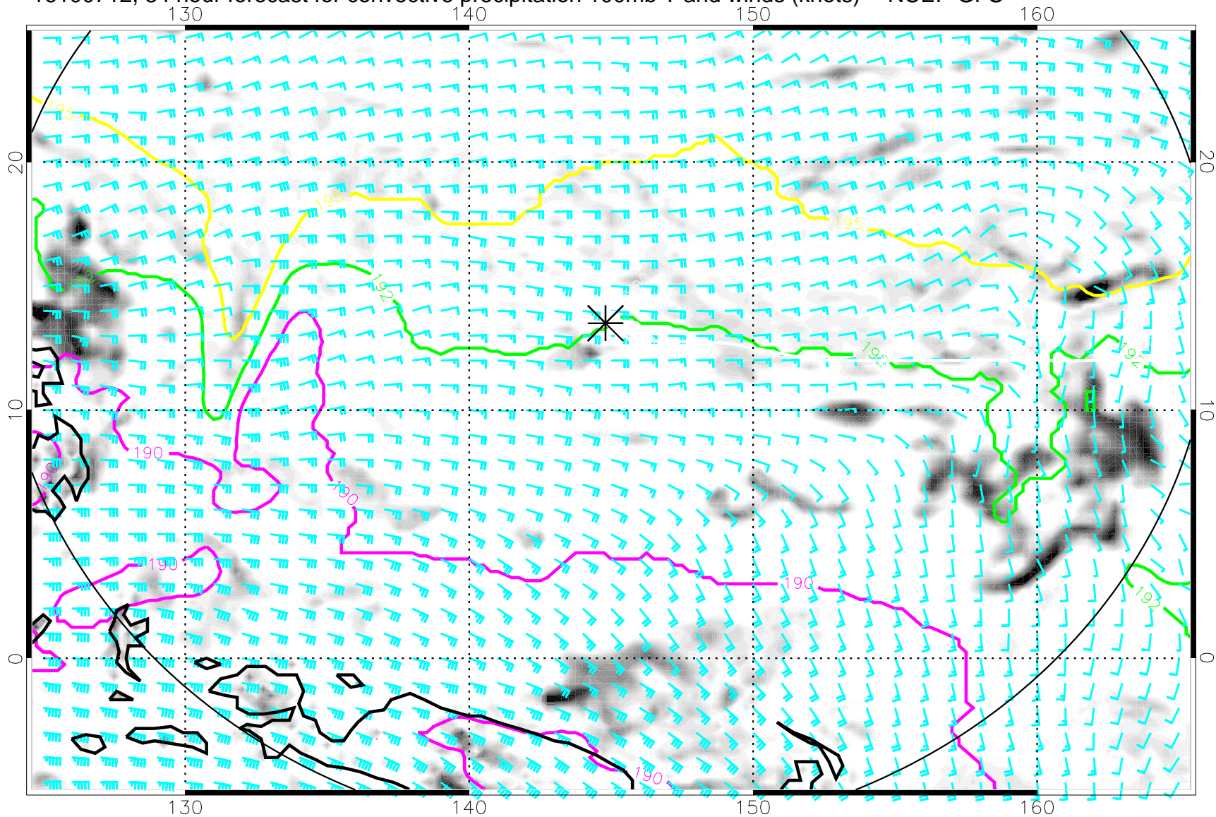
16100712, 84 hour forecast for convective precipitation 100mb T and winds (knots) -- NCEP GFS
