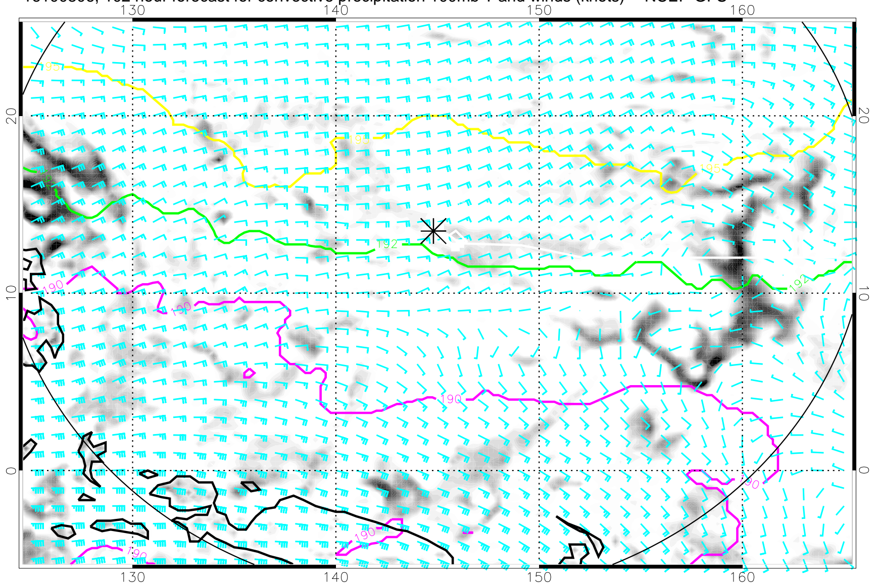
16100806, 102 hour forecast for convective precipitation 100mb T and winds (knots) -- NCEP GFS
