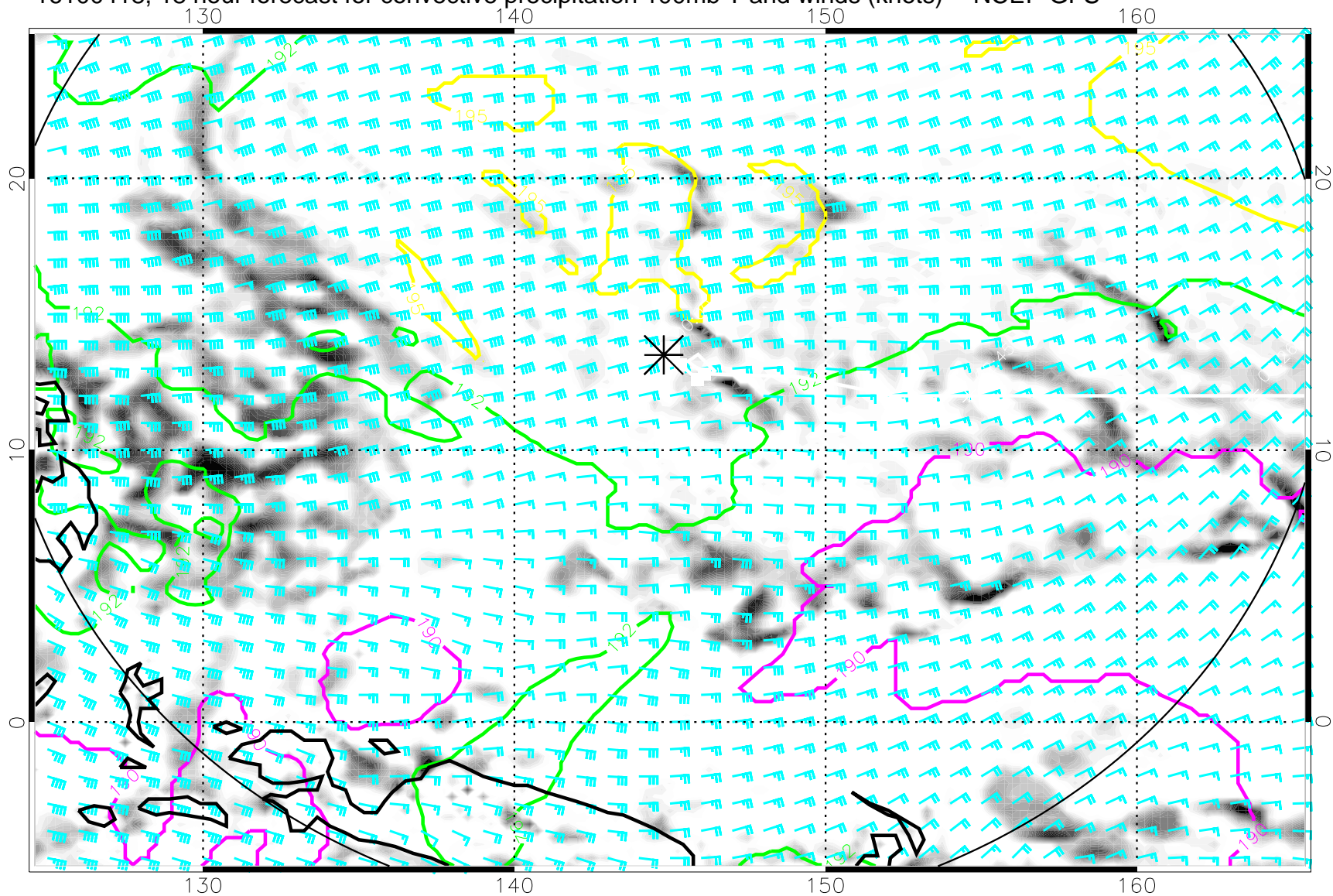
16100418, 18 hour forecast for convective precipitation 100mb T and winds (knots) -- NCEP GFS
