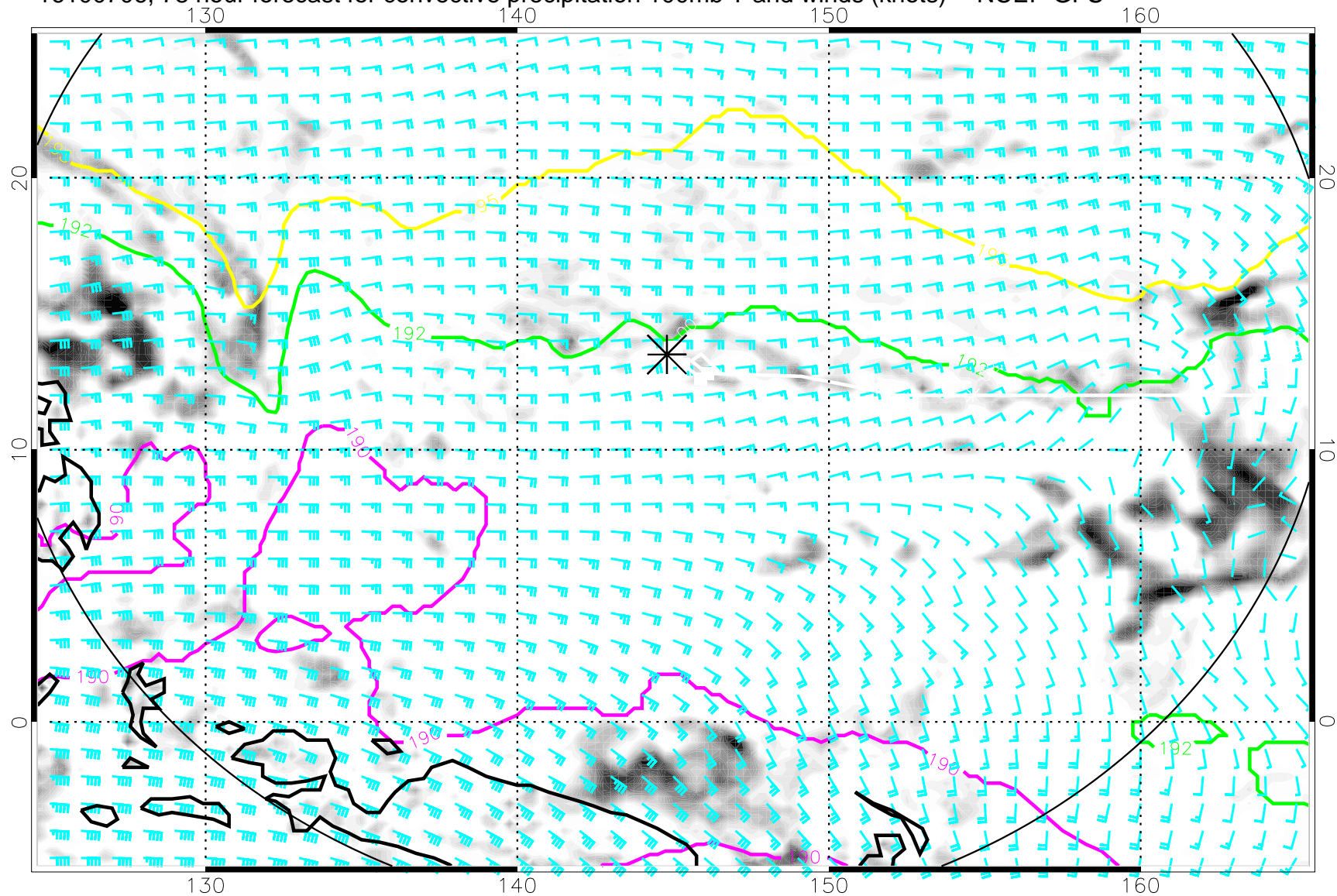
16100706, 78 hour forecast for convective precipitation 100mb T and winds (knots) -- NCEP GFS
