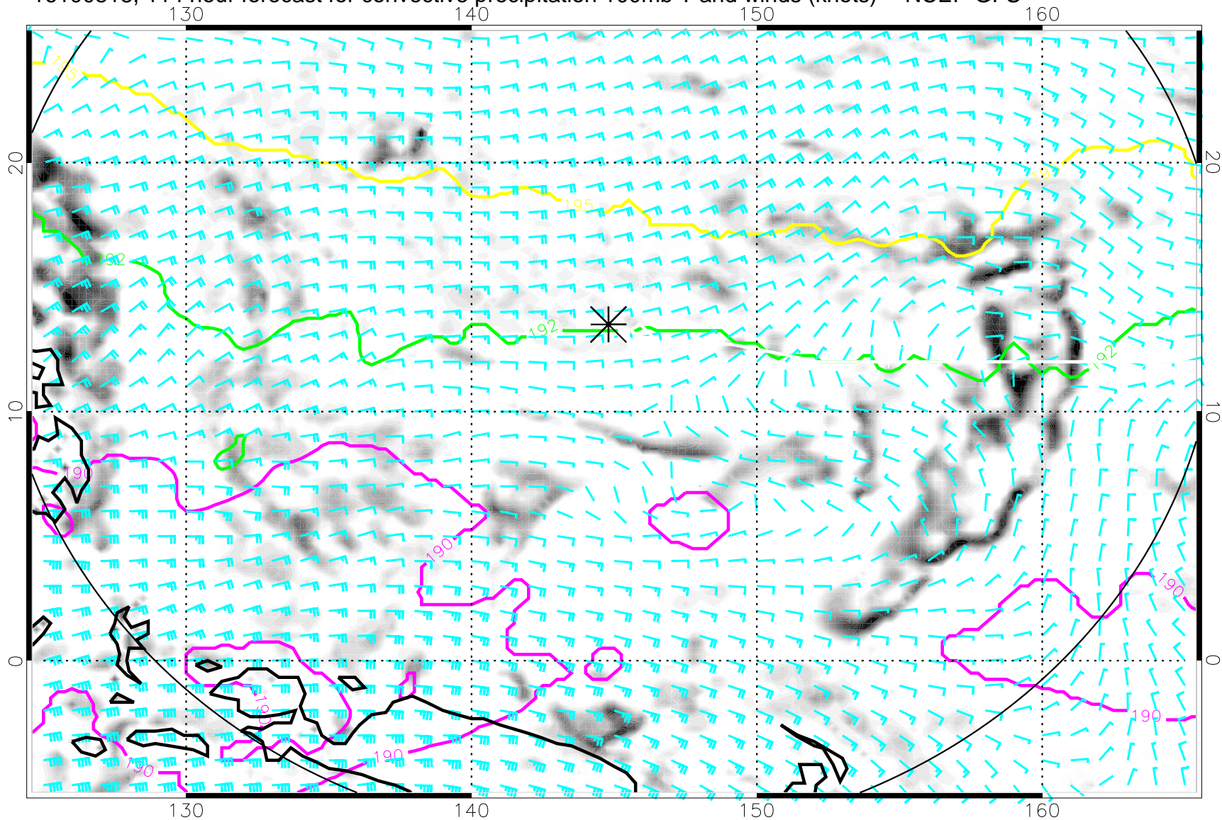
16100818, 114 hour forecast for convective precipitation 100mb T and winds (knots) -- NCEP GFS
