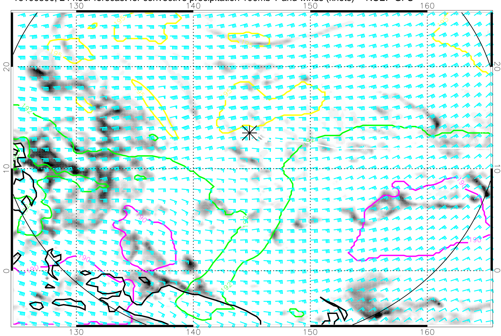
16100500, 24 hour forecast for convective precipitation 100mb T and winds (knots) -- NCEP GFS
