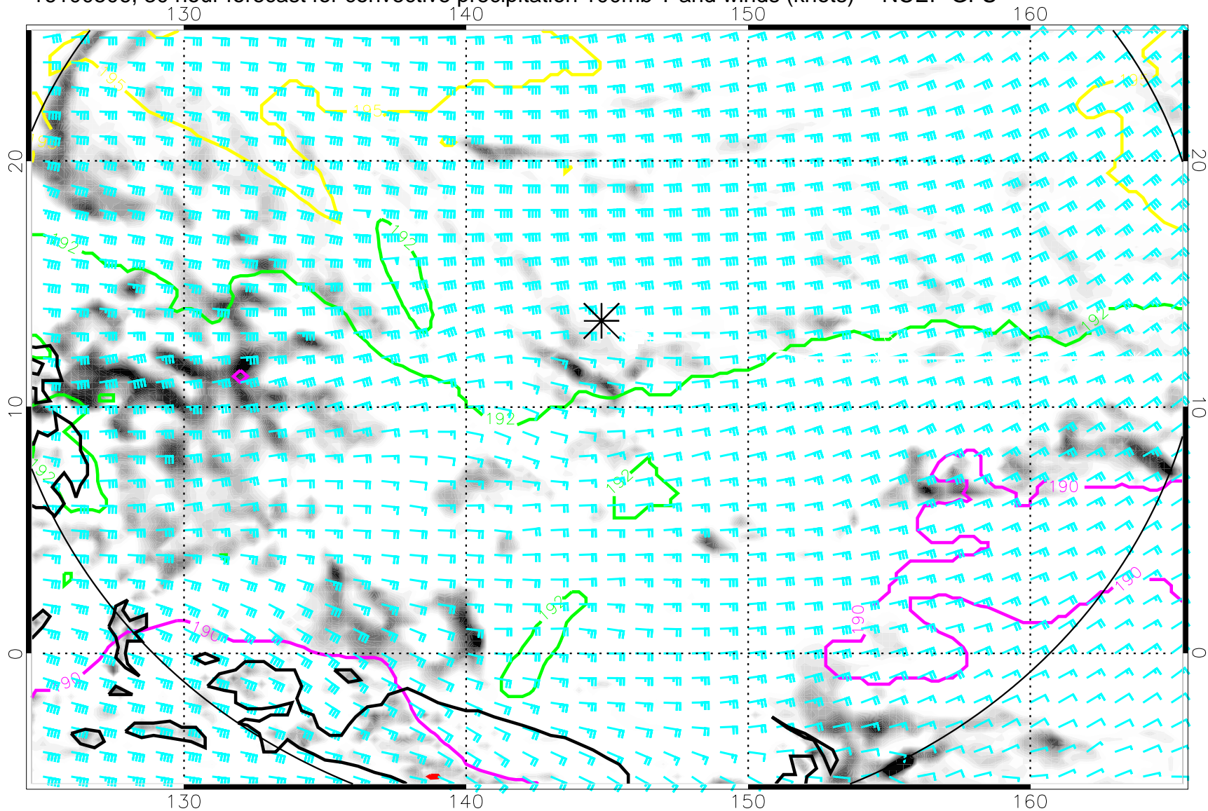
16100506, 30 hour forecast for convective precipitation 100mb T and winds (knots) -- NCEP GFS
