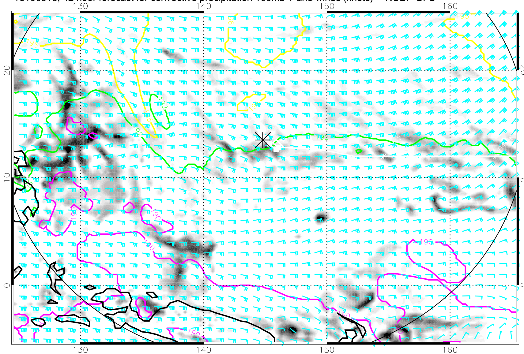
16100518, 42 hour forecast for convective precipitation 100mb T and winds (knots) -- NCEP GFS
