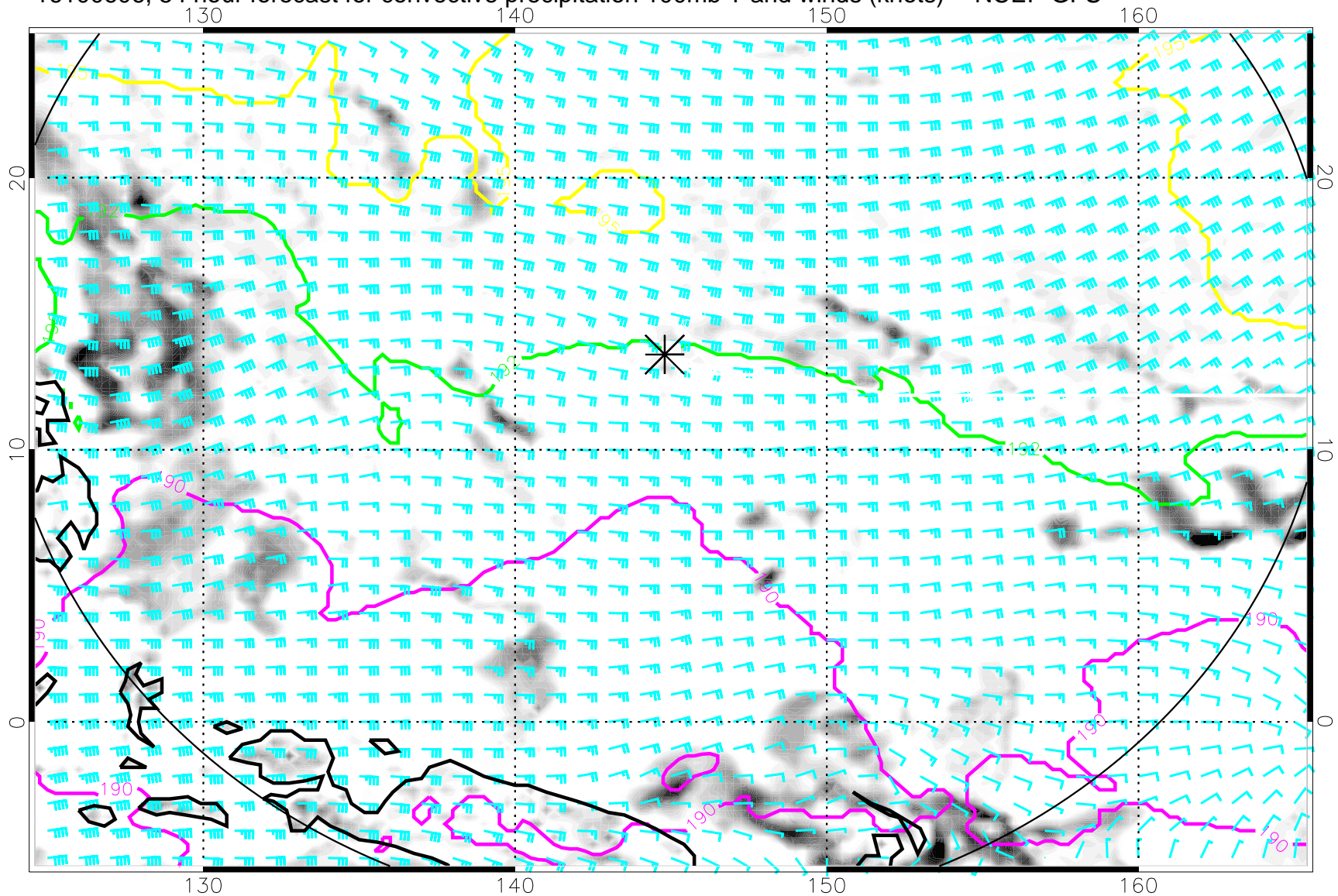
16100606, 54 hour forecast for convective precipitation 100mb T and winds (knots) -- NCEP GFS
