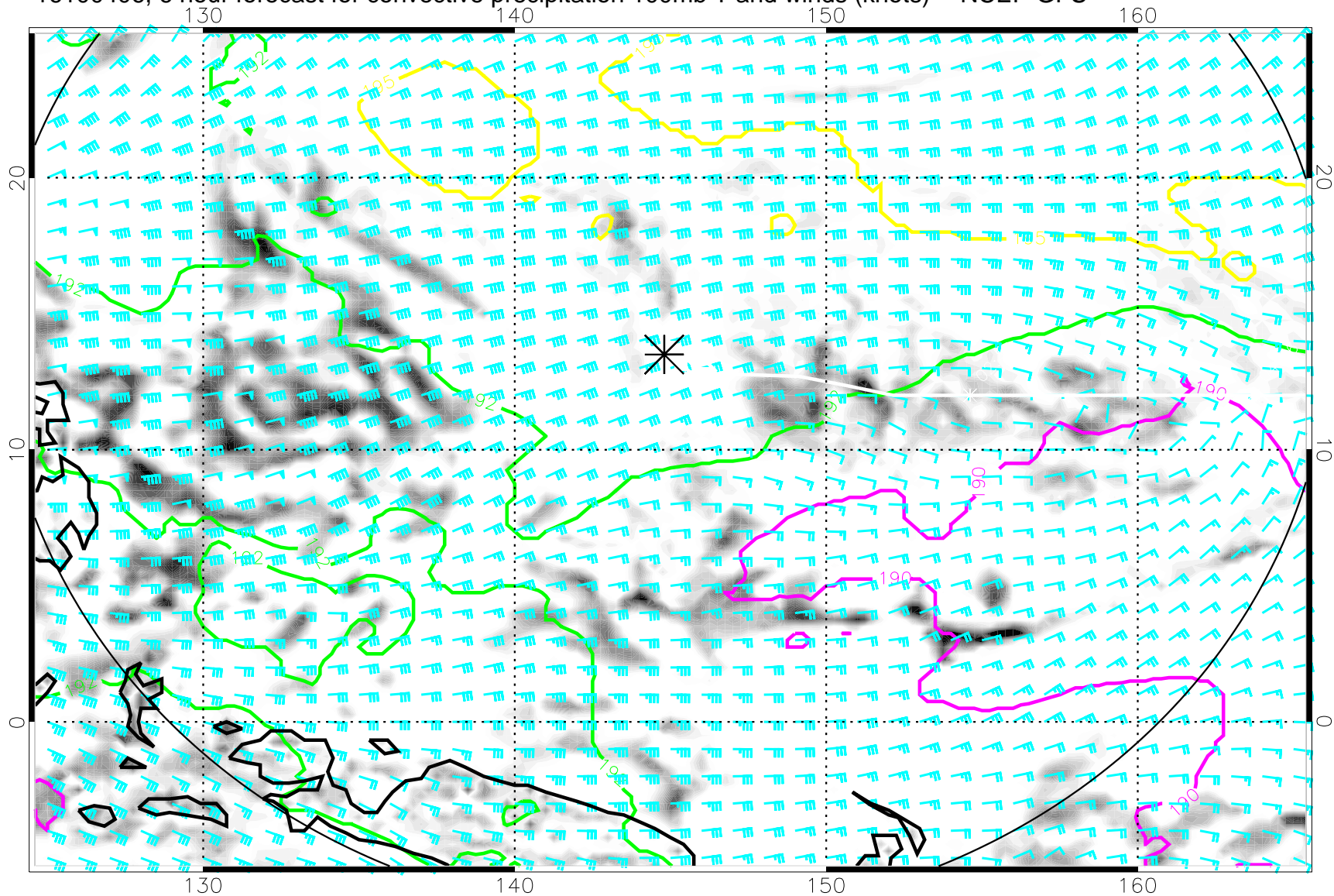
16100406, 6 hour forecast for convective precipitation 100mb T and winds (knots) -- NCEP GFS
