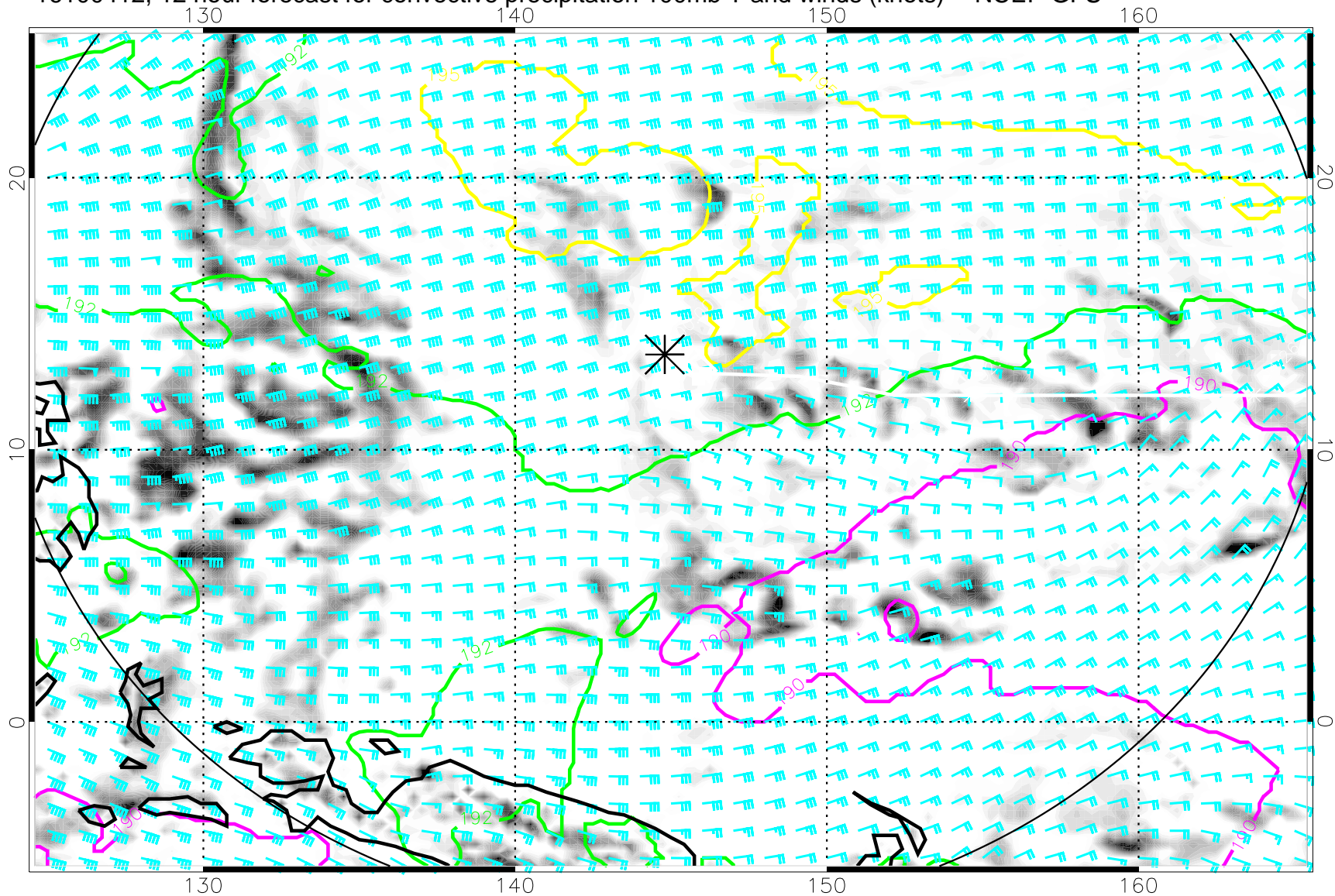
16100412, 12 hour forecast for convective precipitation 100mb T and winds (knots) -- NCEP GFS
