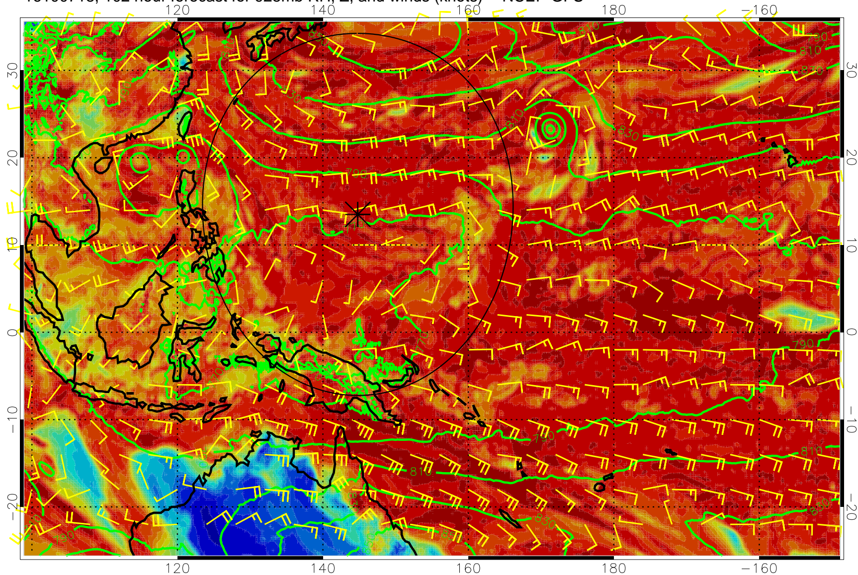
16100718, 102 hour forecast for 925mb RH, Z, and winds (knots) -- NCEP GFS
