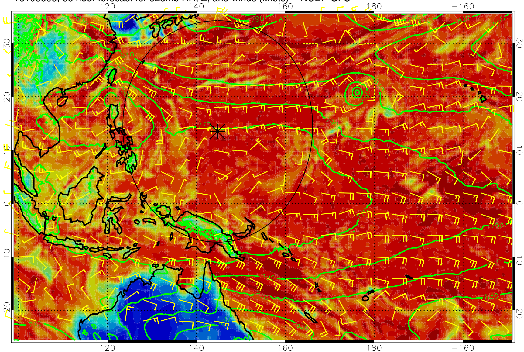
16100606, 66 hour forecast for 925mb RH, Z, and winds (knots) -- NCEP GFS
