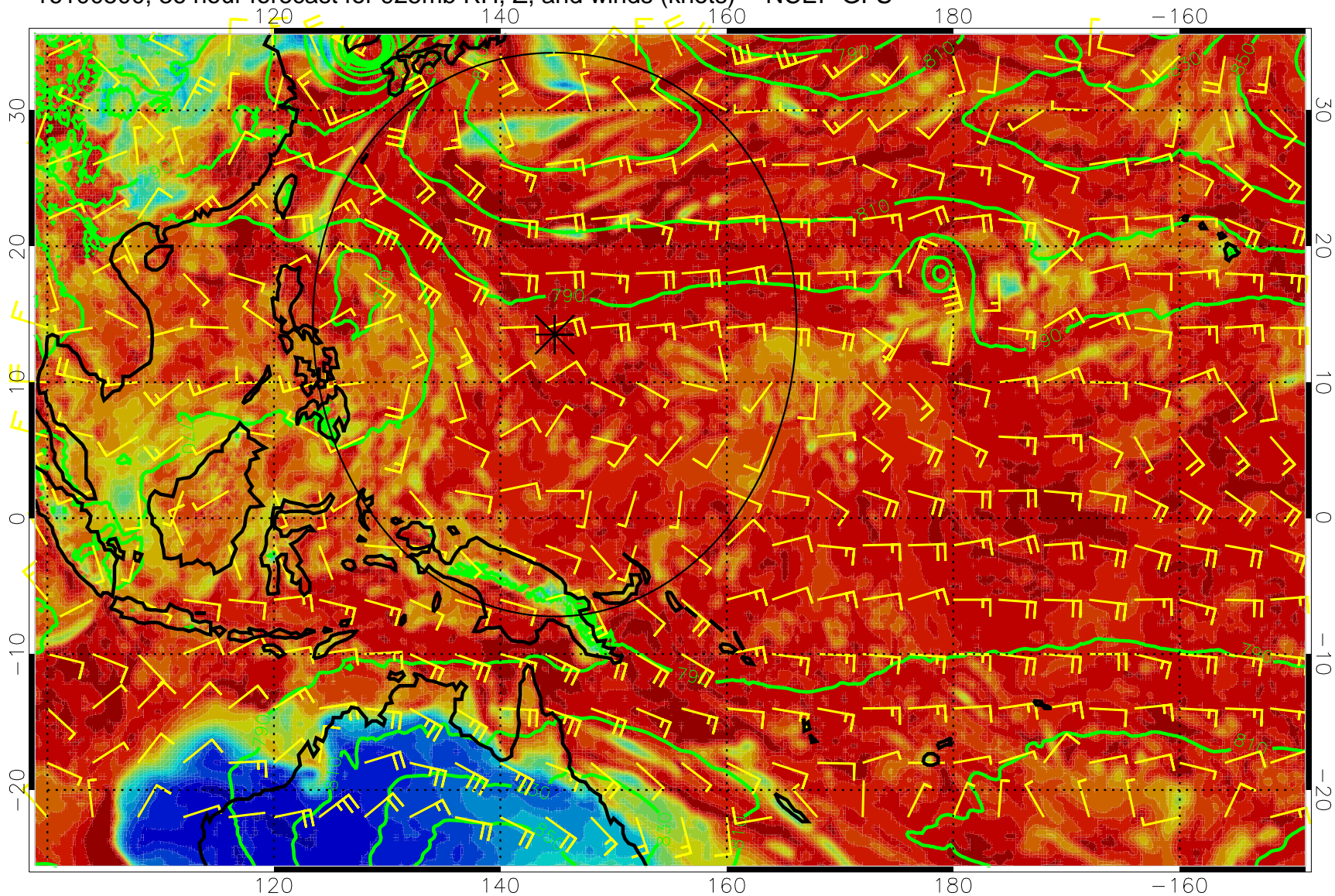
16100500, 36 hour forecast for 925mb RH, Z, and winds (knots) -- NCEP GFS
