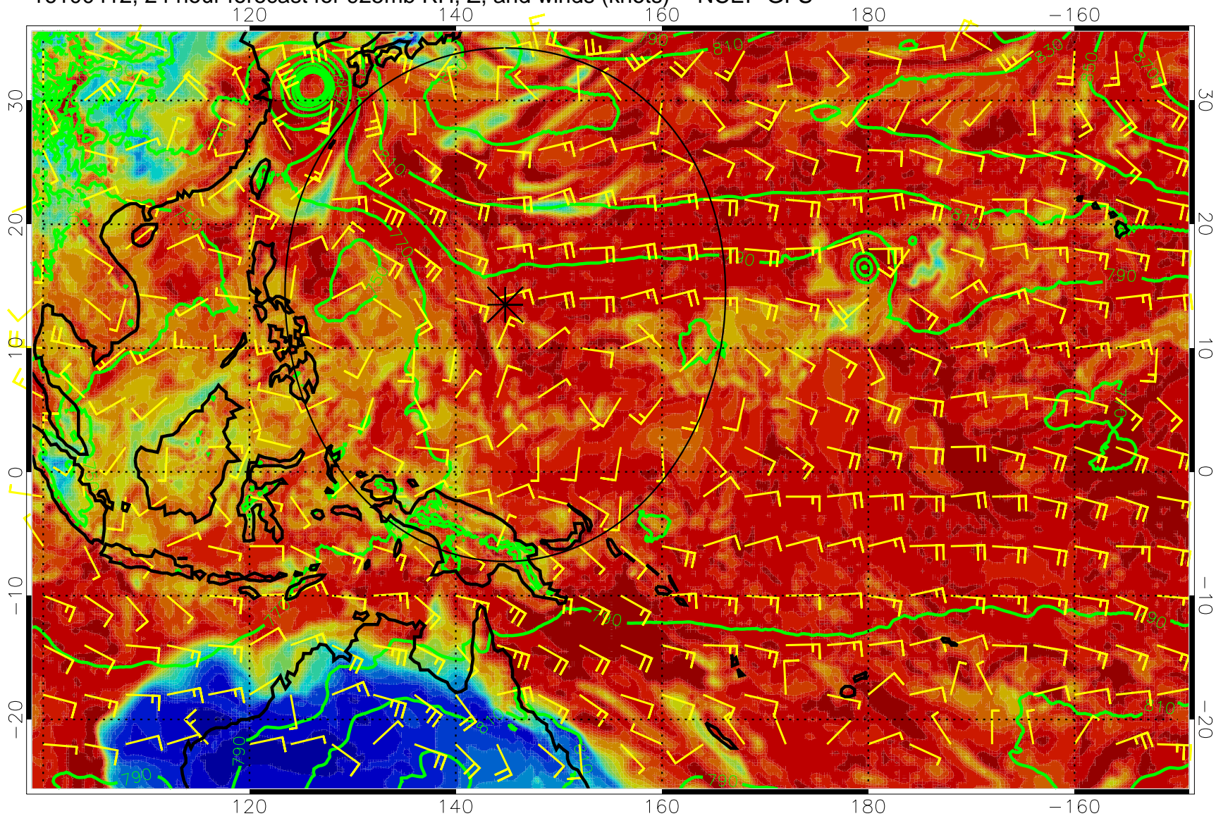
16100412, 24 hour forecast for 925mb RH, Z, and winds (knots) -- NCEP GFS
