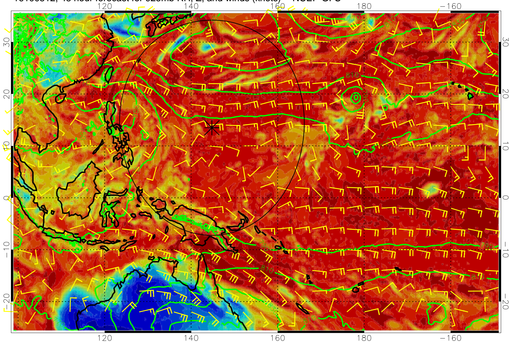
16100512, 48 hour forecast for 925mb RH, Z, and winds (knots) -- NCEP GFS
