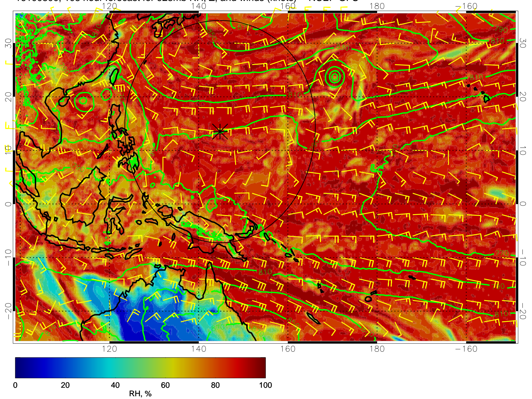
16100800, 108 hour forecast for 925mb RH, Z, and winds (knots) -- NCEP GFS
