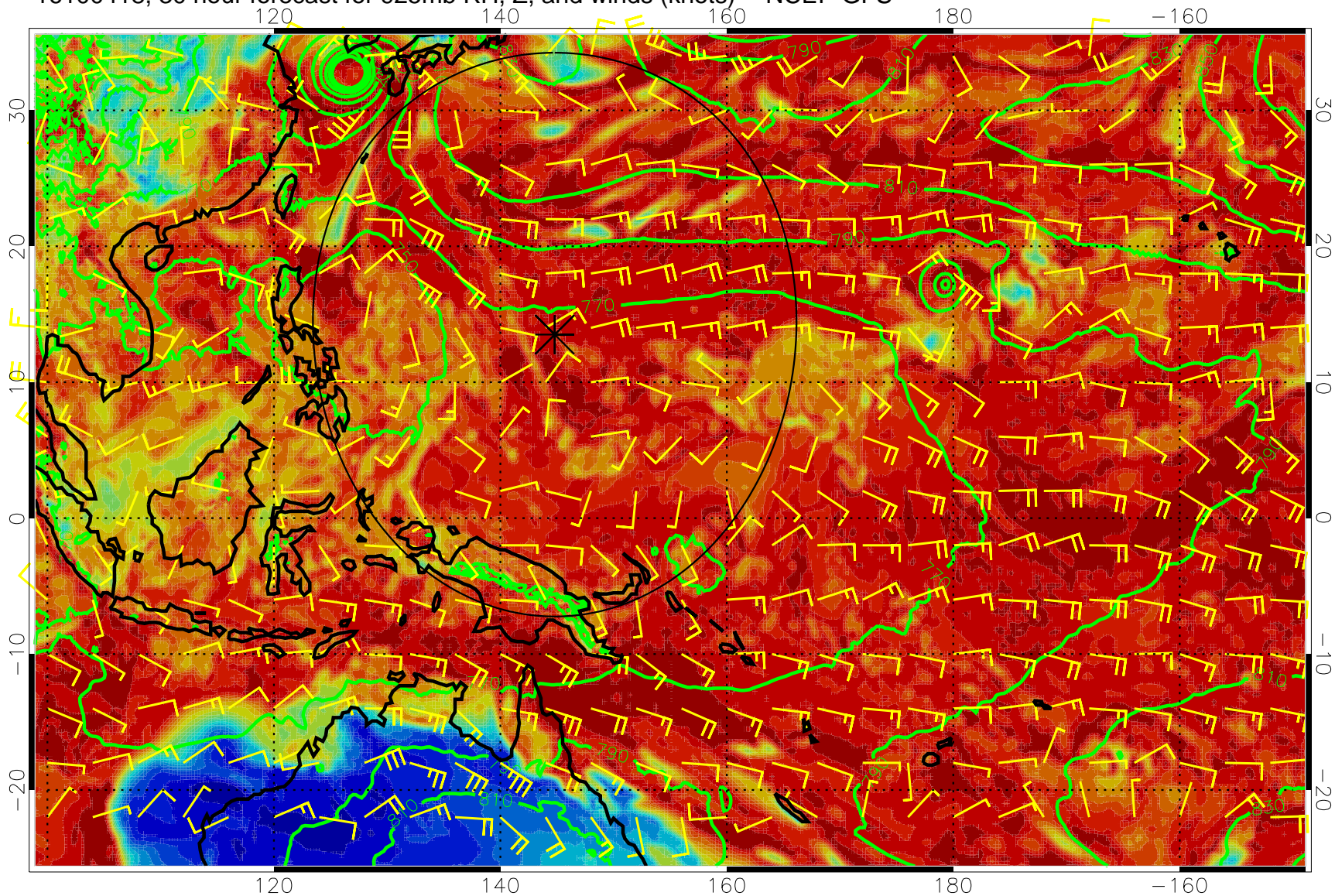
16100418, 30 hour forecast for 925mb RH, Z, and winds (knots) -- NCEP GFS
