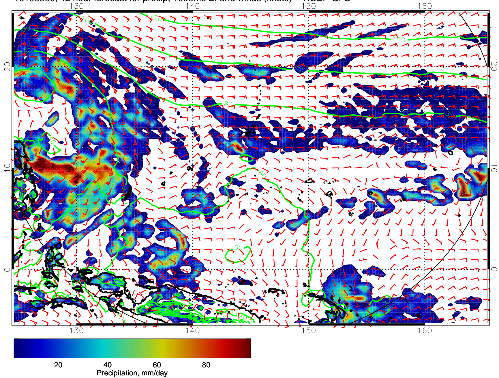
16100506, 42 hour forecast for precip, 1000mb Z, and winds (knots) -- NCEP GFS
