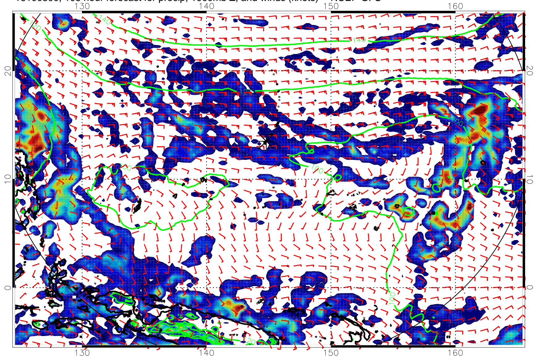
16100800, 108 hour forecast for precip, 1000mb Z, and winds (knots) -- NCEP GFS
