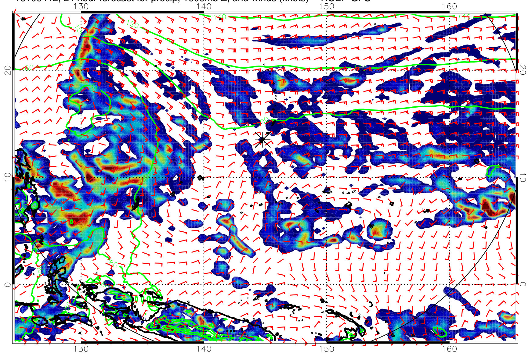
16100412, 24 hour forecast for precip, 1000mb Z, and winds (knots) -- NCEP GFS
