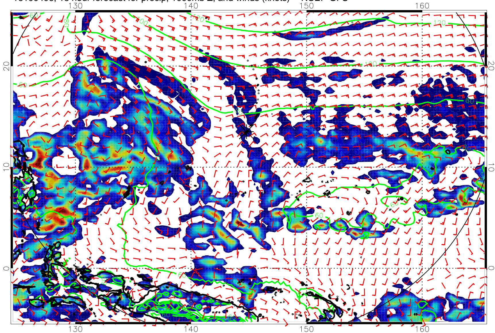
16100406, 18 hour forecast for precip, 1000mb Z, and winds (knots) -- NCEP GFS
