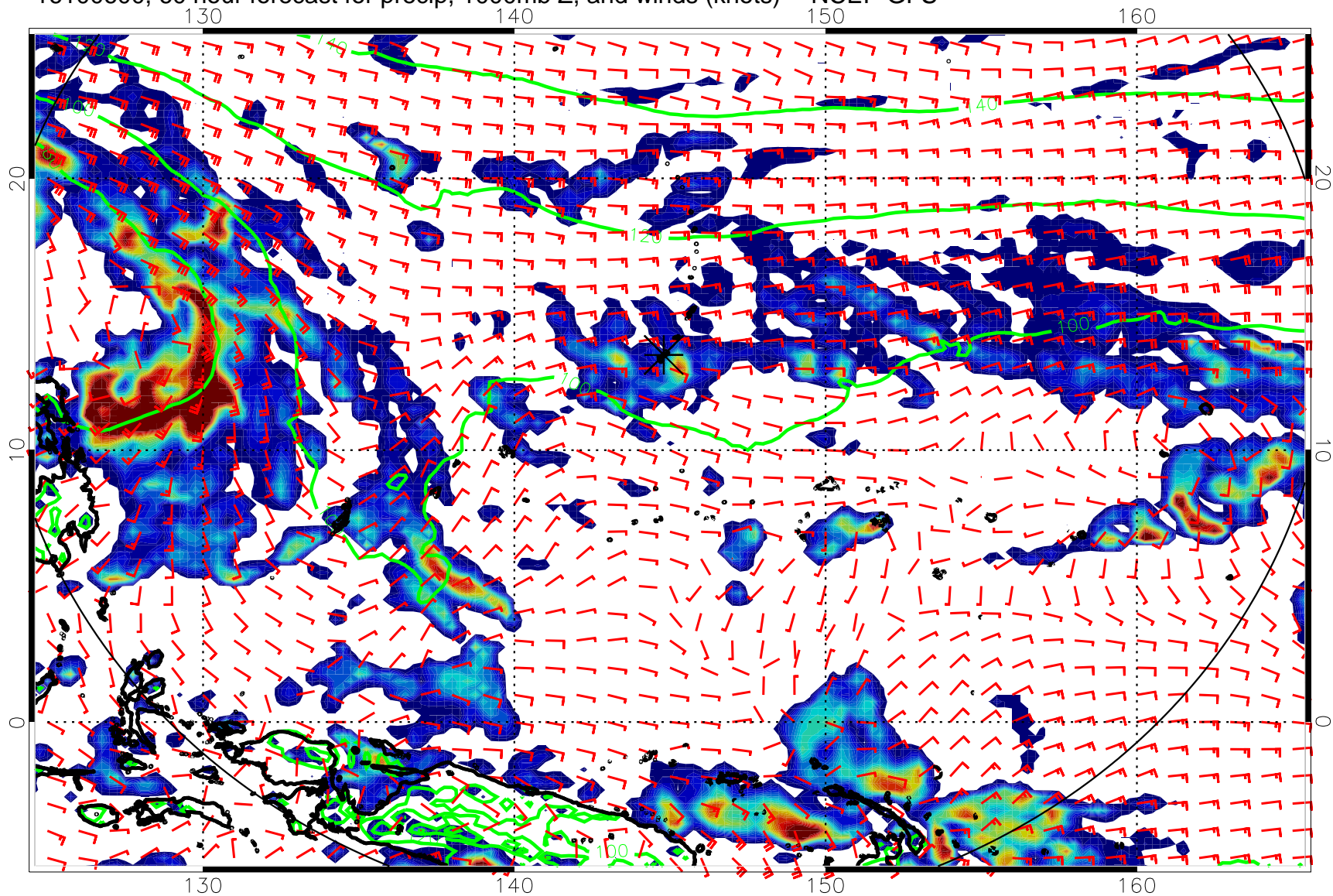
16100600, 60 hour forecast for precip, 1000mb Z, and winds (knots) -- NCEP GFS
