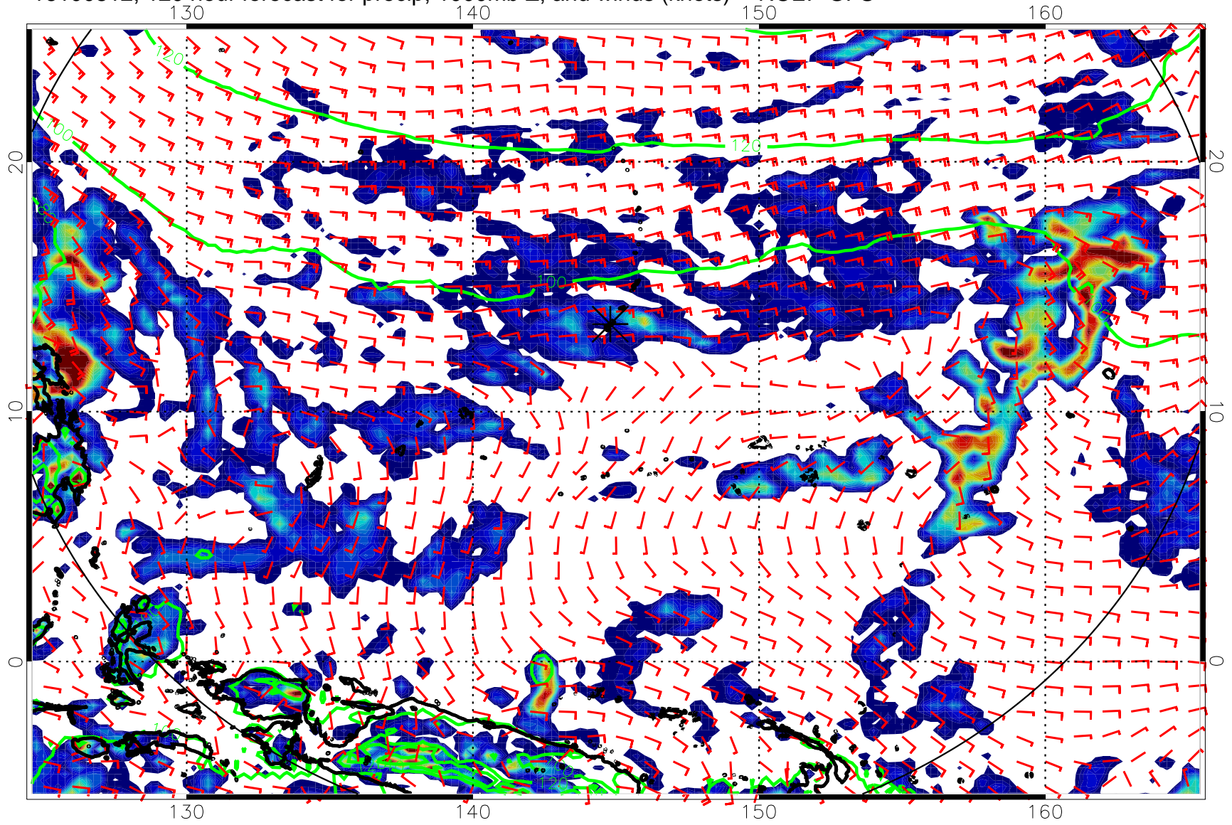
16100812, 120 hour forecast for precip, 1000mb Z, and winds (knots) -- NCEP GFS
