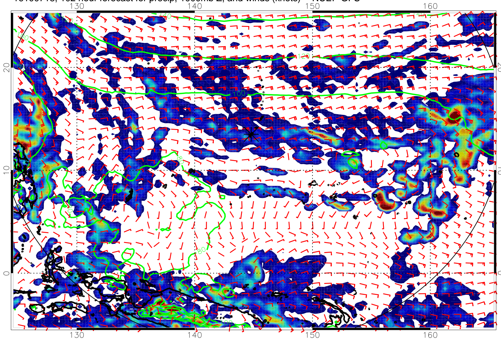
16100718, 102 hour forecast for precip, 1000mb Z, and winds (knots) -- NCEP GFS
