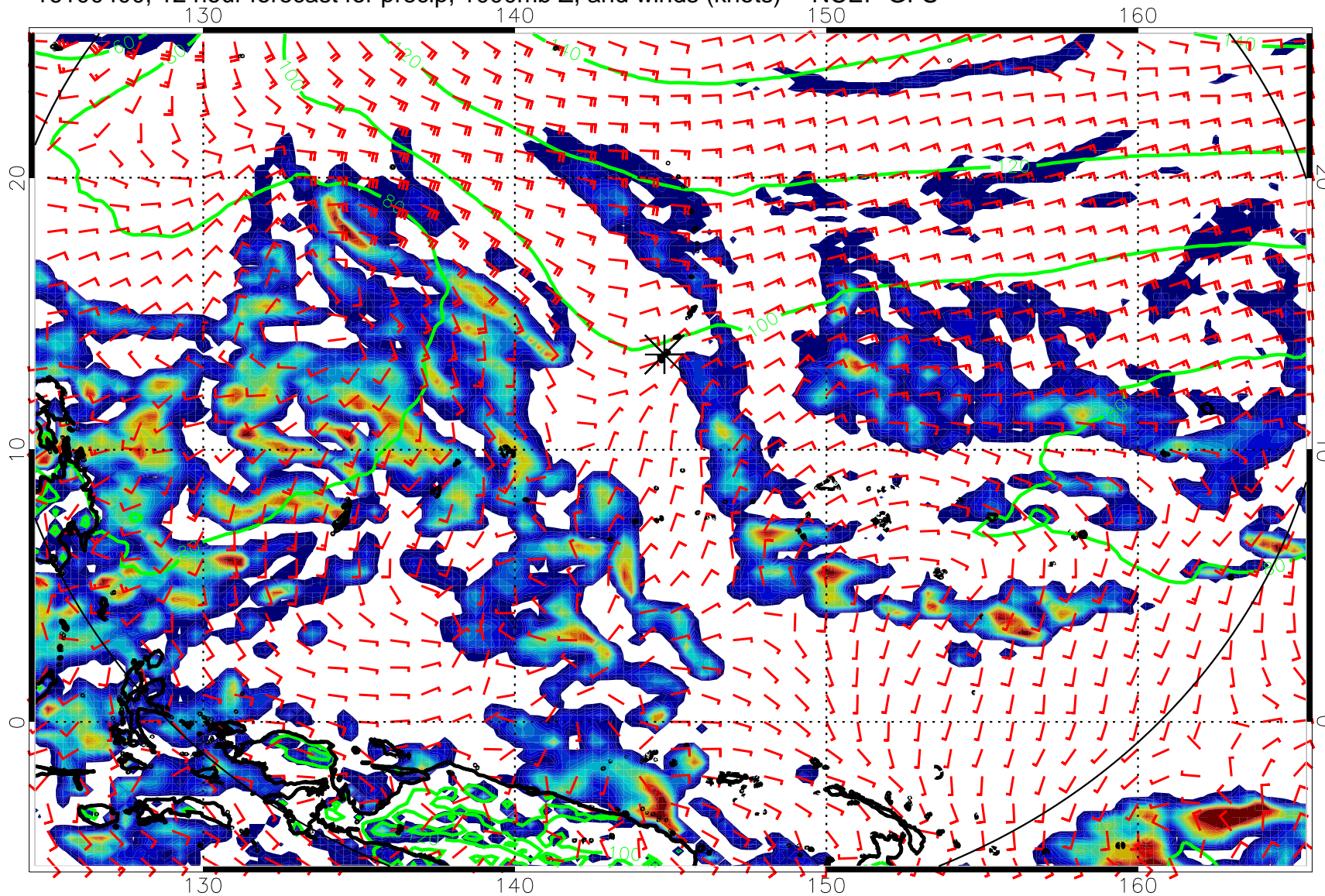
16100400, 12 hour forecast for precip, 1000mb Z, and winds (knots) -- NCEP GFS
