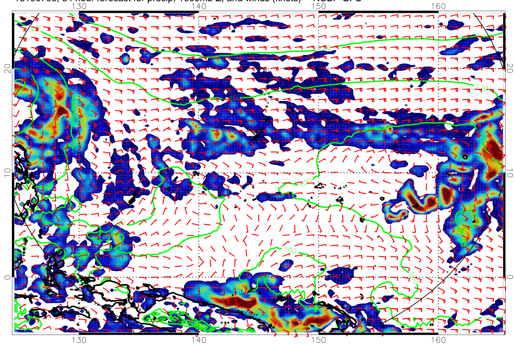
16100700, 84 hour forecast for precip, 1000mb Z, and winds (knots) -- NCEP GFS
