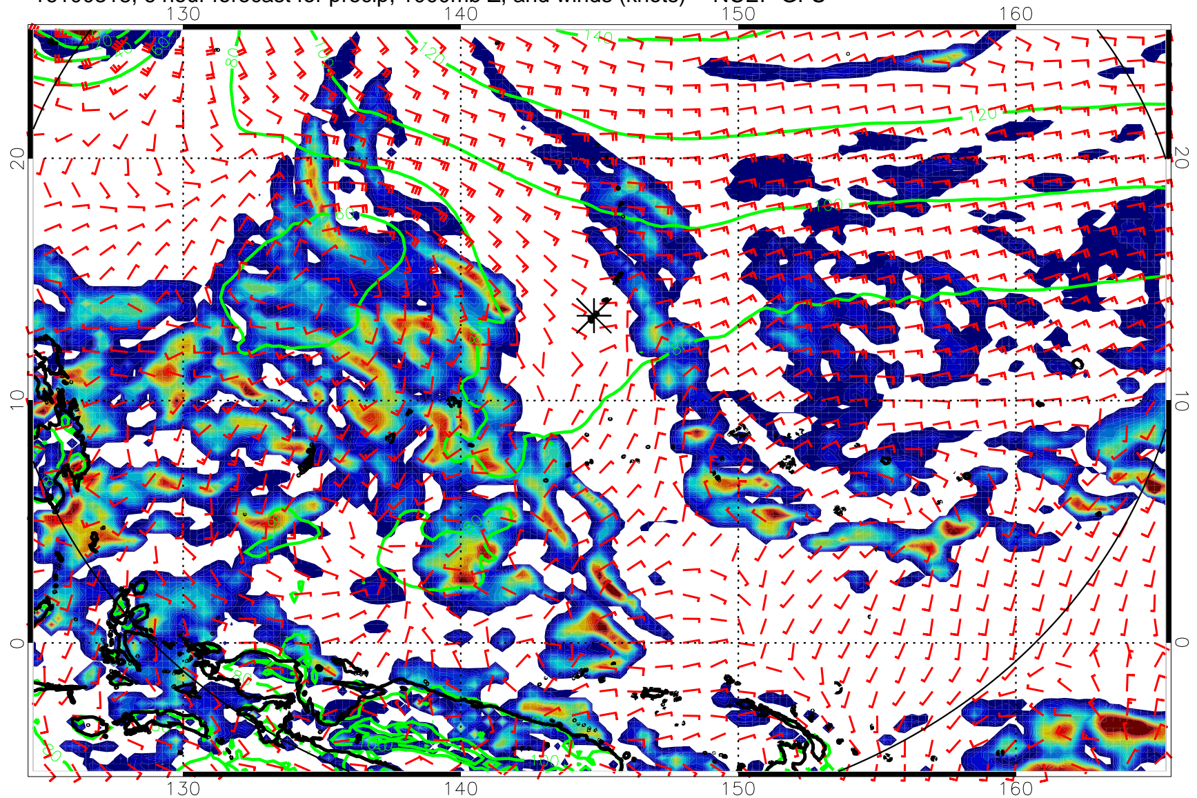
16100318, 6 hour forecast for precip, 1000mb Z, and winds (knots) -- NCEP GFS
