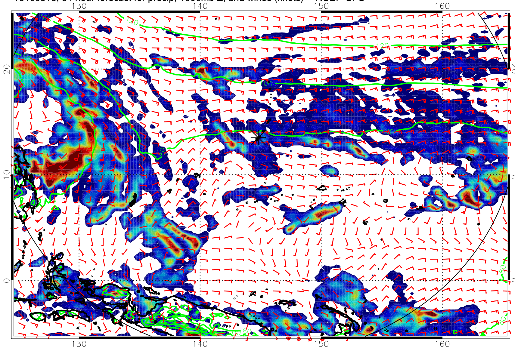
16100518, 54 hour forecast for precip, 1000mb Z, and winds (knots) -- NCEP GFS
