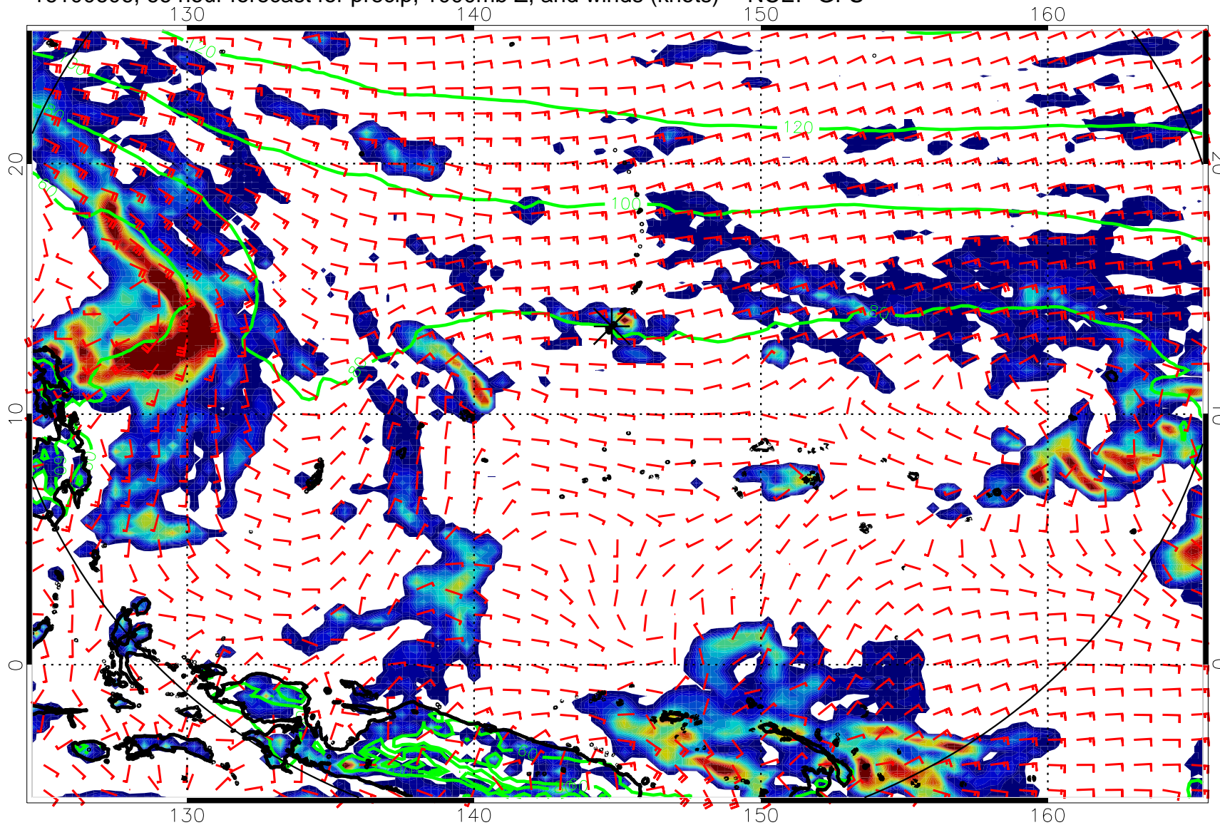
16100606, 66 hour forecast for precip, 1000mb Z, and winds (knots) -- NCEP GFS
