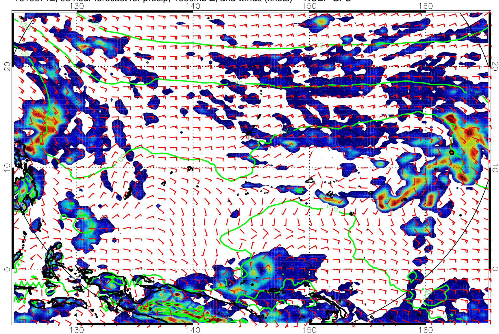
16100712, 96 hour forecast for precip, 1000mb Z, and winds (knots) -- NCEP GFS
