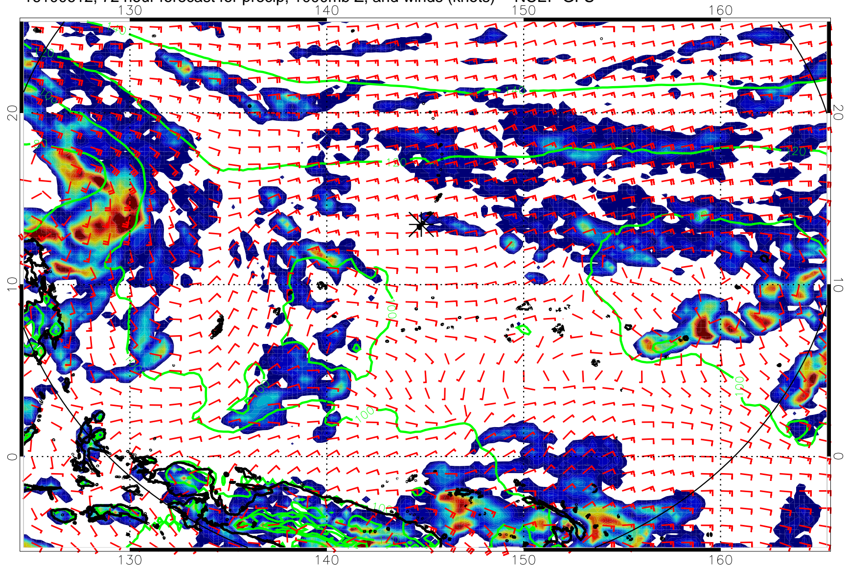
16100612, 72 hour forecast for precip, 1000mb Z, and winds (knots) -- NCEP GFS
