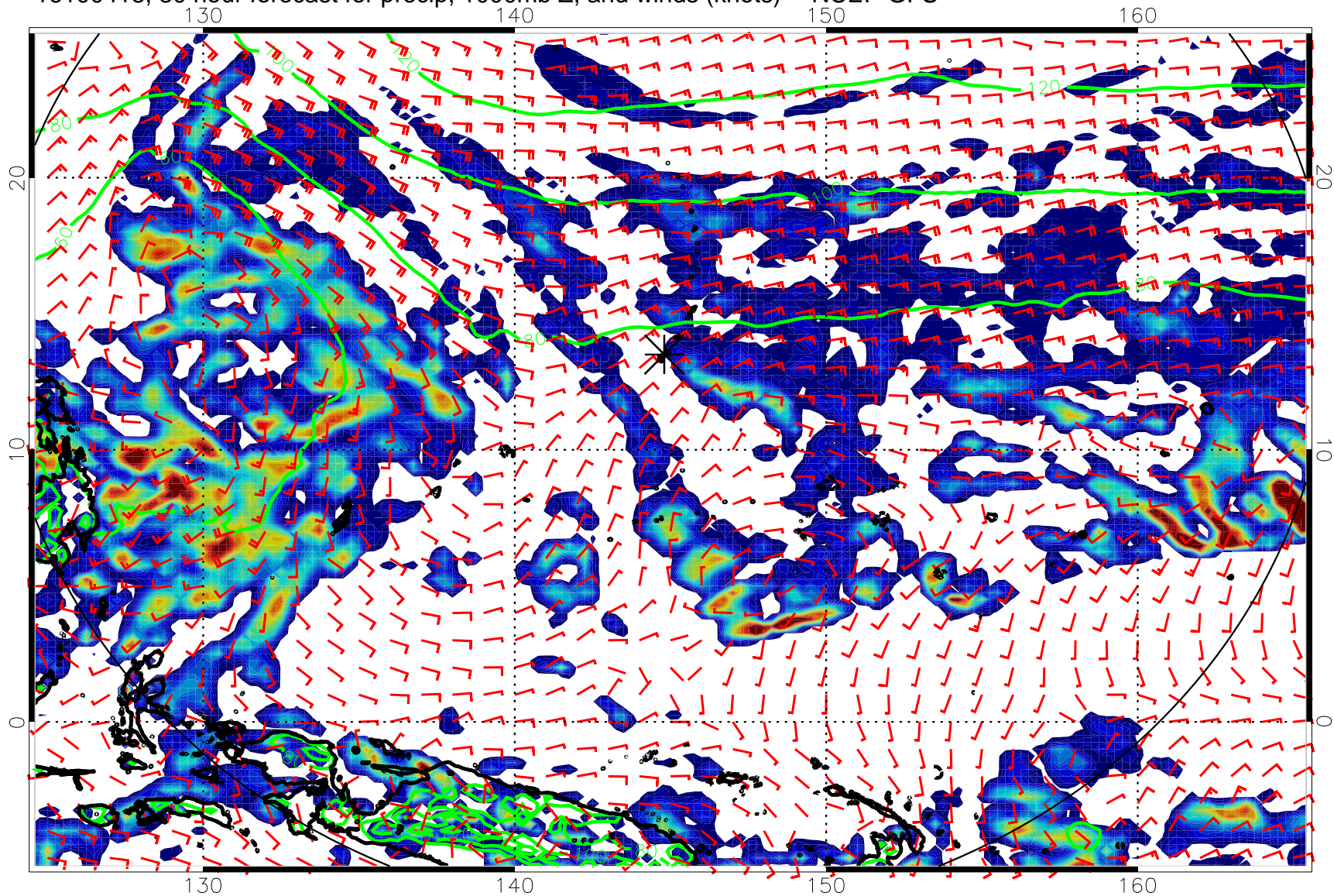
16100418, 30 hour forecast for precip, 1000mb Z, and winds (knots) -- NCEP GFS
