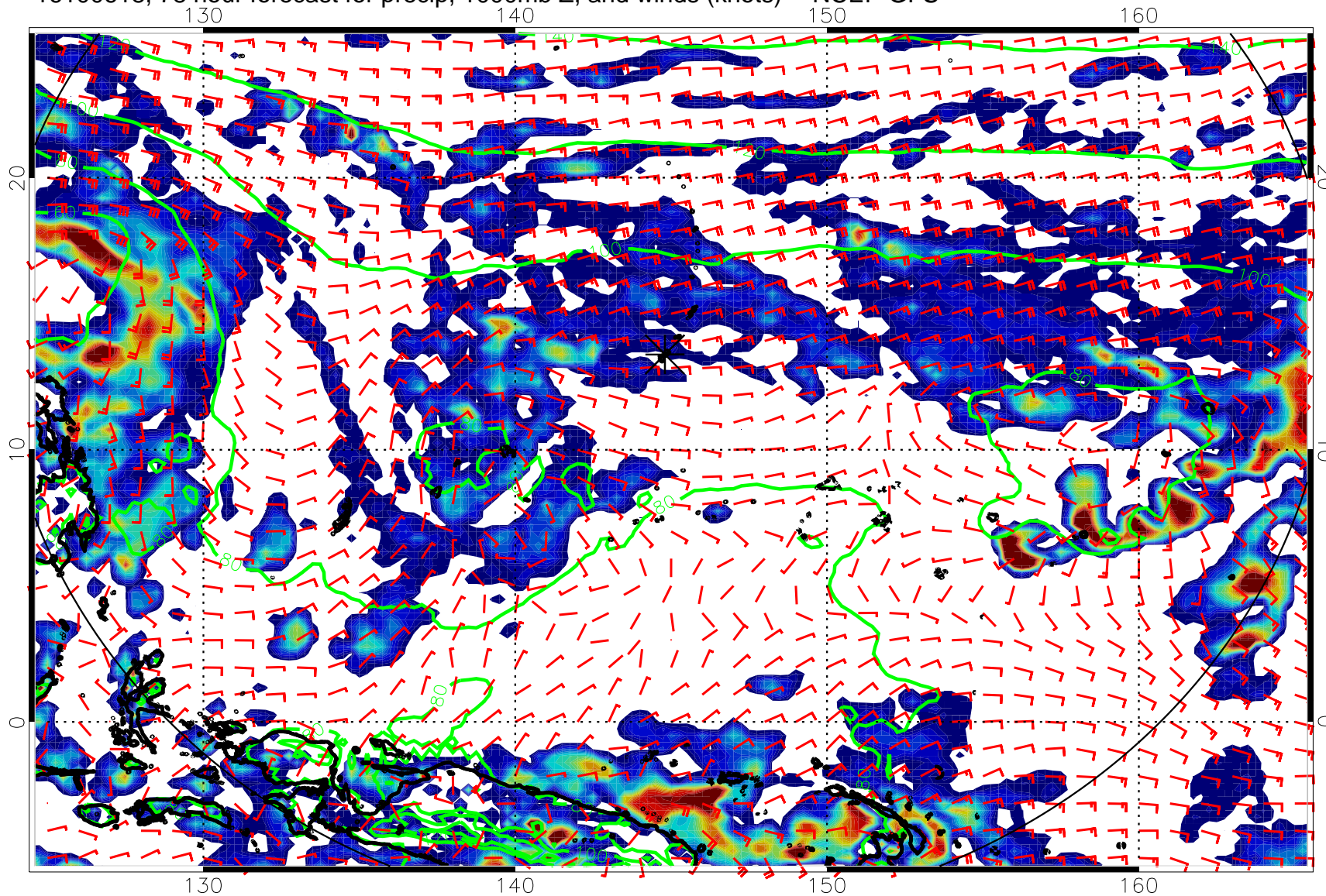
16100618, 78 hour forecast for precip, 1000mb Z, and winds (knots) -- NCEP GFS
