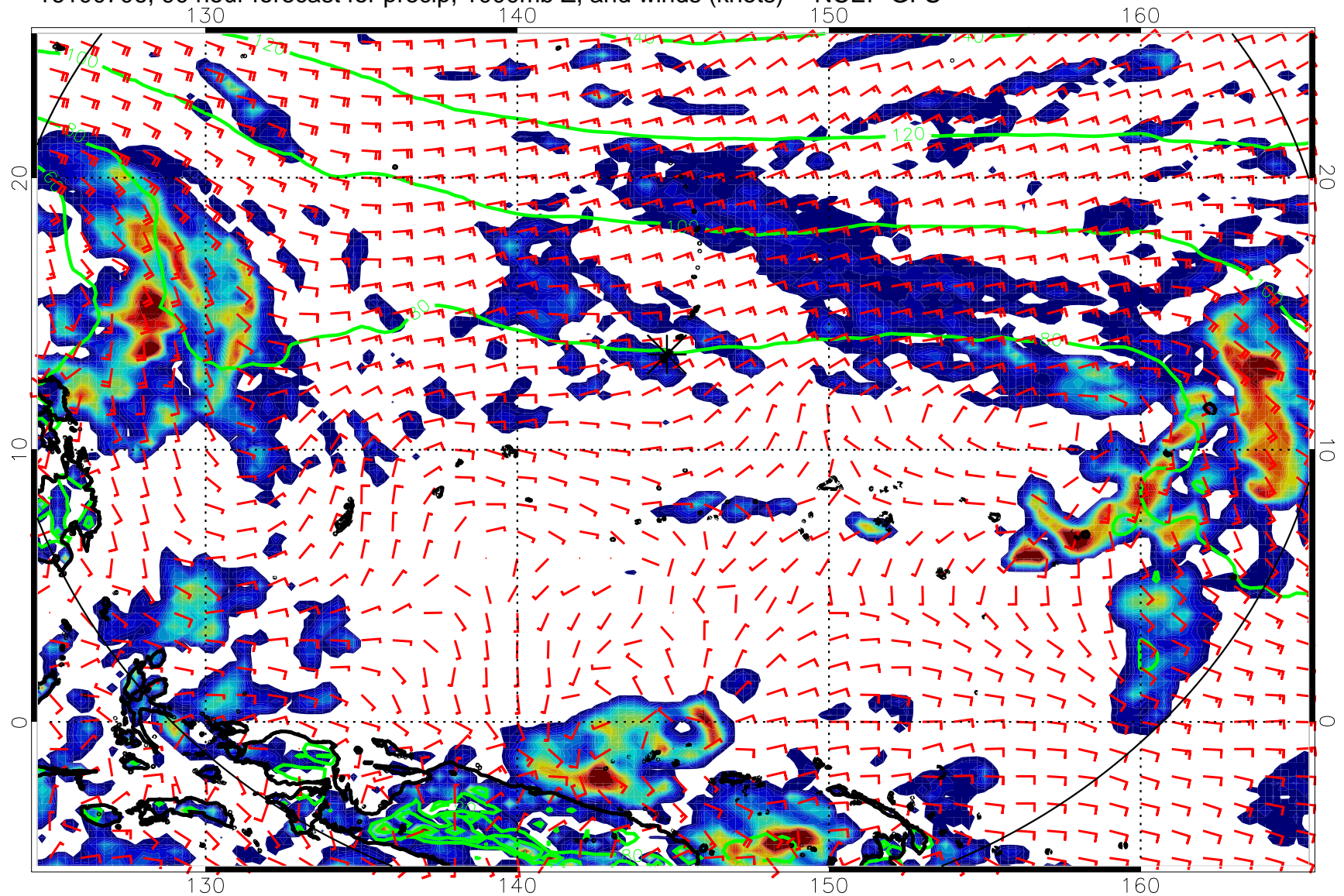
16100706, 90 hour forecast for precip, 1000mb Z, and winds (knots) -- NCEP GFS
