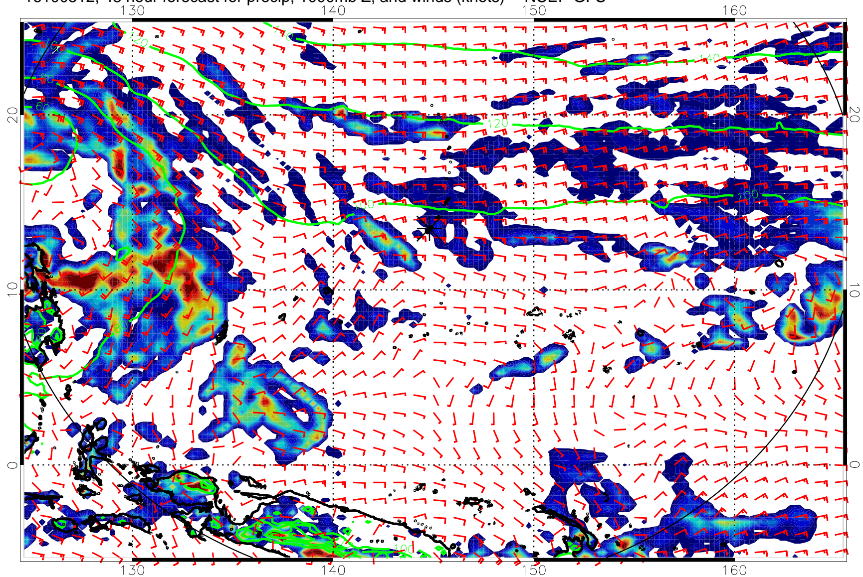
16100512, 48 hour forecast for precip, 1000mb Z, and winds (knots) -- NCEP GFS
