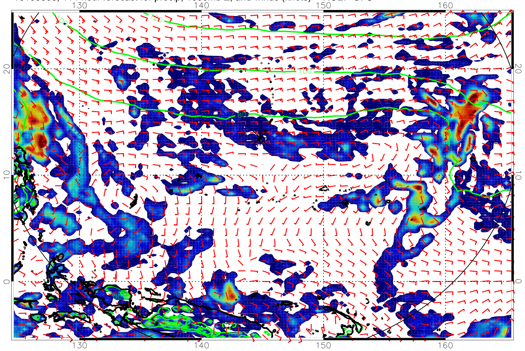
16100806, 114 hour forecast for precip, 1000mb Z, and winds (knots) -- NCEP GFS
