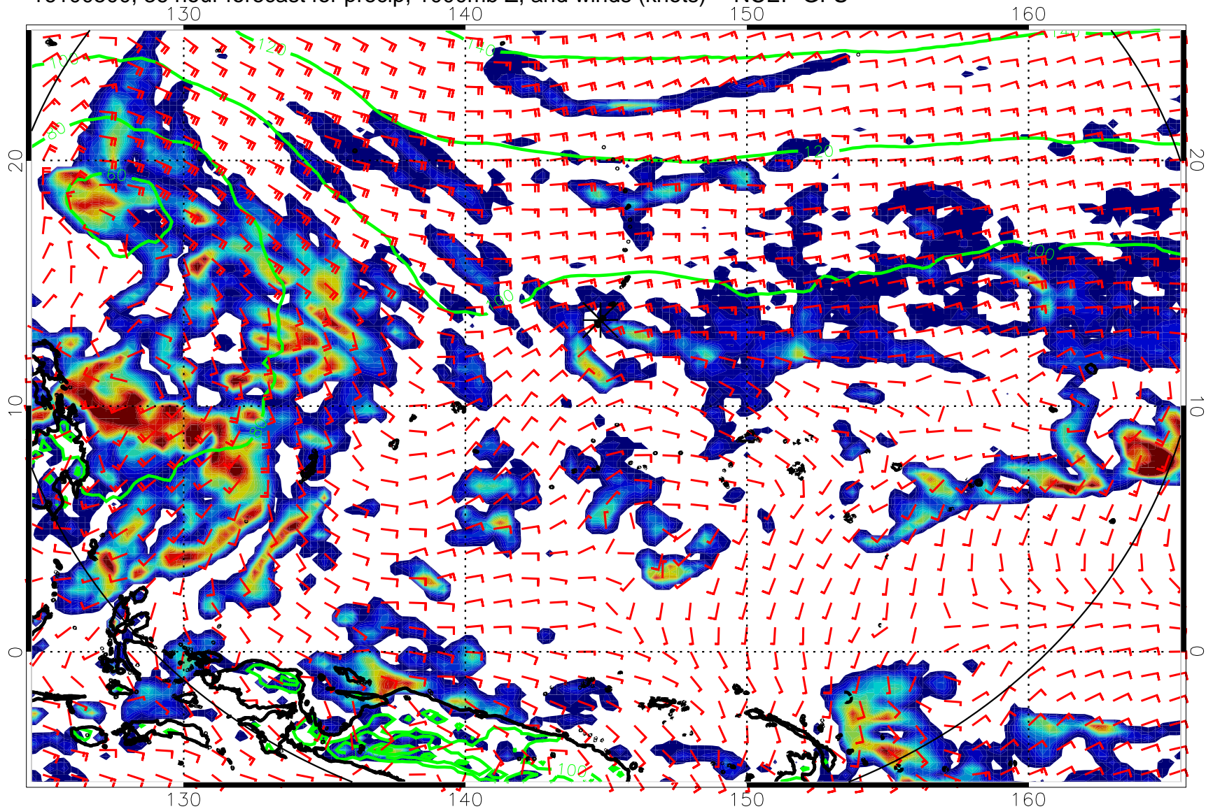
16100500, 36 hour forecast for precip, 1000mb Z, and winds (knots) -- NCEP GFS
