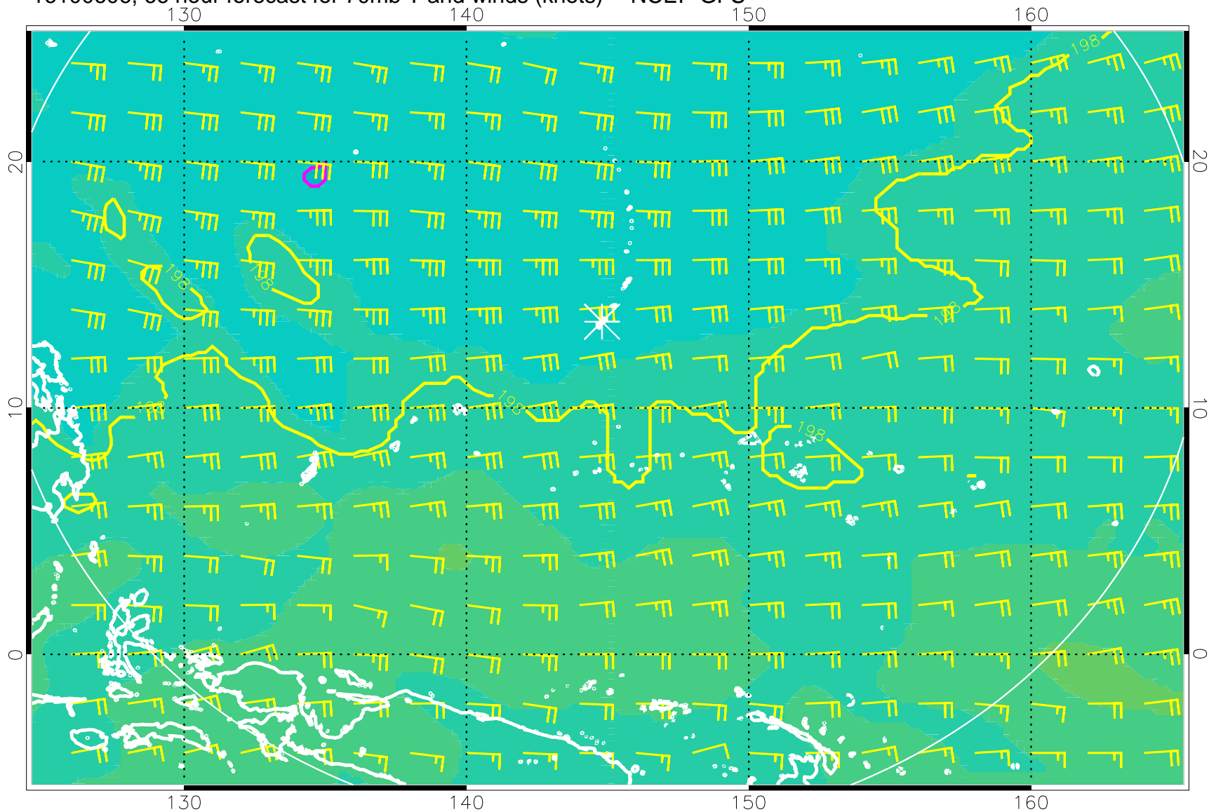
16100606, 66 hour forecast for 70mb T and winds (knots) -- NCEP GFS
