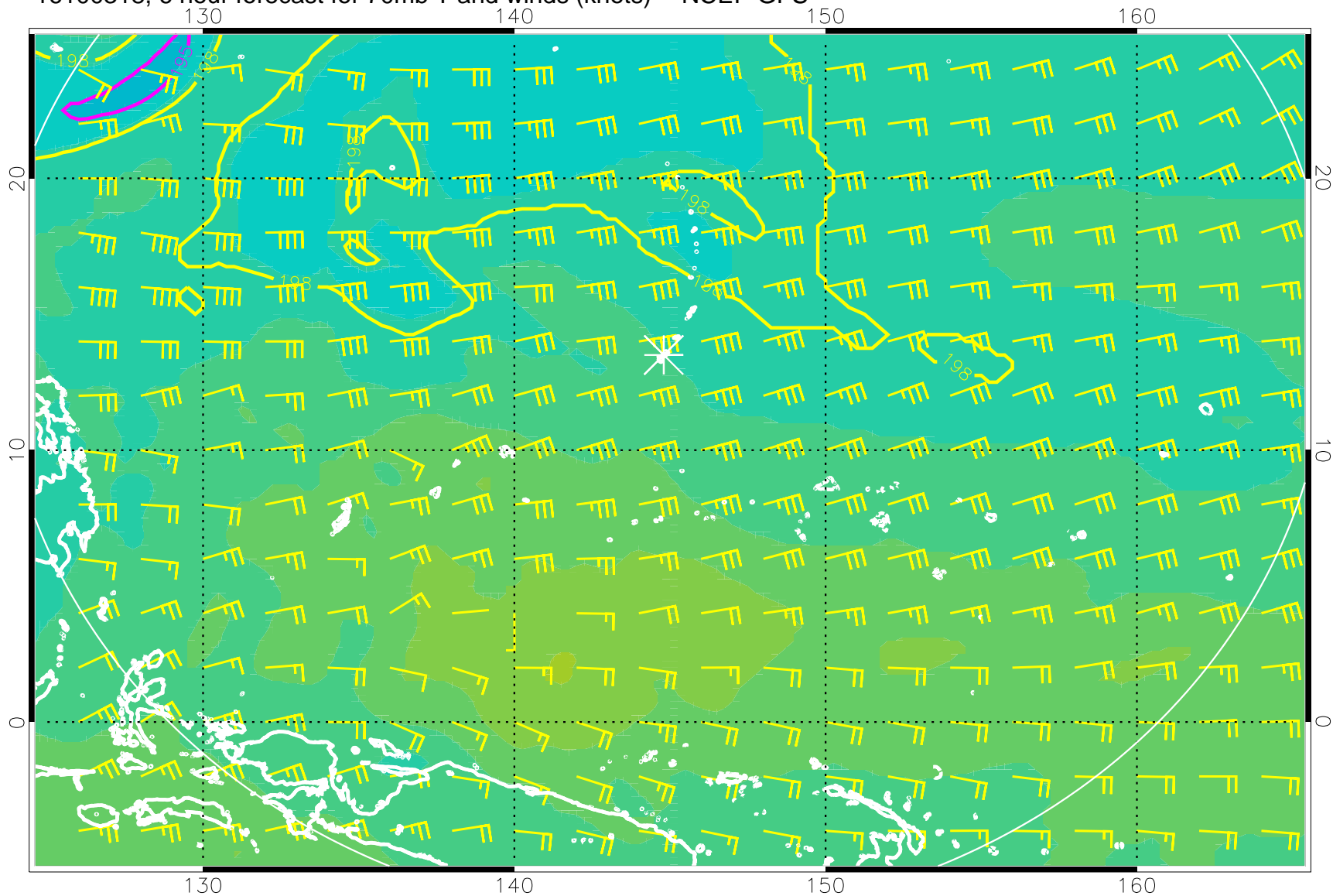
16100318, 6 hour forecast for 70mb T and winds (knots) -- NCEP GFS
