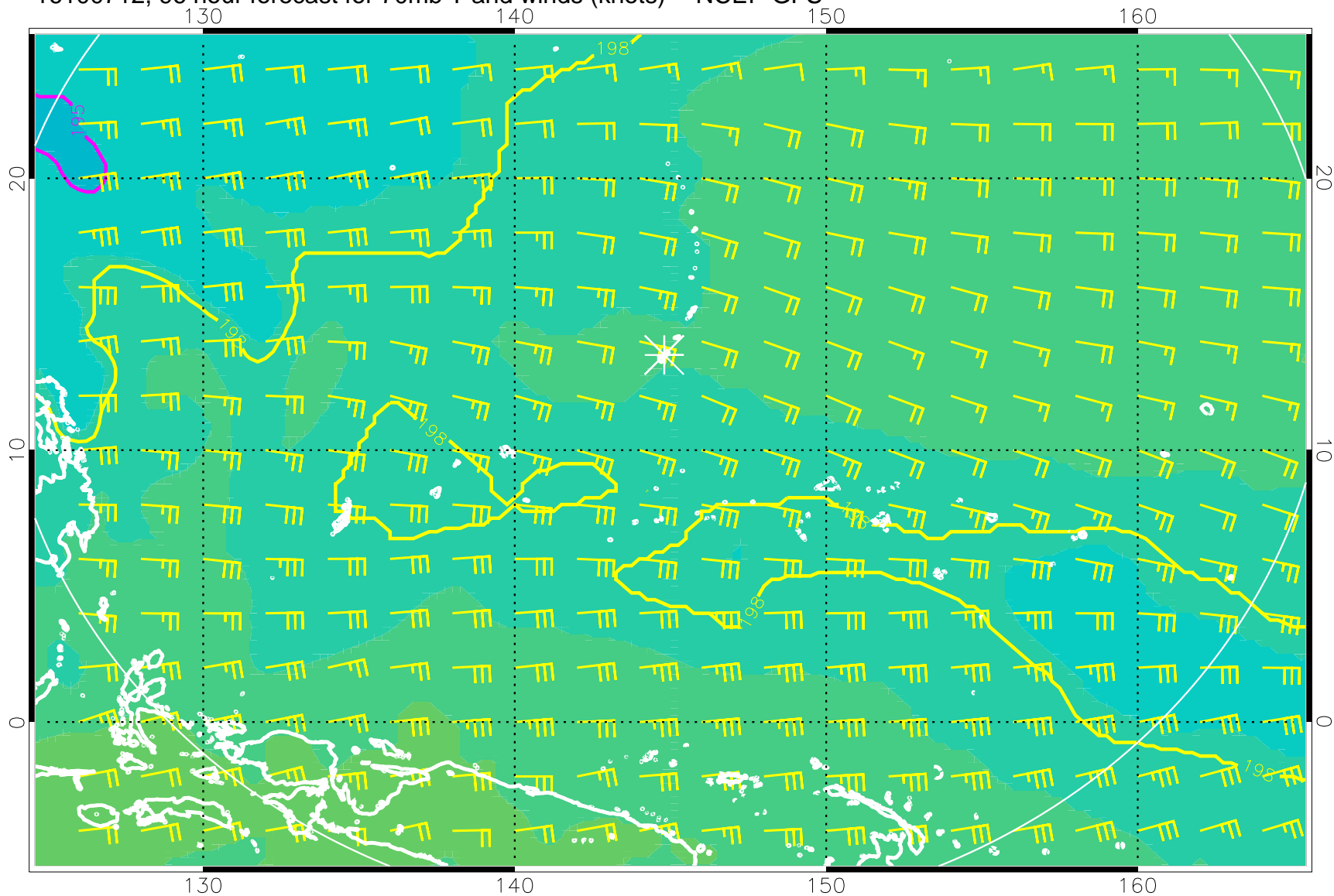
16100712, 96 hour forecast for 70mb T and winds (knots) -- NCEP GFS
