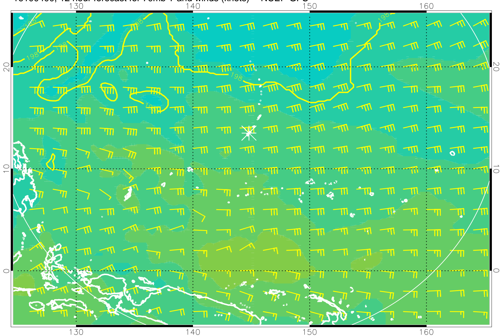
16100400, 12 hour forecast for 70mb T and winds (knots) -- NCEP GFS
