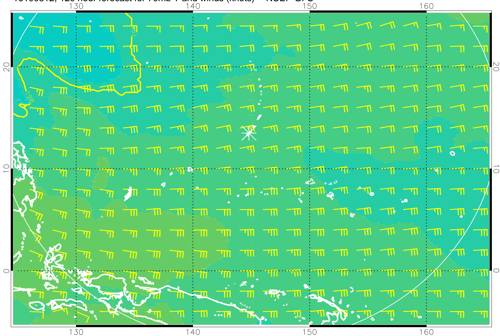
16100812, 120 hour forecast for 70mb T and winds (knots) -- NCEP GFS
