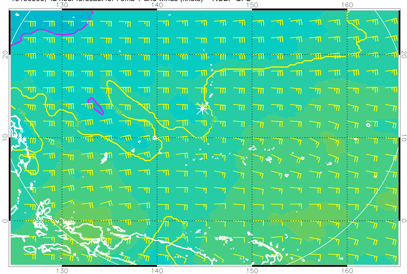
16100506, 42 hour forecast for 70mb T and winds (knots) -- NCEP GFS
