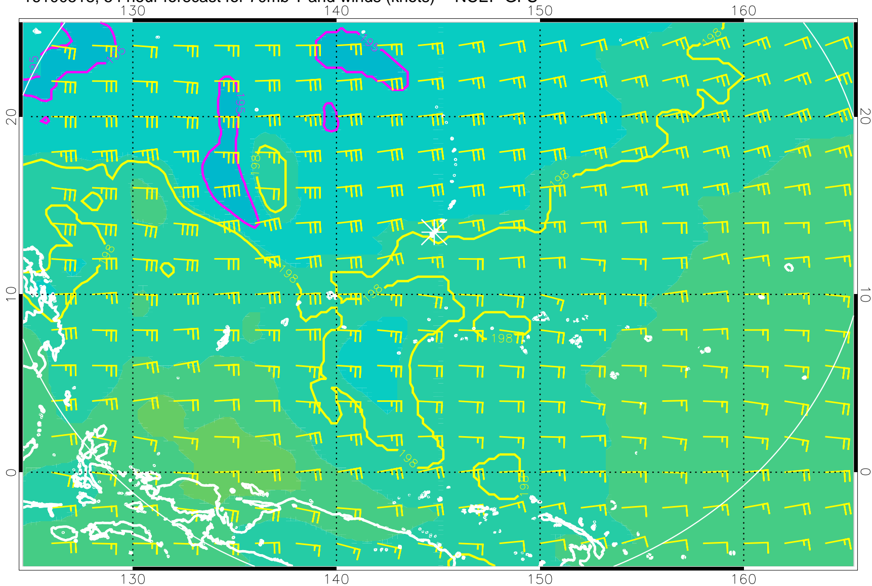
16100518, 54 hour forecast for 70mb T and winds (knots) -- NCEP GFS
