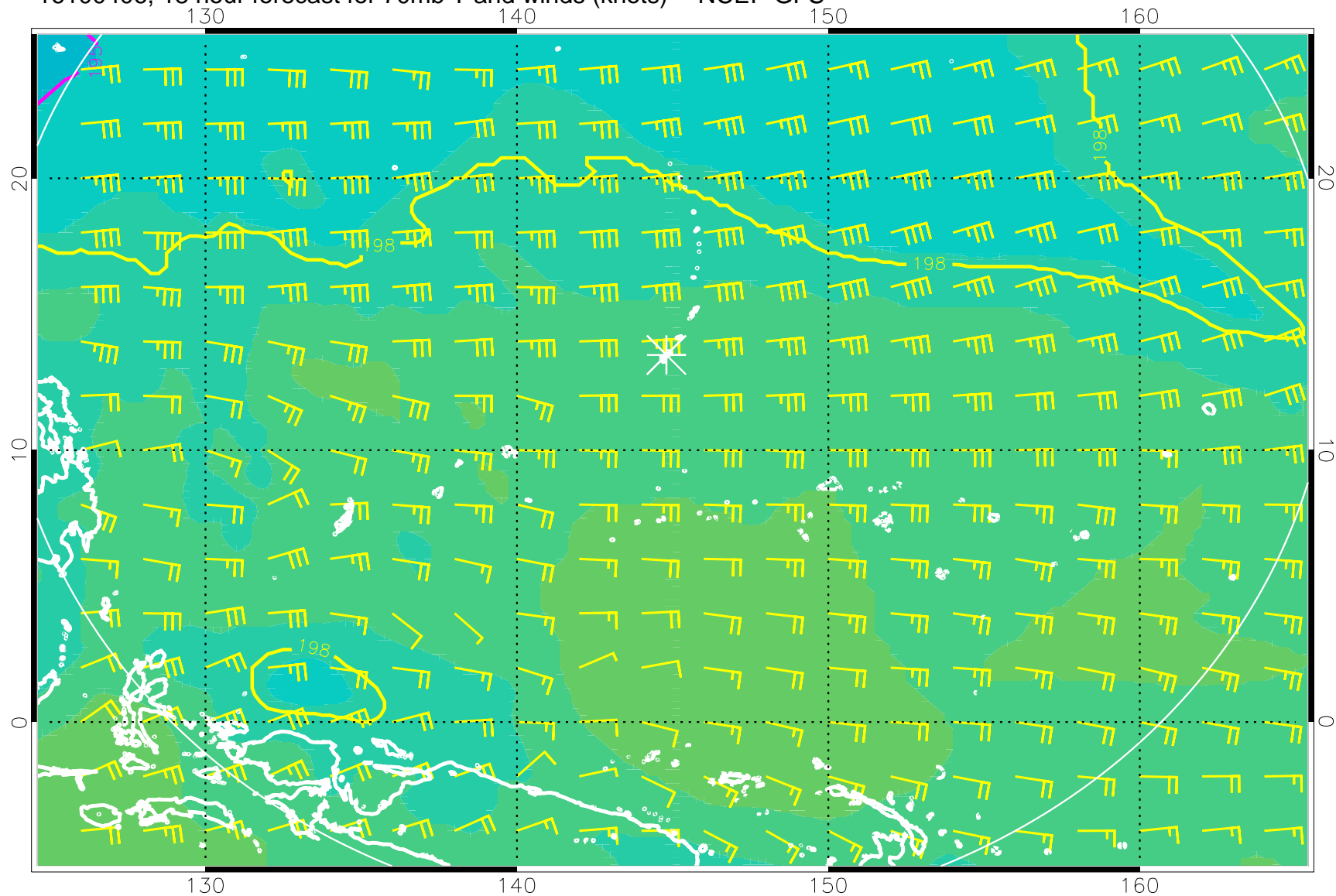
16100406, 18 hour forecast for 70mb T and winds (knots) -- NCEP GFS
