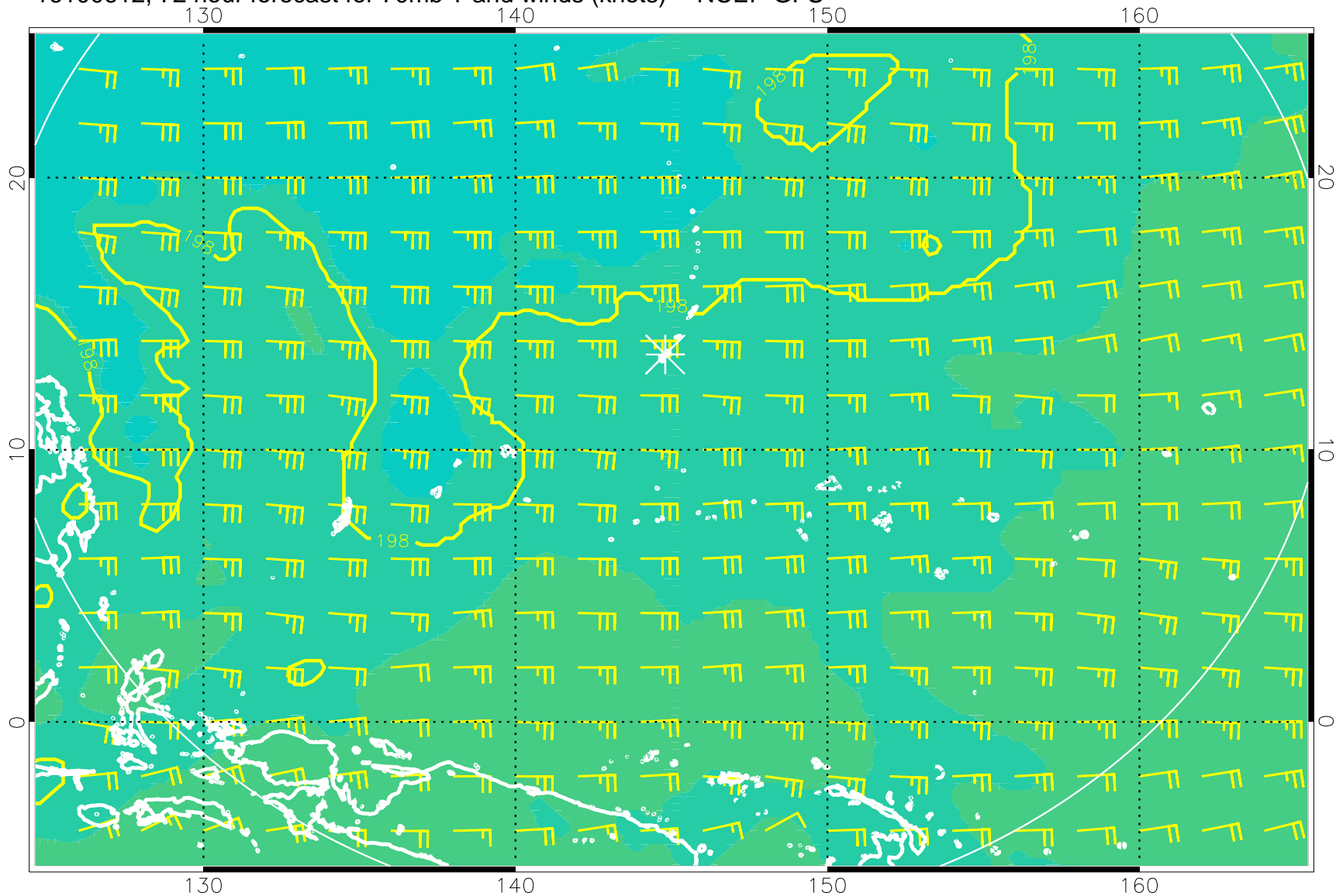
16100612, 72 hour forecast for 70mb T and winds (knots) -- NCEP GFS
