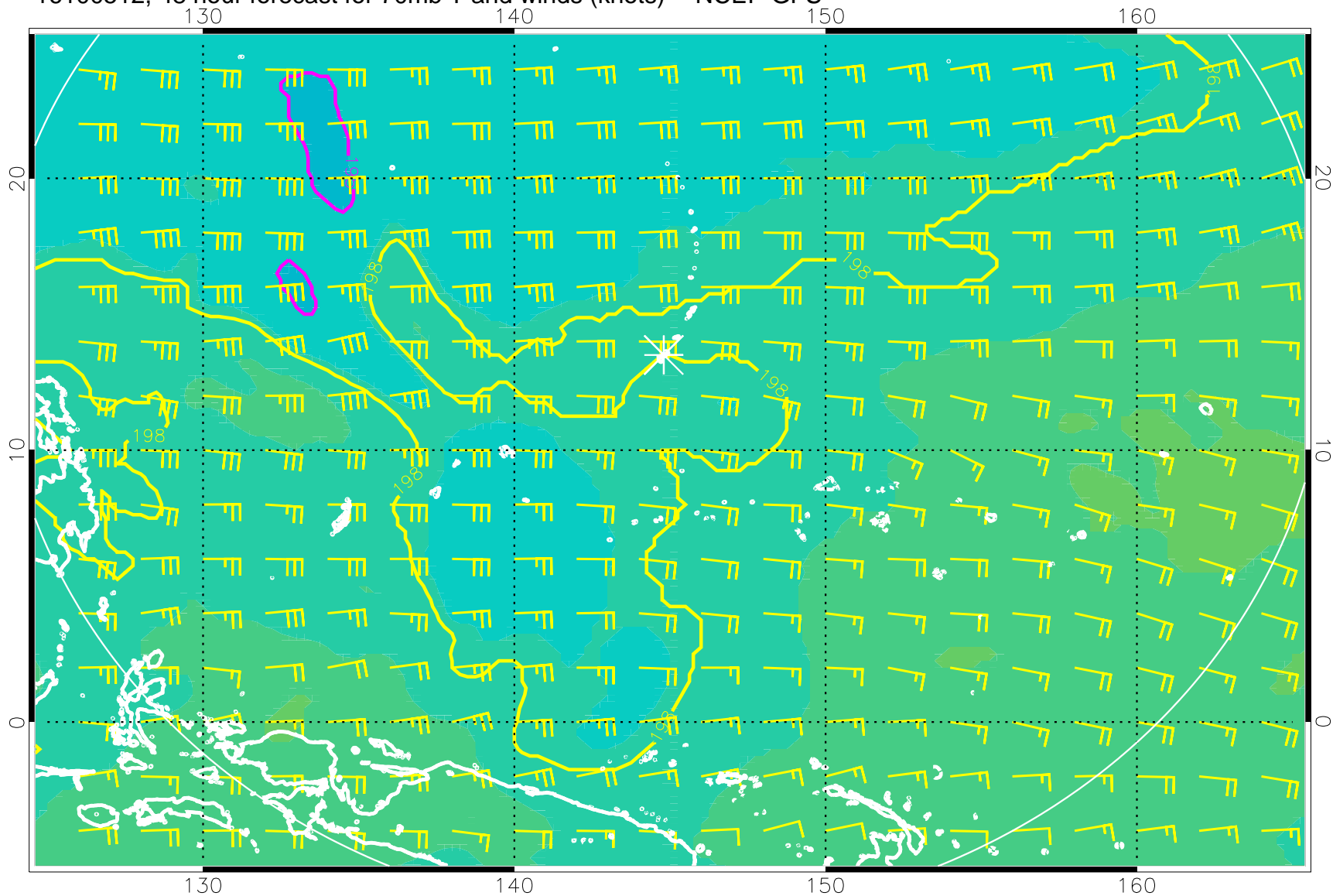
16100512, 48 hour forecast for 70mb T and winds (knots) -- NCEP GFS
