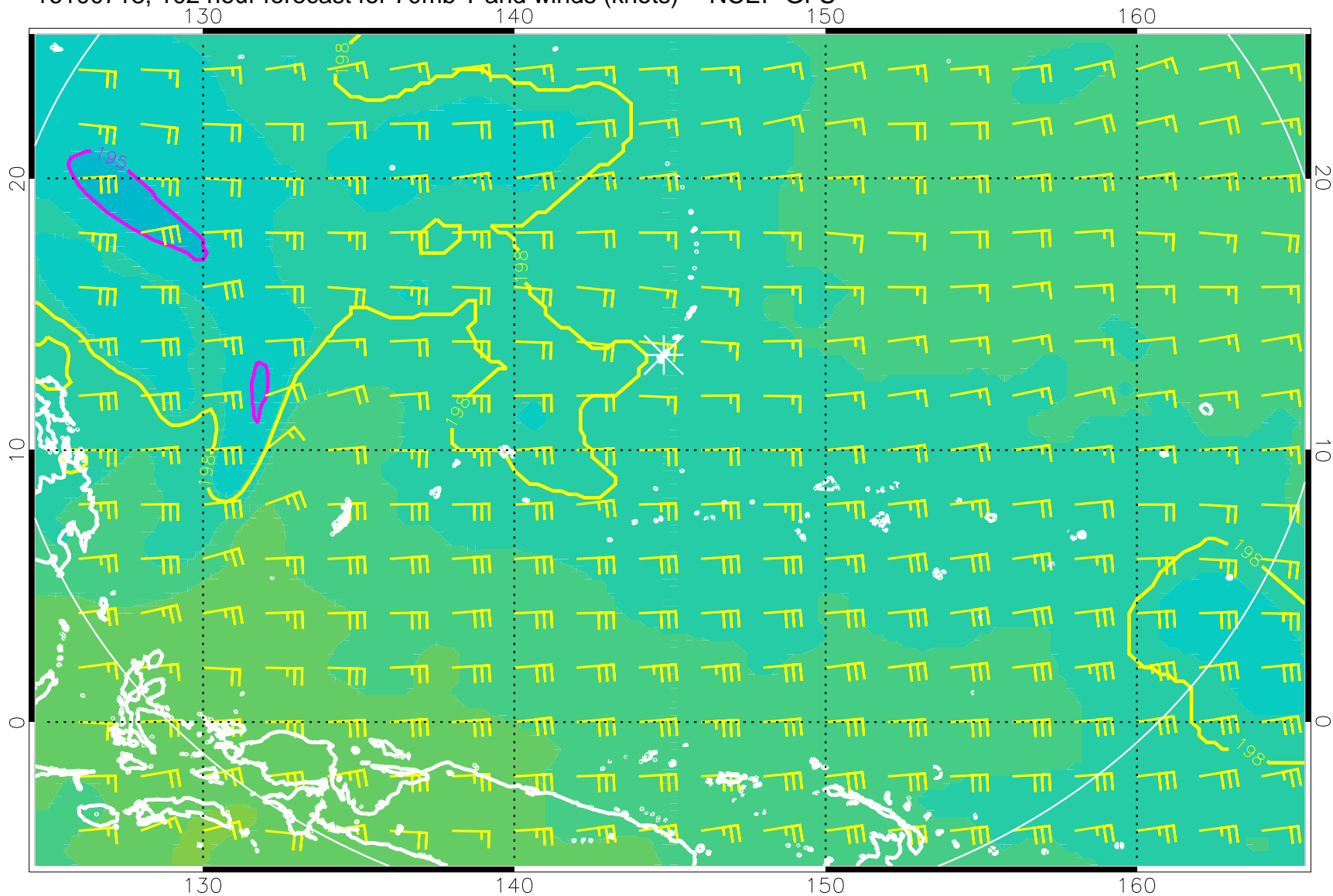
16100718, 102 hour forecast for 70mb T and winds (knots) -- NCEP GFS
