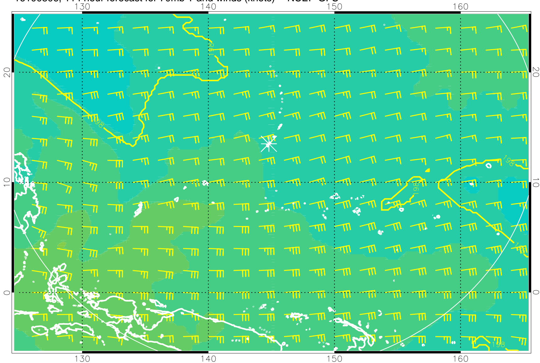
16100806, 114 hour forecast for 70mb T and winds (knots) -- NCEP GFS
