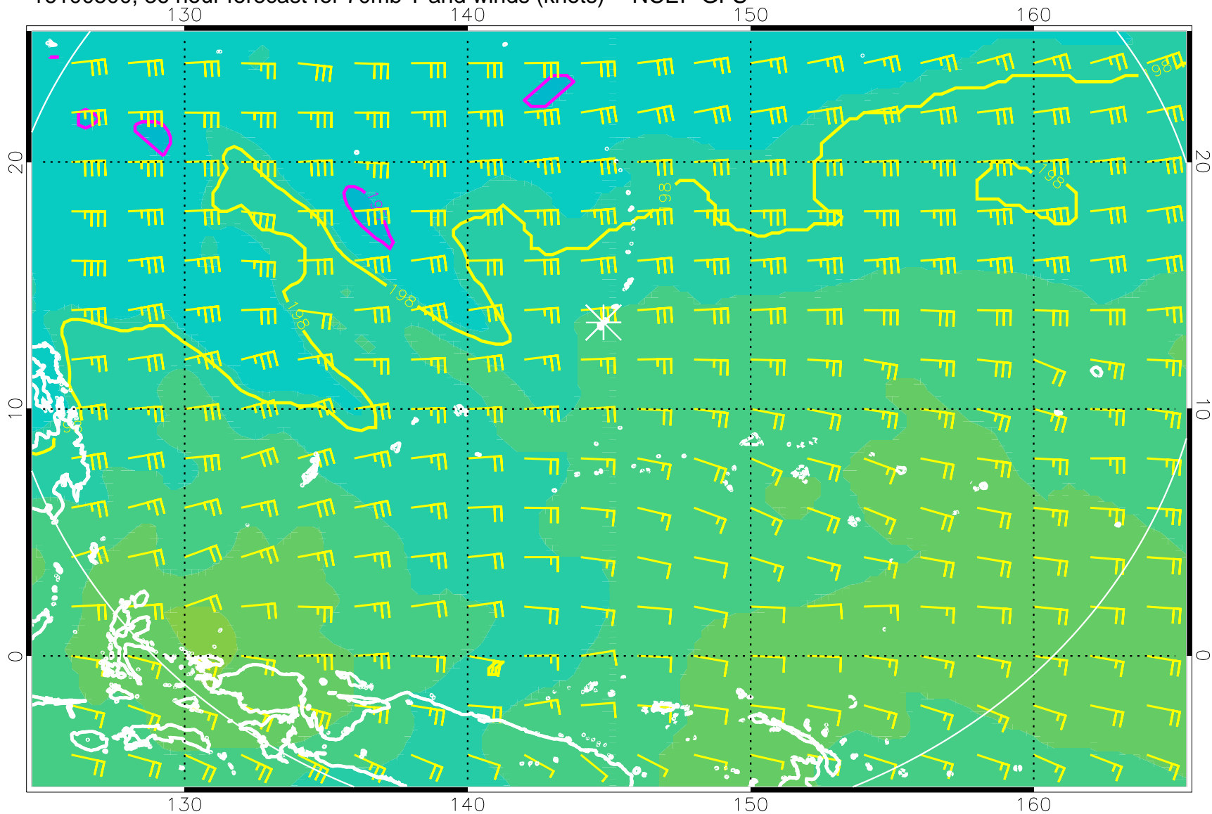
16100500, 36 hour forecast for 70mb T and winds (knots) -- NCEP GFS
