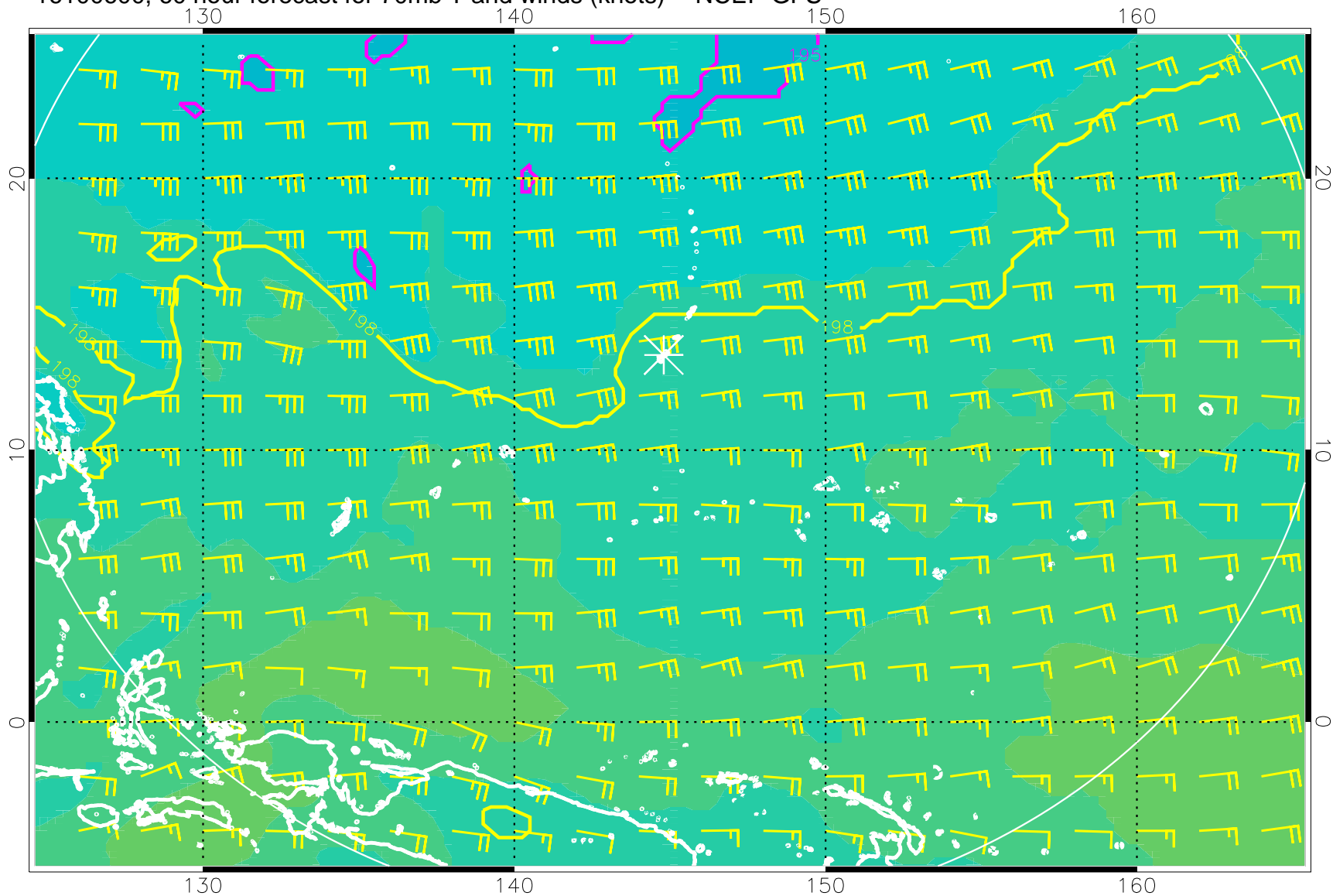
16100600, 60 hour forecast for 70mb T and winds (knots) -- NCEP GFS
