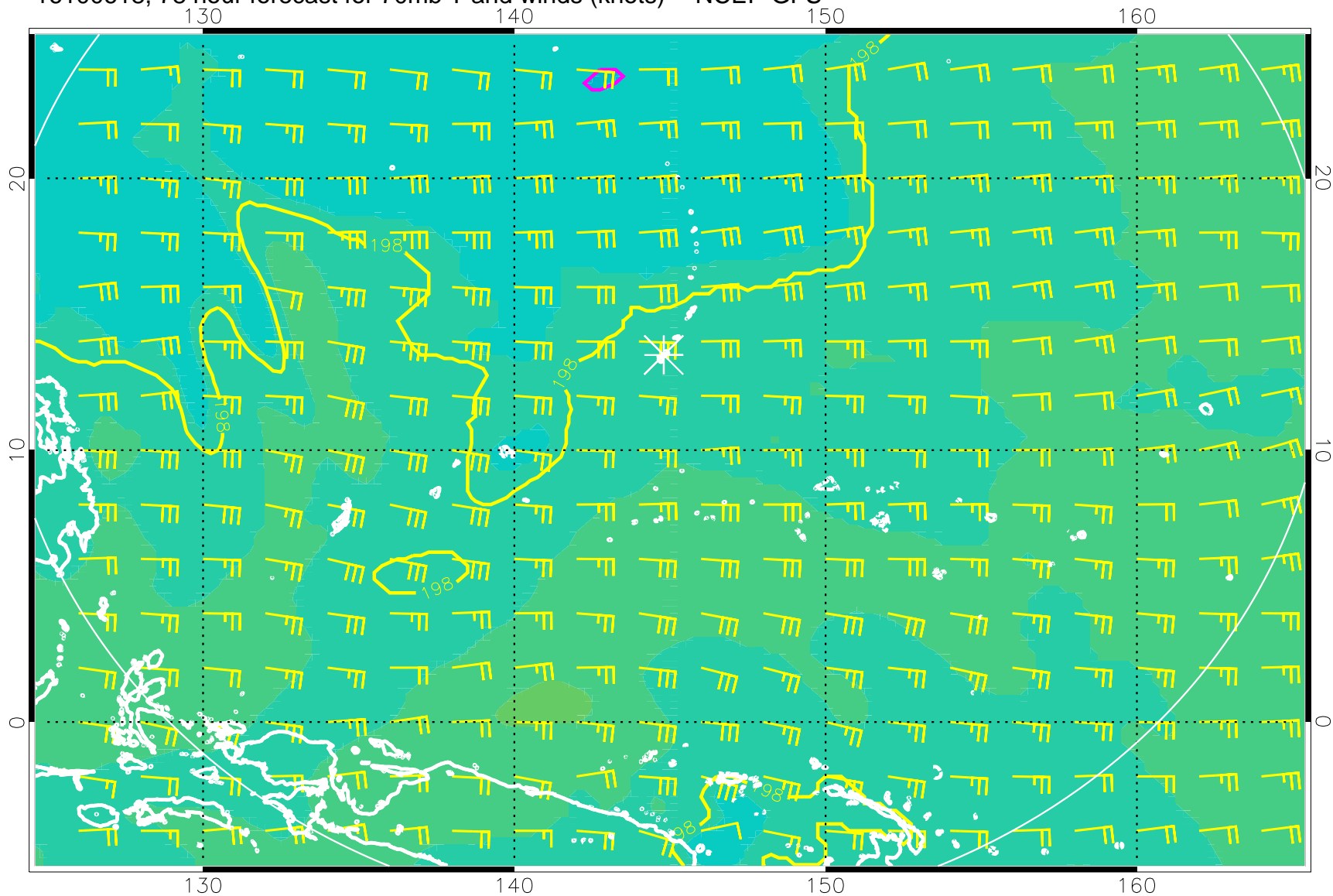
16100618, 78 hour forecast for 70mb T and winds (knots) -- NCEP GFS
