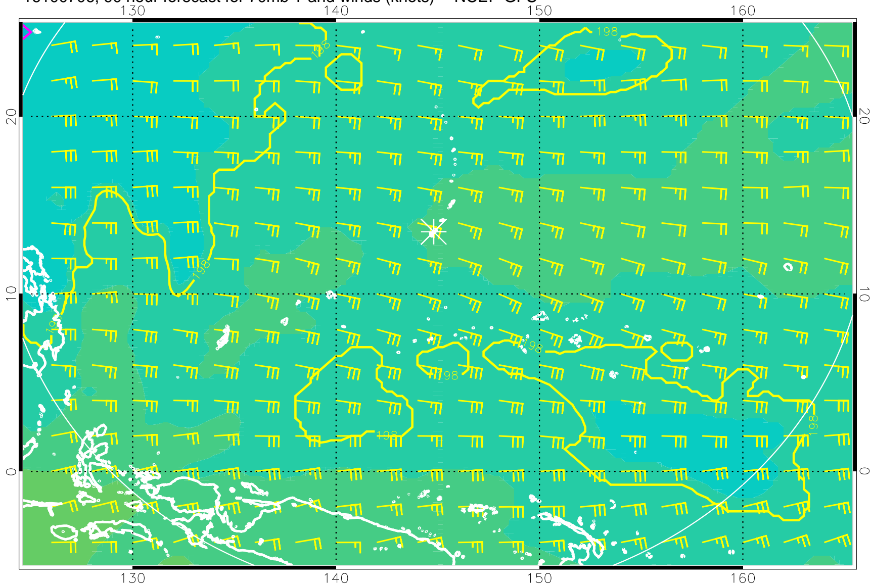
16100706, 90 hour forecast for 70mb T and winds (knots) -- NCEP GFS
