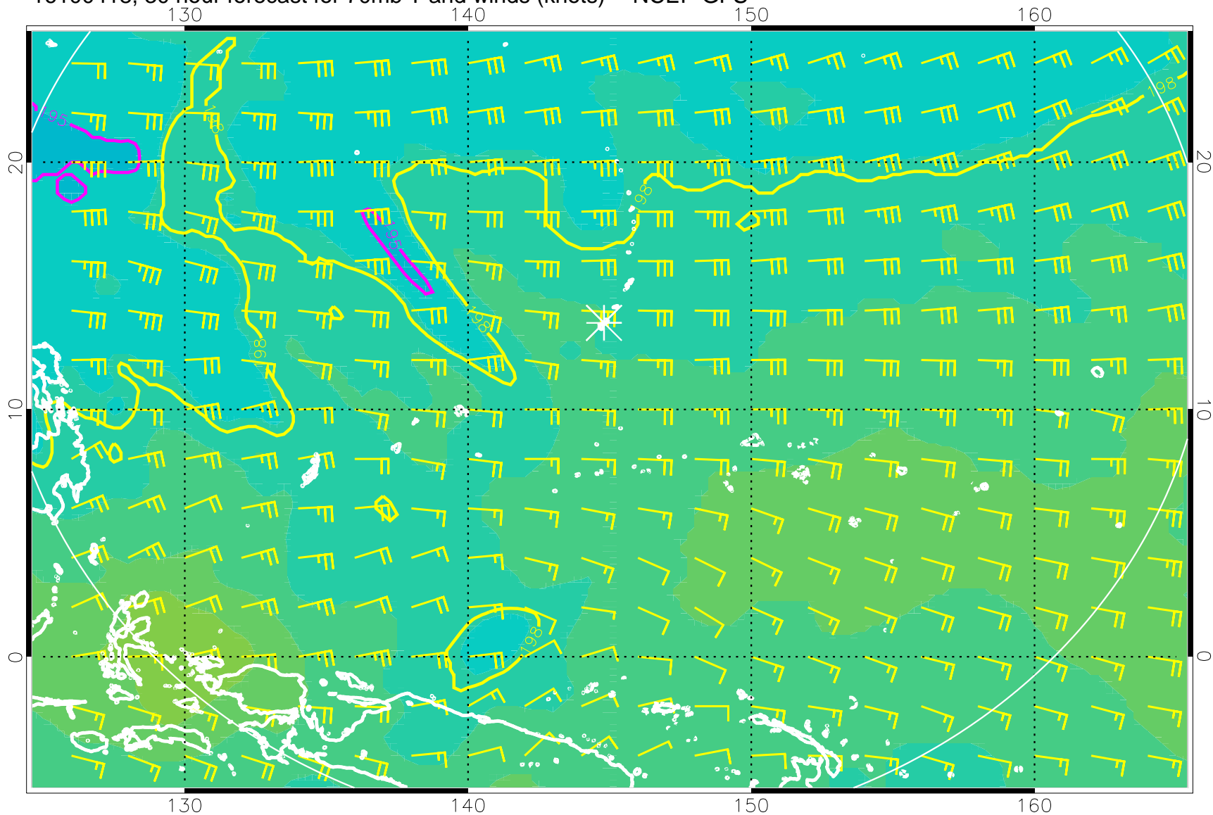
16100418, 30 hour forecast for 70mb T and winds (knots) -- NCEP GFS
