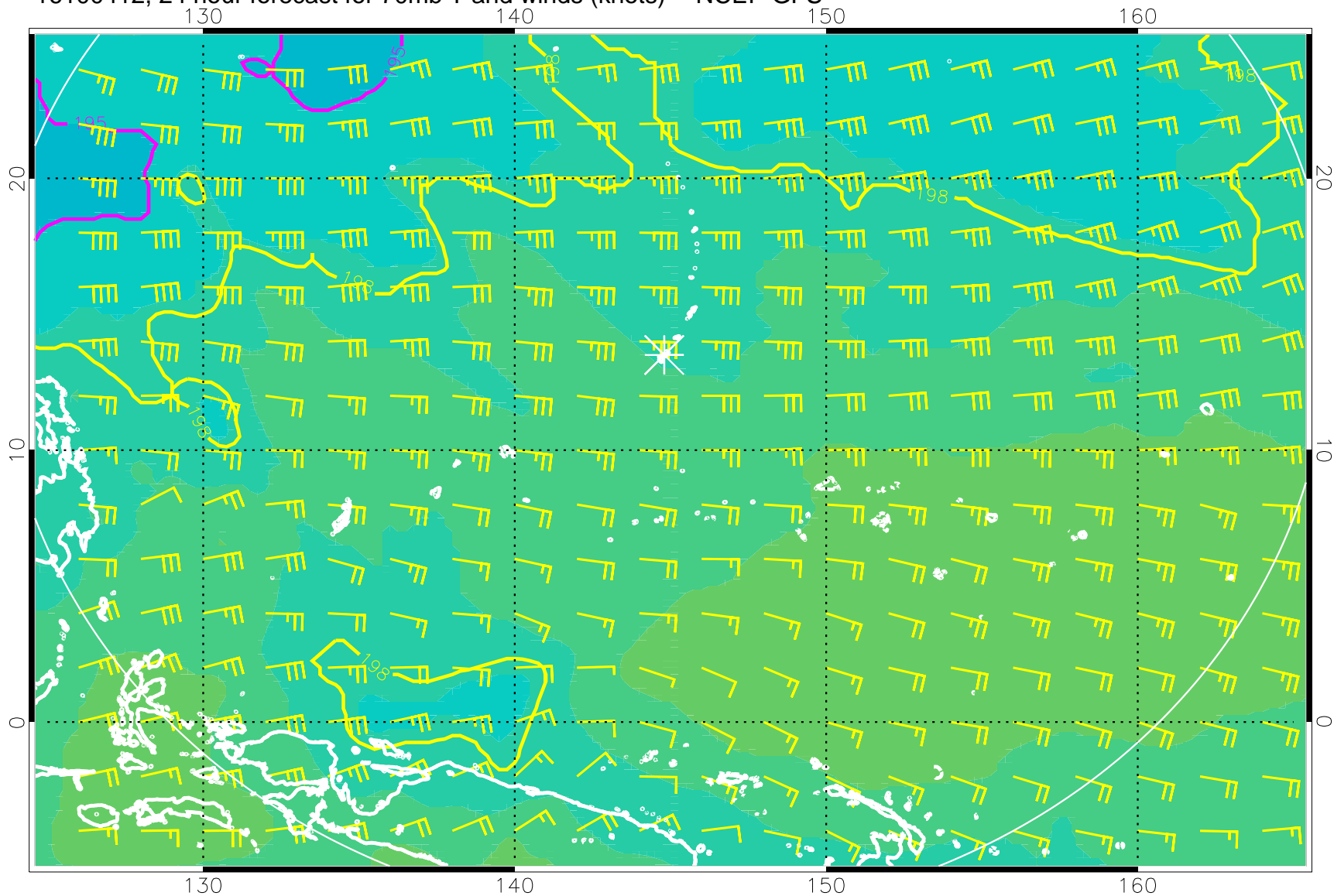
16100412, 24 hour forecast for 70mb T and winds (knots) -- NCEP GFS
