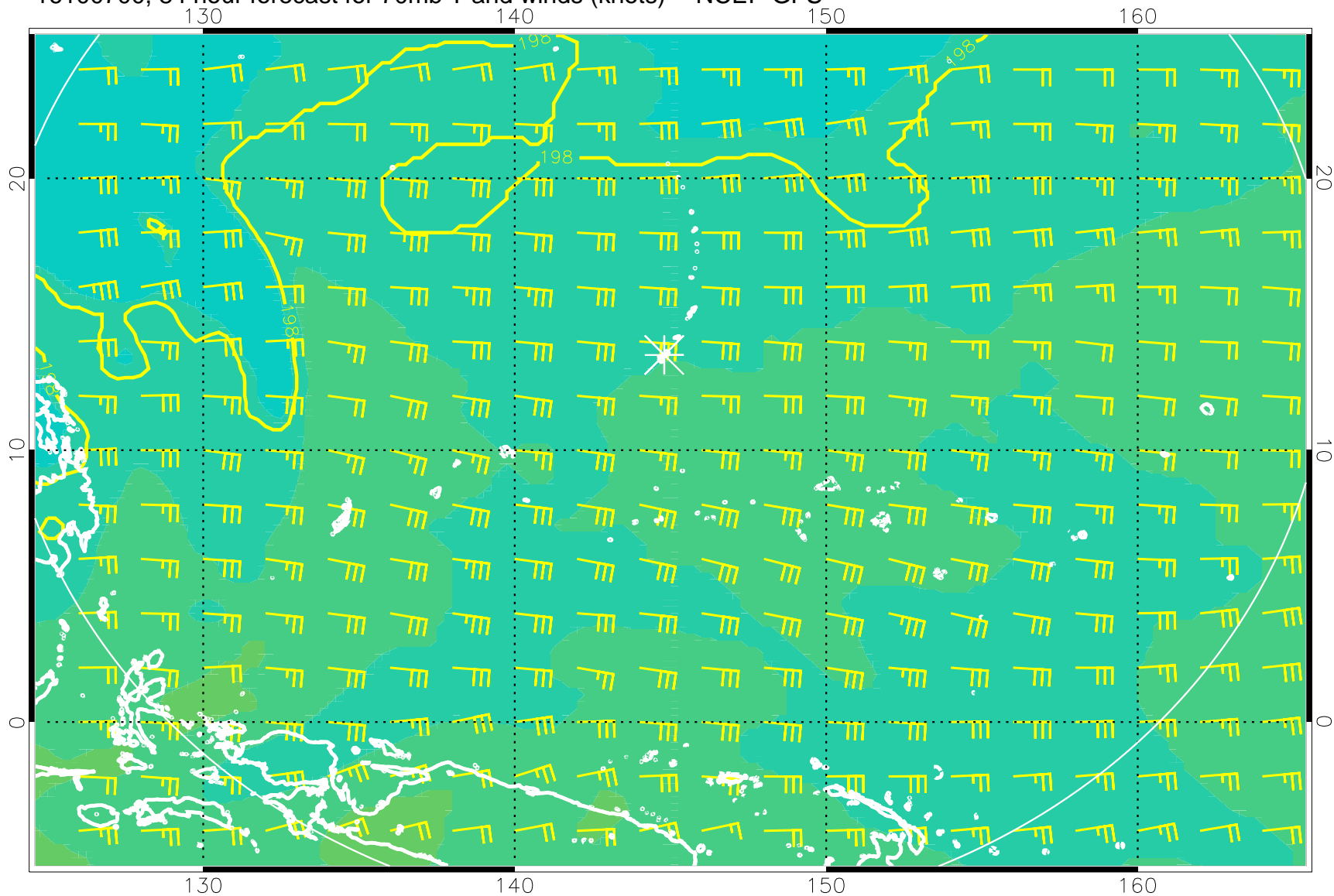
16100700, 84 hour forecast for 70mb T and winds (knots) -- NCEP GFS
