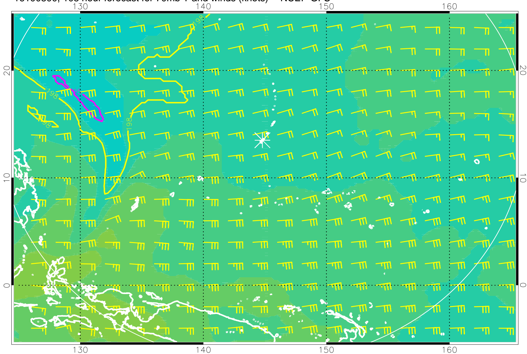
16100800, 108 hour forecast for 70mb T and winds (knots) -- NCEP GFS
