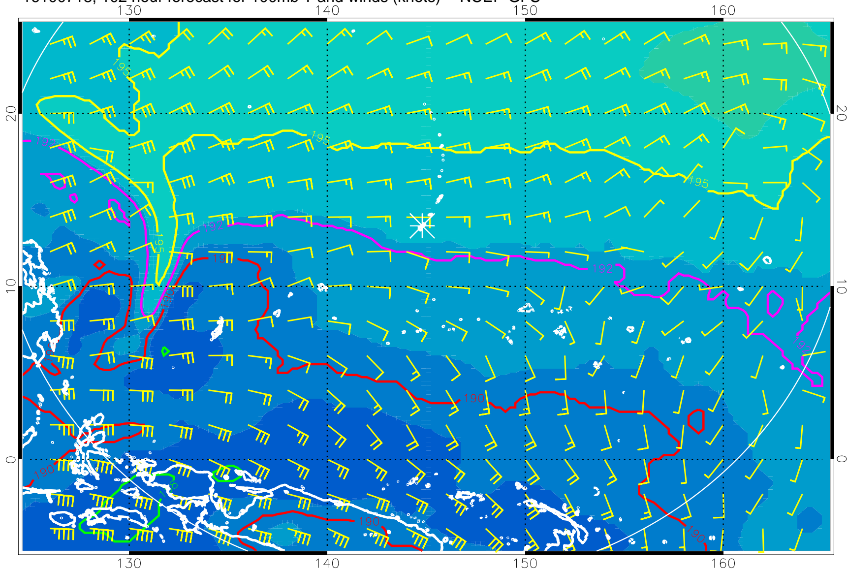
16100718, 102 hour forecast for 100mb T and winds (knots) -- NCEP GFS
