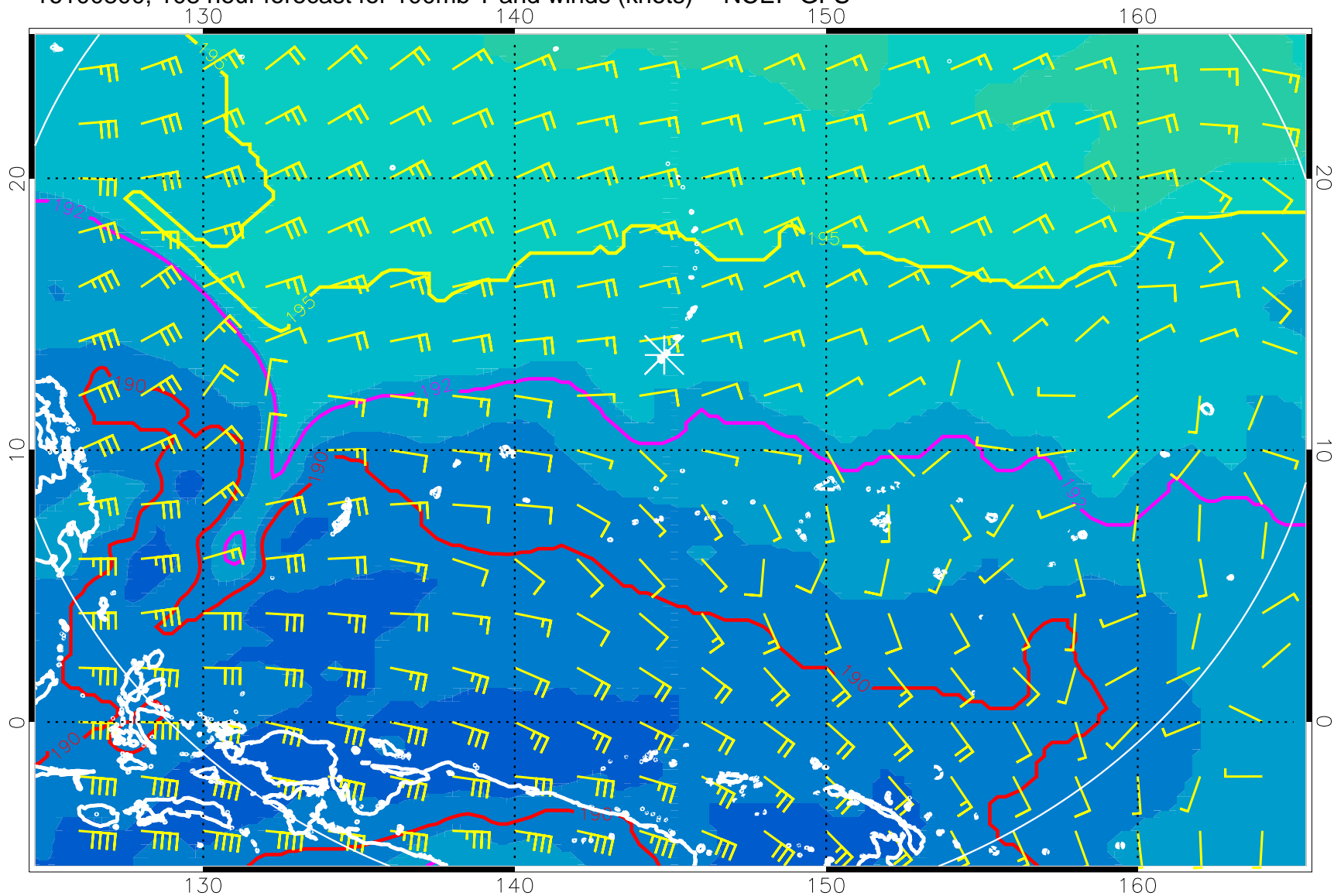
16100800, 108 hour forecast for 100mb T and winds (knots) -- NCEP GFS
