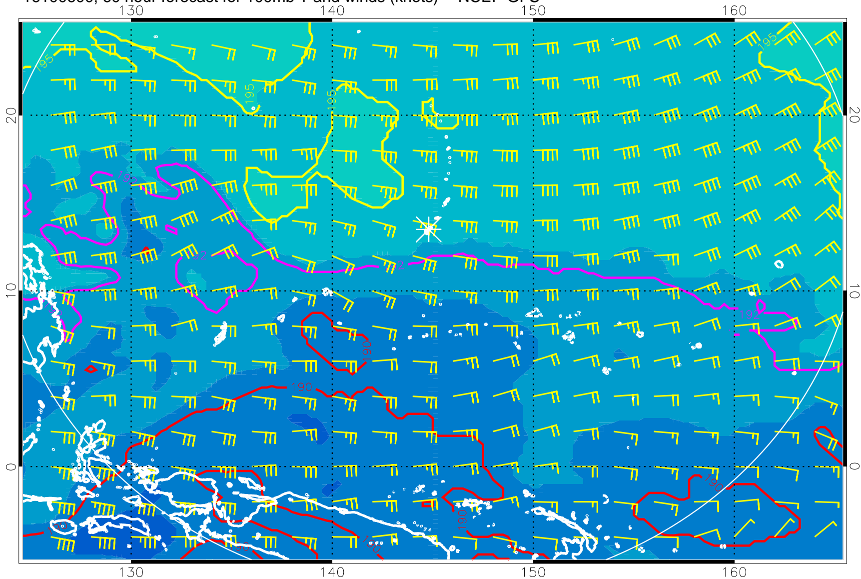
16100600, 60 hour forecast for 100mb T and winds (knots) -- NCEP GFS
