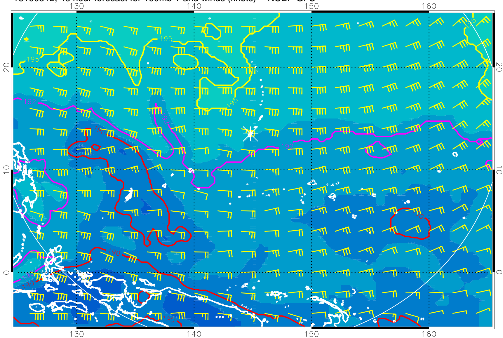
16100512, 48 hour forecast for 100mb T and winds (knots) -- NCEP GFS
