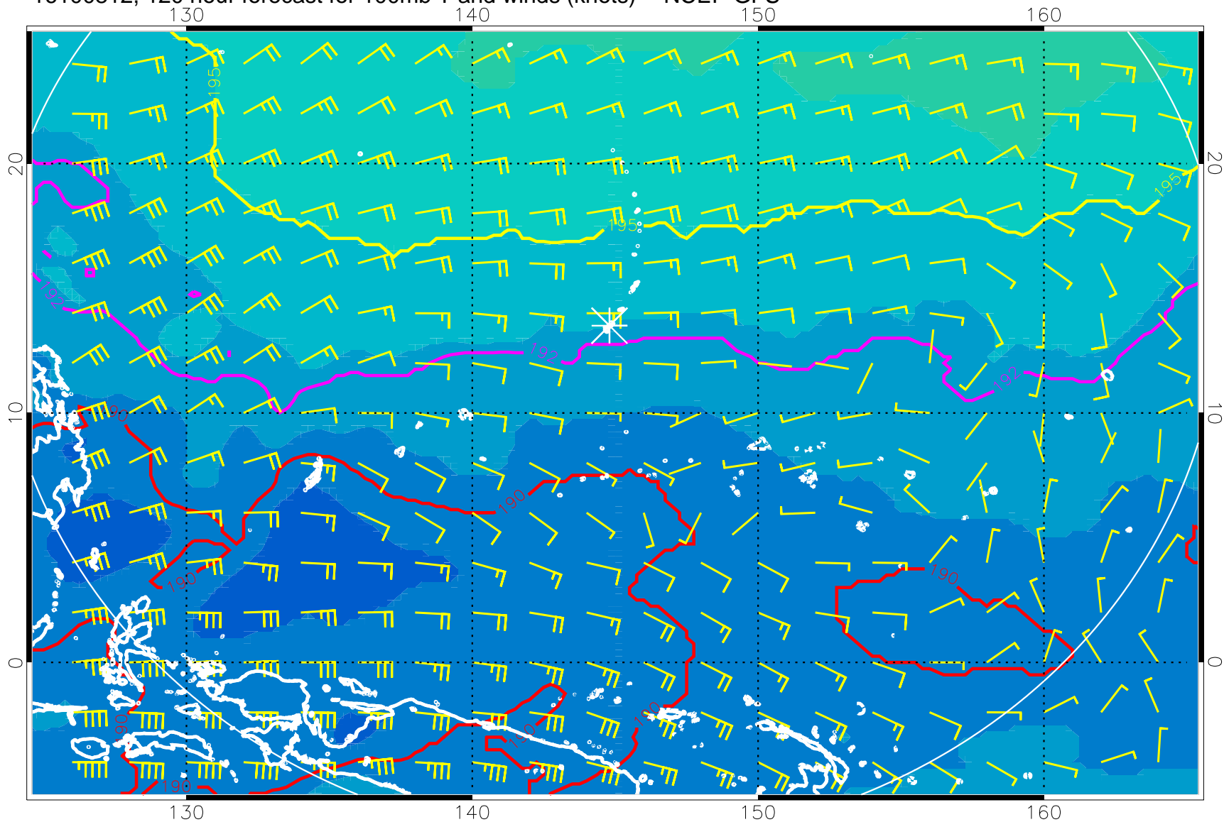
16100812, 120 hour forecast for 100mb T and winds (knots) -- NCEP GFS
