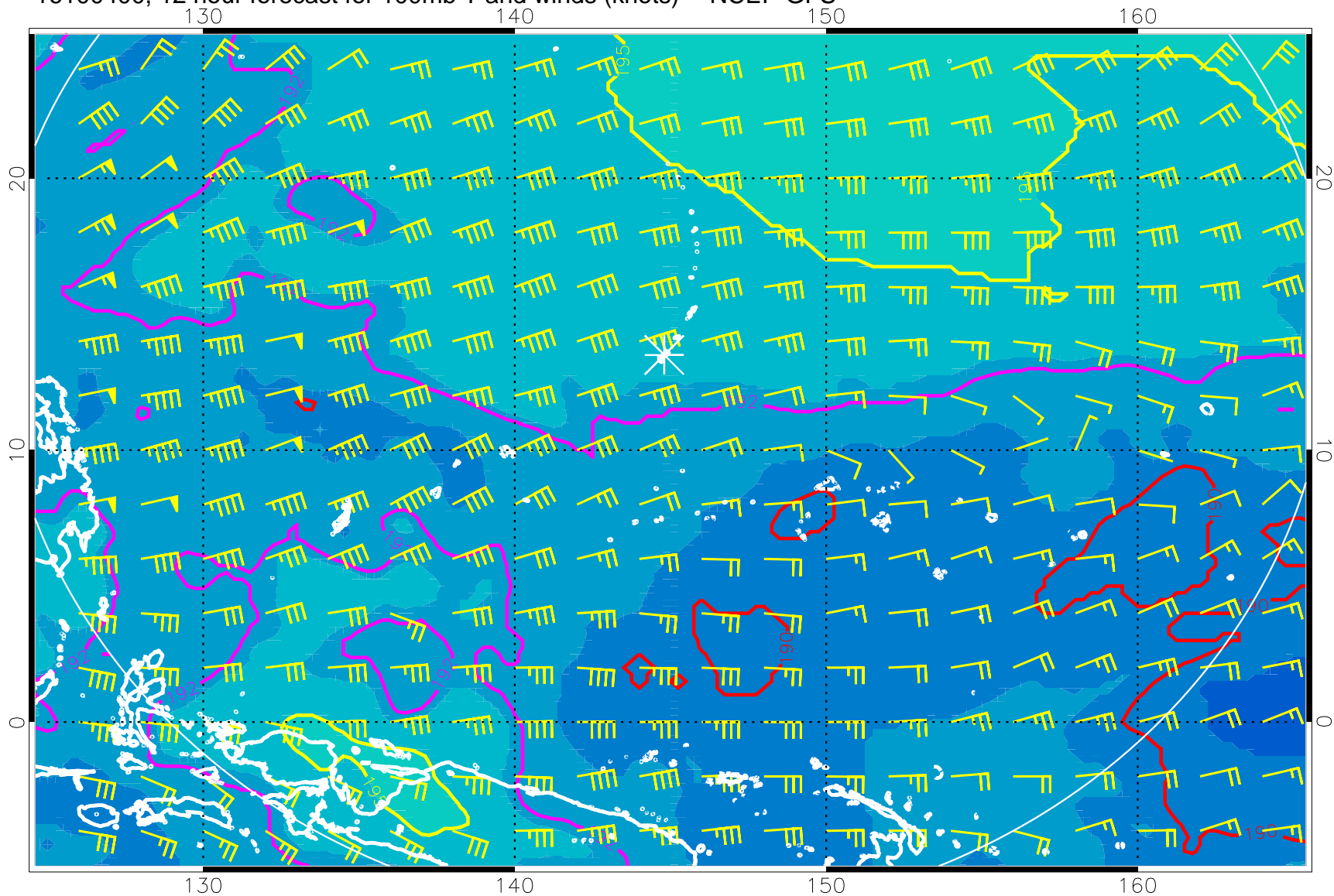
16100400, 12 hour forecast for 100mb T and winds (knots) -- NCEP GFS
