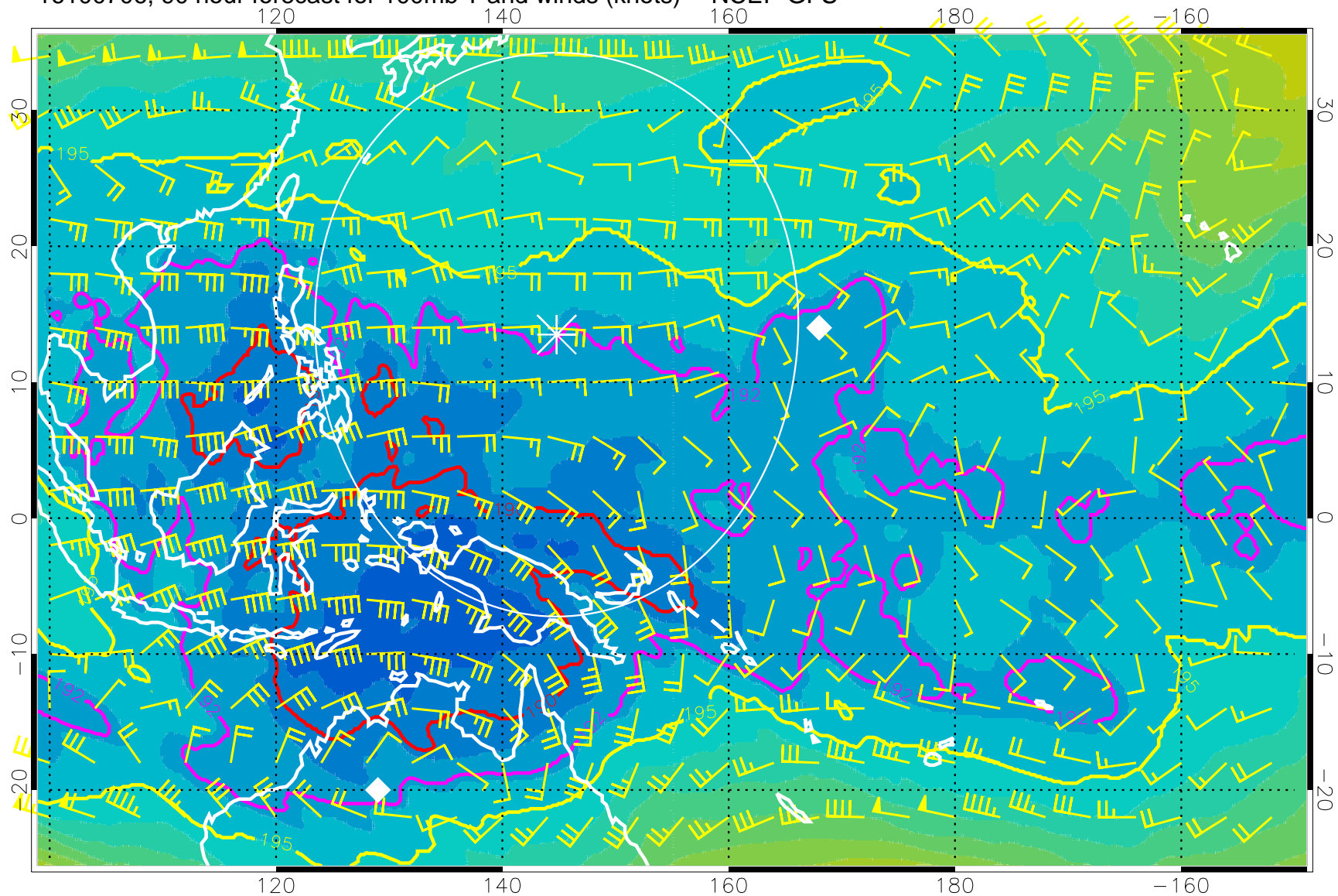
16100706, 90 hour forecast for 100mb T and winds (knots) -- NCEP GFS
