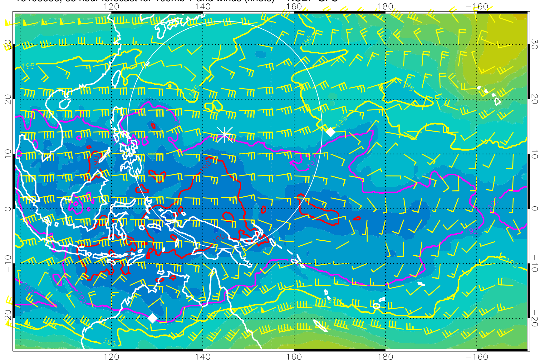
16100606, 66 hour forecast for 100mb T and winds (knots) -- NCEP GFS
