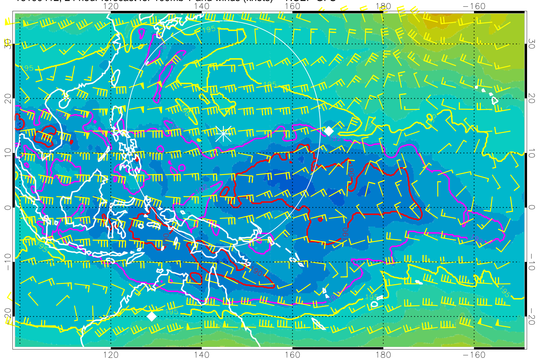
16100412, 24 hour forecast for 100mb T and winds (knots) -- NCEP GFS
