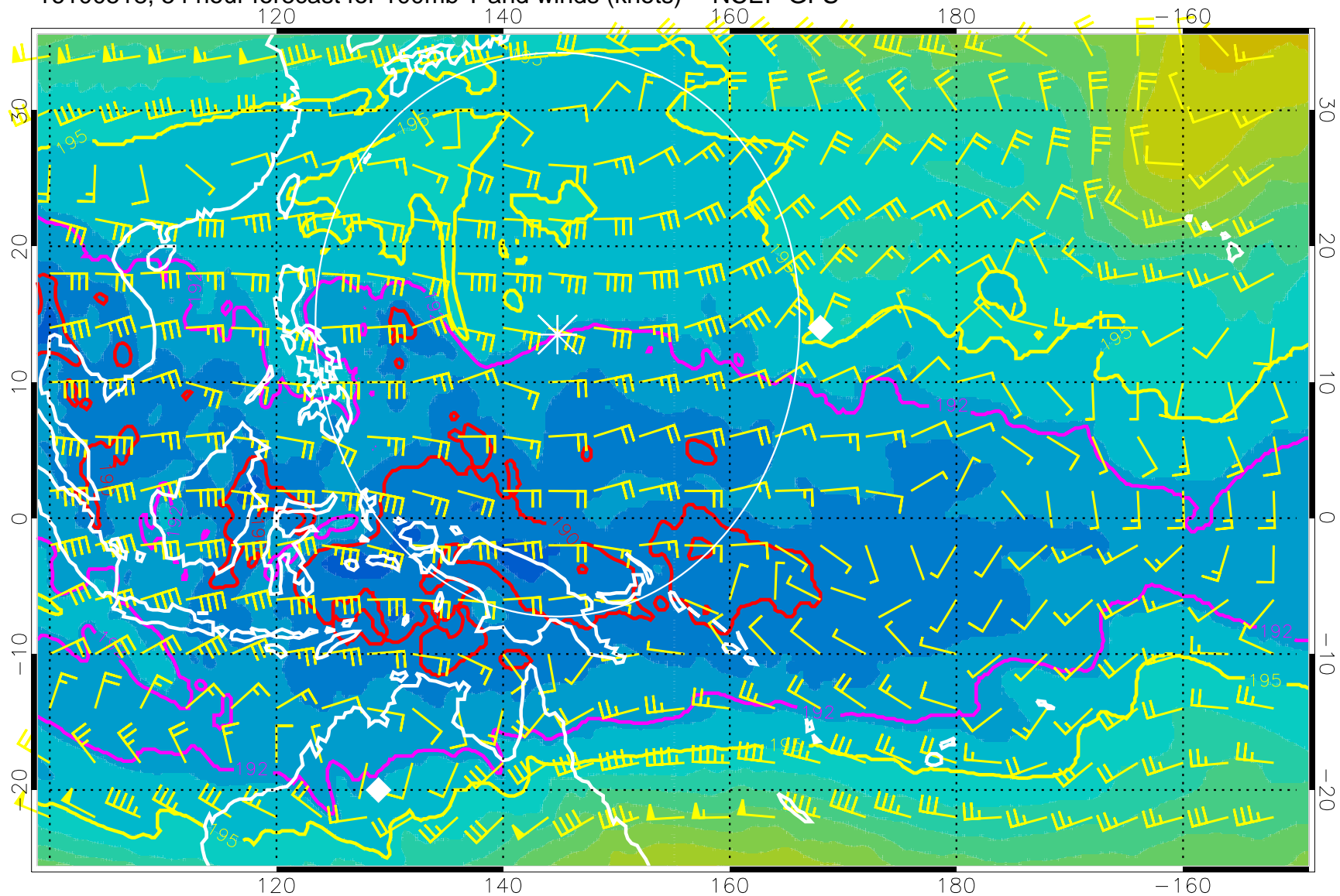
16100518, 54 hour forecast for 100mb T and winds (knots) -- NCEP GFS
