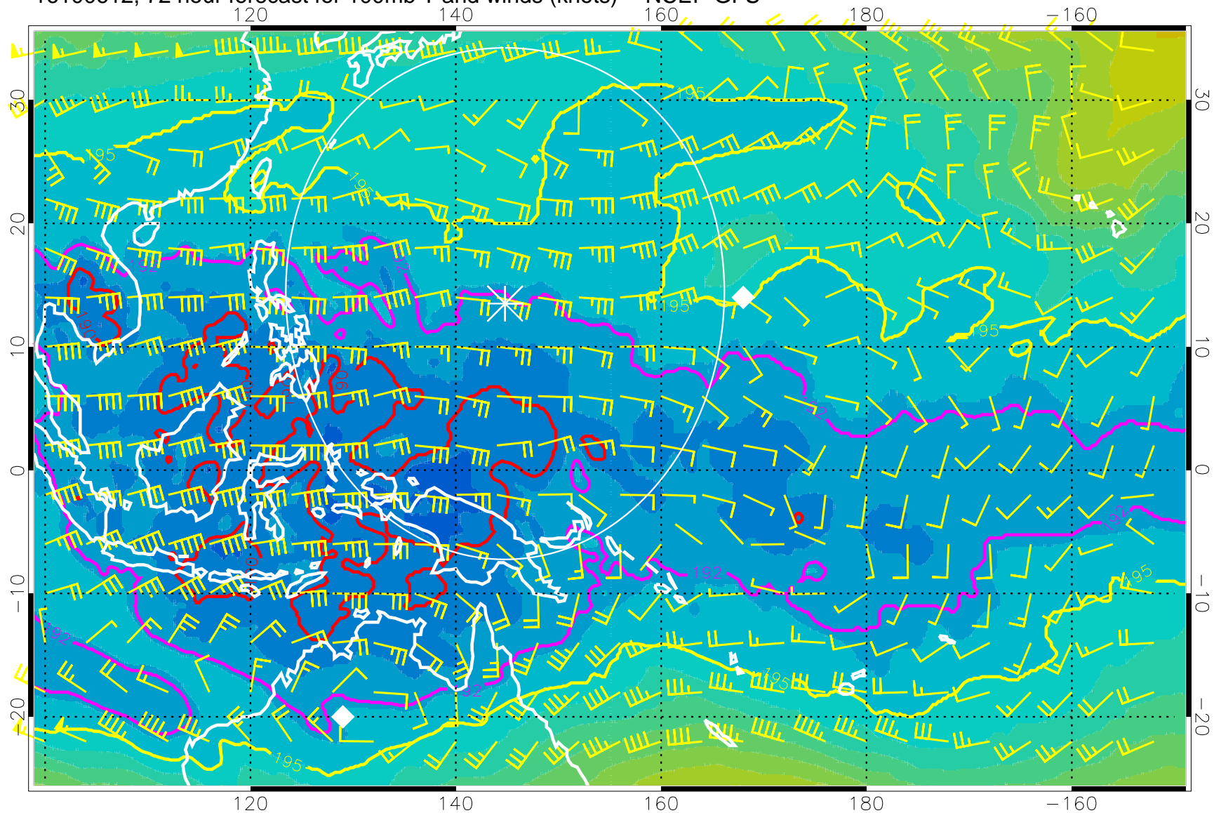
16100612, 72 hour forecast for 100mb T and winds (knots) -- NCEP GFS
