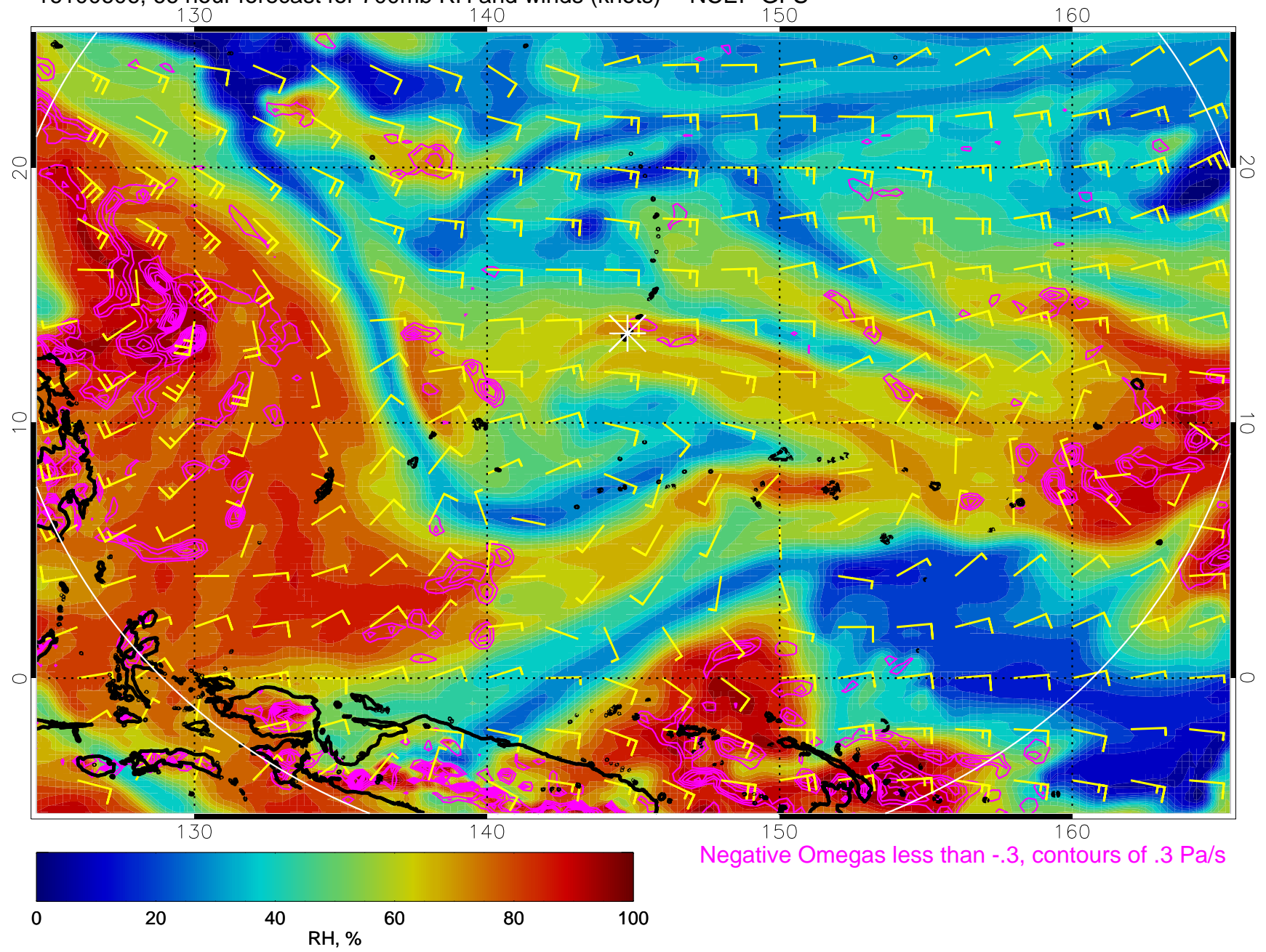
16100606, 66 hour forecast for 700mb RH and winds (knots) -- NCEP GFS
