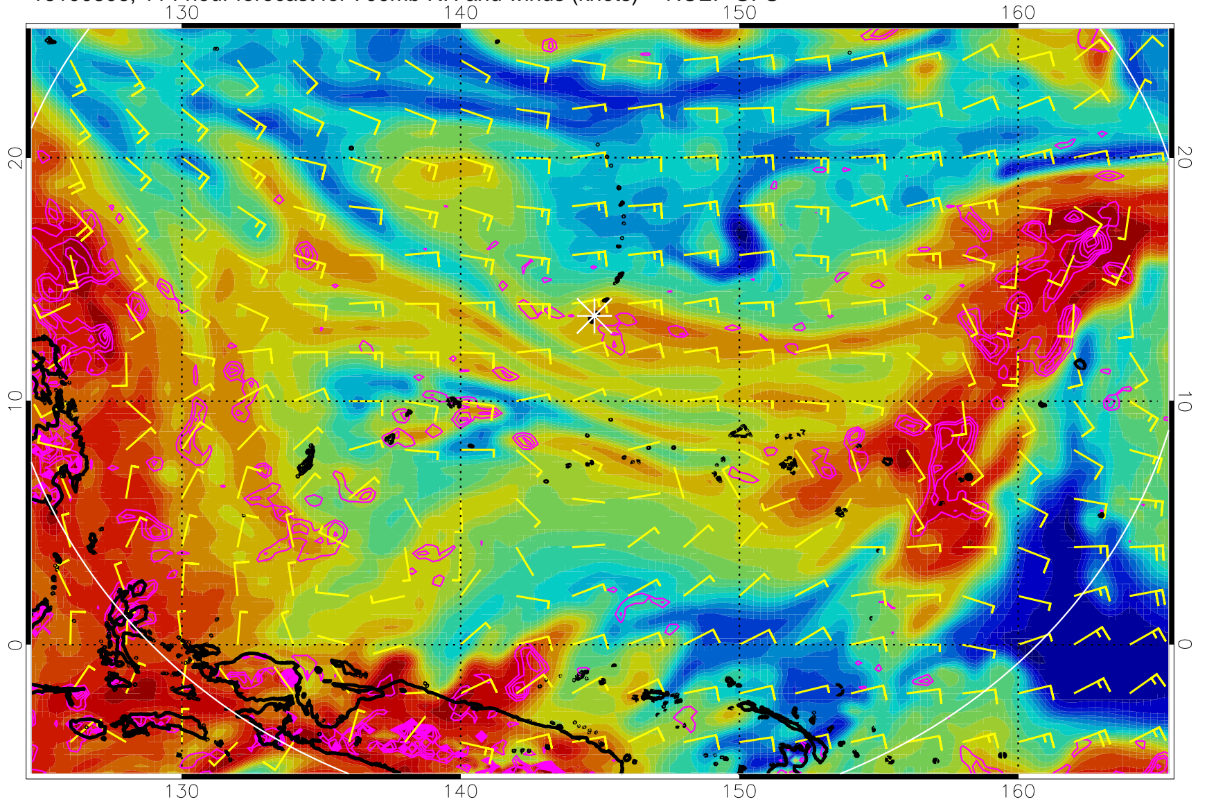
16100806, 114 hour forecast for 700mb RH and winds (knots) -- NCEP GFS
