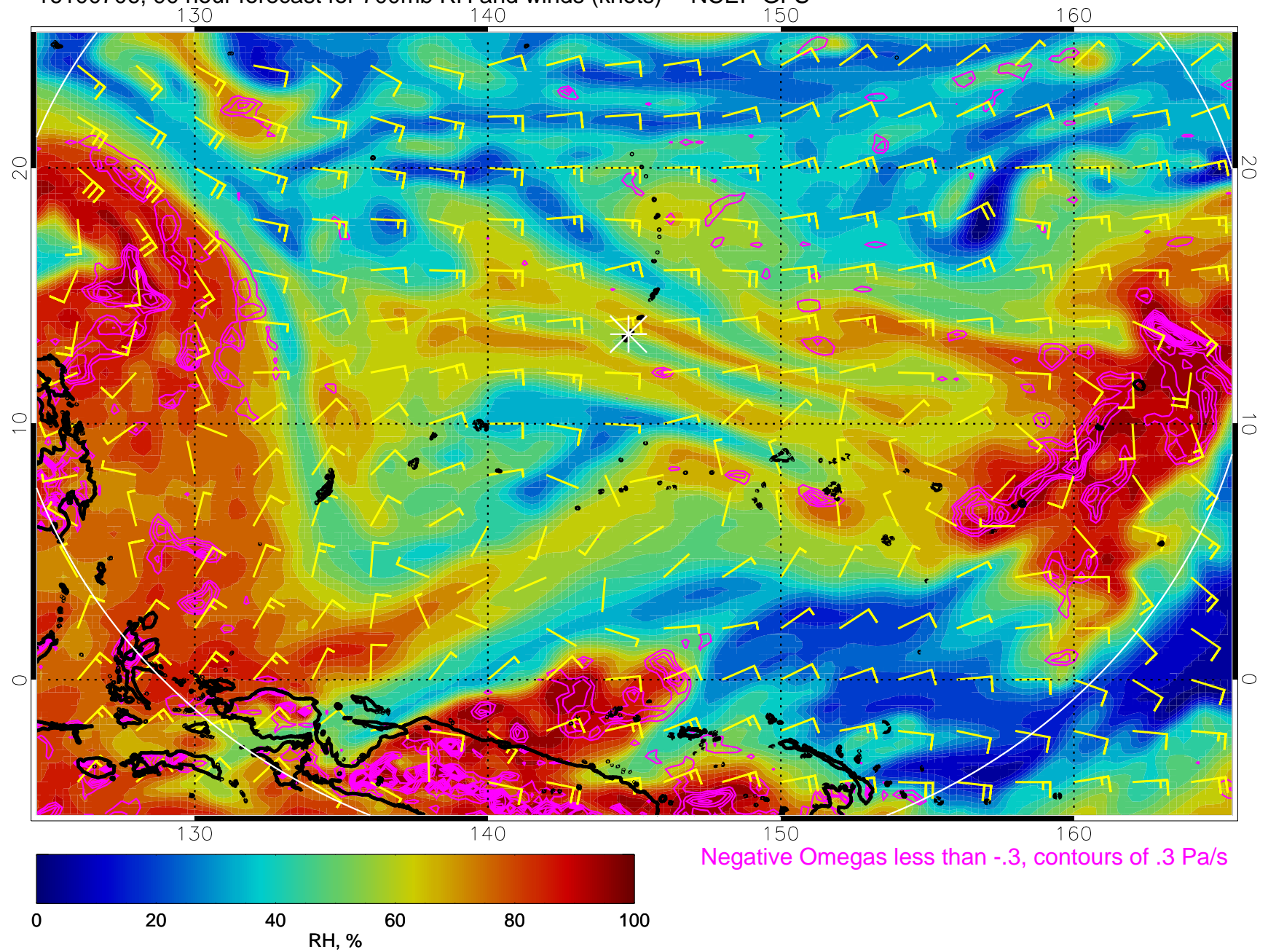
16100706, 90 hour forecast for 700mb RH and winds (knots) -- NCEP GFS
