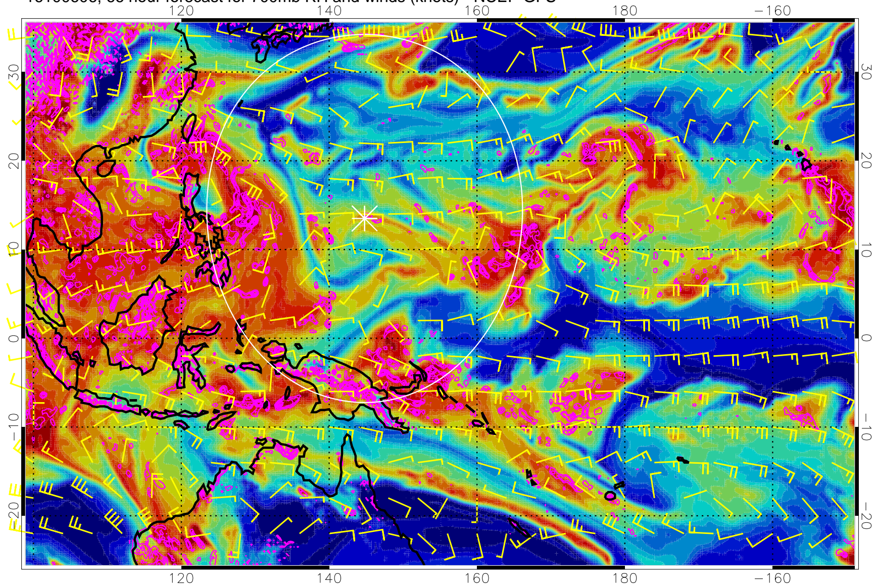
16100606, 66 hour forecast for 700mb RH and winds (knots) - NCEP GFS
