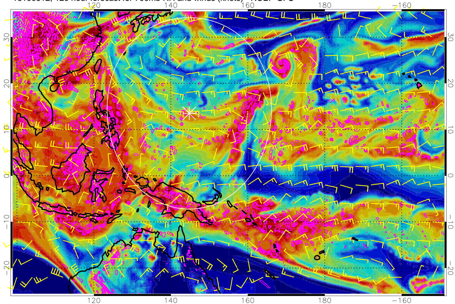
16100812, 120 hour forecast for 700mb RH and winds (knots) - NCEP GFS
