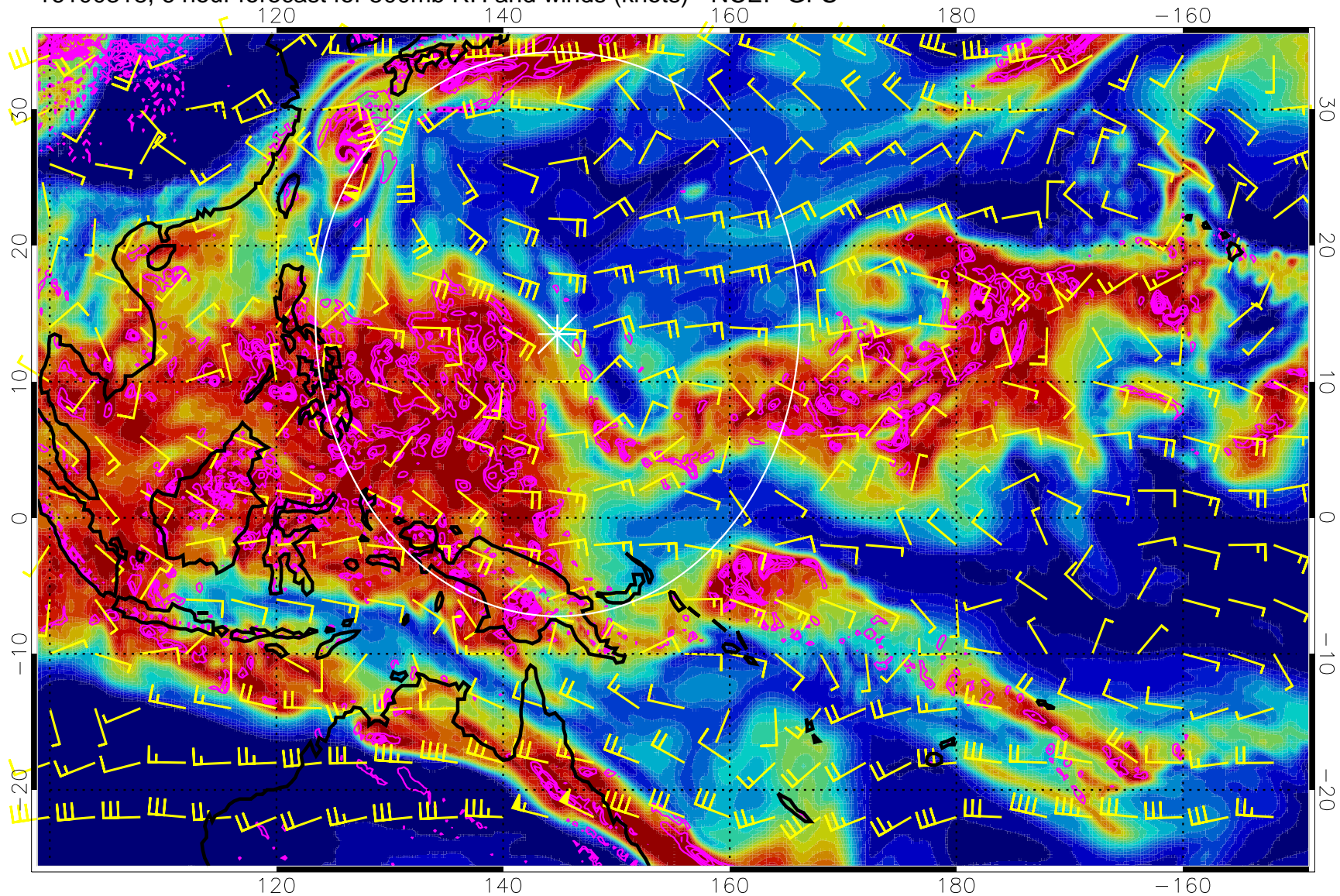
16100318, 6 hour forecast for 500mb RH and winds (knots) - NCEP GFS
