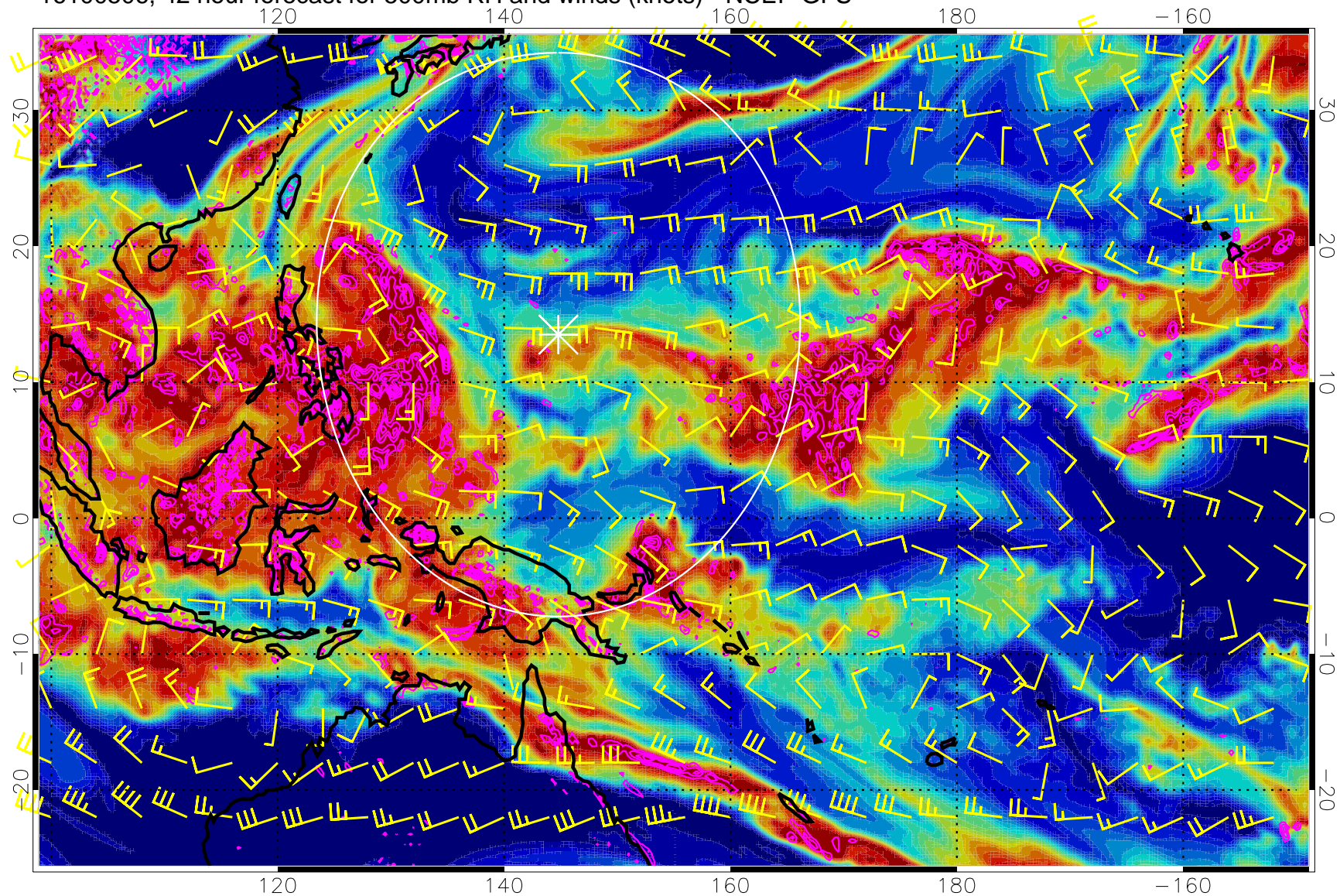
16100506, 42 hour forecast for 500mb RH and winds (knots) - NCEP GFS
