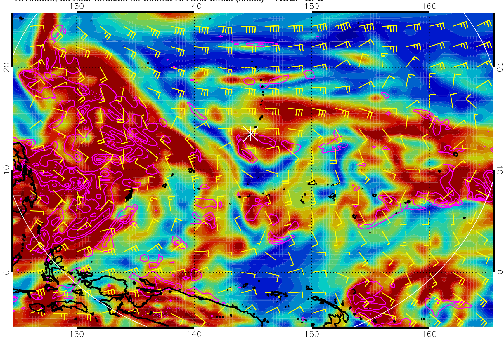
16100500, 36 hour forecast for 300mb RH and winds (knots) -- NCEP GFS
