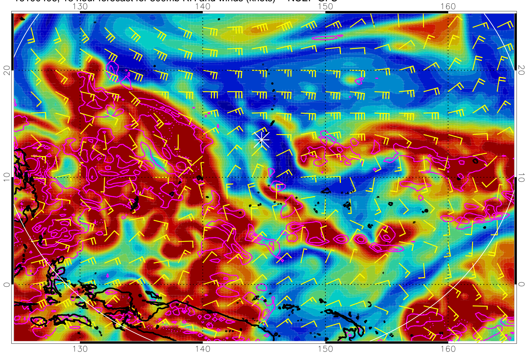
16100406, 18 hour forecast for 300mb RH and winds (knots) -- NCEP GFS
