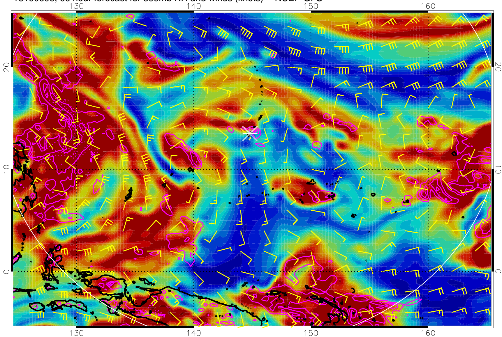
16100606, 66 hour forecast for 300mb RH and winds (knots) -- NCEP GFS
