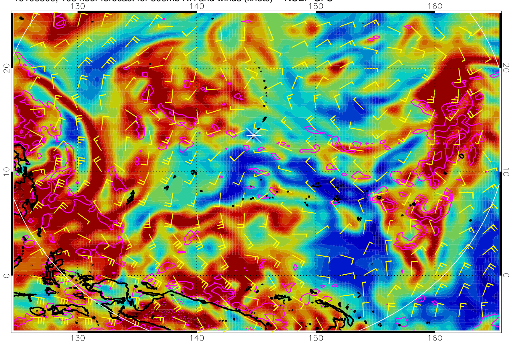
16100800, 108 hour forecast for 300mb RH and winds (knots) -- NCEP GFS
