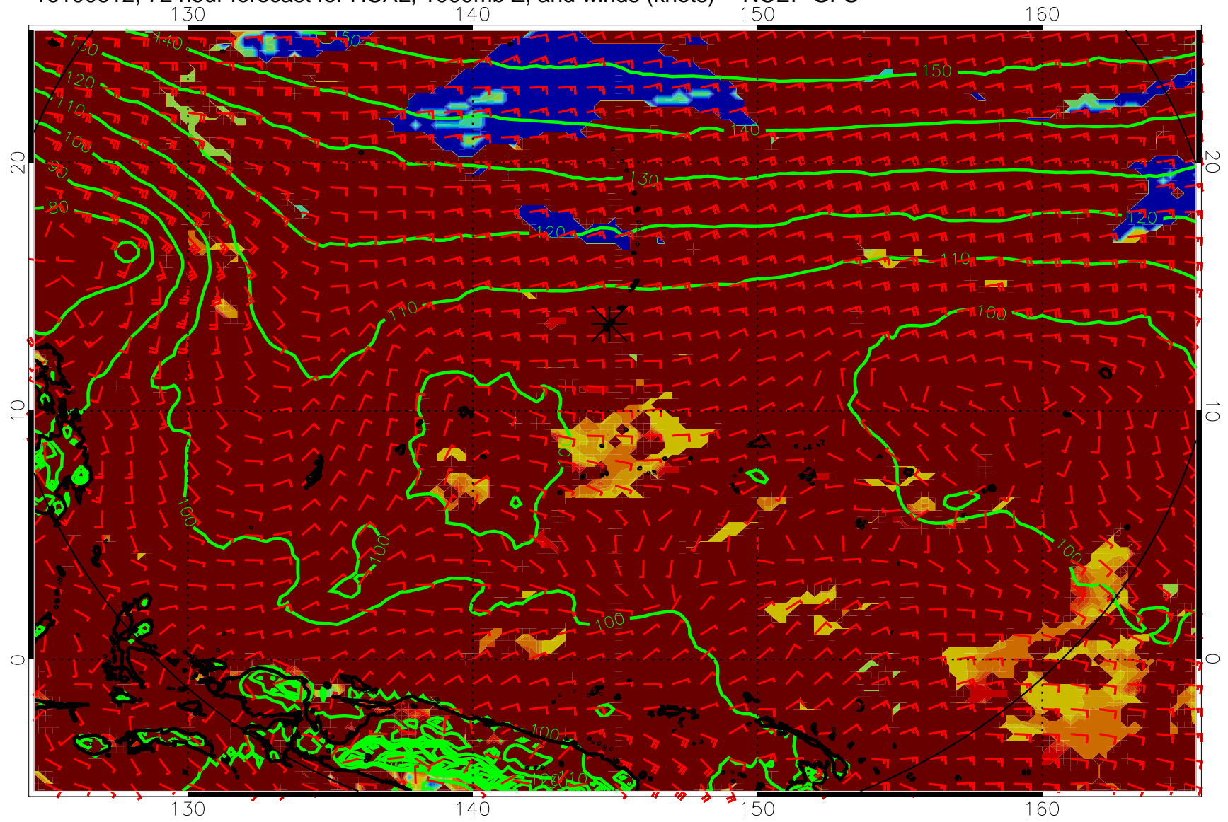
16100612, 72 hour forecast for HCAL, 1000mb Z, and winds (knots) -- NCEP GFS
