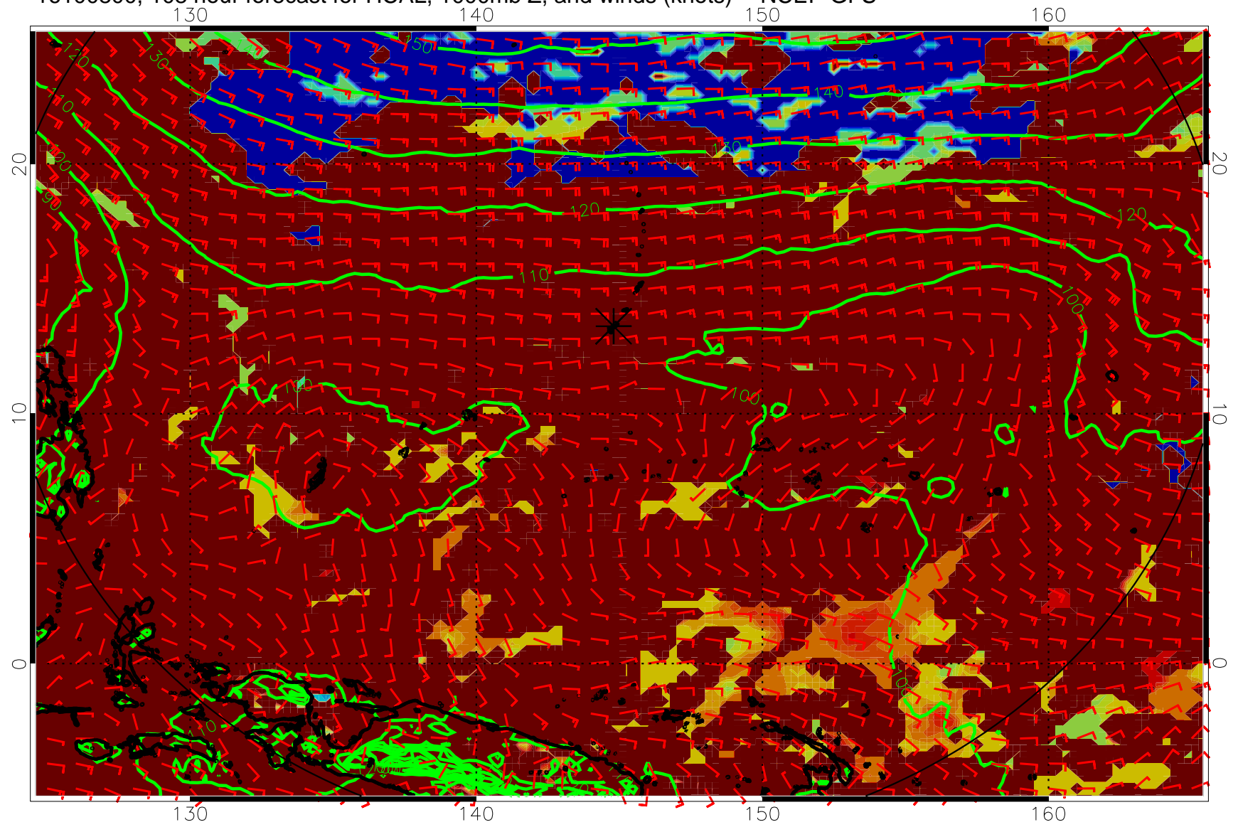
16100800, 108 hour forecast for HCAL, 1000mb Z, and winds (knots) -- NCEP GFS
