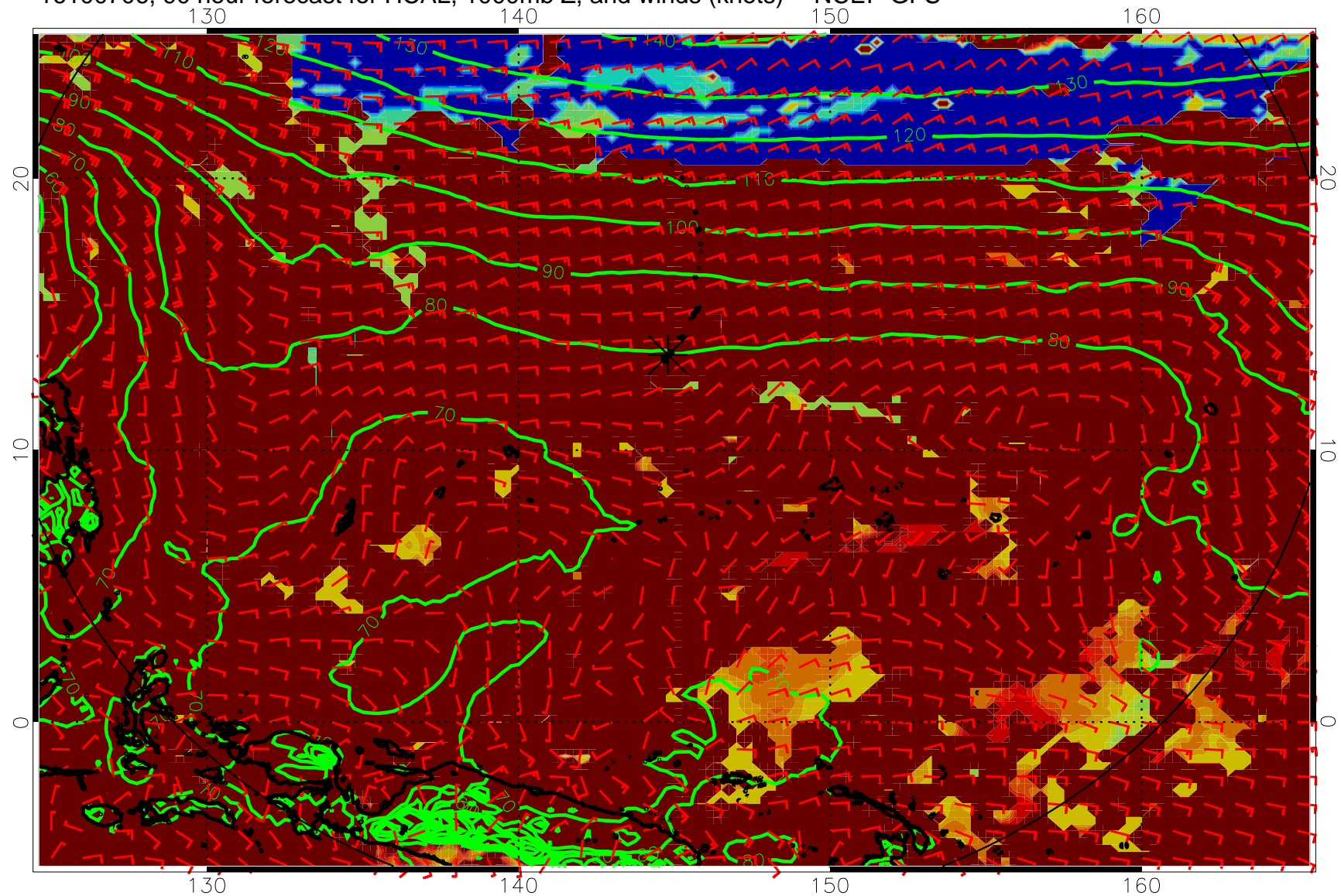
16100706, 90 hour forecast for HCAL, 1000mb Z, and winds (knots) -- NCEP GFS
