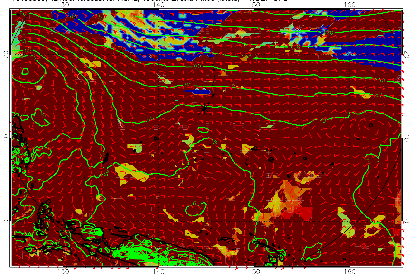
16100506, 42 hour forecast for HCAL, 1000mb Z, and winds (knots) -- NCEP GFS
