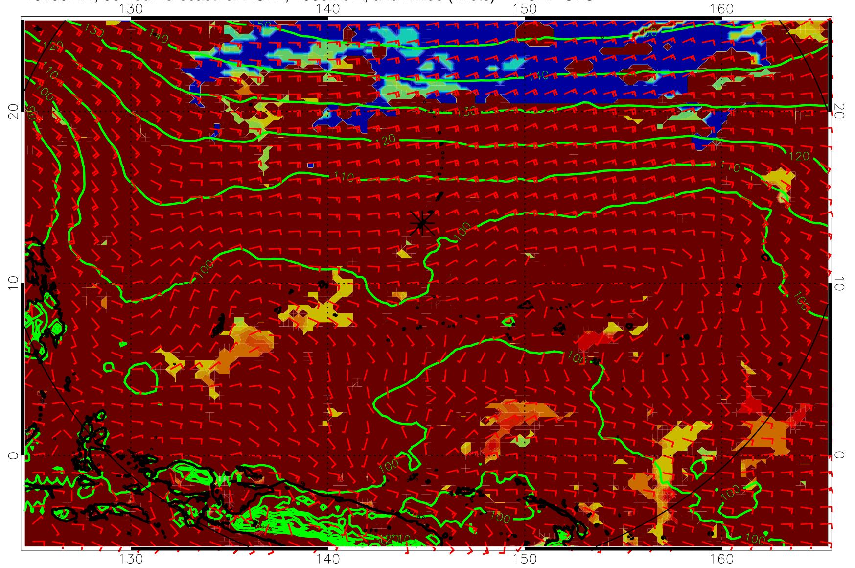
16100712, 96 hour forecast for HCAL, 1000mb Z, and winds (knots) -- NCEP GFS
