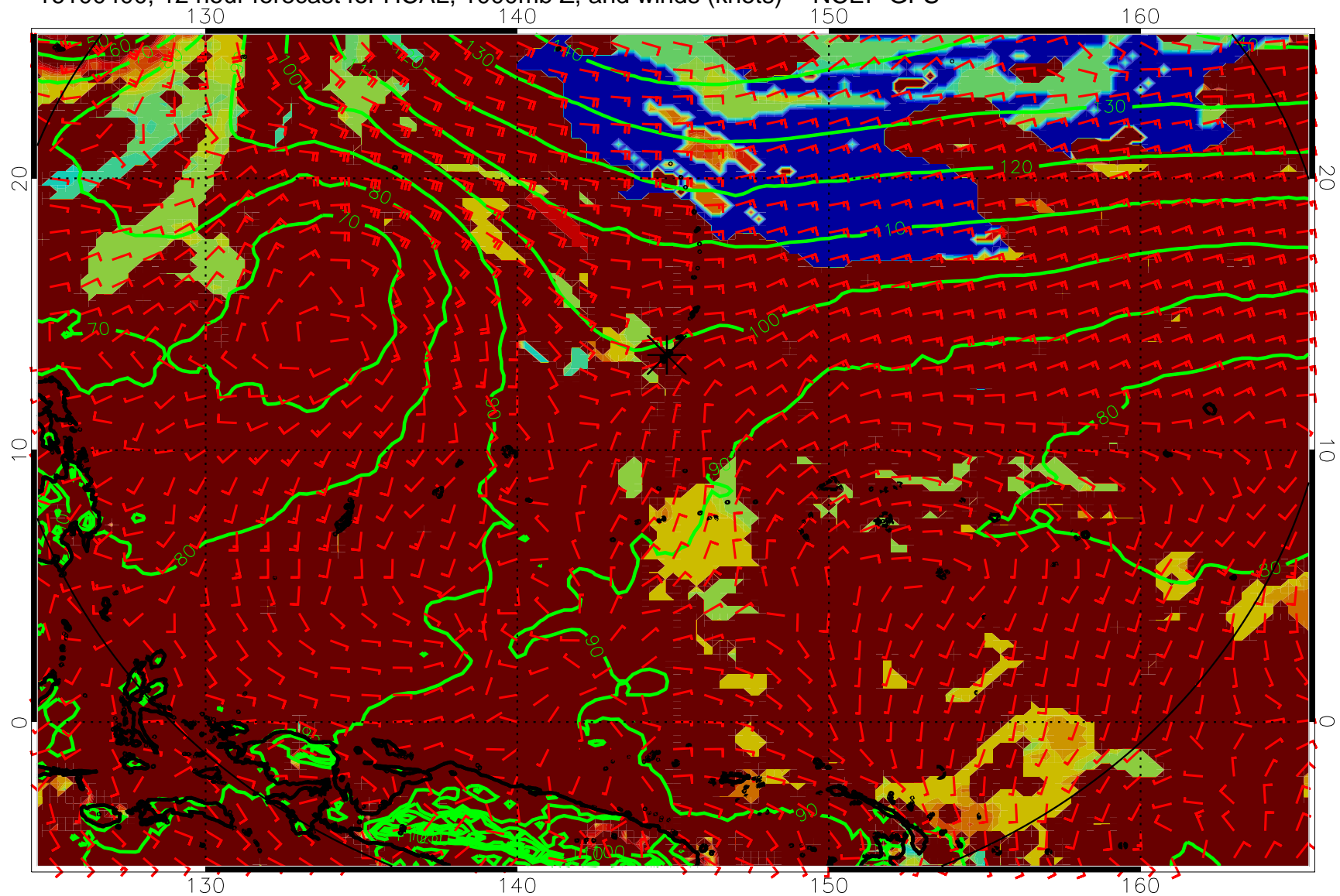
16100400, 12 hour forecast for HCAL, 1000mb Z, and winds (knots) -- NCEP GFS
