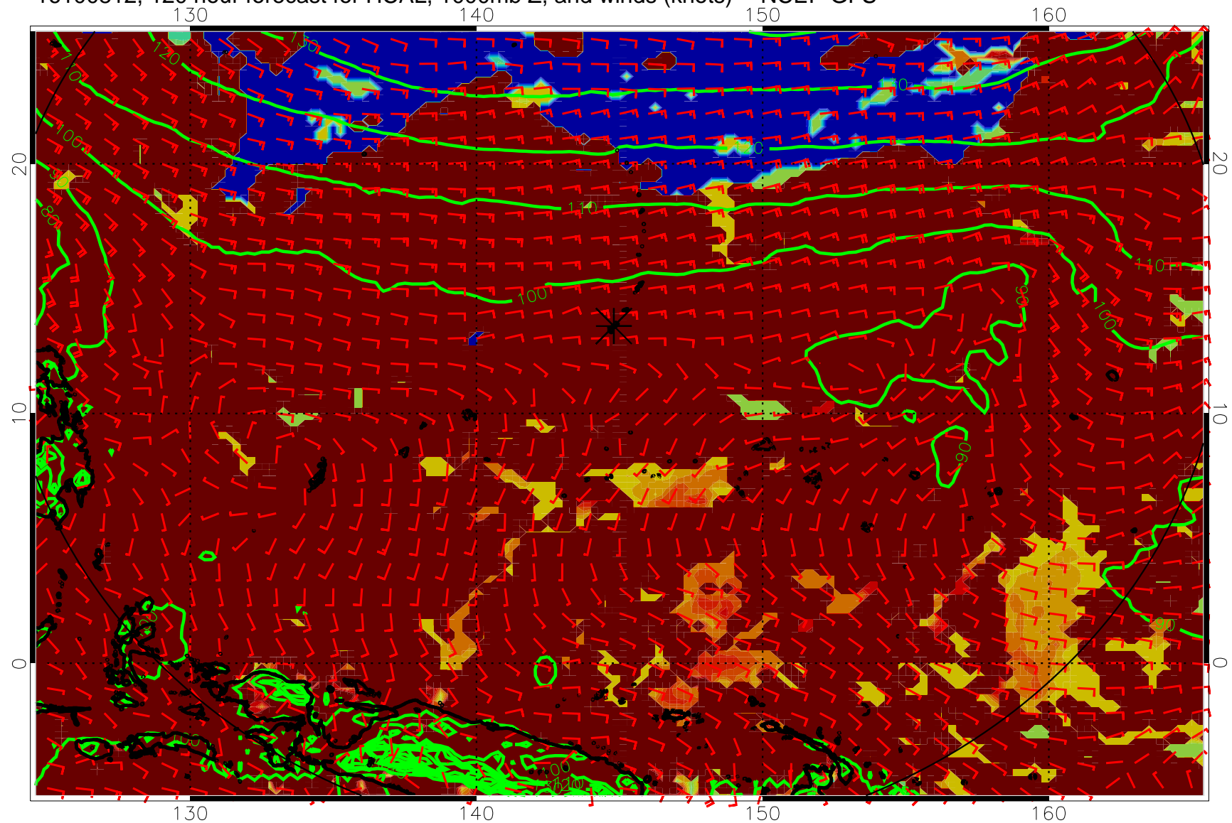
16100812, 120 hour forecast for HCAL, 1000mb Z, and winds (knots) -- NCEP GFS
