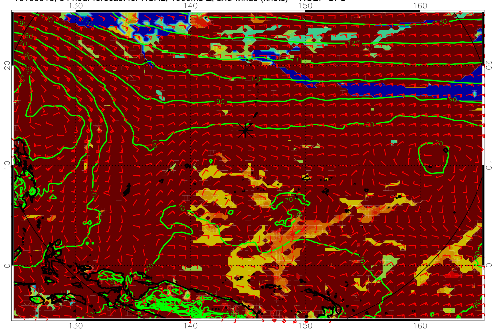
16100518, 54 hour forecast for HCAL, 1000mb Z, and winds (knots) -- NCEP GFS
