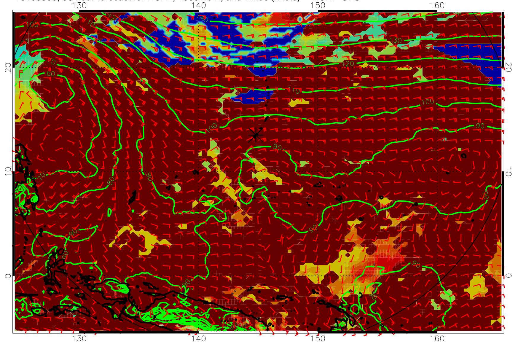
16100500, 36 hour forecast for HCAL, 1000mb Z, and winds (knots) -- NCEP GFS
