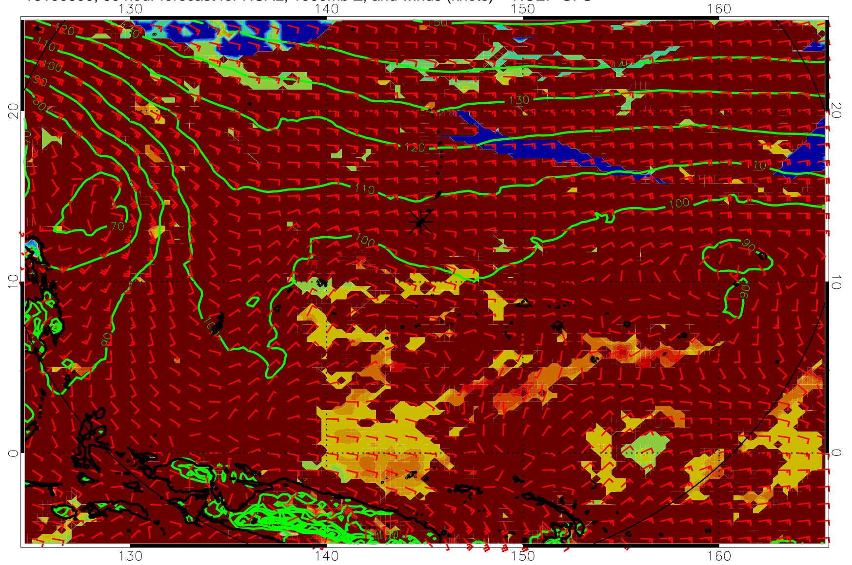
16100600, 60 hour forecast for HCAL, 1000mb Z, and winds (knots) -- NCEP GFS
