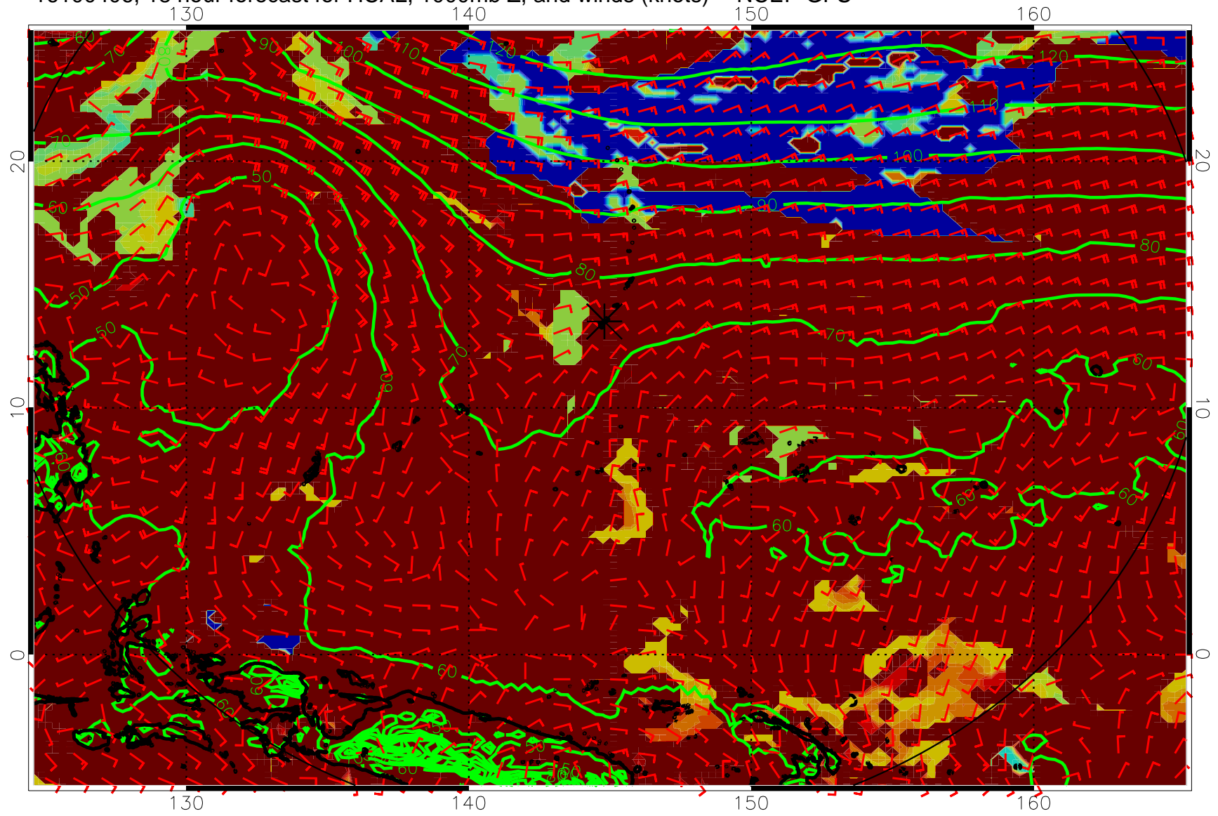
16100406, 18 hour forecast for HCAL, 1000mb Z, and winds (knots) -- NCEP GFS
