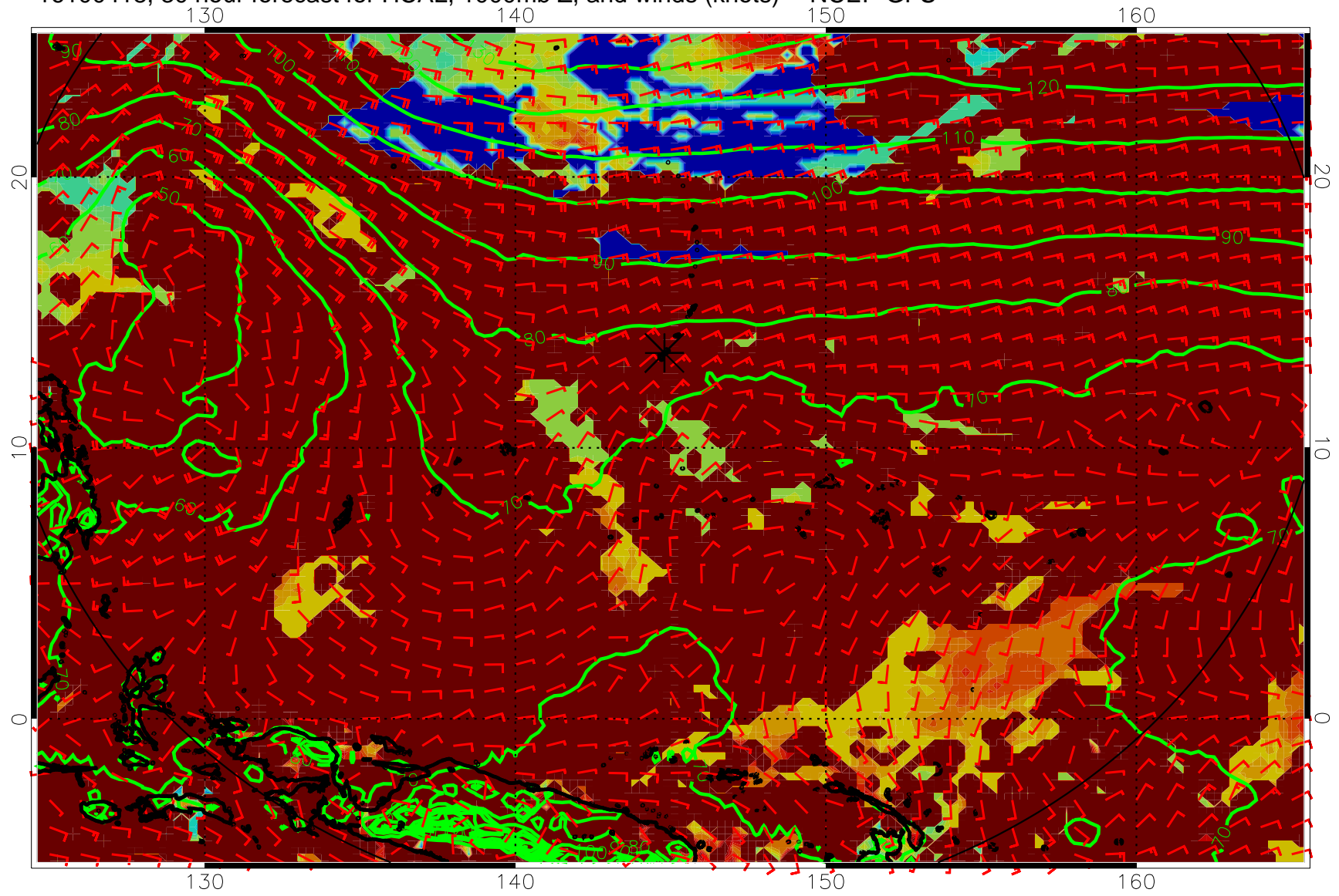
16100418, 30 hour forecast for HCAL, 1000mb Z, and winds (knots) -- NCEP GFS
