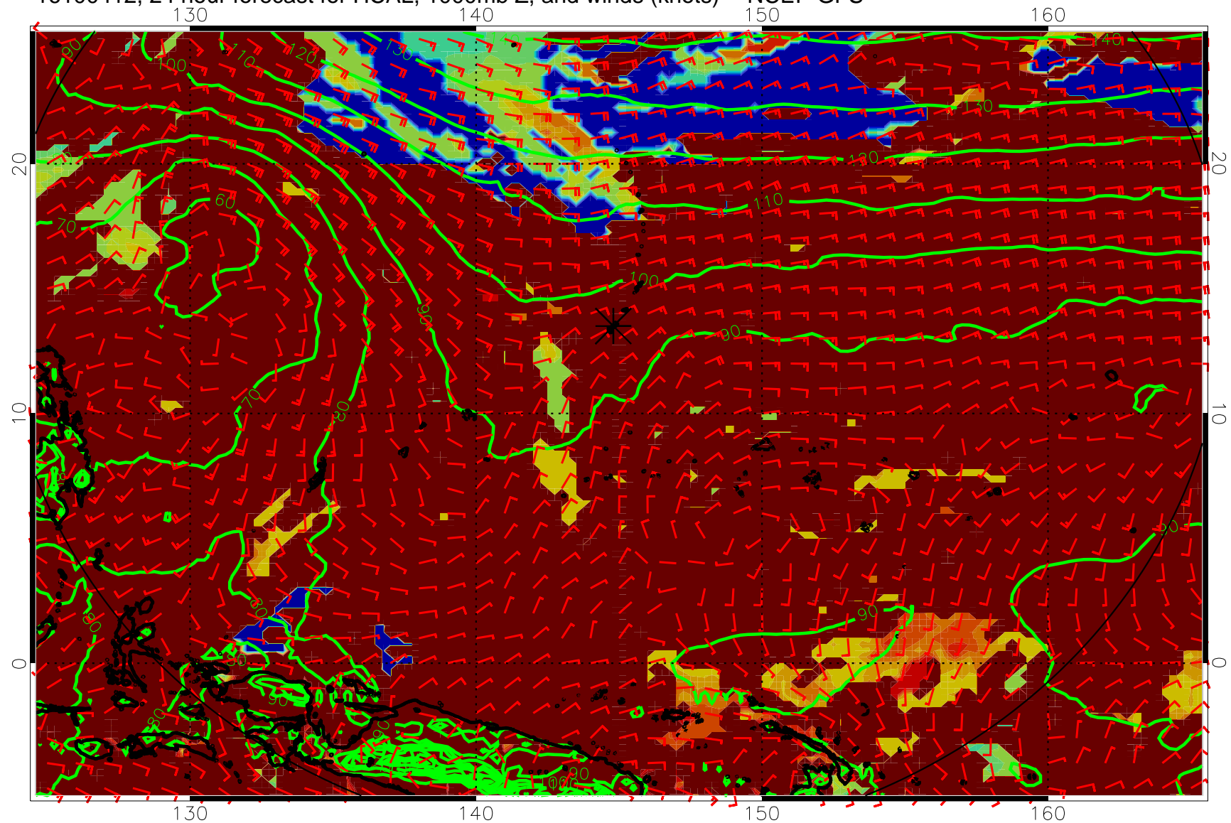
16100412, 24 hour forecast for HCAL, 1000mb Z, and winds (knots) -- NCEP GFS
