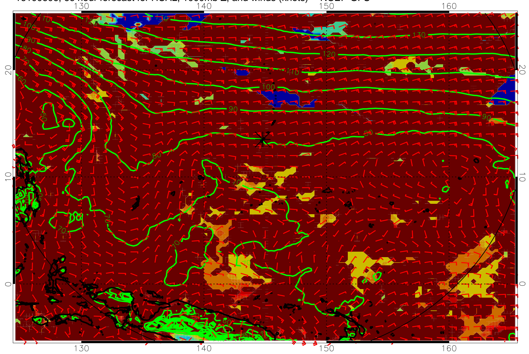
16100606, 66 hour forecast for HCAL, 1000mb Z, and winds (knots) -- NCEP GFS
