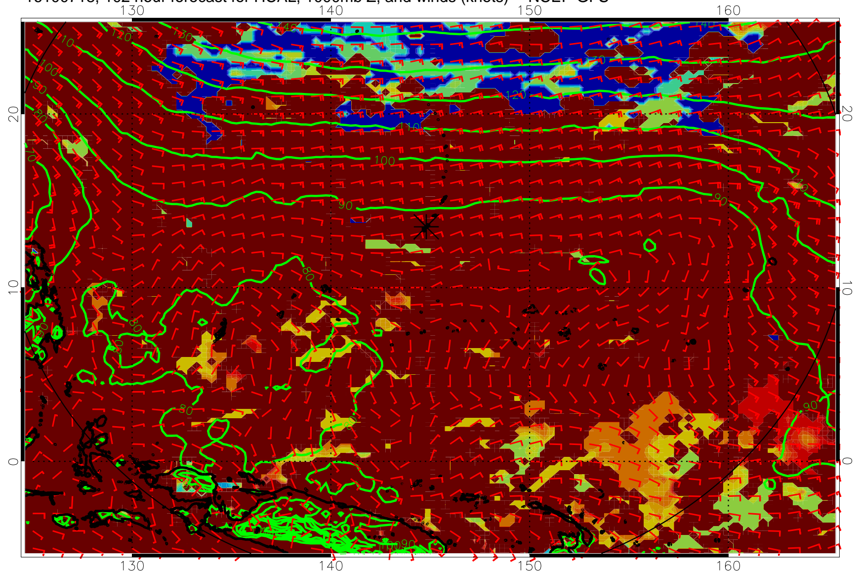
16100718, 102 hour forecast for HCAL, 1000mb Z, and winds (knots) -- NCEP GFS
