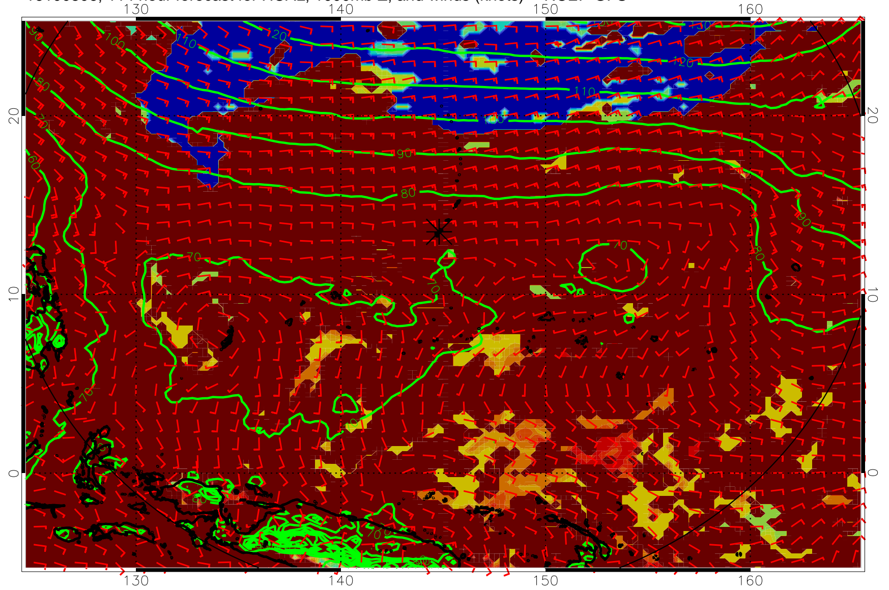
16100806, 114 hour forecast for HCAL, 1000mb Z, and winds (knots) -- NCEP GFS
