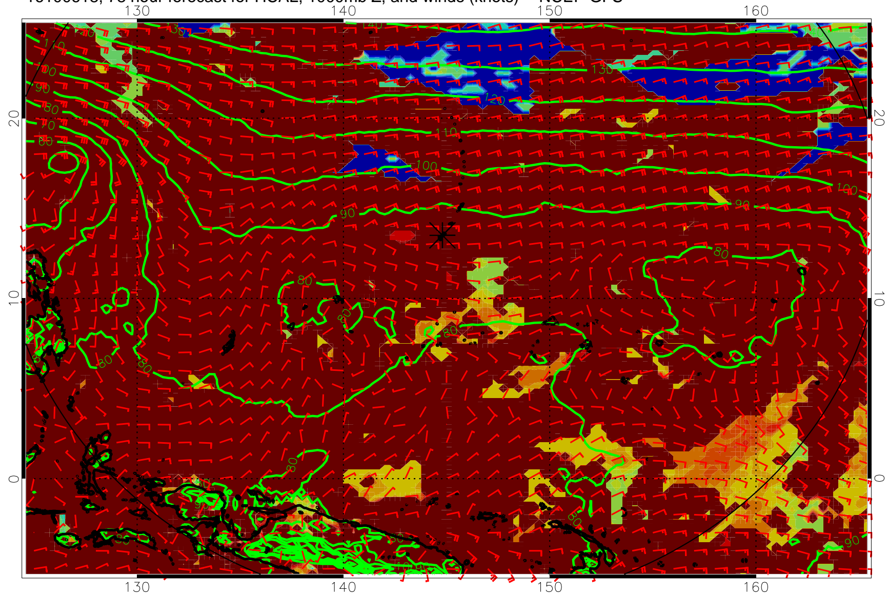
16100618, 78 hour forecast for HCAL, 1000mb Z, and winds (knots) -- NCEP GFS
