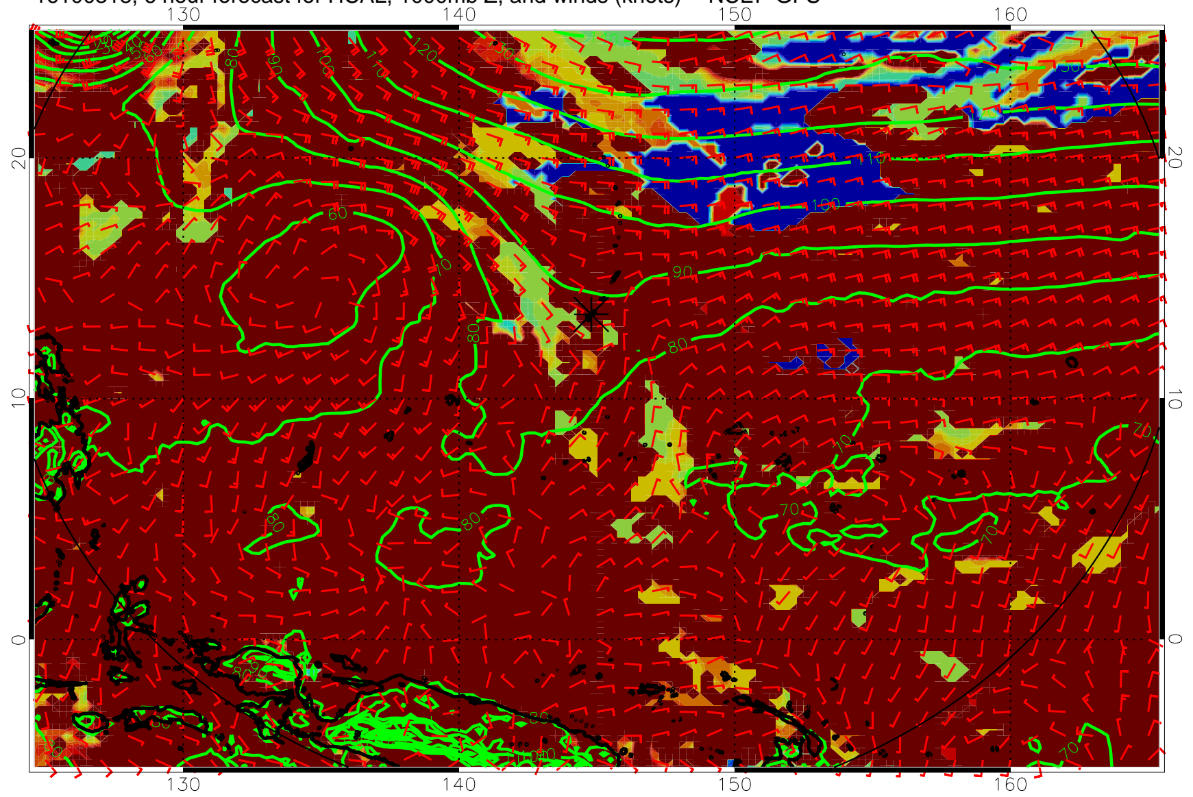
16100318, 6 hour forecast for HCAL, 1000mb Z, and winds (knots) -- NCEP GFS
