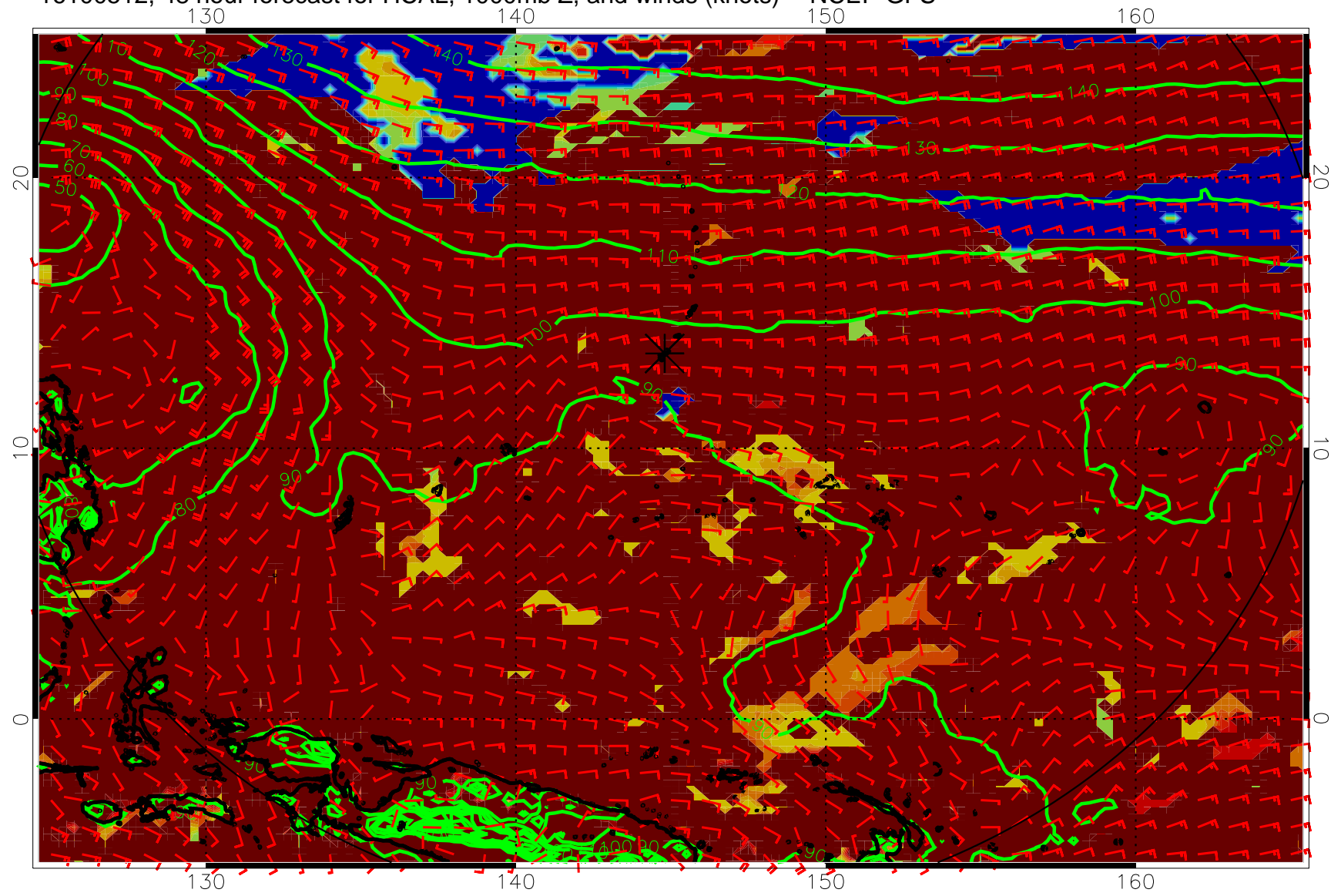
16100512, 48 hour forecast for HCAL, 1000mb Z, and winds (knots) -- NCEP GFS
