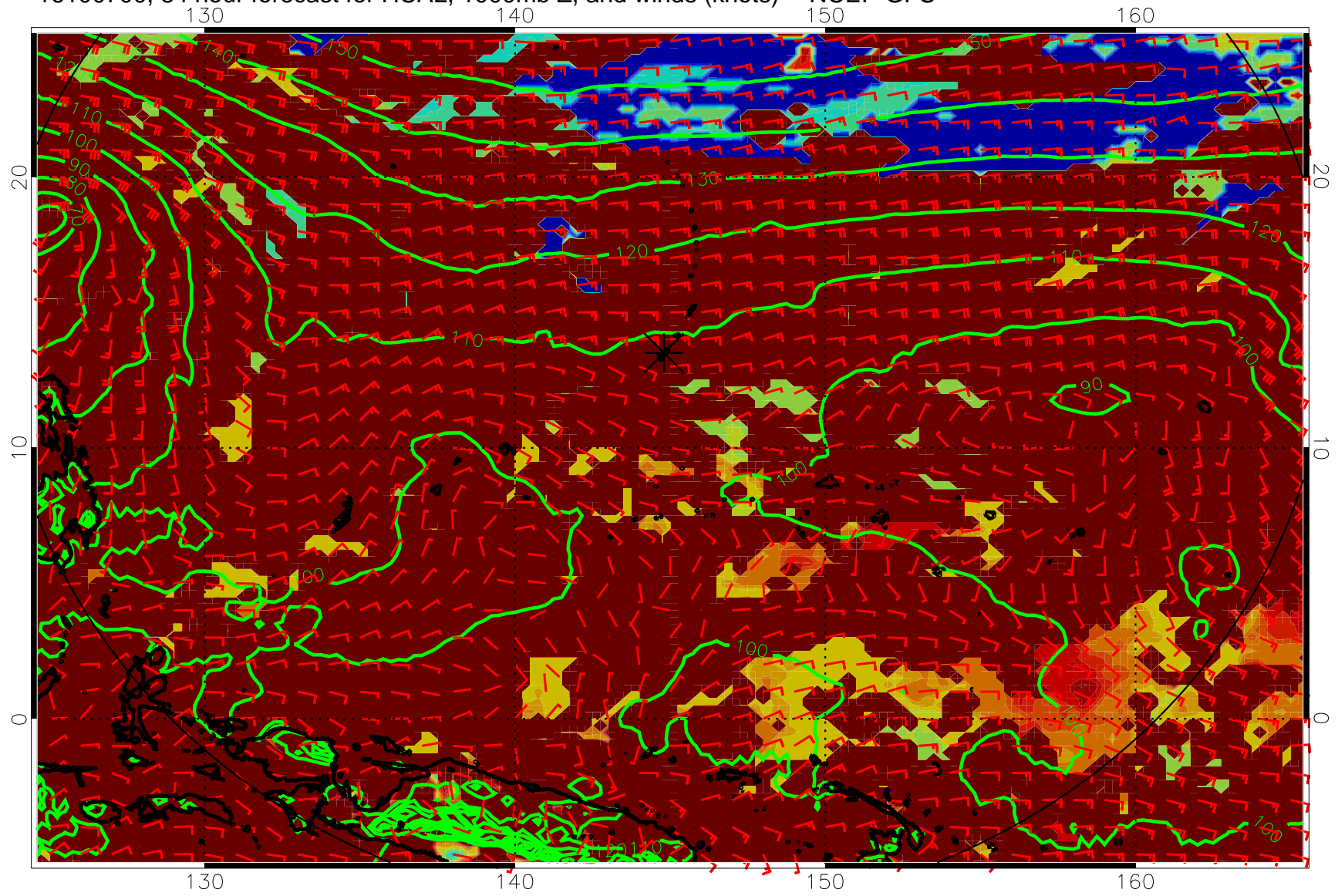
16100700, 84 hour forecast for HCAL, 1000mb Z, and winds (knots) -- NCEP GFS
