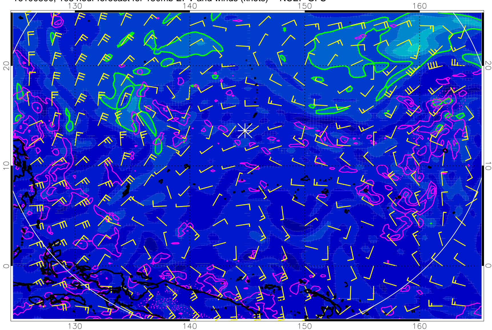
16100800, 108 hour forecast for 150mb EPV and winds (knots) -- NCEP GFS
