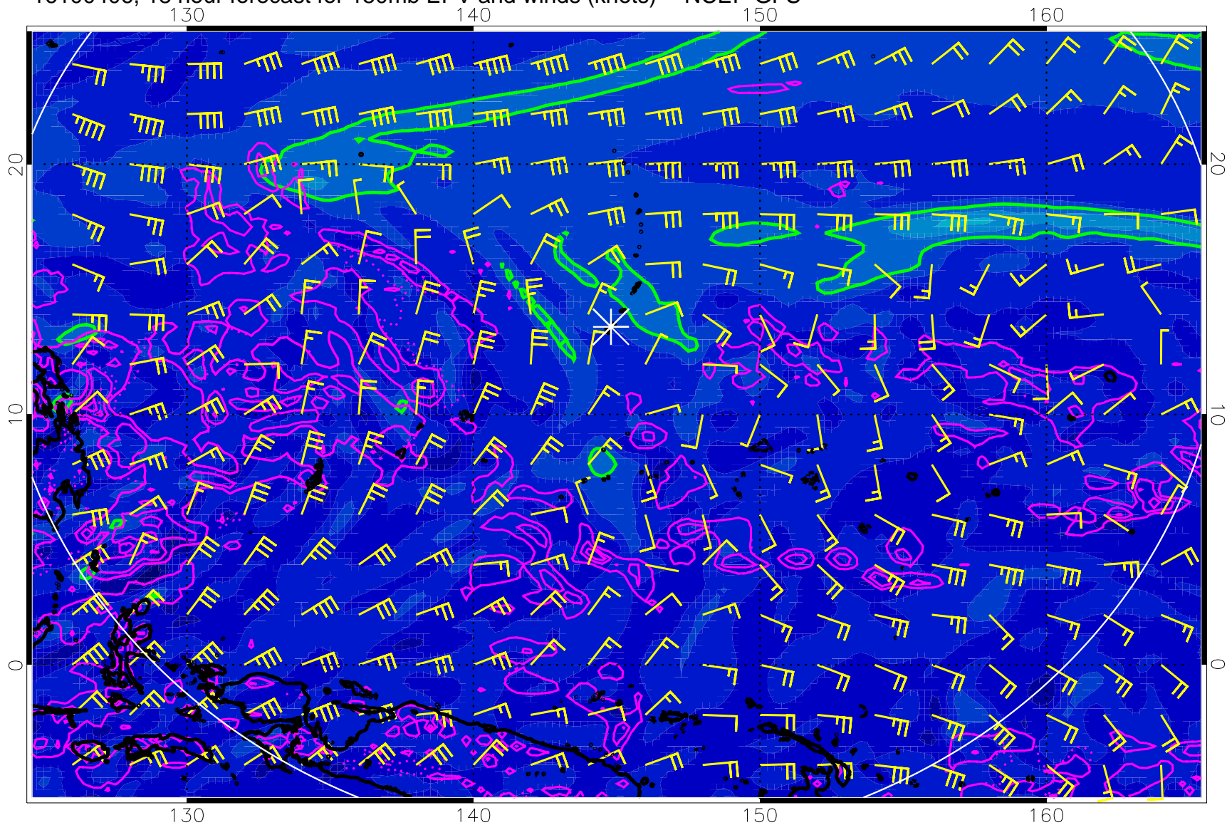
16100406, 18 hour forecast for 150mb EPV and winds (knots) -- NCEP GFS
