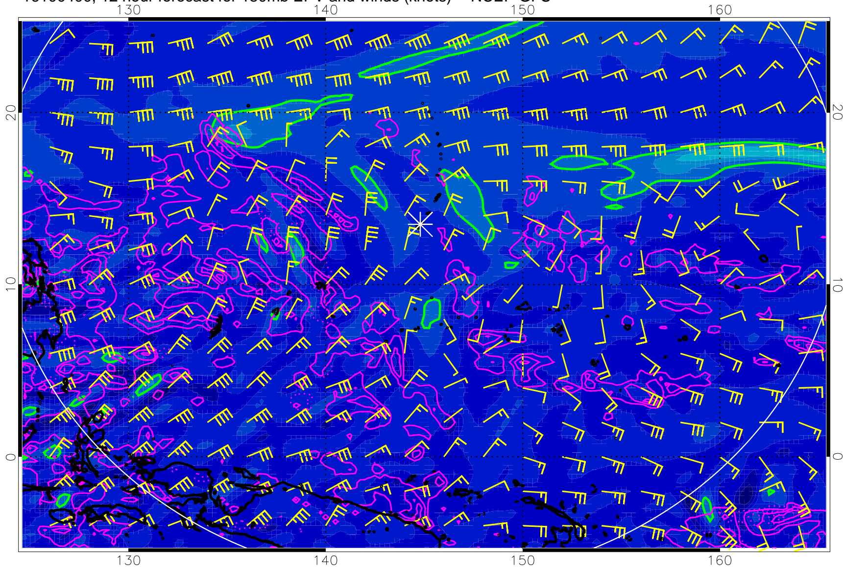
16100400, 12 hour forecast for 150mb EPV and winds (knots) -- NCEP GFS
