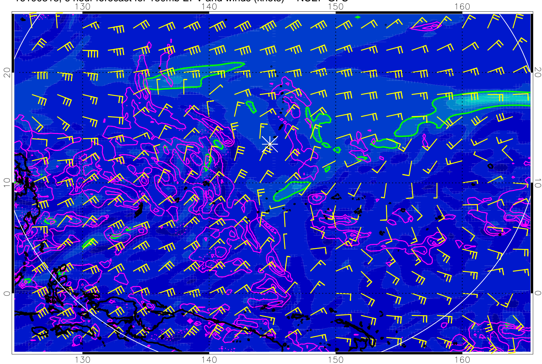
16100318, 6 hour forecast for 150mb EPV and winds (knots) -- NCEP GFS
