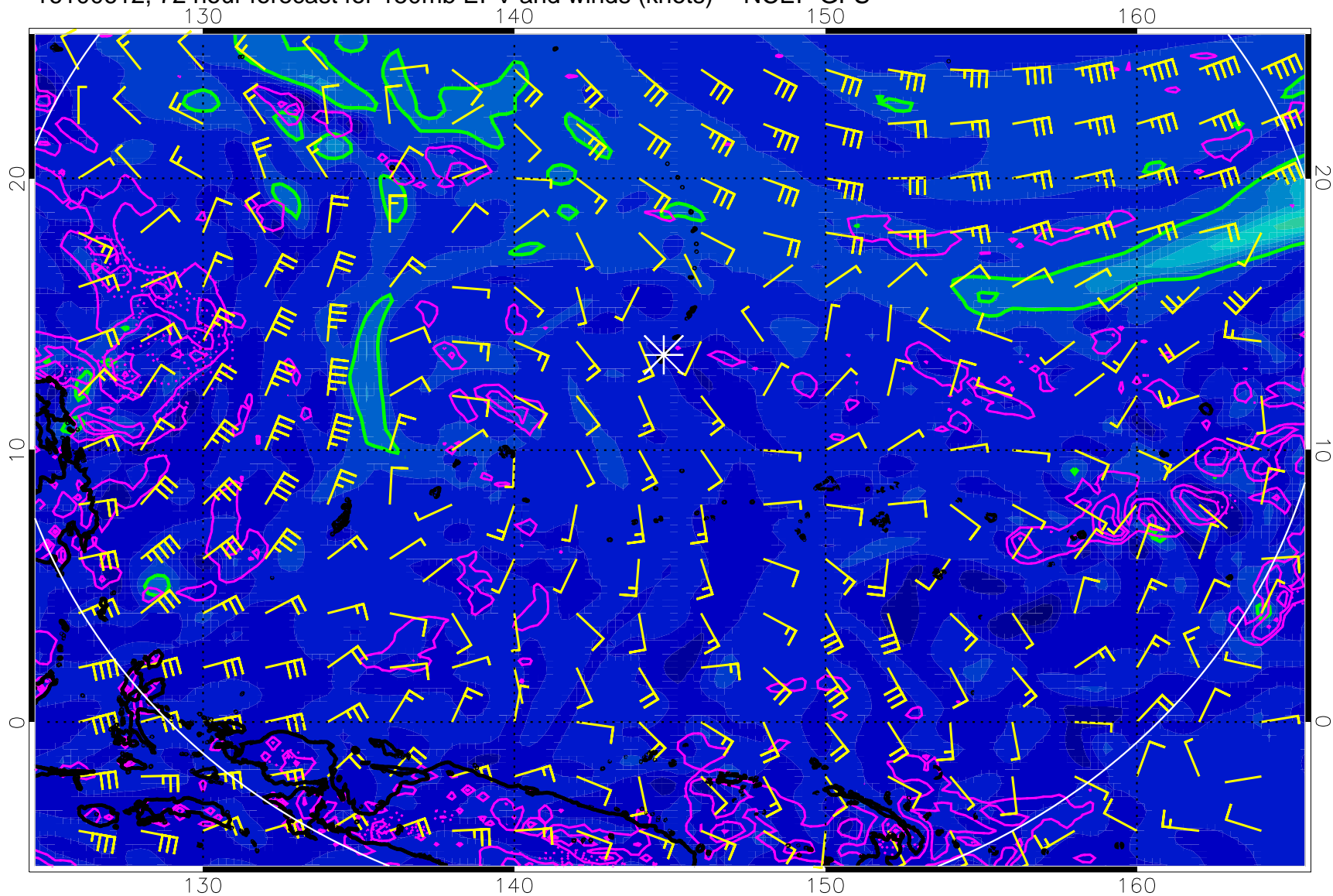
16100612, 72 hour forecast for 150mb EPV and winds (knots) -- NCEP GFS
