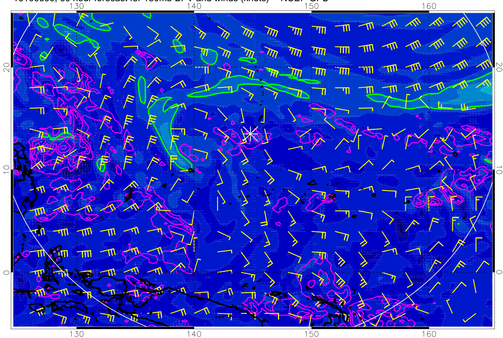
16100600, 60 hour forecast for 150mb EPV and winds (knots) -- NCEP GFS
