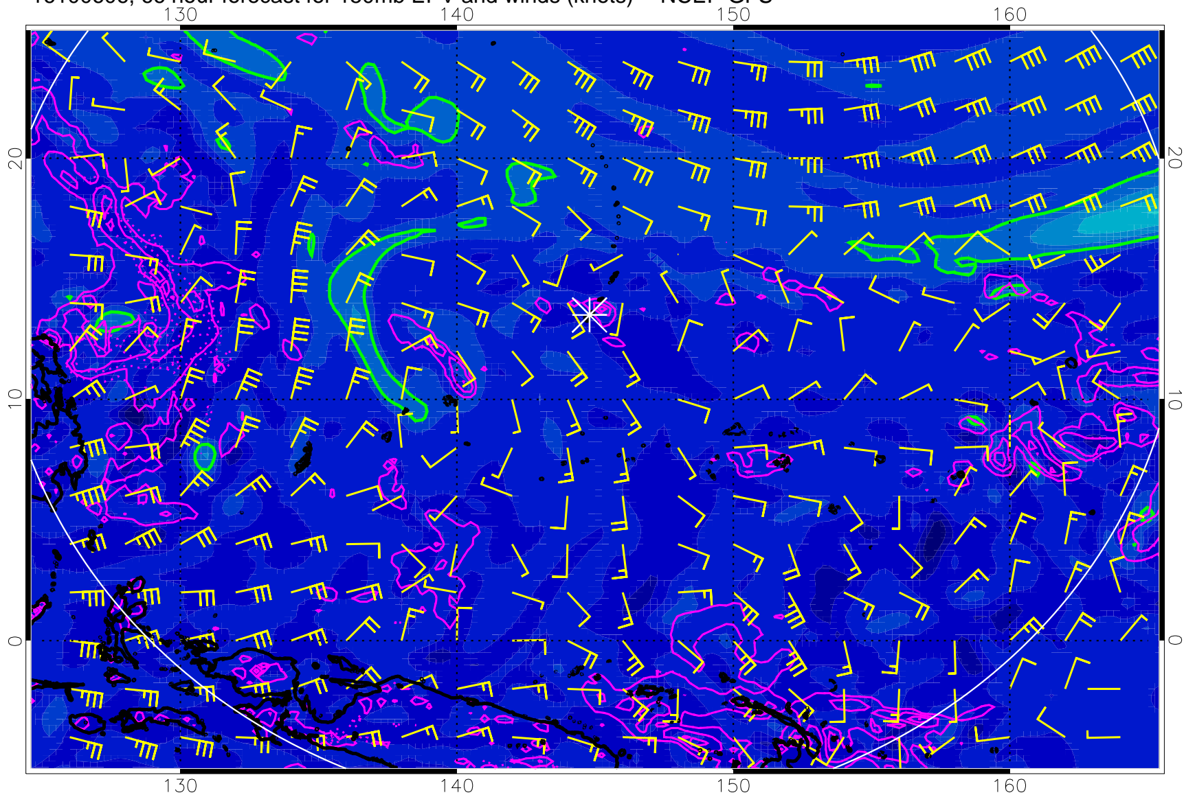
16100606, 66 hour forecast for 150mb EPV and winds (knots) -- NCEP GFS
