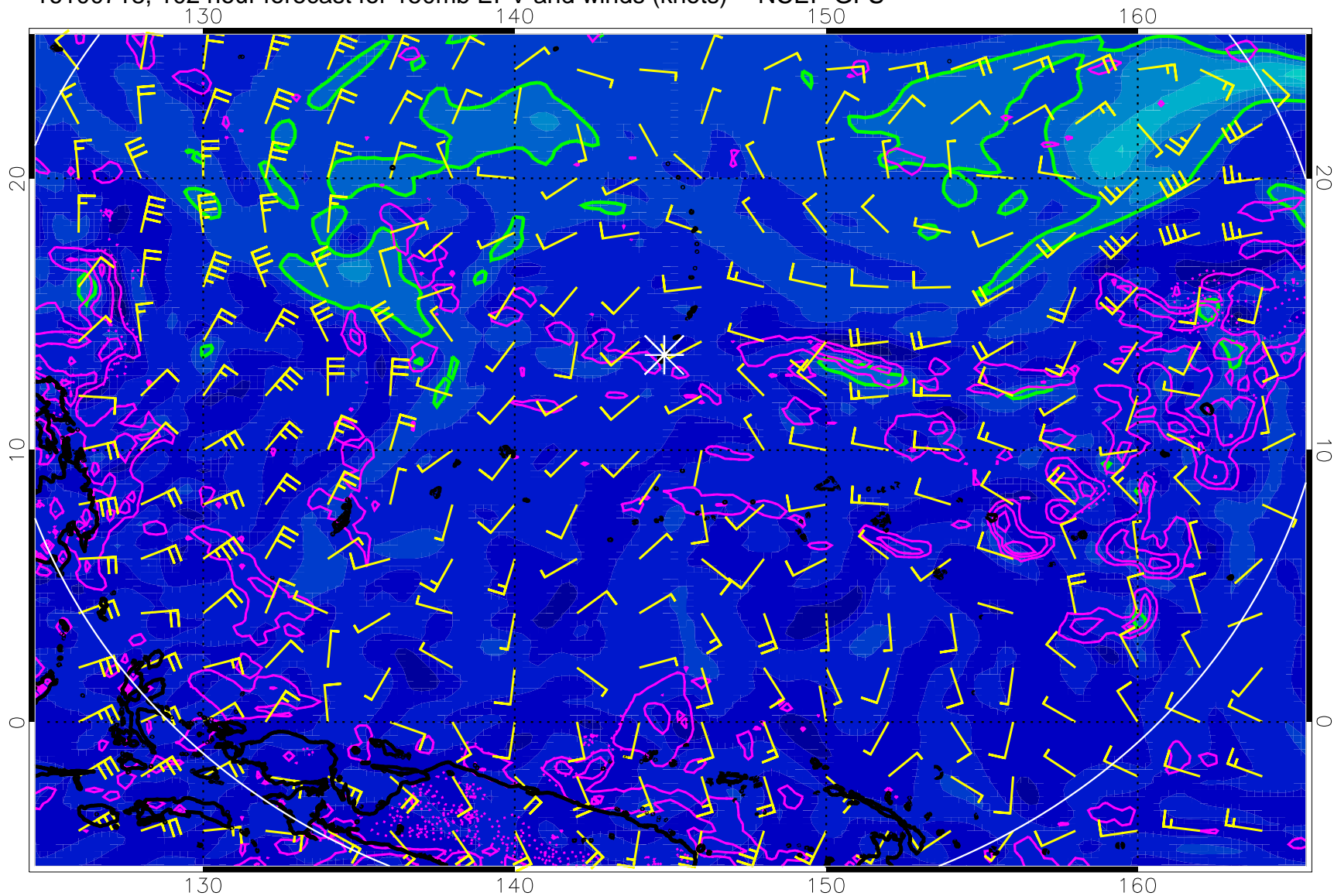
16100718, 102 hour forecast for 150mb EPV and winds (knots) -- NCEP GFS
