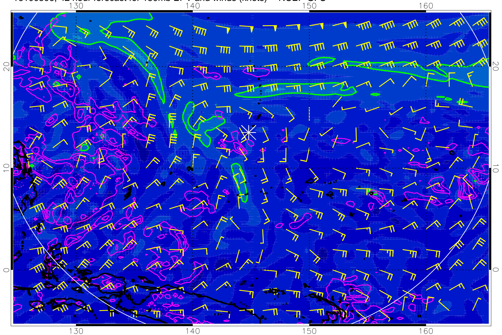
16100506, 42 hour forecast for 150mb EPV and winds (knots) -- NCEP GFS
