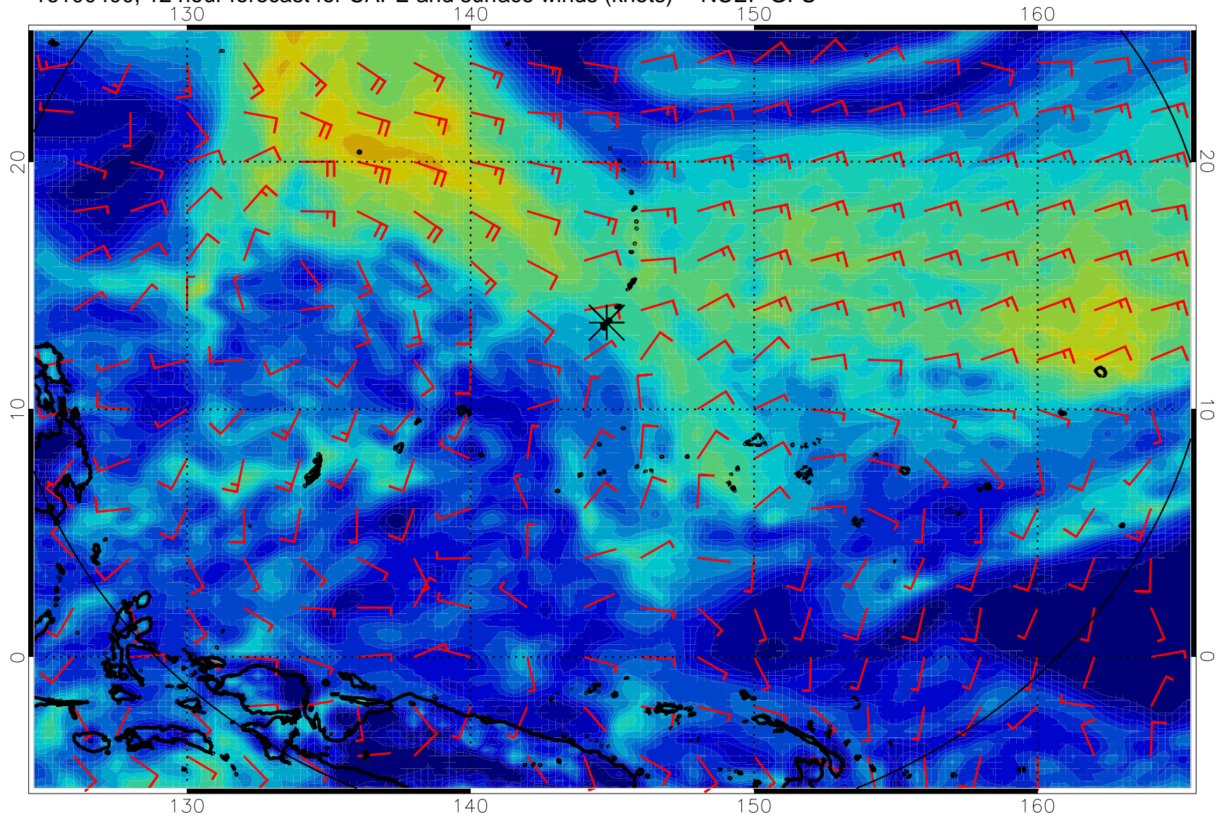
16100400, 12 hour forecast for CAPE and surface winds (knots) -- NCEP GFS
