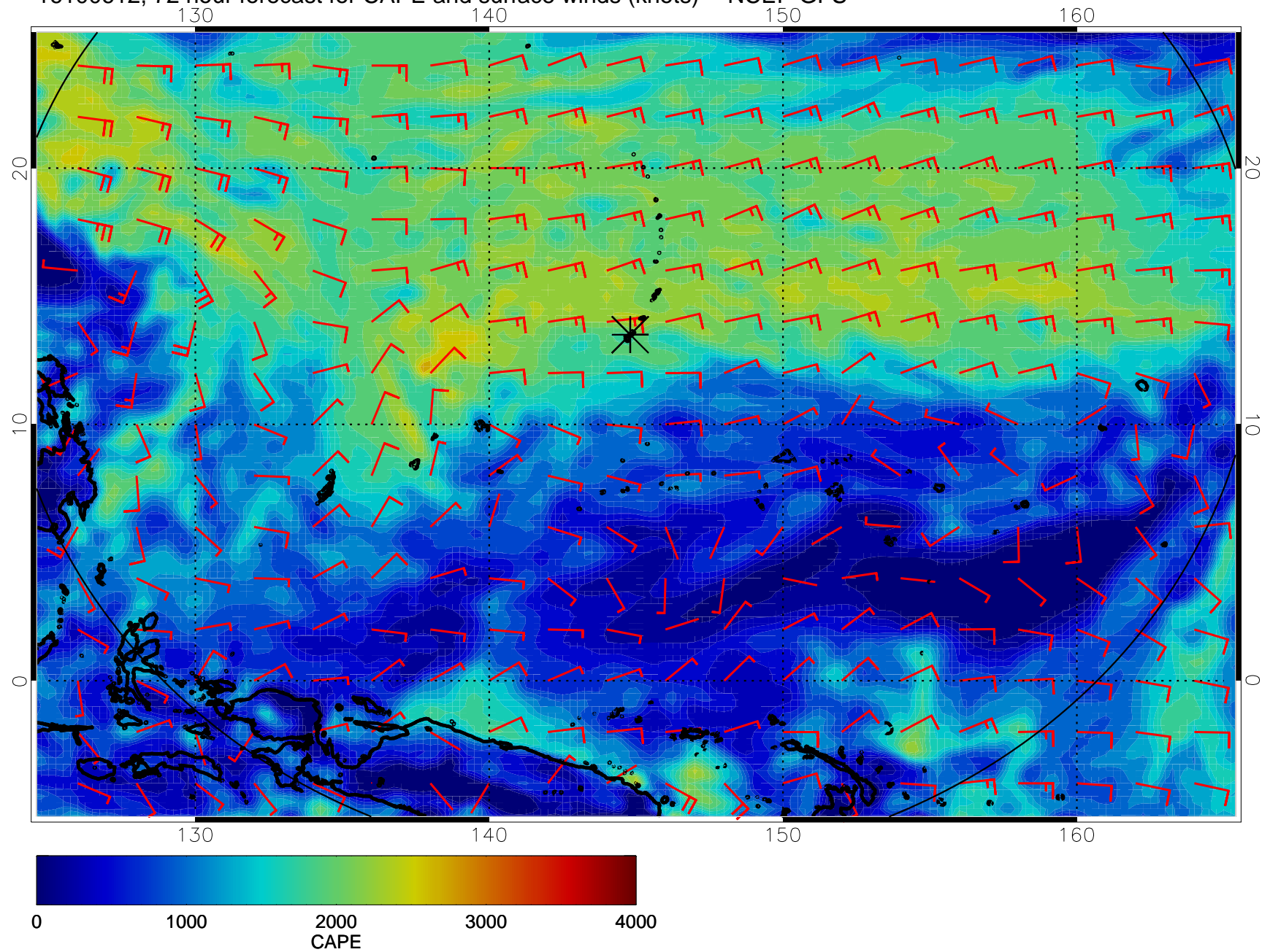
16100612, 72 hour forecast for CAPE and surface winds (knots) -- NCEP GFS
