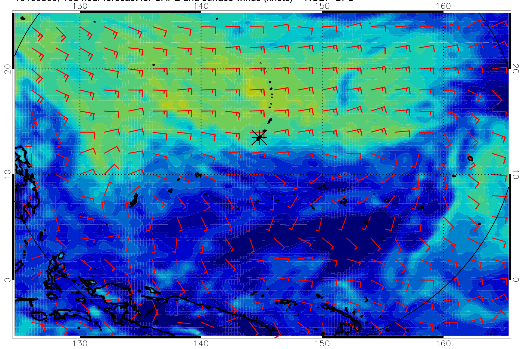
16100800, 108 hour forecast for CAPE and surface winds (knots) -- NCEP GFS
