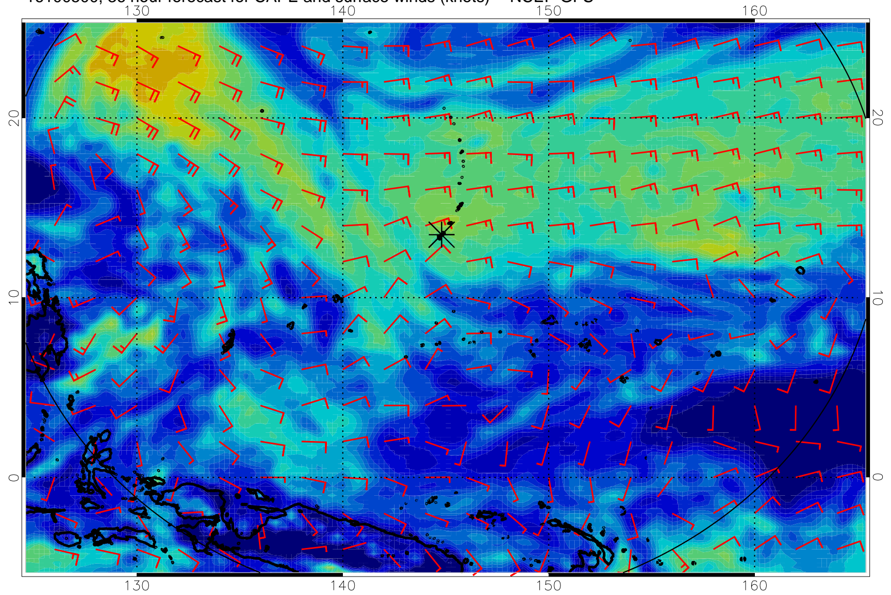
16100500, 36 hour forecast for CAPE and surface winds (knots) -- NCEP GFS
