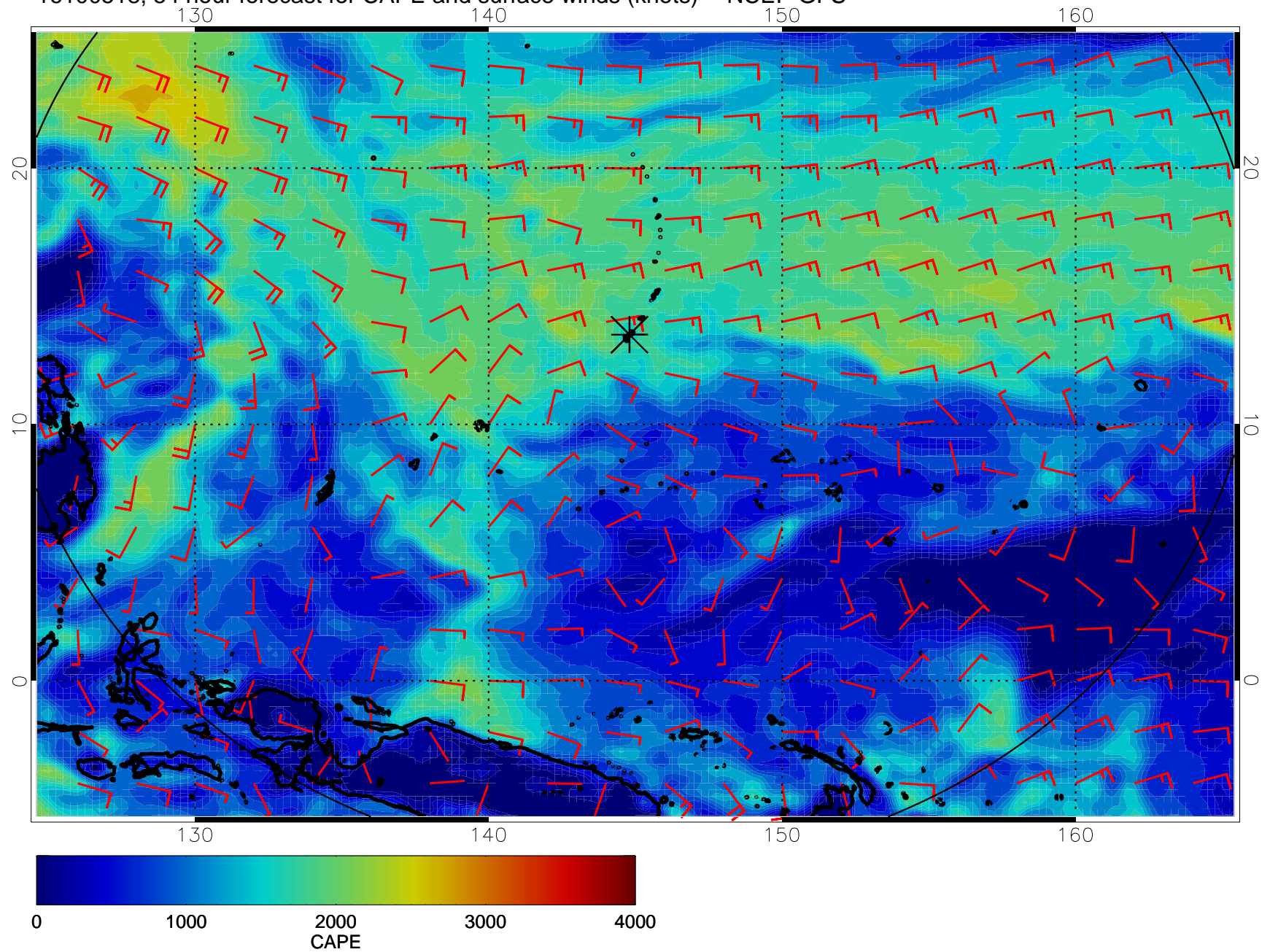
16100518, 54 hour forecast for CAPE and surface winds (knots) -- NCEP GFS
