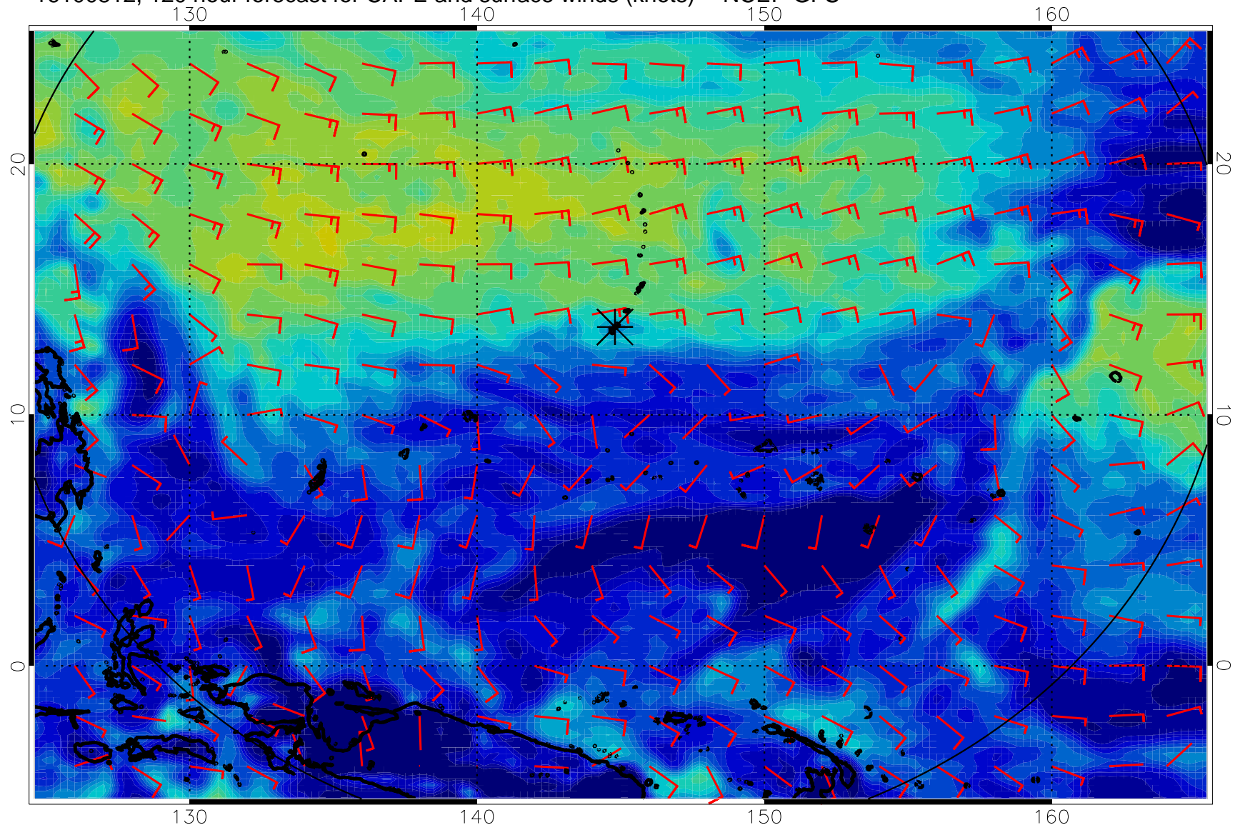
16100812, 120 hour forecast for CAPE and surface winds (knots) -- NCEP GFS
