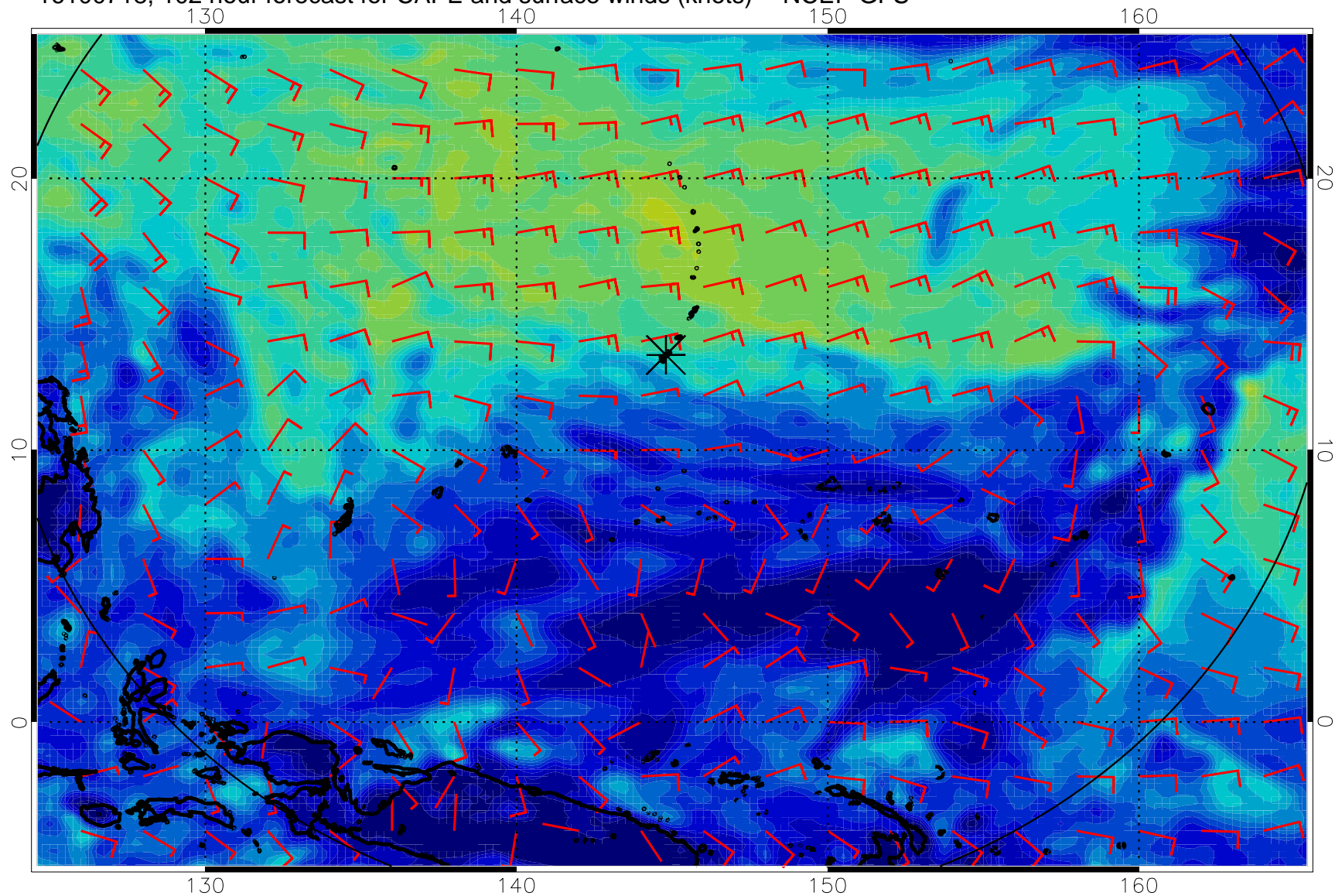
16100718, 102 hour forecast for CAPE and surface winds (knots) -- NCEP GFS
