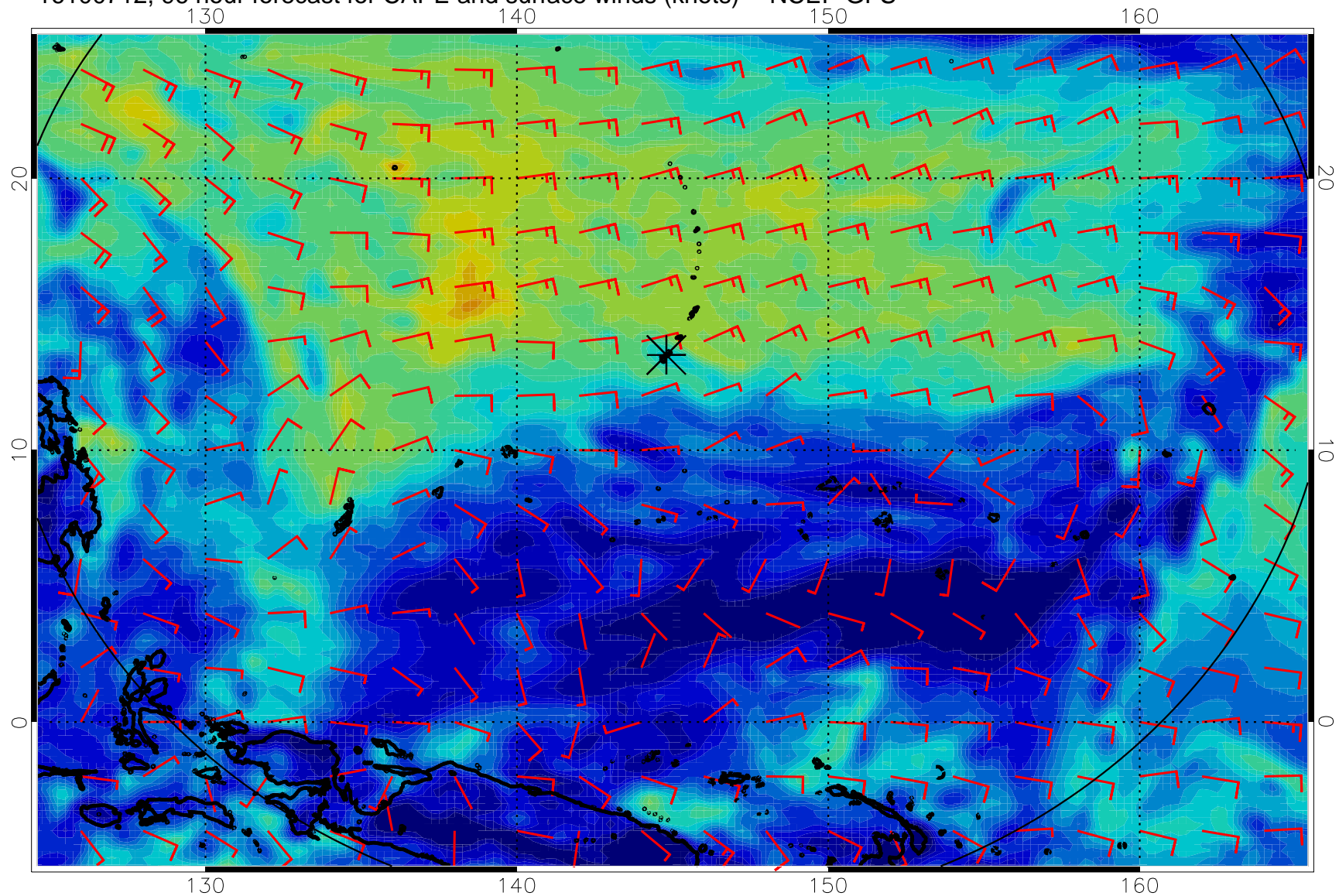
16100712, 96 hour forecast for CAPE and surface winds (knots) -- NCEP GFS
