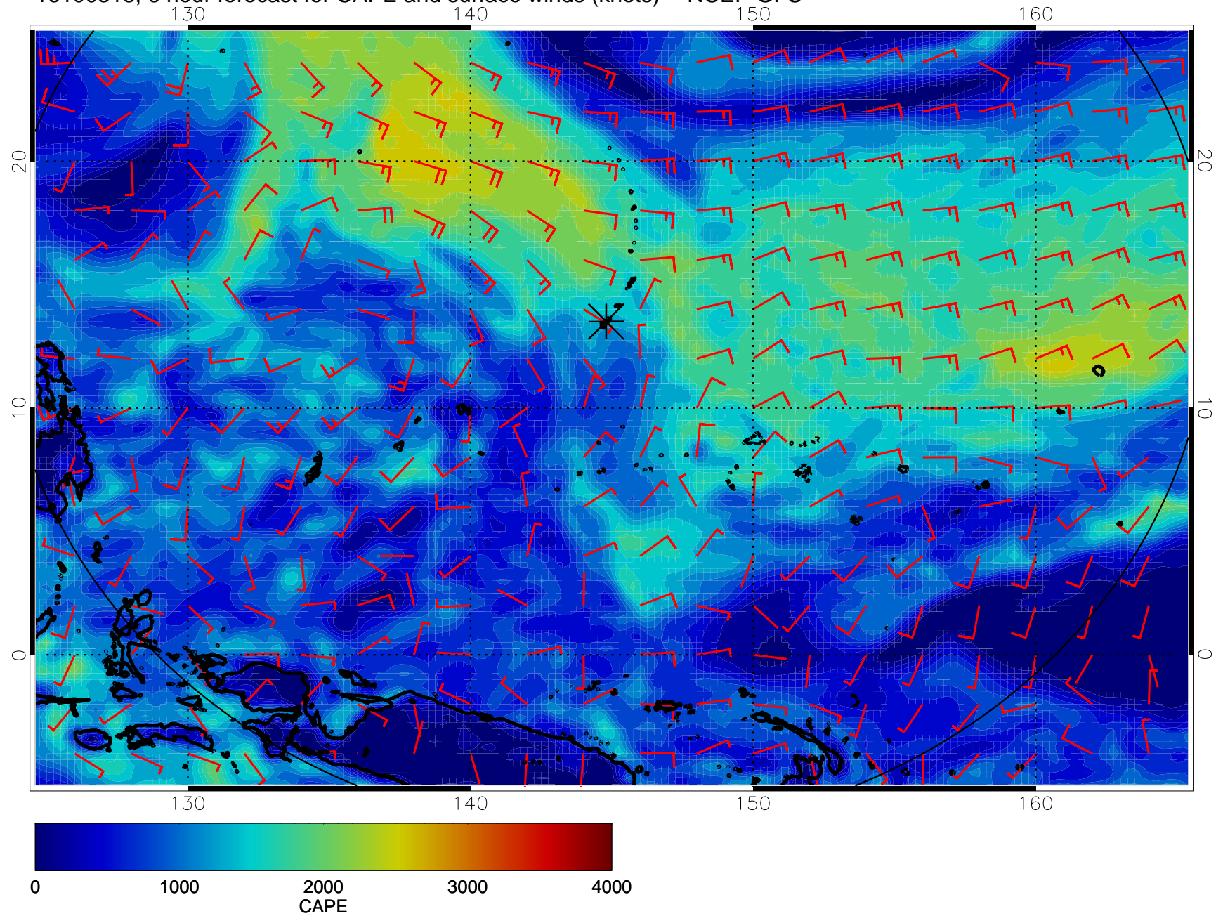
16100318, 6 hour forecast for CAPE and surface winds (knots) -- NCEP GFS
