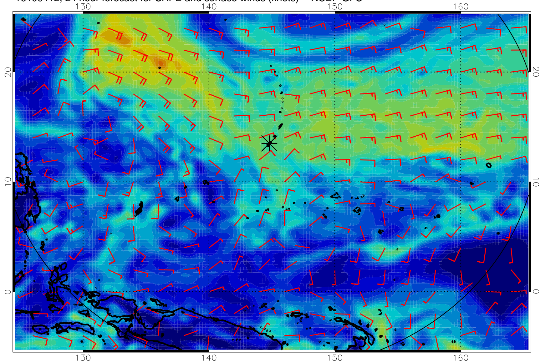
16100412, 24 hour forecast for CAPE and surface winds (knots) -- NCEP GFS
