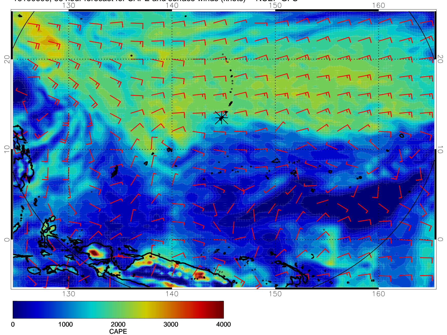
16100606, 66 hour forecast for CAPE and surface winds (knots) -- NCEP GFS
