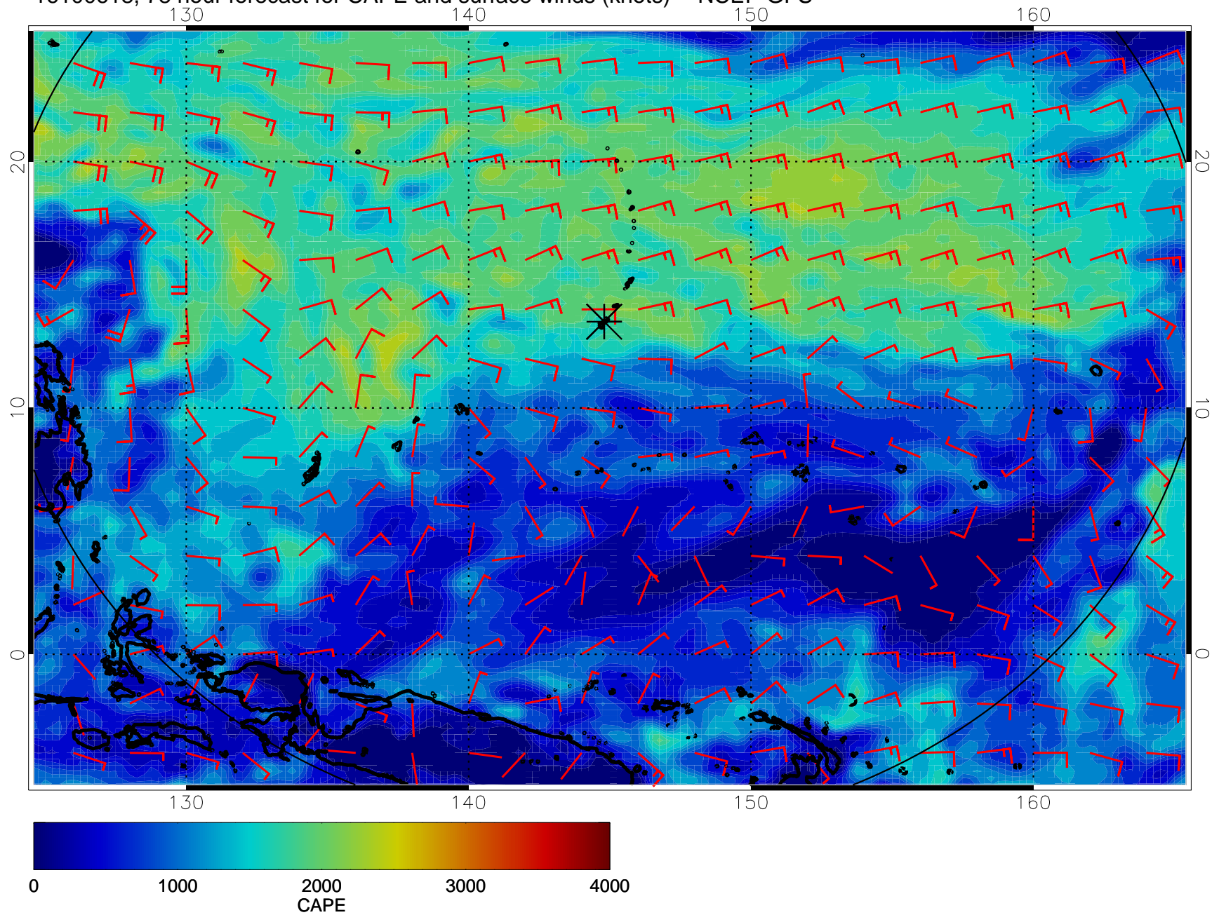
16100618, 78 hour forecast for CAPE and surface winds (knots) -- NCEP GFS
