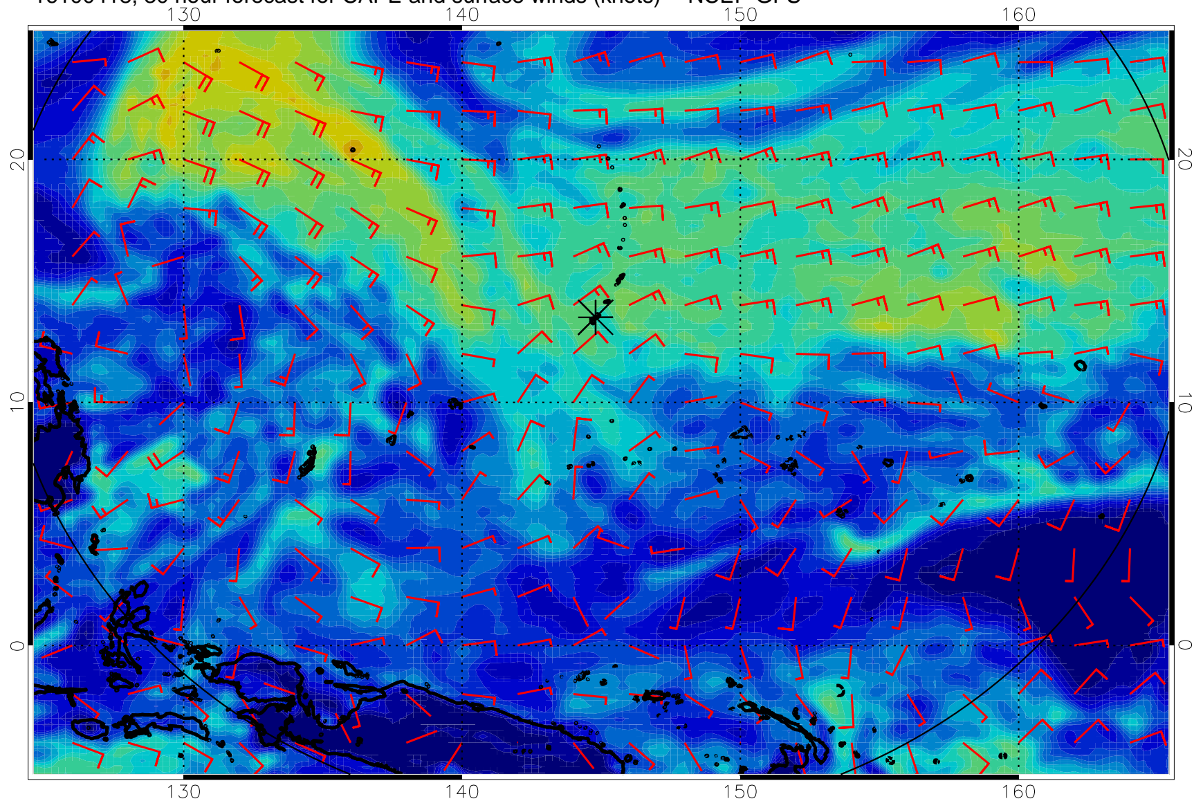
16100418, 30 hour forecast for CAPE and surface winds (knots) -- NCEP GFS
