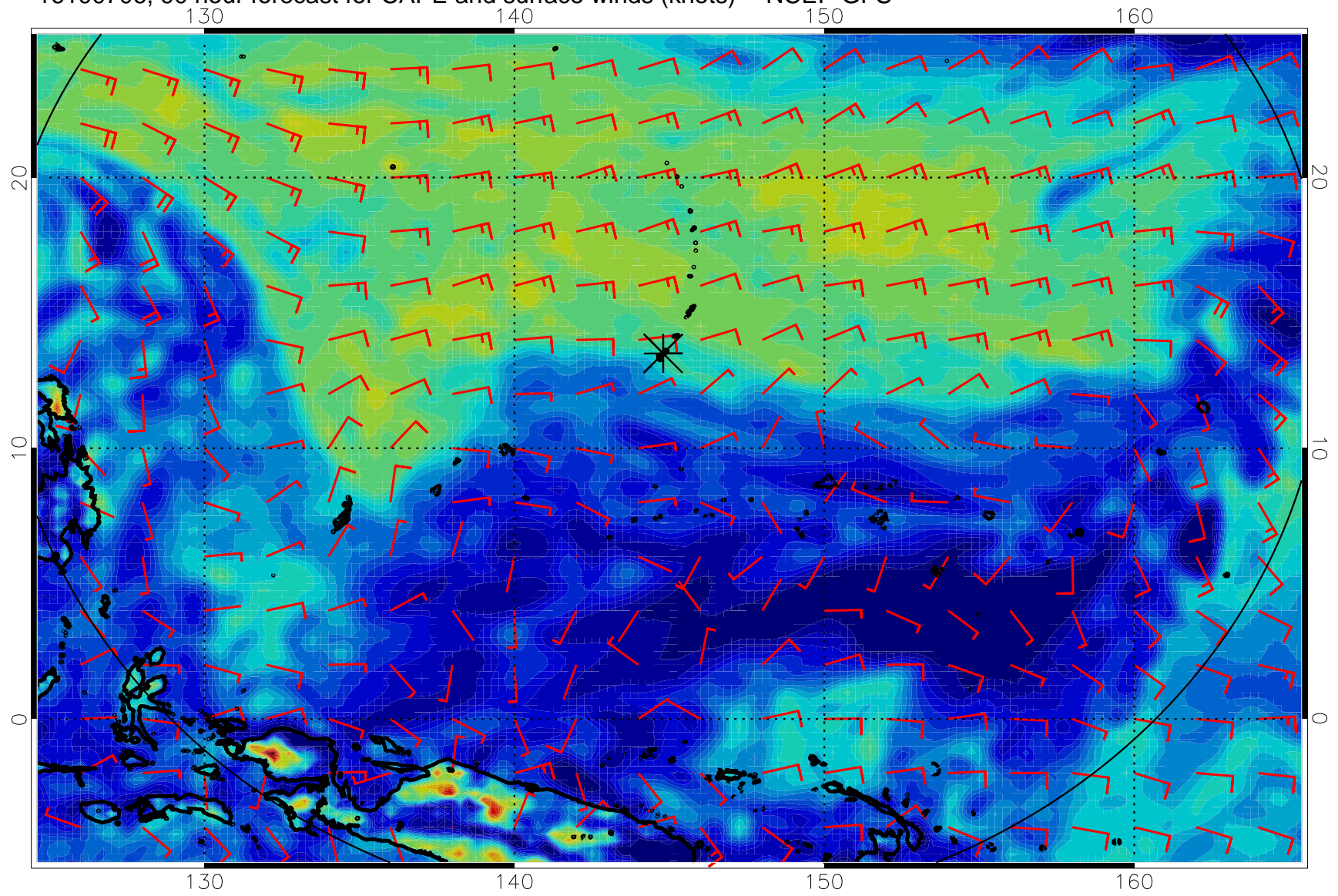
16100706, 90 hour forecast for CAPE and surface winds (knots) -- NCEP GFS
