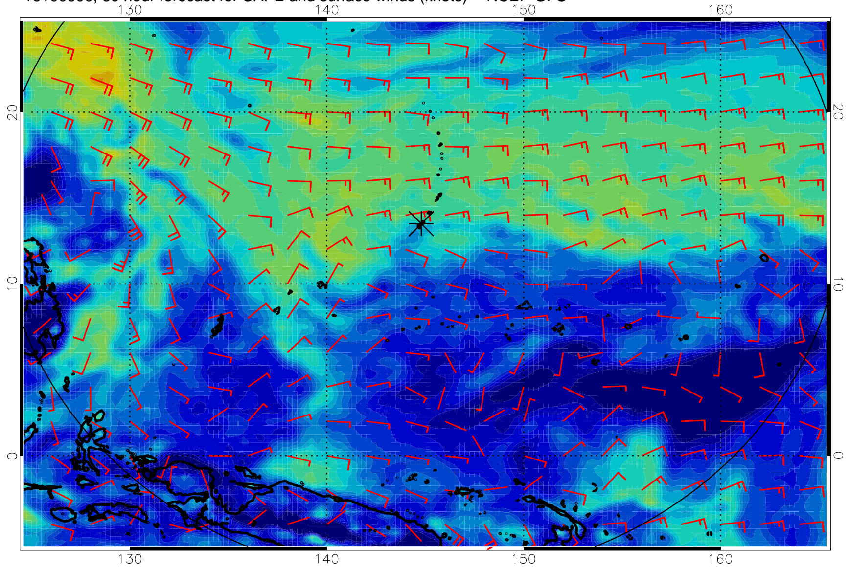
16100600, 60 hour forecast for CAPE and surface winds (knots) -- NCEP GFS
