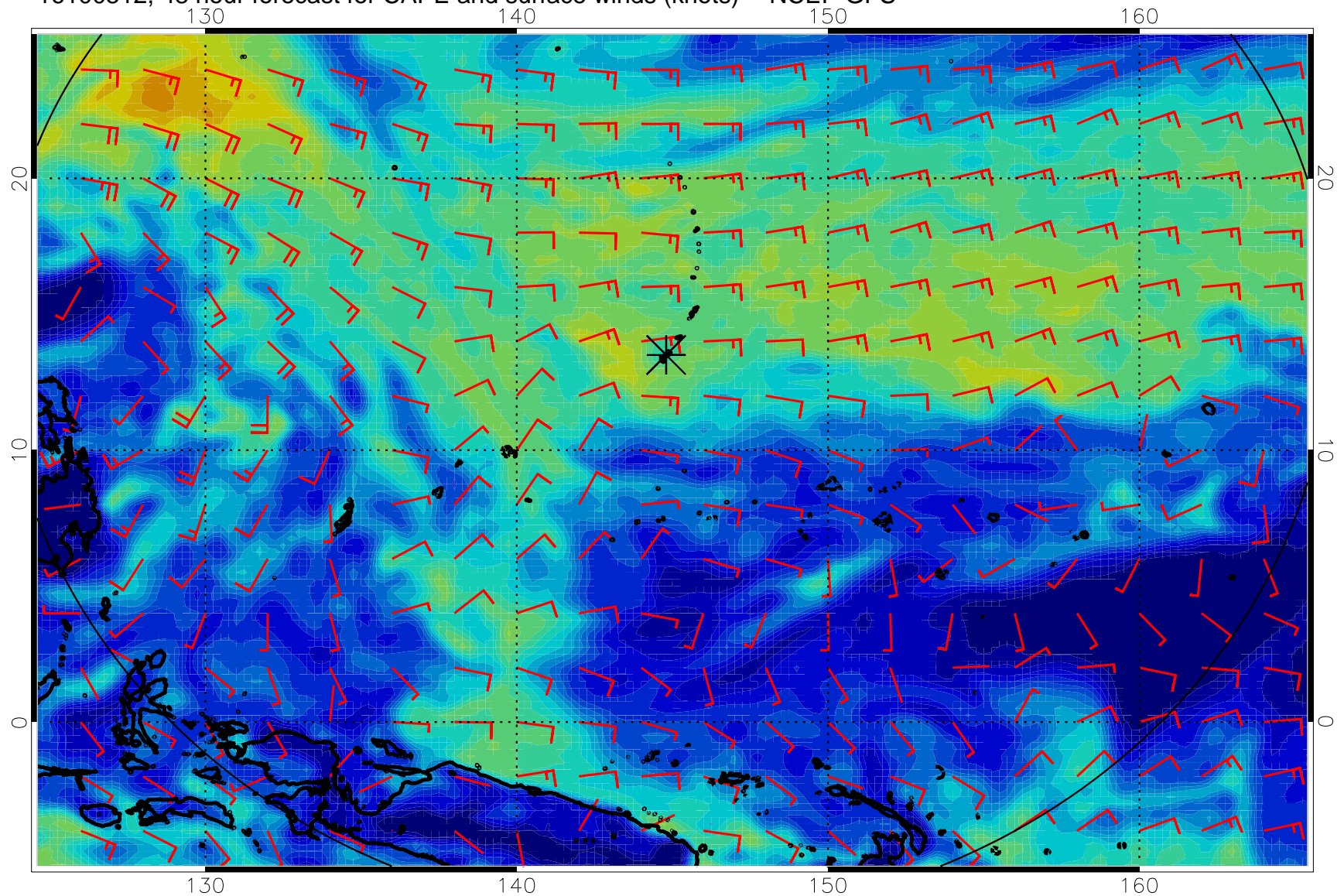
16100512, 48 hour forecast for CAPE and surface winds (knots) -- NCEP GFS
