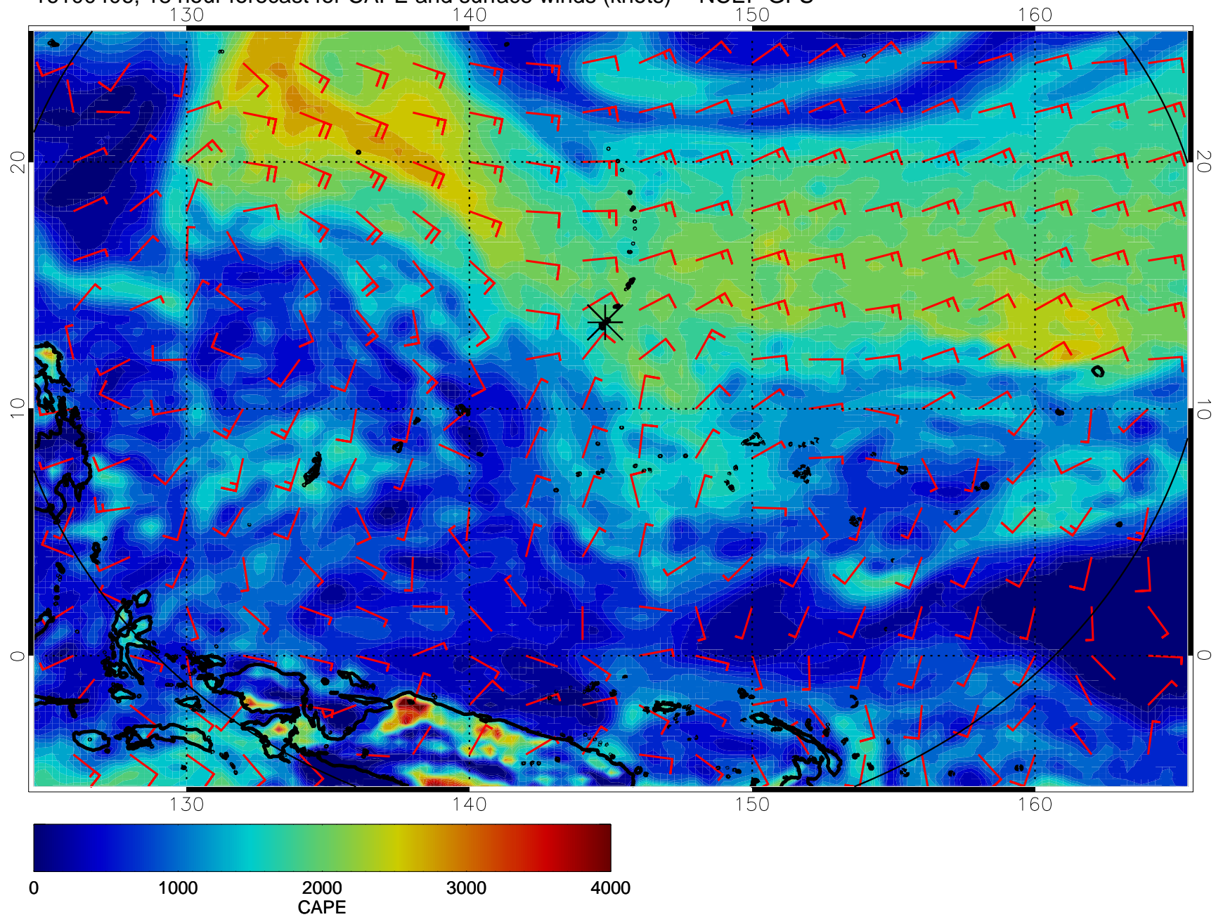
16100406, 18 hour forecast for CAPE and surface winds (knots) -- NCEP GFS
