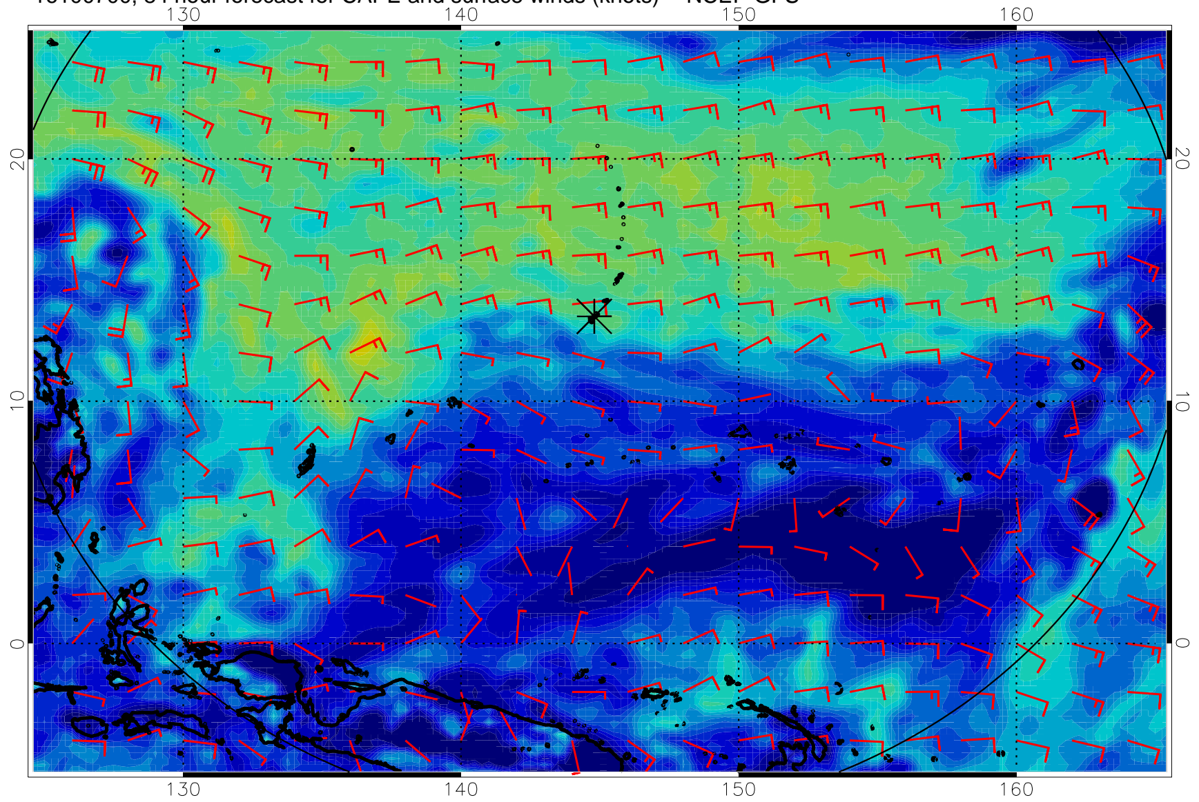
16100700, 84 hour forecast for CAPE and surface winds (knots) -- NCEP GFS
