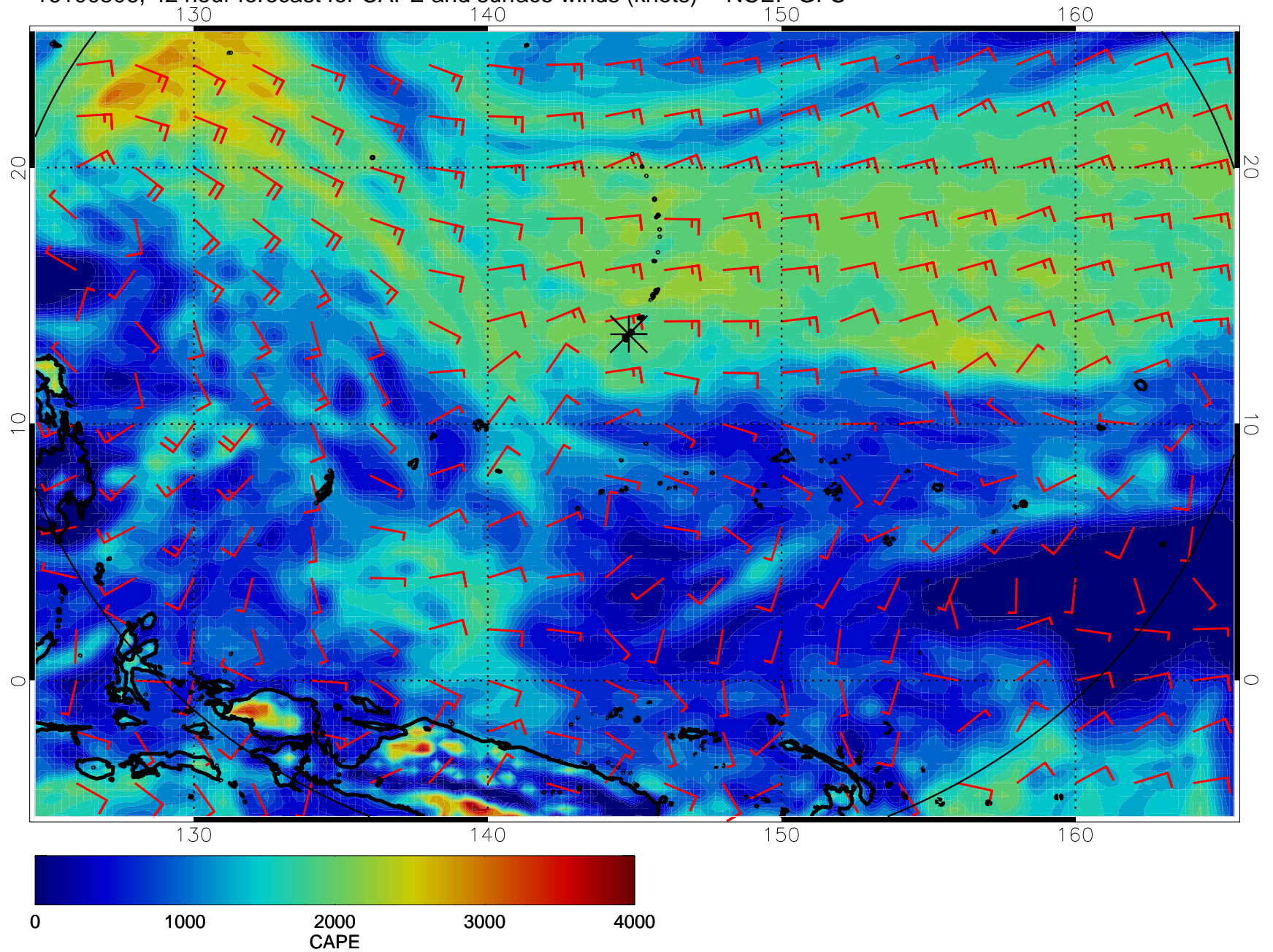
16100506, 42 hour forecast for CAPE and surface winds (knots) -- NCEP GFS
