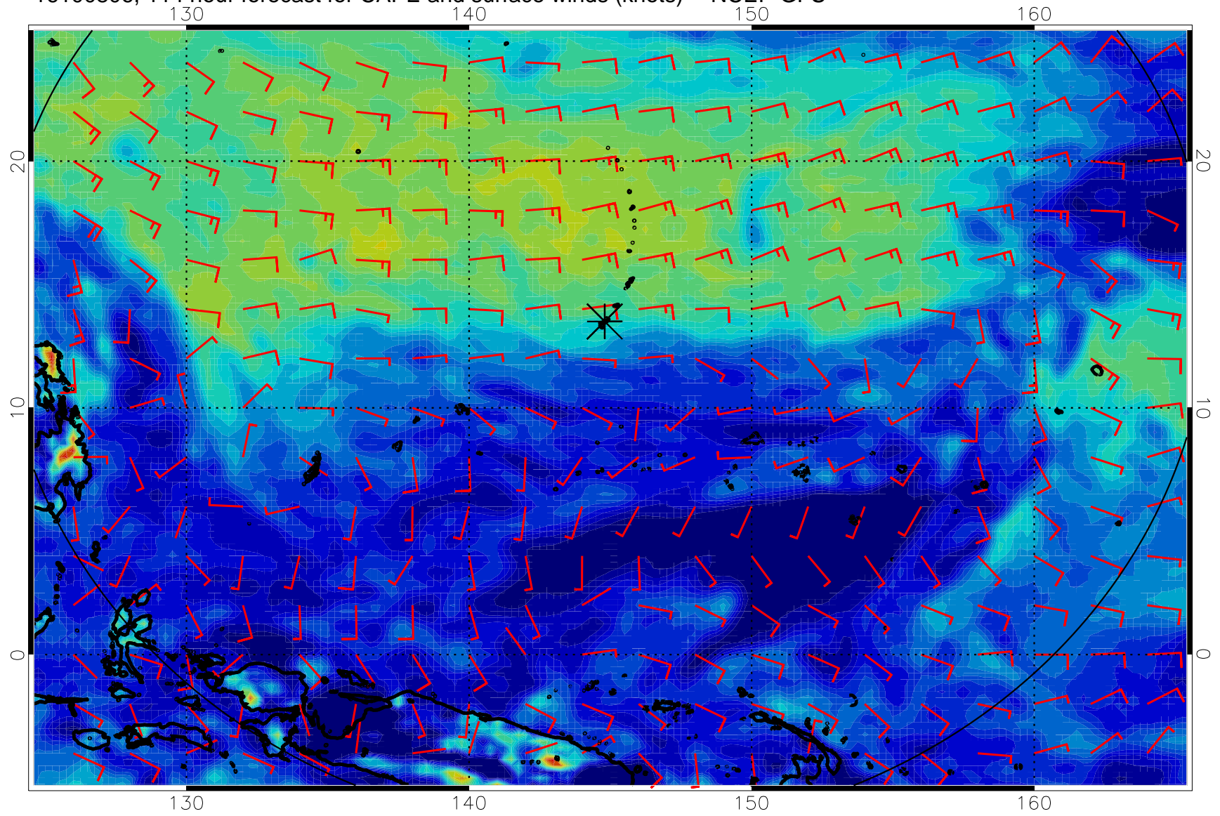
16100806, 114 hour forecast for CAPE and surface winds (knots) -- NCEP GFS
