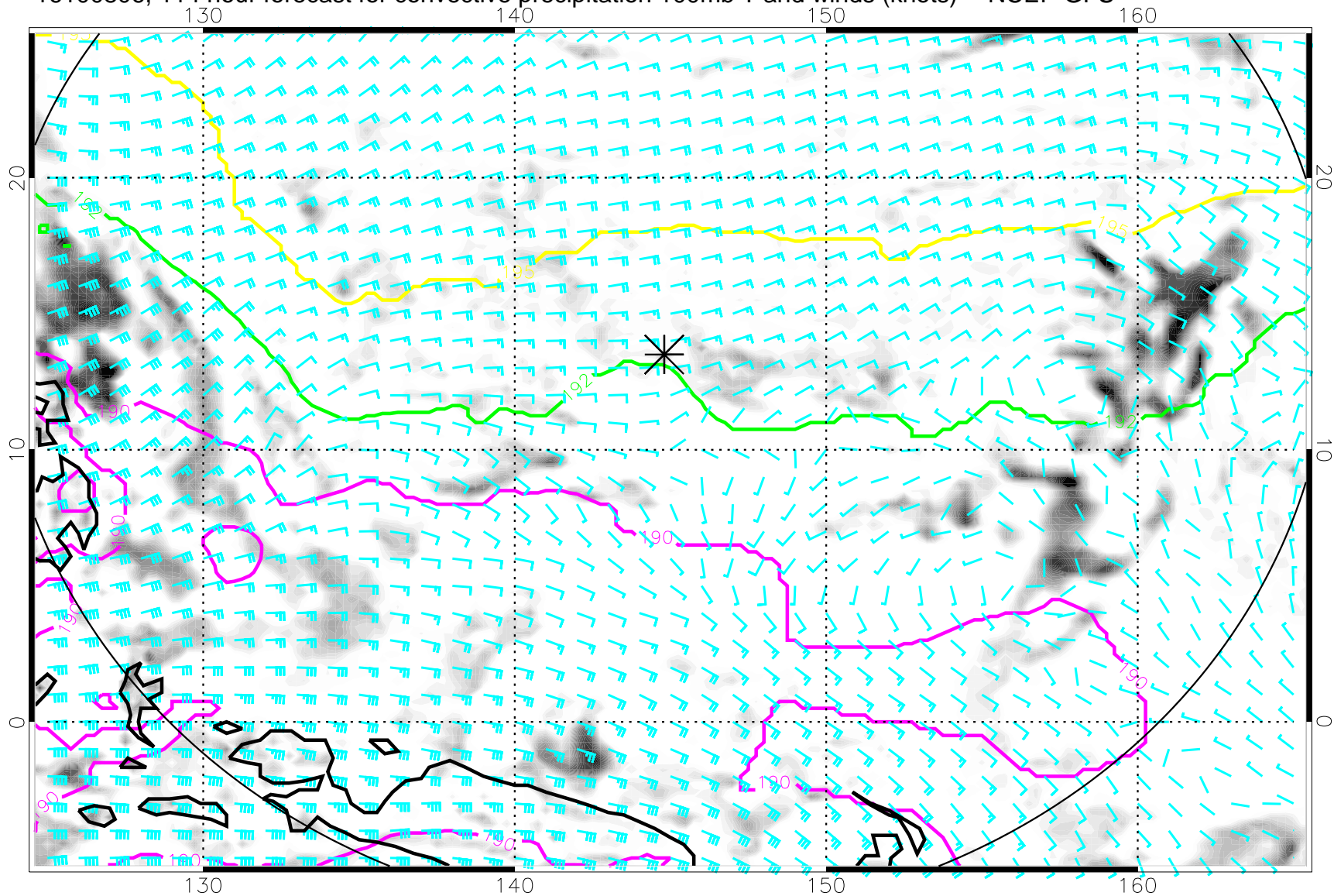
16100806, 114 hour forecast for convective precipitation 100mb T and winds (knots) -- NCEP GFS
