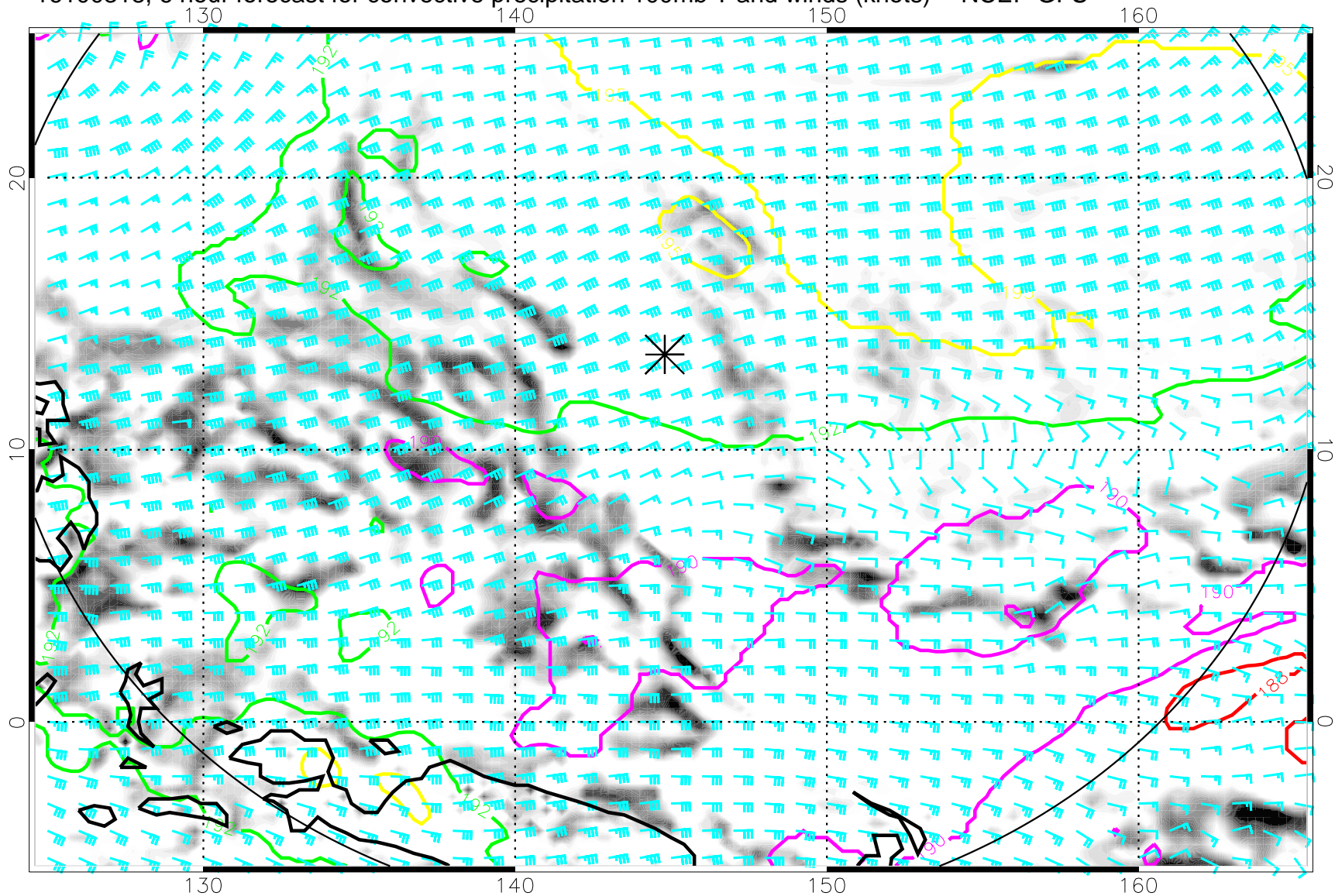
16100318, 6 hour forecast for convective precipitation 100mb T and winds (knots) -- NCEP GFS
