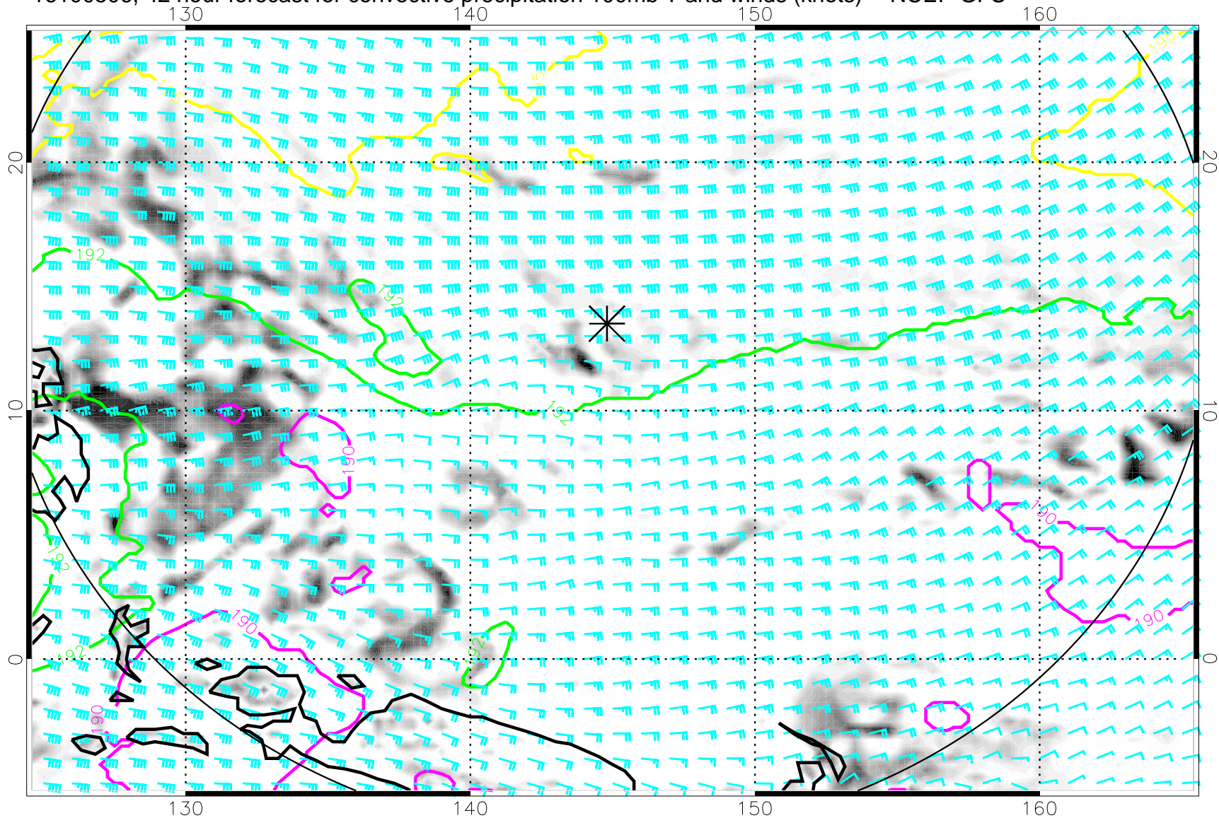
16100506, 42 hour forecast for convective precipitation 100mb T and winds (knots) -- NCEP GFS
