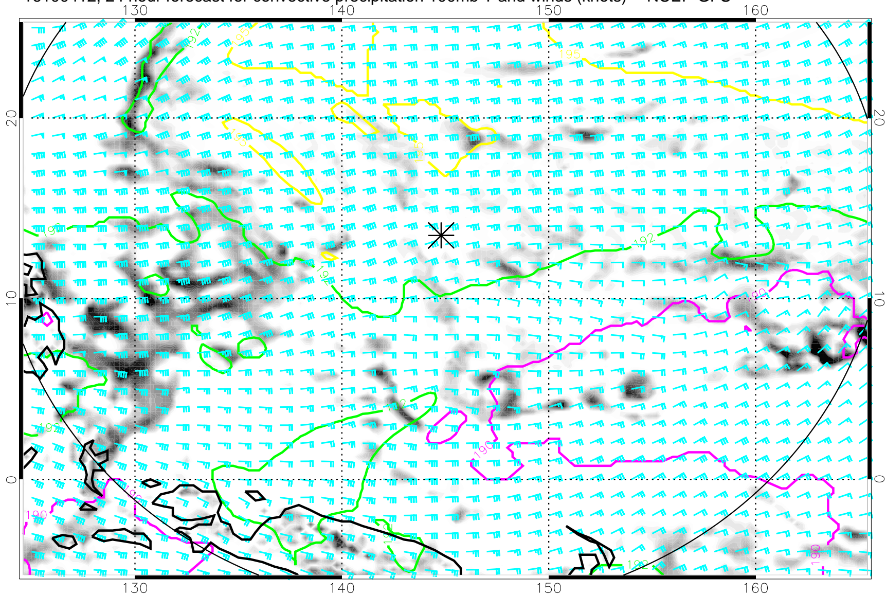
16100412, 24 hour forecast for convective precipitation 100mb T and winds (knots) -- NCEP GFS
