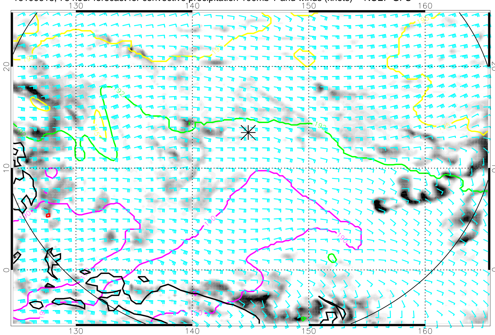
16100618, 78 hour forecast for convective precipitation 100mb T and winds (knots) -- NCEP GFS
