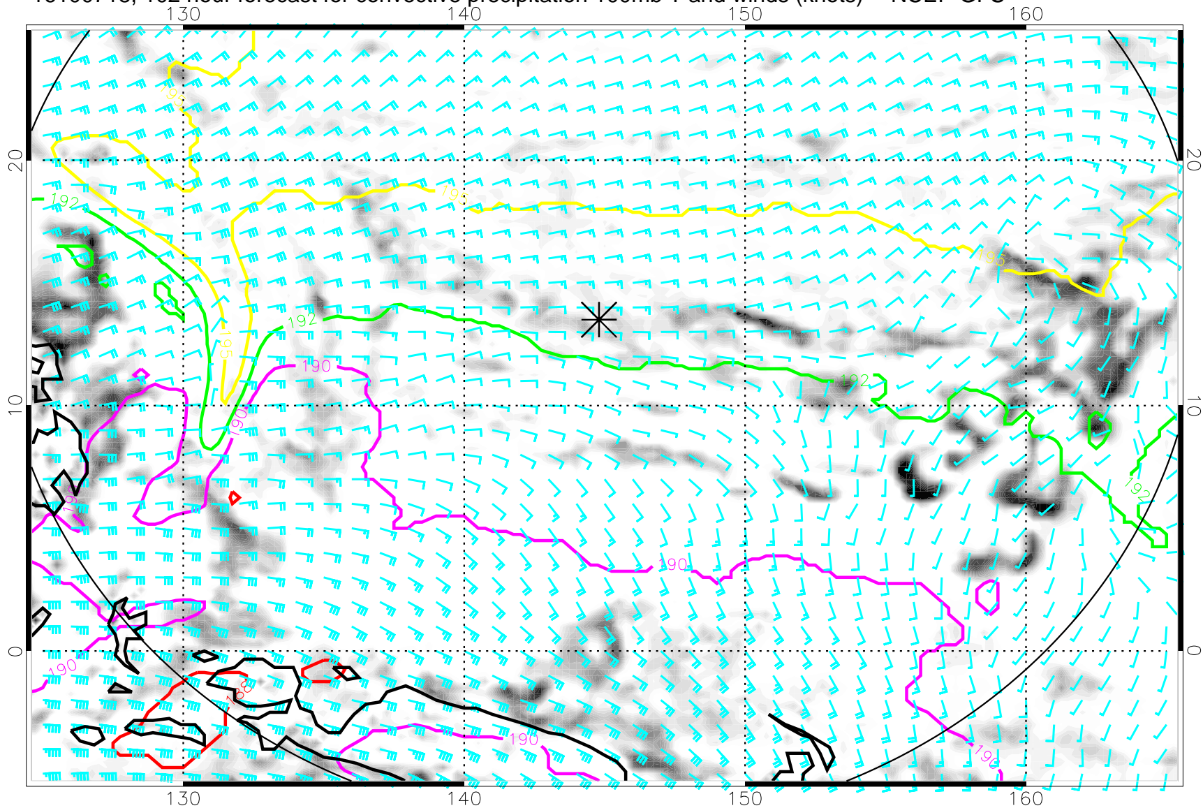
16100718, 102 hour forecast for convective precipitation 100mb T and winds (knots) -- NCEP GFS
