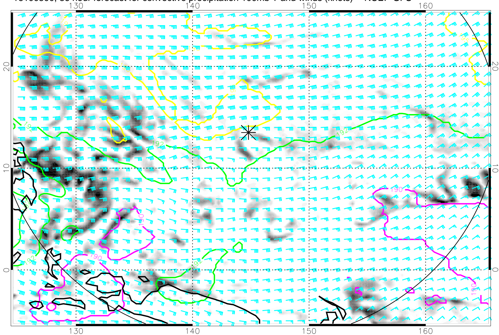
16100500, 36 hour forecast for convective precipitation 100mb T and winds (knots) -- NCEP GFS
