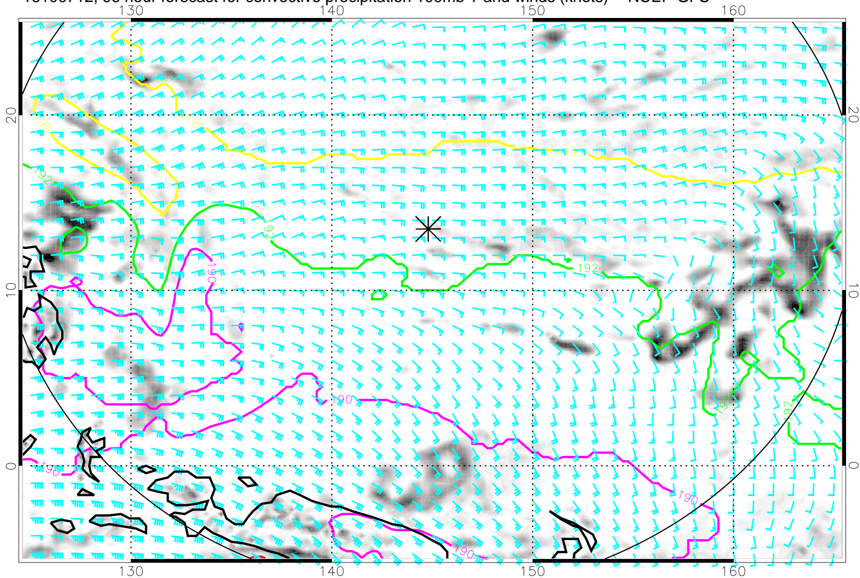
16100712, 96 hour forecast for convective precipitation 100mb T and winds (knots) -- NCEP GFS
