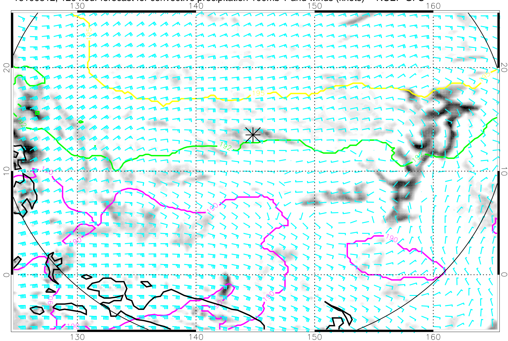
16100812, 120 hour forecast for convective precipitation 100mb T and winds (knots) -- NCEP GFS
