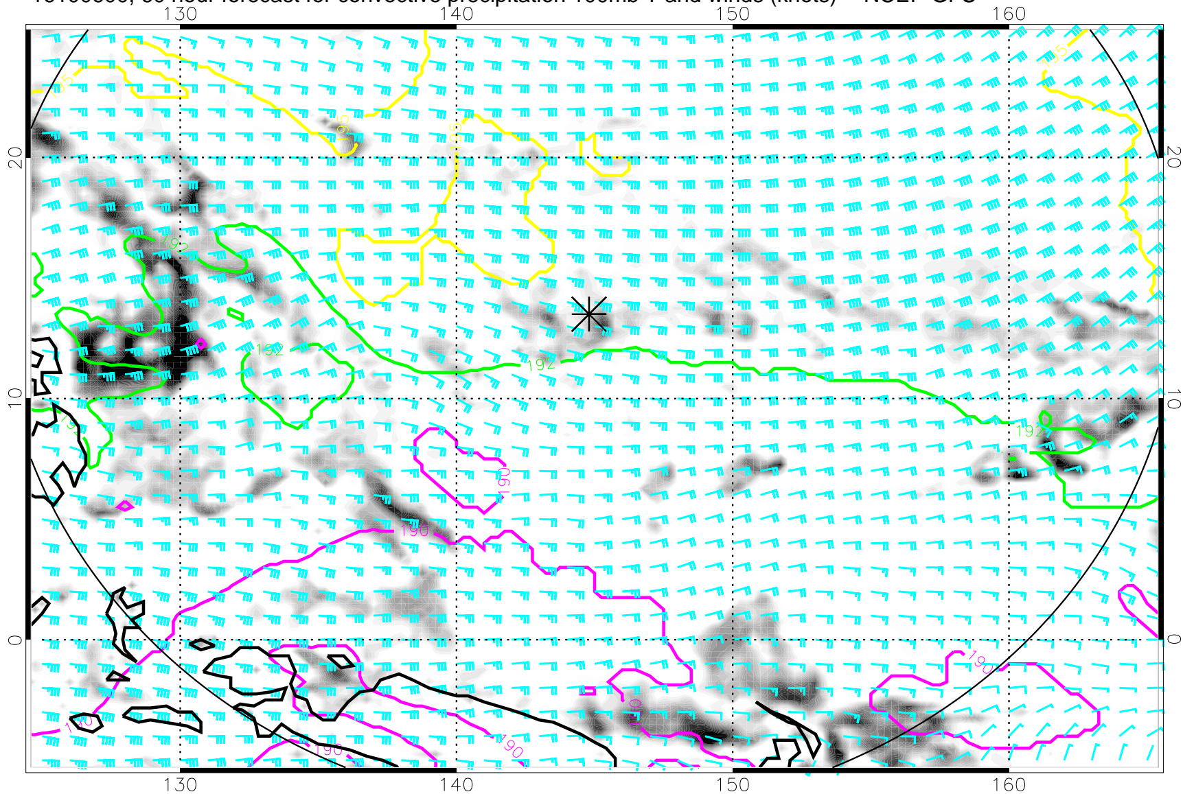
16100600, 60 hour forecast for convective precipitation 100mb T and winds (knots) -- NCEP GFS
