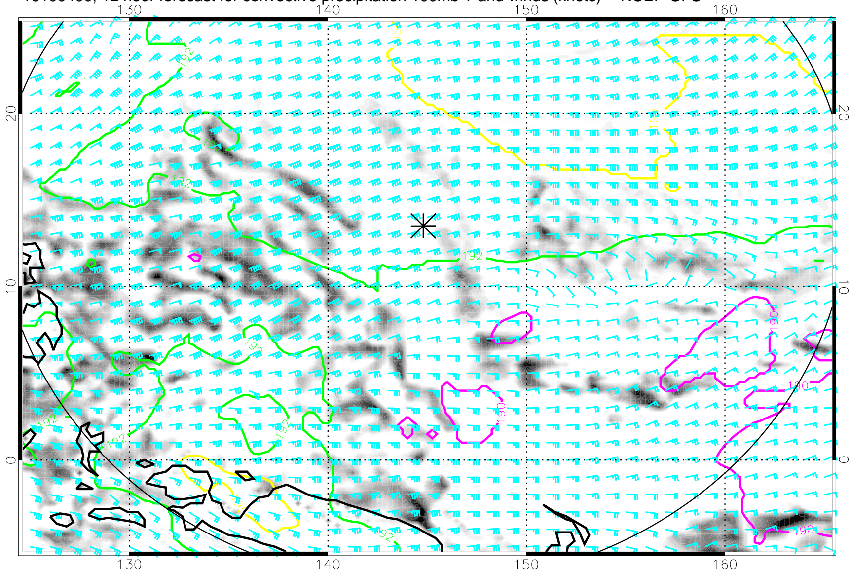
16100400, 12 hour forecast for convective precipitation 100mb T and winds (knots) -- NCEP GFS
