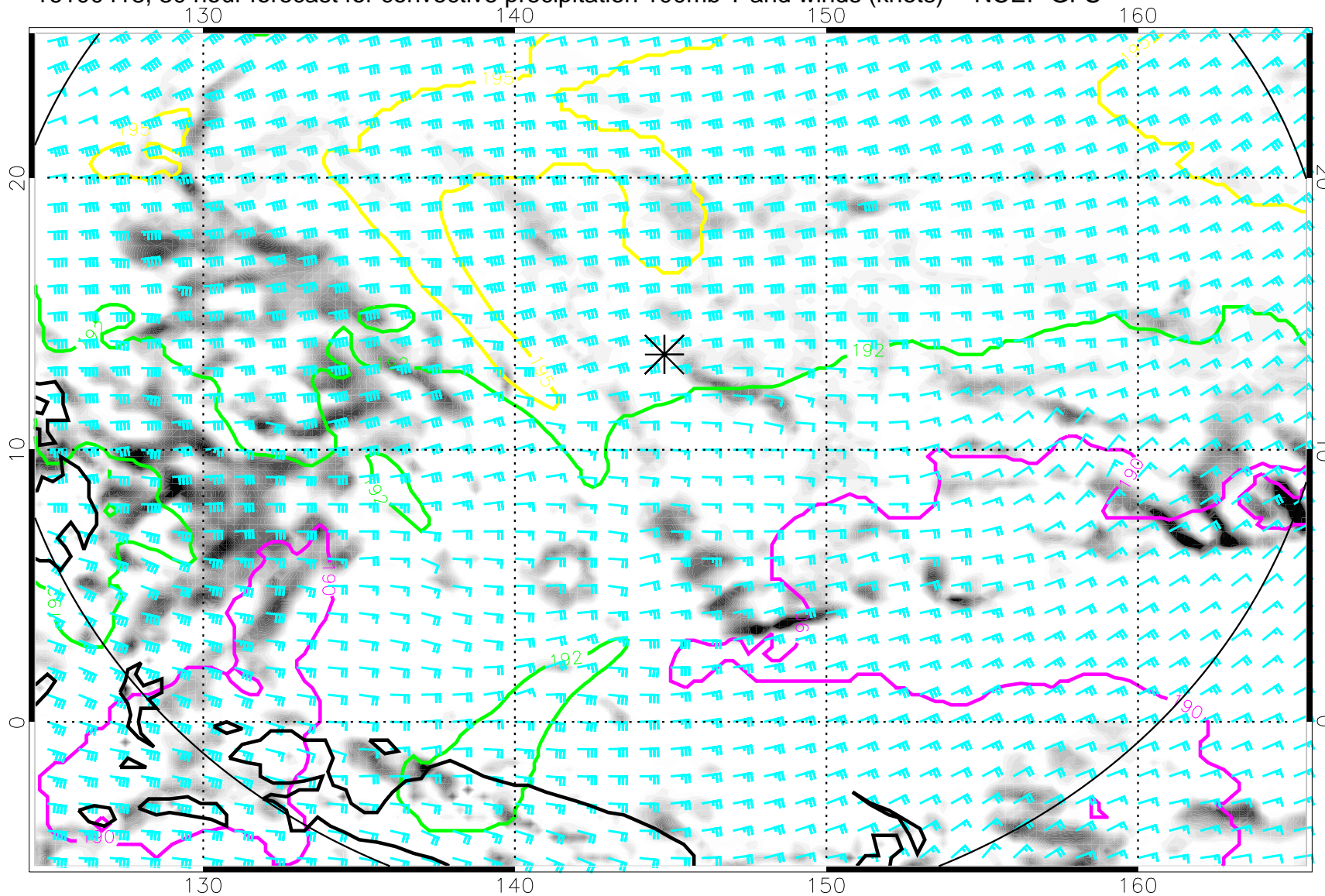
16100418, 30 hour forecast for convective precipitation 100mb T and winds (knots) -- NCEP GFS
