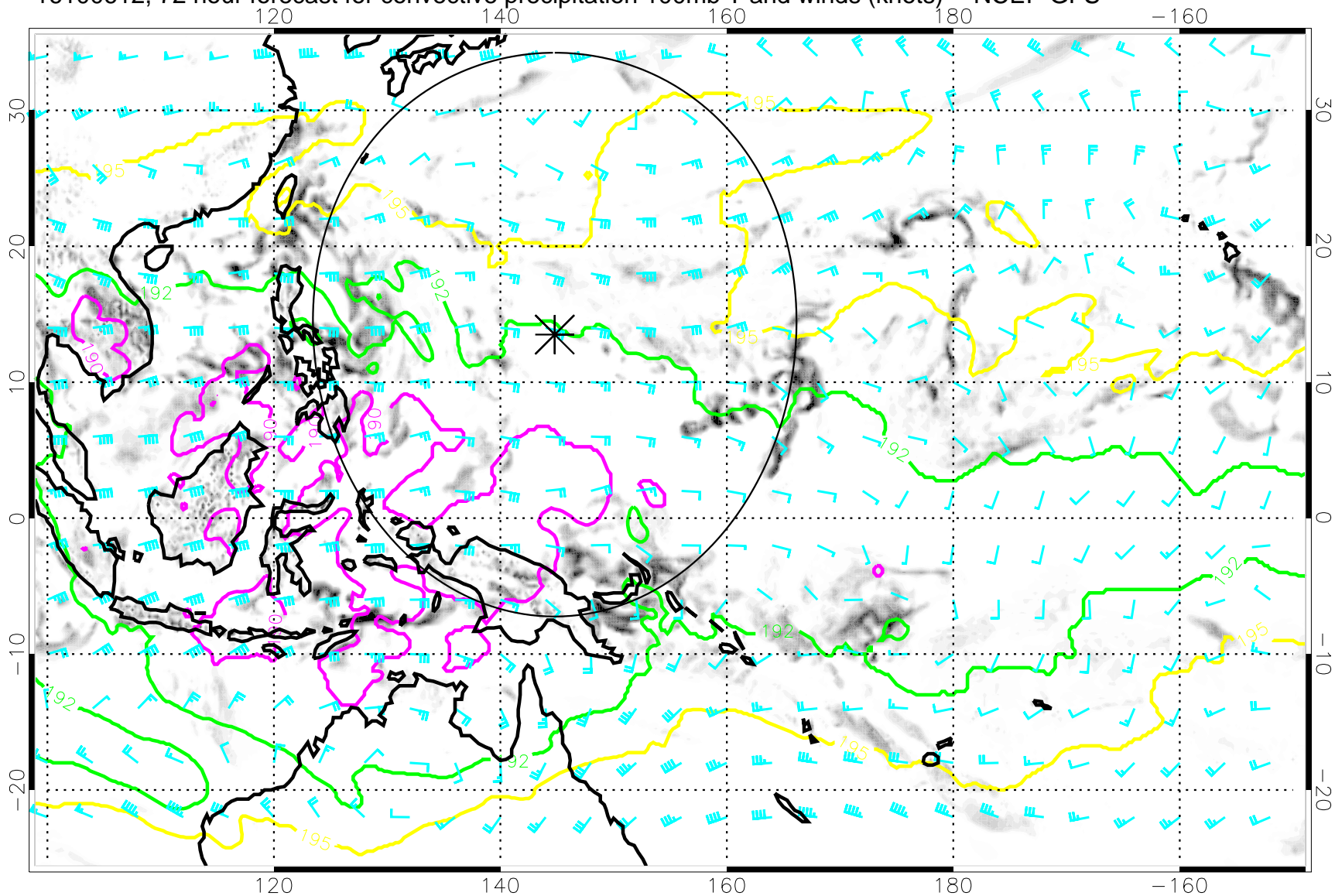
16100612, 72 hour forecast for convective precipitation 100mb T and winds (knots) -- NCEP GFS
