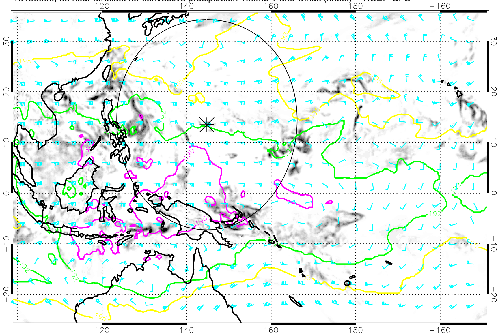
16100606, 66 hour forecast for convective precipitation 100mb T and winds (knots) -- NCEP GFS
