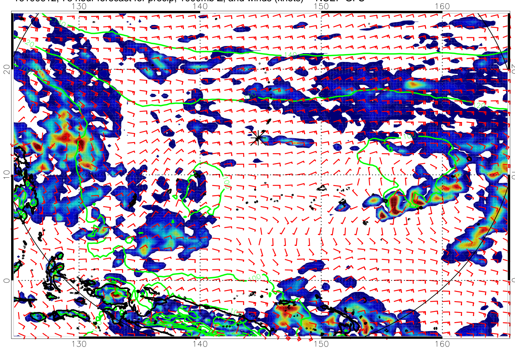
16100612, 78 hour forecast for precip, 1000mb Z, and winds (knots) -- NCEP GFS
