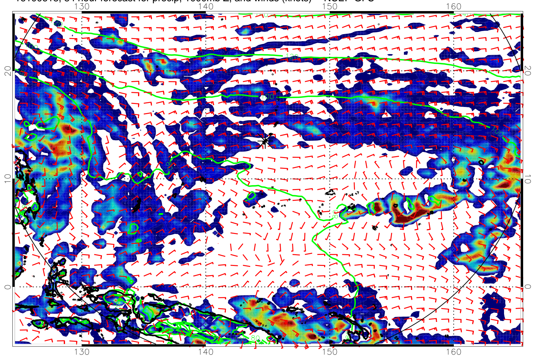
16100618, 84 hour forecast for precip, 1000mb Z, and winds (knots) -- NCEP GFS
