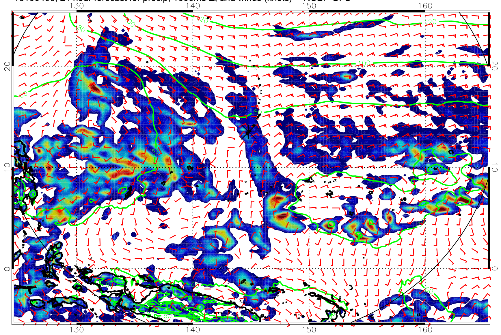
16100406, 24 hour forecast for precip, 1000mb Z, and winds (knots) -- NCEP GFS
