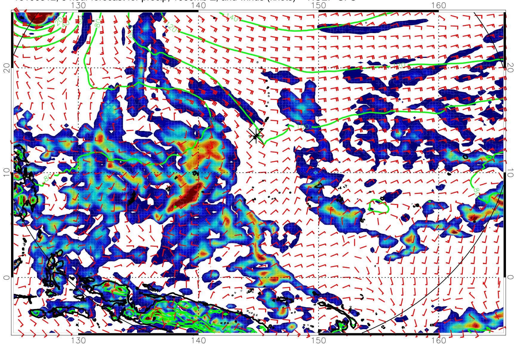
16100312, 6 hour forecast for precip, 1000mb Z, and winds (knots) -- NCEP GFS
