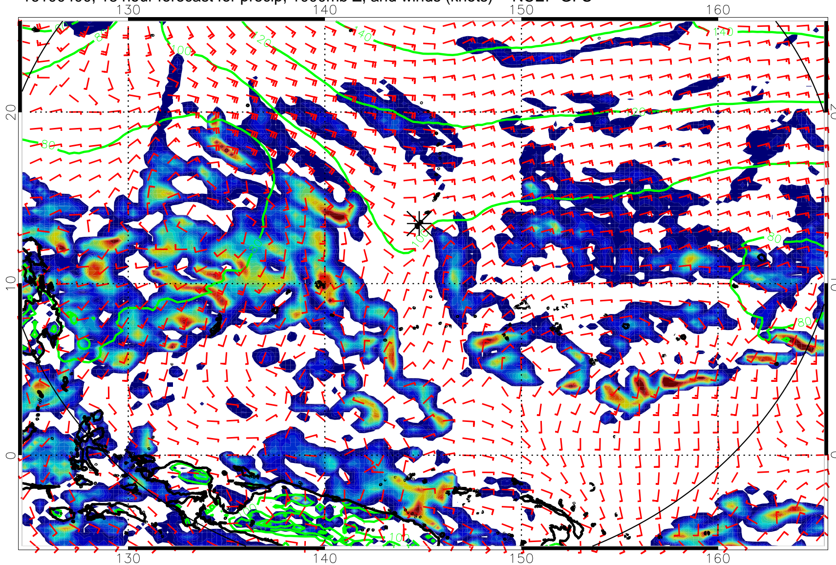
16100400, 18 hour forecast for precip, 1000mb Z, and winds (knots) -- NCEP GFS
