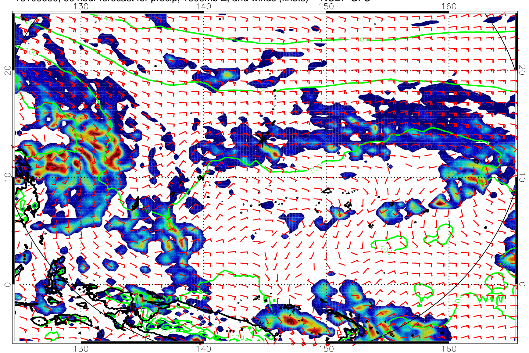
16100600, 66 hour forecast for precip, 1000mb Z, and winds (knots) -- NCEP GFS
