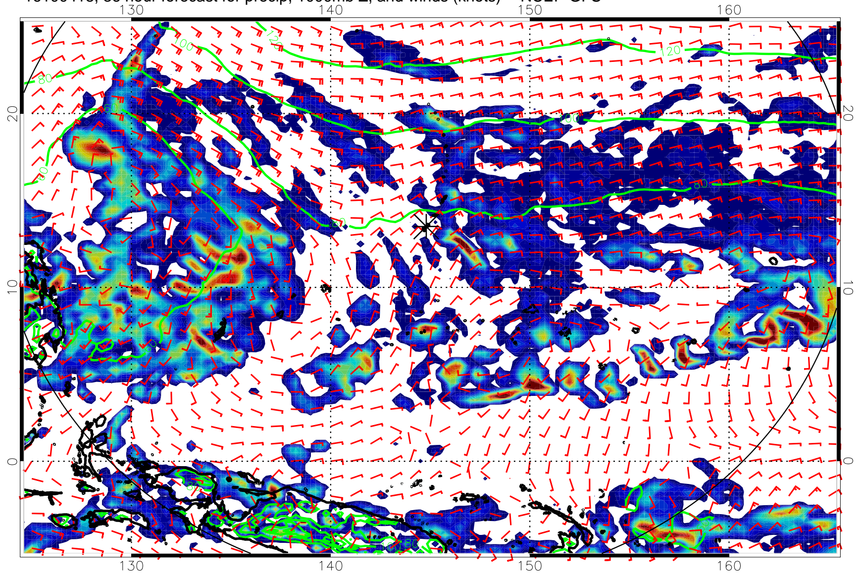
16100418, 36 hour forecast for precip, 1000mb Z, and winds (knots) -- NCEP GFS
