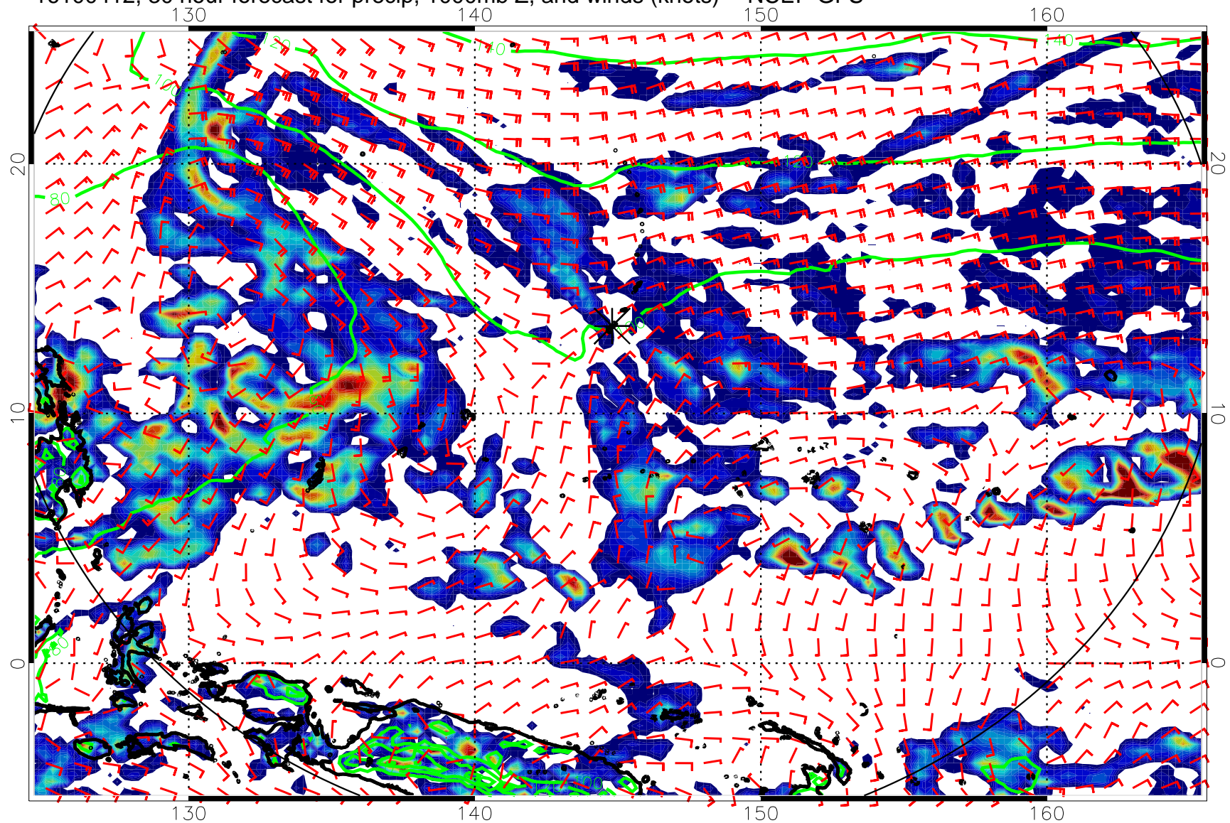
16100412, 30 hour forecast for precip, 1000mb Z, and winds (knots) -- NCEP GFS
