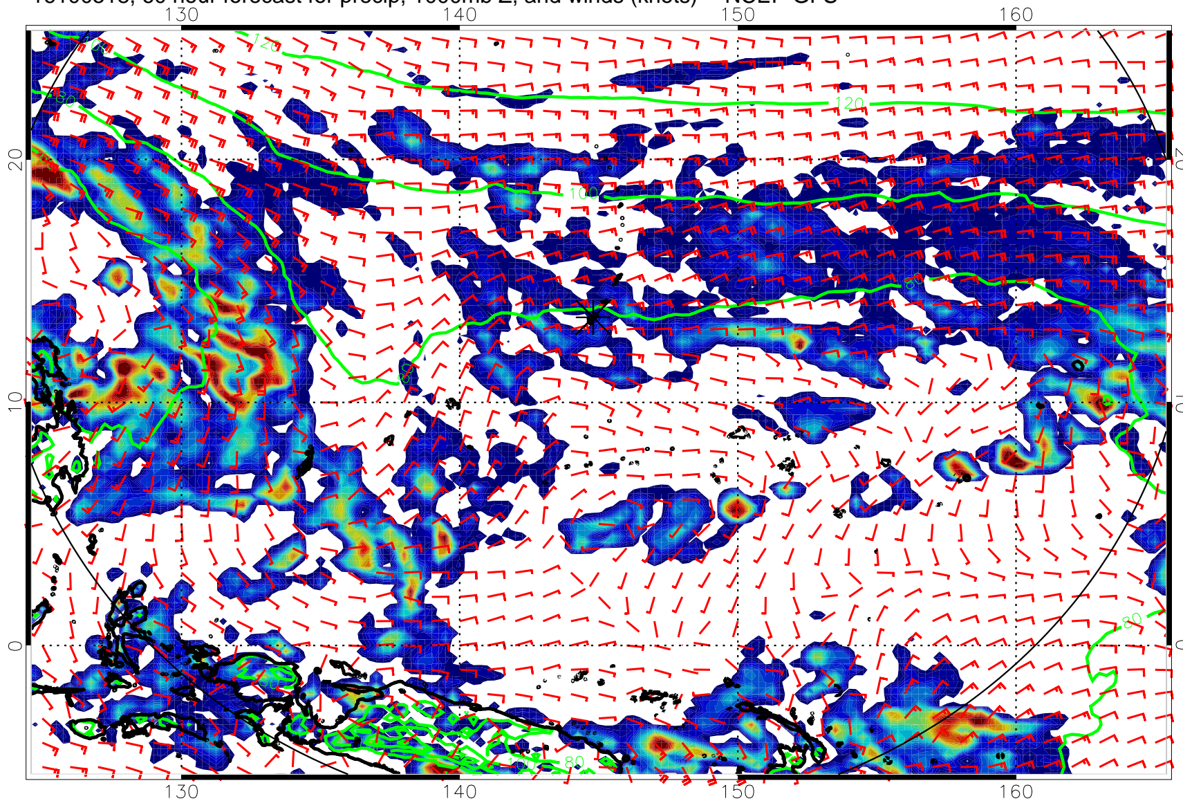
16100518, 60 hour forecast for precip, 1000mb Z, and winds (knots) -- NCEP GFS
