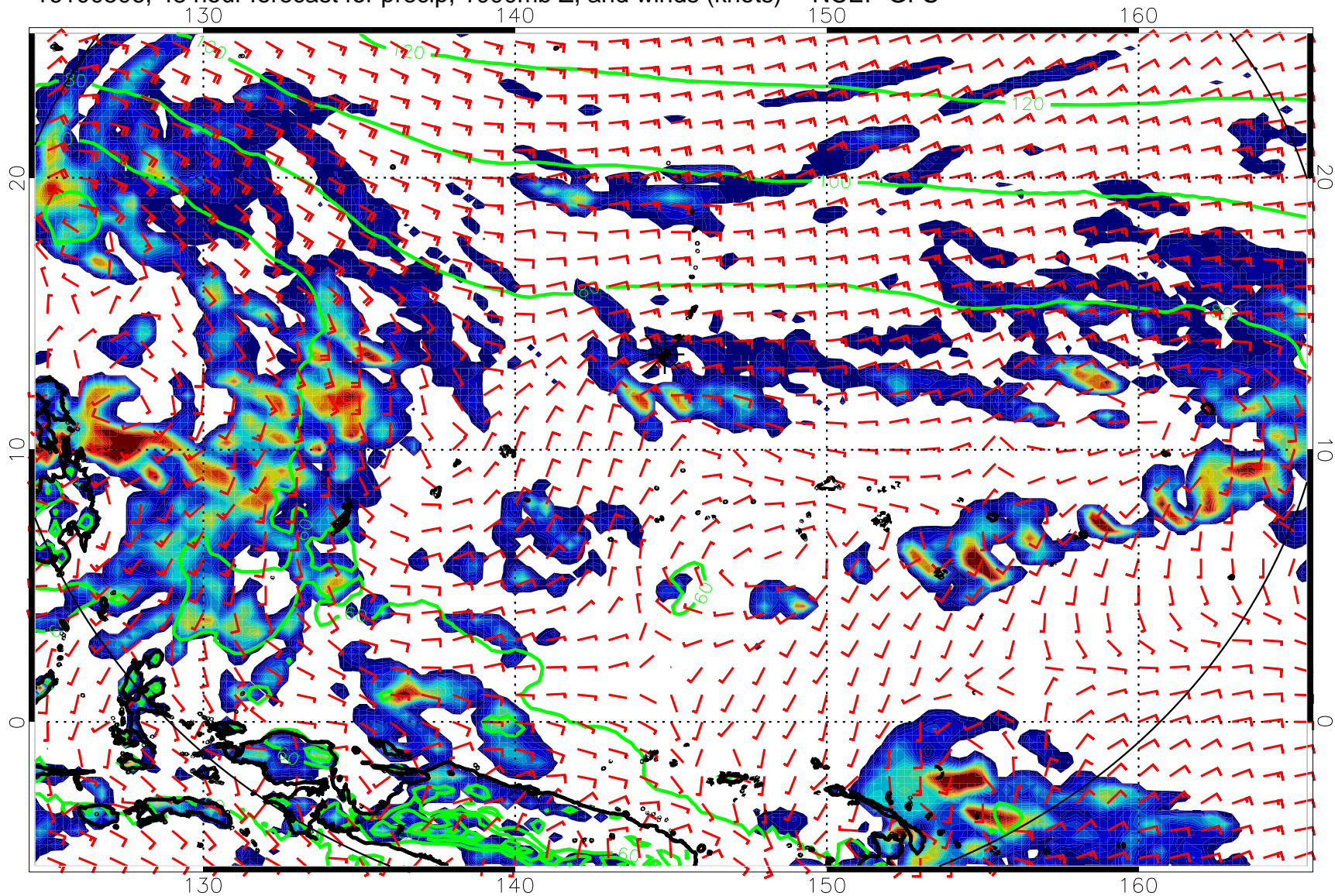
16100506, 48 hour forecast for precip, 1000mb Z, and winds (knots) -- NCEP GFS
