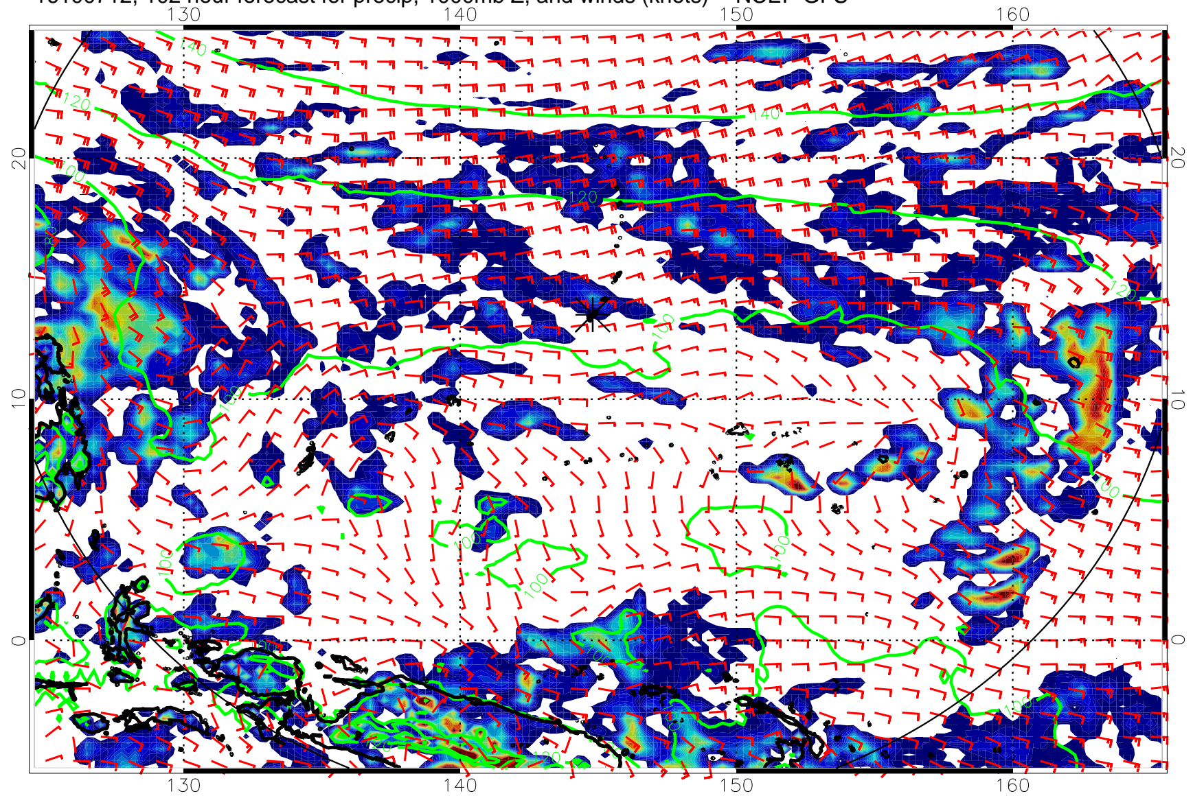
16100712, 102 hour forecast for precip, 1000mb Z, and winds (knots) -- NCEP GFS
