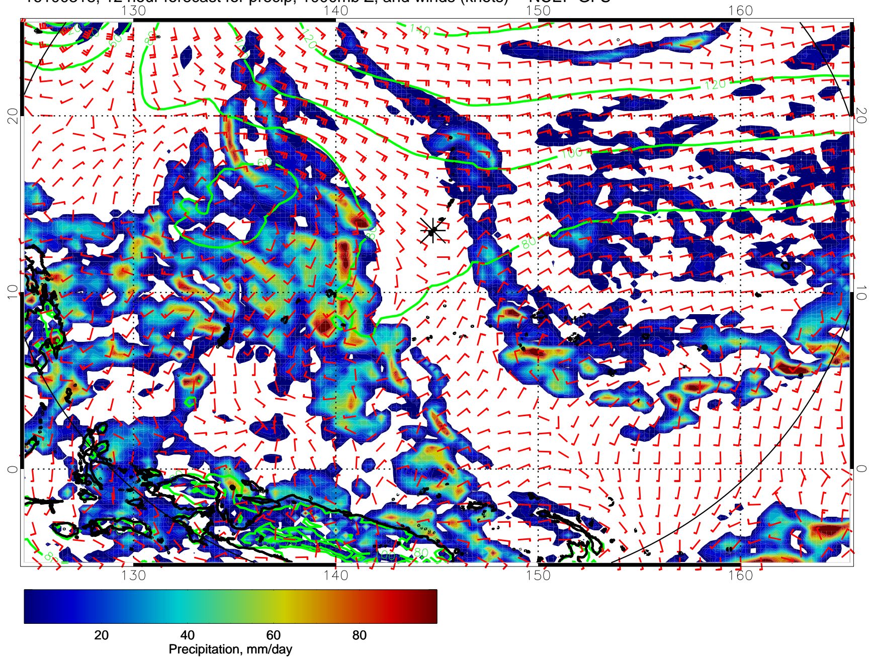
16100318, 12 hour forecast for precip, 1000mb Z, and winds (knots) -- NCEP GFS
