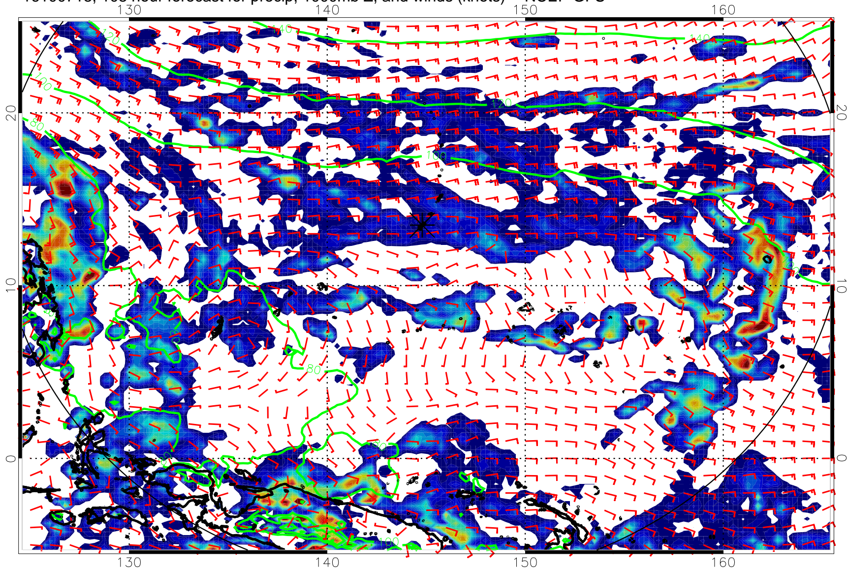
16100718, 108 hour forecast for precip, 1000mb Z, and winds (knots) -- NCEP GFS
