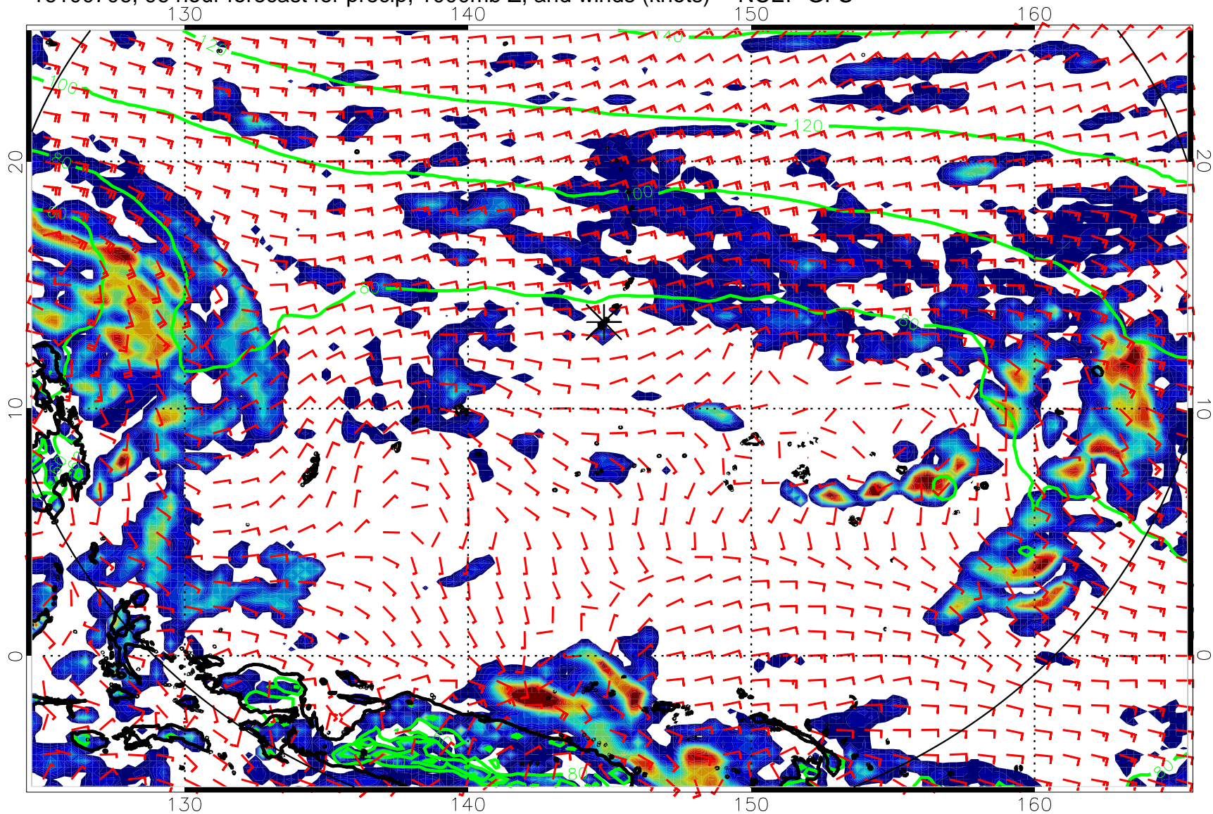
16100706, 96 hour forecast for precip, 1000mb Z, and winds (knots) -- NCEP GFS
