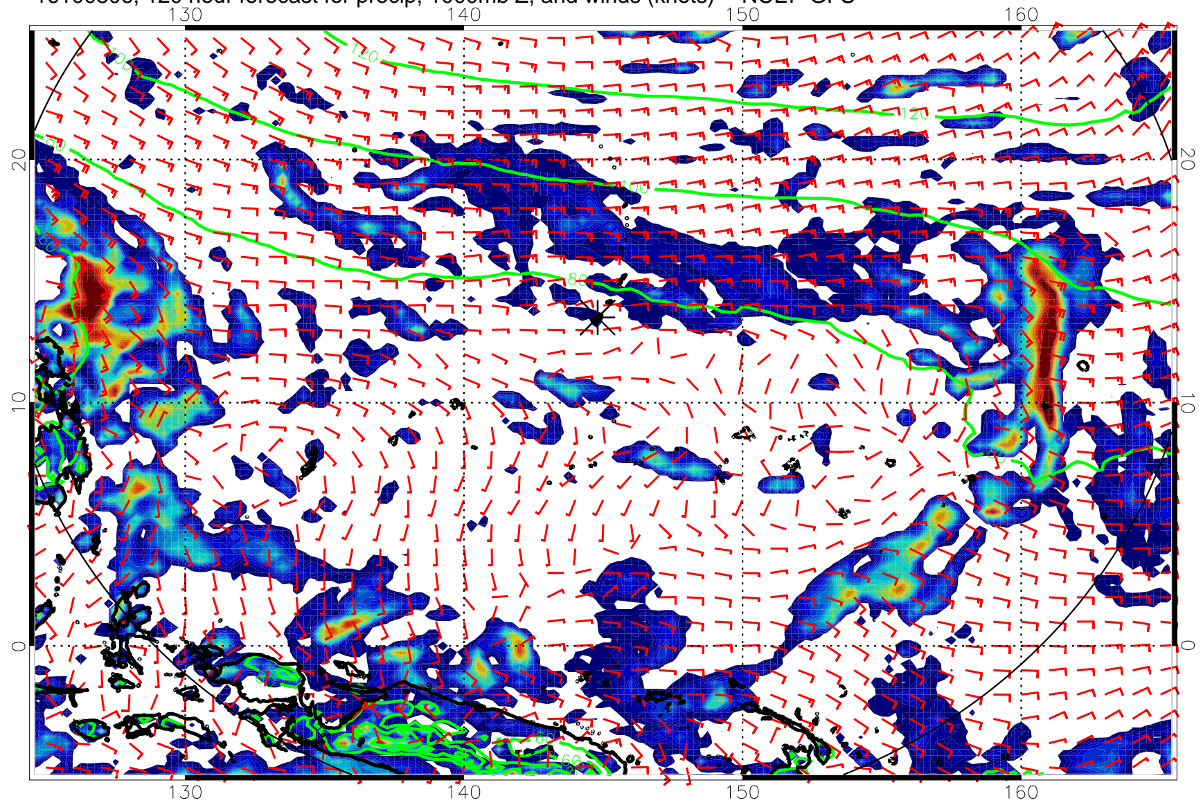
16100806, 120 hour forecast for precip, 1000mb Z, and winds (knots) -- NCEP GFS
