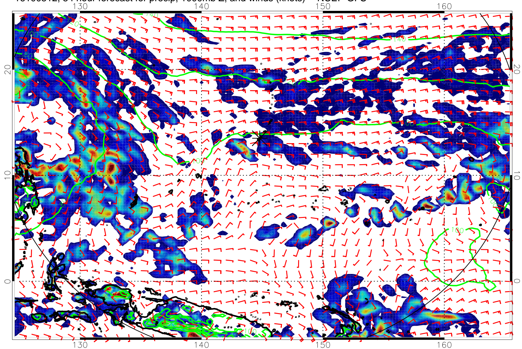
16100512, 54 hour forecast for precip, 1000mb Z, and winds (knots) -- NCEP GFS
