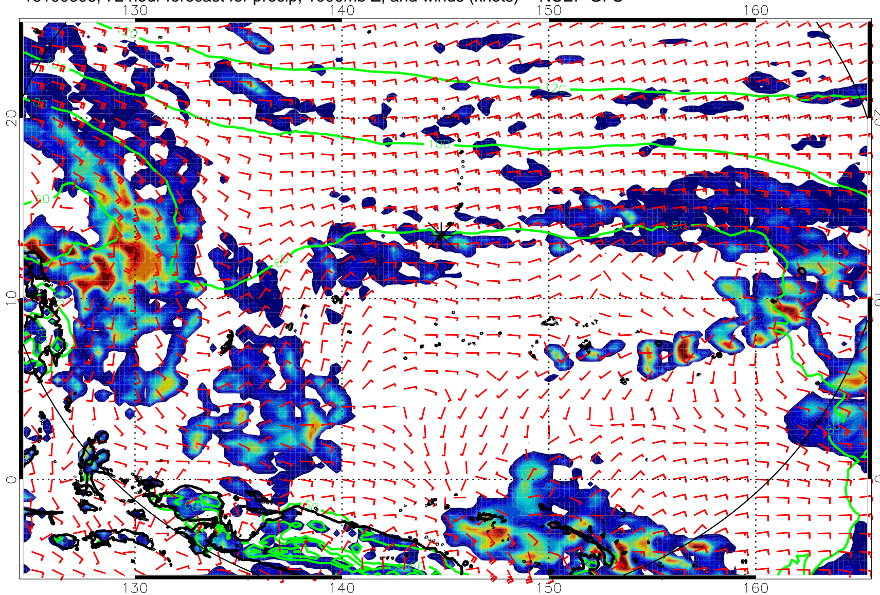
16100606, 72 hour forecast for precip, 1000mb Z, and winds (knots) -- NCEP GFS
