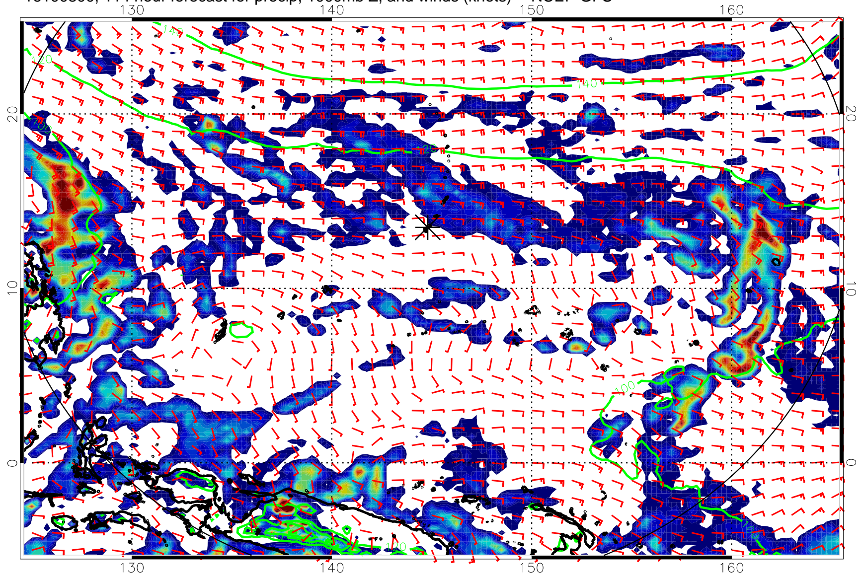
16100800, 114 hour forecast for precip, 1000mb Z, and winds (knots) -- NCEP GFS
