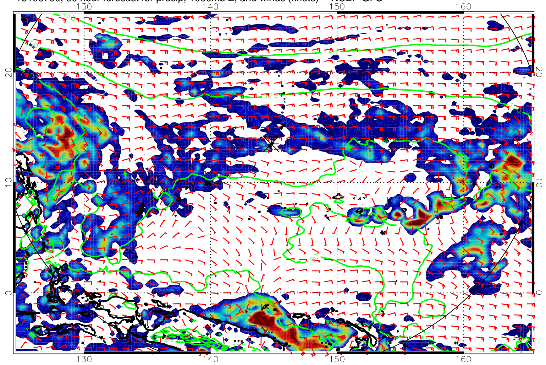
16100700, 90 hour forecast for precip, 1000mb Z, and winds (knots) -- NCEP GFS
