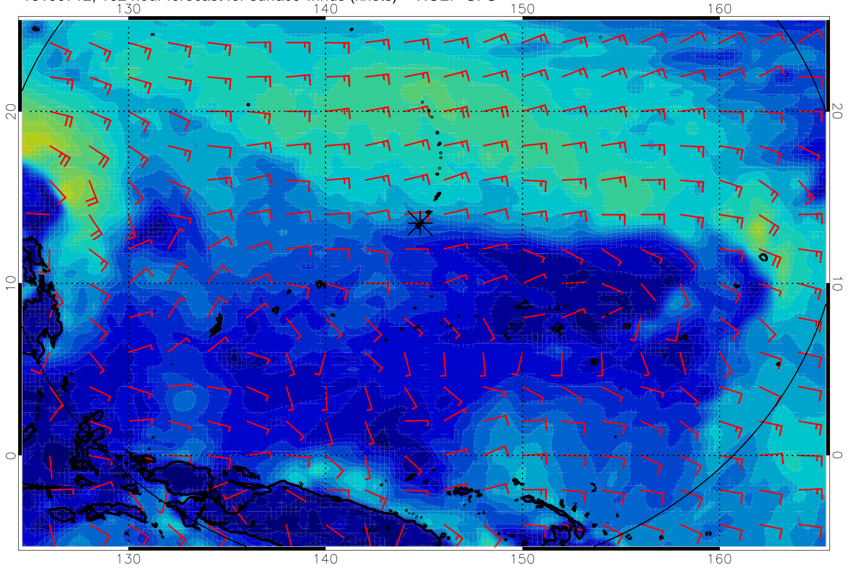
16100712, 102 hour forecast for surface winds (knots) -- NCEP GFS
