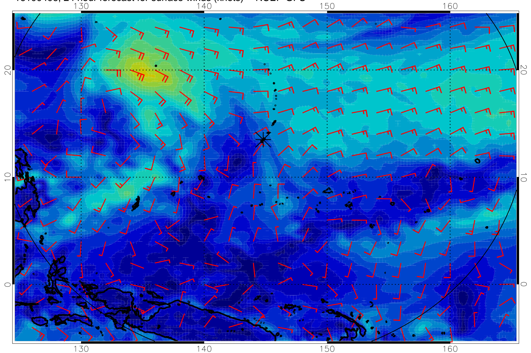
16100406, 24 hour forecast for surface winds (knots) -- NCEP GFS
