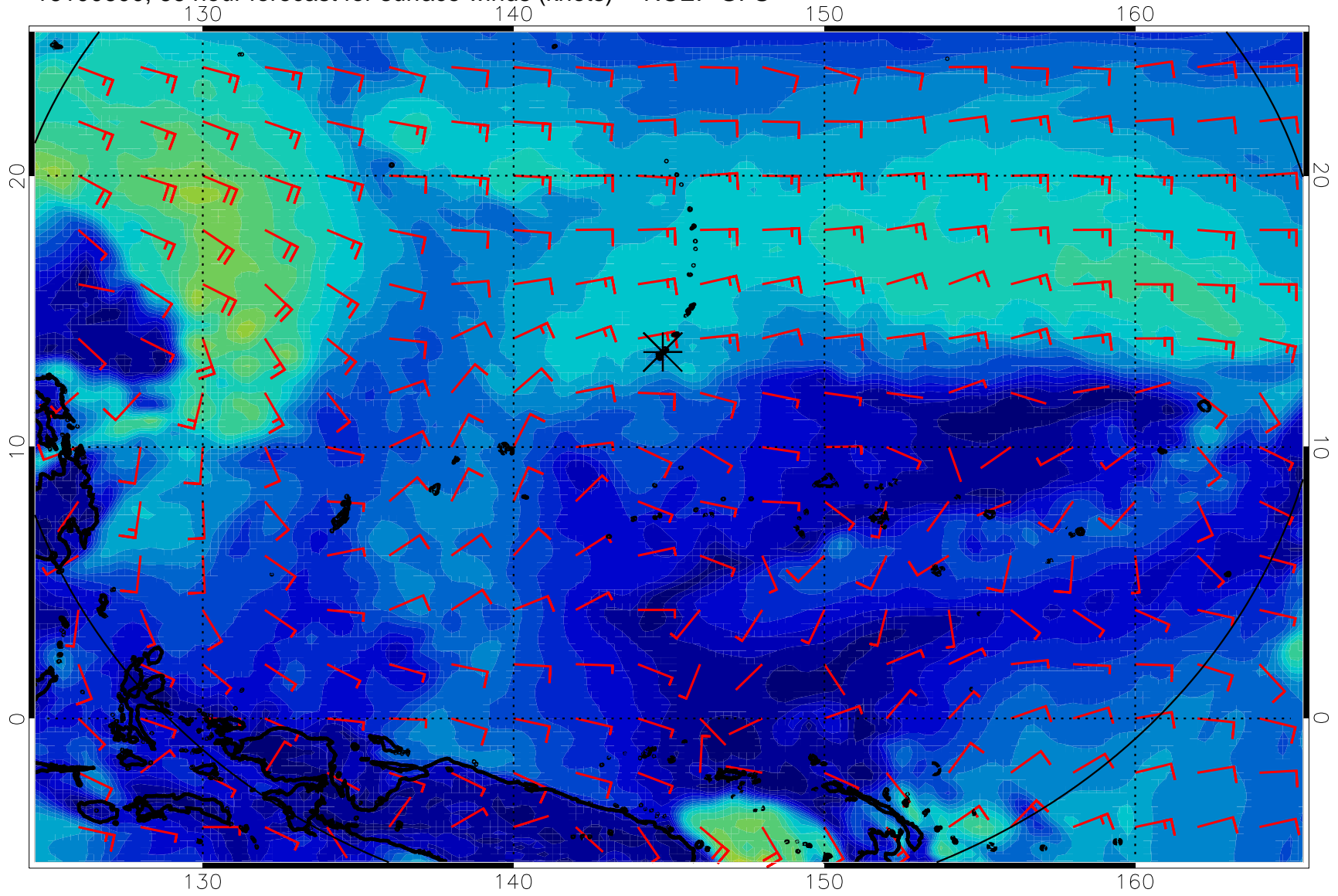
16100600, 66 hour forecast for surface winds (knots) -- NCEP GFS
