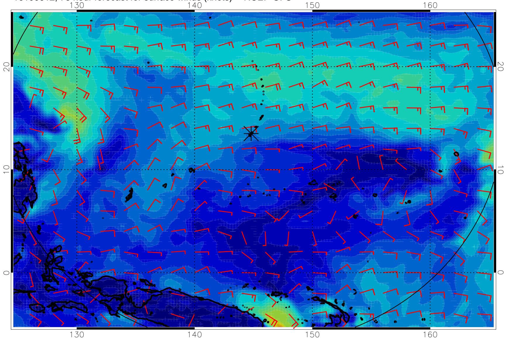
16100612, 78 hour forecast for surface winds (knots) -- NCEP GFS
