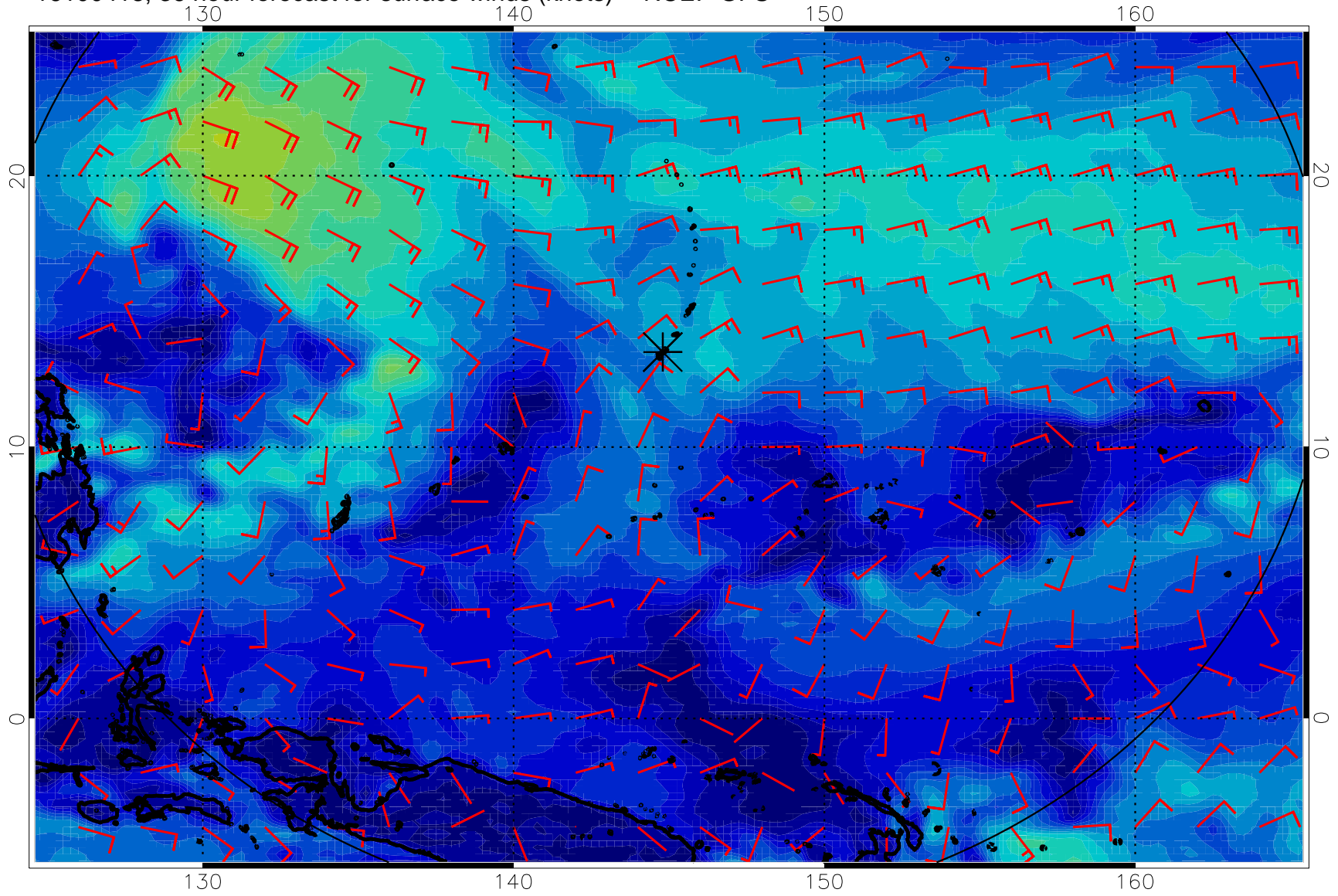
16100418, 36 hour forecast for surface winds (knots) -- NCEP GFS
