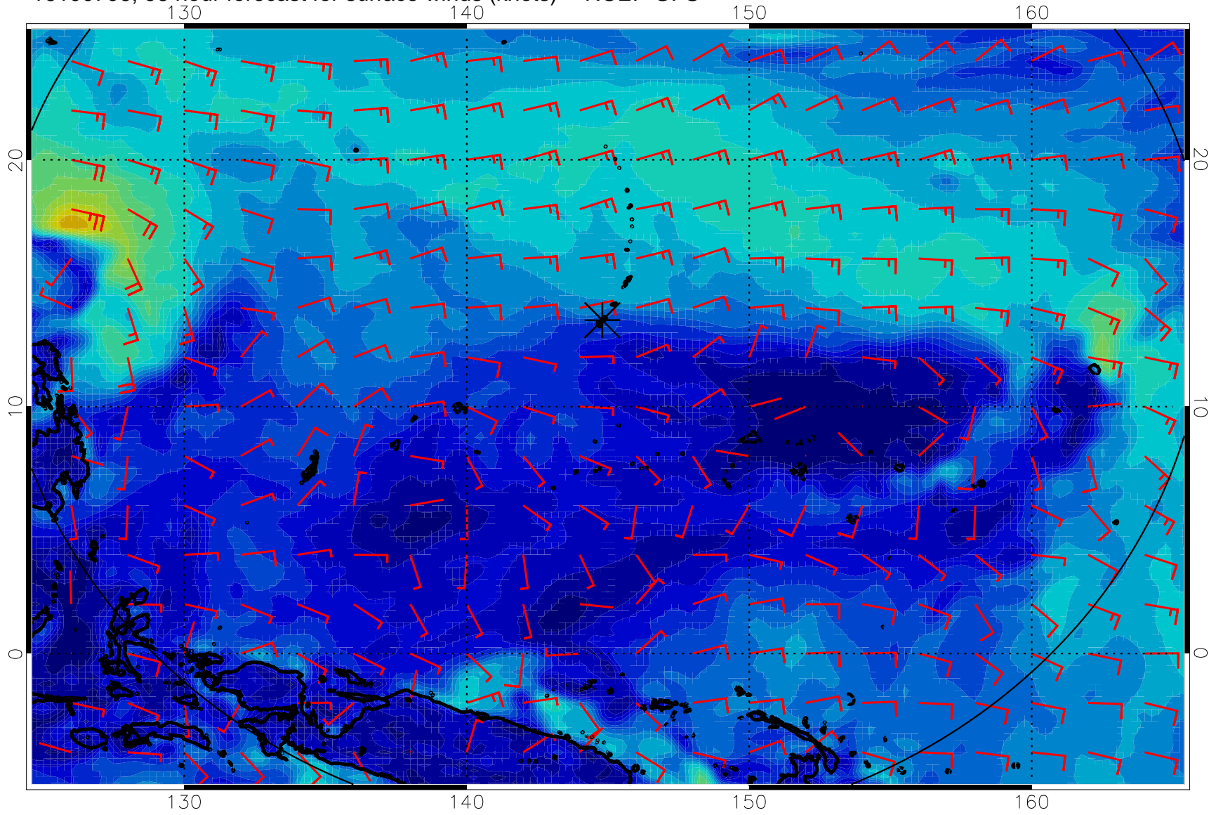
16100706, 96 hour forecast for surface winds (knots) -- NCEP GFS
