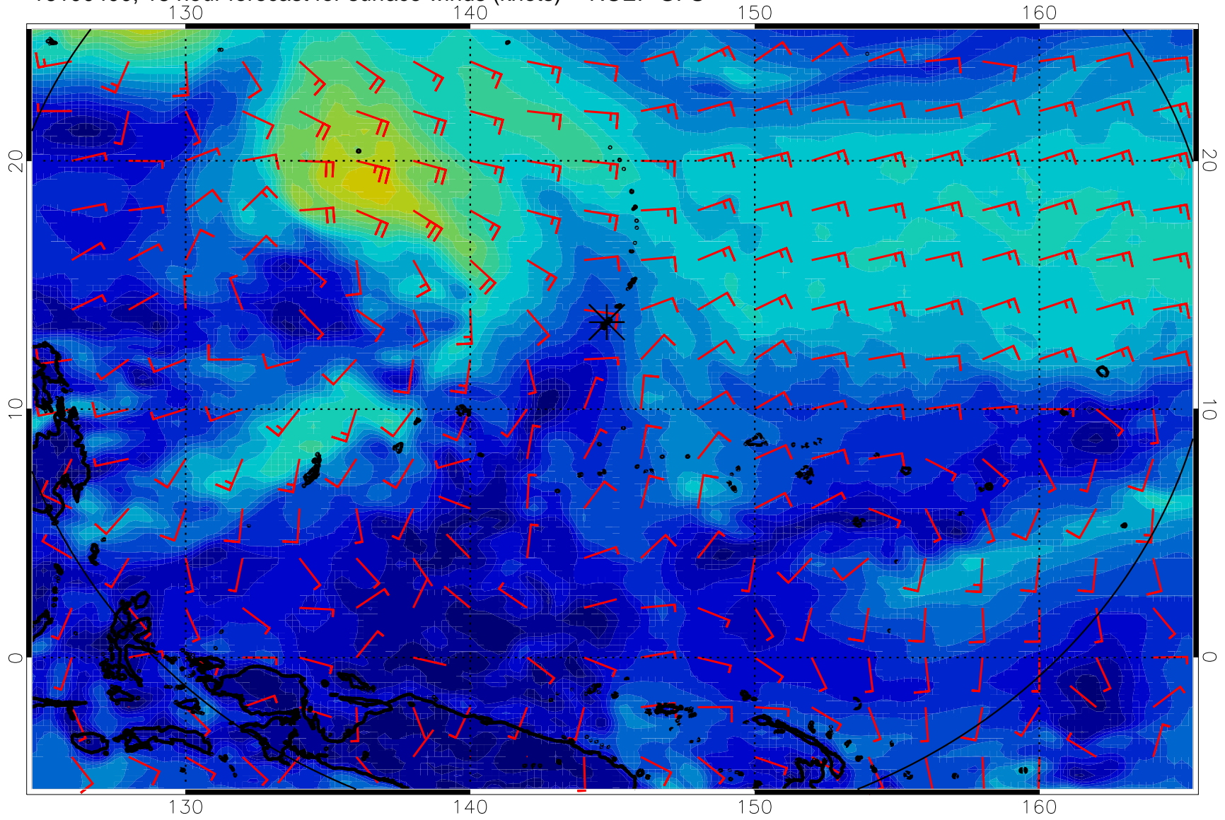
16100400, 18 hour forecast for surface winds (knots) -- NCEP GFS
