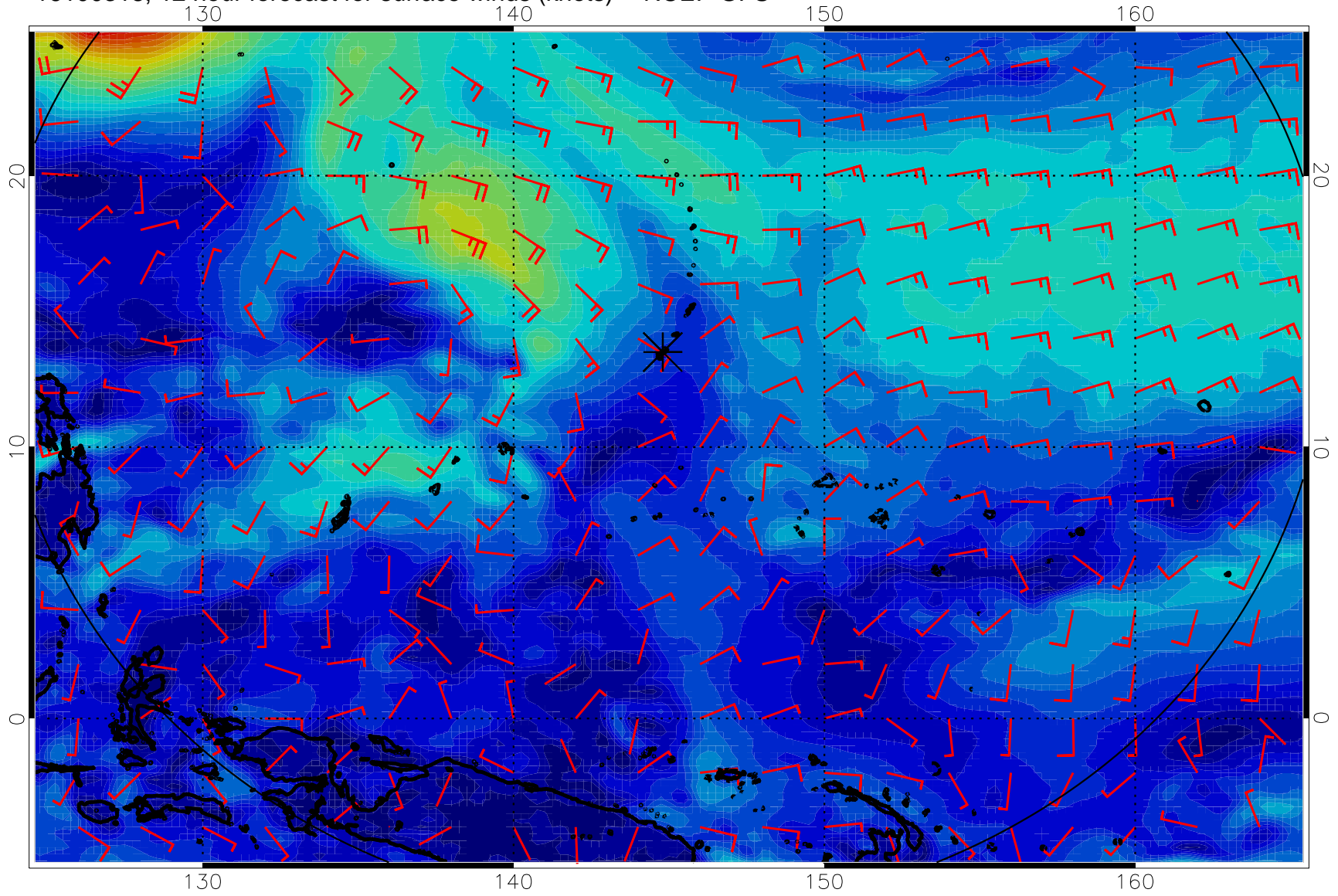
16100318, 12 hour forecast for surface winds (knots) -- NCEP GFS
