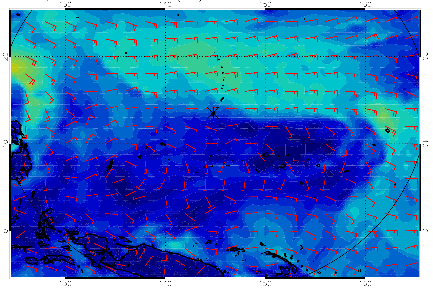
16100718, 108 hour forecast for surface winds (knots) -- NCEP GFS
