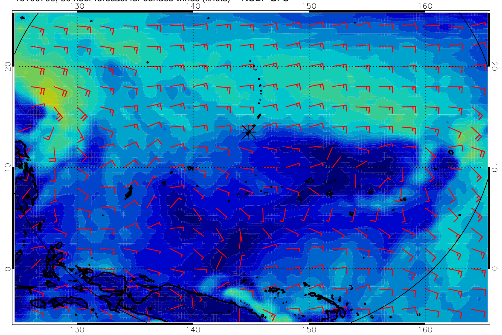
16100700, 90 hour forecast for surface winds (knots) -- NCEP GFS
