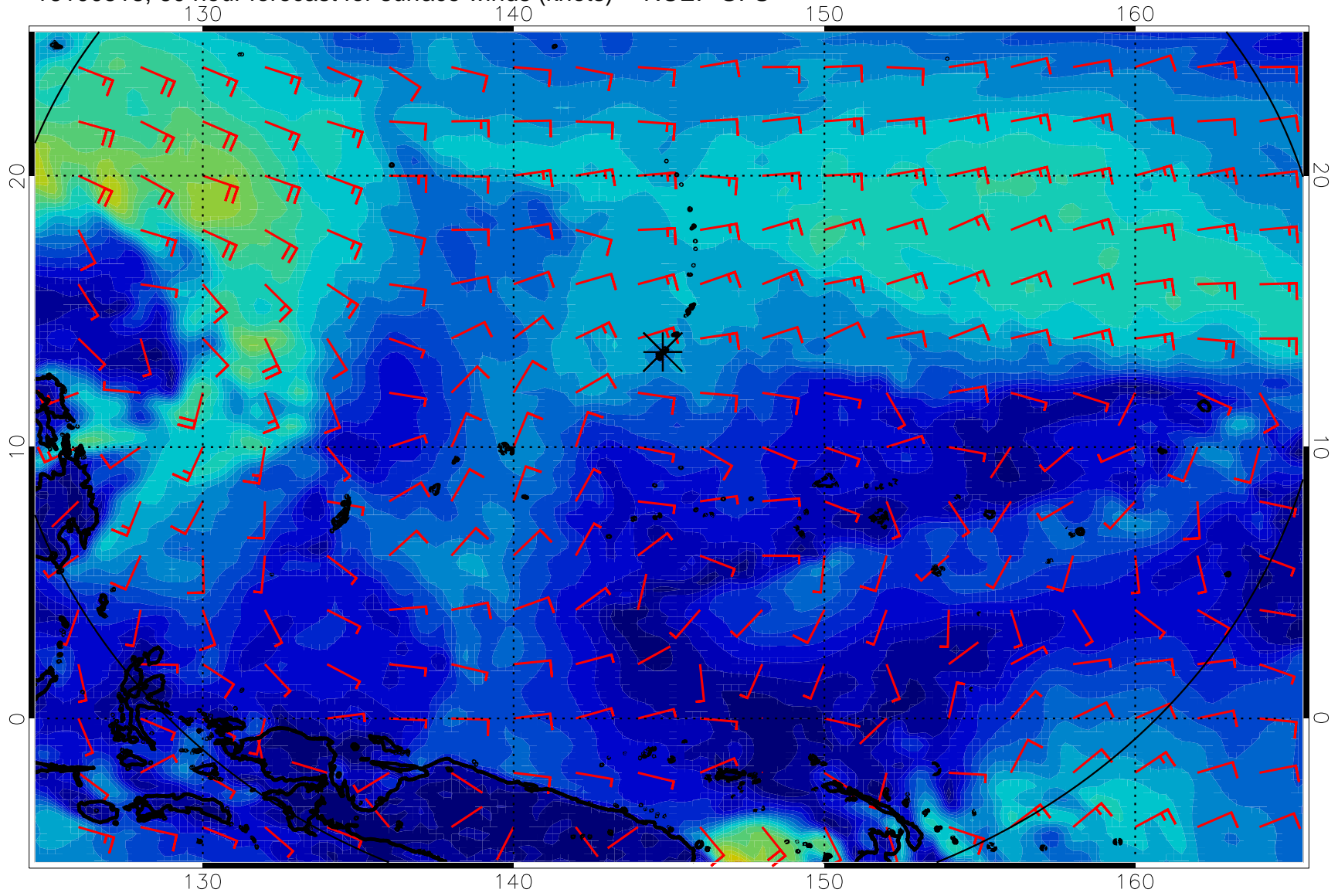
16100518, 60 hour forecast for surface winds (knots) -- NCEP GFS
