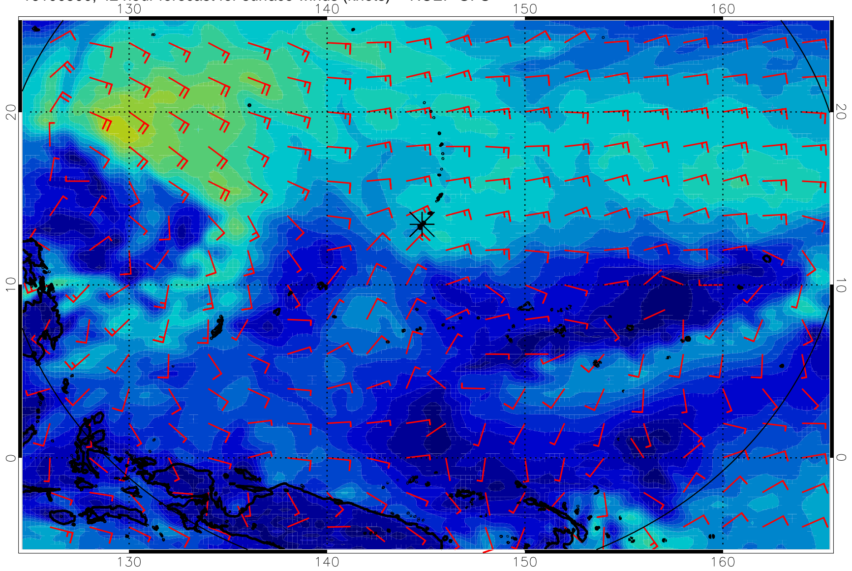
16100500, 42 hour forecast for surface winds (knots) -- NCEP GFS
