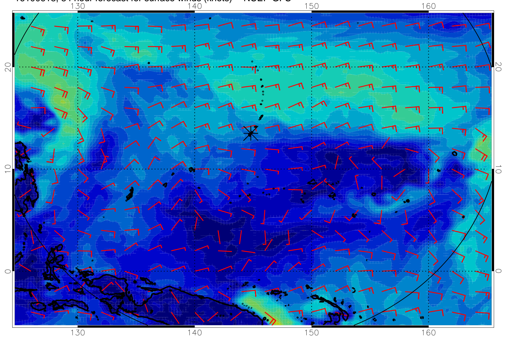
16100618, 84 hour forecast for surface winds (knots) -- NCEP GFS
