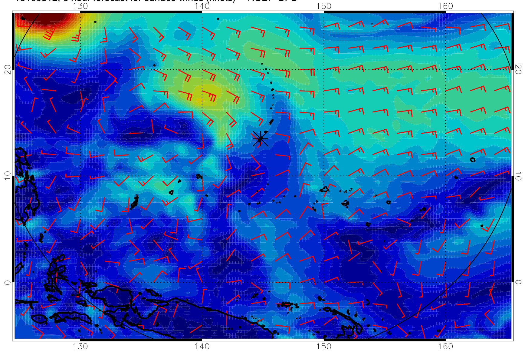
16100312, 6 hour forecast for surface winds (knots) -- NCEP GFS
