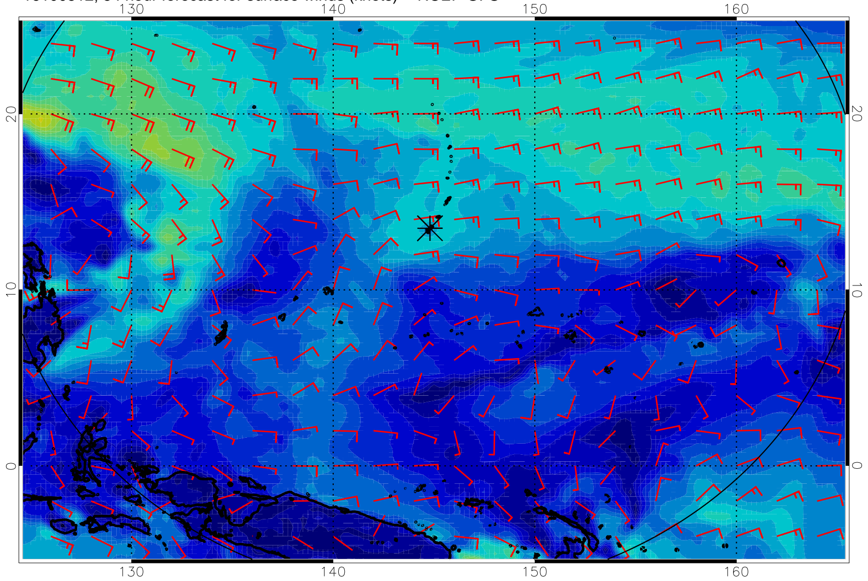
16100512, 54 hour forecast for surface winds (knots) -- NCEP GFS
