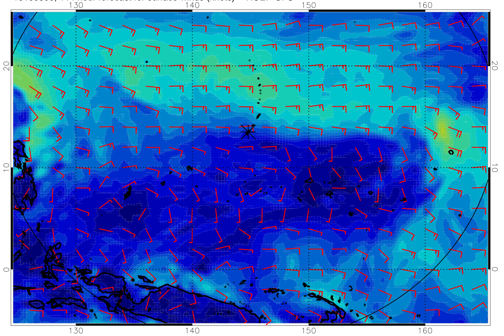
16100800, 114 hour forecast for surface winds (knots) -- NCEP GFS
