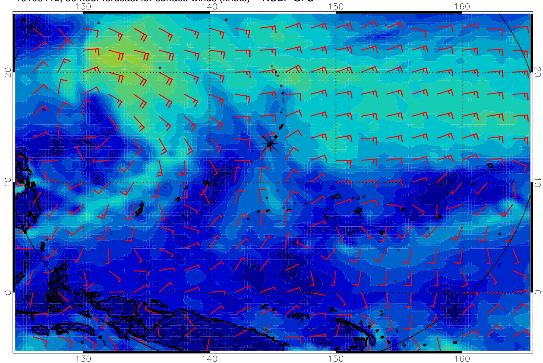
16100412, 30 hour forecast for surface winds (knots) -- NCEP GFS
