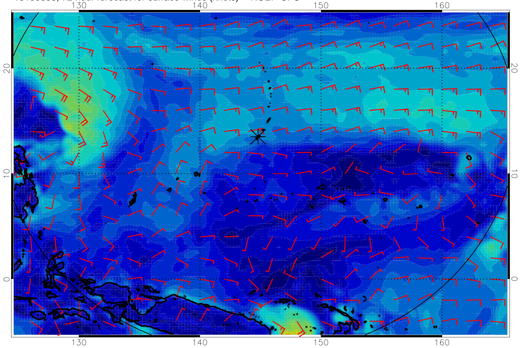
16100606, 72 hour forecast for surface winds (knots) -- NCEP GFS
