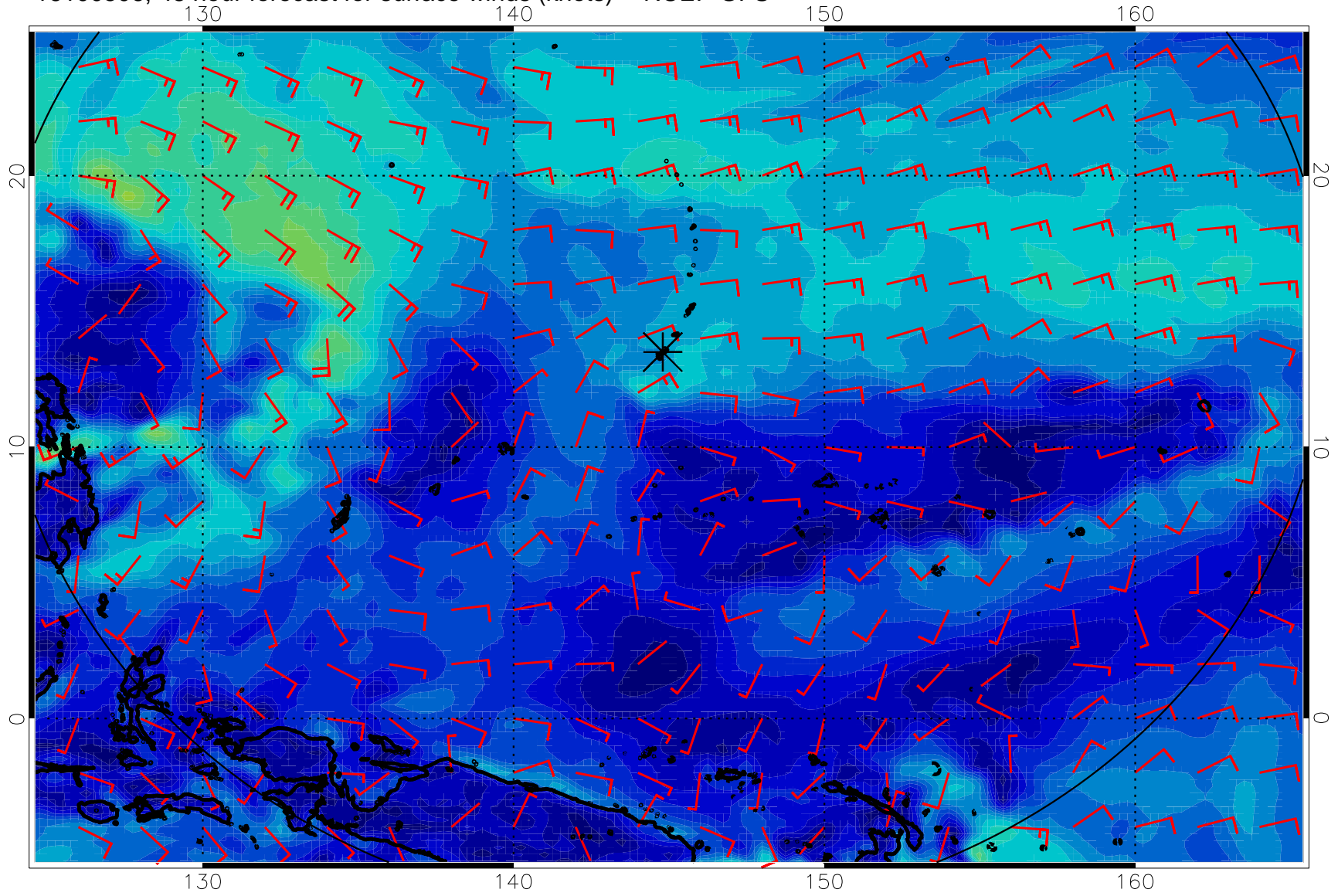
16100506, 48 hour forecast for surface winds (knots) -- NCEP GFS
