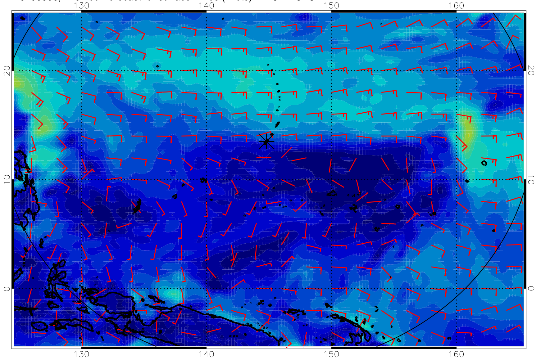
16100806, 120 hour forecast for surface winds (knots) -- NCEP GFS
