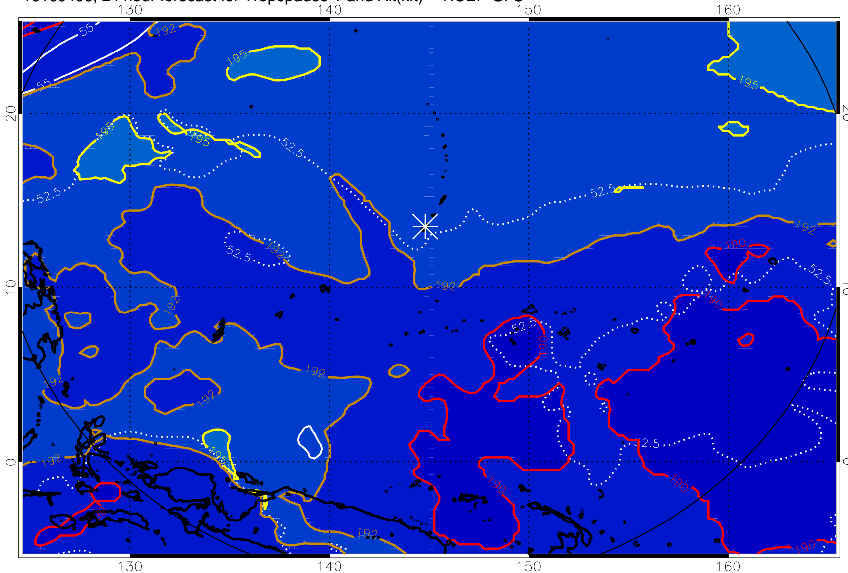
16100406, 24 hour forecast for Tropopause T and Alt(kft) -- NCEP GFS
