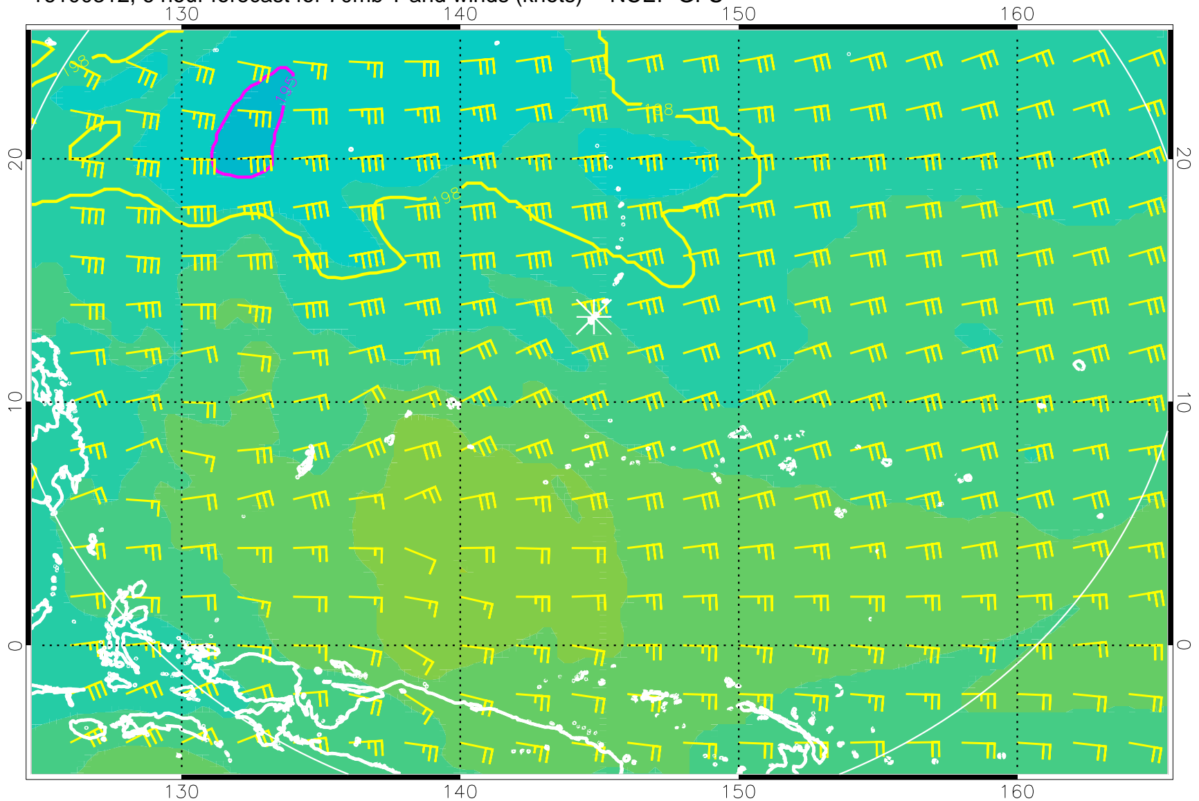
16100312, 6 hour forecast for 70mb T and winds (knots) -- NCEP GFS
