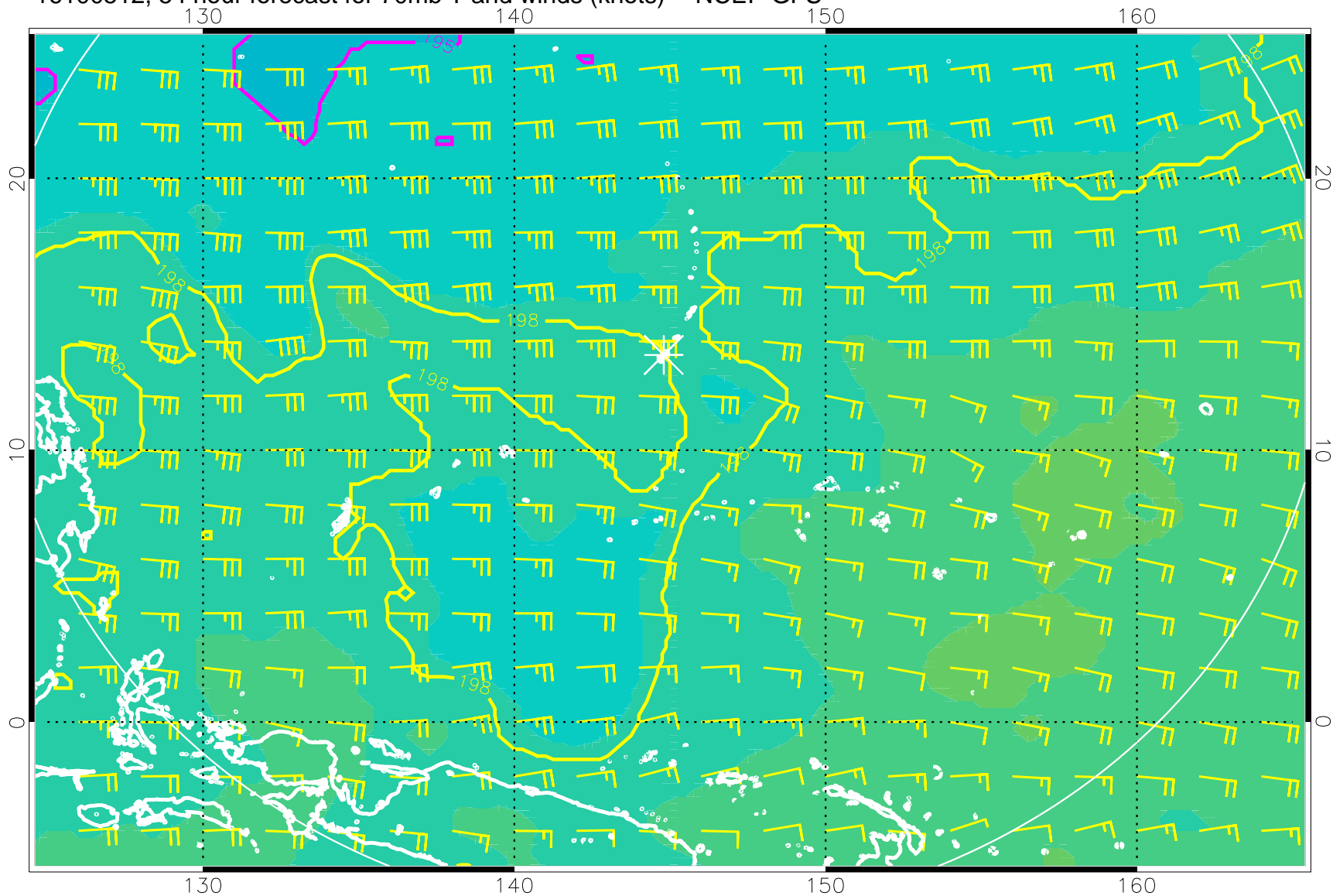
16100512, 54 hour forecast for 70mb T and winds (knots) -- NCEP GFS
