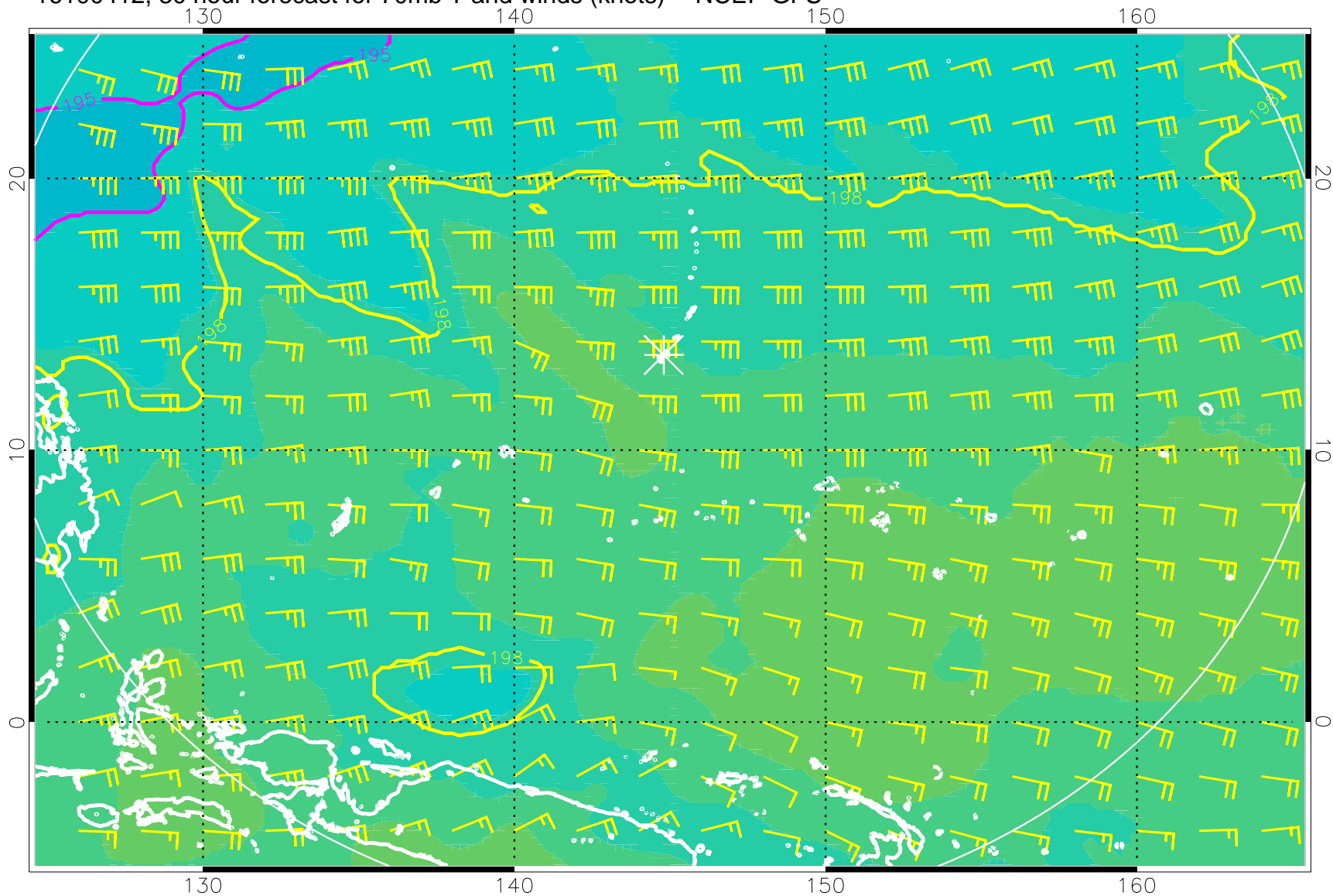
16100412, 30 hour forecast for 70mb T and winds (knots) -- NCEP GFS
