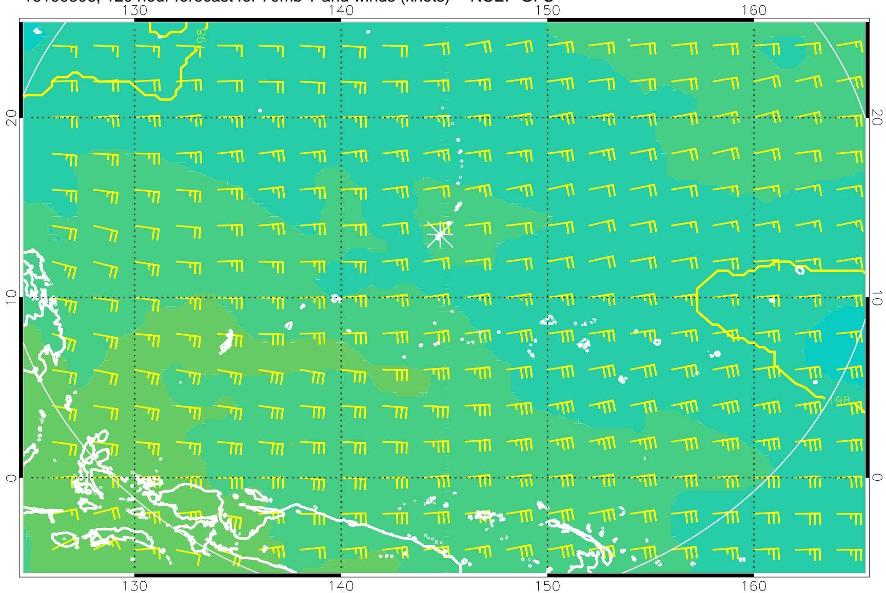
16100806, 120 hour forecast for 70mb T and winds (knots) -- NCEP GFS
