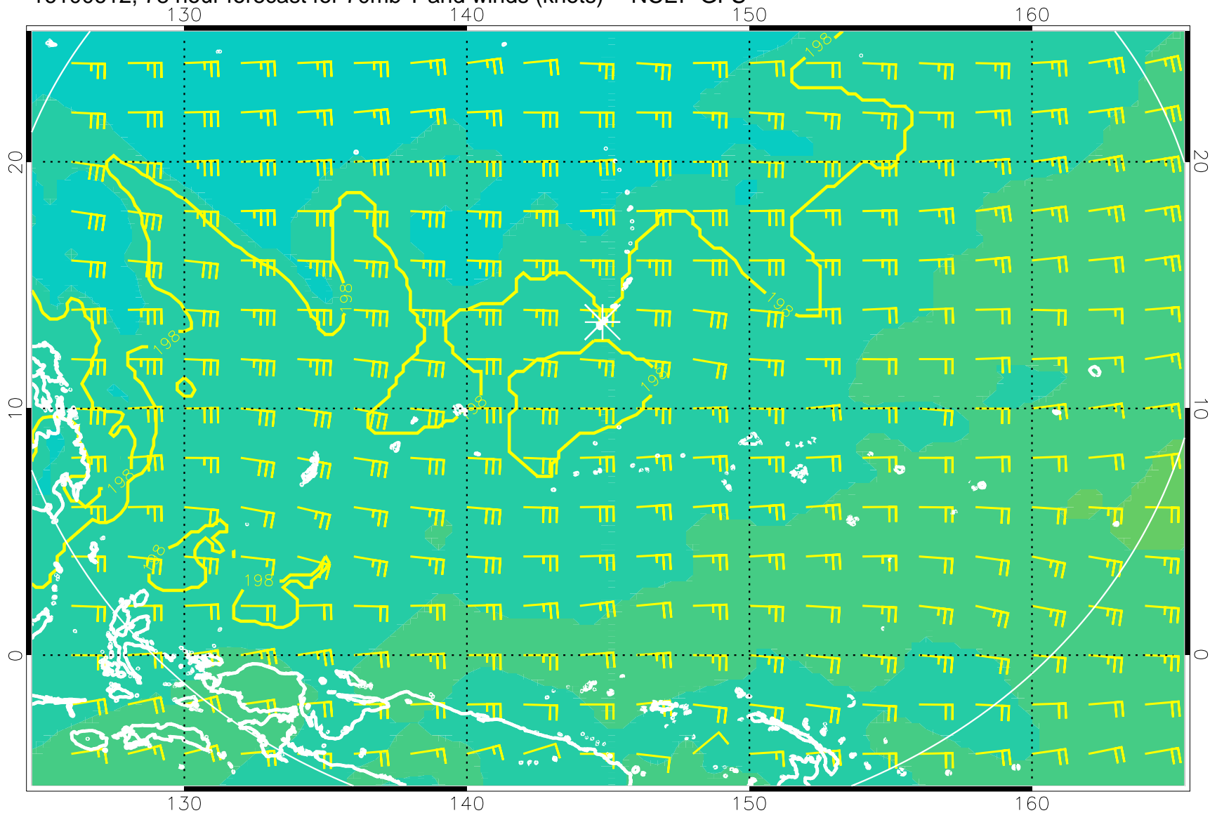
16100612, 78 hour forecast for 70mb T and winds (knots) -- NCEP GFS
