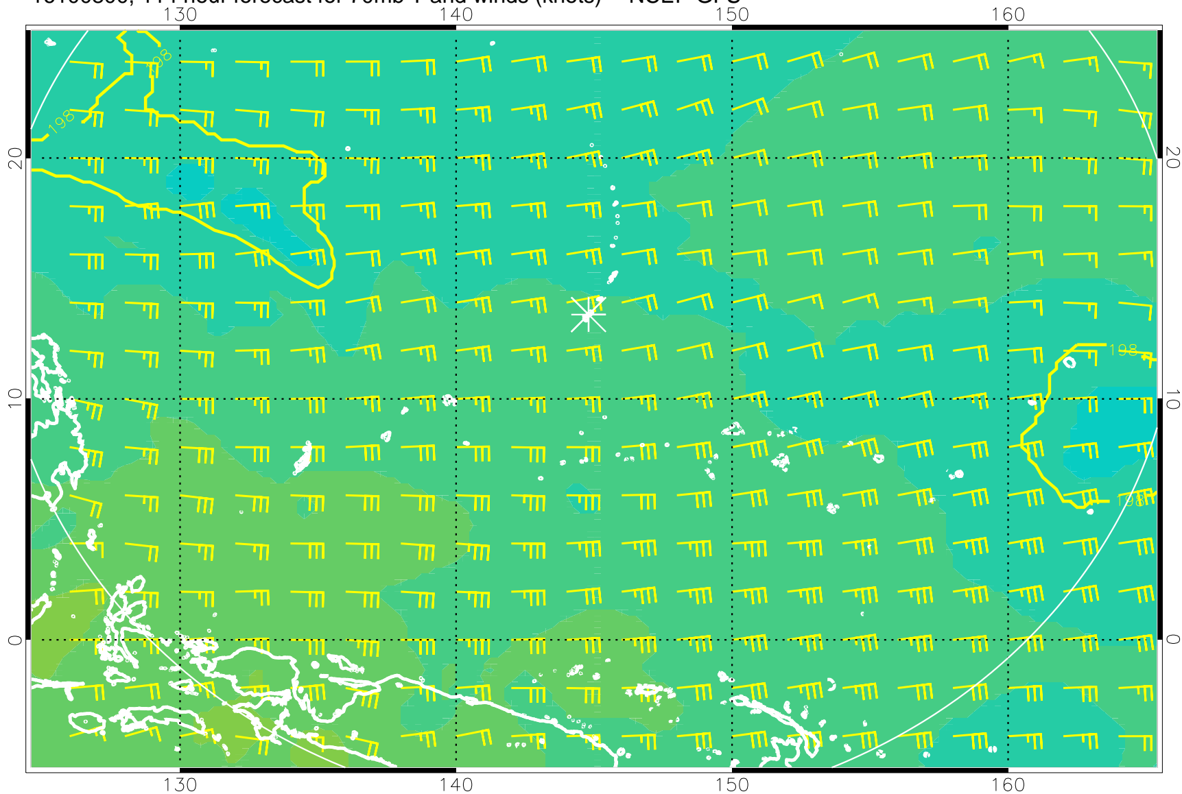
16100800, 114 hour forecast for 70mb T and winds (knots) -- NCEP GFS
