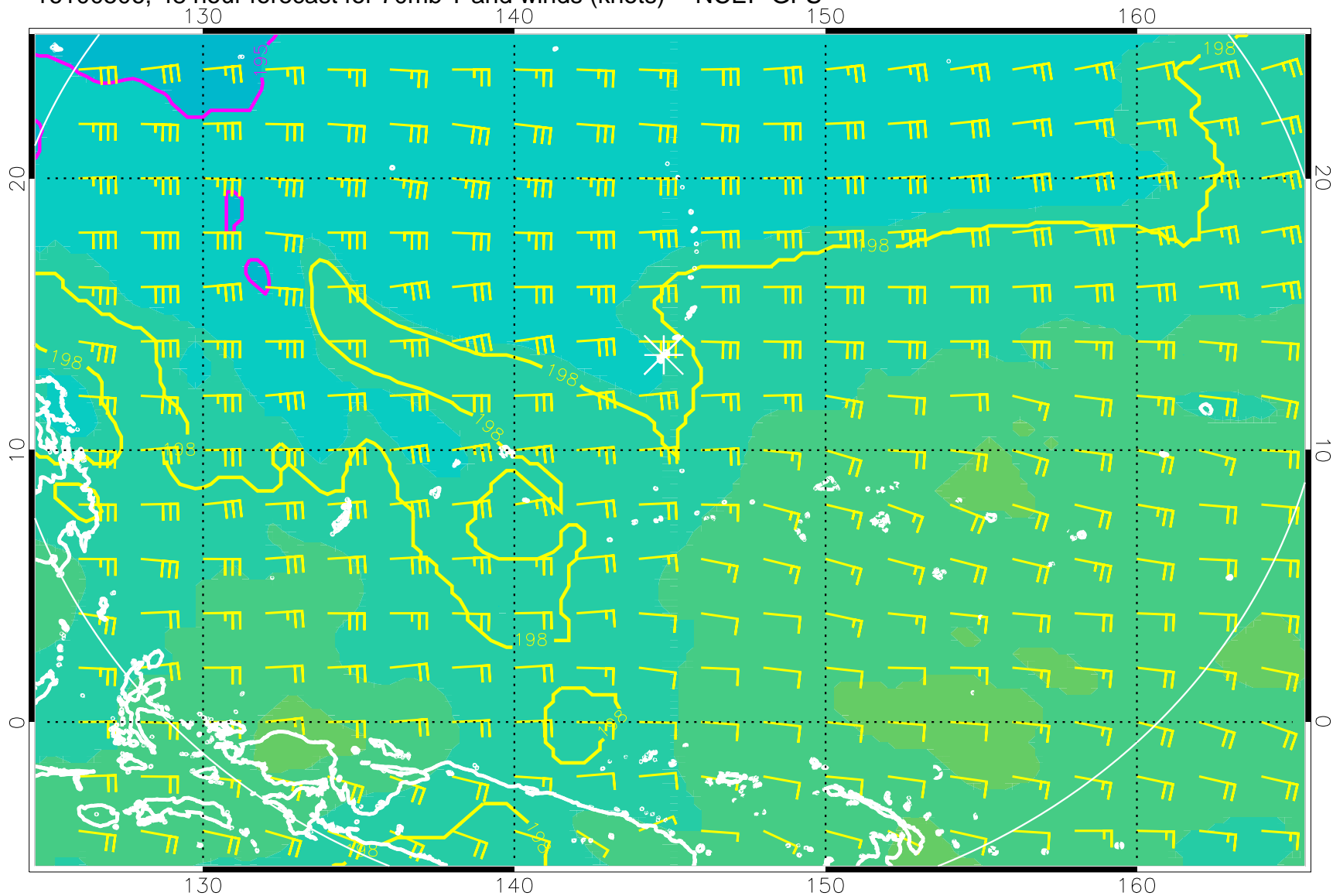
16100506, 48 hour forecast for 70mb T and winds (knots) -- NCEP GFS
