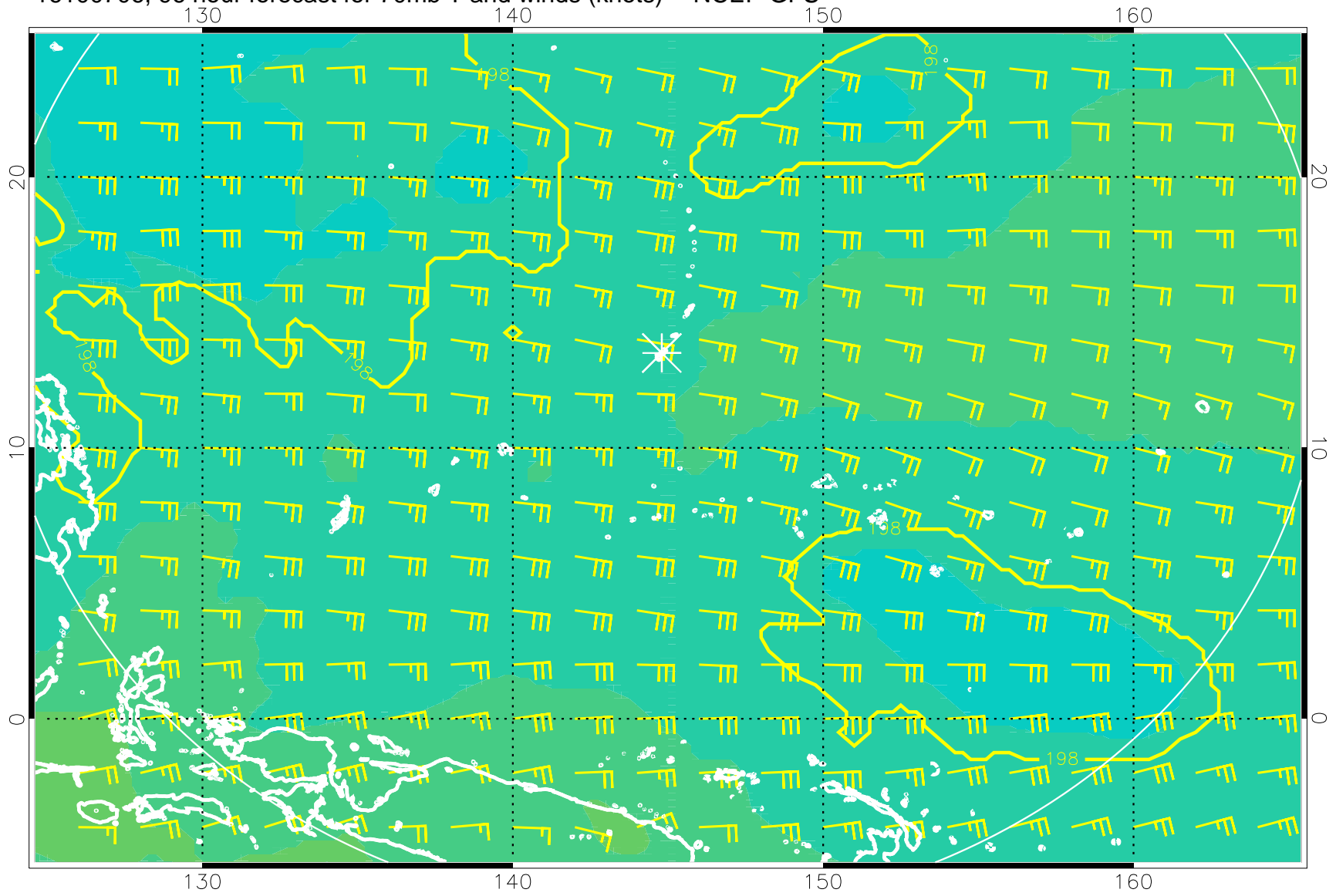
16100706, 96 hour forecast for 70mb T and winds (knots) -- NCEP GFS
