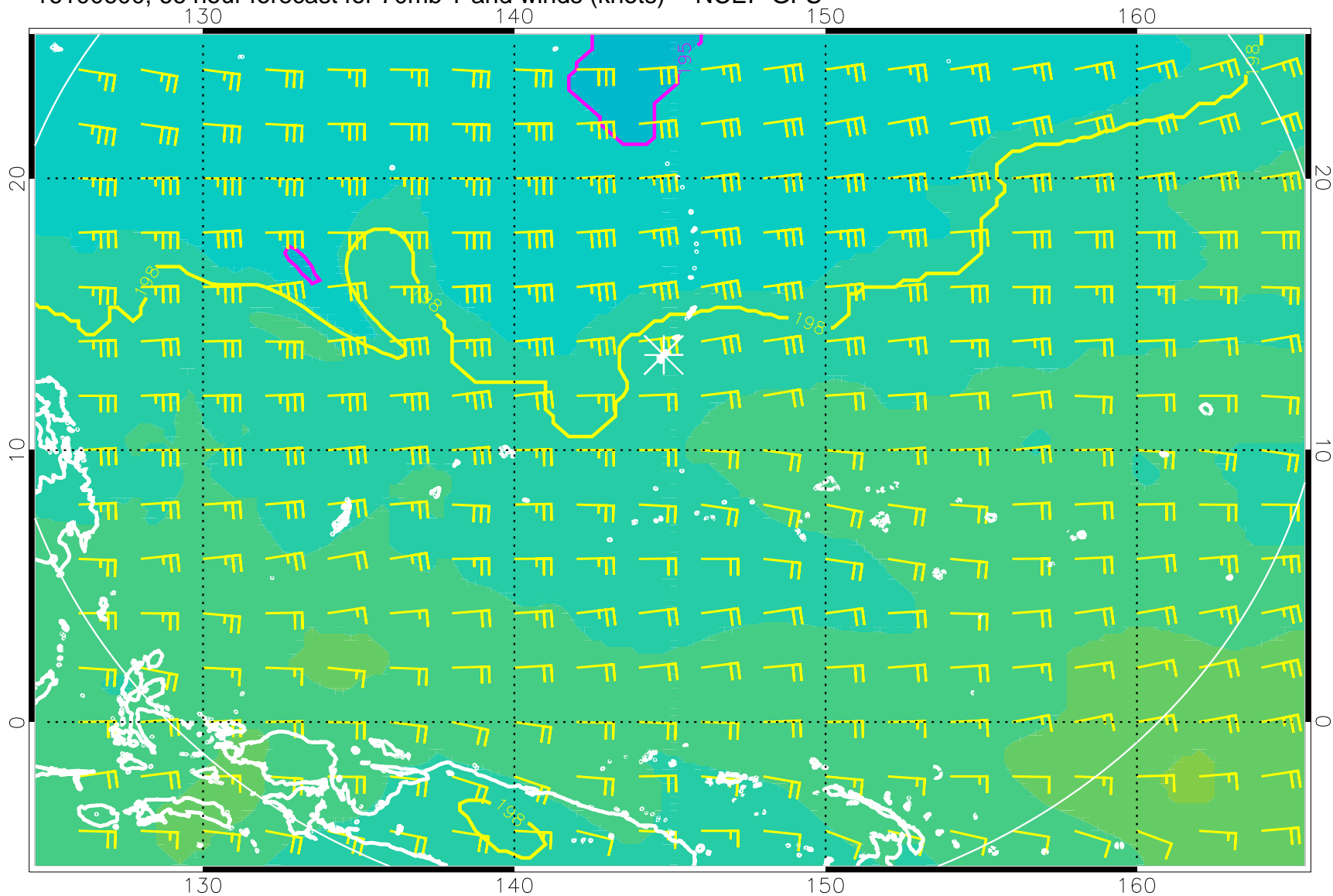
16100600, 66 hour forecast for 70mb T and winds (knots) -- NCEP GFS
