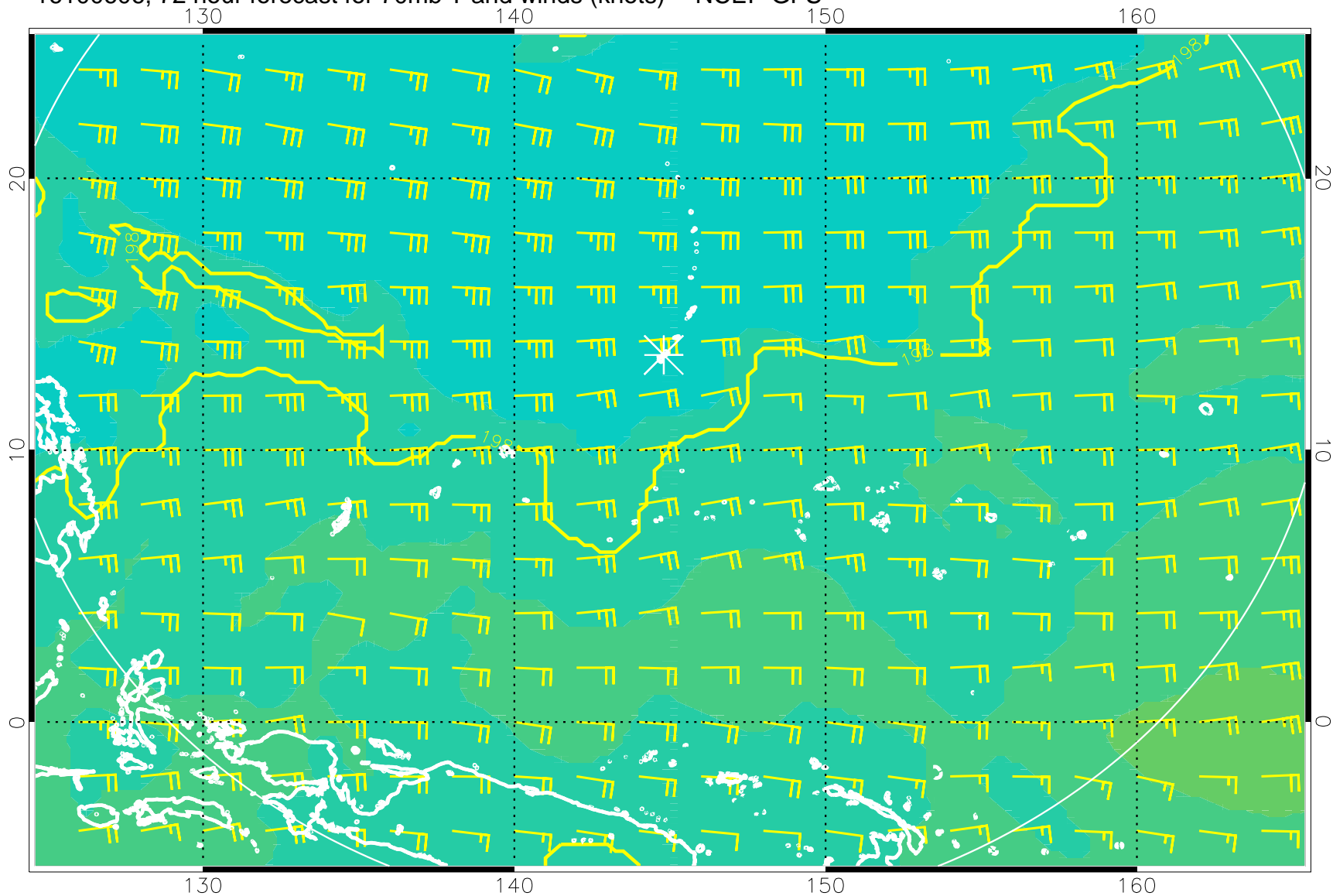
16100606, 72 hour forecast for 70mb T and winds (knots) -- NCEP GFS
