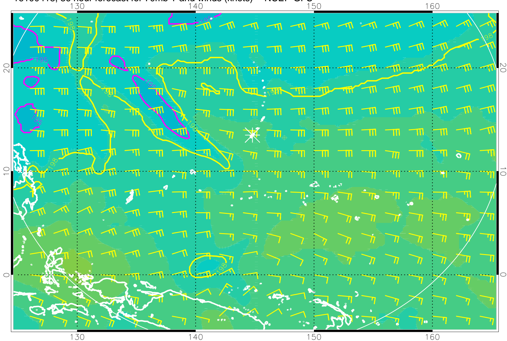
16100418, 36 hour forecast for 70mb T and winds (knots) -- NCEP GFS
