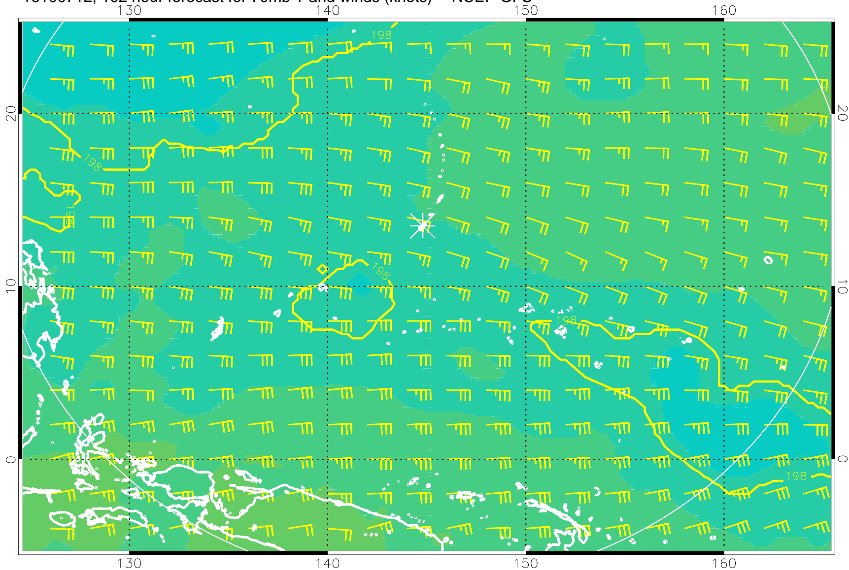
16100712, 102 hour forecast for 70mb T and winds (knots) -- NCEP GFS
