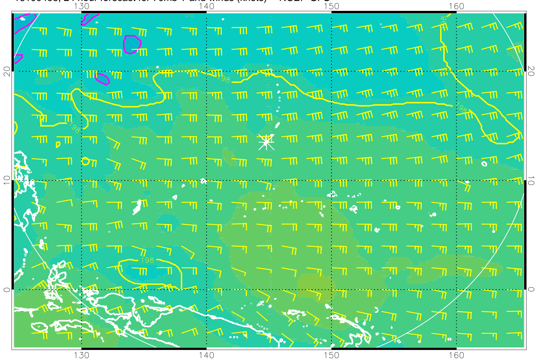
16100406, 24 hour forecast for 70mb T and winds (knots) -- NCEP GFS
