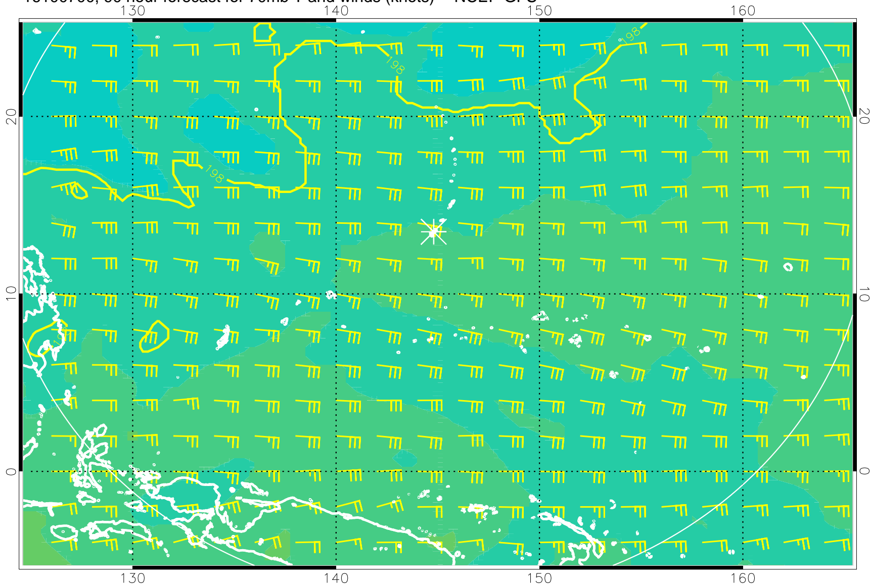
16100700, 90 hour forecast for 70mb T and winds (knots) -- NCEP GFS
