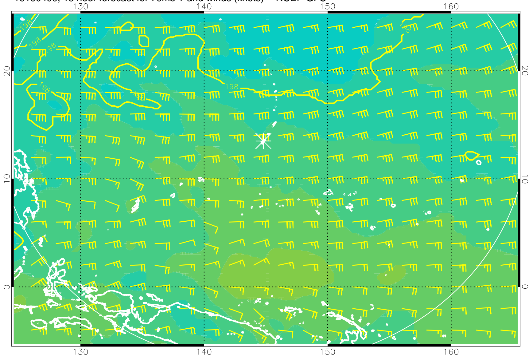
16100400, 18 hour forecast for 70mb T and winds (knots) -- NCEP GFS
