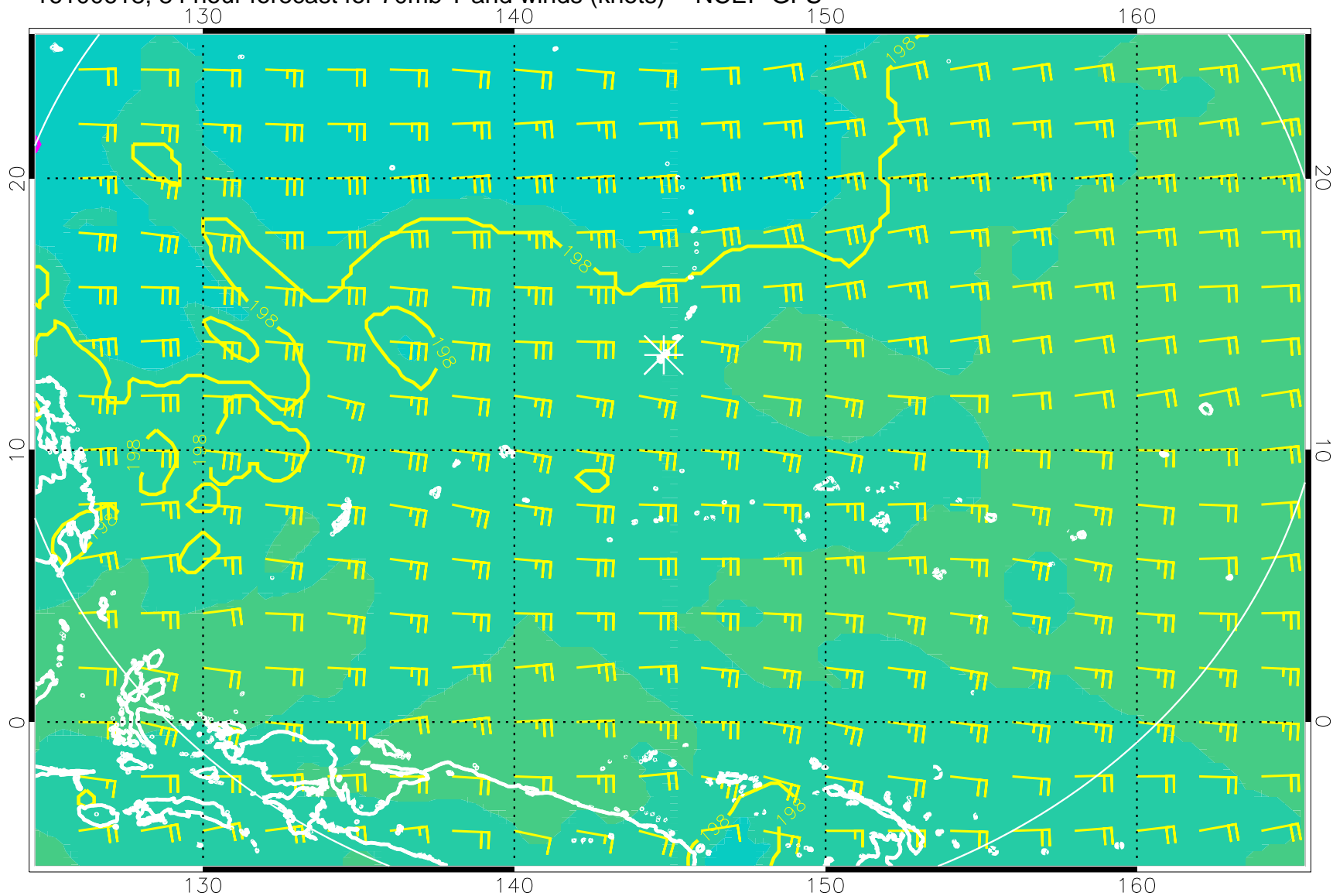
16100618, 84 hour forecast for 70mb T and winds (knots) -- NCEP GFS
