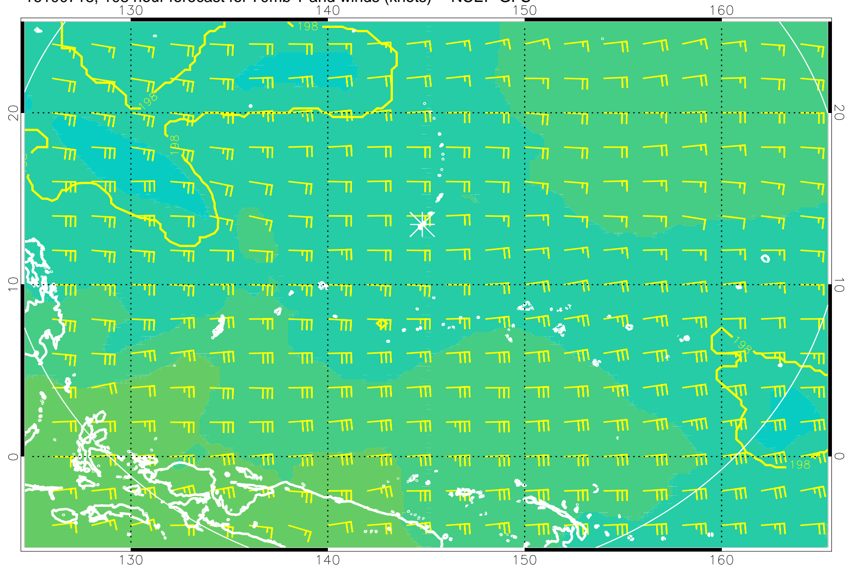
16100718, 108 hour forecast for 70mb T and winds (knots) -- NCEP GFS
