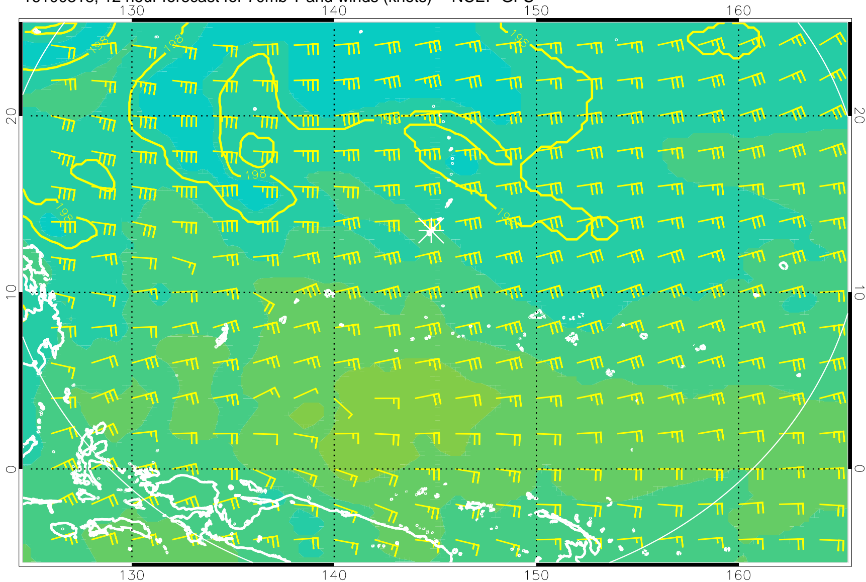
16100318, 12 hour forecast for 70mb T and winds (knots) -- NCEP GFS
