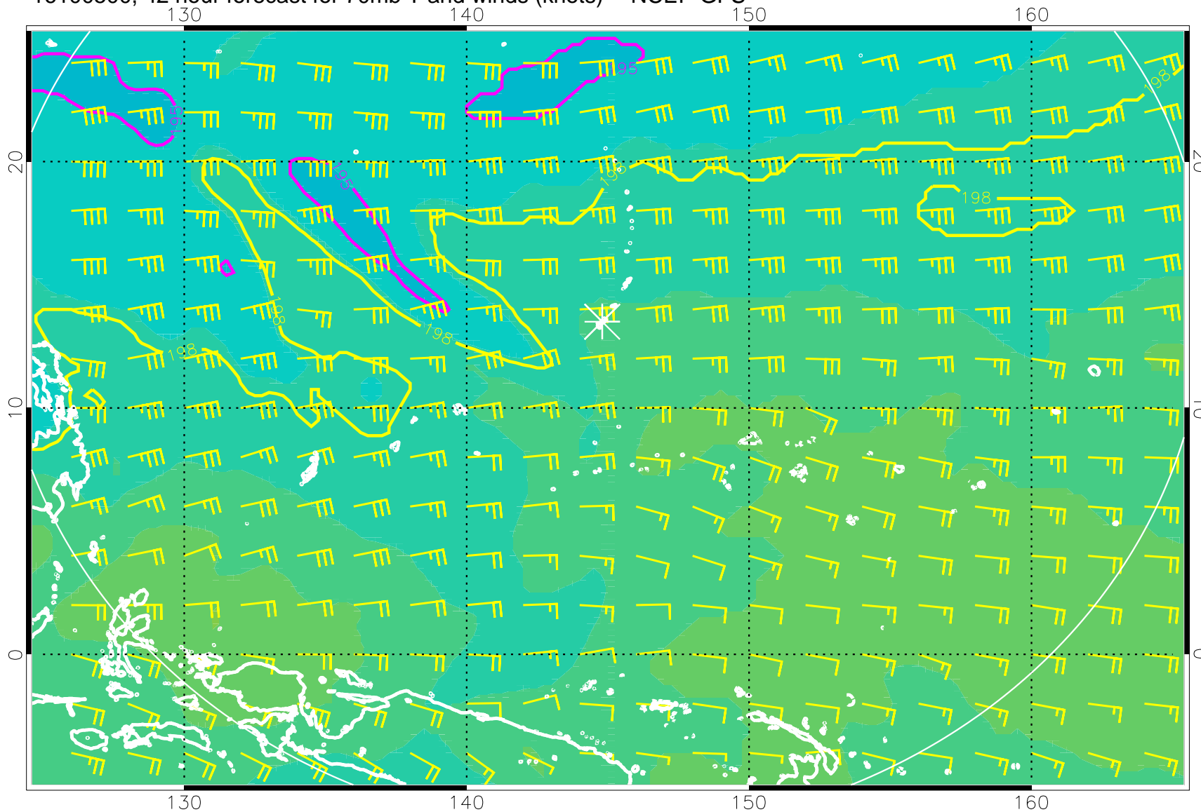
16100500, 42 hour forecast for 70mb T and winds (knots) -- NCEP GFS
