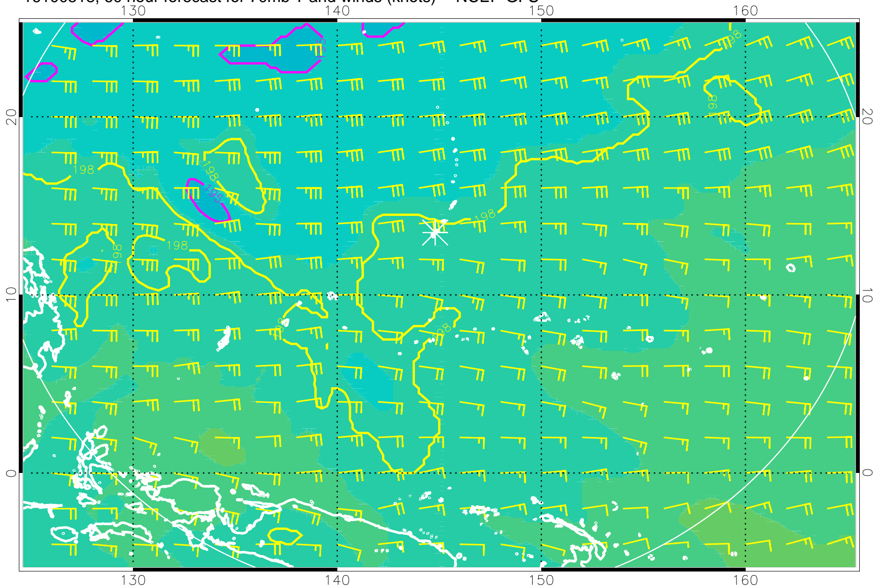
16100518, 60 hour forecast for 70mb T and winds (knots) -- NCEP GFS
