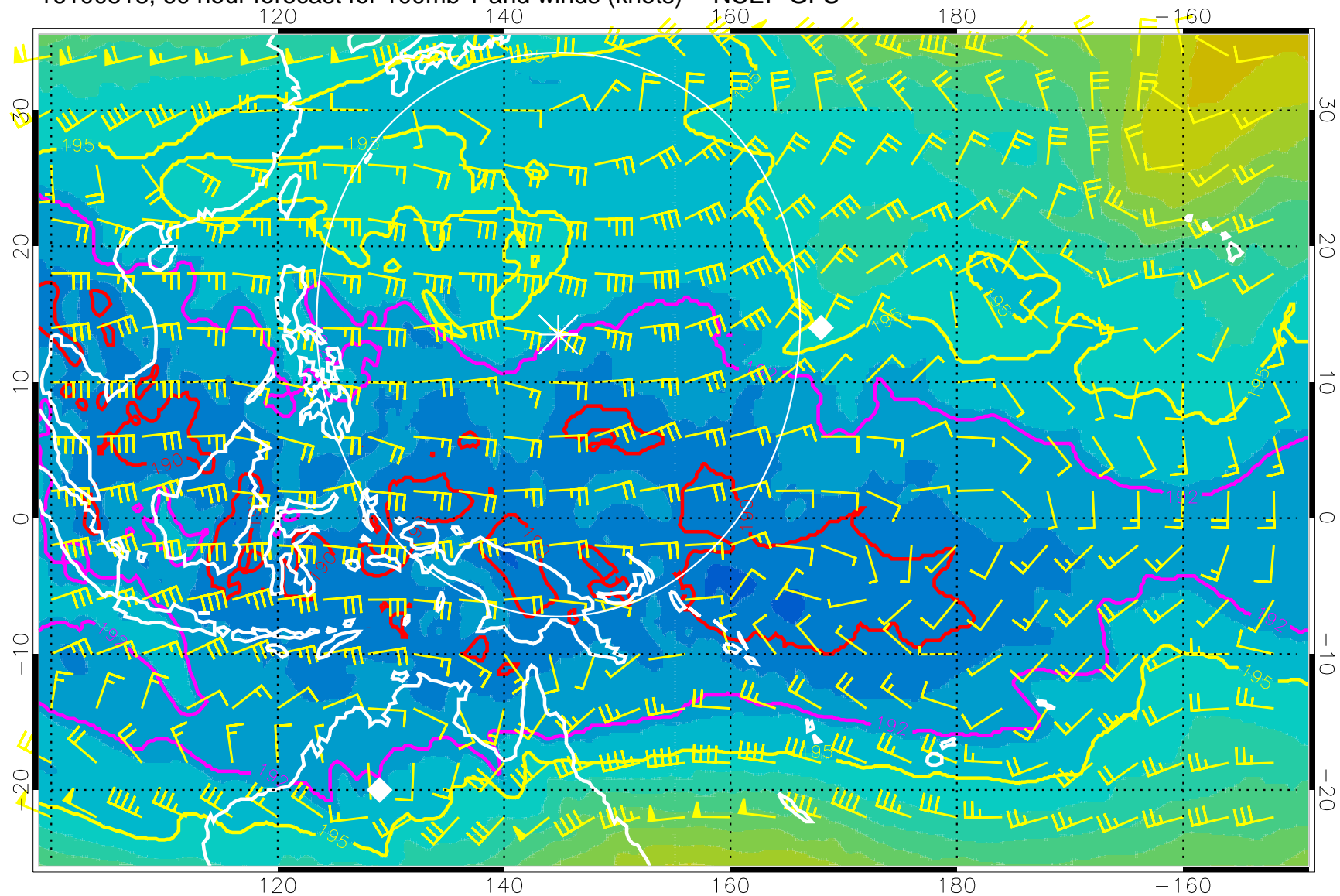
16100518, 60 hour forecast for 100mb T and winds (knots) -- NCEP GFS
