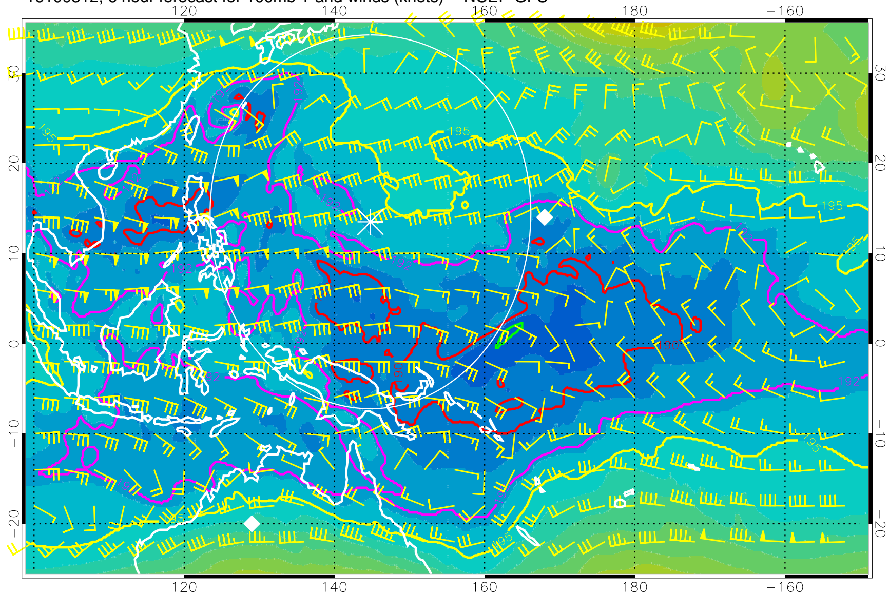
16100312, 6 hour forecast for 100mb T and winds (knots) -- NCEP GFS
