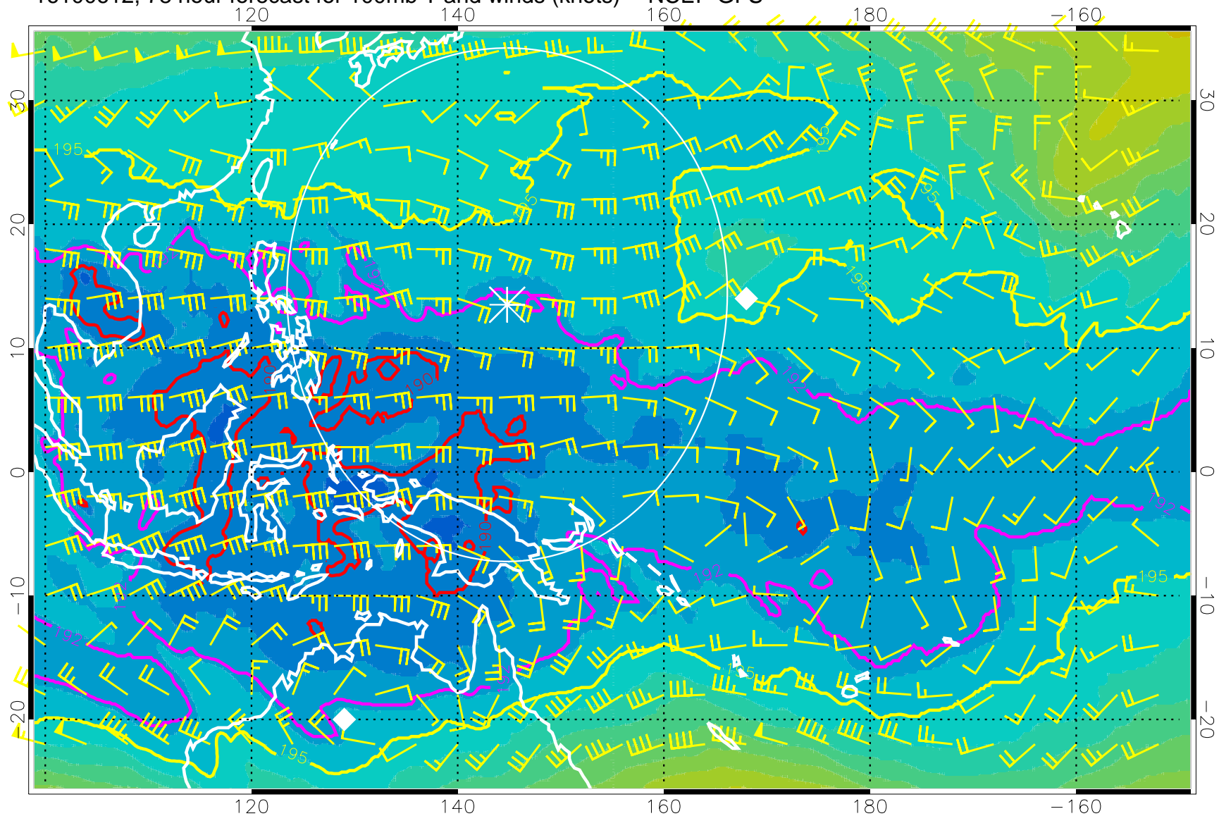
16100612, 78 hour forecast for 100mb T and winds (knots) -- NCEP GFS
