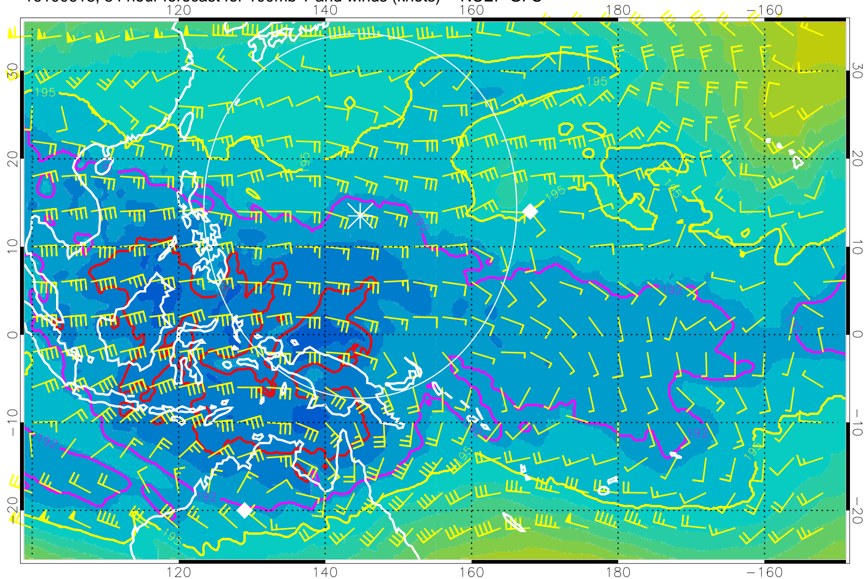
16100618, 84 hour forecast for 100mb T and winds (knots) -- NCEP GFS
