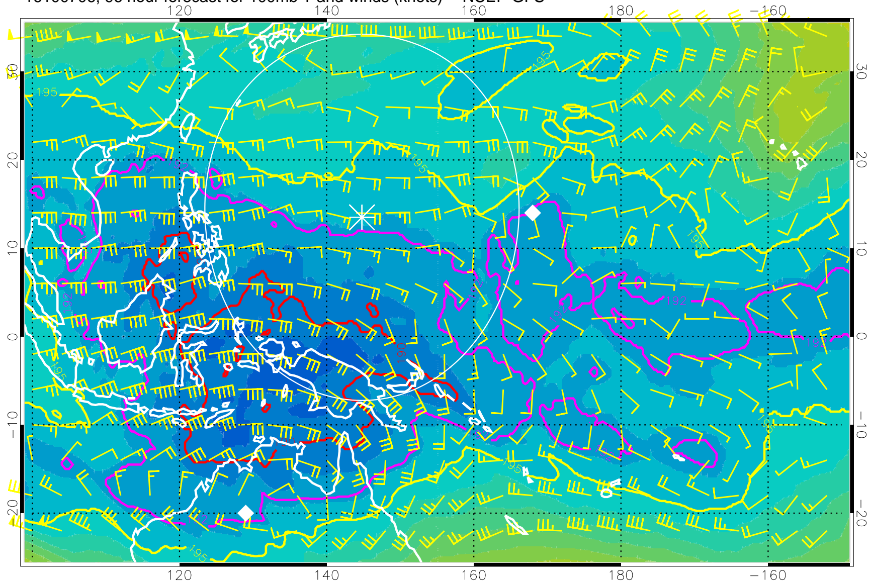
16100706, 96 hour forecast for 100mb T and winds (knots) -- NCEP GFS
