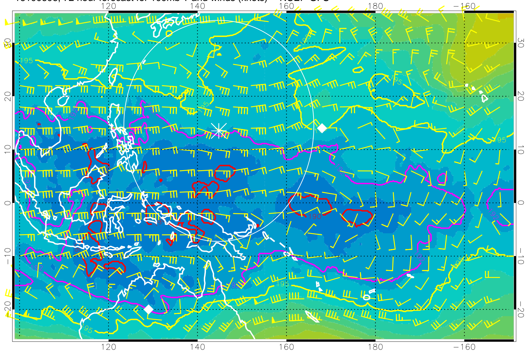
16100606, 72 hour forecast for 100mb T and winds (knots) -- NCEP GFS
