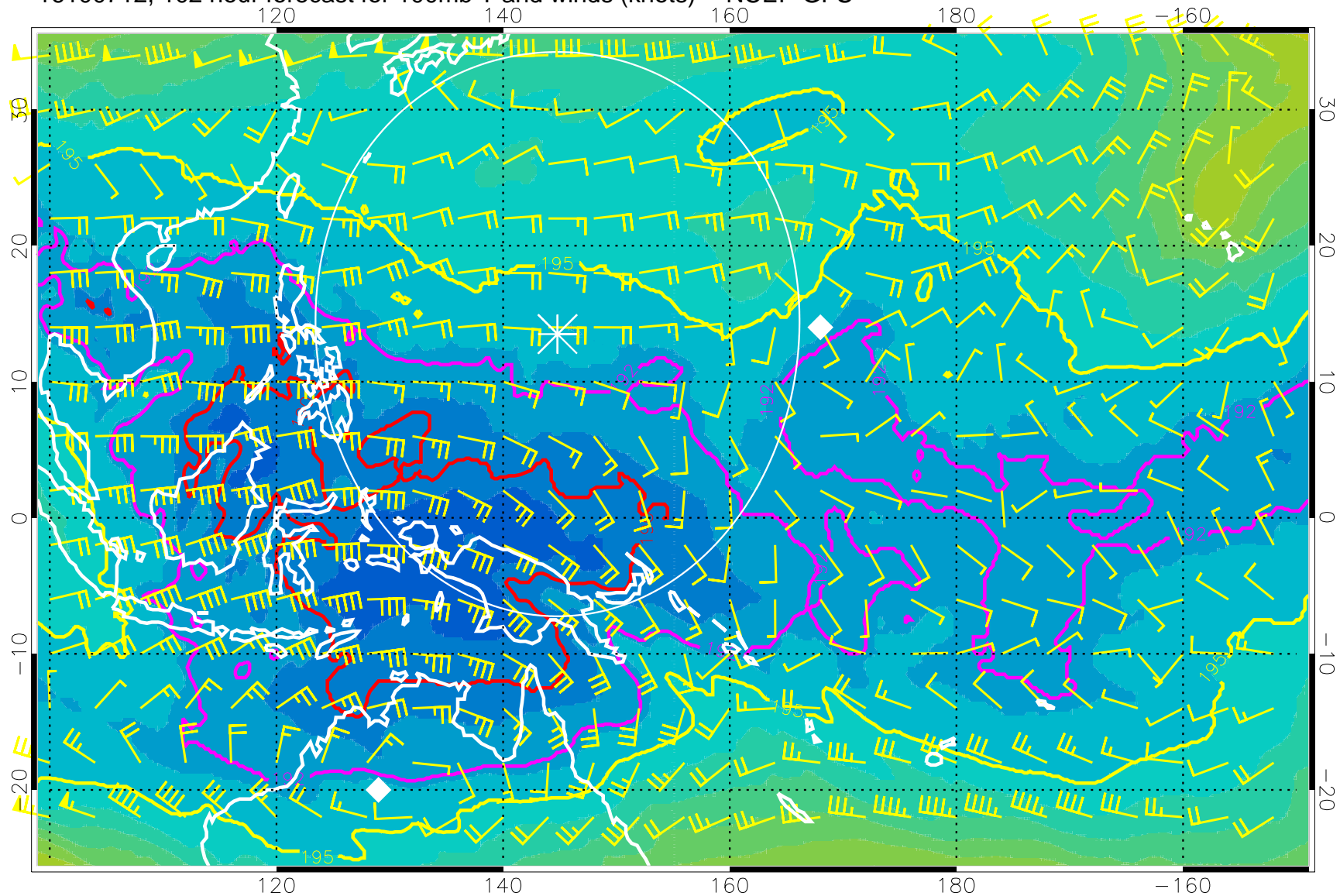
16100712, 102 hour forecast for 100mb T and winds (knots) -- NCEP GFS
