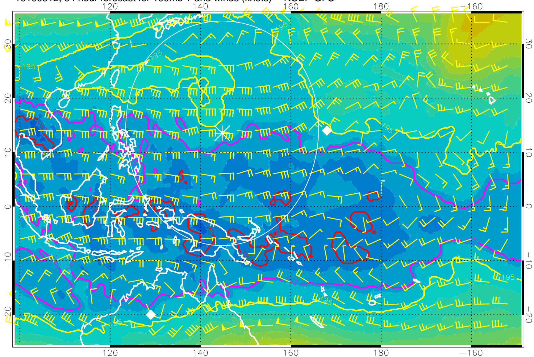
16100512, 54 hour forecast for 100mb T and winds (knots) -- NCEP GFS
