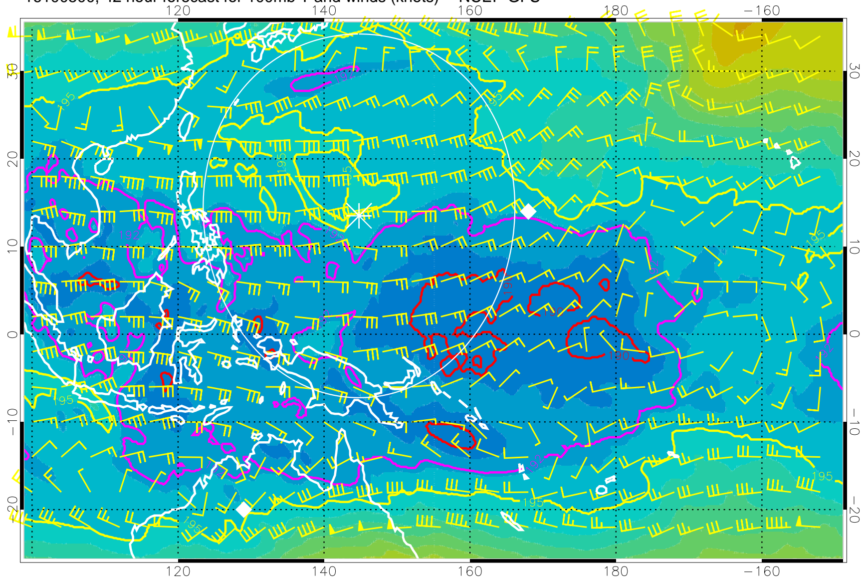
16100500, 42 hour forecast for 100mb T and winds (knots) -- NCEP GFS
