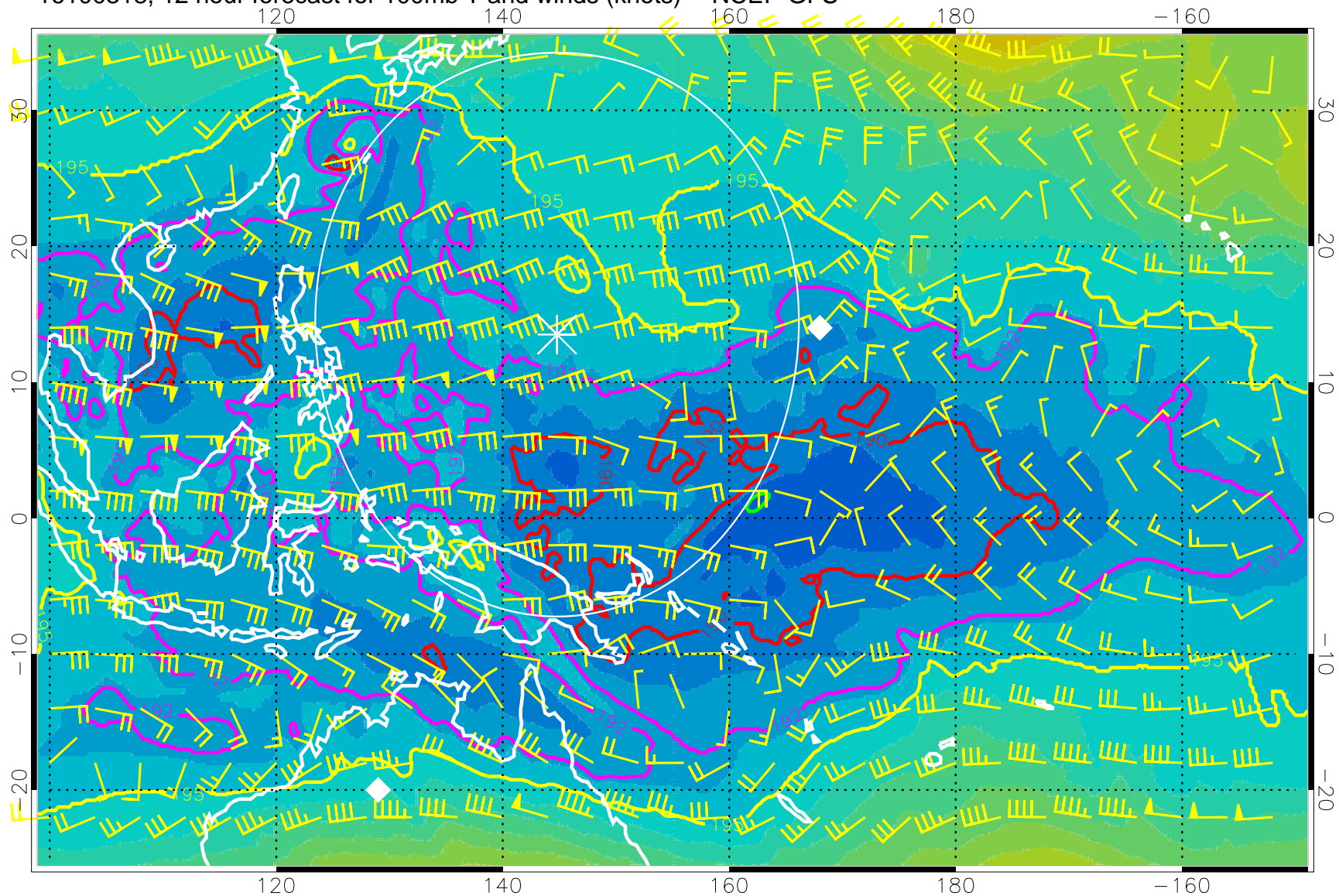
16100318, 12 hour forecast for 100mb T and winds (knots) -- NCEP GFS
