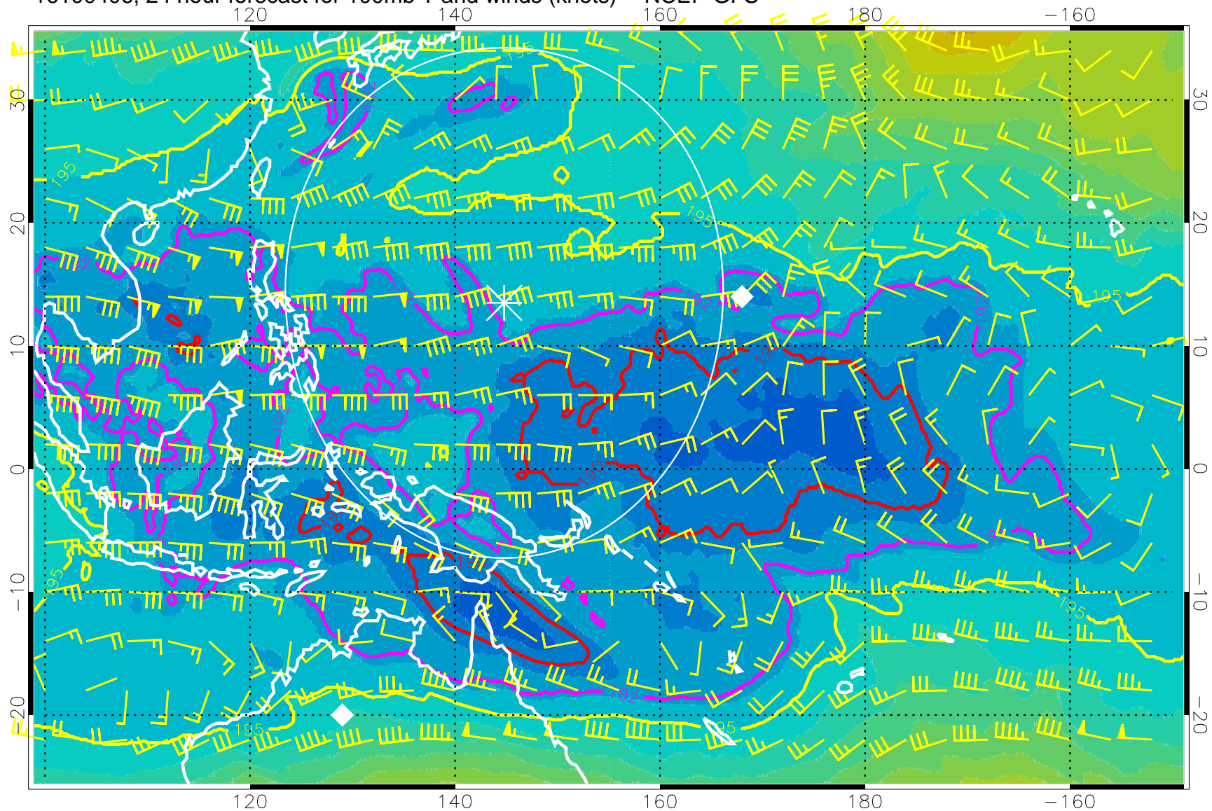
16100406, 24 hour forecast for 100mb T and winds (knots) -- NCEP GFS
