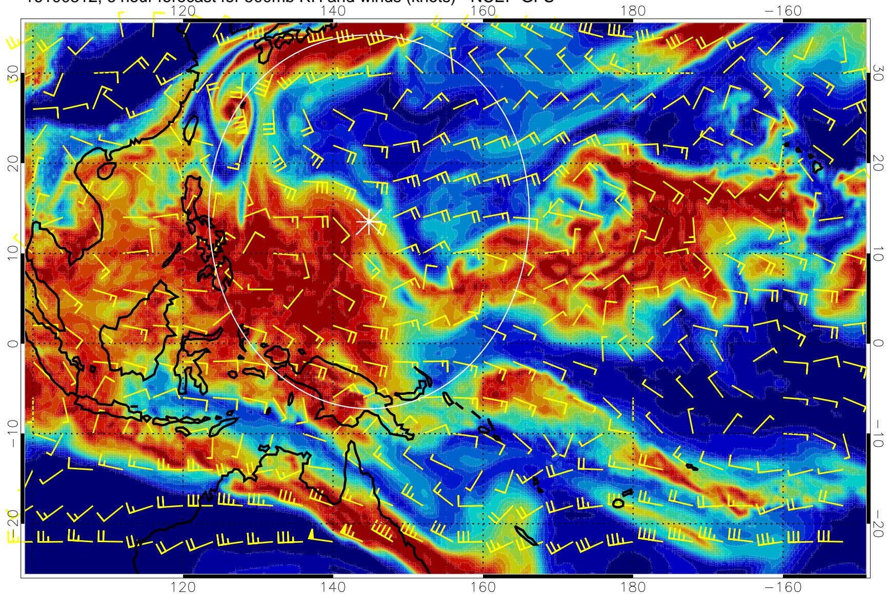
16100312, 6 hour forecast for 500mb RH and winds (knots) - NCEP GFS
