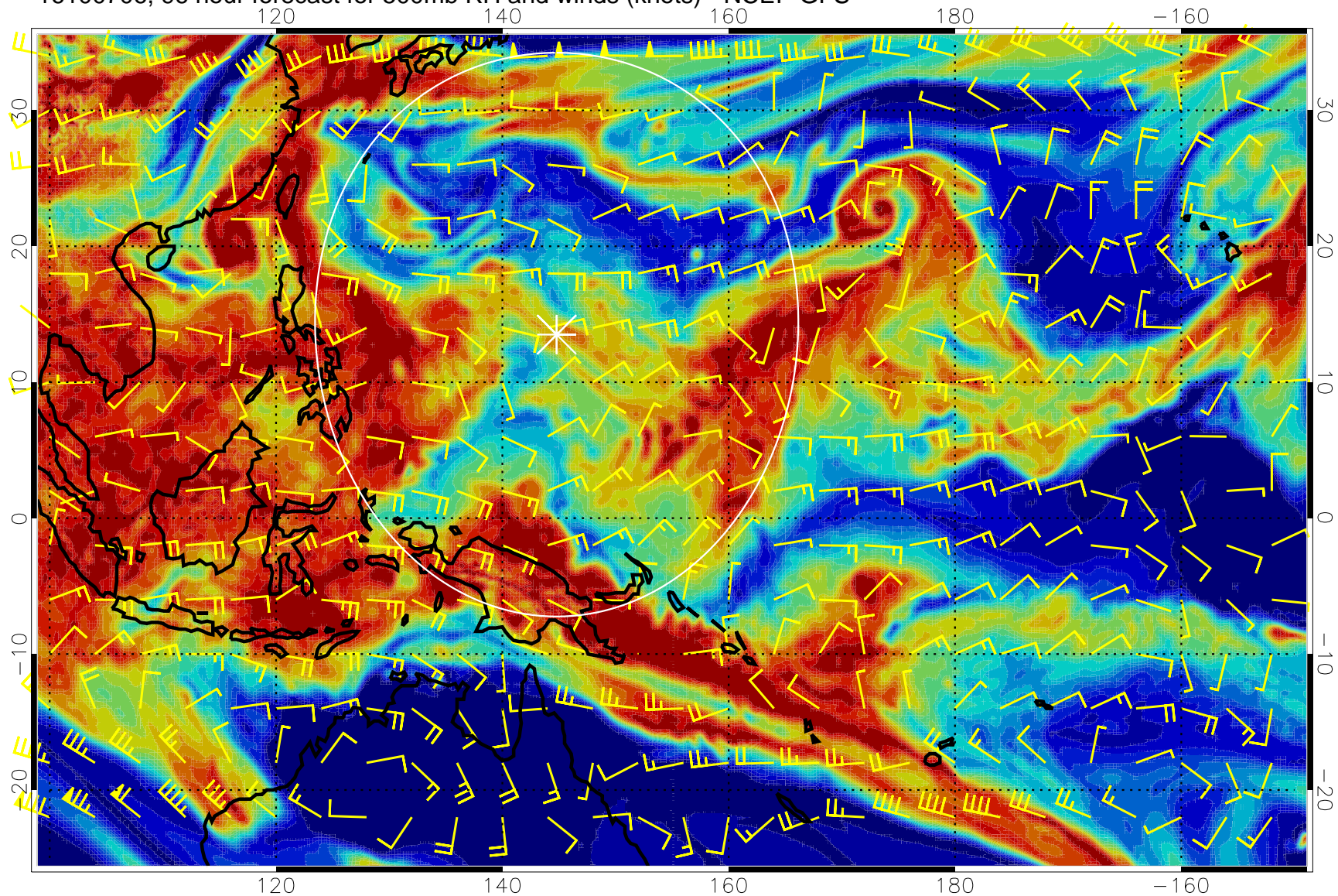
16100706, 96 hour forecast for 500mb RH and winds (knots) - NCEP GFS
