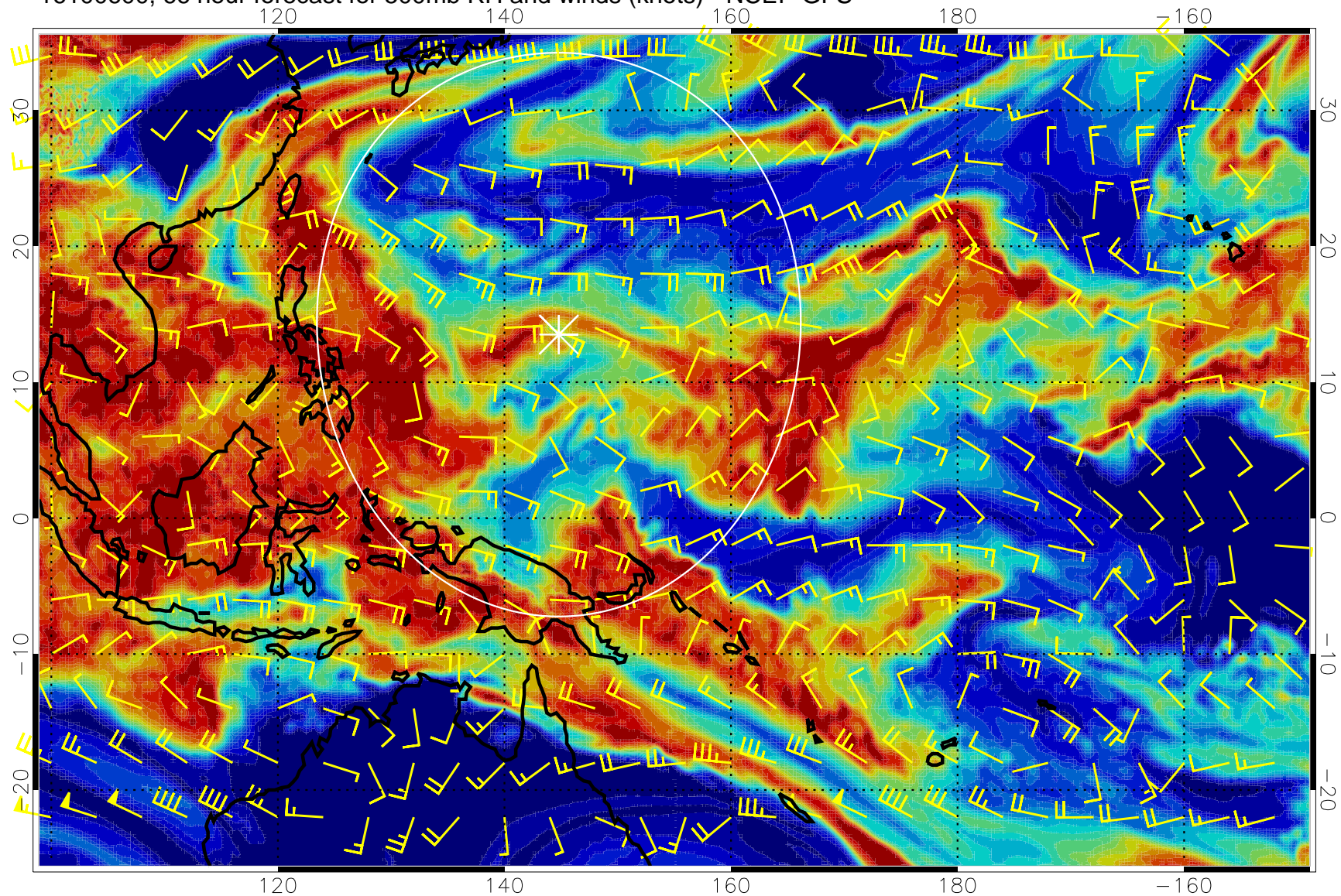
16100600, 66 hour forecast for 500mb RH and winds (knots) - NCEP GFS
