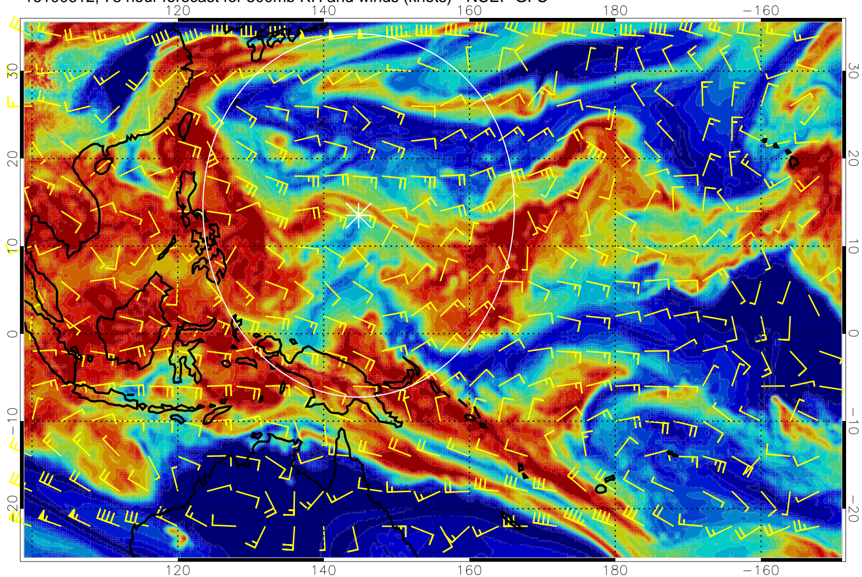
16100612, 78 hour forecast for 500mb RH and winds (knots) - NCEP GFS
