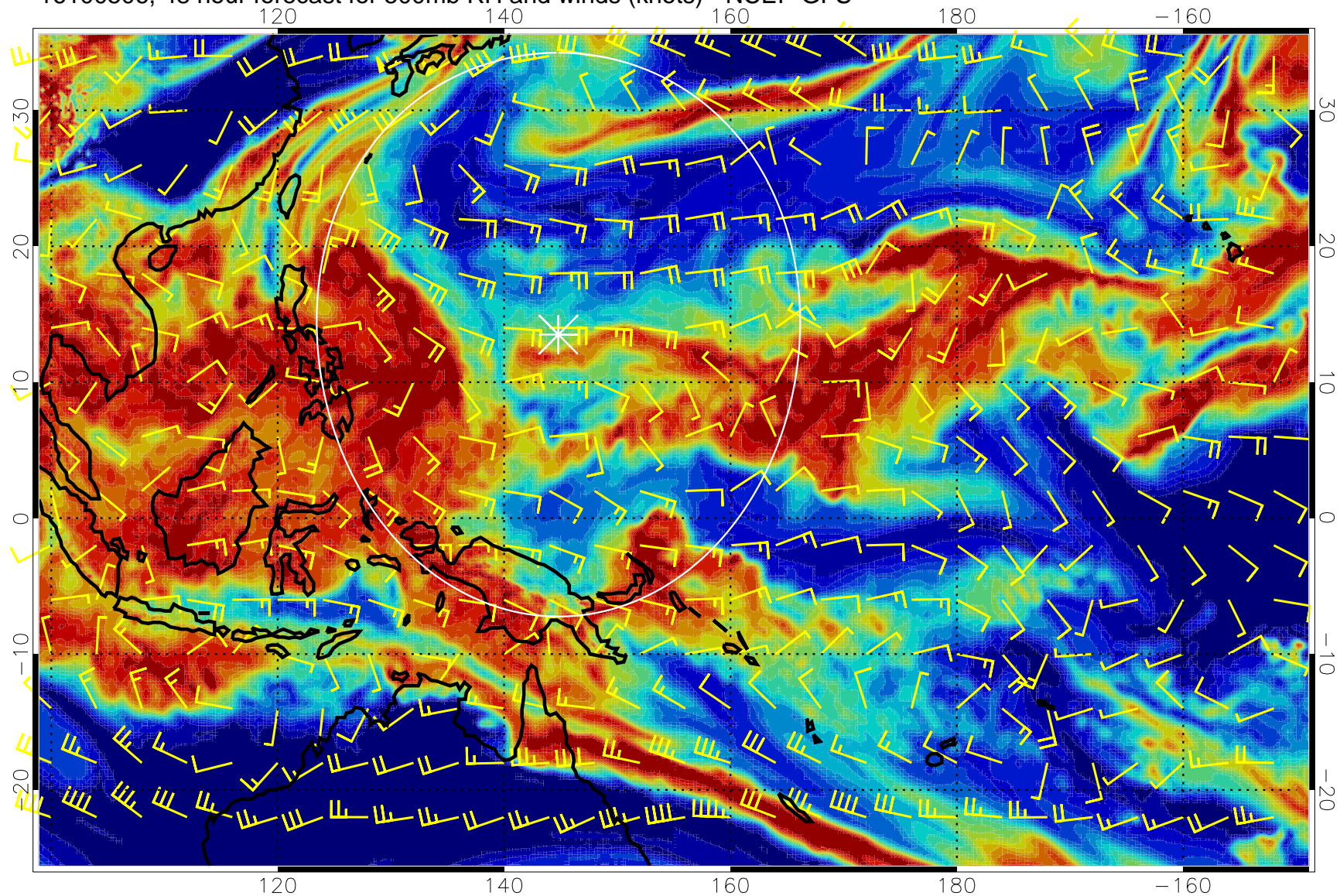
16100506, 48 hour forecast for 500mb RH and winds (knots) - NCEP GFS
