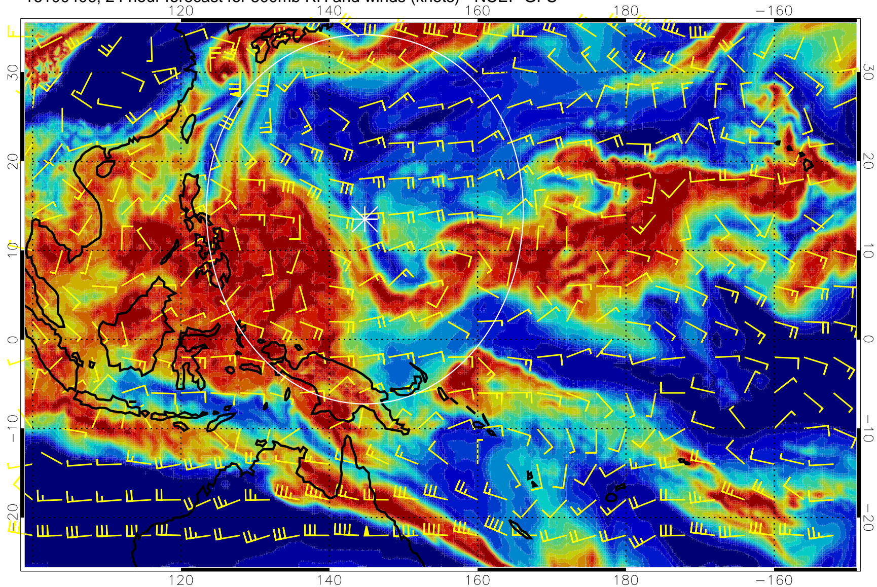
16100406, 24 hour forecast for 500mb RH and winds (knots) - NCEP GFS
