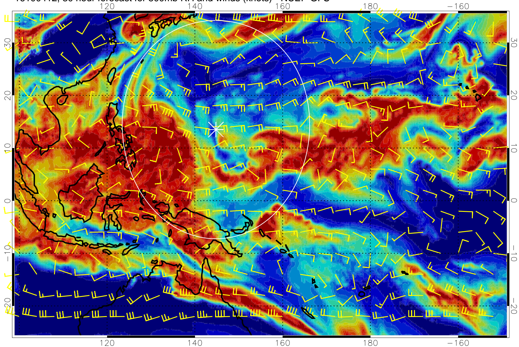
16100412, 30 hour forecast for 500mb RH and winds (knots) - NCEP GFS
