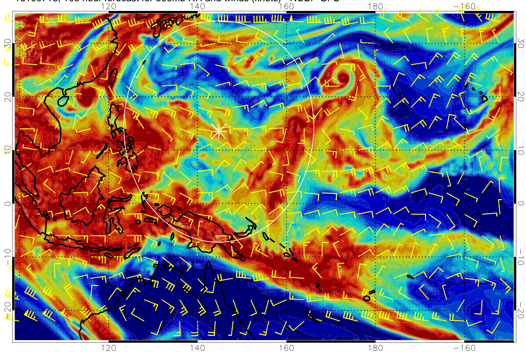
16100718, 108 hour forecast for 500mb RH and winds (knots) - NCEP GFS
