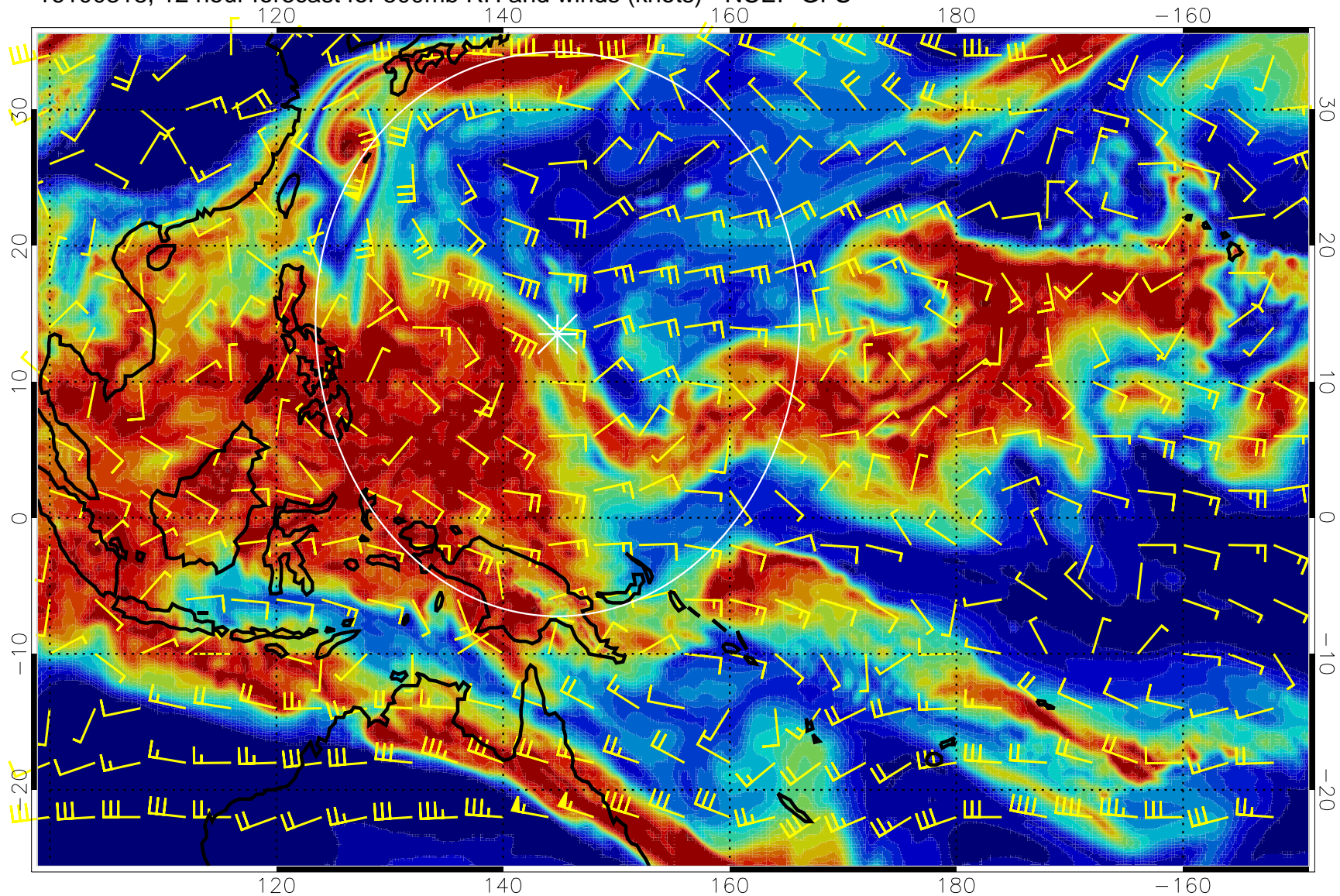
16100318, 12 hour forecast for 500mb RH and winds (knots) - NCEP GFS
