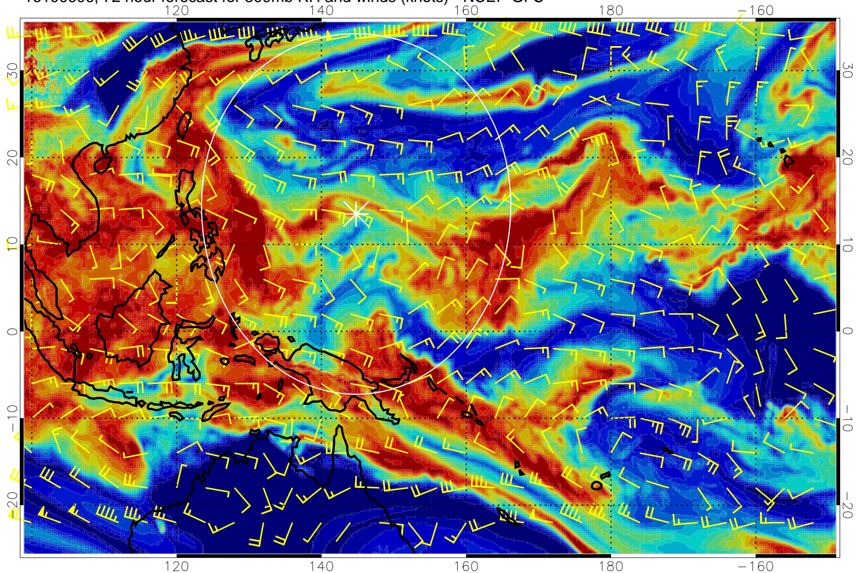
16100606, 72 hour forecast for 500mb RH and winds (knots) - NCEP GFS
