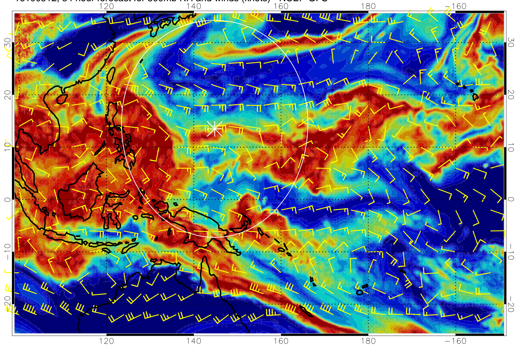
16100512, 54 hour forecast for 500mb RH and winds (knots) - NCEP GFS
