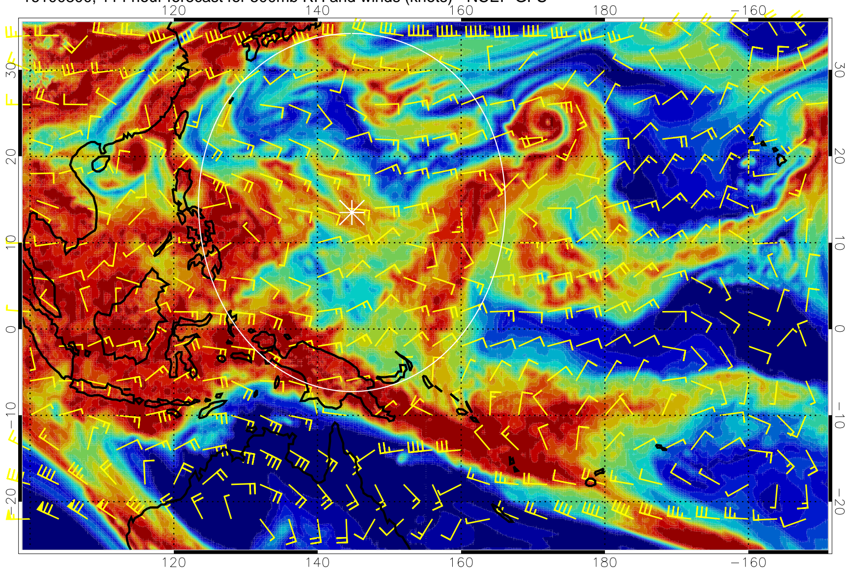
16100800, 114 hour forecast for 500mb RH and winds (knots) - NCEP GFS
