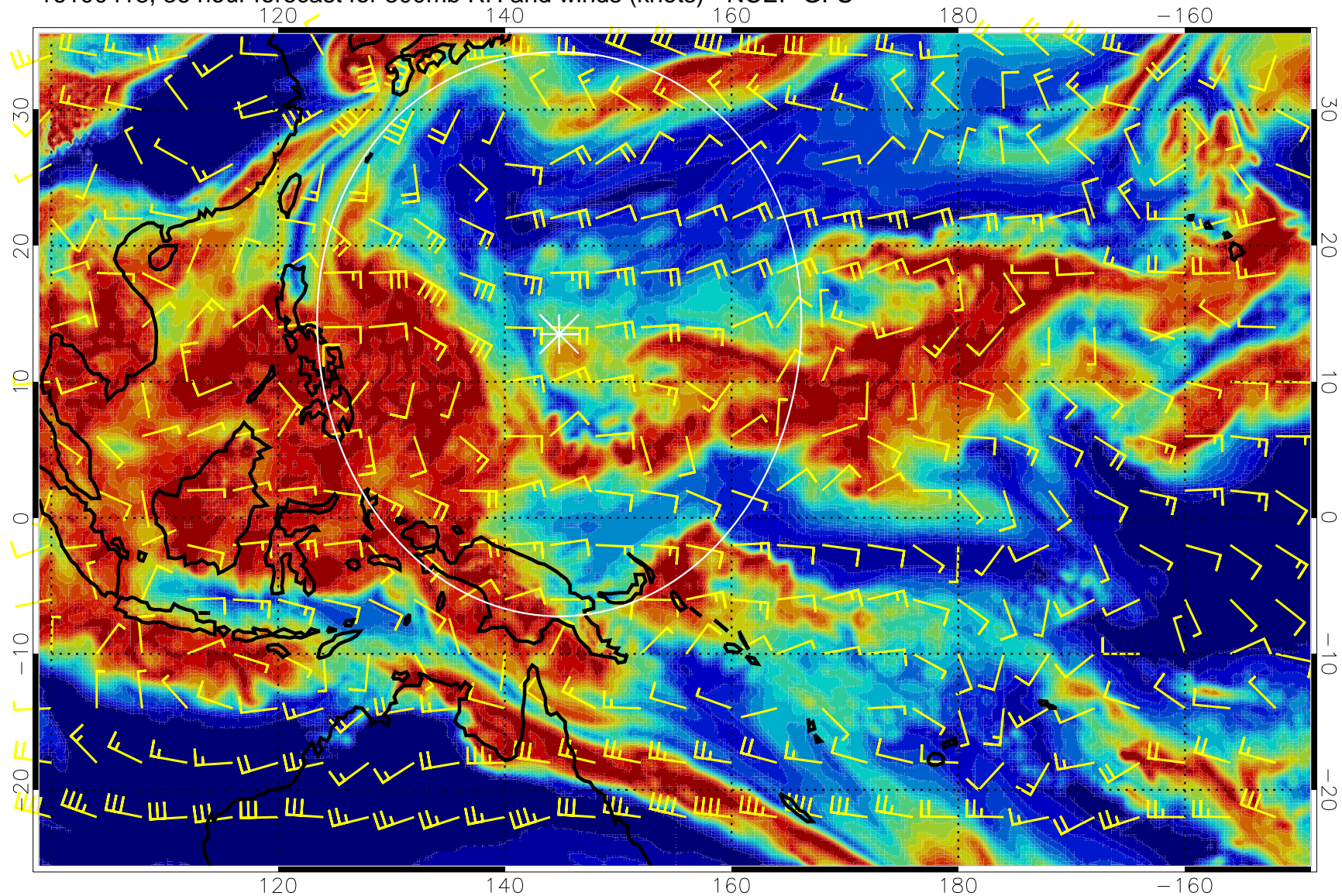
16100418, 36 hour forecast for 500mb RH and winds (knots) - NCEP GFS
