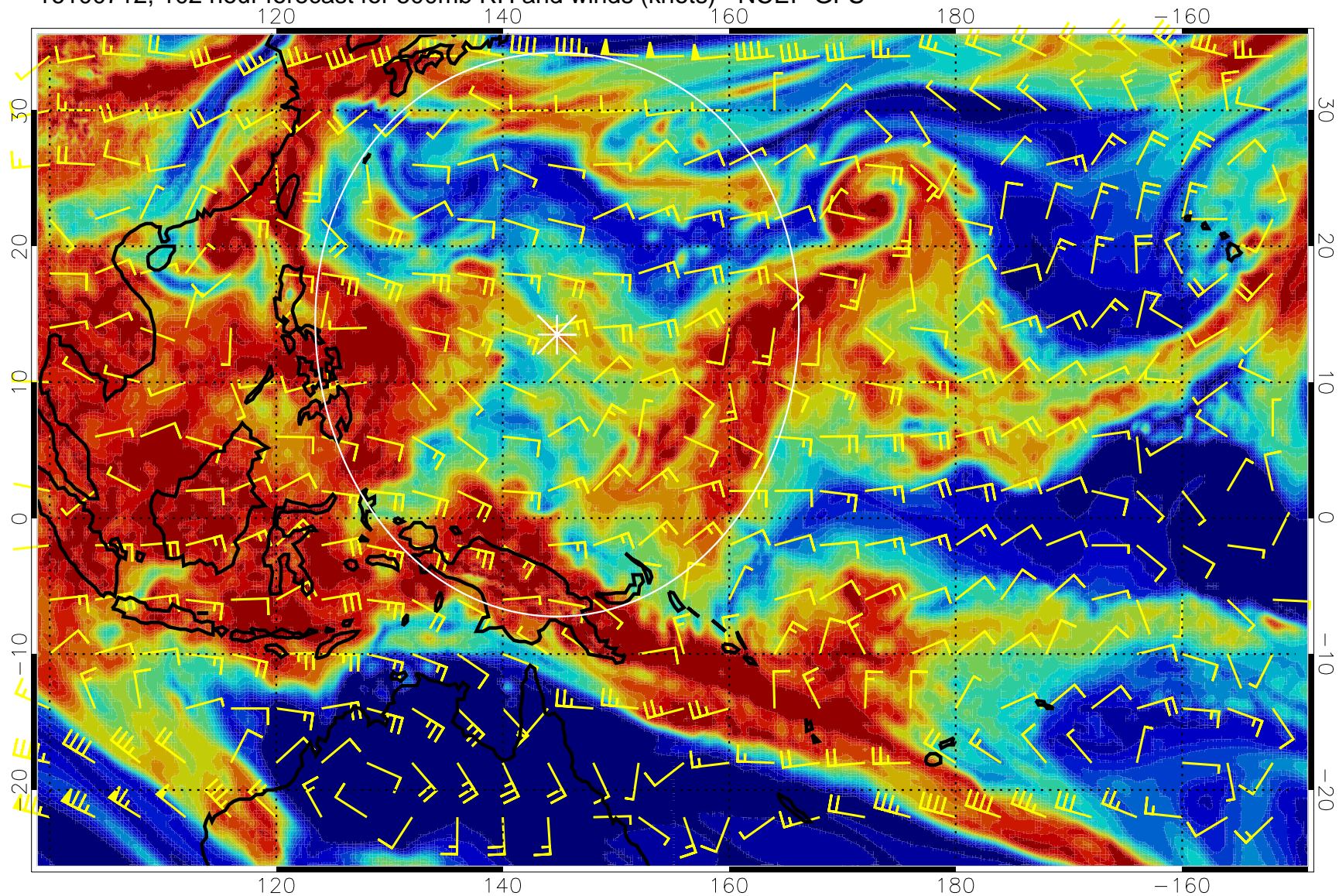
16100712, 102 hour forecast for 500mb RH and winds (knots) - NCEP GFS
