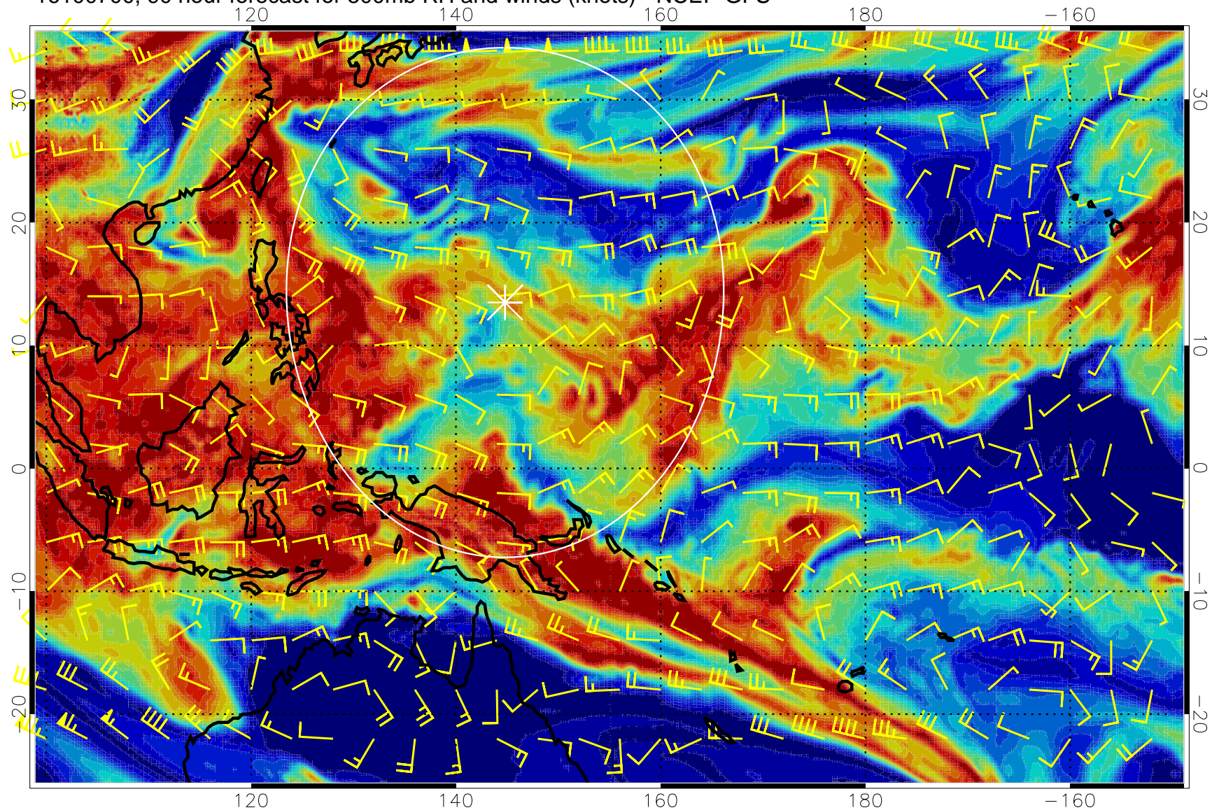
16100700, 90 hour forecast for 500mb RH and winds (knots) - NCEP GFS
