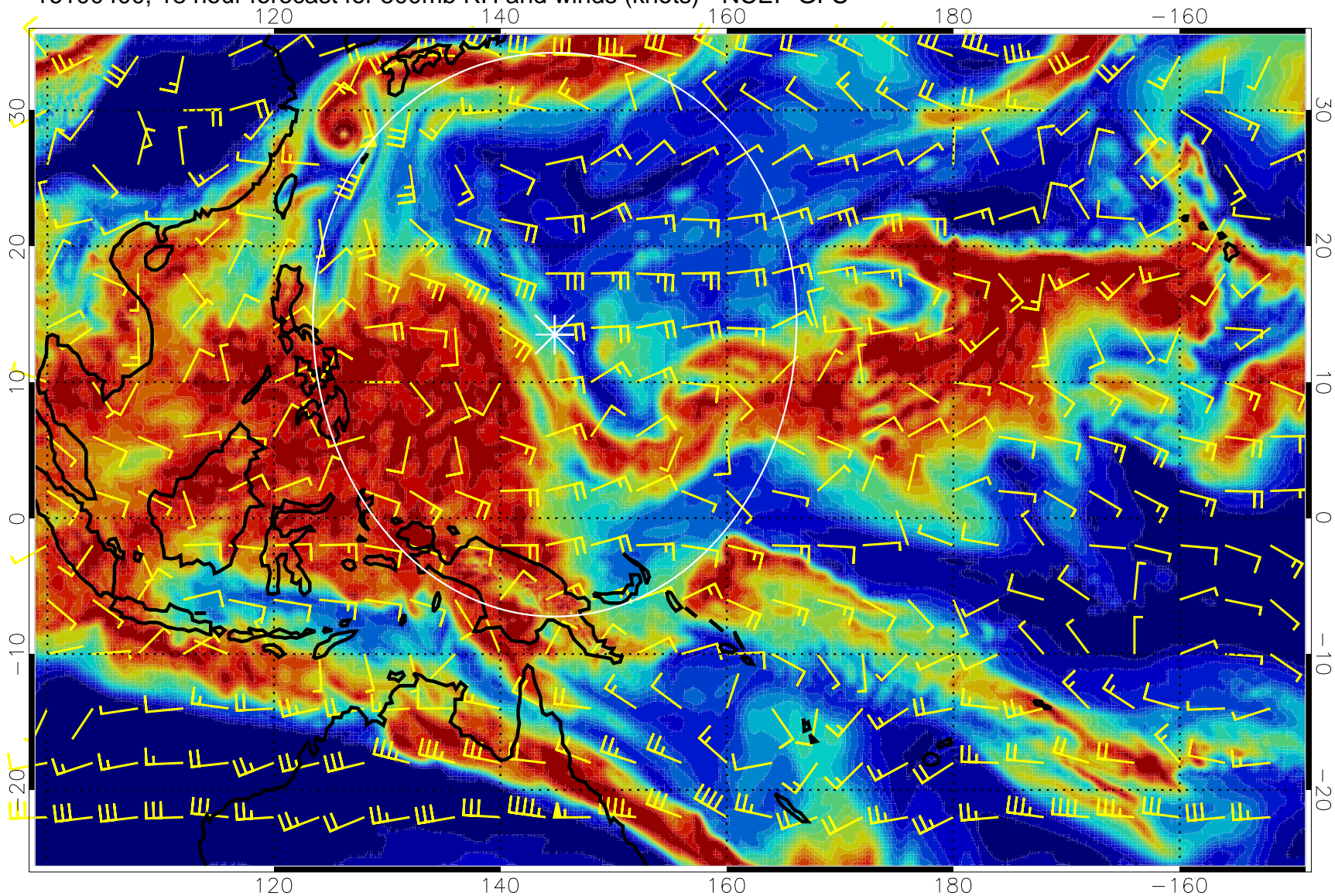
16100400, 18 hour forecast for 500mb RH and winds (knots) - NCEP GFS
