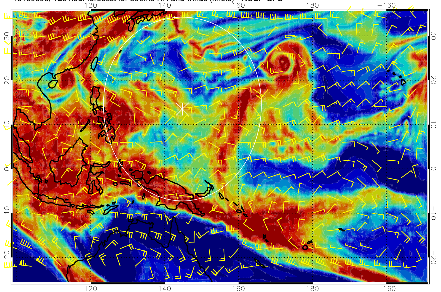
16100806, 120 hour forecast for 500mb RH and winds (knots) - NCEP GFS
