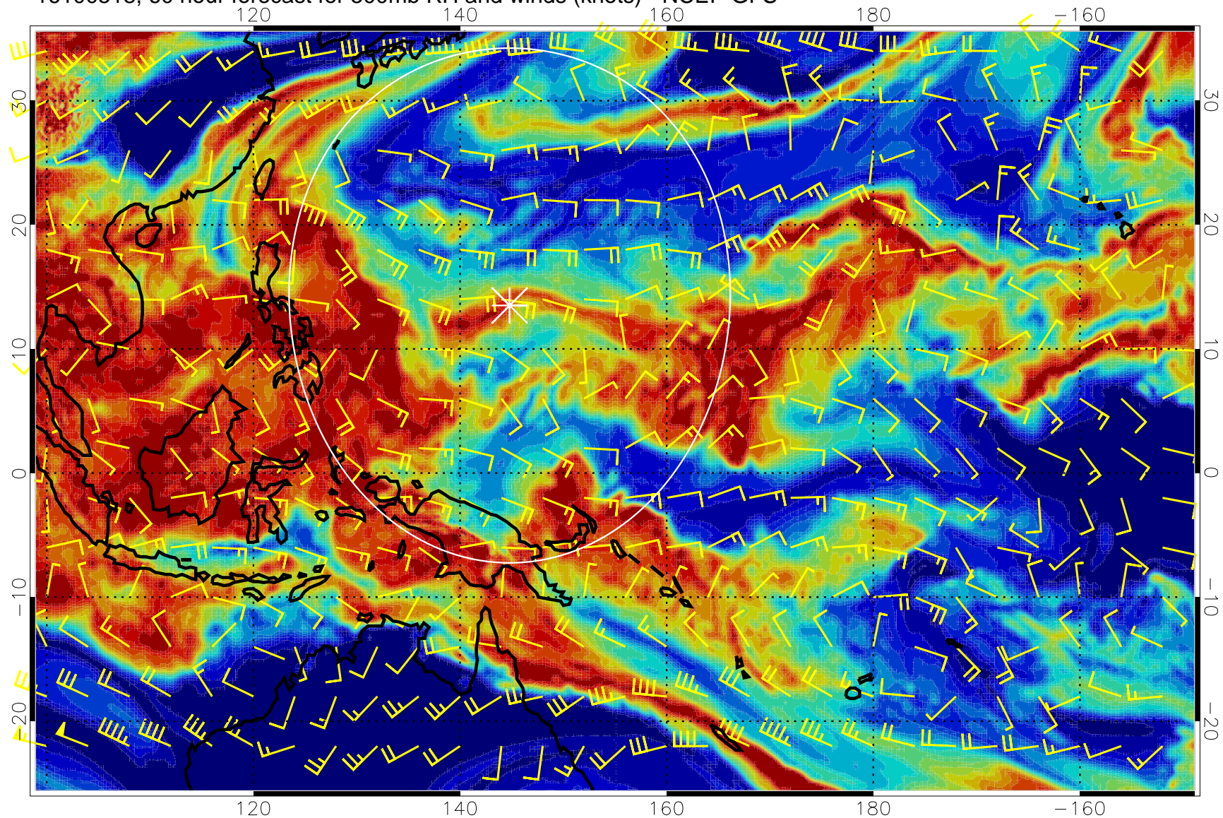
16100518, 60 hour forecast for 500mb RH and winds (knots) - NCEP GFS
