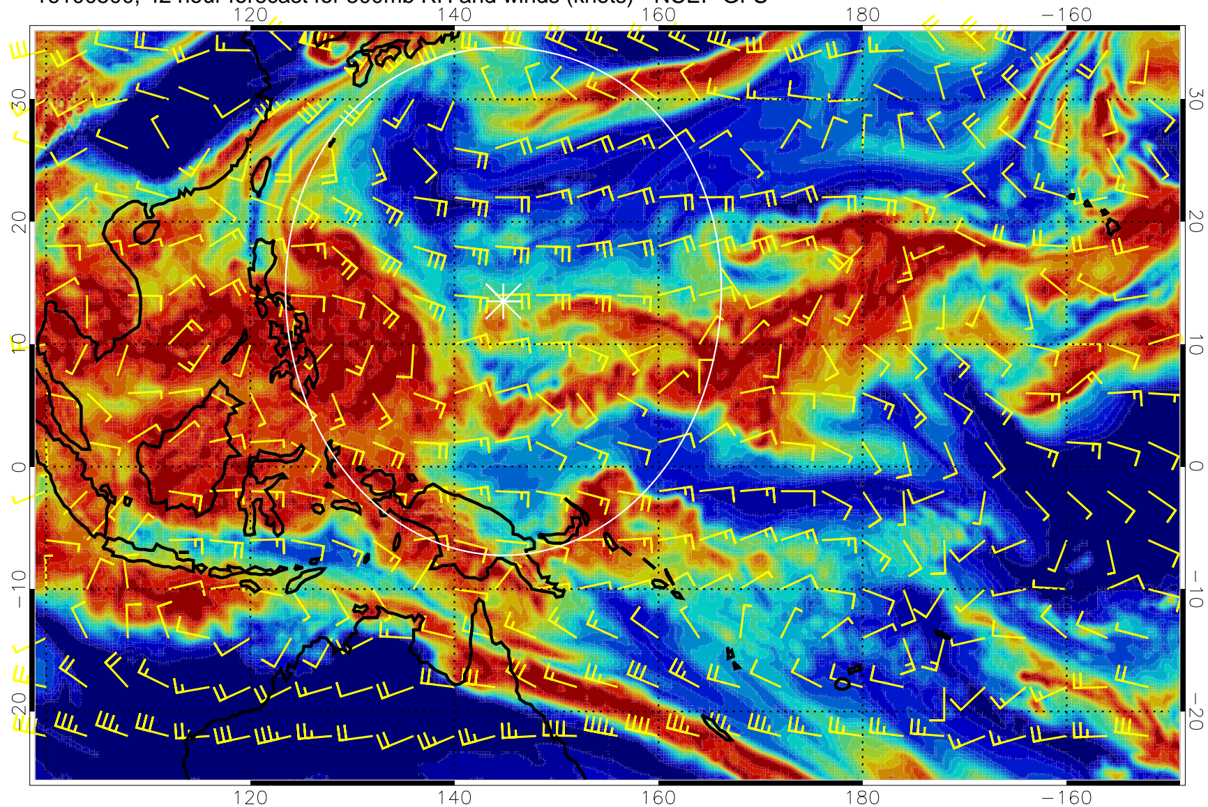
16100500, 42 hour forecast for 500mb RH and winds (knots) - NCEP GFS
