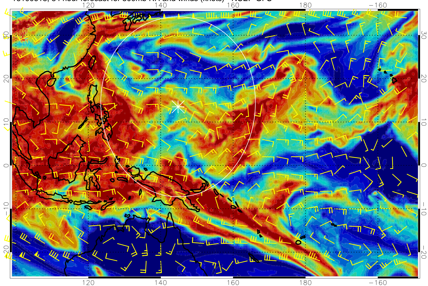
16100618, 84 hour forecast for 500mb RH and winds (knots) - NCEP GFS
