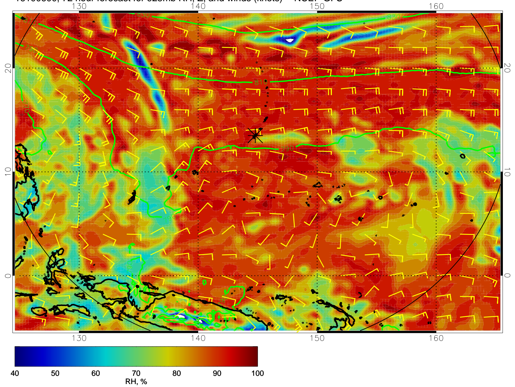
16100600, 72 hour forecast for 925mb RH, Z, and winds (knots) -- NCEP GFS
