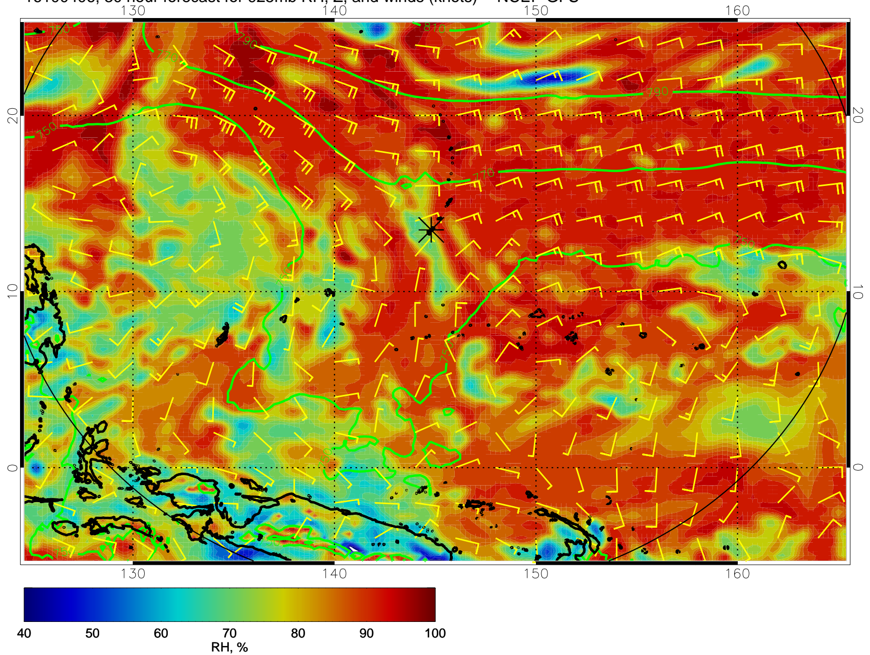
16100406, 30 hour forecast for 925mb RH, Z, and winds (knots) -- NCEP GFS
