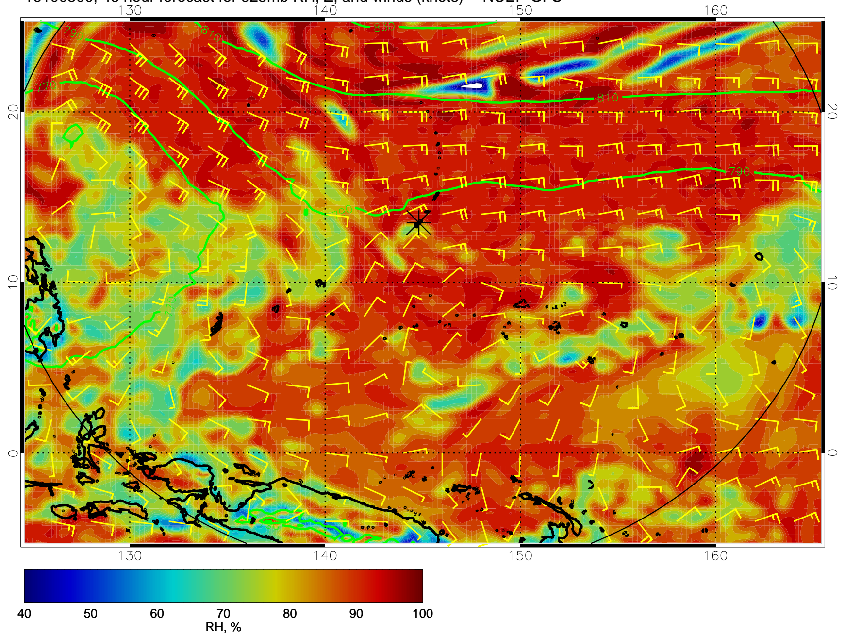
16100500, 48 hour forecast for 925mb RH, Z, and winds (knots) -- NCEP GFS
