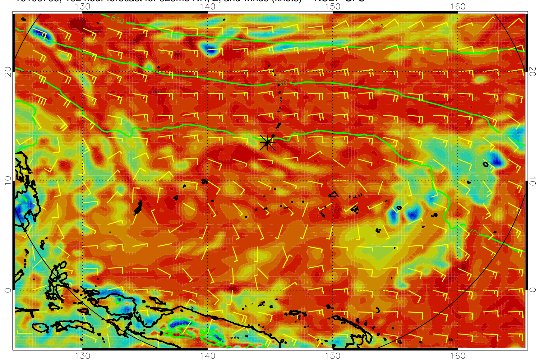
16100706, 102 hour forecast for 925mb RH, Z, and winds (knots) -- NCEP GFS
