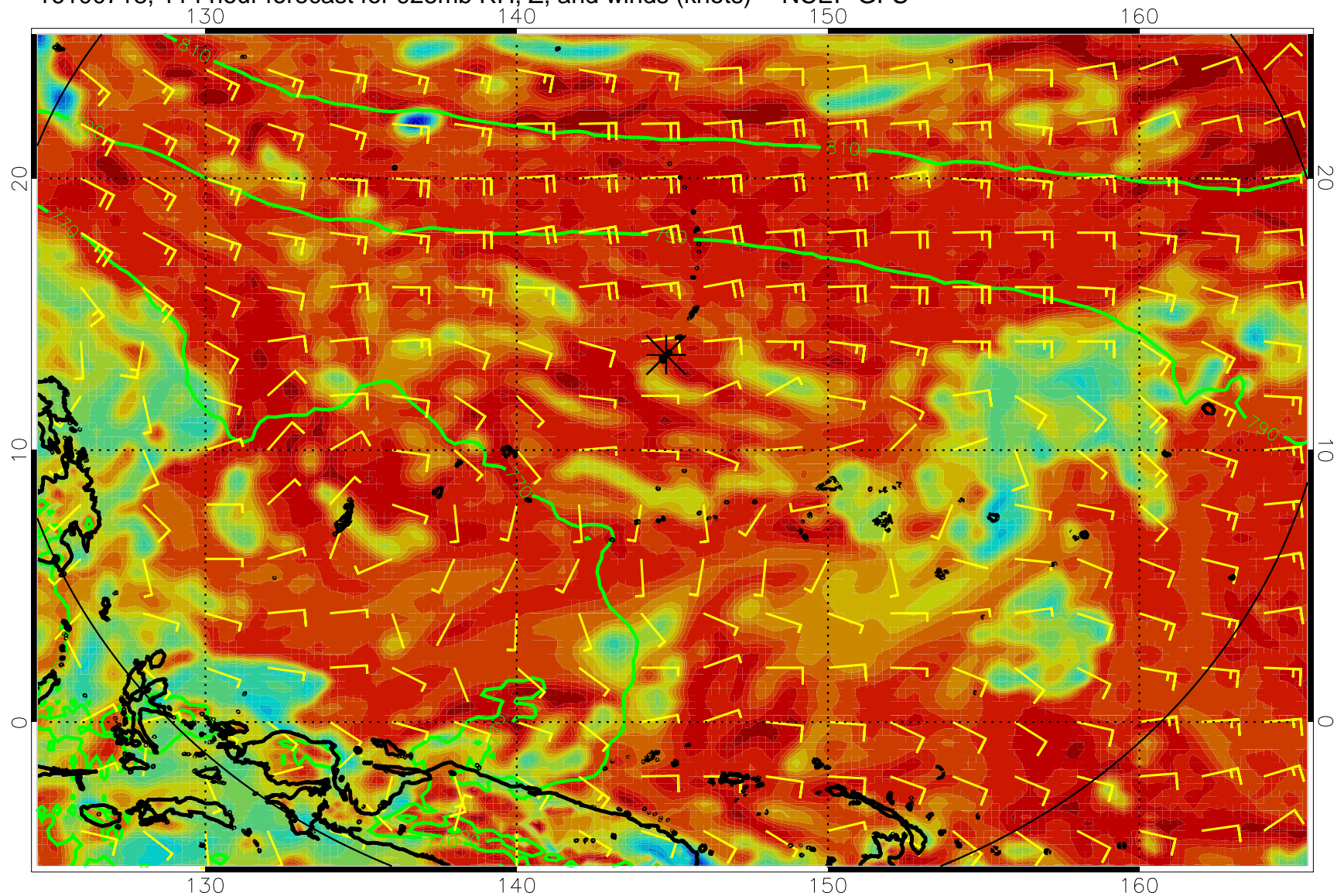
16100718, 114 hour forecast for 925mb RH, Z, and winds (knots) -- NCEP GFS
