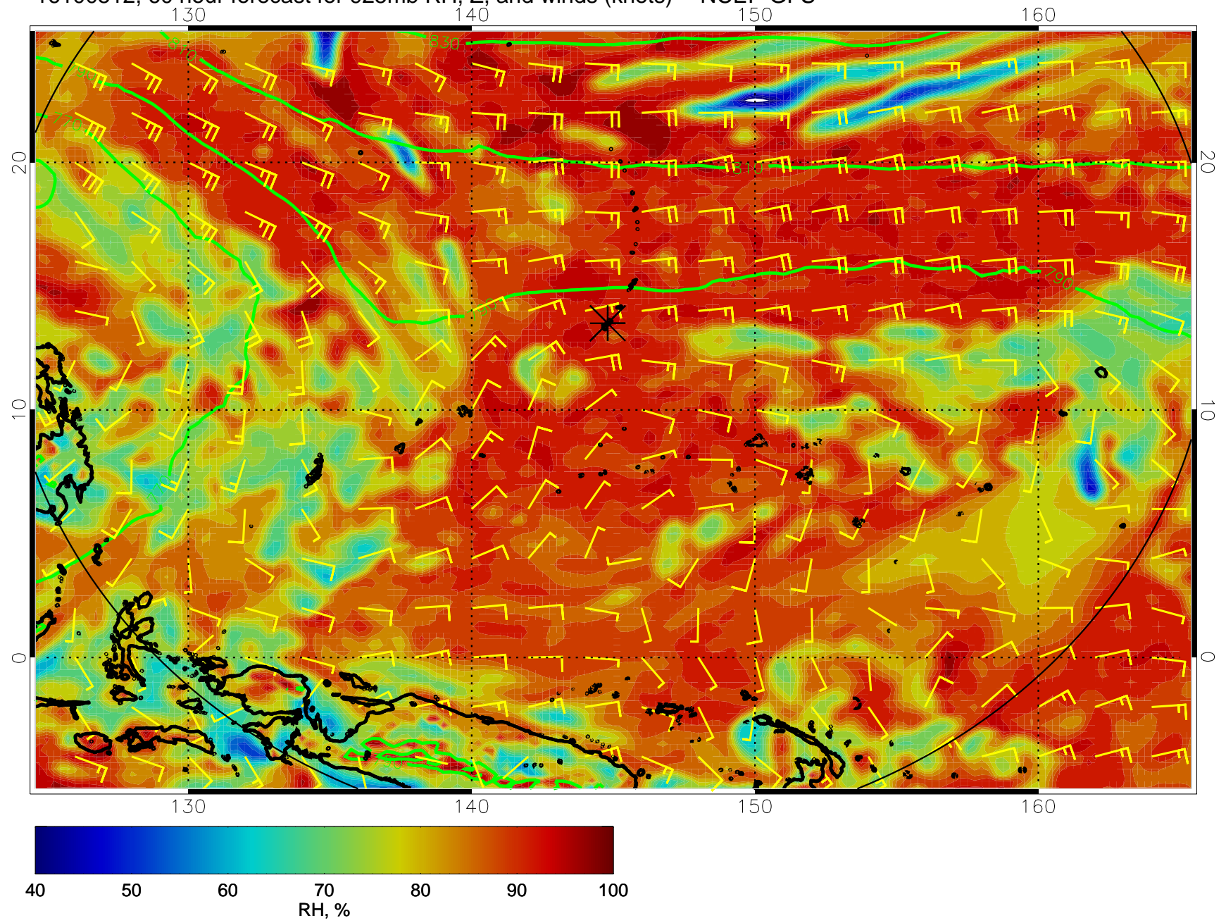
16100512, 60 hour forecast for 925mb RH, Z, and winds (knots) -- NCEP GFS
