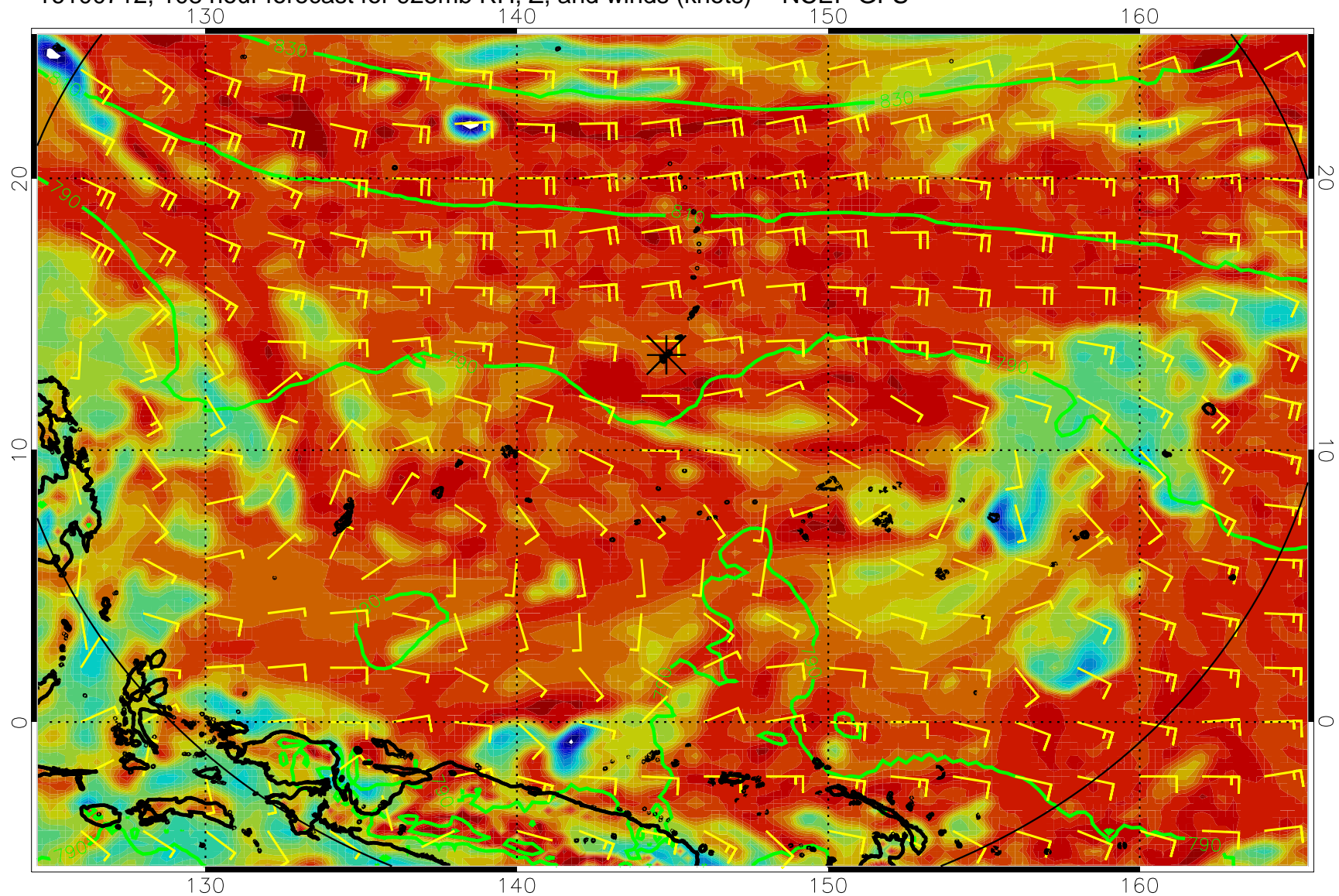
16100712, 108 hour forecast for 925mb RH, Z, and winds (knots) -- NCEP GFS
