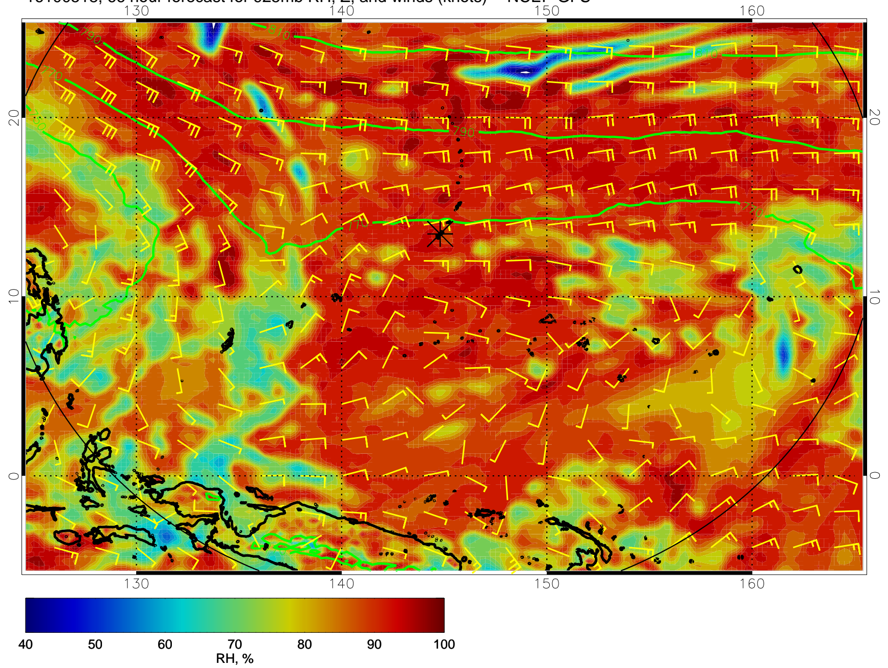
16100518, 66 hour forecast for 925mb RH, Z, and winds (knots) -- NCEP GFS
