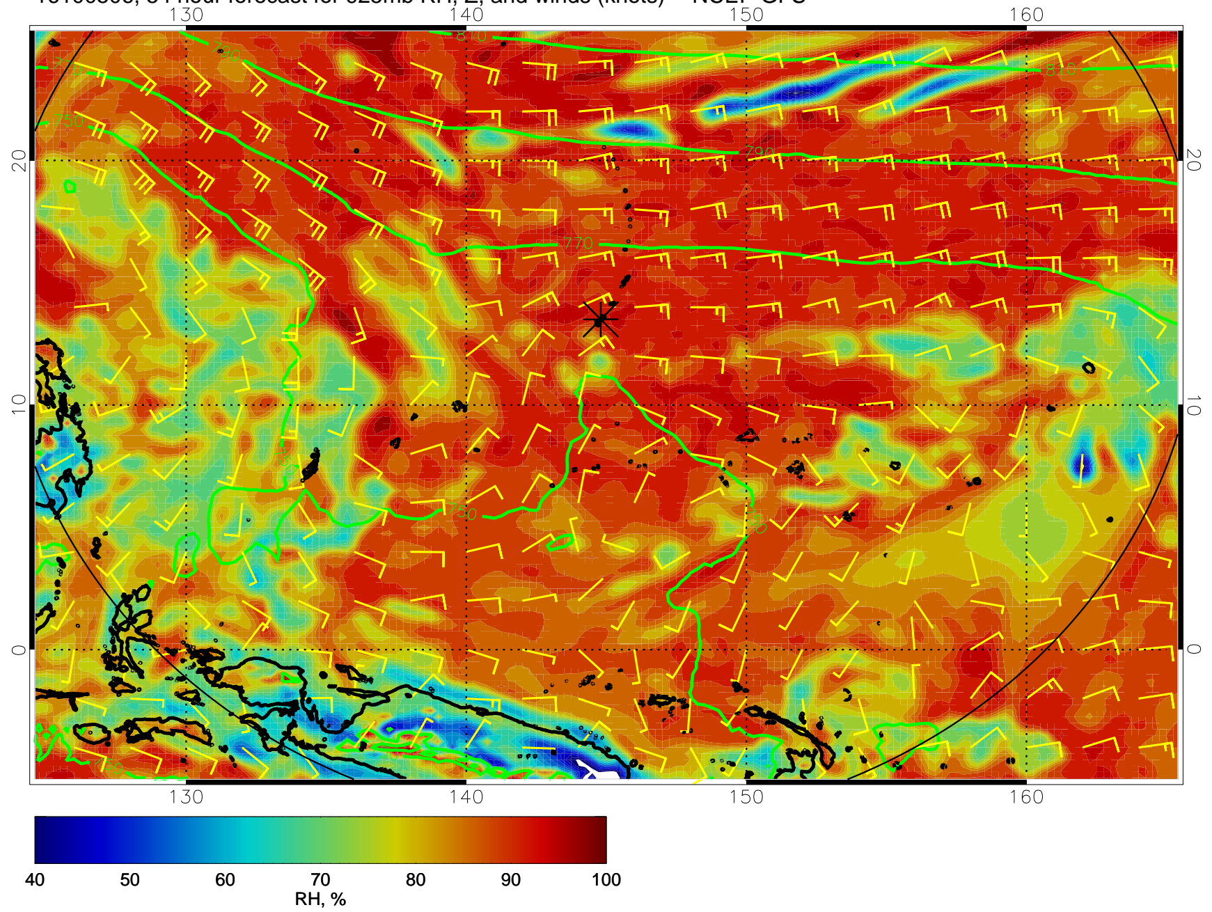
16100506, 54 hour forecast for 925mb RH, Z, and winds (knots) -- NCEP GFS
