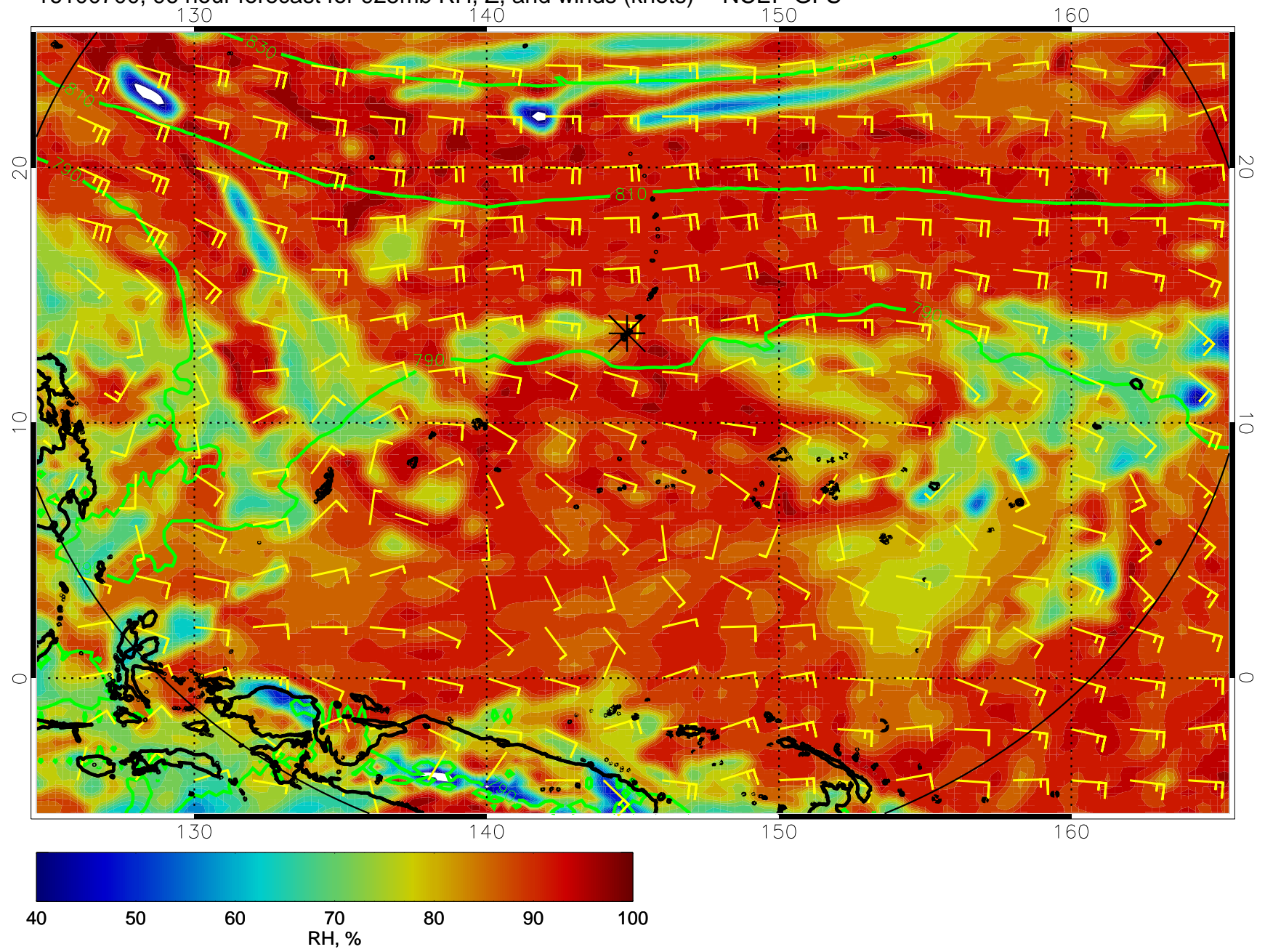
16100700, 96 hour forecast for 925mb RH, Z, and winds (knots) -- NCEP GFS
