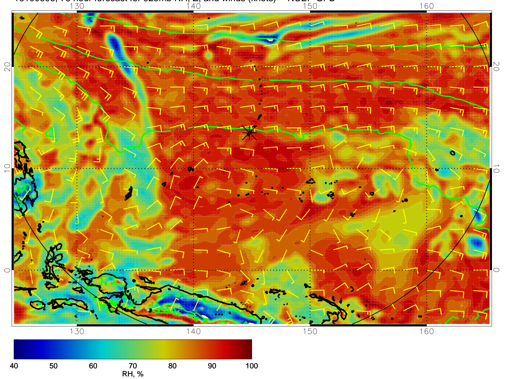
16100606, 78 hour forecast for 925mb RH, Z, and winds (knots) -- NCEP GFS
