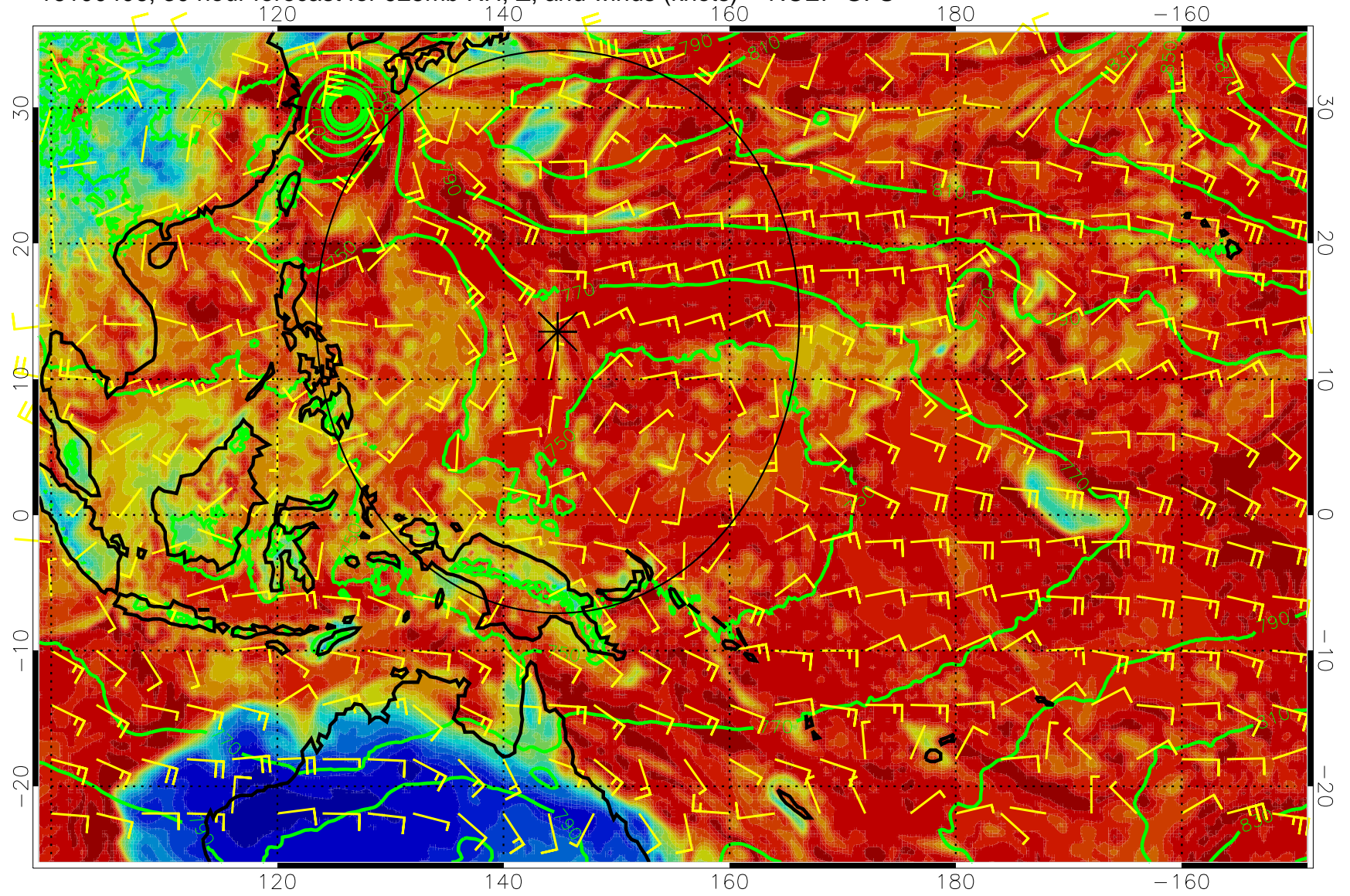
16100406, 30 hour forecast for 925mb RH, Z, and winds (knots) -- NCEP GFS
