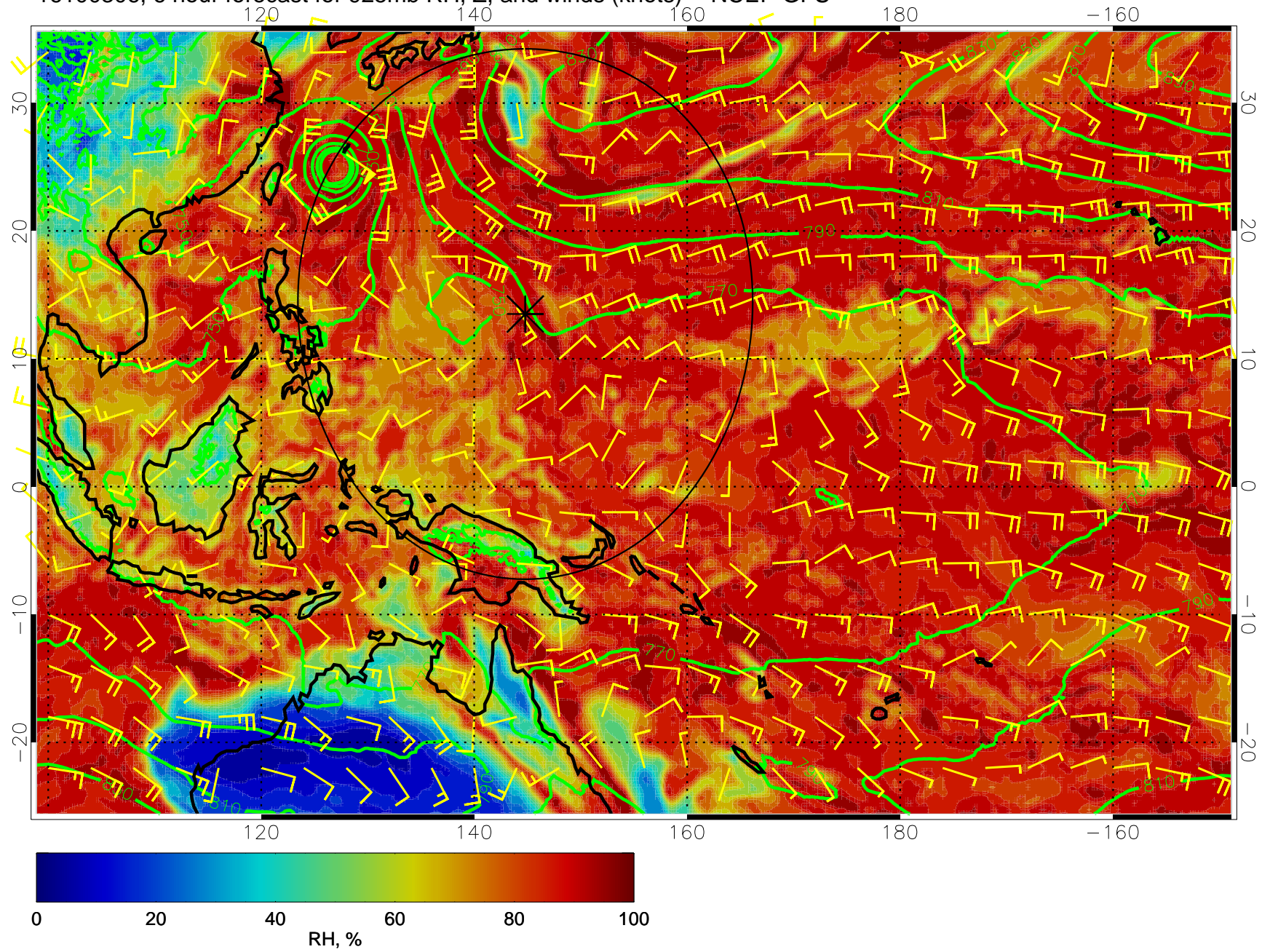
16100306, 6 hour forecast for 925mb RH, Z, and winds (knots) -- NCEP GFS
