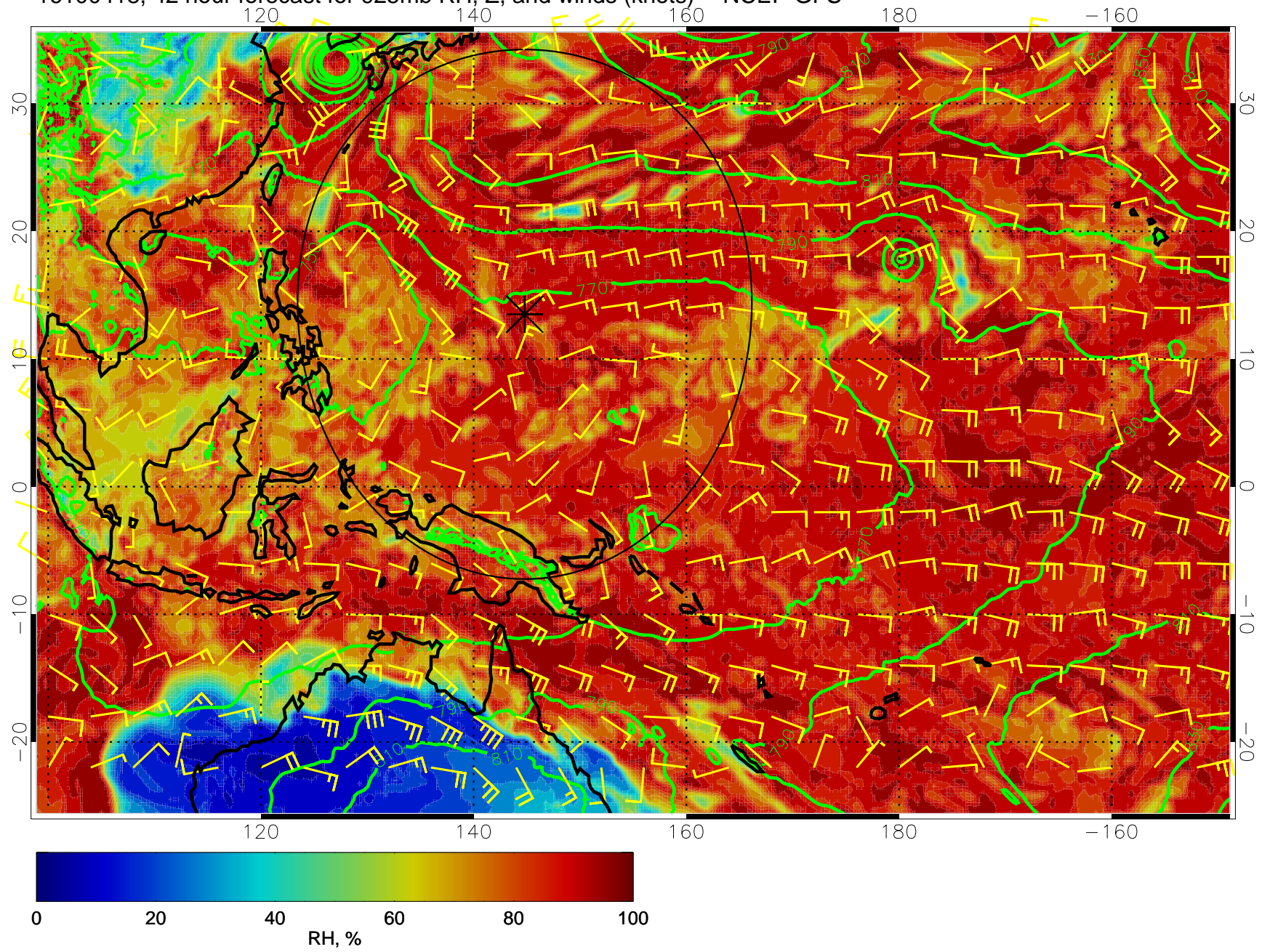
16100418, 42 hour forecast for 925mb RH, Z, and winds (knots) -- NCEP GFS
