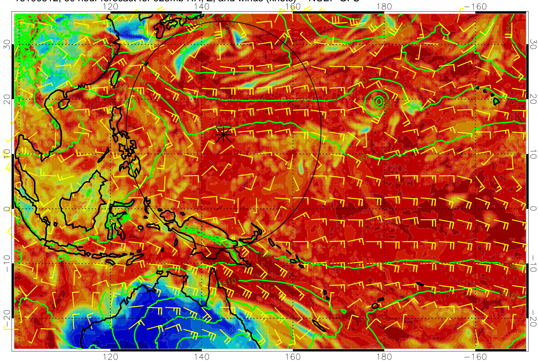
16100512, 60 hour forecast for 925mb RH, Z, and winds (knots) -- NCEP GFS
