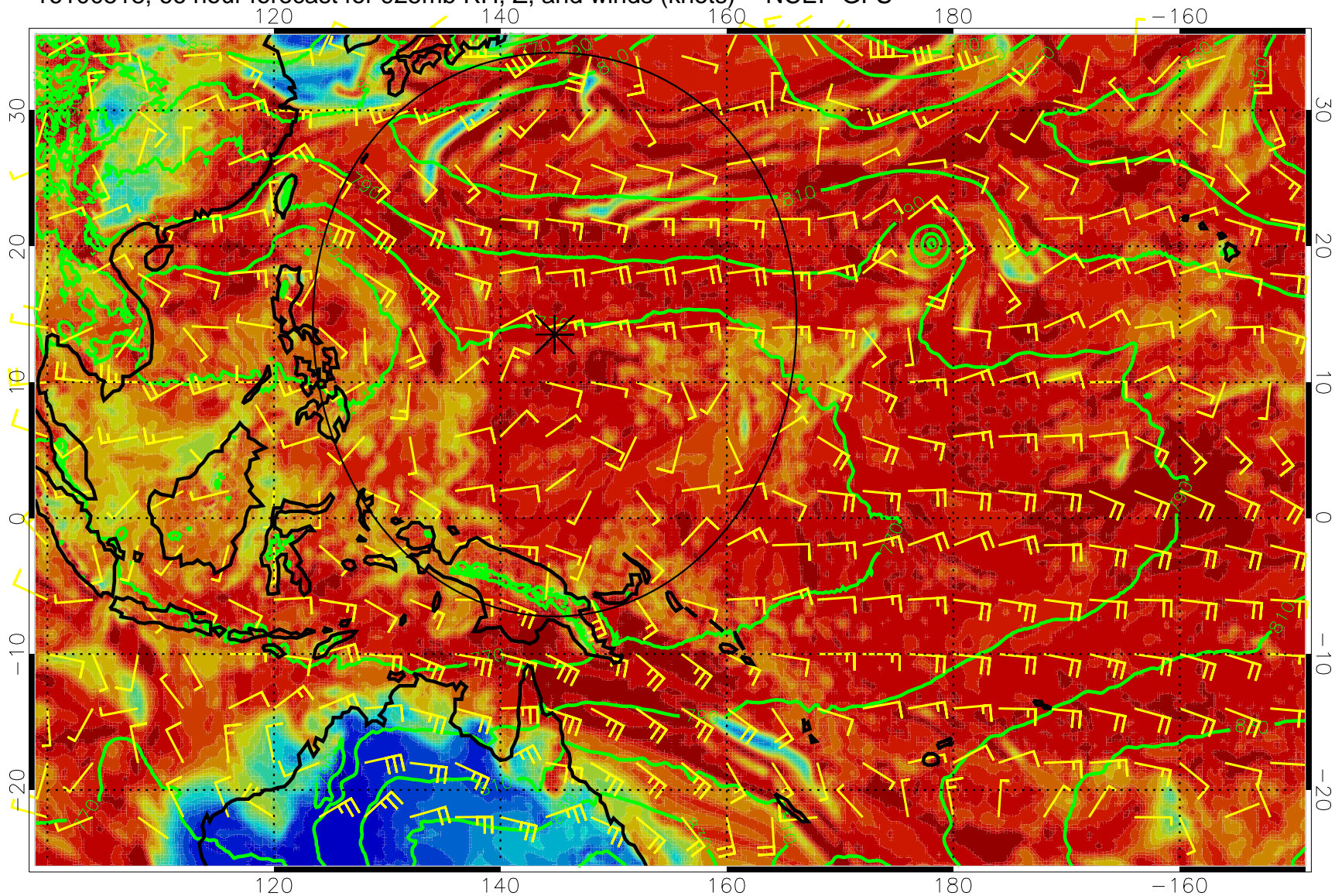
16100518, 66 hour forecast for 925mb RH, Z, and winds (knots) -- NCEP GFS
