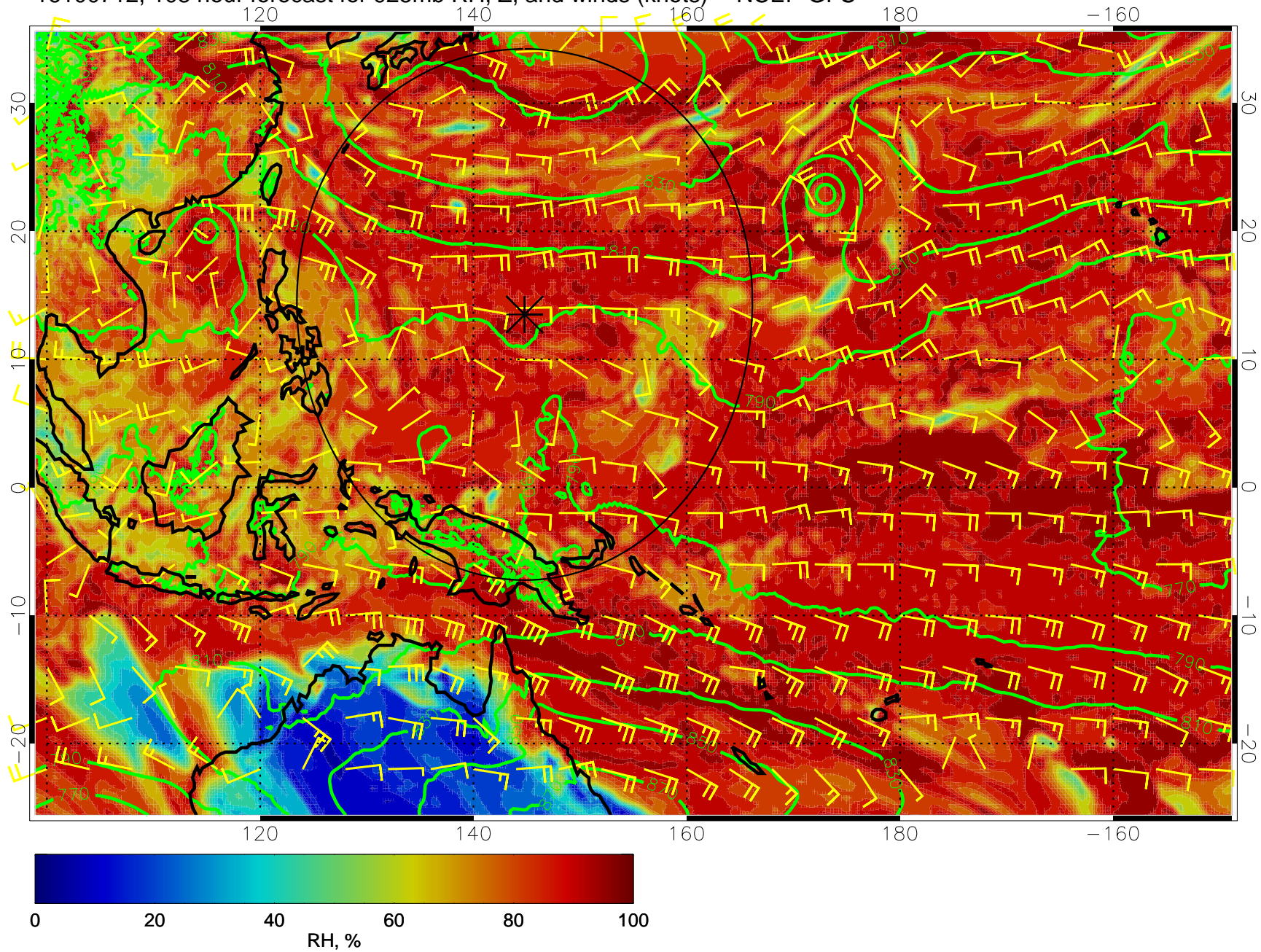
16100712, 108 hour forecast for 925mb RH, Z, and winds (knots) -- NCEP GFS
