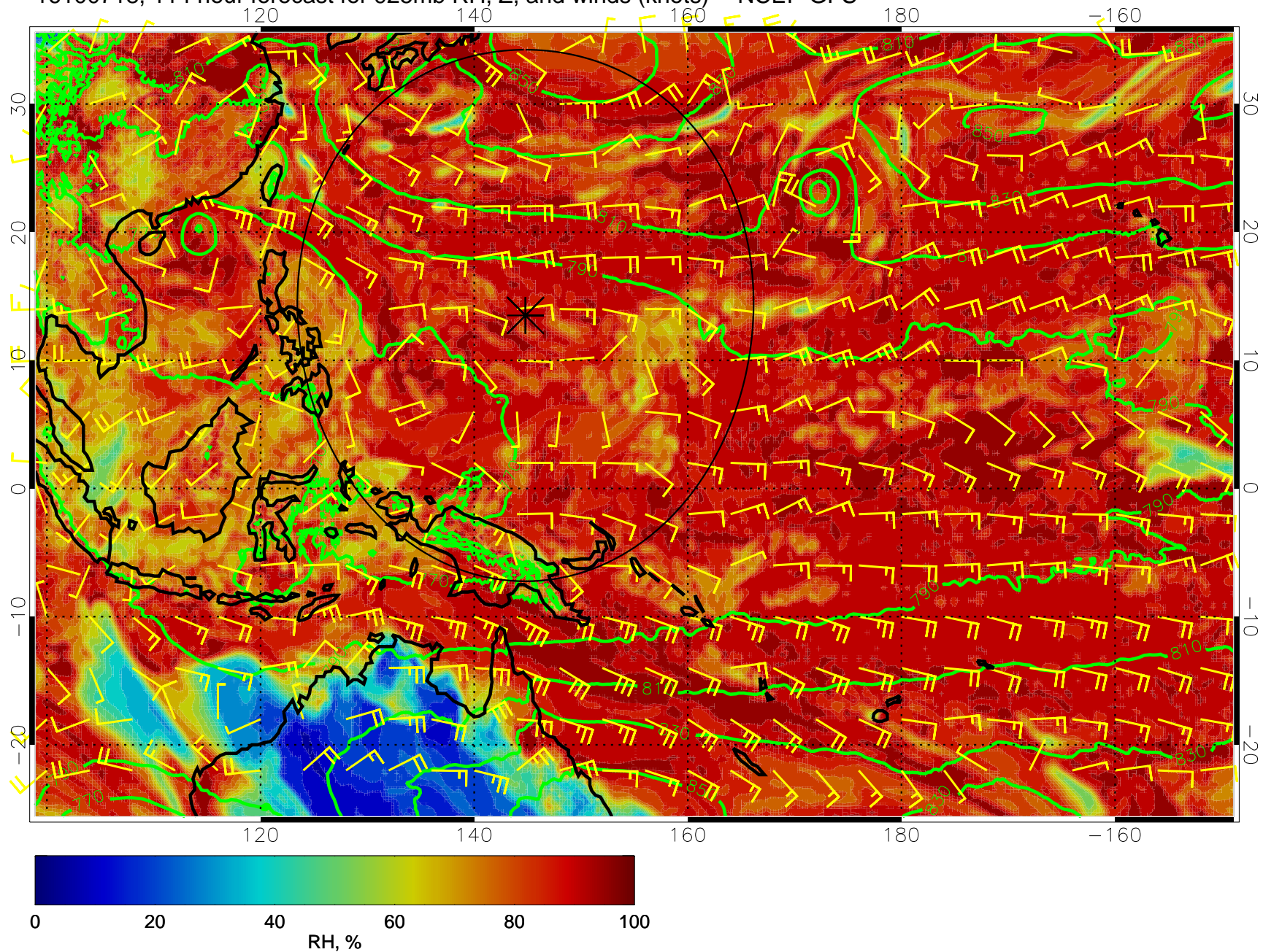
16100718, 114 hour forecast for 925mb RH, Z, and winds (knots) -- NCEP GFS
