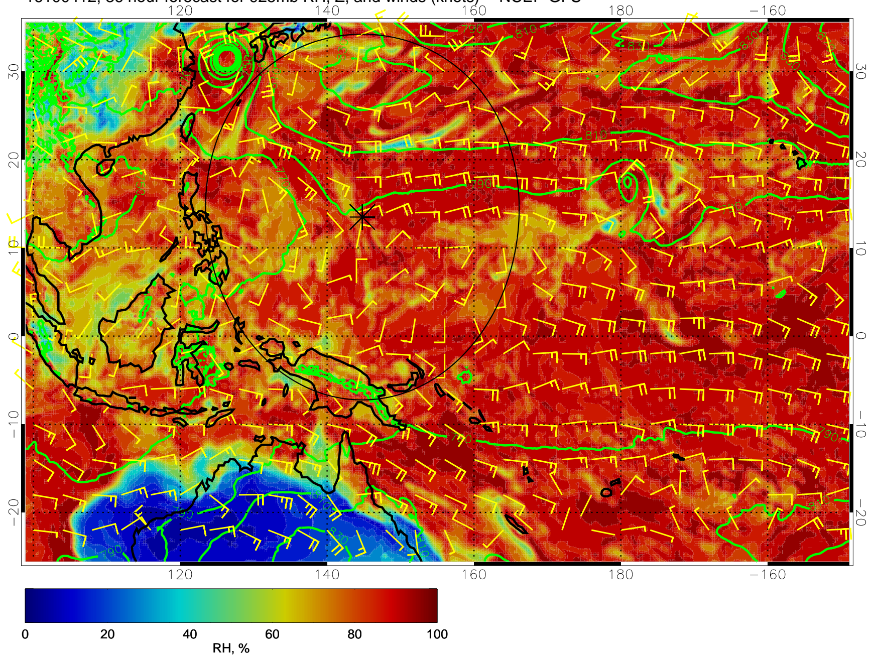
16100412, 36 hour forecast for 925mb RH, Z, and winds (knots) -- NCEP GFS
