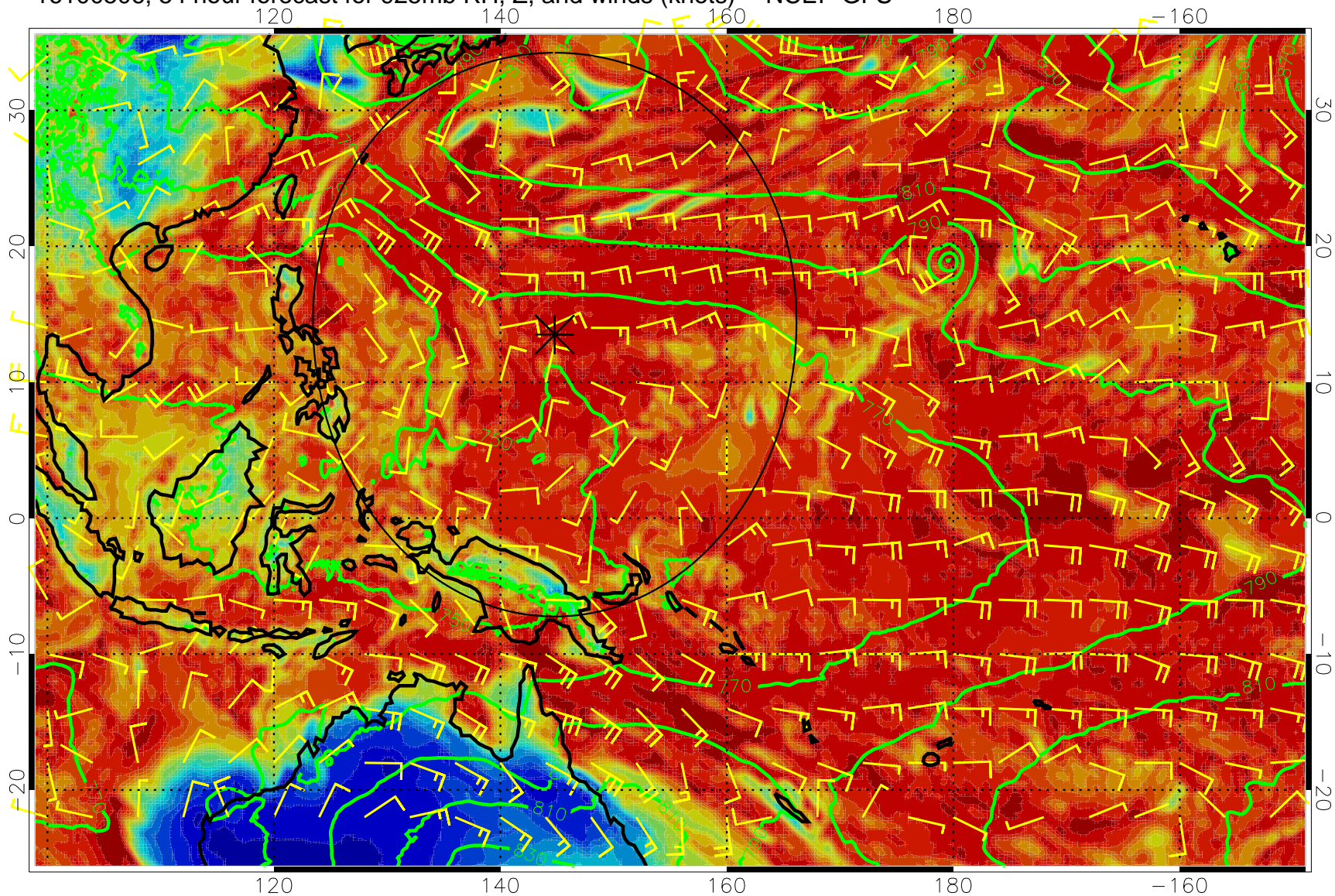
16100506, 54 hour forecast for 925mb RH, Z, and winds (knots) -- NCEP GFS
