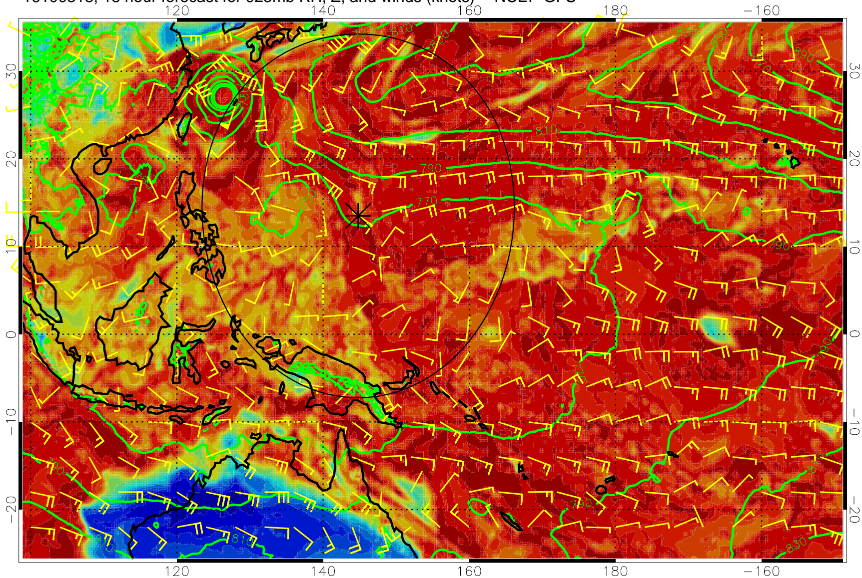
16100318, 18 hour forecast for 925mb RH, Z, and winds (knots) -- NCEP GFS
