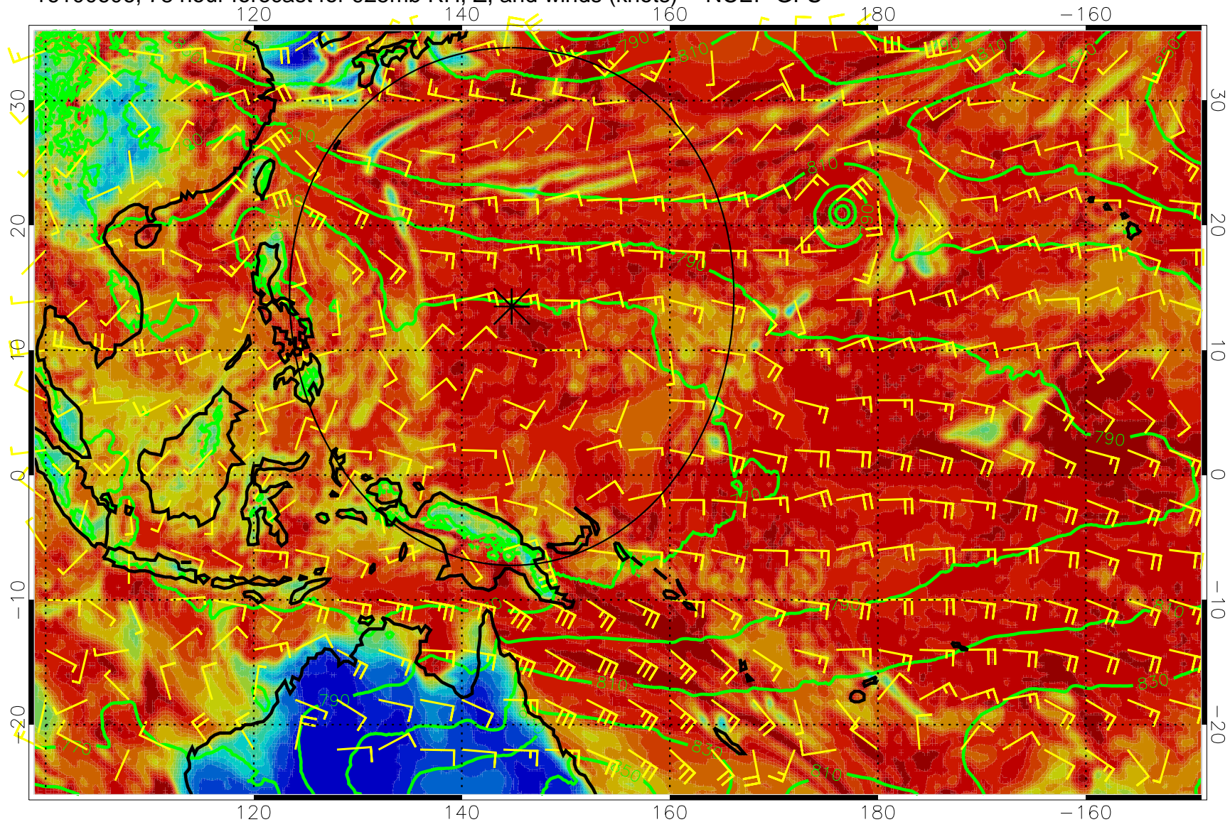
16100606, 78 hour forecast for 925mb RH, Z, and winds (knots) -- NCEP GFS
