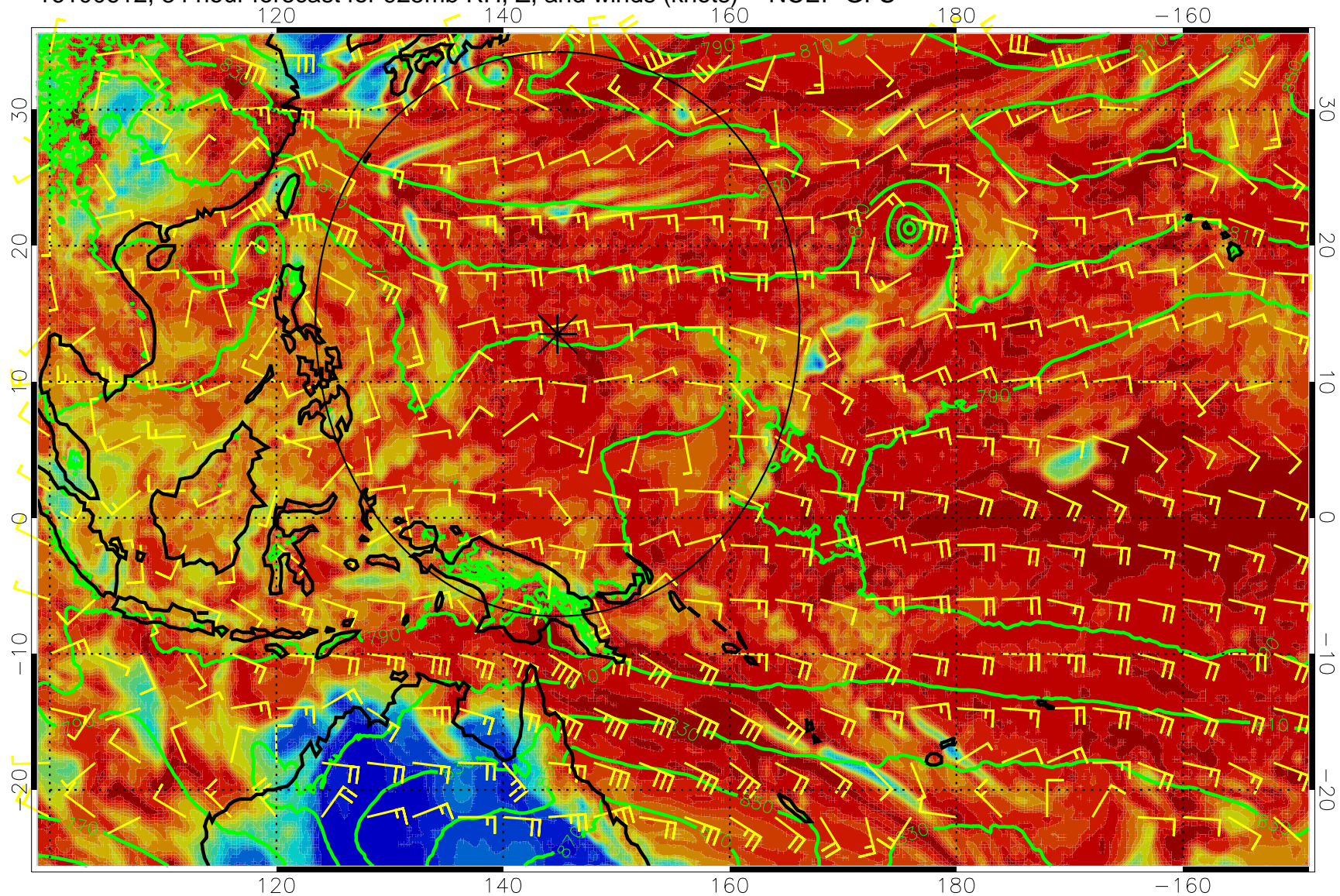
16100612, 84 hour forecast for 925mb RH, Z, and winds (knots) -- NCEP GFS
