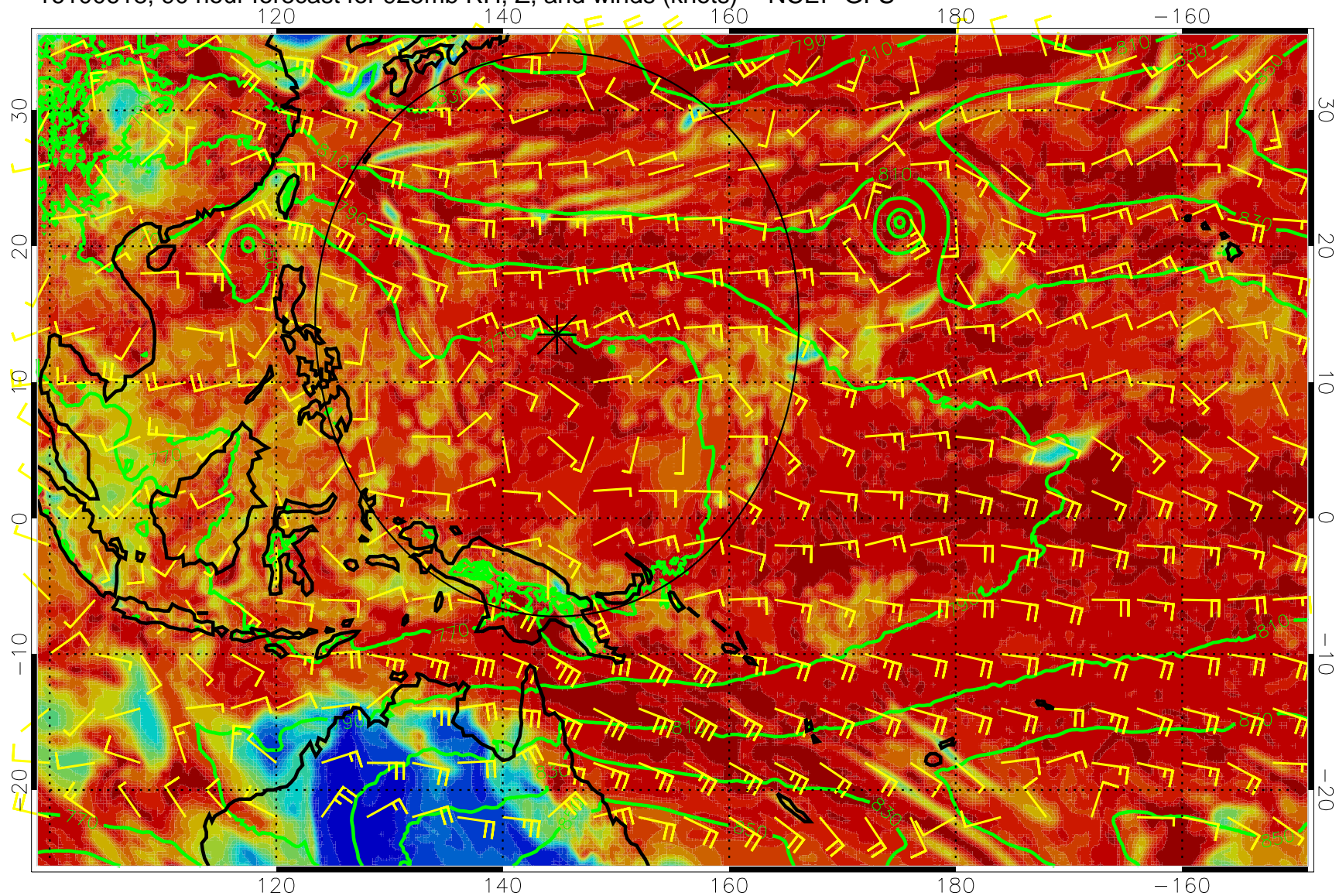
16100618, 90 hour forecast for 925mb RH, Z, and winds (knots) -- NCEP GFS
