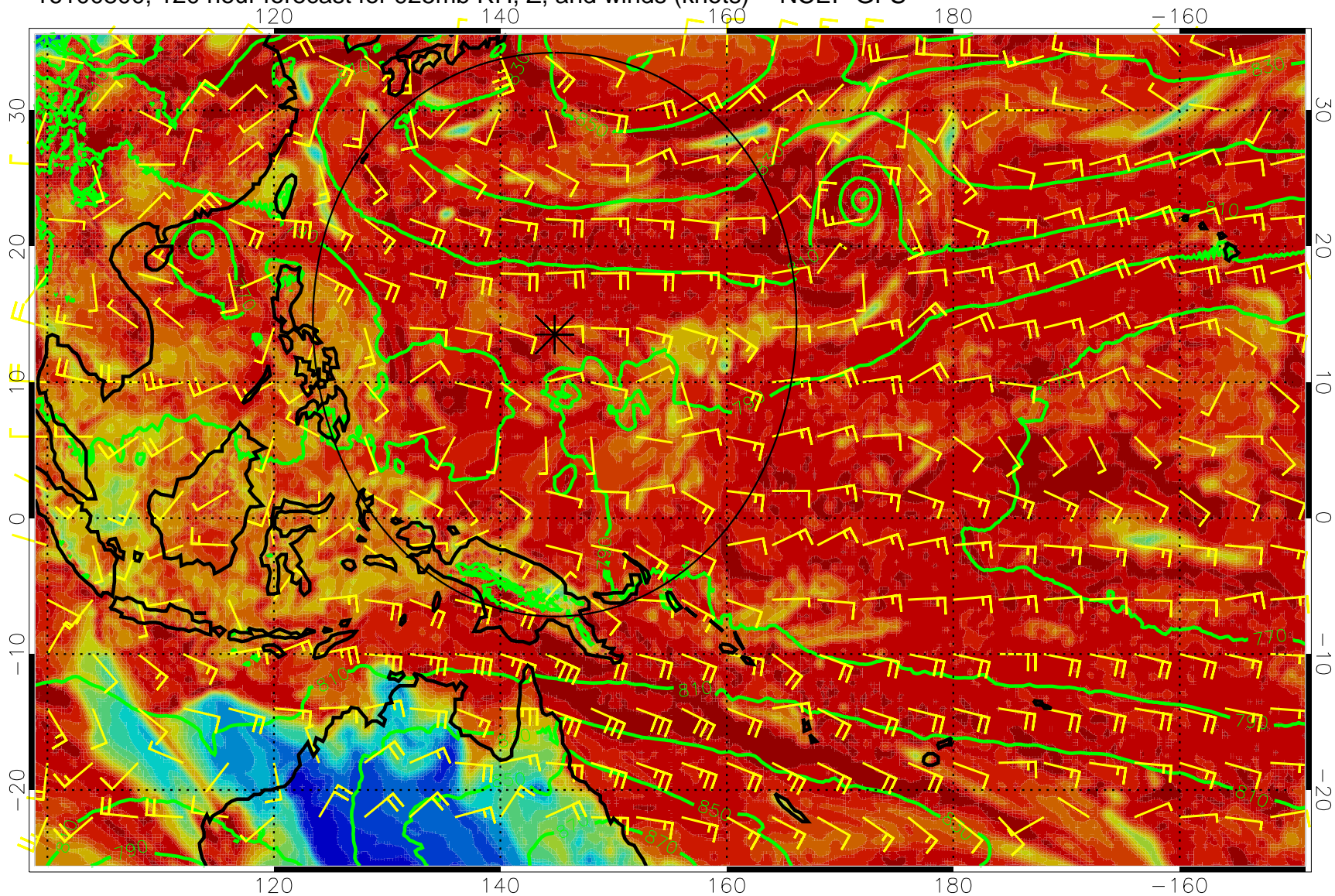
16100800, 120 hour forecast for 925mb RH, Z, and winds (knots) -- NCEP GFS
