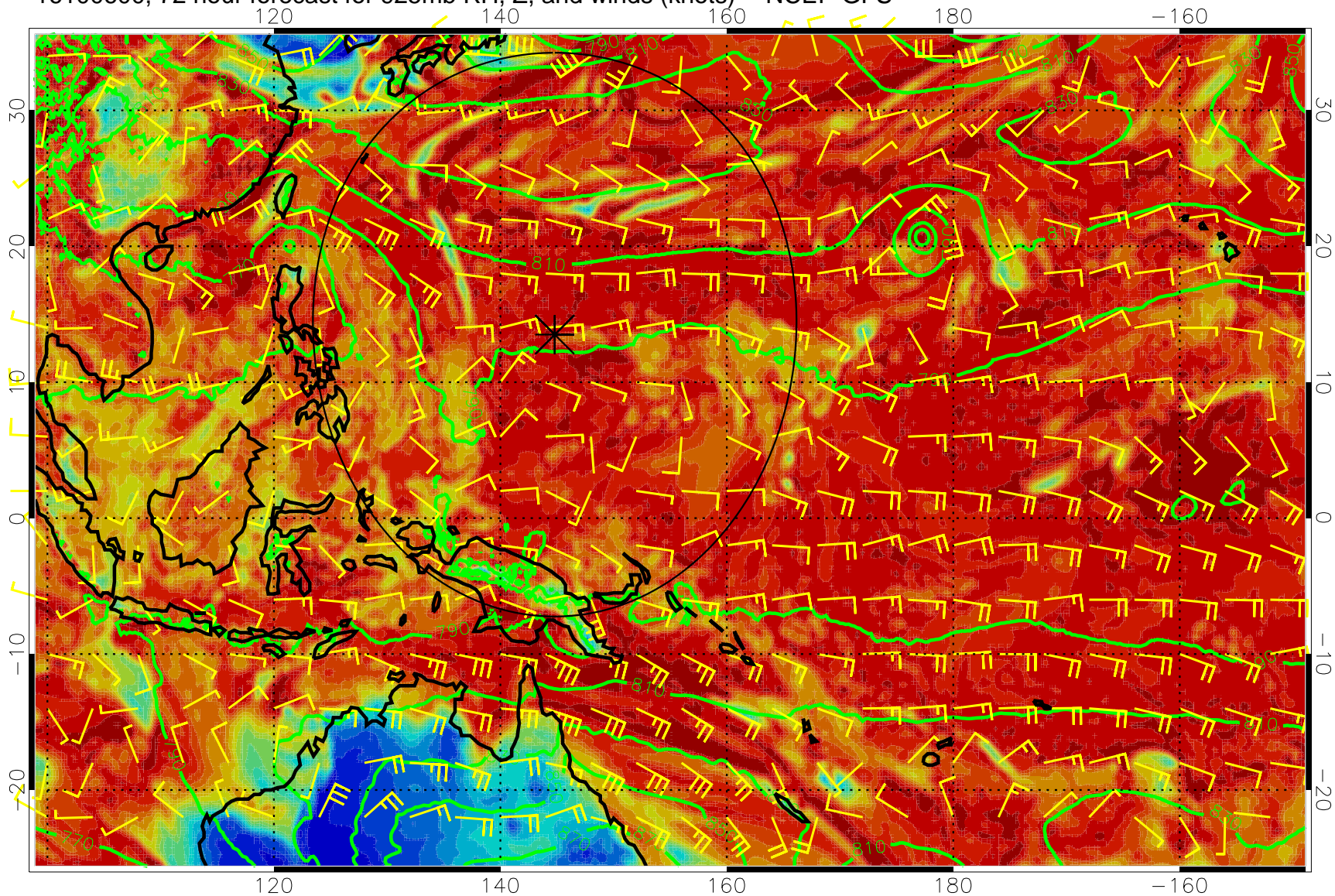
16100600, 72 hour forecast for 925mb RH, Z, and winds (knots) -- NCEP GFS
