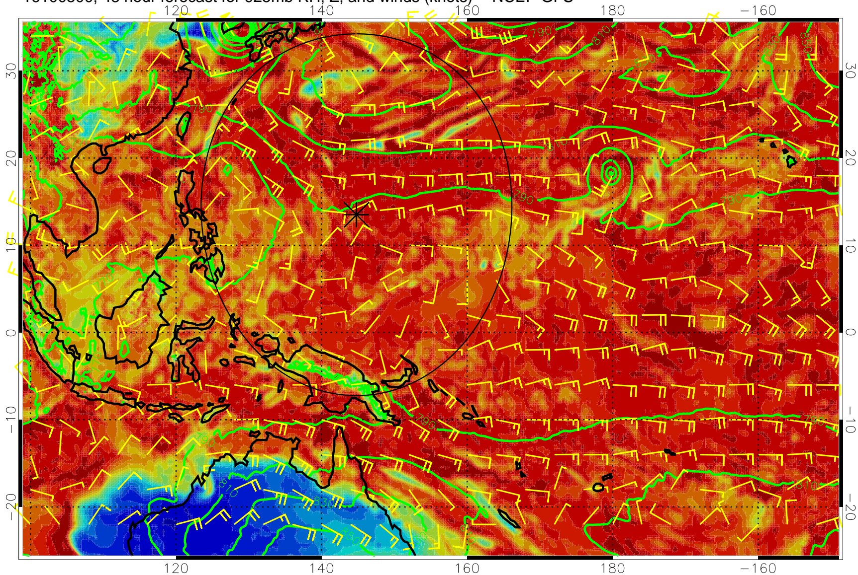
16100500, 48 hour forecast for 925mb RH, Z, and winds (knots) -- NCEP GFS
