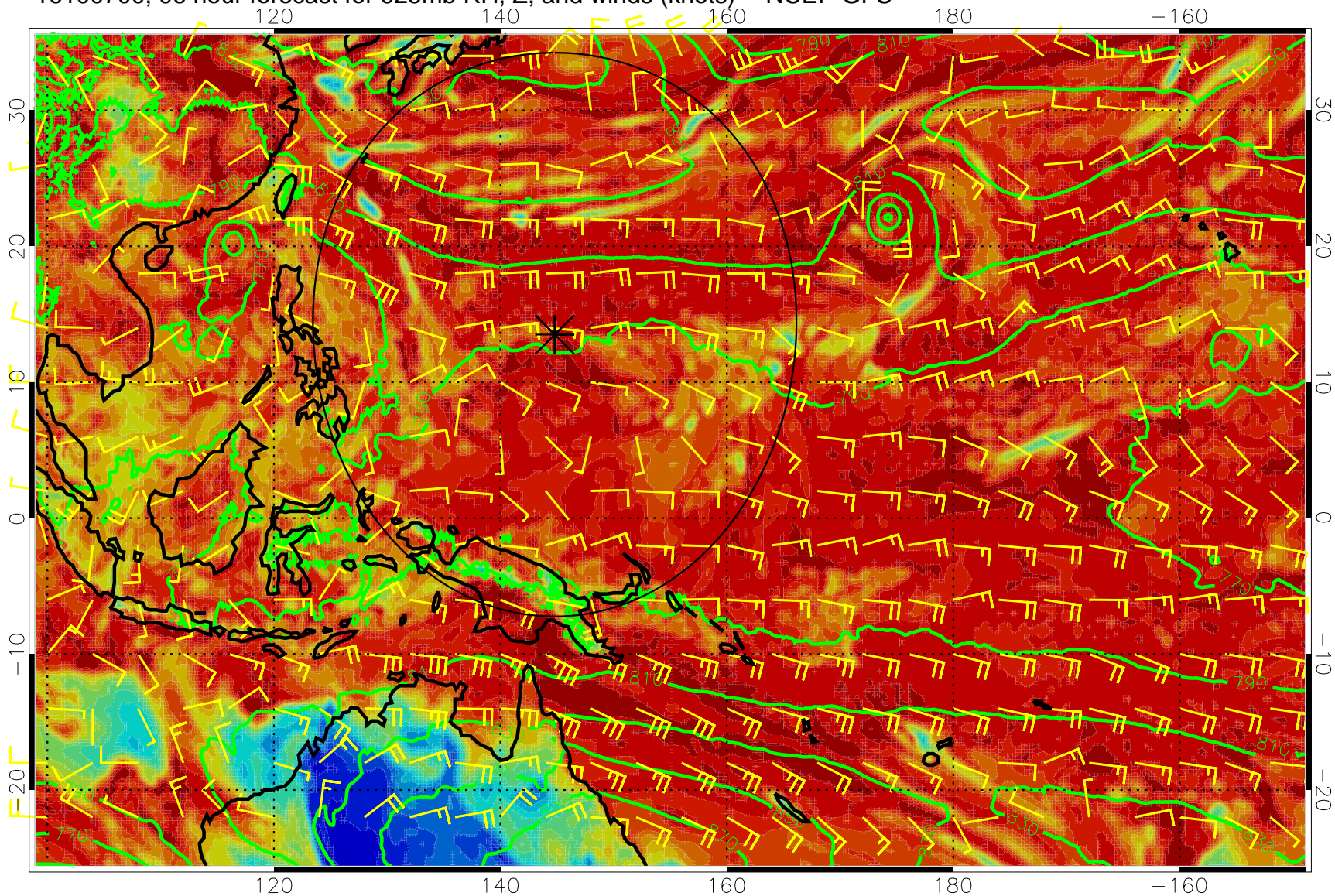
16100700, 96 hour forecast for 925mb RH, Z, and winds (knots) -- NCEP GFS
