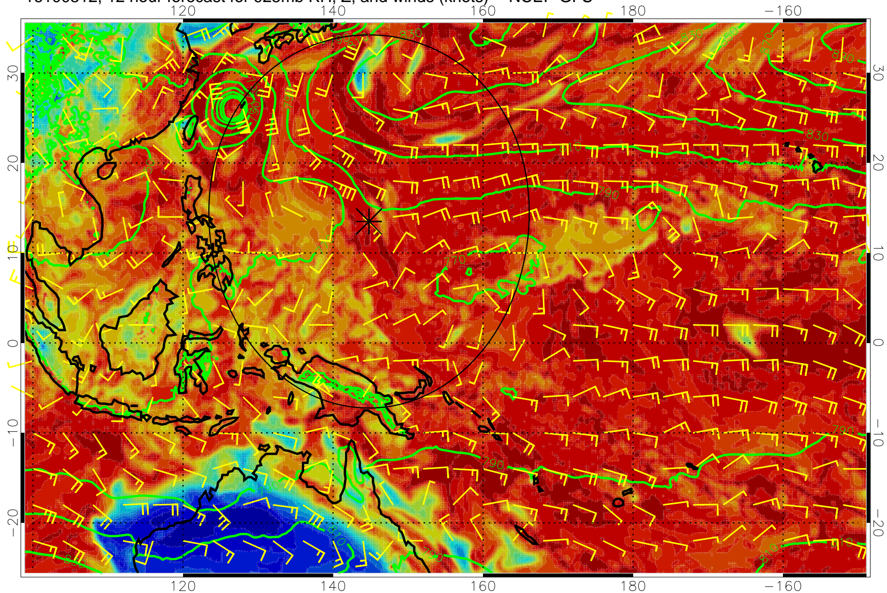
16100312, 12 hour forecast for 925mb RH, Z, and winds (knots) -- NCEP GFS
