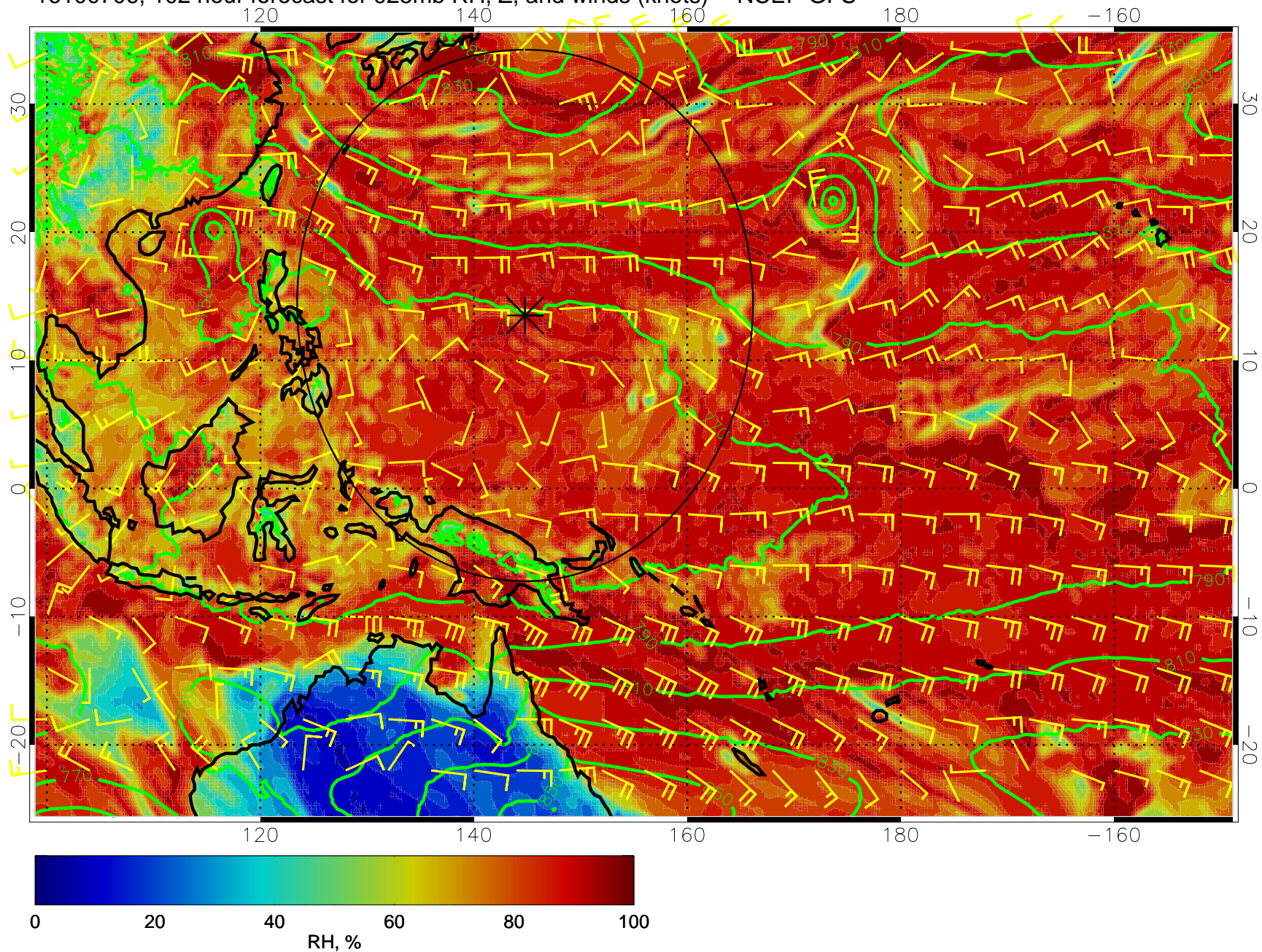
16100706, 102 hour forecast for 925mb RH, Z, and winds (knots) -- NCEP GFS
