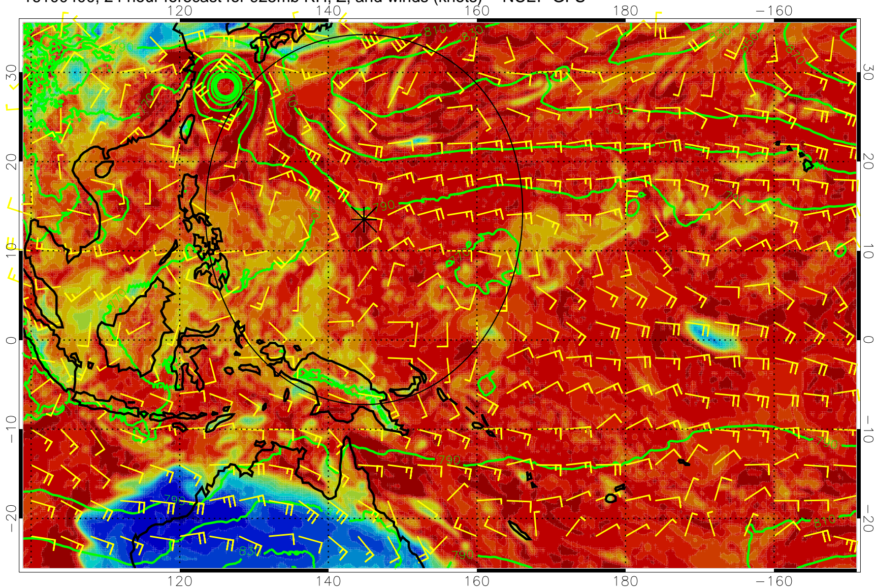
16100400, 24 hour forecast for 925mb RH, Z, and winds (knots) -- NCEP GFS
