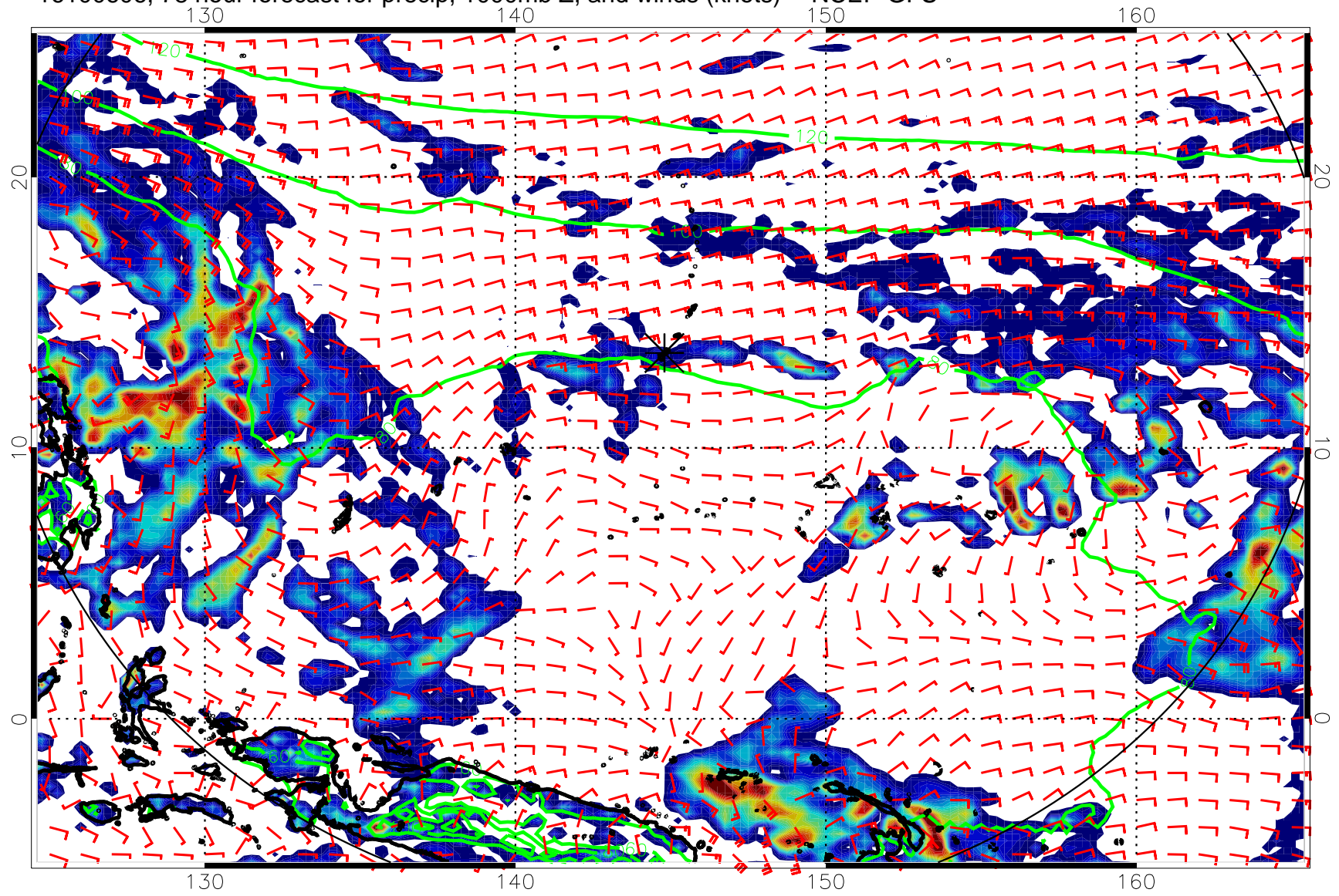
16100606, 78 hour forecast for precip, 1000mb Z, and winds (knots) -- NCEP GFS
