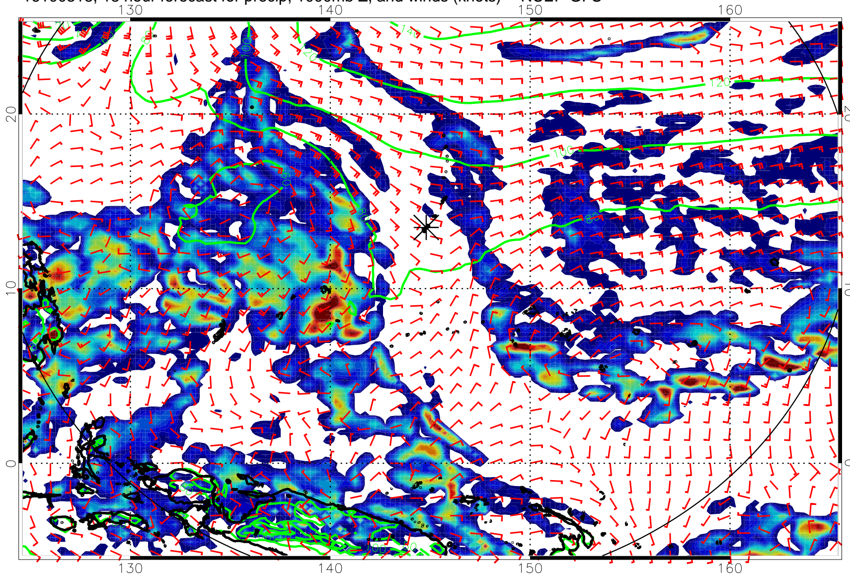
16100318, 18 hour forecast for precip, 1000mb Z, and winds (knots) -- NCEP GFS
