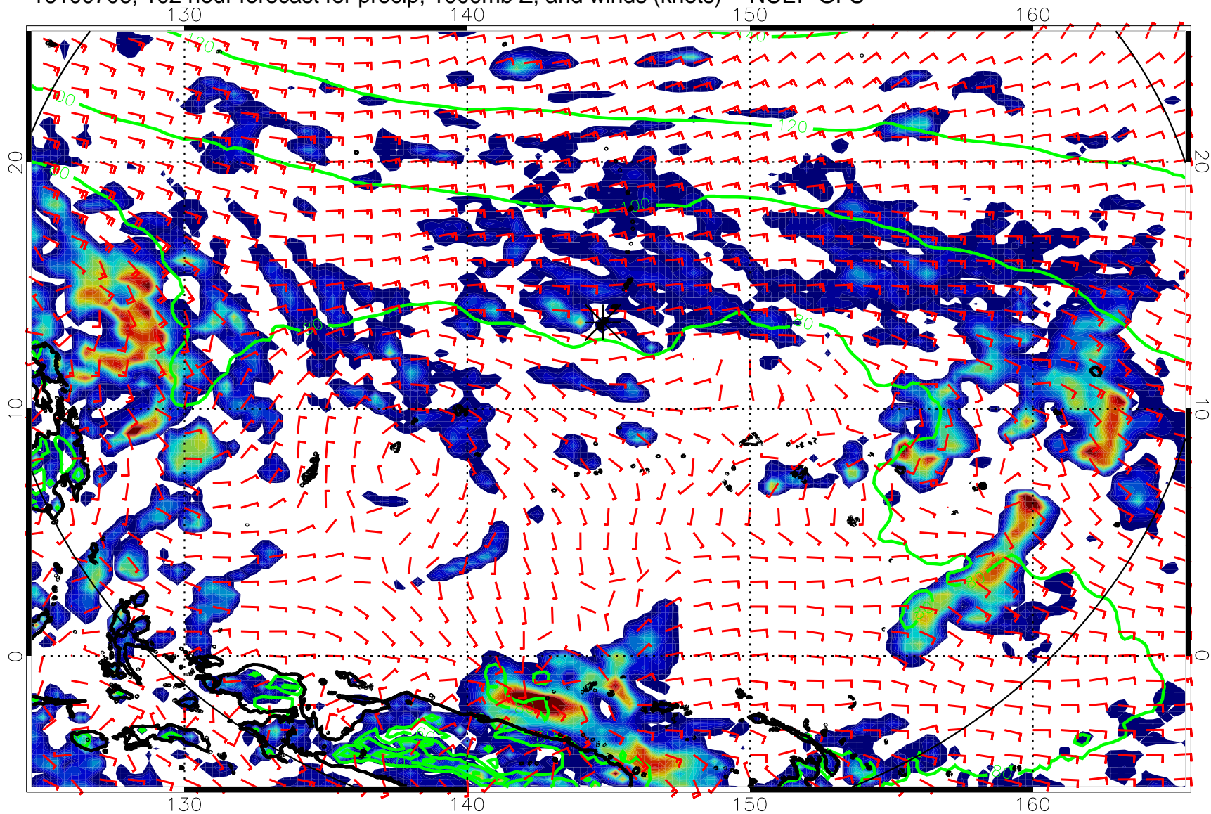
16100706, 102 hour forecast for precip, 1000mb Z, and winds (knots) -- NCEP GFS
