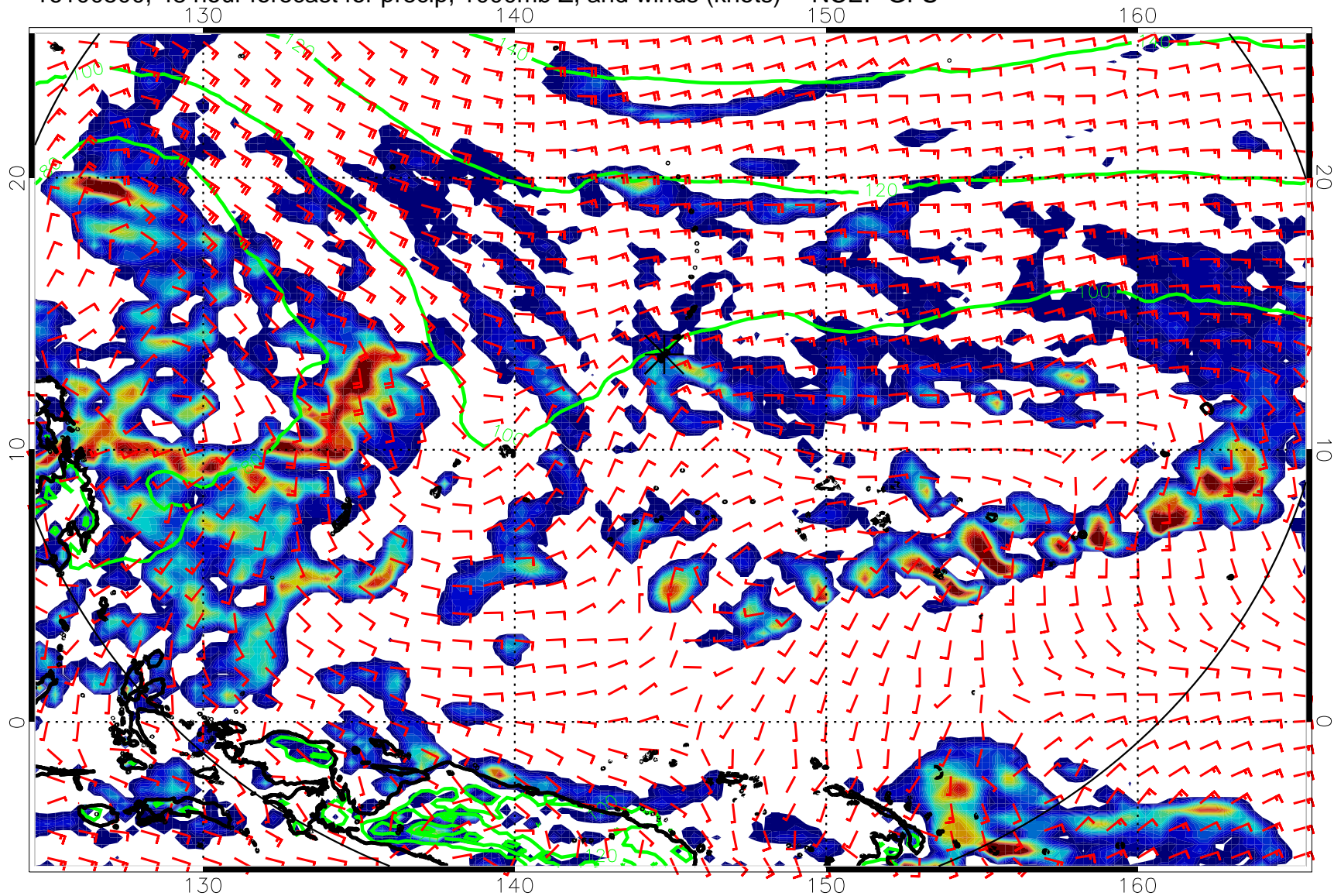
16100500, 48 hour forecast for precip, 1000mb Z, and winds (knots) -- NCEP GFS
