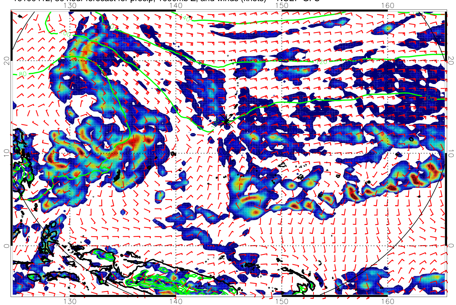
16100412, 36 hour forecast for precip, 1000mb Z, and winds (knots) -- NCEP GFS
