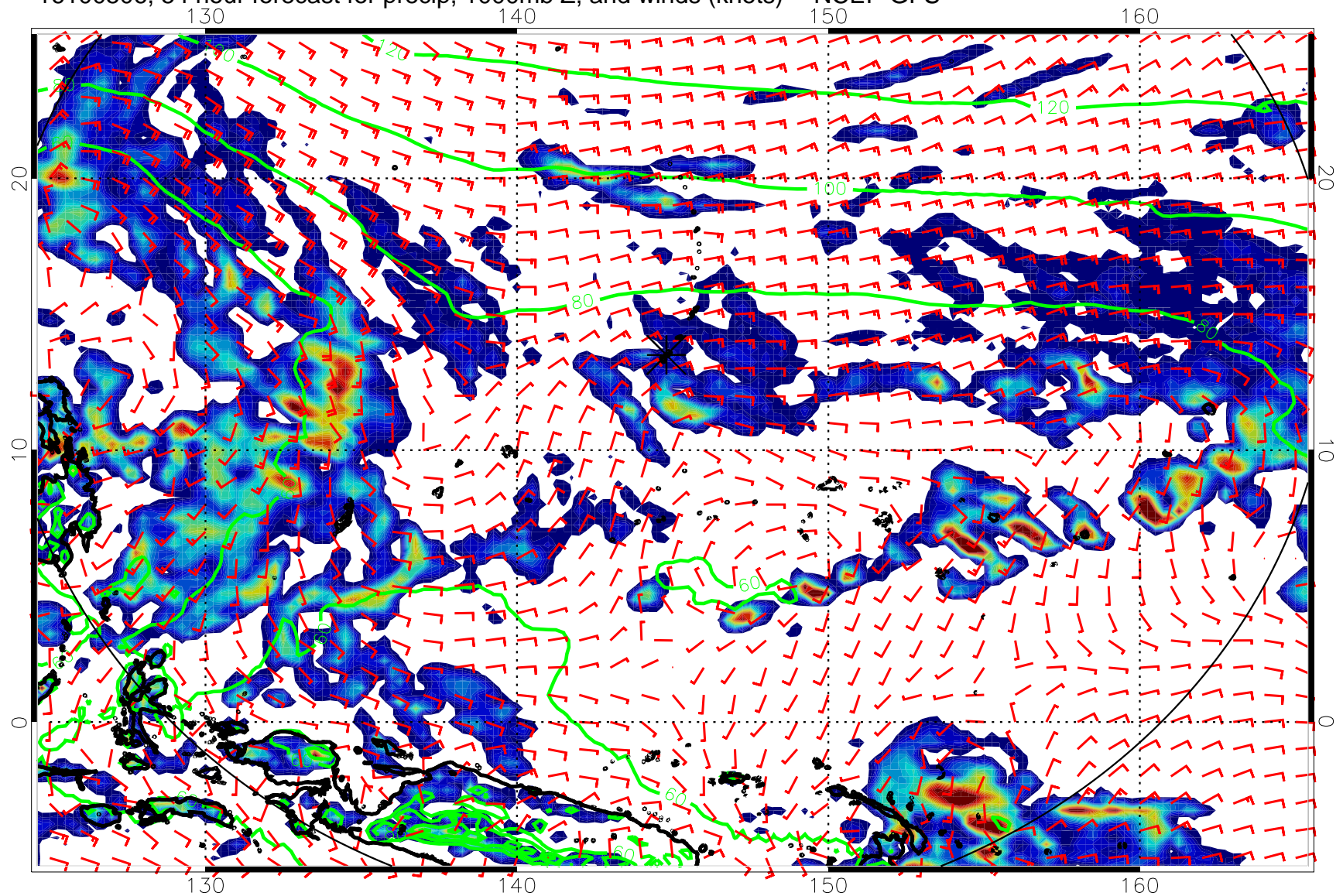
16100506, 54 hour forecast for precip, 1000mb Z, and winds (knots) -- NCEP GFS
