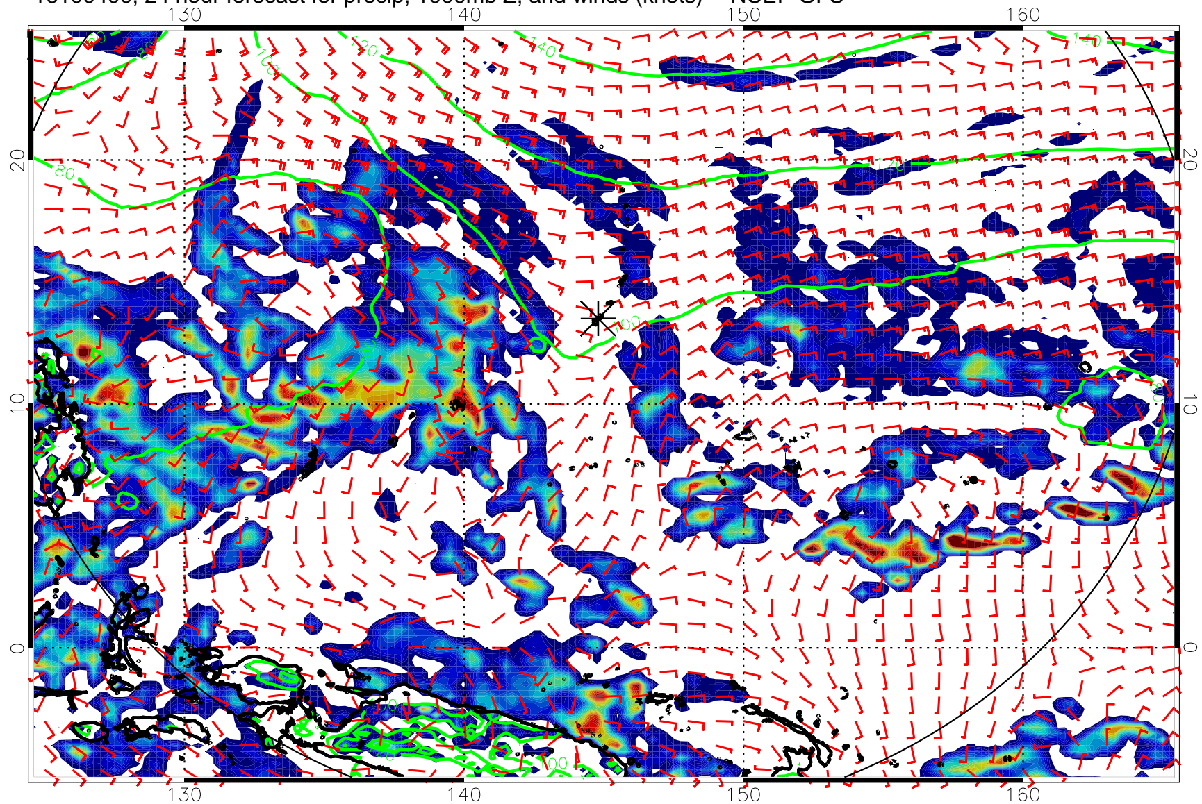
16100400, 24 hour forecast for precip, 1000mb Z, and winds (knots) -- NCEP GFS
