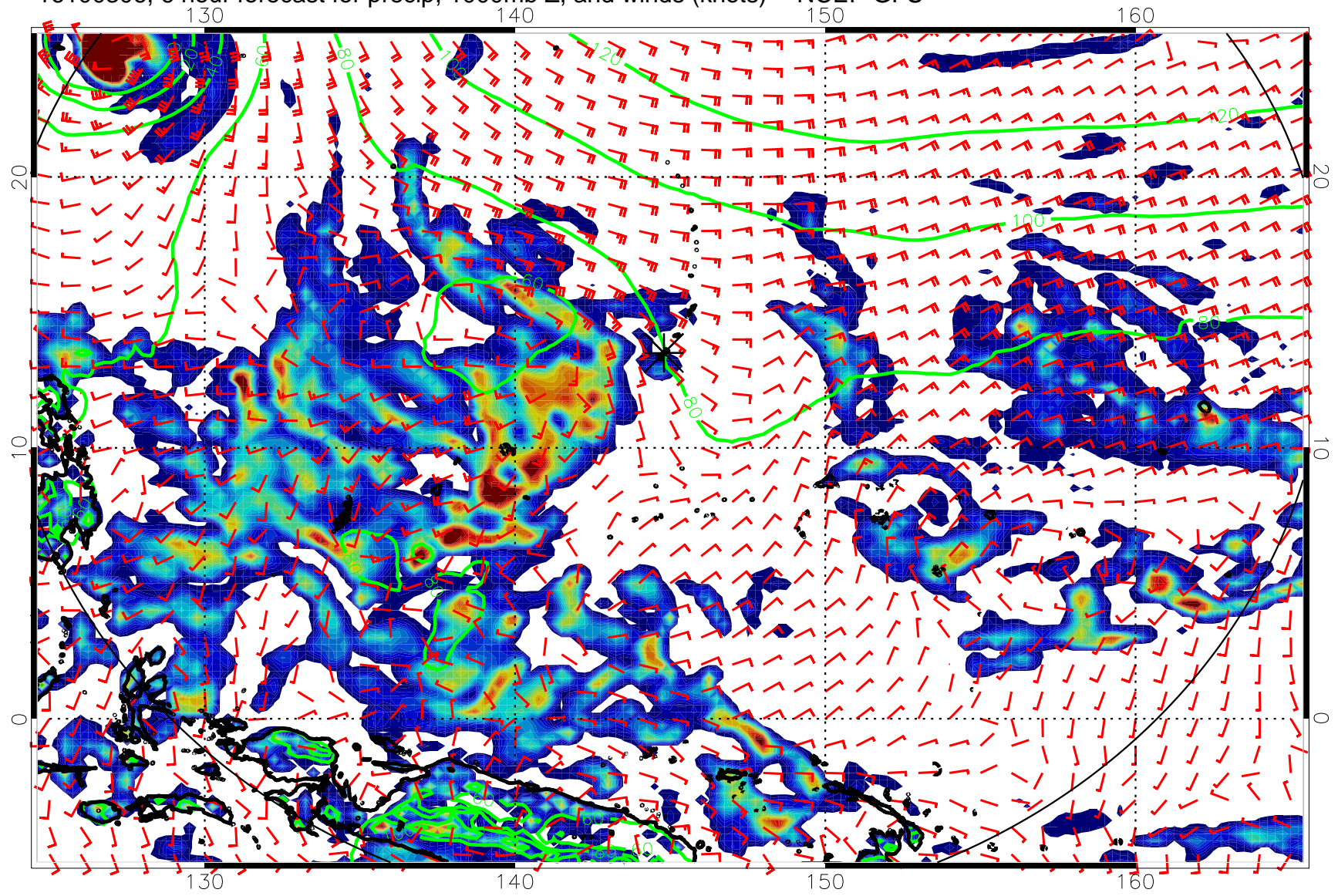
16100306, 6 hour forecast for precip, 1000mb Z, and winds (knots) -- NCEP GFS
