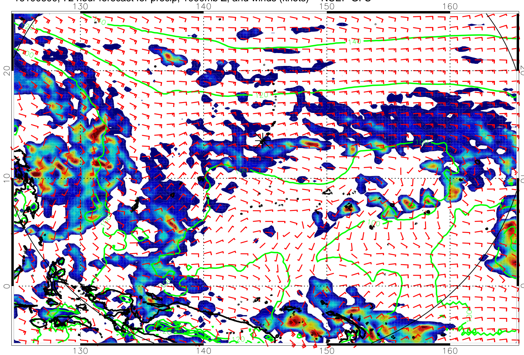
16100600, 72 hour forecast for precip, 1000mb Z, and winds (knots) -- NCEP GFS
