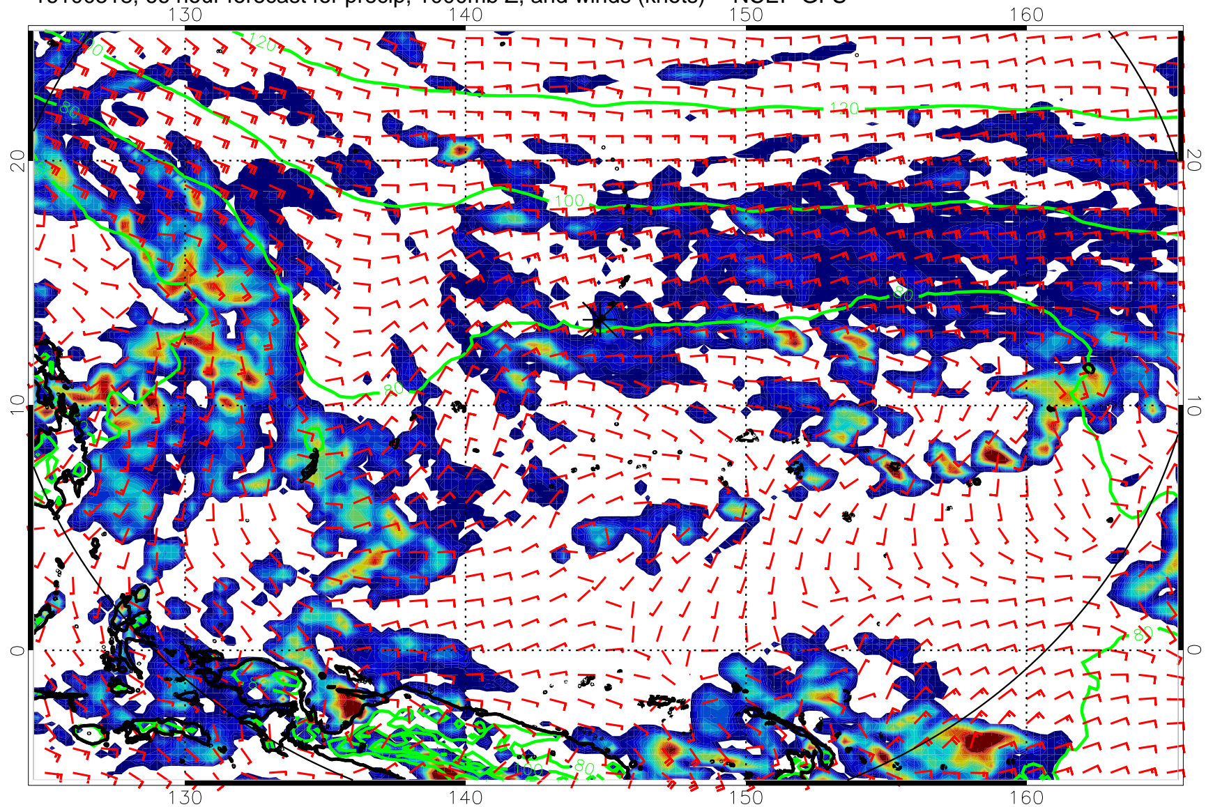
16100518, 66 hour forecast for precip, 1000mb Z, and winds (knots) -- NCEP GFS
