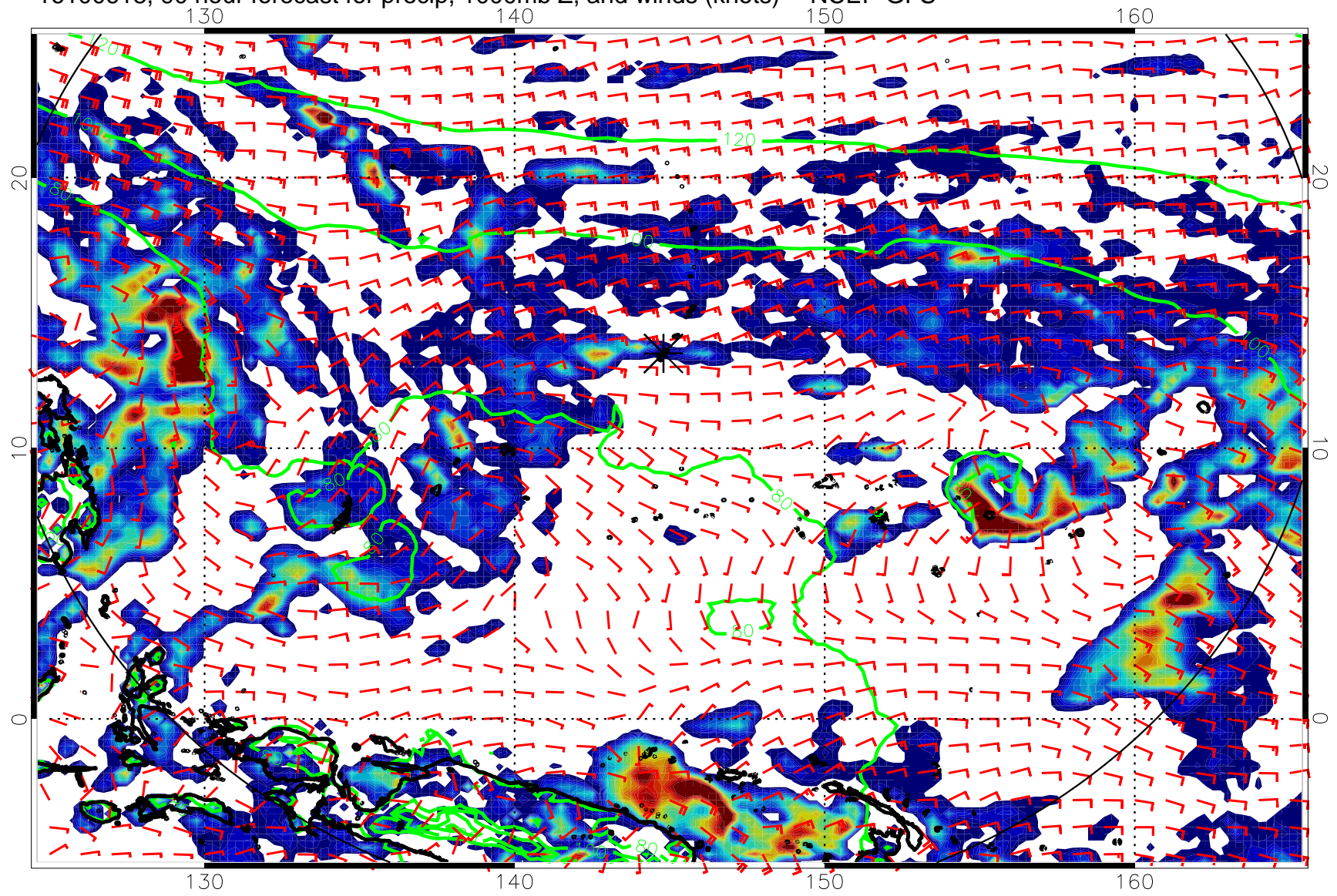
16100618, 90 hour forecast for precip, 1000mb Z, and winds (knots) -- NCEP GFS
