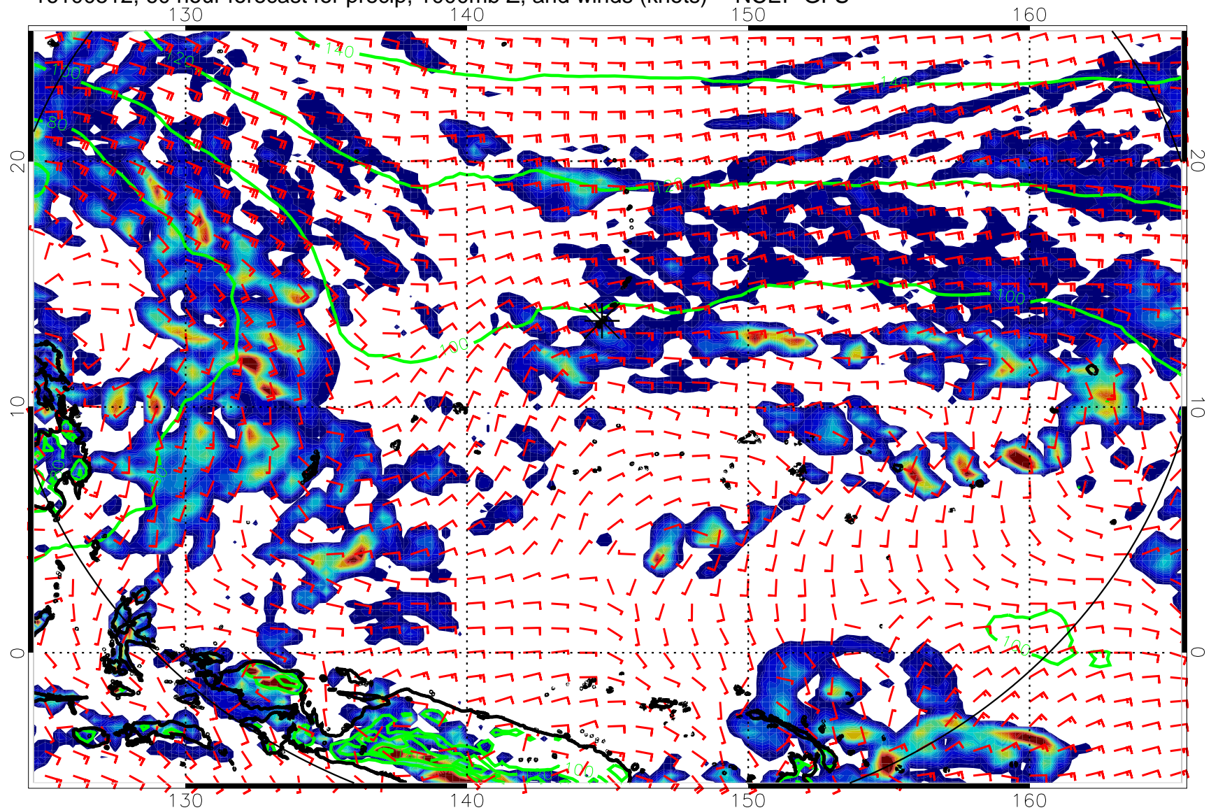
16100512, 60 hour forecast for precip, 1000mb Z, and winds (knots) -- NCEP GFS
