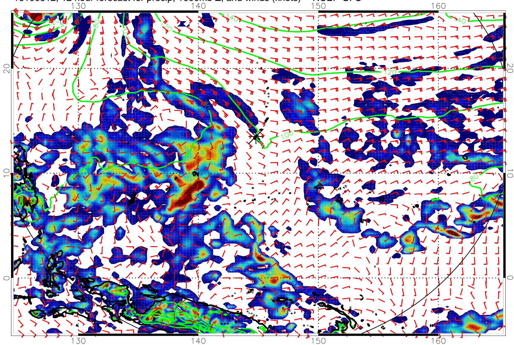
16100312, 12 hour forecast for precip, 1000mb Z, and winds (knots) -- NCEP GFS
