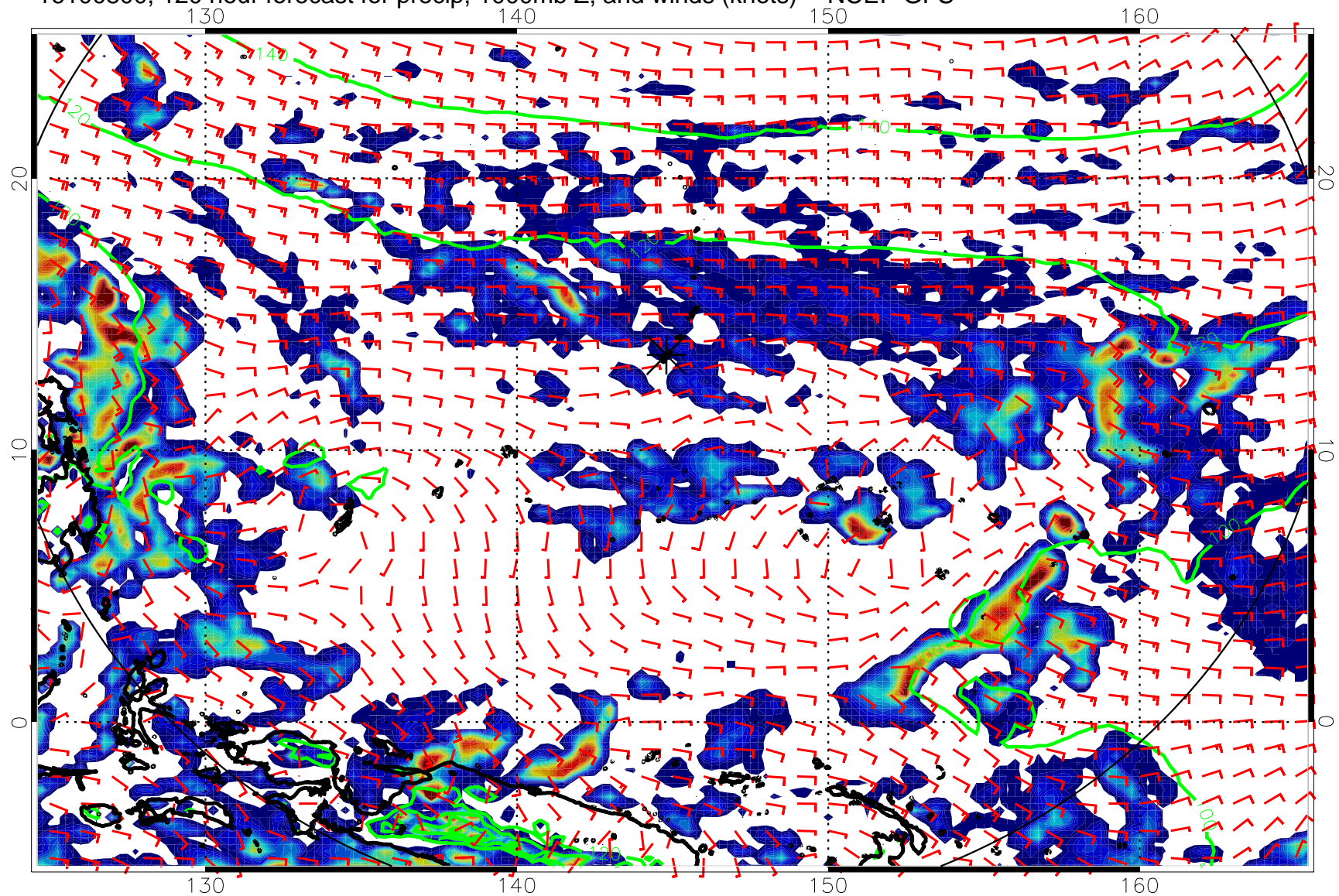
16100800, 120 hour forecast for precip, 1000mb Z, and winds (knots) -- NCEP GFS
