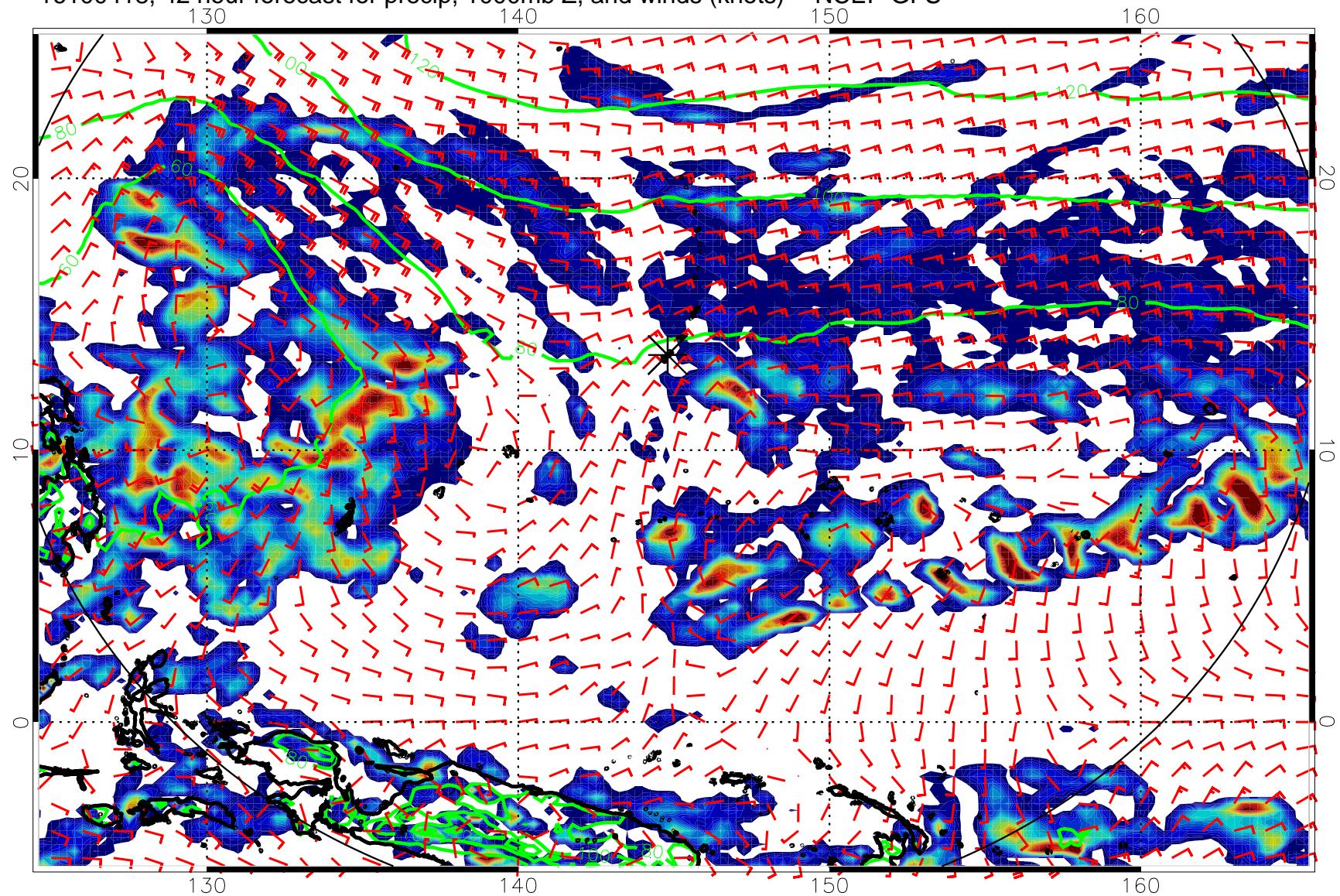
16100418, 42 hour forecast for precip, 1000mb Z, and winds (knots) -- NCEP GFS
