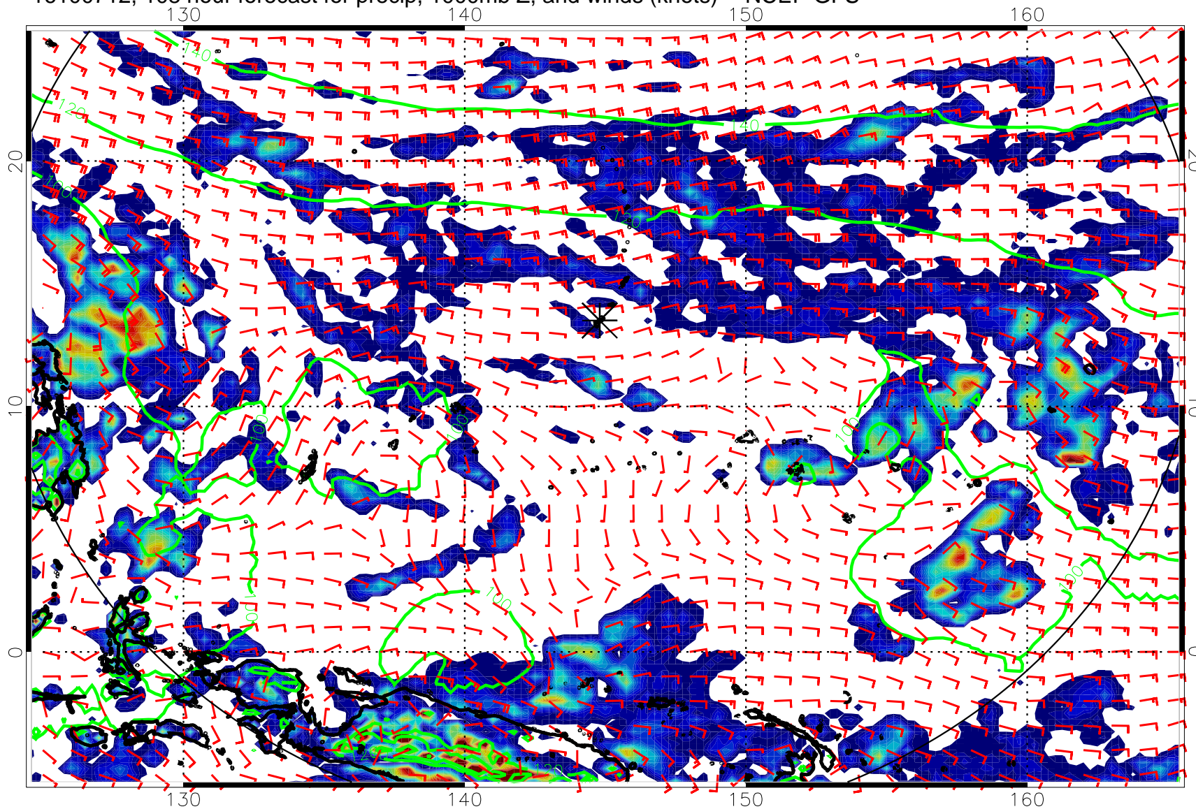
16100712, 108 hour forecast for precip, 1000mb Z, and winds (knots) -- NCEP GFS
