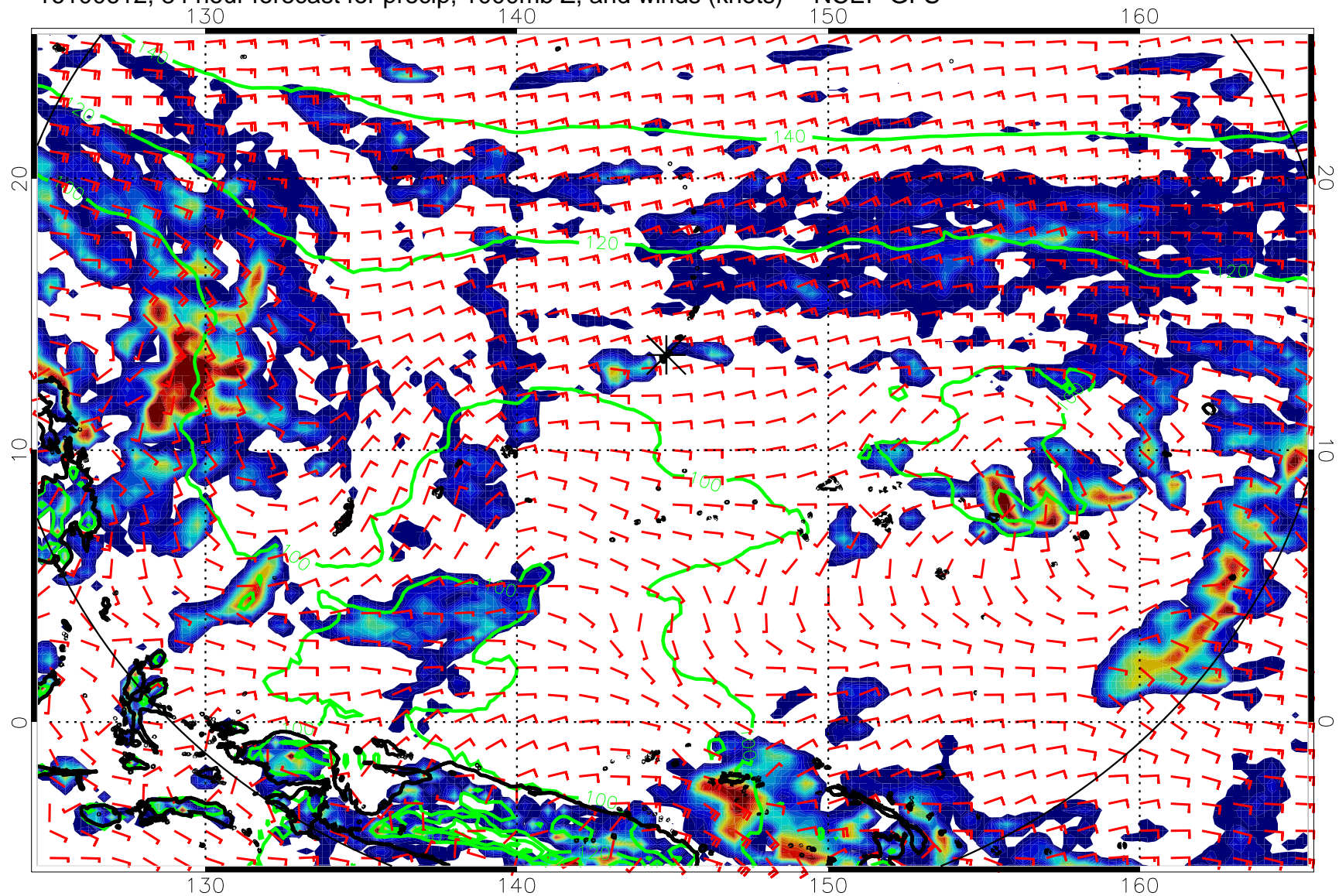
16100612, 84 hour forecast for precip, 1000mb Z, and winds (knots) -- NCEP GFS
