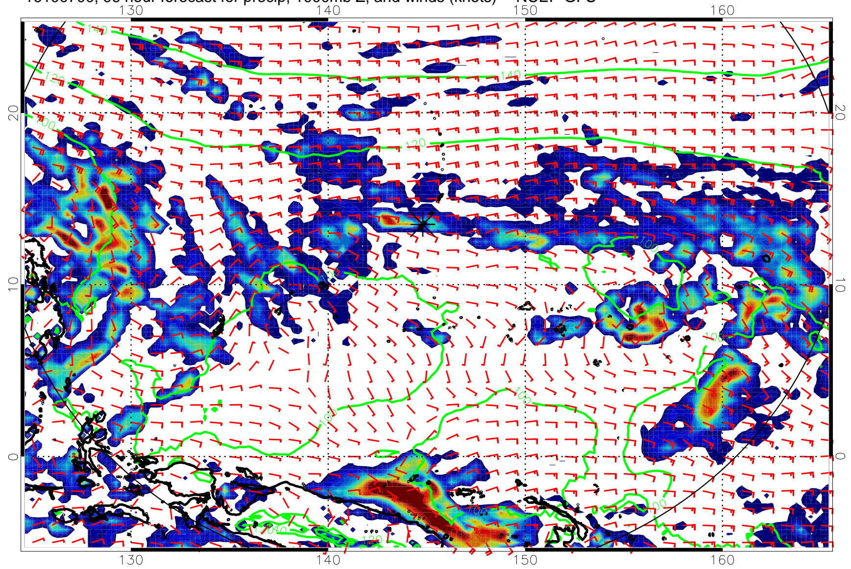
16100700, 96 hour forecast for precip, 1000mb Z, and winds (knots) -- NCEP GFS
