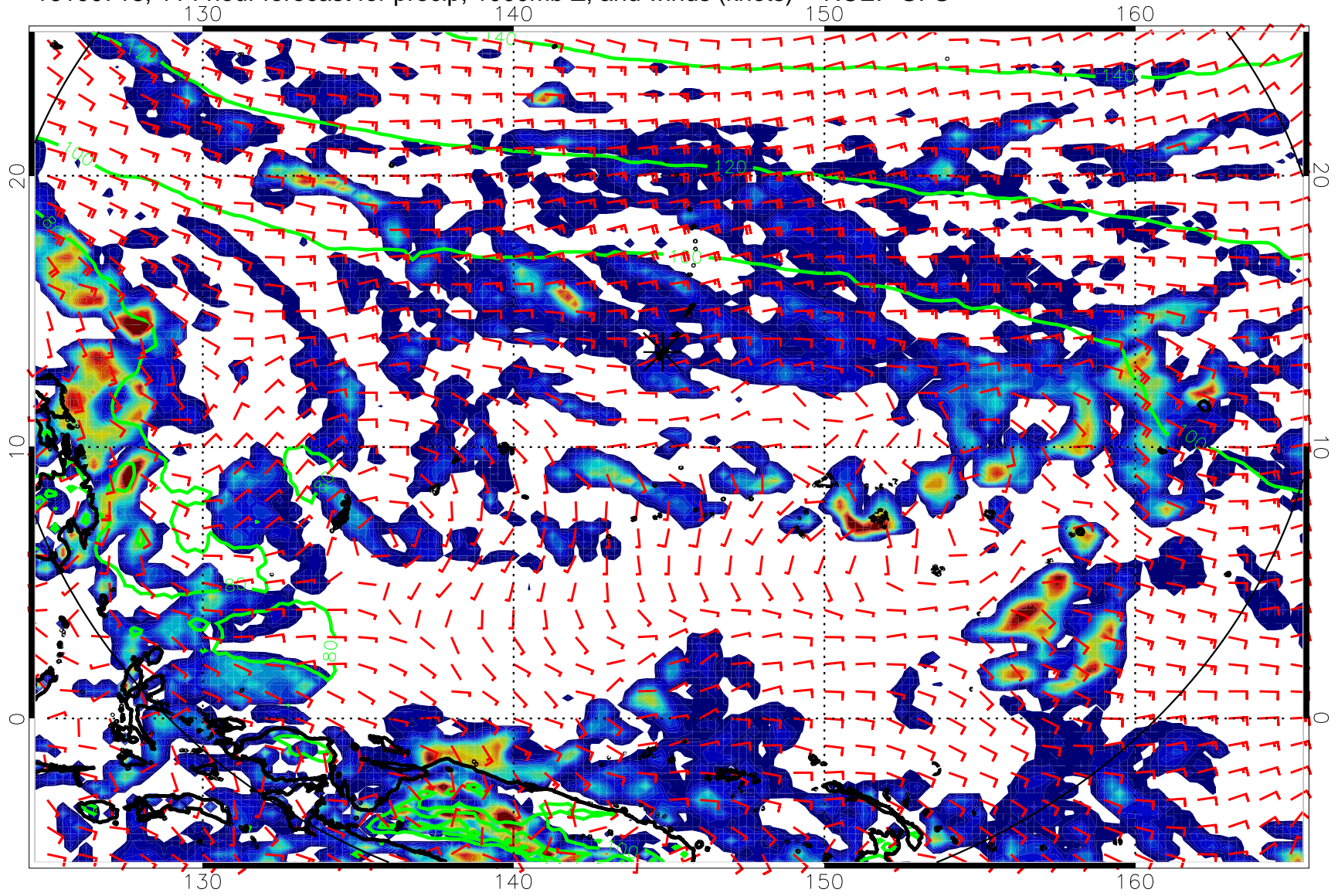
16100718, 114 hour forecast for precip, 1000mb Z, and winds (knots) -- NCEP GFS
