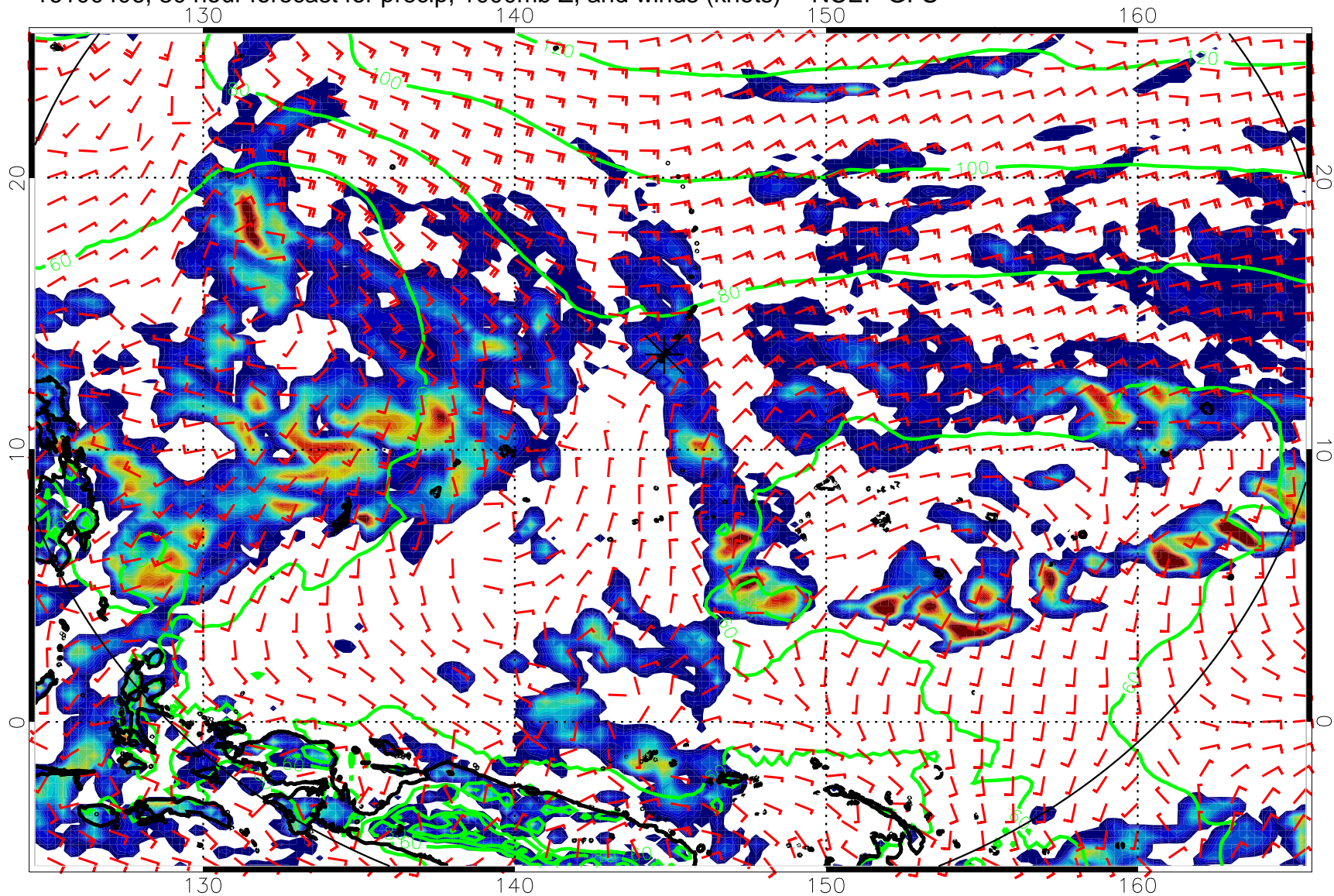
16100406, 30 hour forecast for precip, 1000mb Z, and winds (knots) -- NCEP GFS
