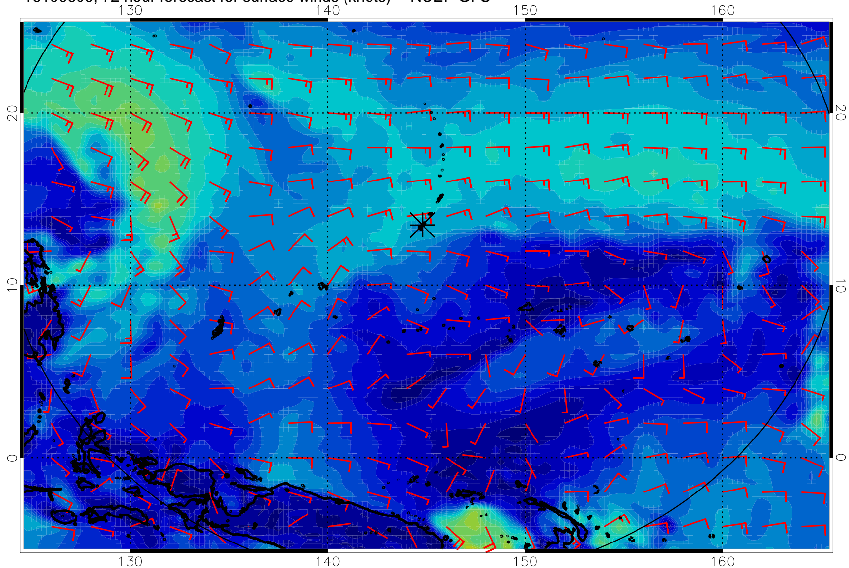
16100600, 72 hour forecast for surface winds (knots) -- NCEP GFS
