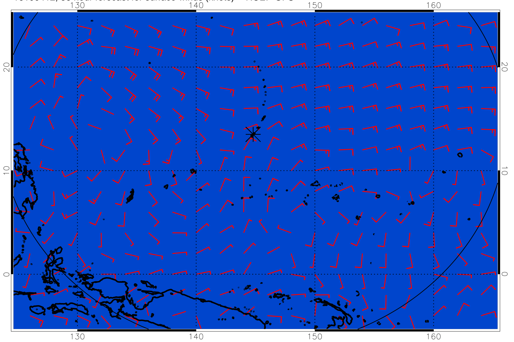
16100412, 36 hour forecast for surface winds (knots) -- NCEP GFS
