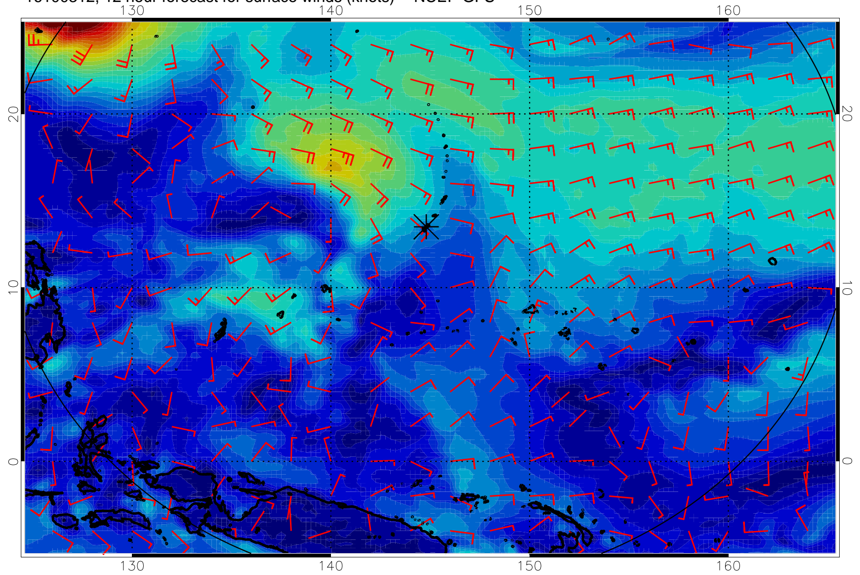
16100312, 12 hour forecast for surface winds (knots) -- NCEP GFS
