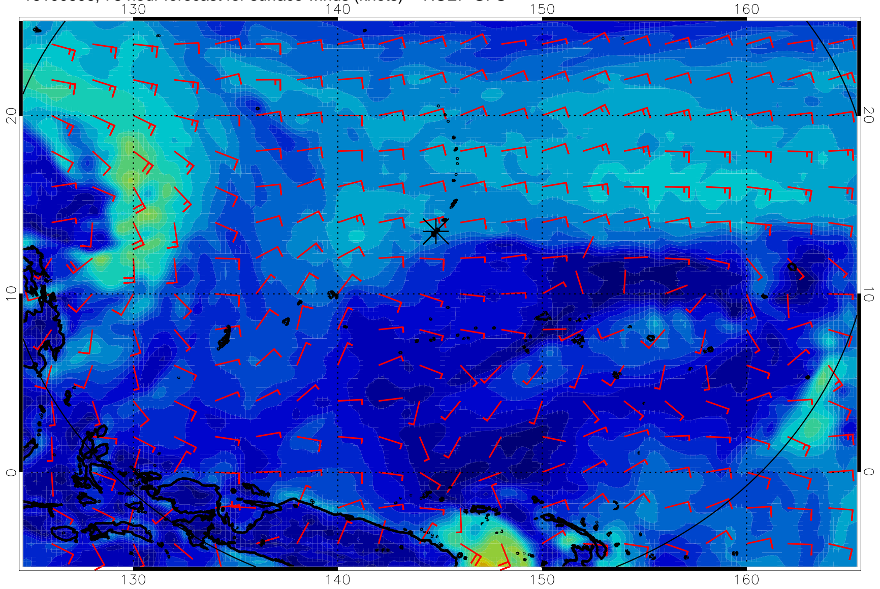
16100606, 78 hour forecast for surface winds (knots) -- NCEP GFS
