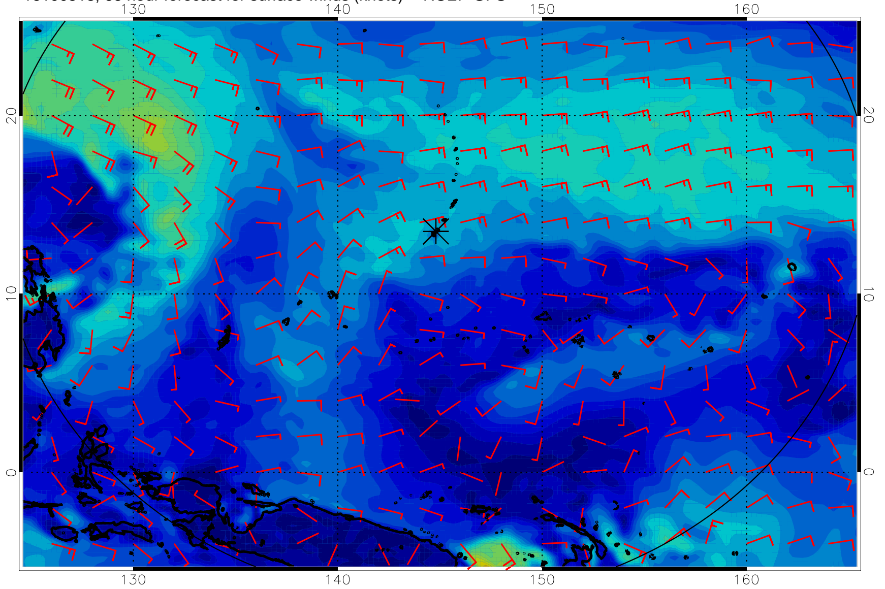
16100518, 66 hour forecast for surface winds (knots) -- NCEP GFS
