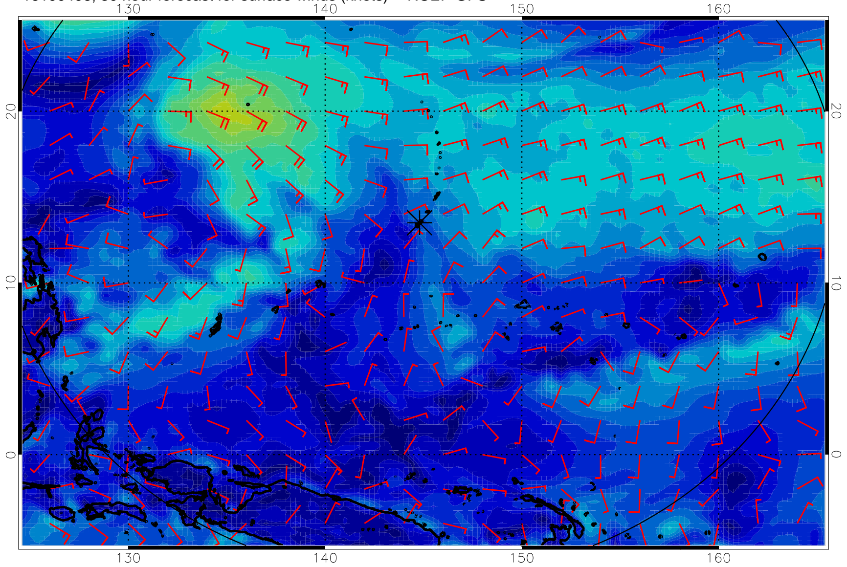
16100406, 30 hour forecast for surface winds (knots) -- NCEP GFS
