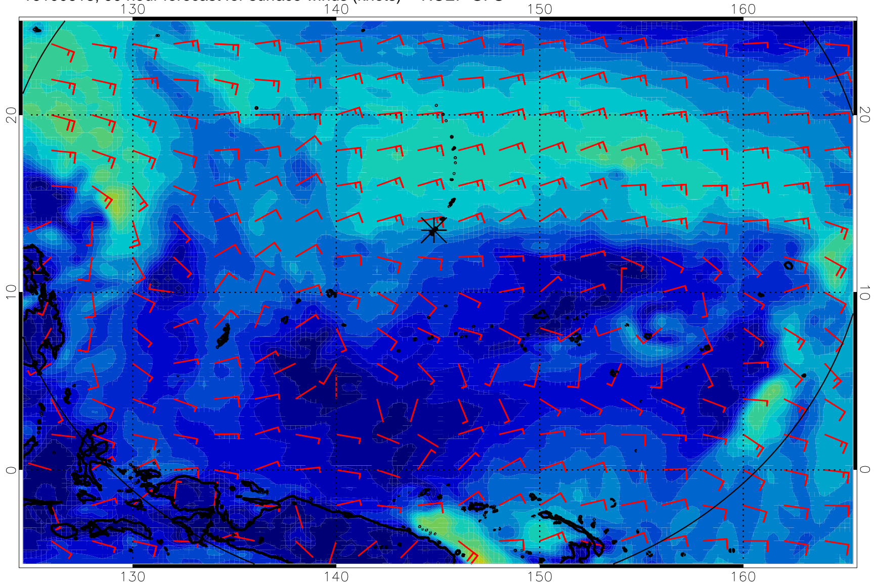
16100618, 90 hour forecast for surface winds (knots) -- NCEP GFS
