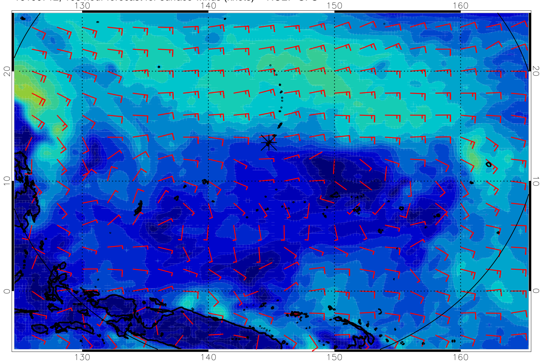
16100712, 108 hour forecast for surface winds (knots) -- NCEP GFS
