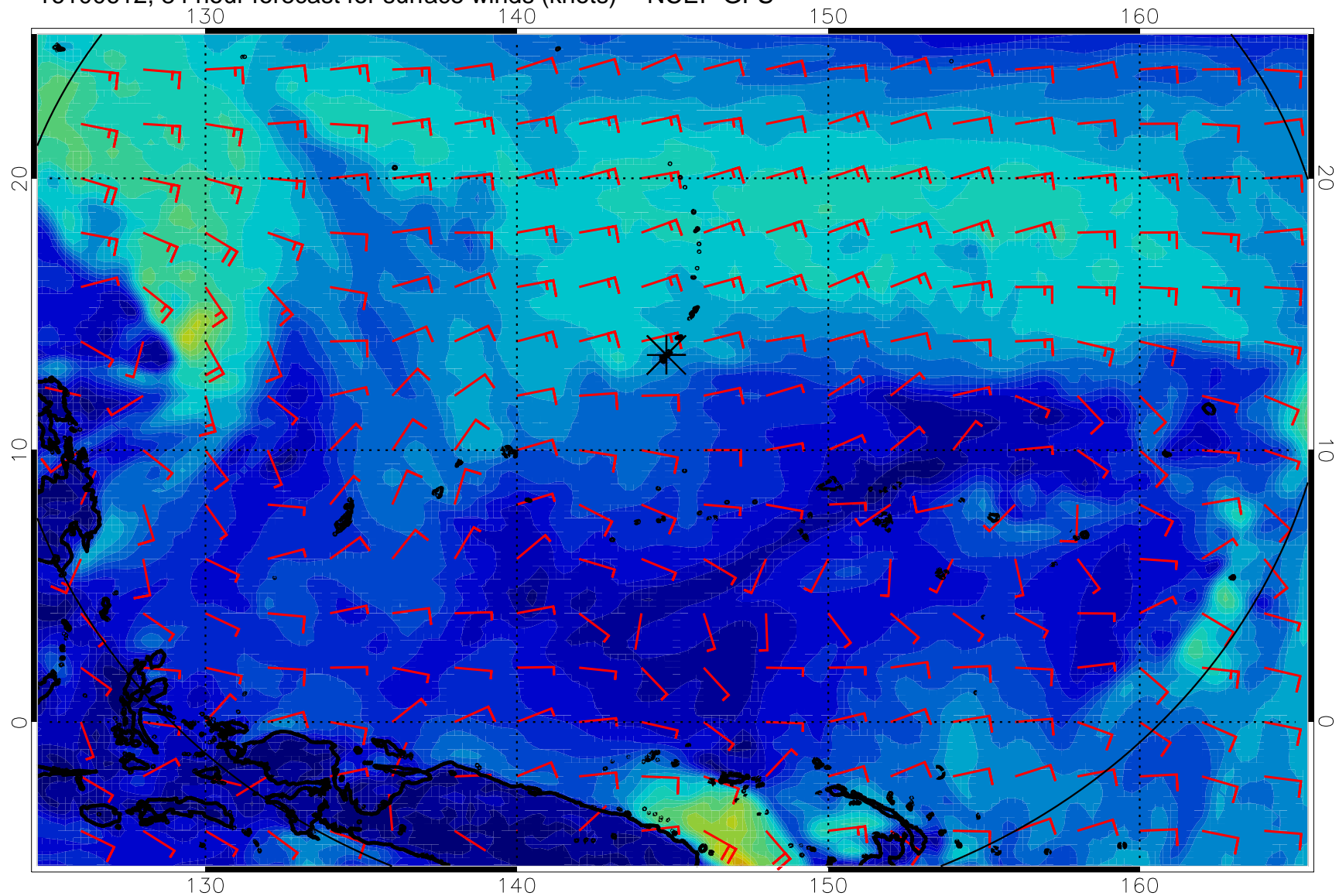
16100612, 84 hour forecast for surface winds (knots) -- NCEP GFS
