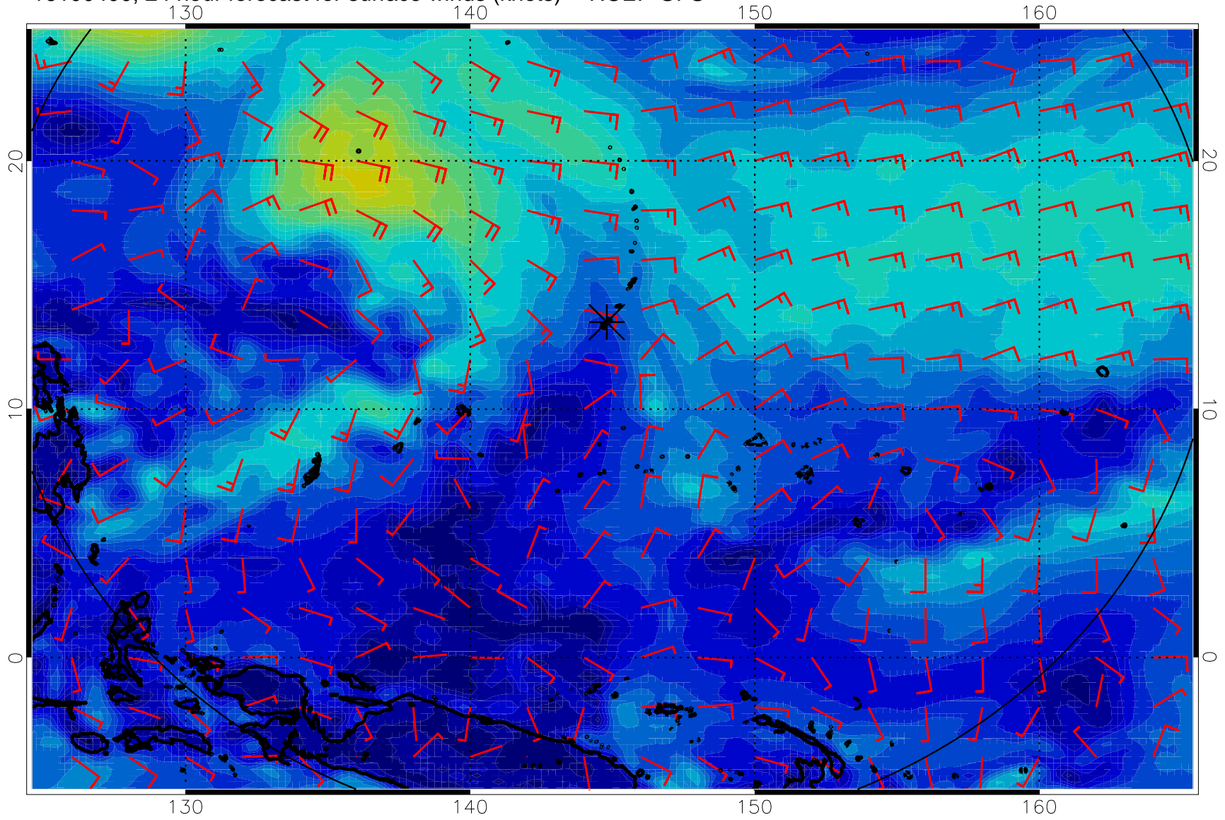
16100400, 24 hour forecast for surface winds (knots) -- NCEP GFS
