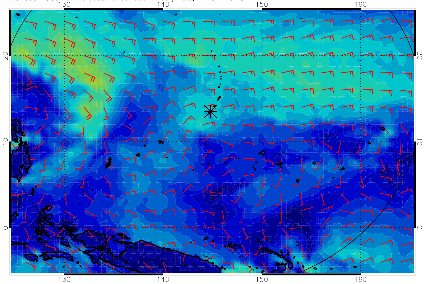
16100512, 60 hour forecast for surface winds (knots) -- NCEP GFS
