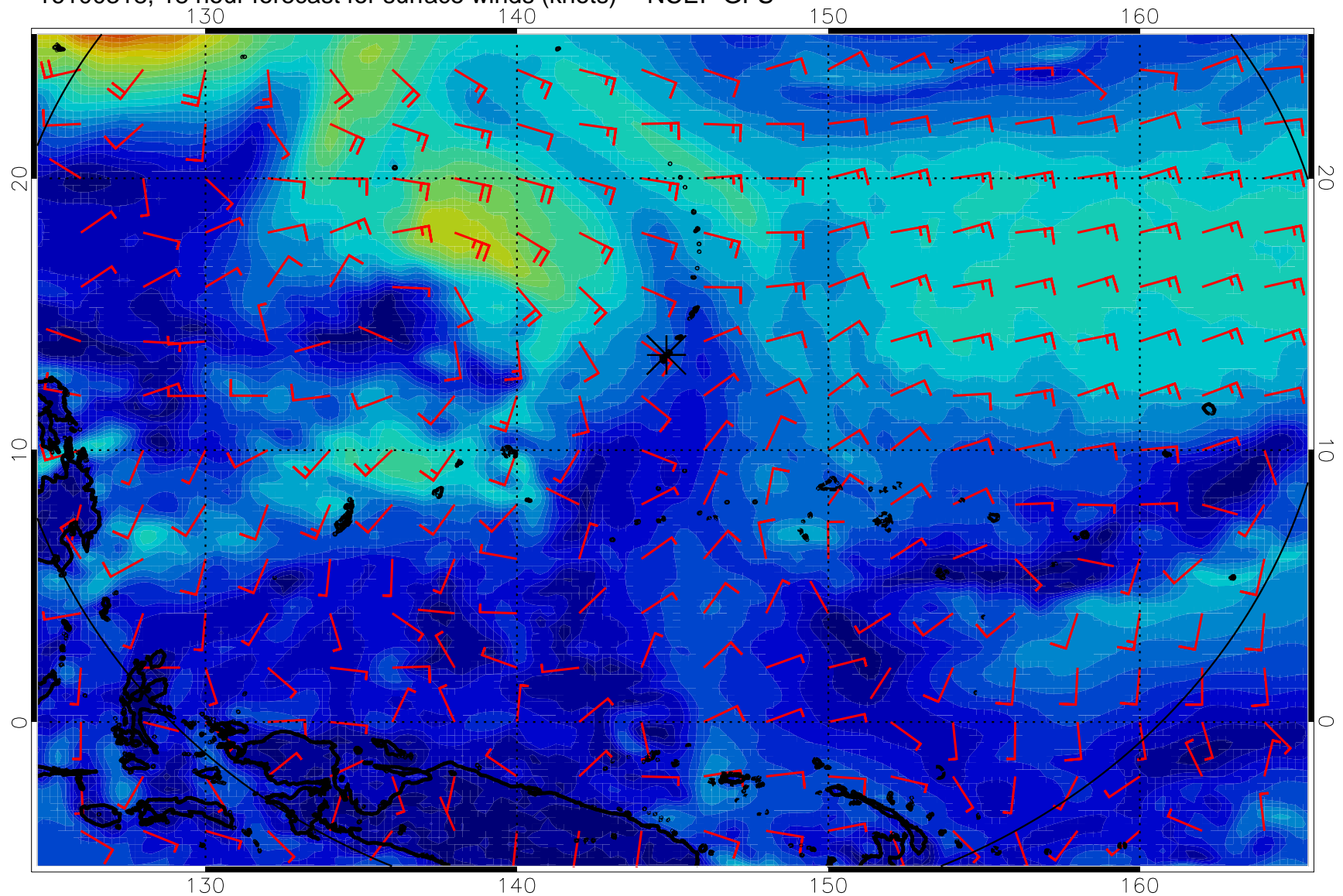
16100318, 18 hour forecast for surface winds (knots) -- NCEP GFS
