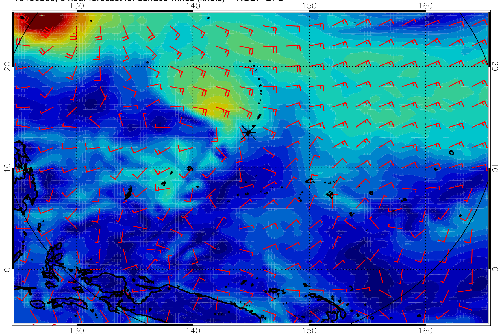
16100306, 6 hour forecast for surface winds (knots) -- NCEP GFS
