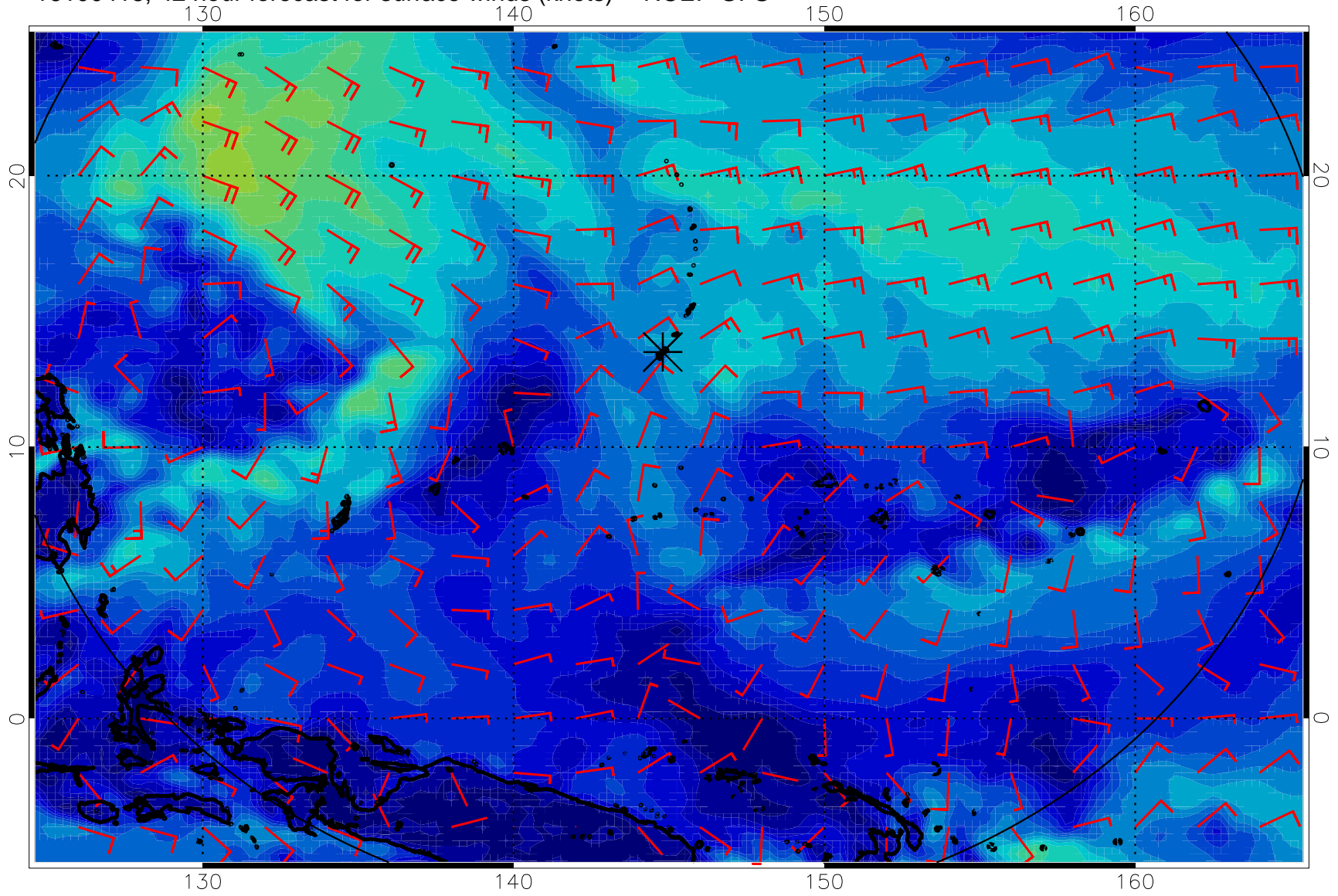
16100418, 42 hour forecast for surface winds (knots) -- NCEP GFS
