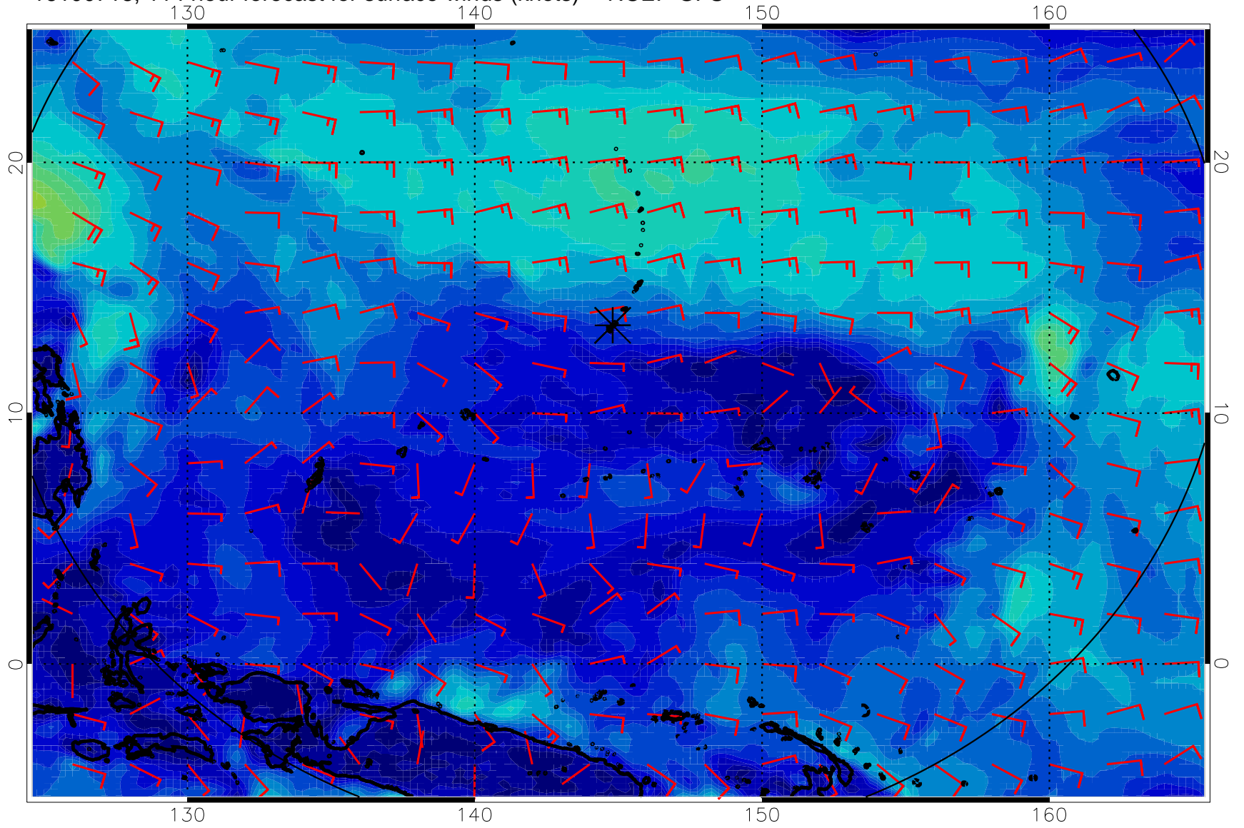
16100718, 114 hour forecast for surface winds (knots) -- NCEP GFS
