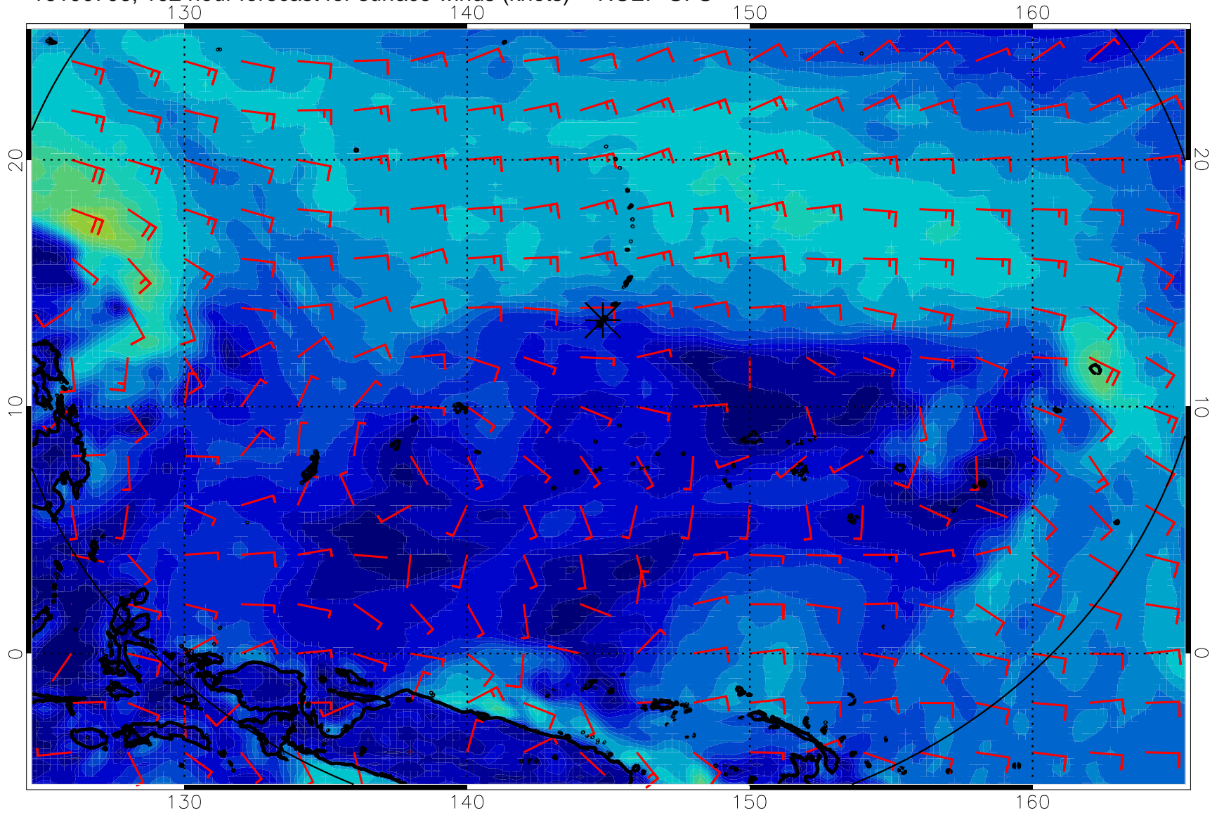
16100706, 102 hour forecast for surface winds (knots) -- NCEP GFS
