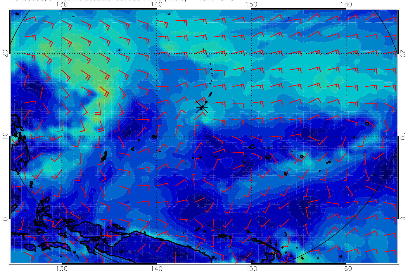
16100506, 54 hour forecast for surface winds (knots) -- NCEP GFS
