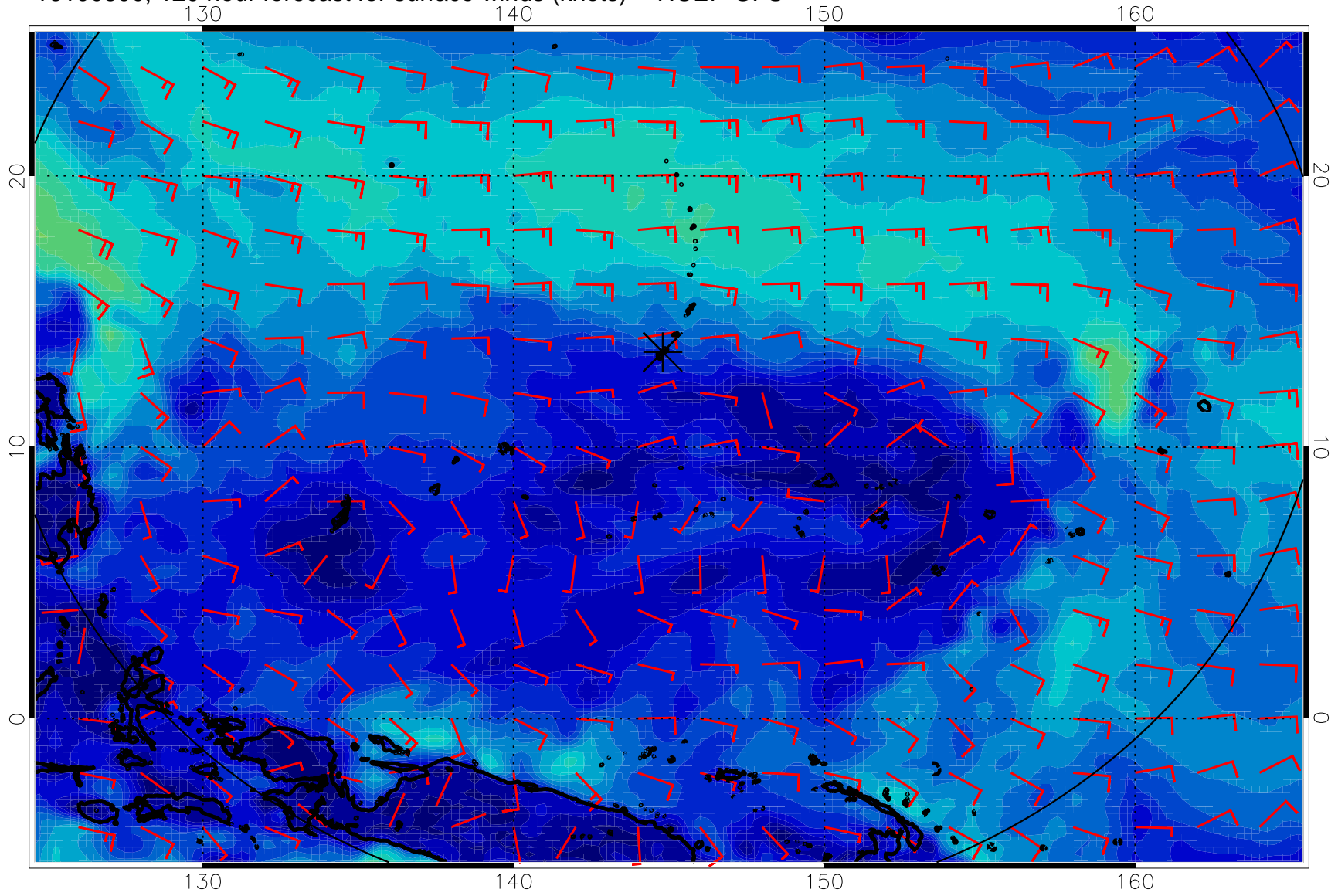
16100800, 120 hour forecast for surface winds (knots) -- NCEP GFS
