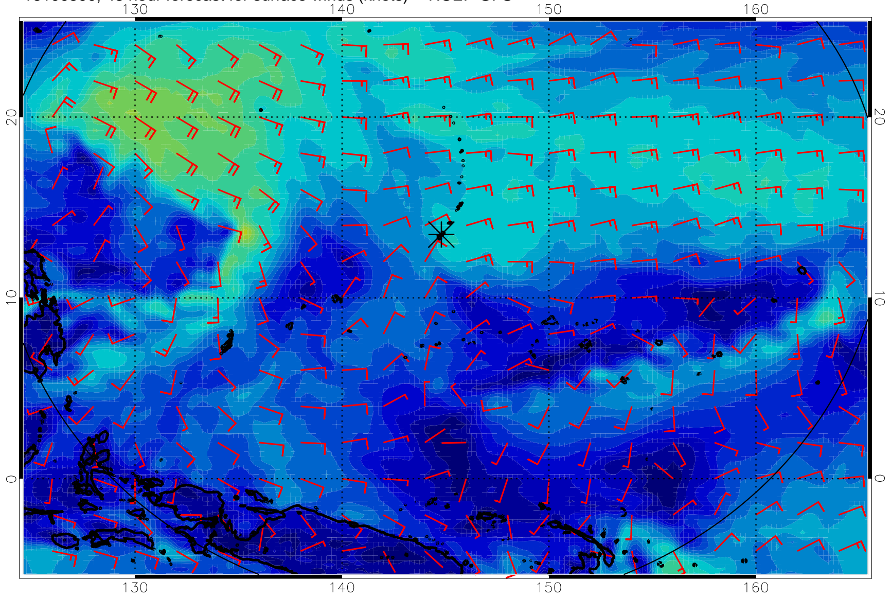
16100500, 48 hour forecast for surface winds (knots) -- NCEP GFS
