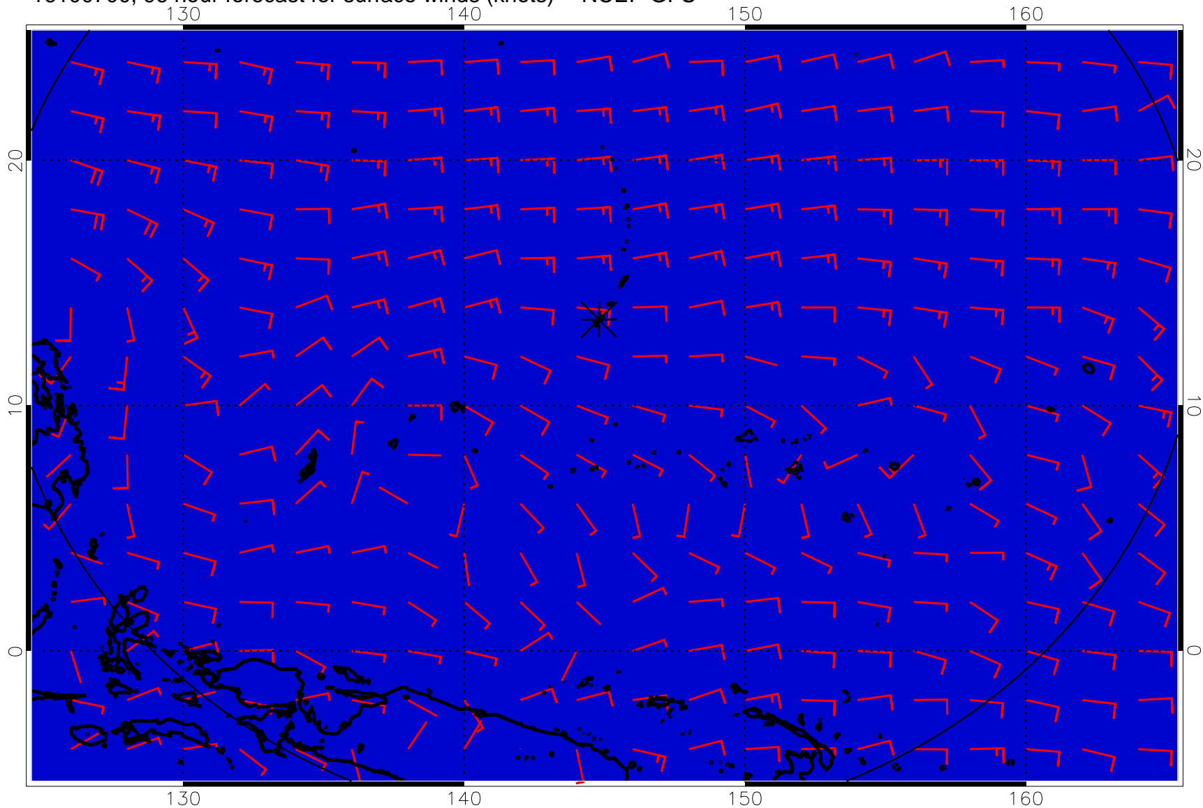
16100700, 96 hour forecast for surface winds (knots) -- NCEP GFS
