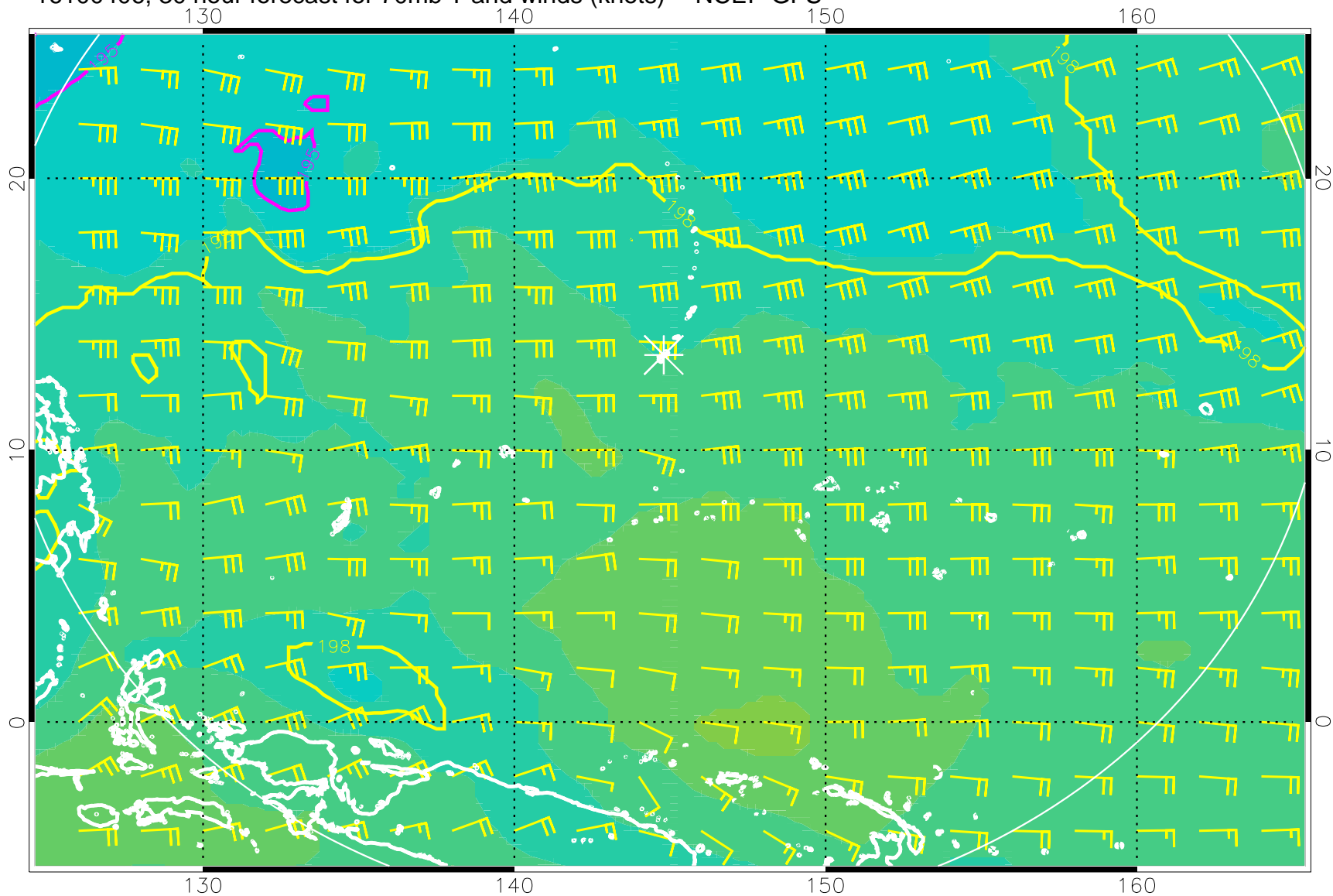
16100406, 30 hour forecast for 70mb T and winds (knots) -- NCEP GFS
