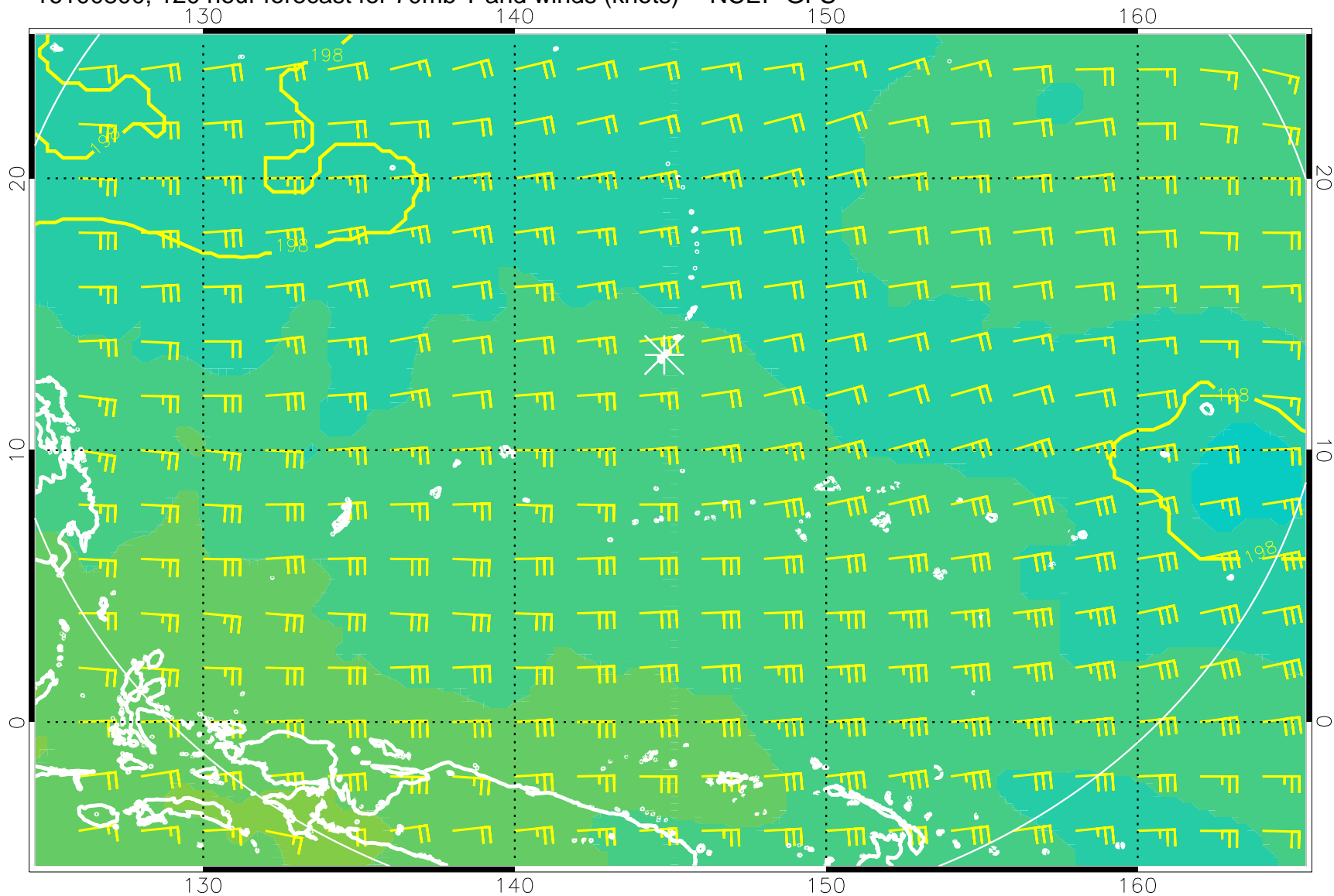
16100800, 120 hour forecast for 70mb T and winds (knots) -- NCEP GFS
