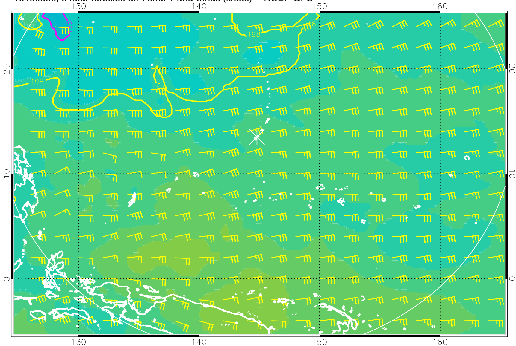
16100306, 6 hour forecast for 70mb T and winds (knots) -- NCEP GFS
