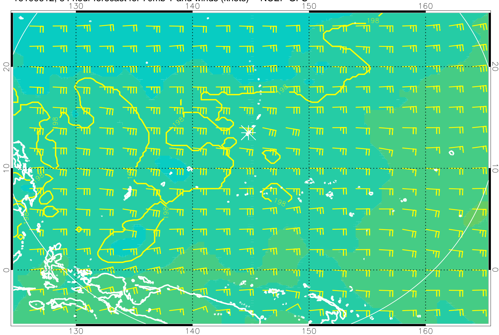
16100612, 84 hour forecast for 70mb T and winds (knots) -- NCEP GFS
