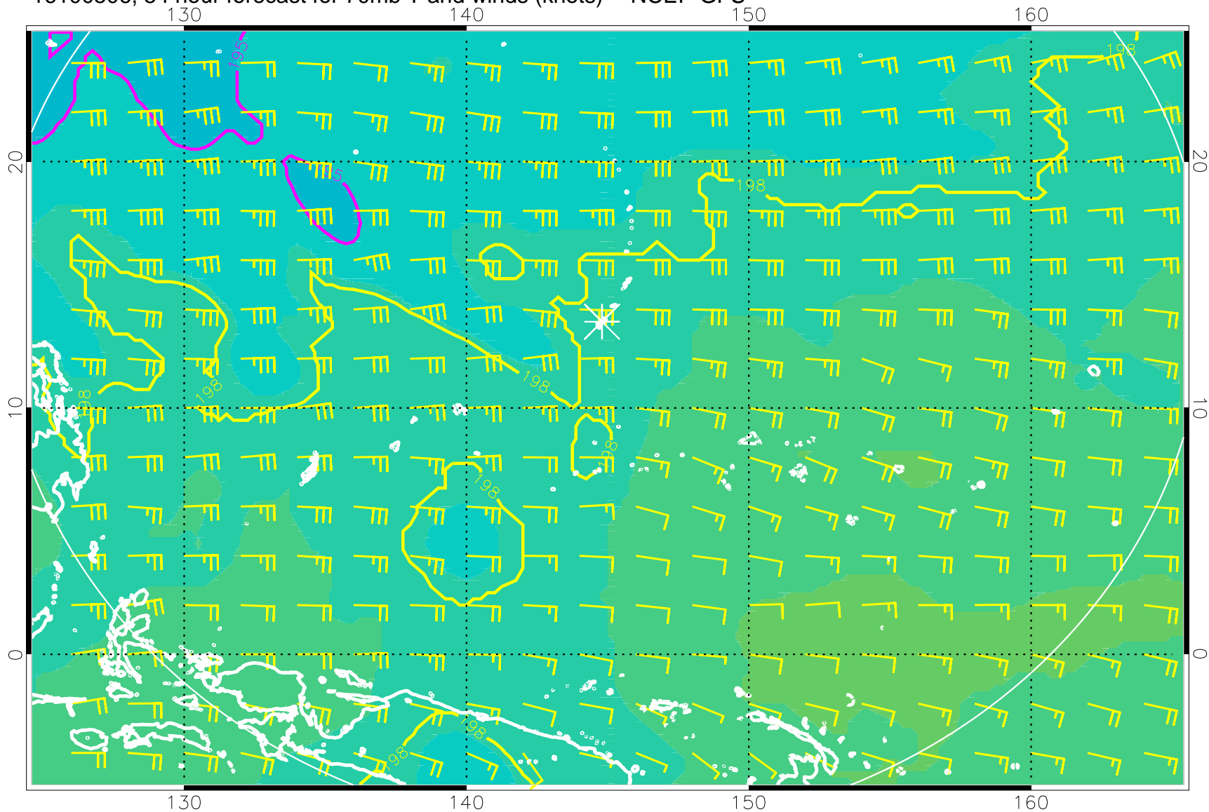
16100506, 54 hour forecast for 70mb T and winds (knots) -- NCEP GFS
