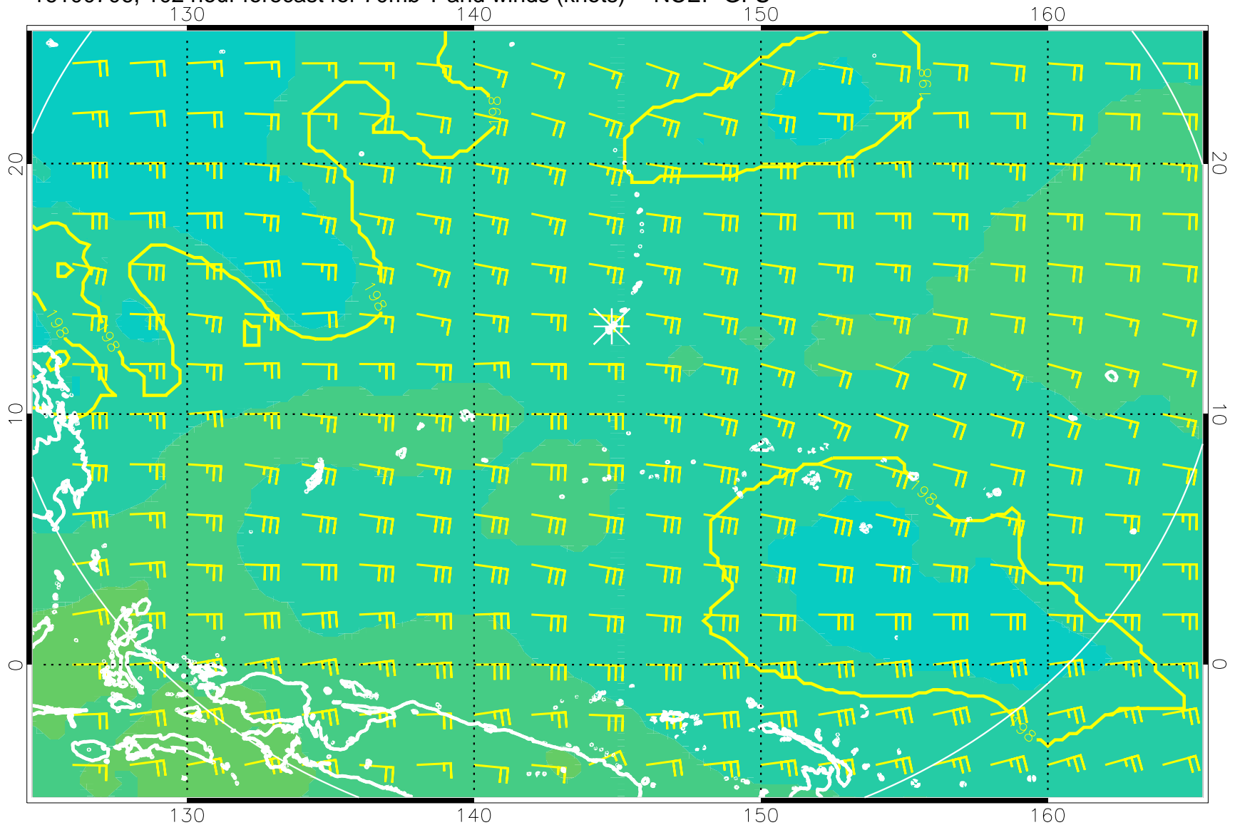
16100706, 102 hour forecast for 70mb T and winds (knots) -- NCEP GFS
