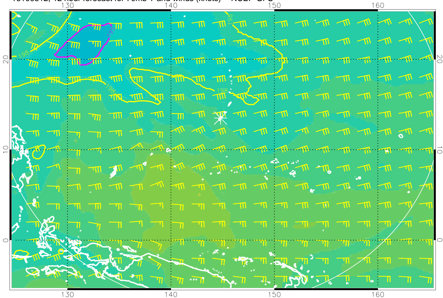
16100312, 12 hour forecast for 70mb T and winds (knots) -- NCEP GFS
