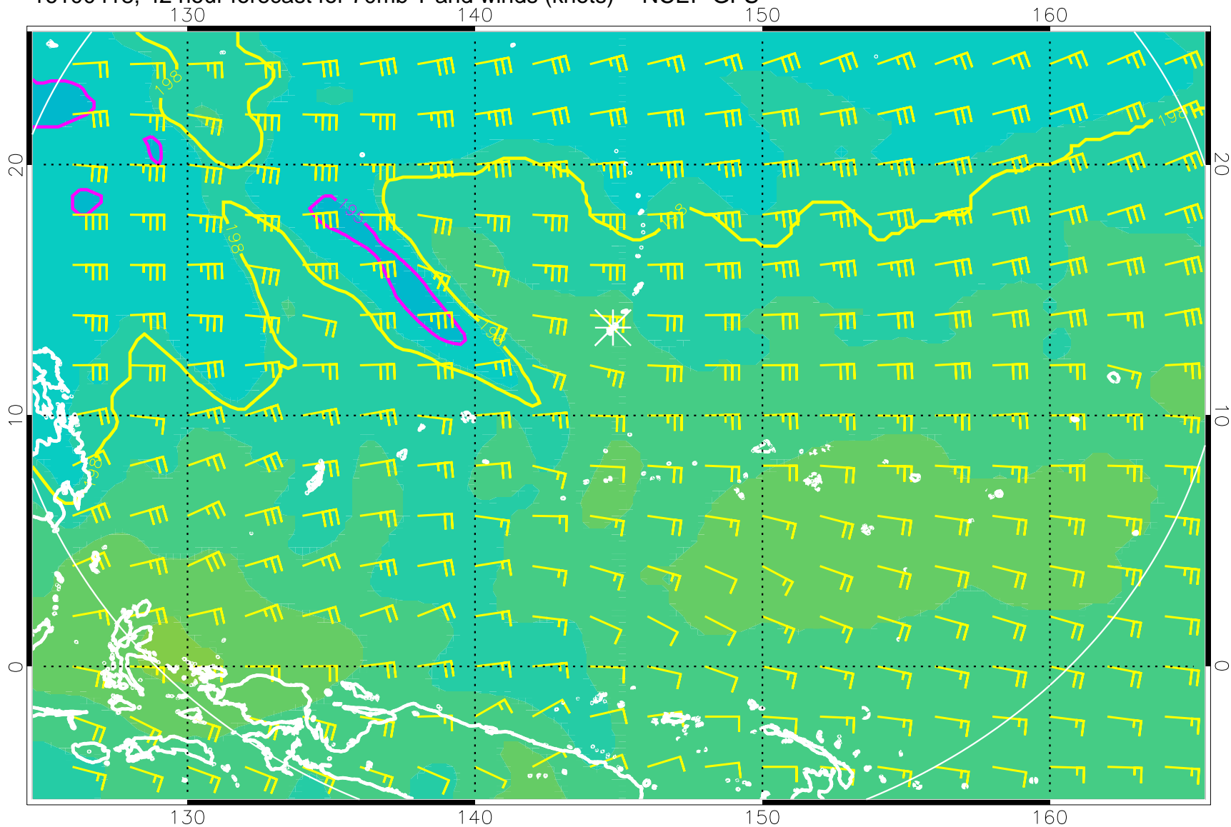
16100418, 42 hour forecast for 70mb T and winds (knots) -- NCEP GFS
