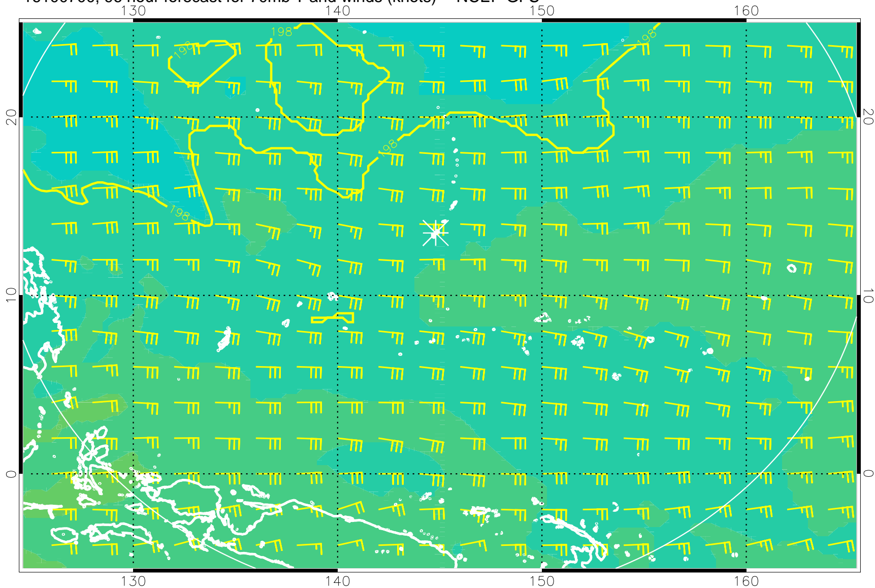
16100700, 96 hour forecast for 70mb T and winds (knots) -- NCEP GFS
