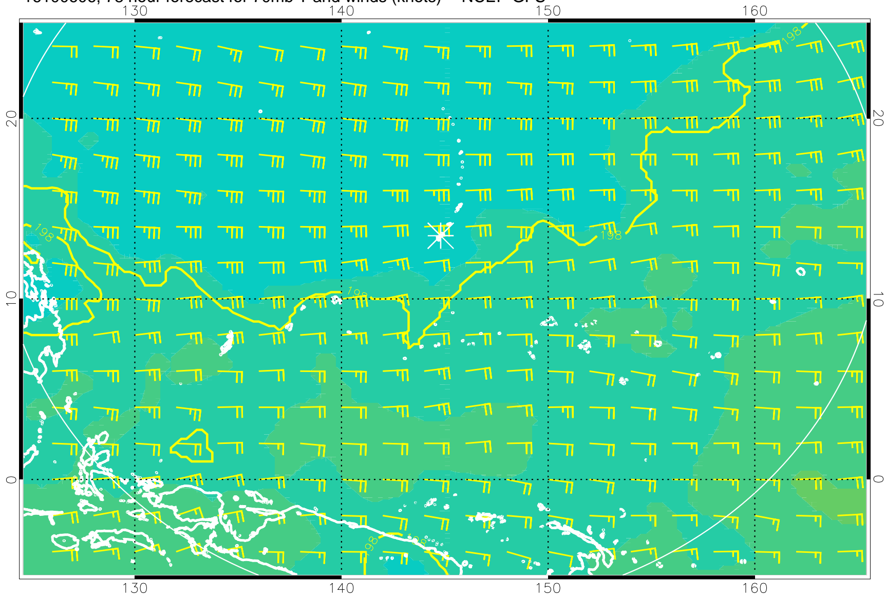
16100606, 78 hour forecast for 70mb T and winds (knots) -- NCEP GFS
