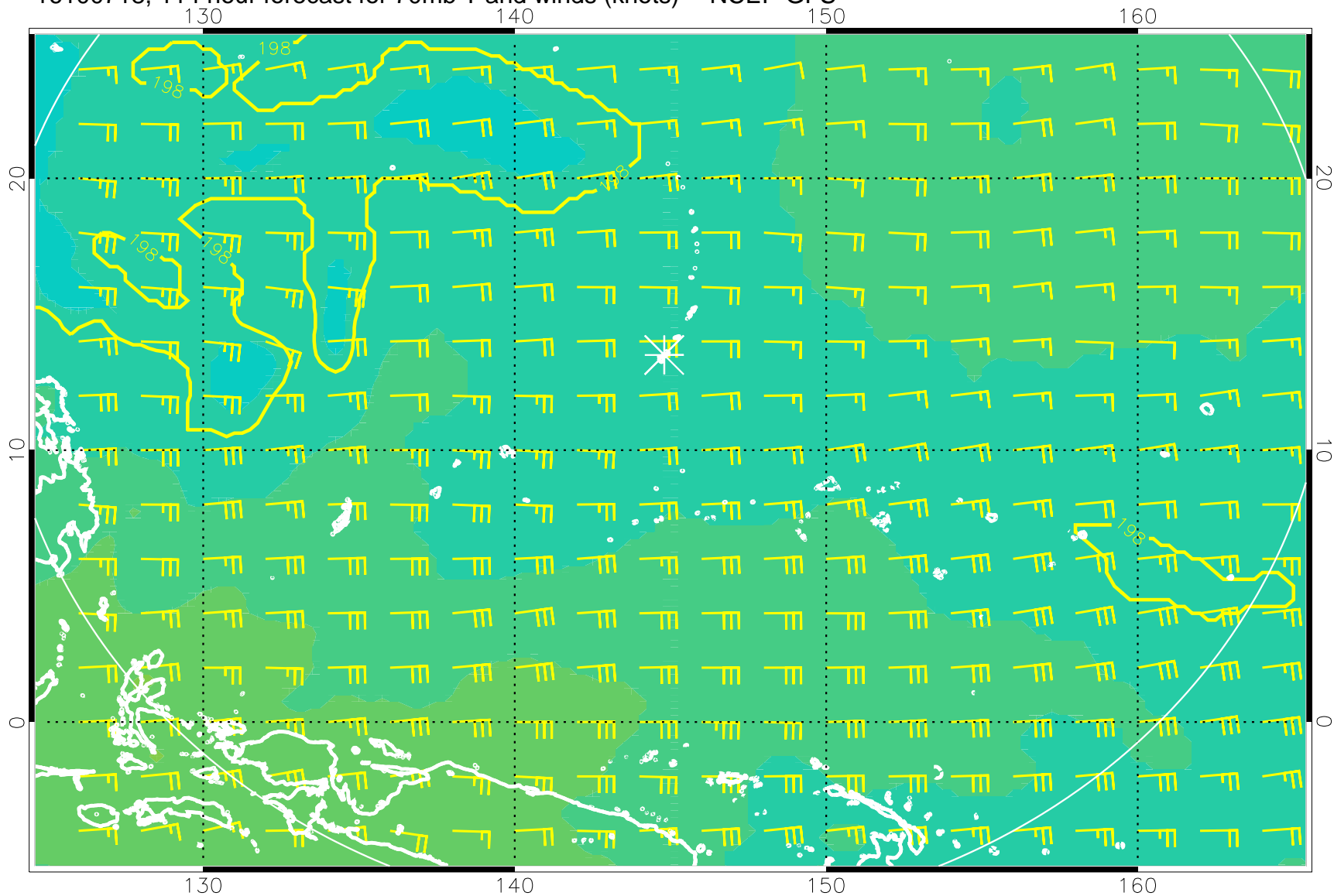
16100718, 114 hour forecast for 70mb T and winds (knots) -- NCEP GFS
