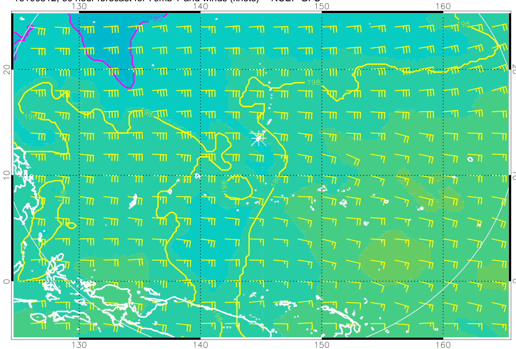
16100512, 60 hour forecast for 70mb T and winds (knots) -- NCEP GFS
