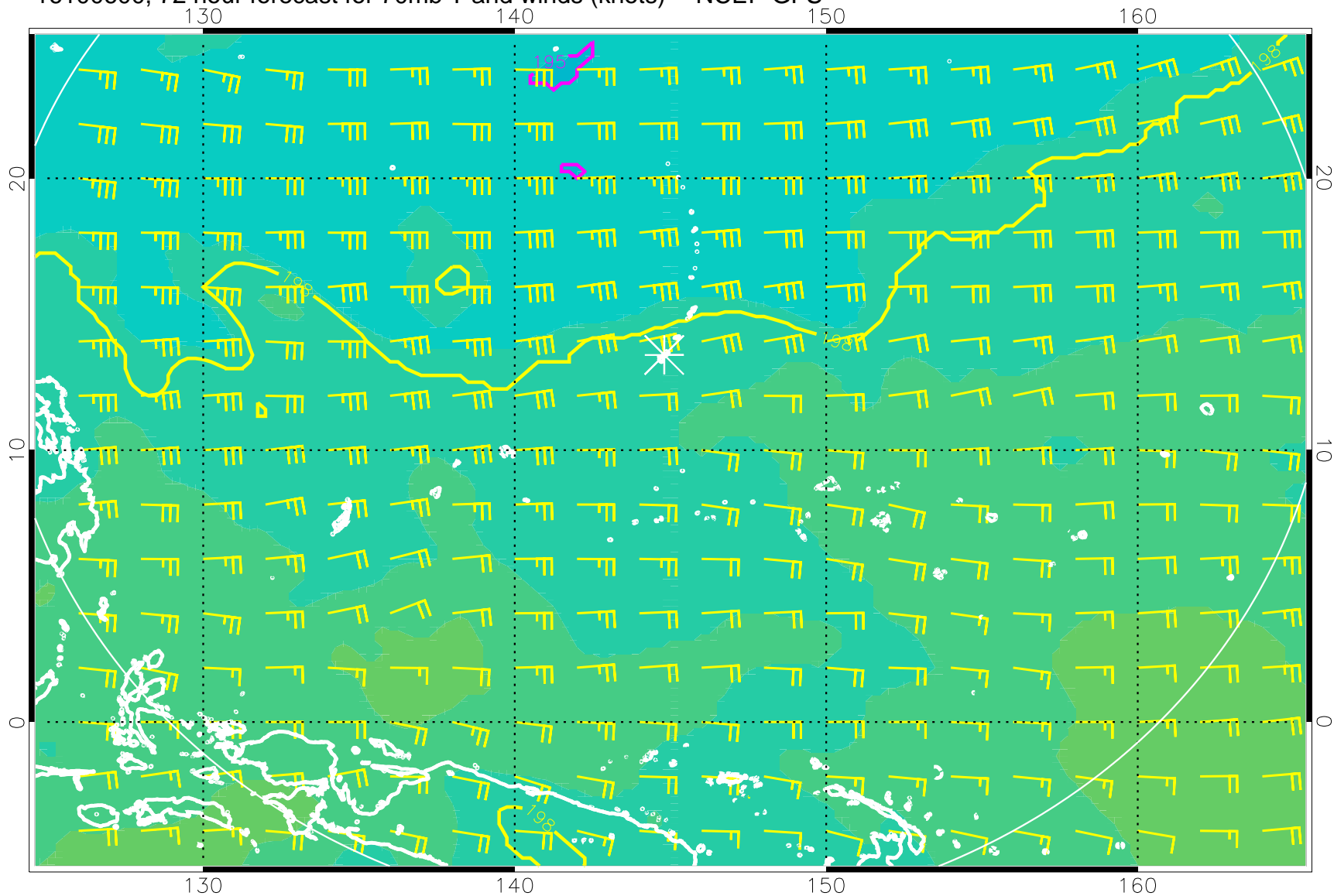
16100600, 72 hour forecast for 70mb T and winds (knots) -- NCEP GFS
