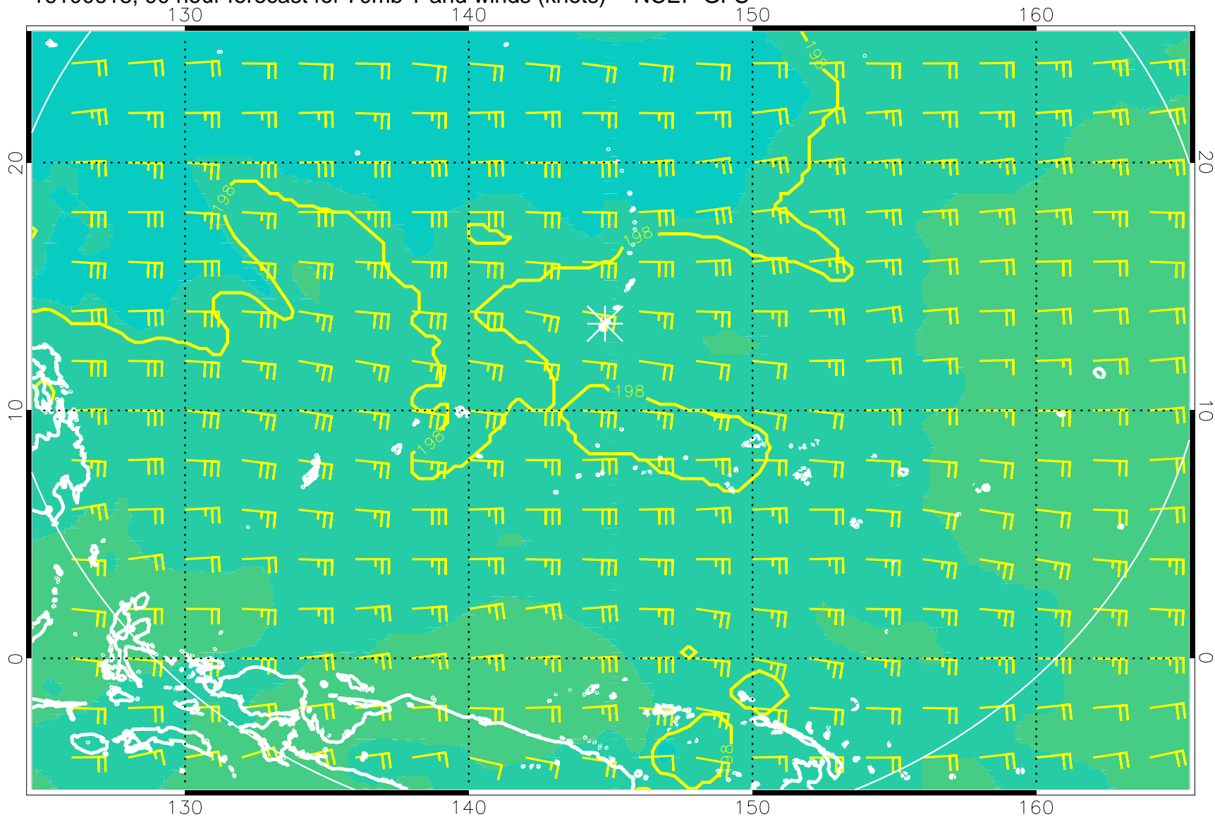
16100618, 90 hour forecast for 70mb T and winds (knots) -- NCEP GFS
