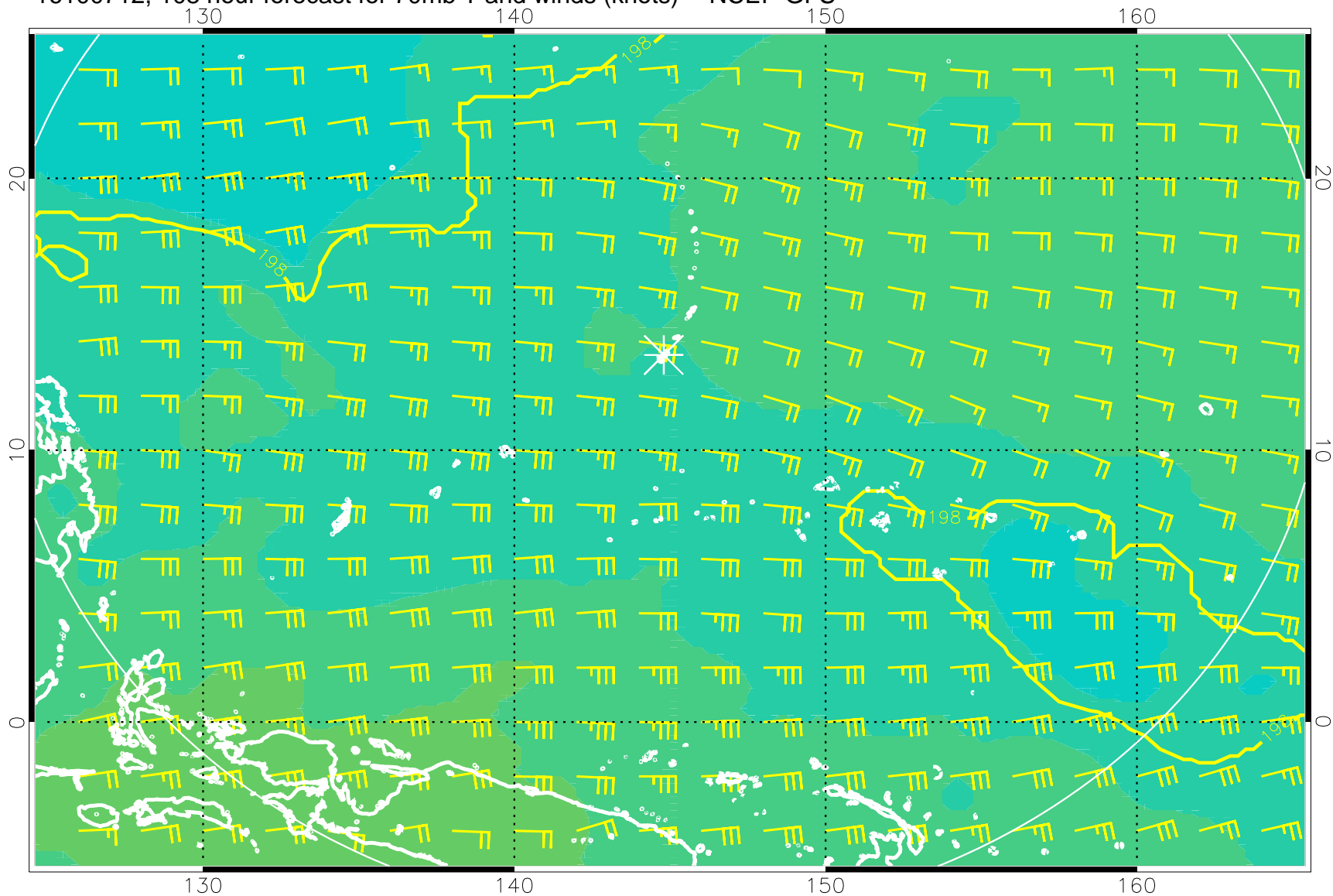
16100712, 108 hour forecast for 70mb T and winds (knots) -- NCEP GFS
