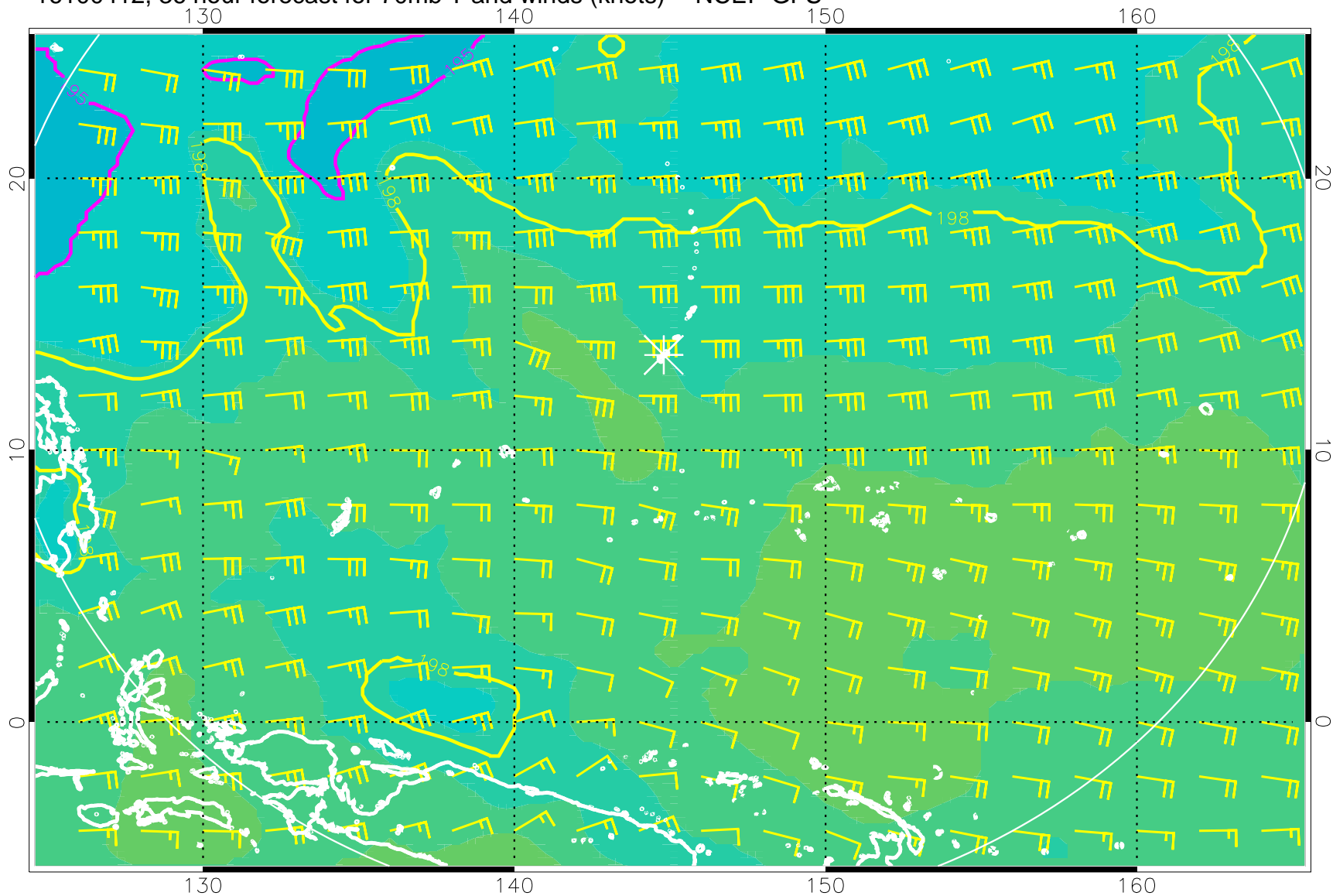
16100412, 36 hour forecast for 70mb T and winds (knots) -- NCEP GFS
