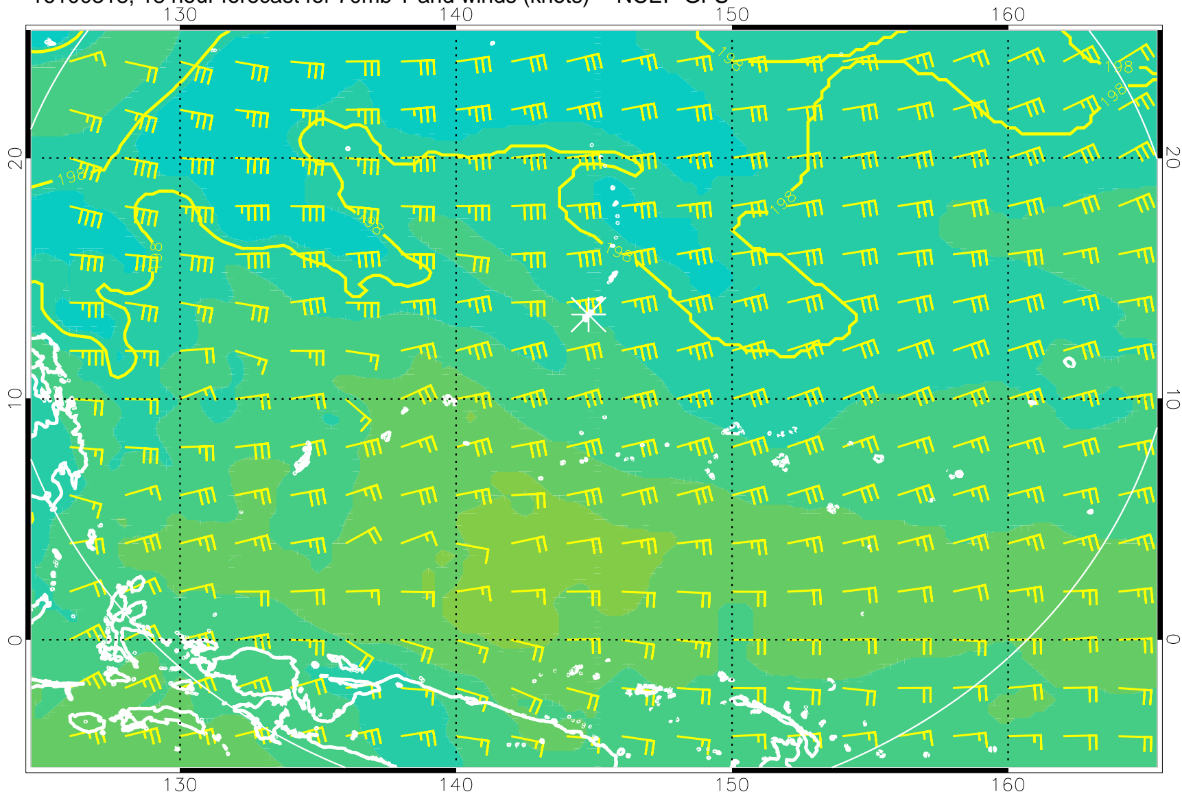
16100318, 18 hour forecast for 70mb T and winds (knots) -- NCEP GFS
