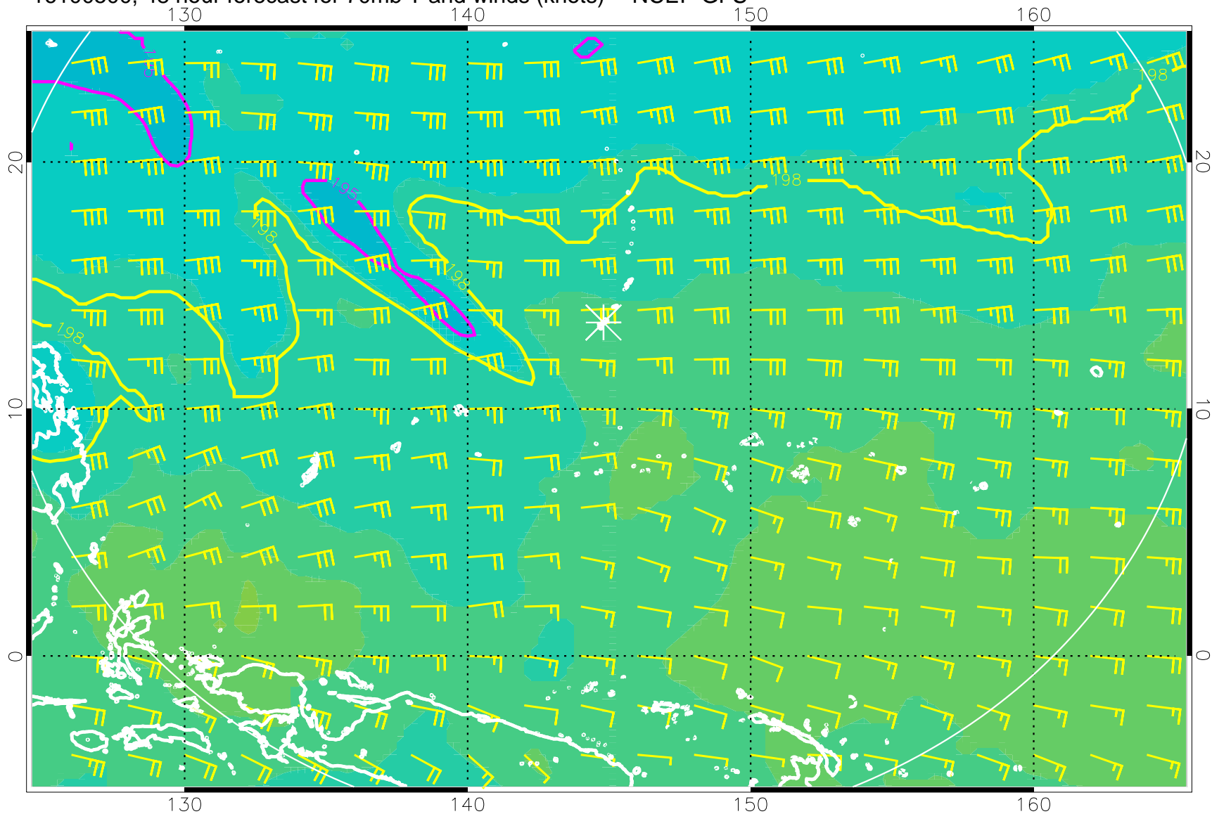
16100500, 48 hour forecast for 70mb T and winds (knots) -- NCEP GFS
