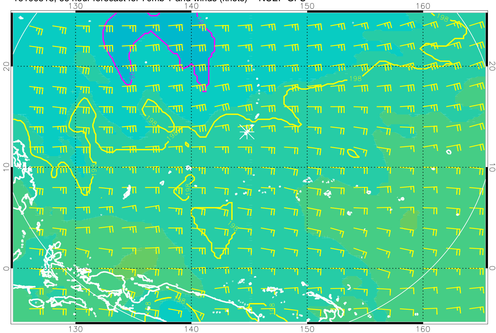
16100518, 66 hour forecast for 70mb T and winds (knots) -- NCEP GFS
