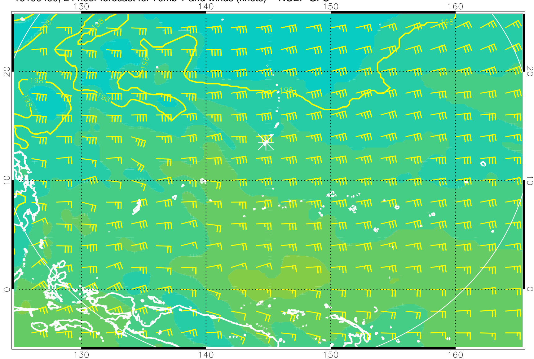
16100400, 24 hour forecast for 70mb T and winds (knots) -- NCEP GFS
