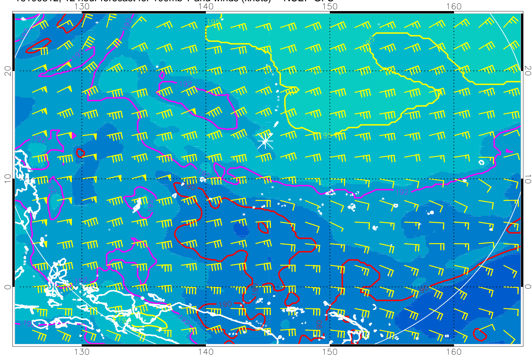
16100312, 12 hour forecast for 100mb T and winds (knots) -- NCEP GFS
