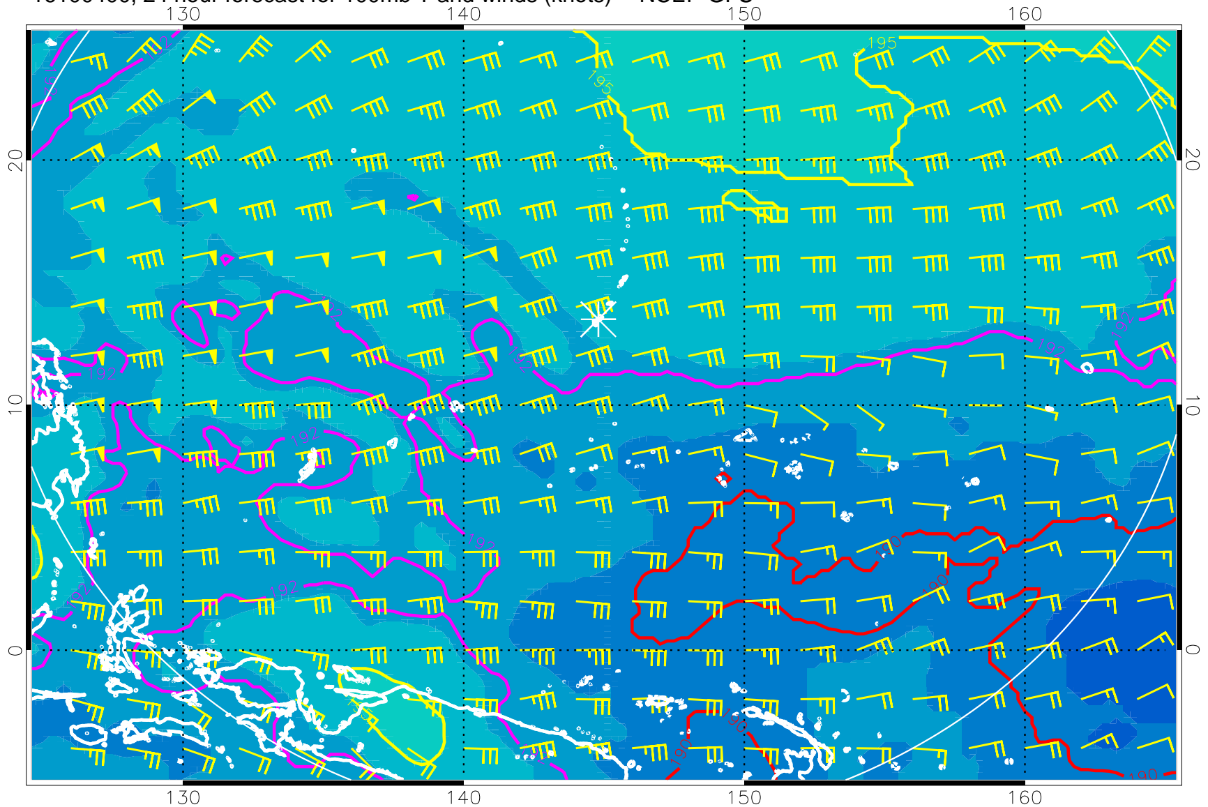
16100400, 24 hour forecast for 100mb T and winds (knots) -- NCEP GFS
