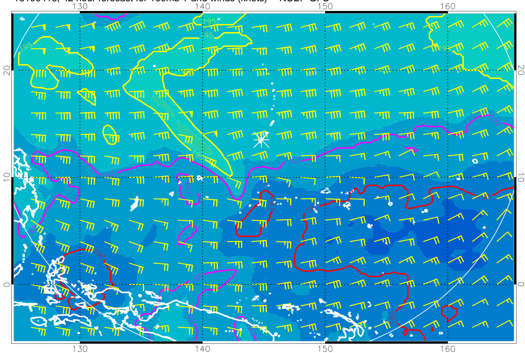
16100418, 42 hour forecast for 100mb T and winds (knots) -- NCEP GFS
