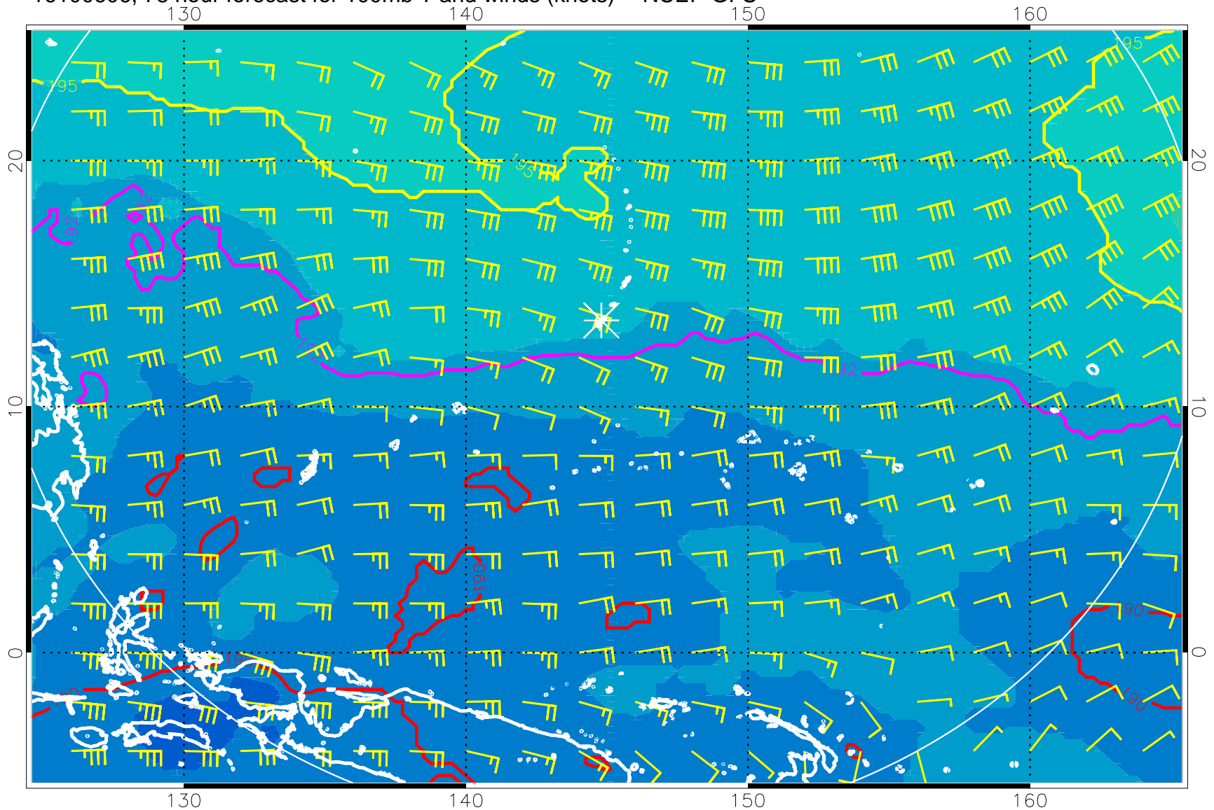
16100606, 78 hour forecast for 100mb T and winds (knots) -- NCEP GFS
