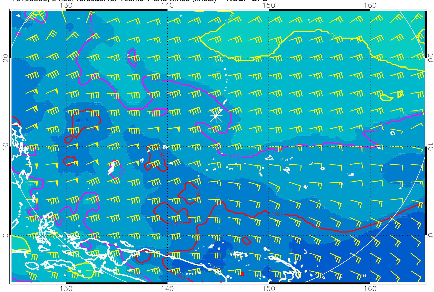
16100306, 6 hour forecast for 100mb T and winds (knots) -- NCEP GFS
