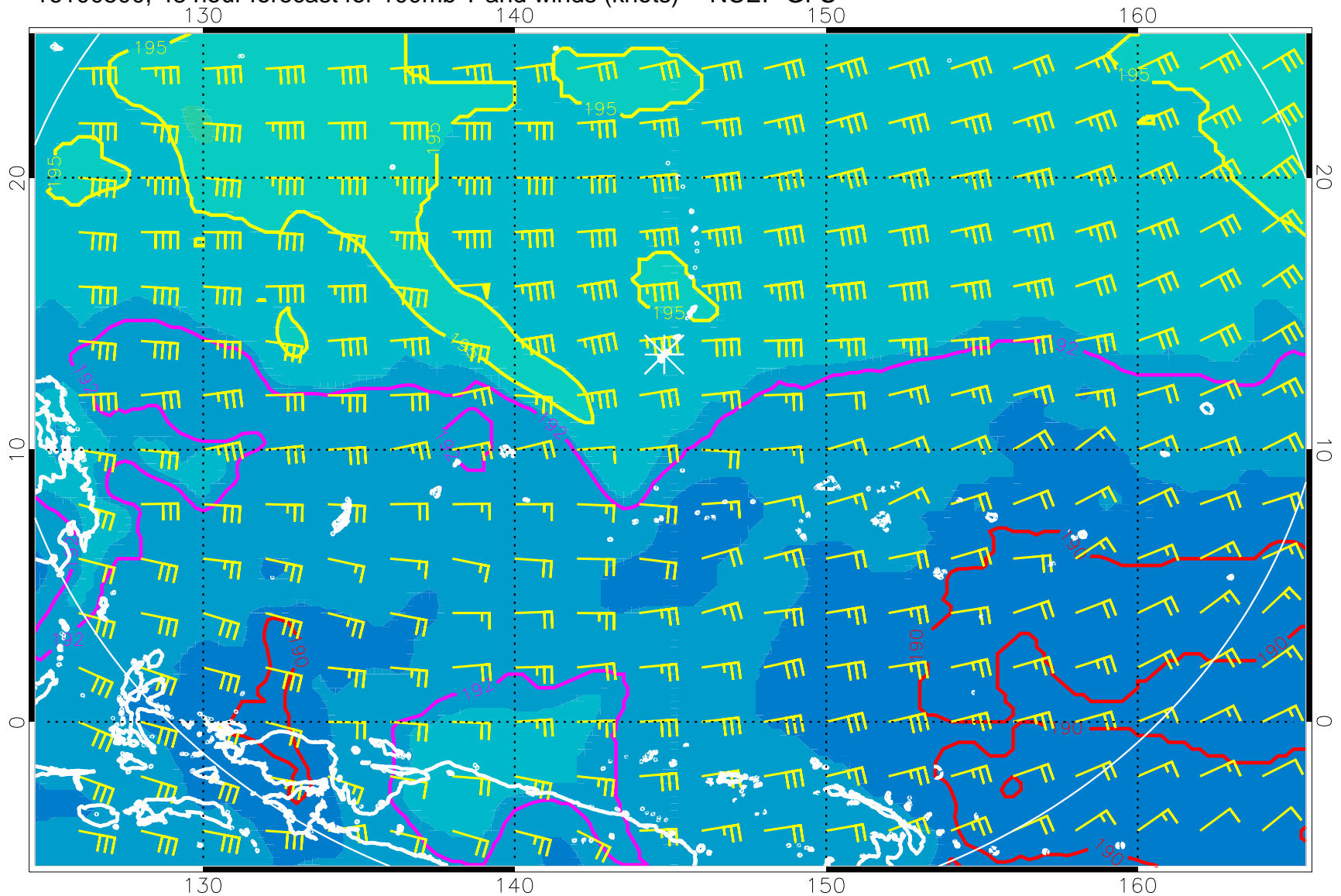
16100500, 48 hour forecast for 100mb T and winds (knots) -- NCEP GFS
