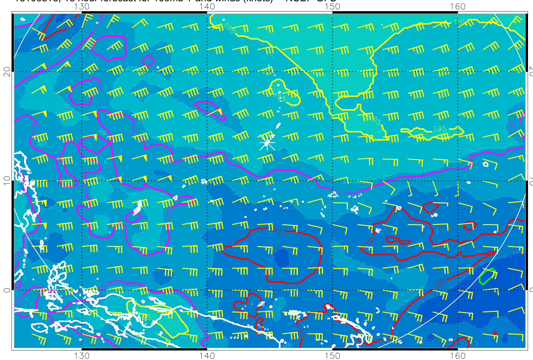
16100318, 18 hour forecast for 100mb T and winds (knots) -- NCEP GFS
