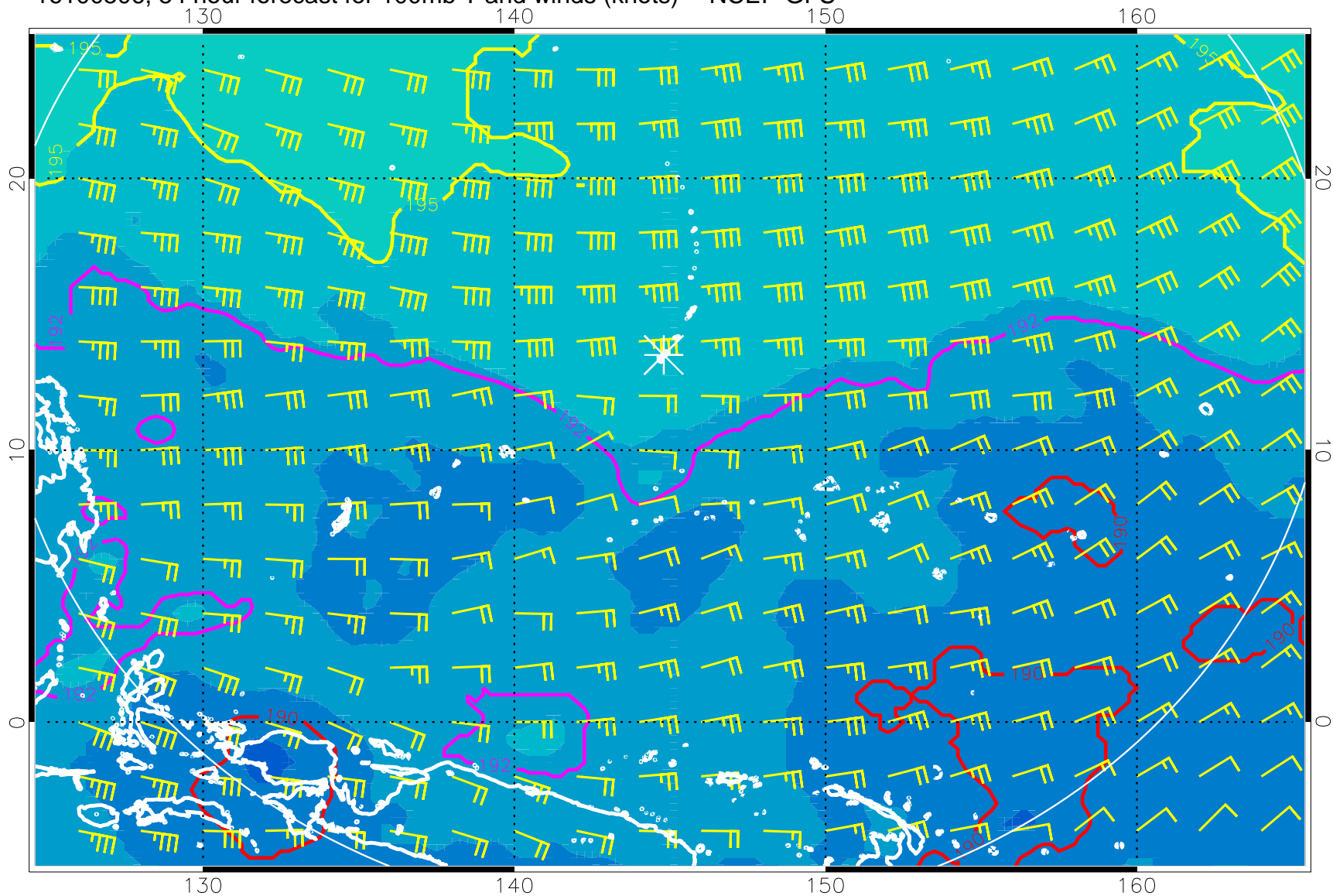
16100506, 54 hour forecast for 100mb T and winds (knots) -- NCEP GFS
