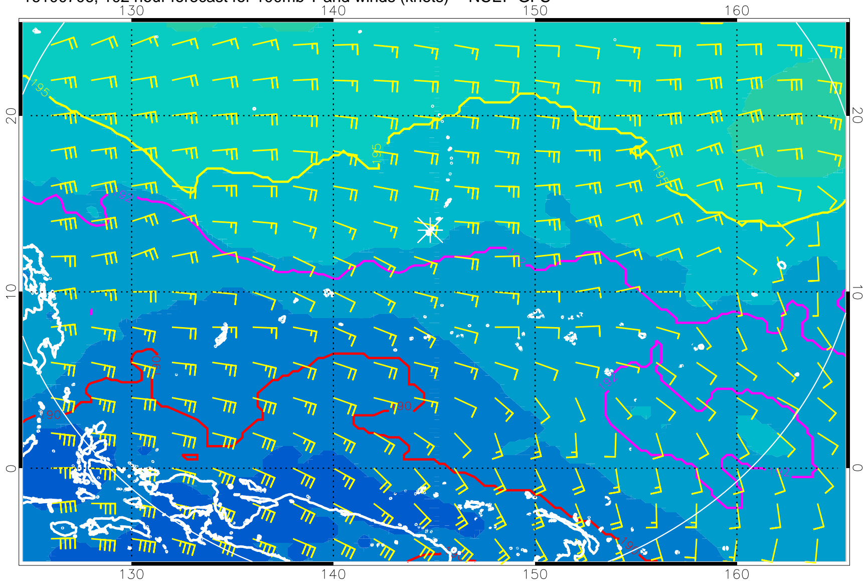
16100706, 102 hour forecast for 100mb T and winds (knots) -- NCEP GFS
