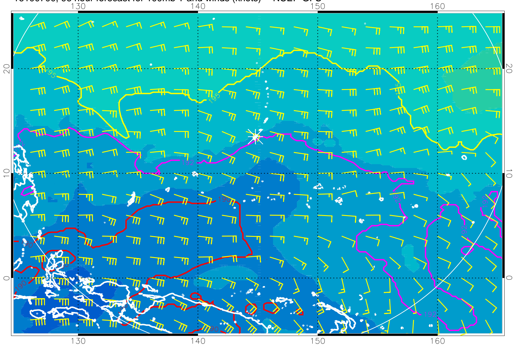
16100700, 96 hour forecast for 100mb T and winds (knots) -- NCEP GFS
