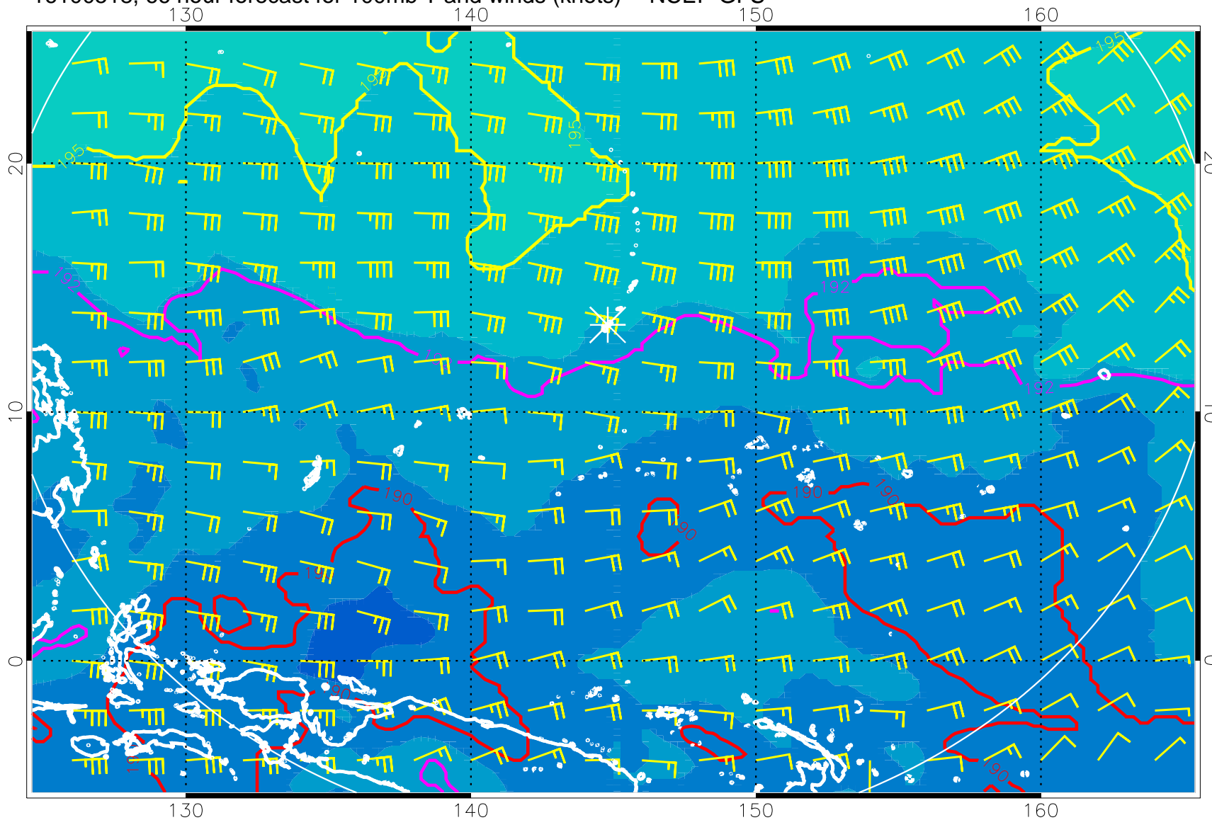
16100518, 66 hour forecast for 100mb T and winds (knots) -- NCEP GFS
