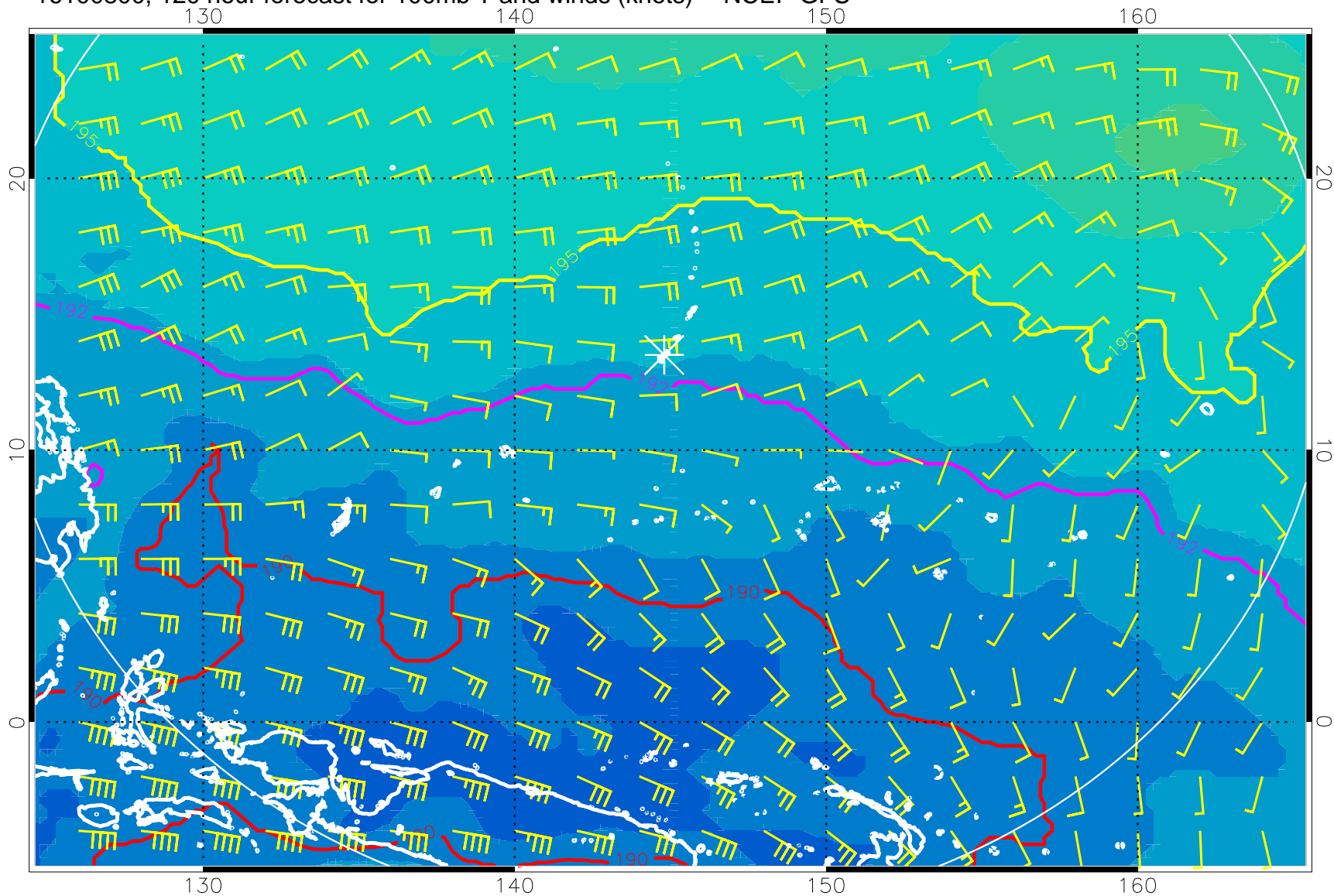
16100800, 120 hour forecast for 100mb T and winds (knots) -- NCEP GFS
