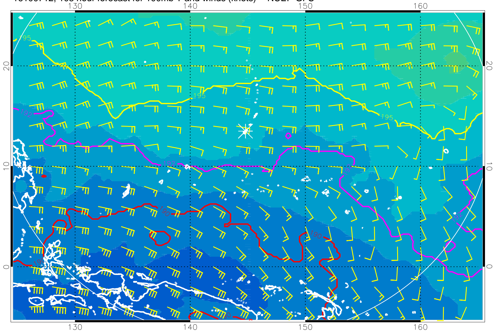
16100712, 108 hour forecast for 100mb T and winds (knots) -- NCEP GFS
