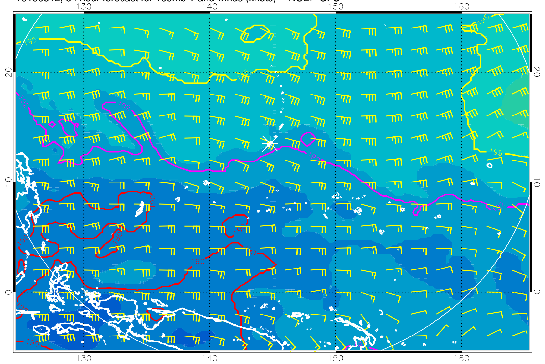
16100612, 84 hour forecast for 100mb T and winds (knots) -- NCEP GFS
