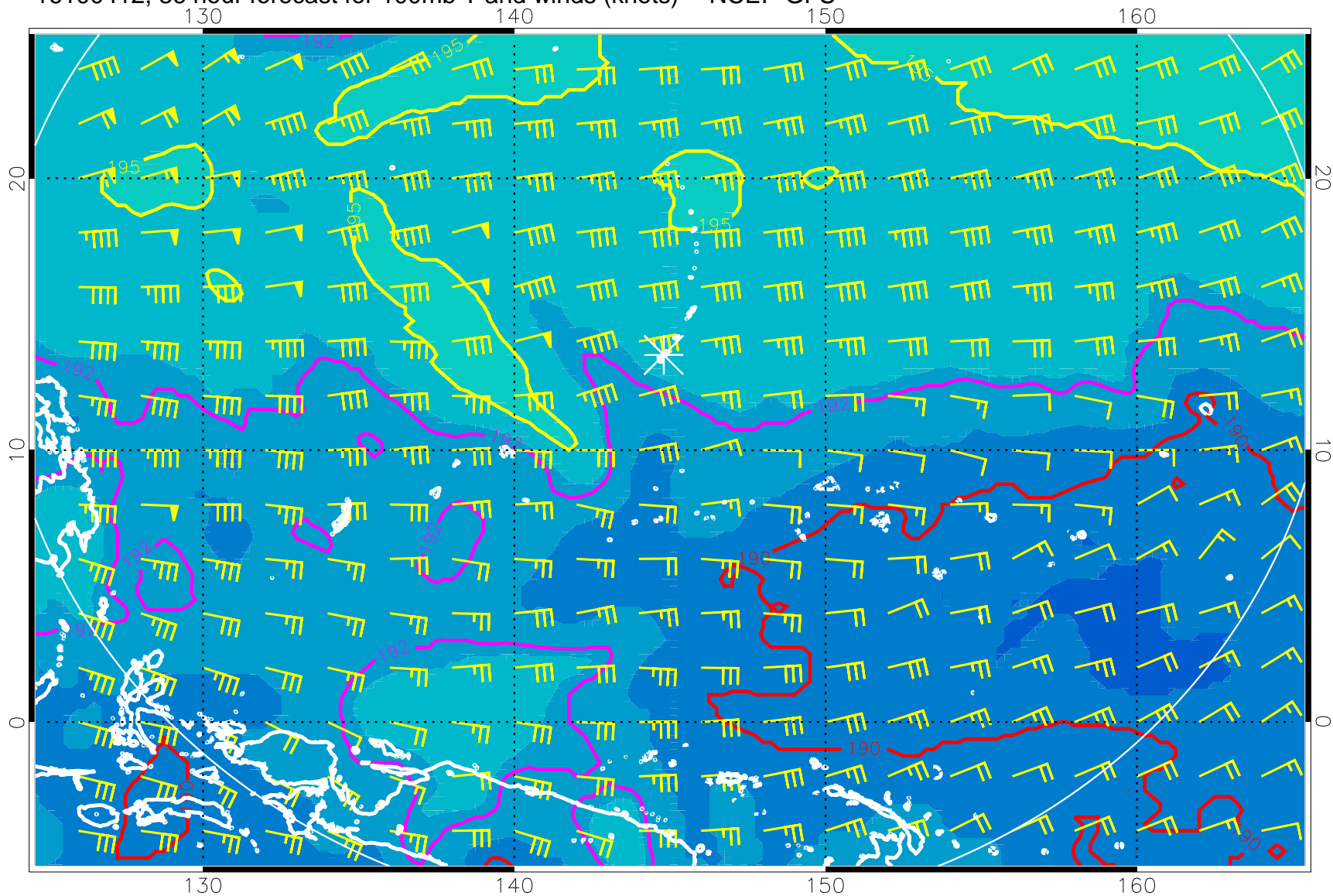
16100412, 36 hour forecast for 100mb T and winds (knots) -- NCEP GFS
