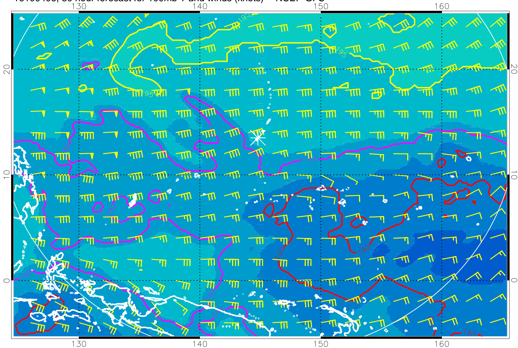
16100406, 30 hour forecast for 100mb T and winds (knots) -- NCEP GFS
