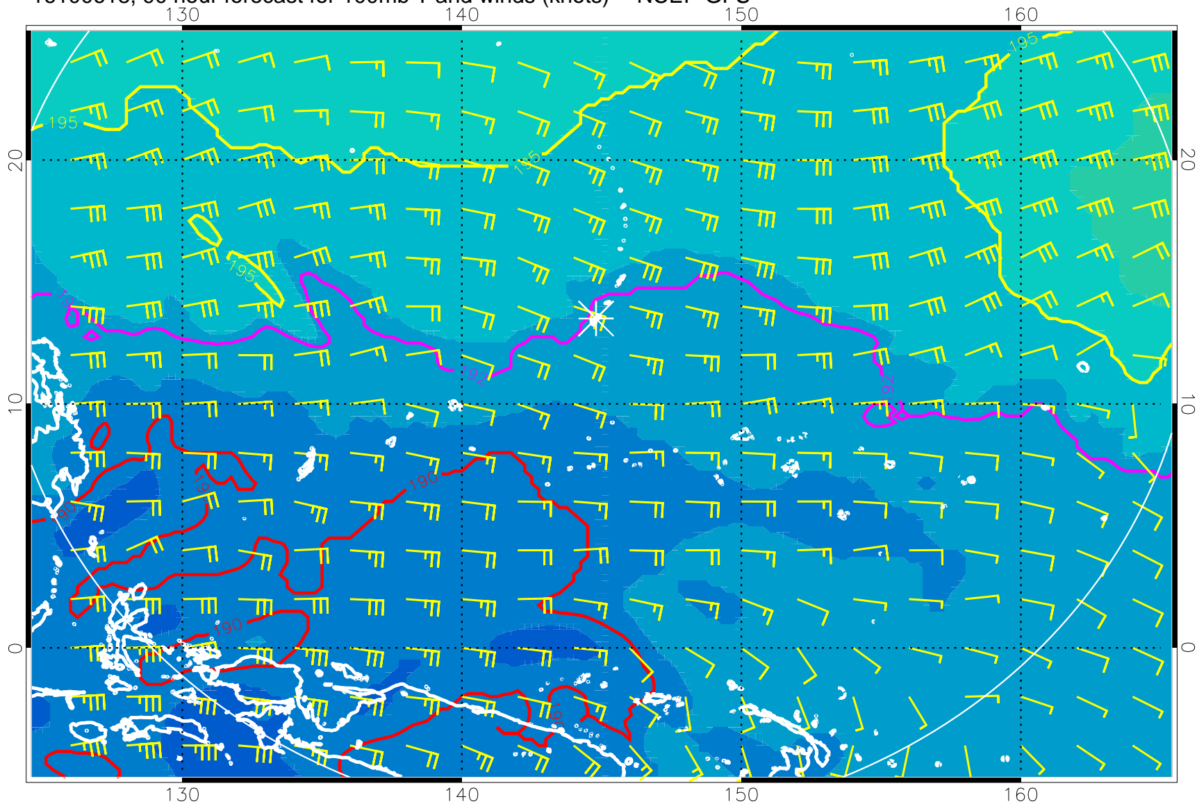
16100618, 90 hour forecast for 100mb T and winds (knots) -- NCEP GFS
