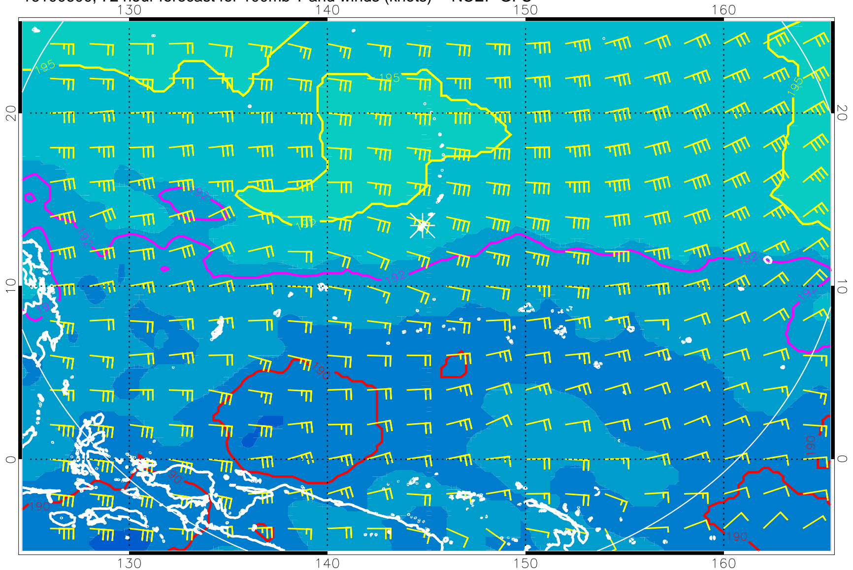
16100600, 72 hour forecast for 100mb T and winds (knots) -- NCEP GFS
