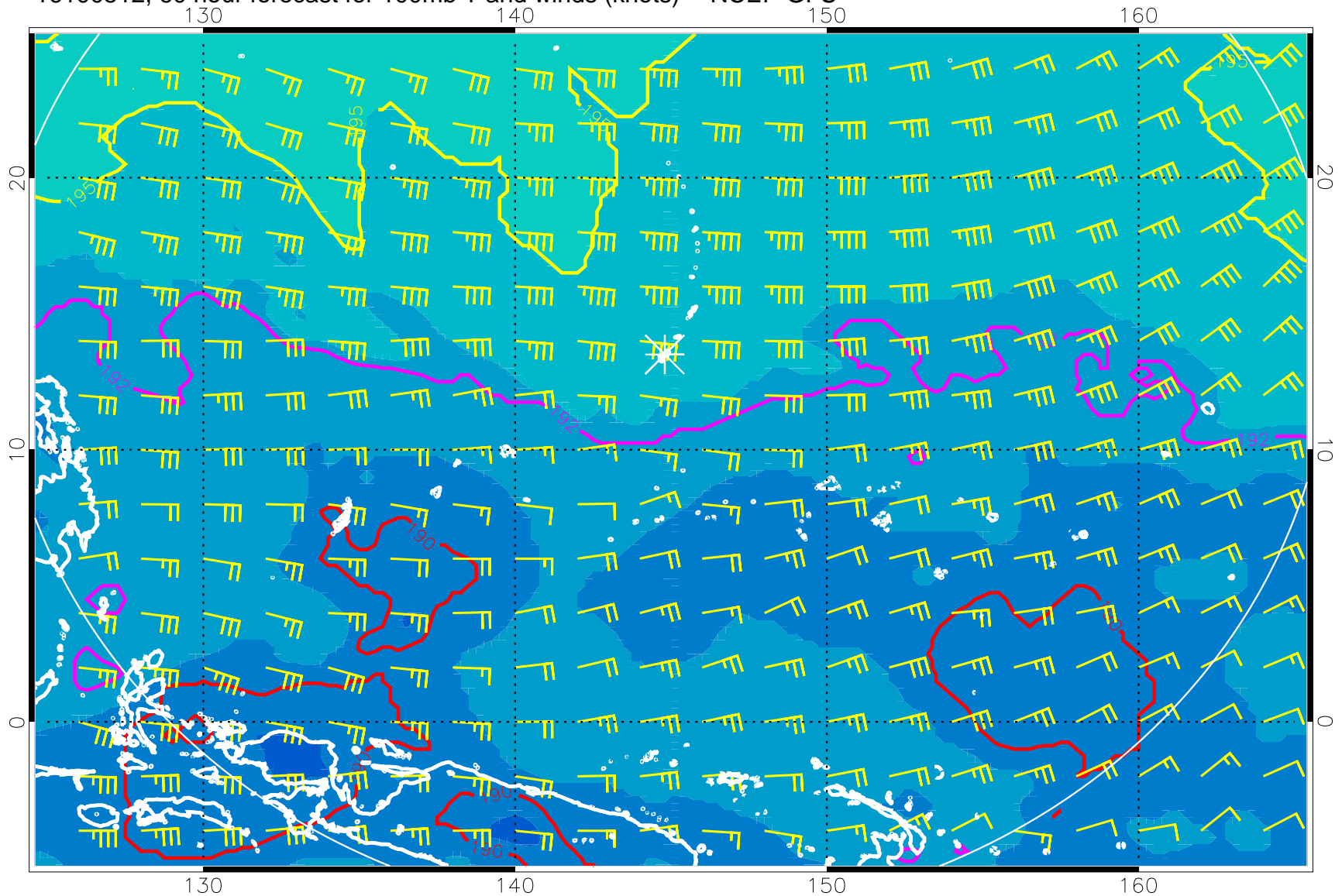
16100512, 60 hour forecast for 100mb T and winds (knots) -- NCEP GFS
