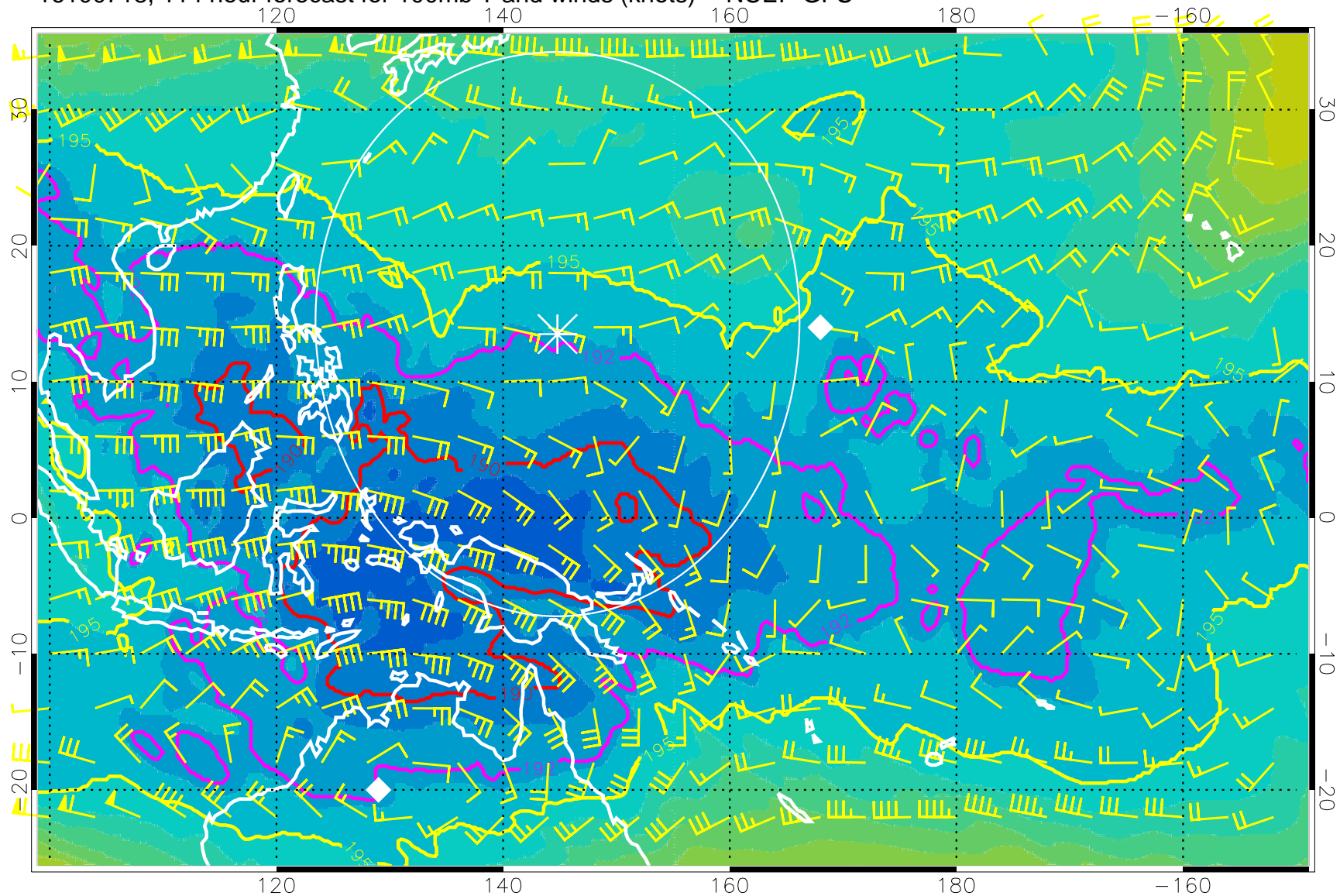
16100718, 114 hour forecast for 100mb T and winds (knots) -- NCEP GFS
