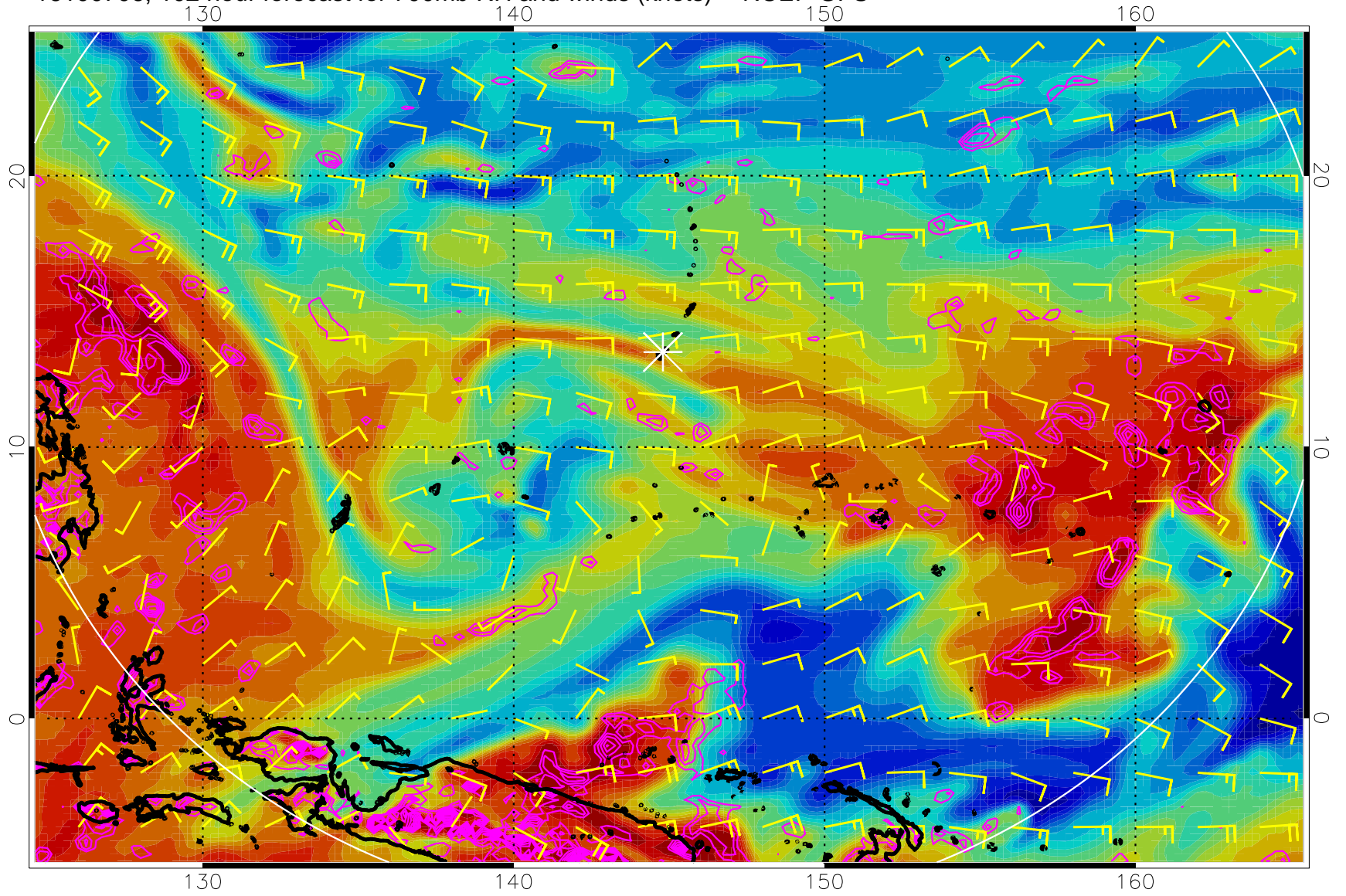
16100706, 102 hour forecast for 700mb RH and winds (knots) -- NCEP GFS
