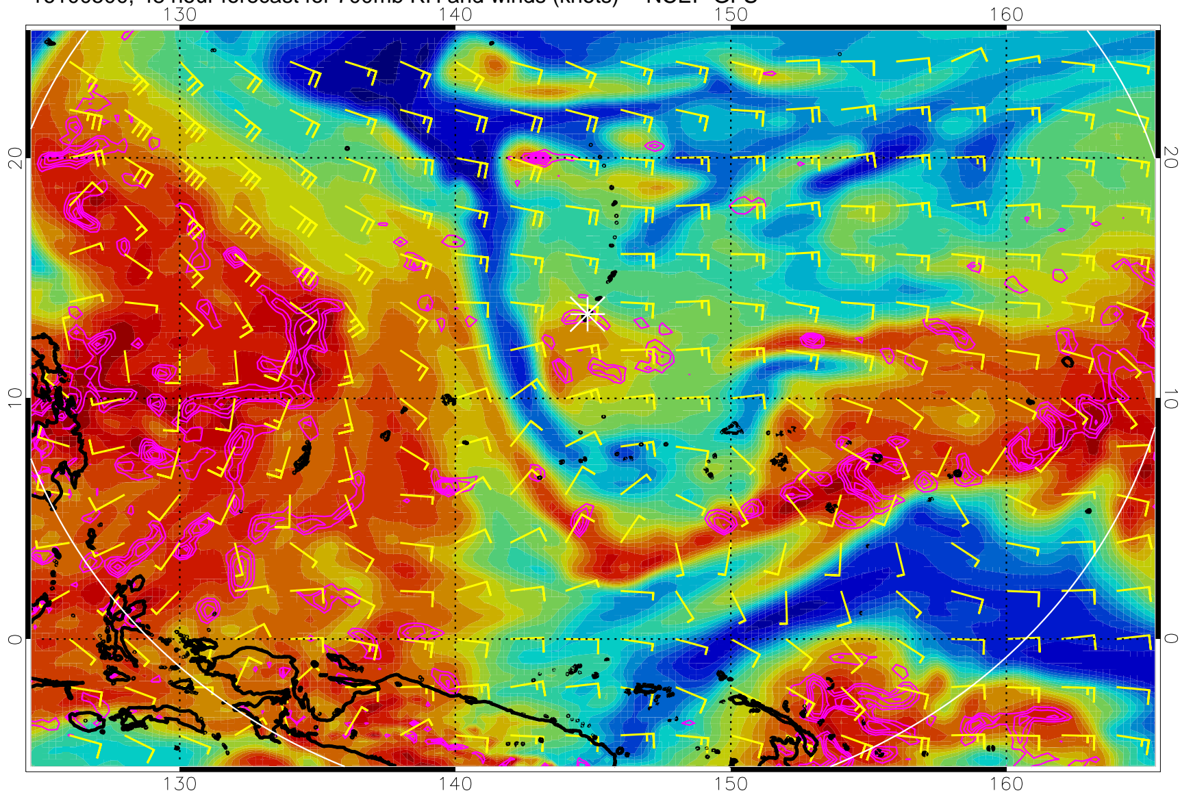
16100500, 48 hour forecast for 700mb RH and winds (knots) -- NCEP GFS
