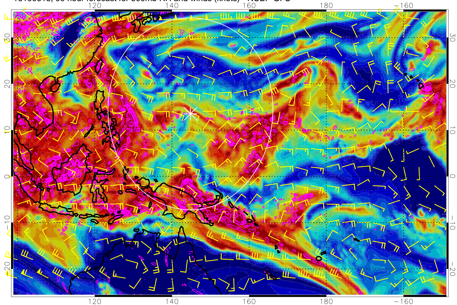
16100618, 90 hour forecast for 500mb RH and winds (knots) - NCEP GFS
