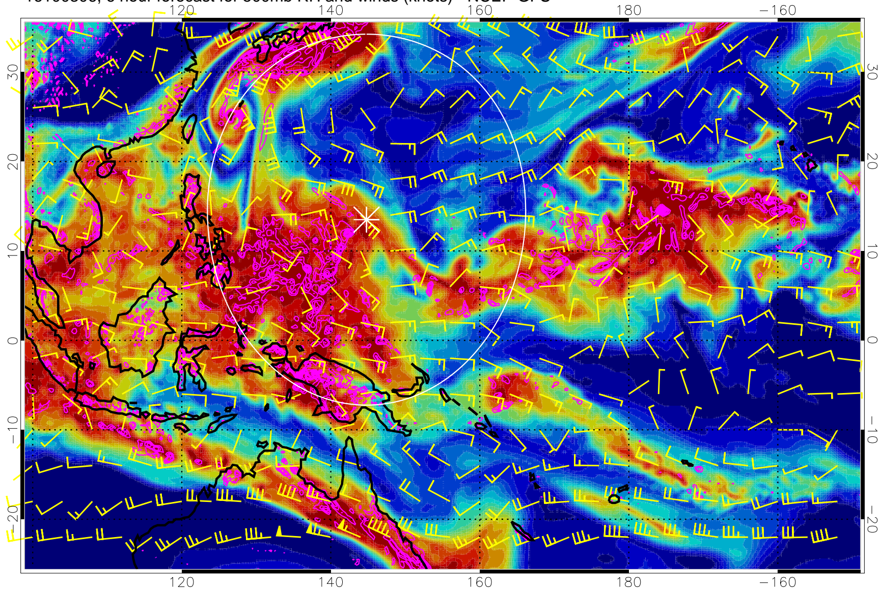
16100306, 6 hour forecast for 500mb RH and winds (knots) - NCEP GFS
