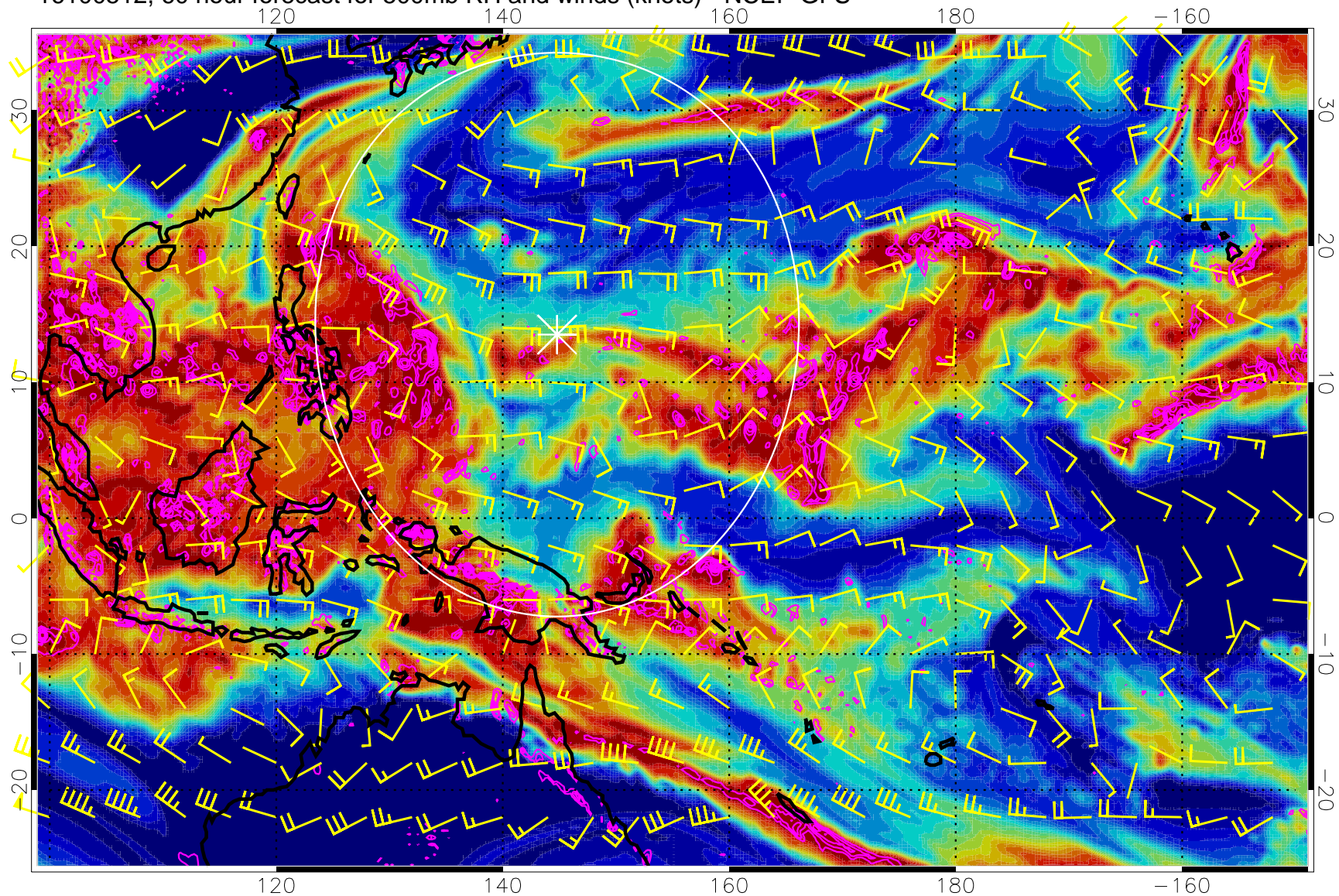
16100512, 60 hour forecast for 500mb RH and winds (knots) - NCEP GFS
