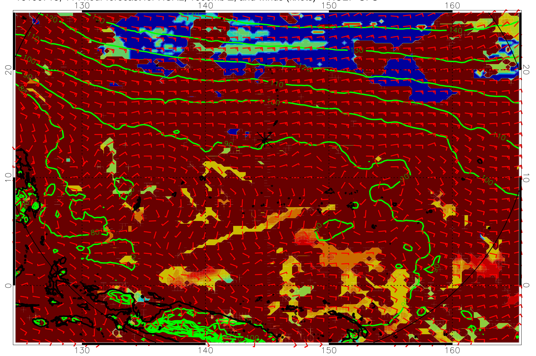
16100718, 114 hour forecast for HCAL, 1000mb Z, and winds (knots) -- NCEP GFS
