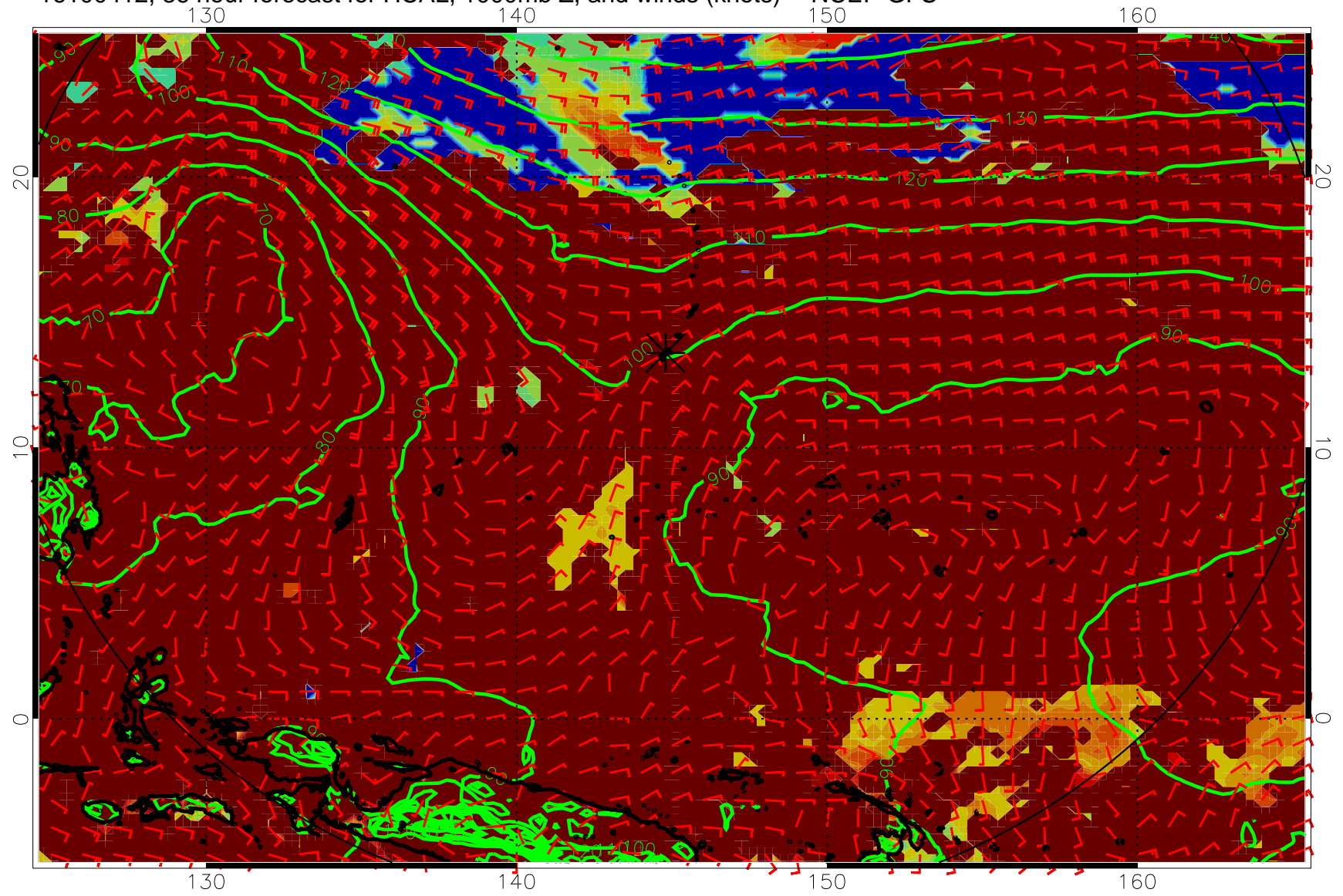
16100412, 36 hour forecast for HCAL, 1000mb Z, and winds (knots) -- NCEP GFS
