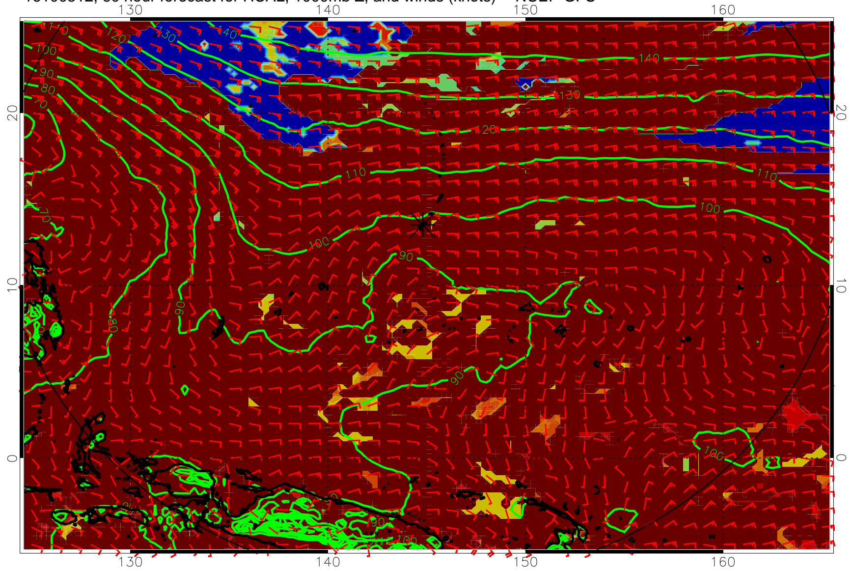
16100512, 60 hour forecast for HCAL, 1000mb Z, and winds (knots) -- NCEP GFS
