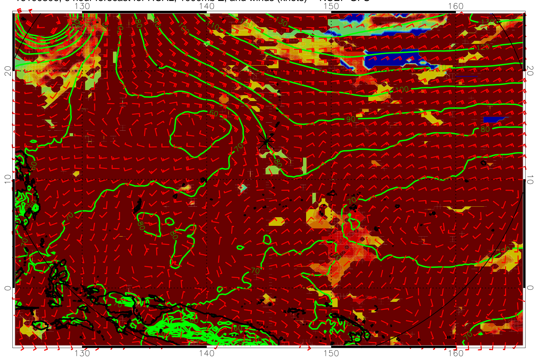
16100306, 6 hour forecast for HCAL, 1000mb Z, and winds (knots) -- NCEP GFS
