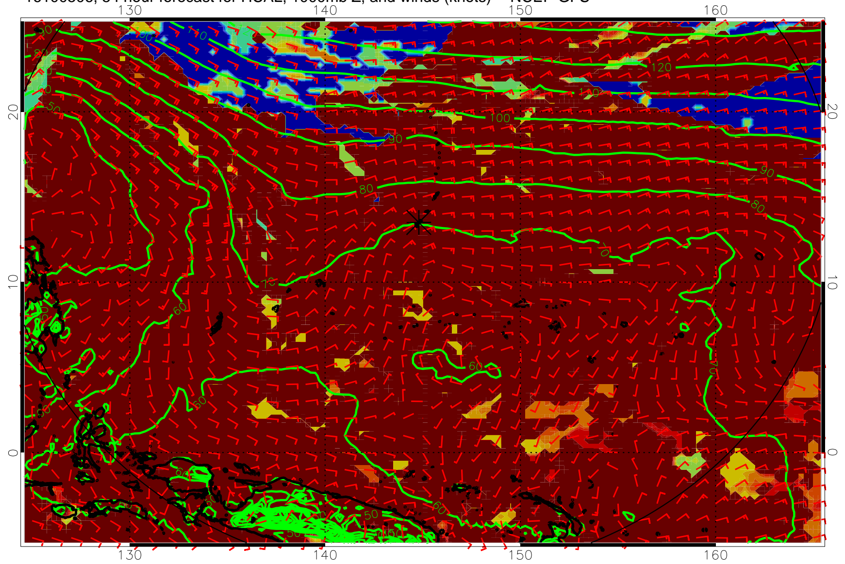
16100506, 54 hour forecast for HCAL, 1000mb Z, and winds (knots) -- NCEP GFS
