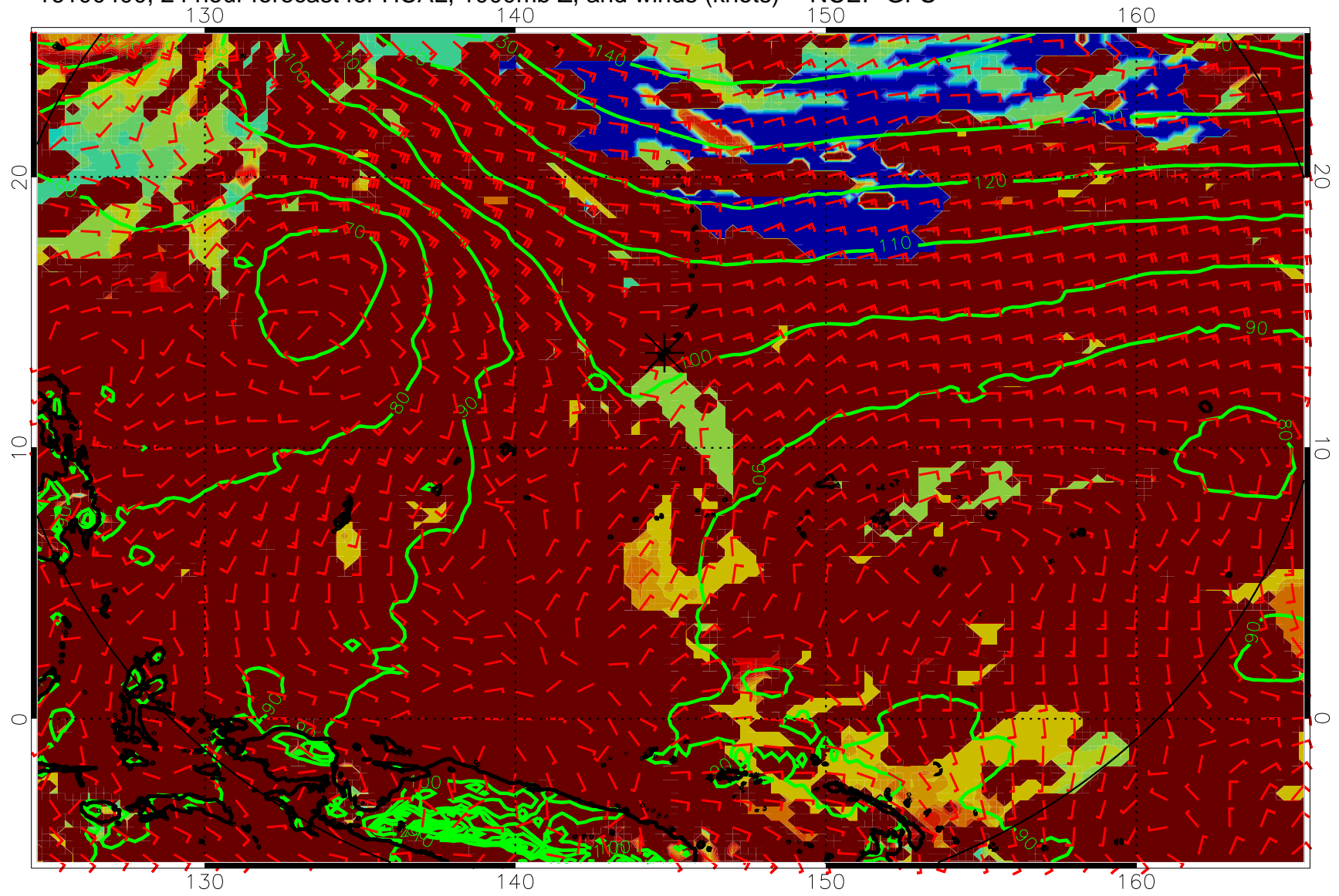
16100400, 24 hour forecast for HCAL, 1000mb Z, and winds (knots) -- NCEP GFS
