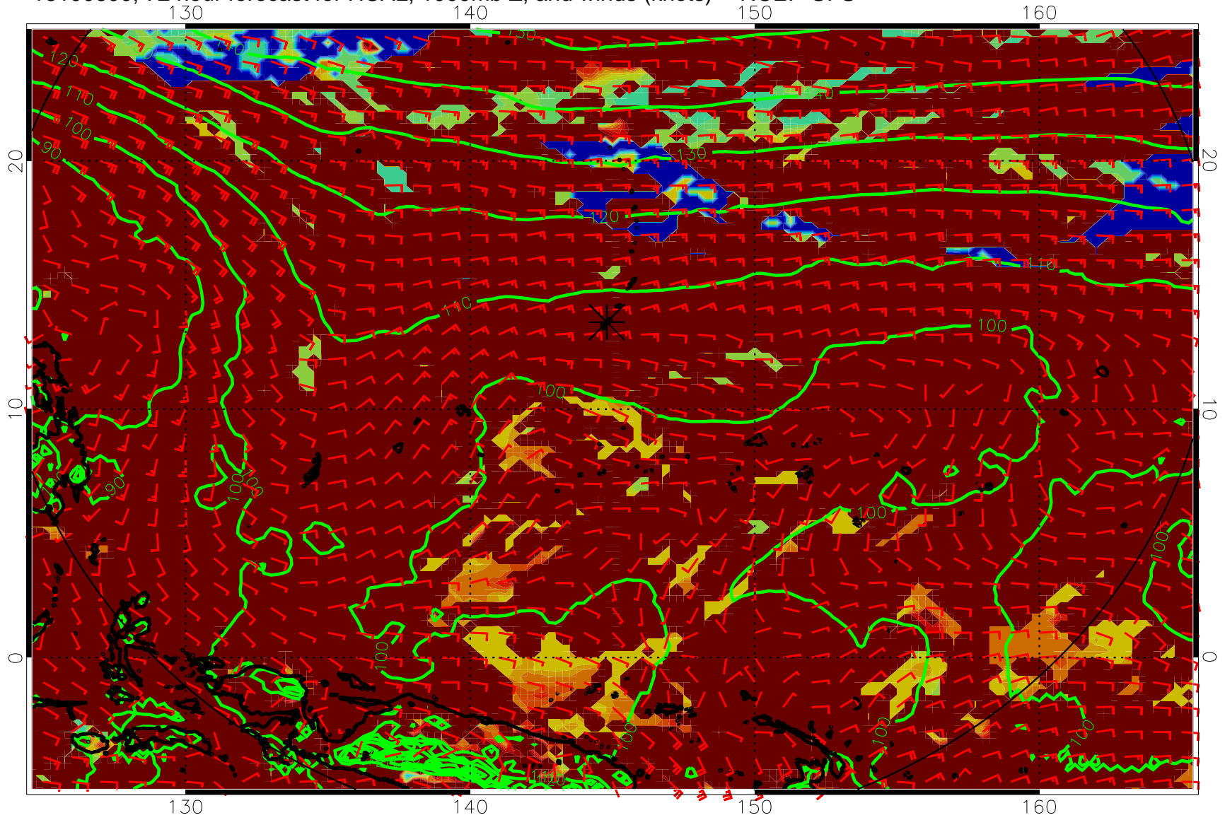
16100600, 72 hour forecast for HCAL, 1000mb Z, and winds (knots) -- NCEP GFS
