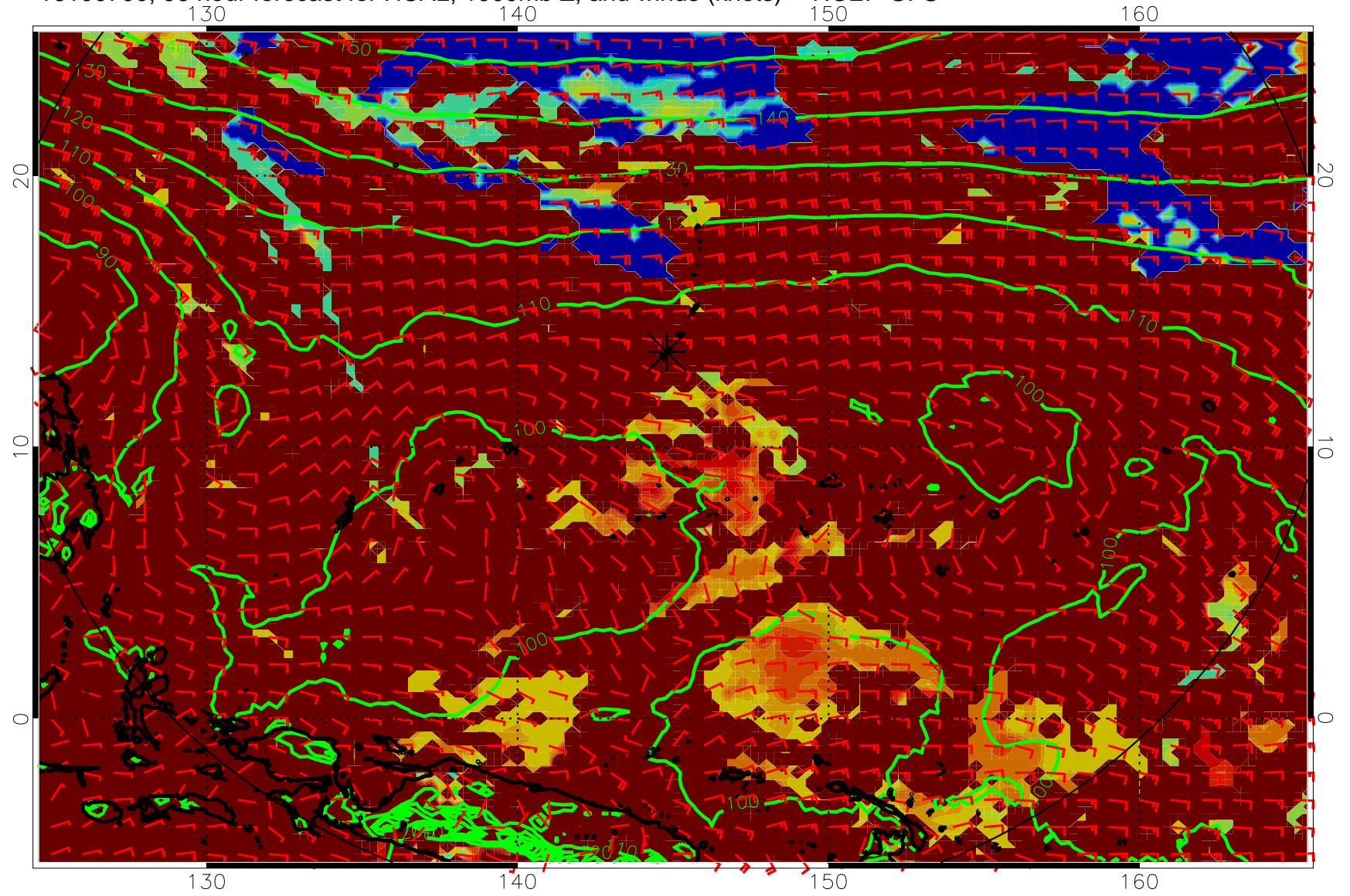
16100700, 96 hour forecast for HCAL, 1000mb Z, and winds (knots) -- NCEP GFS
