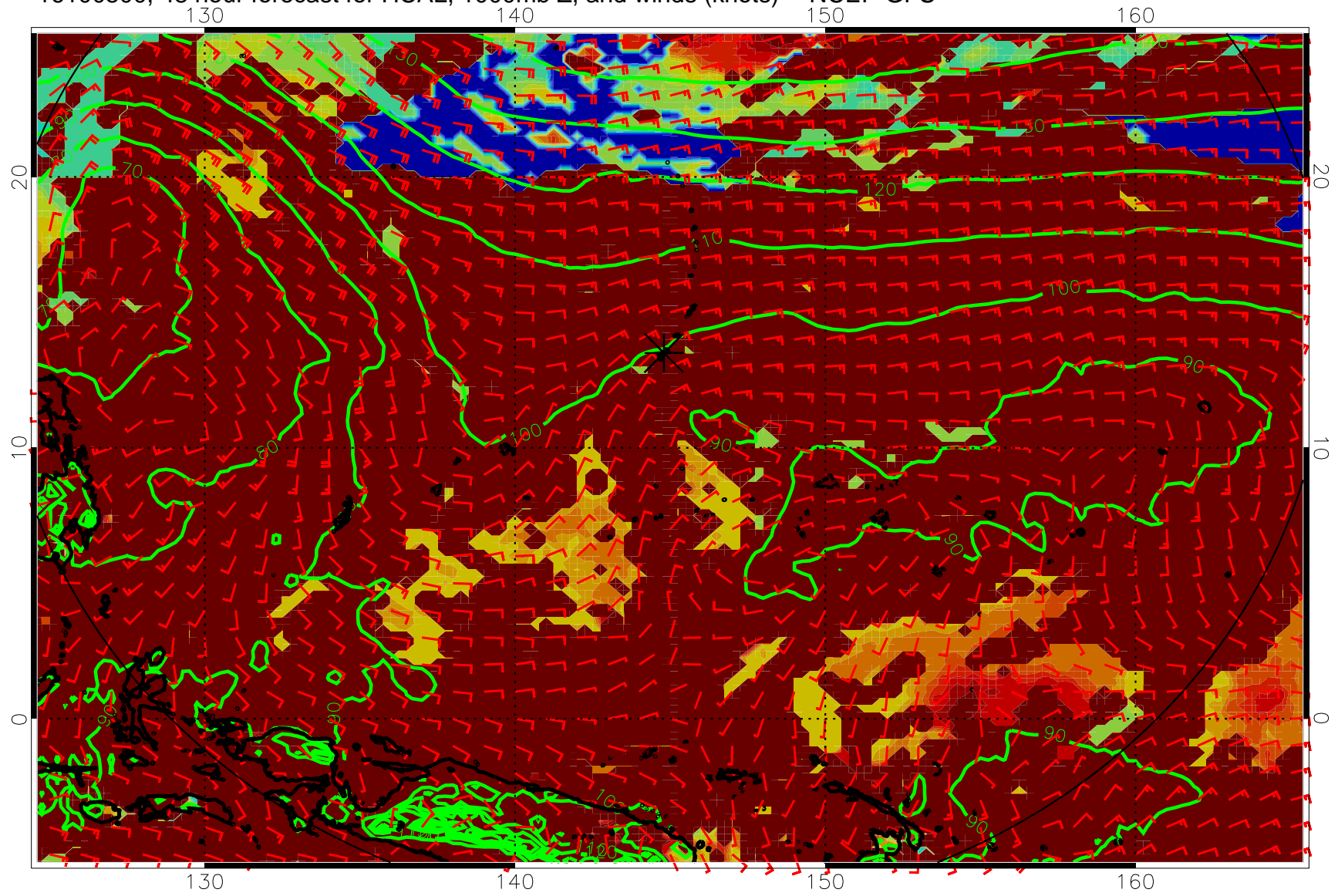
16100500, 48 hour forecast for HCAL, 1000mb Z, and winds (knots) -- NCEP GFS
