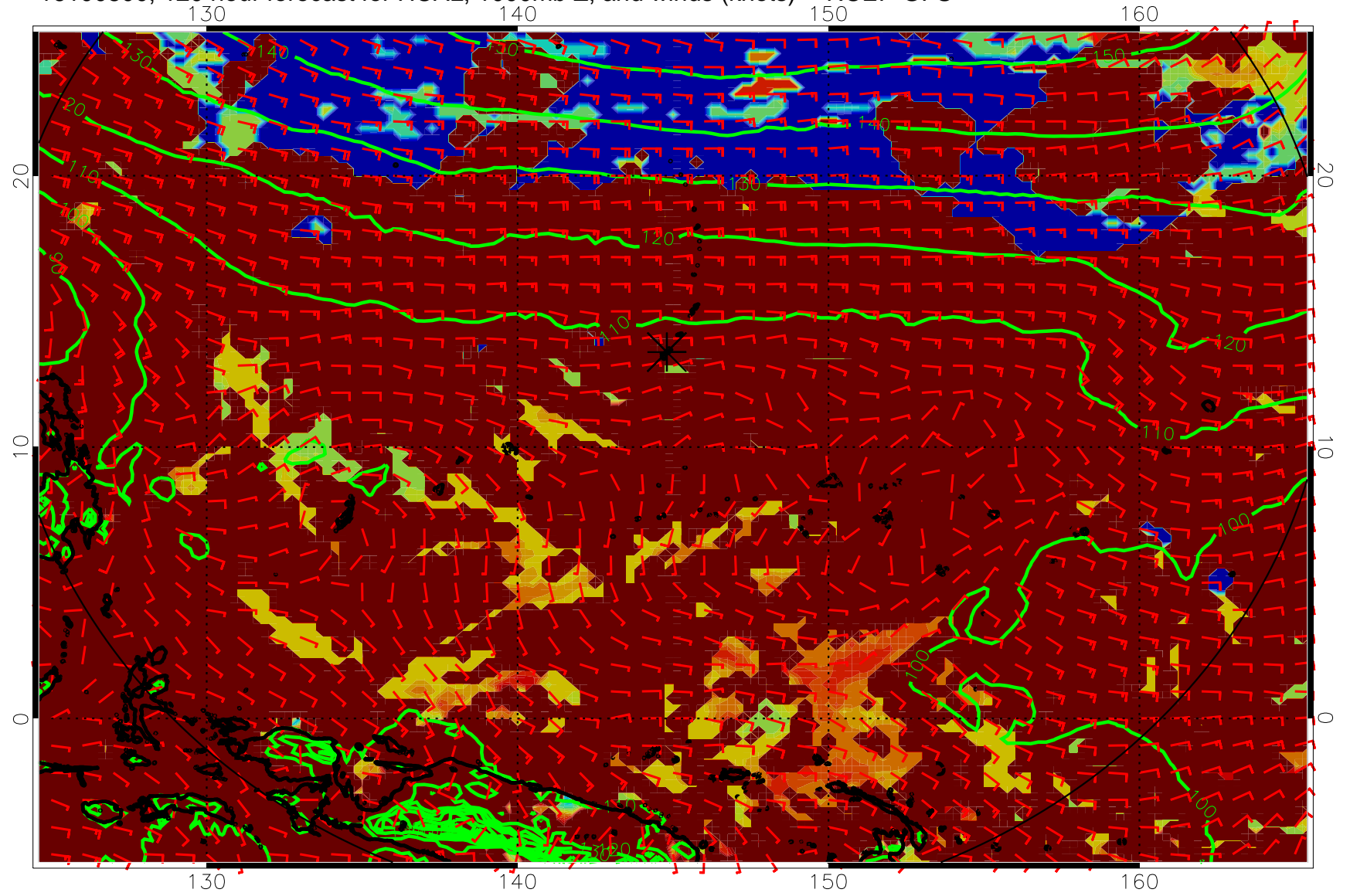
16100800, 120 hour forecast for HCAL, 1000mb Z, and winds (knots) -- NCEP GFS
