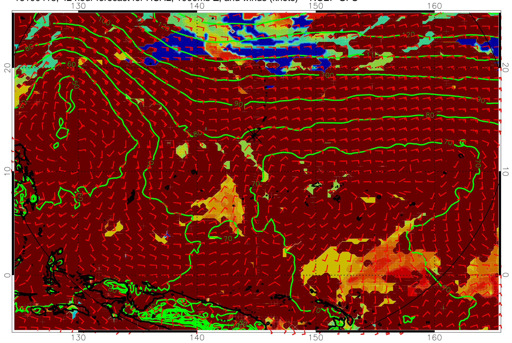
16100418, 42 hour forecast for HCAL, 1000mb Z, and winds (knots) -- NCEP GFS
