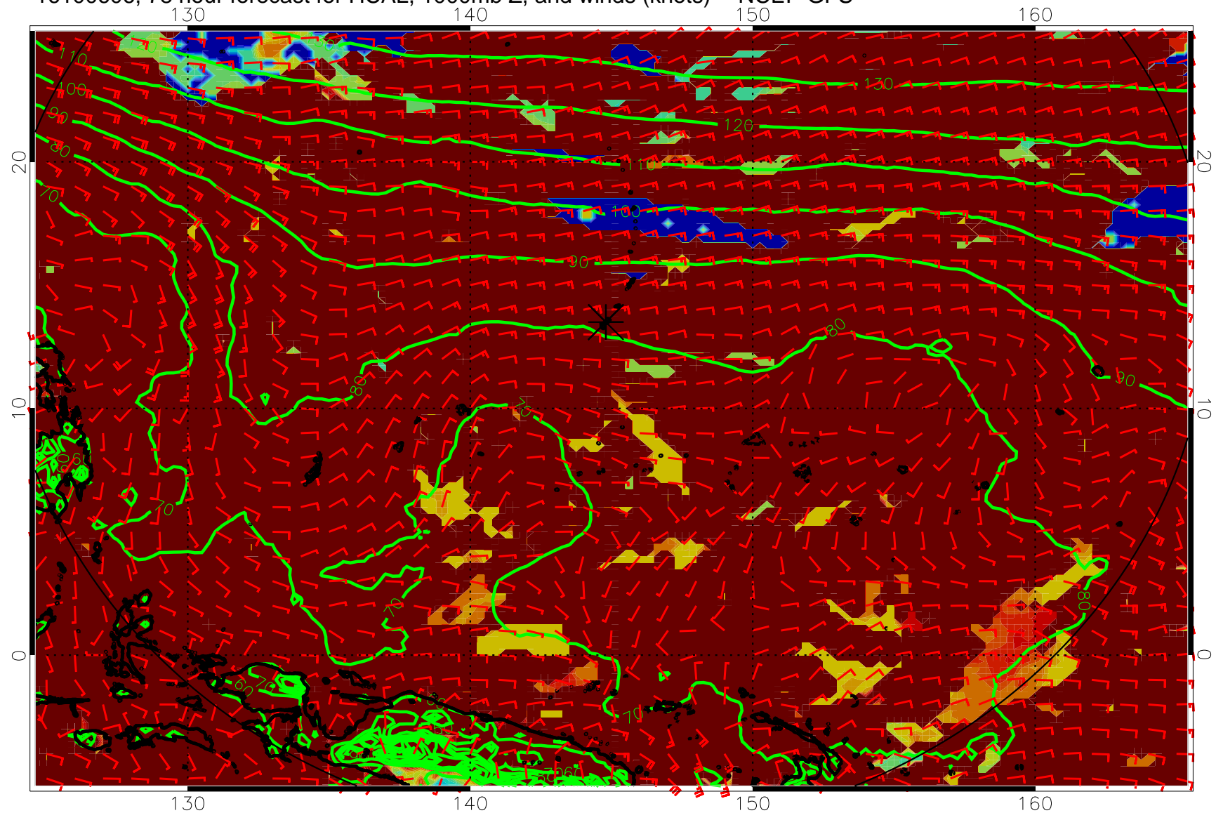
16100606, 78 hour forecast for HCAL, 1000mb Z, and winds (knots) -- NCEP GFS
