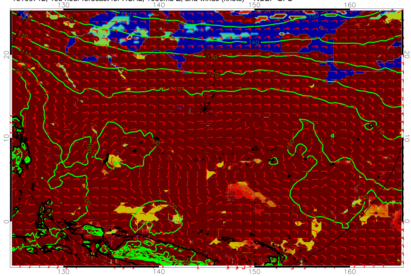
16100712, 108 hour forecast for HCAL, 1000mb Z, and winds (knots) -- NCEP GFS
