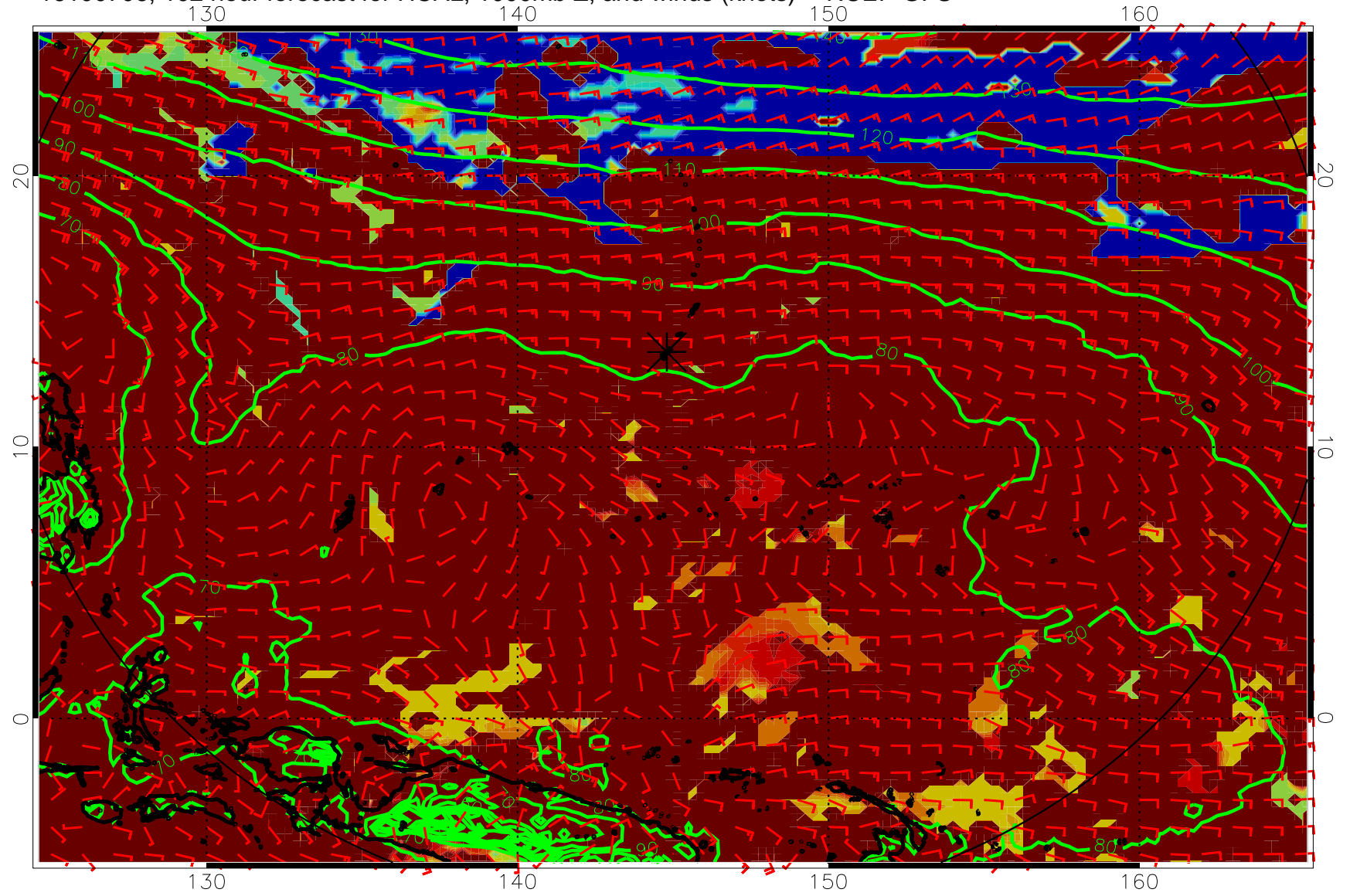
16100706, 102 hour forecast for HCAL, 1000mb Z, and winds (knots) -- NCEP GFS
