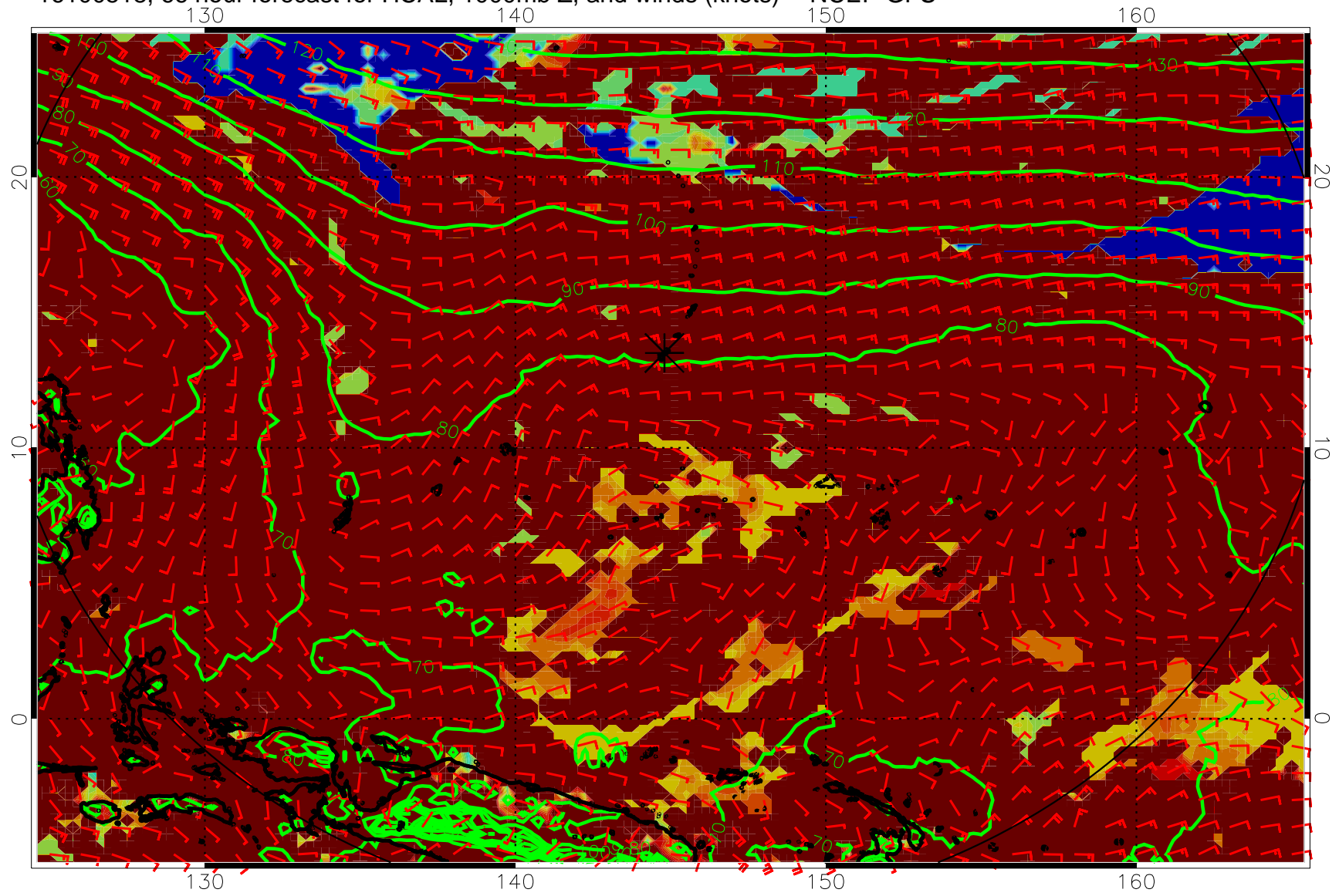
16100518, 66 hour forecast for HCAL, 1000mb Z, and winds (knots) -- NCEP GFS
