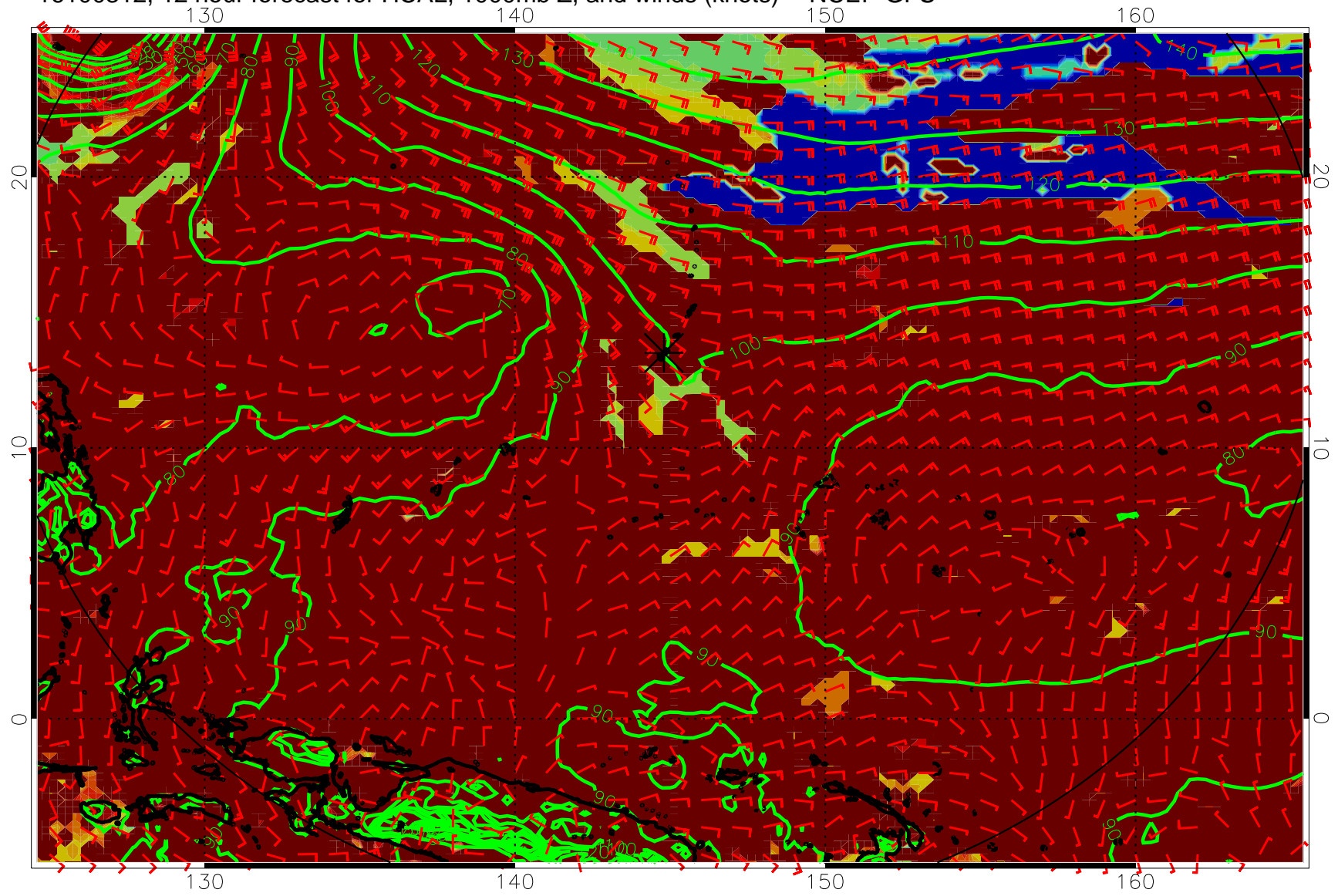
16100312, 12 hour forecast for HCAL, 1000mb Z, and winds (knots) -- NCEP GFS
