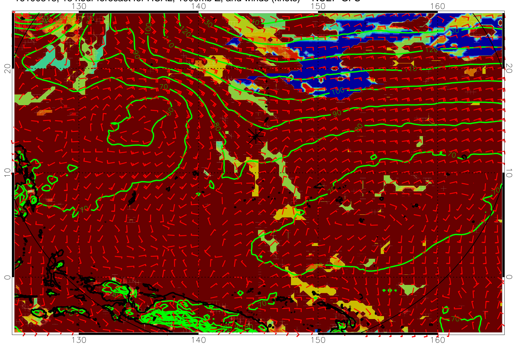
16100318, 18 hour forecast for HCAL, 1000mb Z, and winds (knots) -- NCEP GFS
