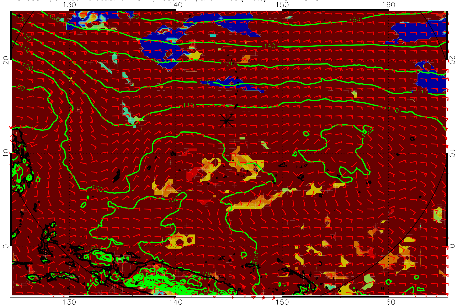
16100612, 84 hour forecast for HCAL, 1000mb Z, and winds (knots) -- NCEP GFS
