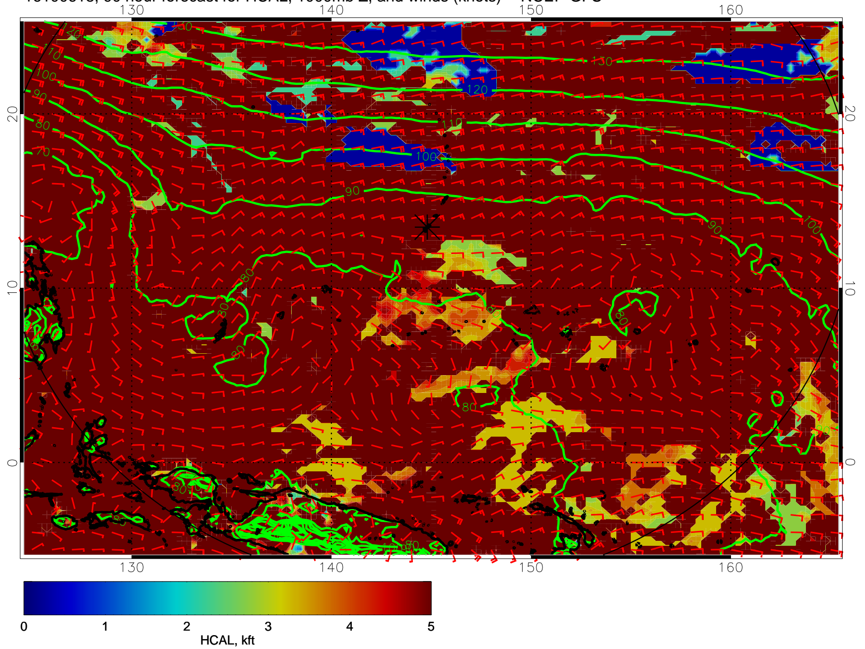
16100618, 90 hour forecast for HCAL, 1000mb Z, and winds (knots) -- NCEP GFS
