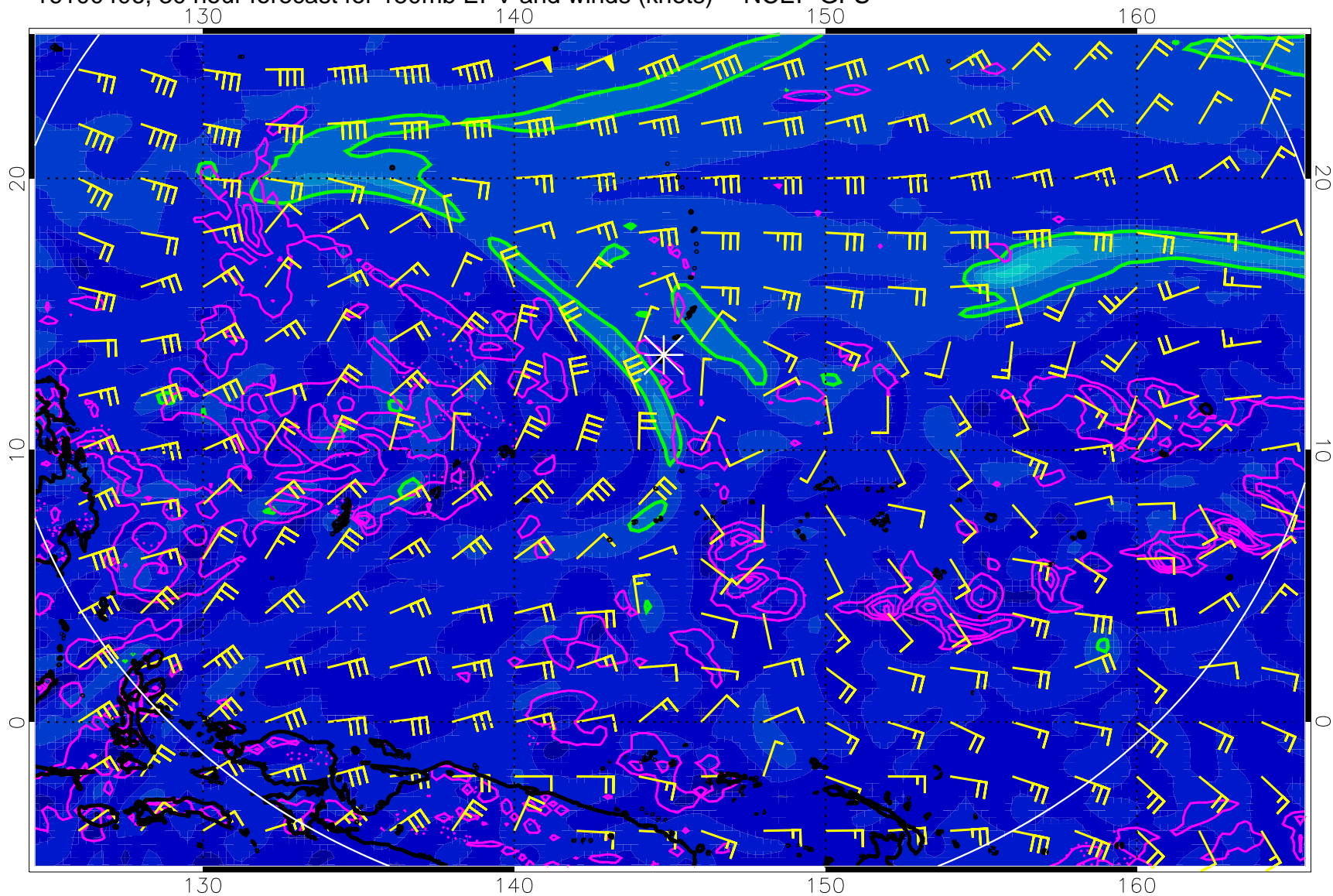
16100406, 30 hour forecast for 150mb EPV and winds (knots) -- NCEP GFS
