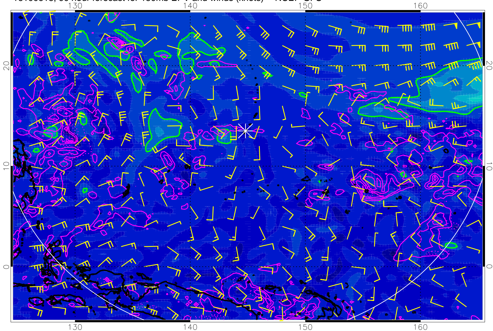
16100618, 90 hour forecast for 150mb EPV and winds (knots) -- NCEP GFS
