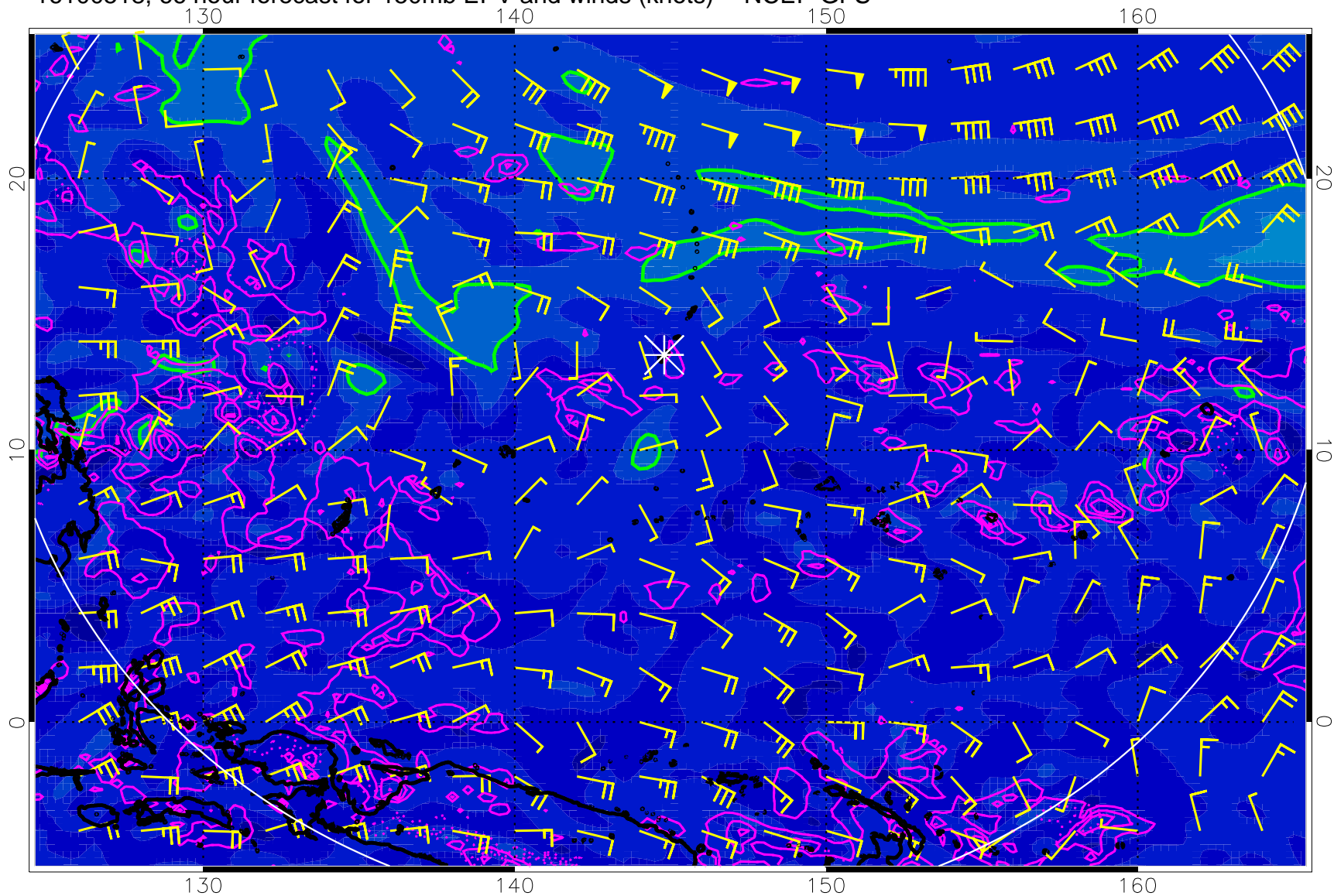
16100518, 66 hour forecast for 150mb EPV and winds (knots) -- NCEP GFS
