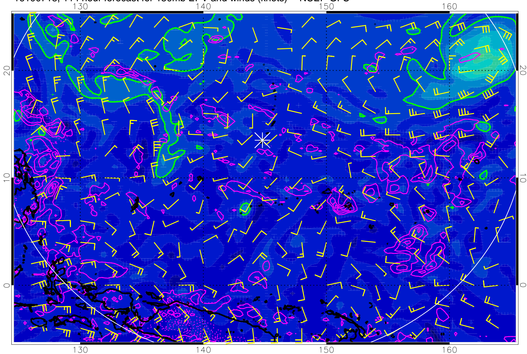
16100718, 114 hour forecast for 150mb EPV and winds (knots) -- NCEP GFS
