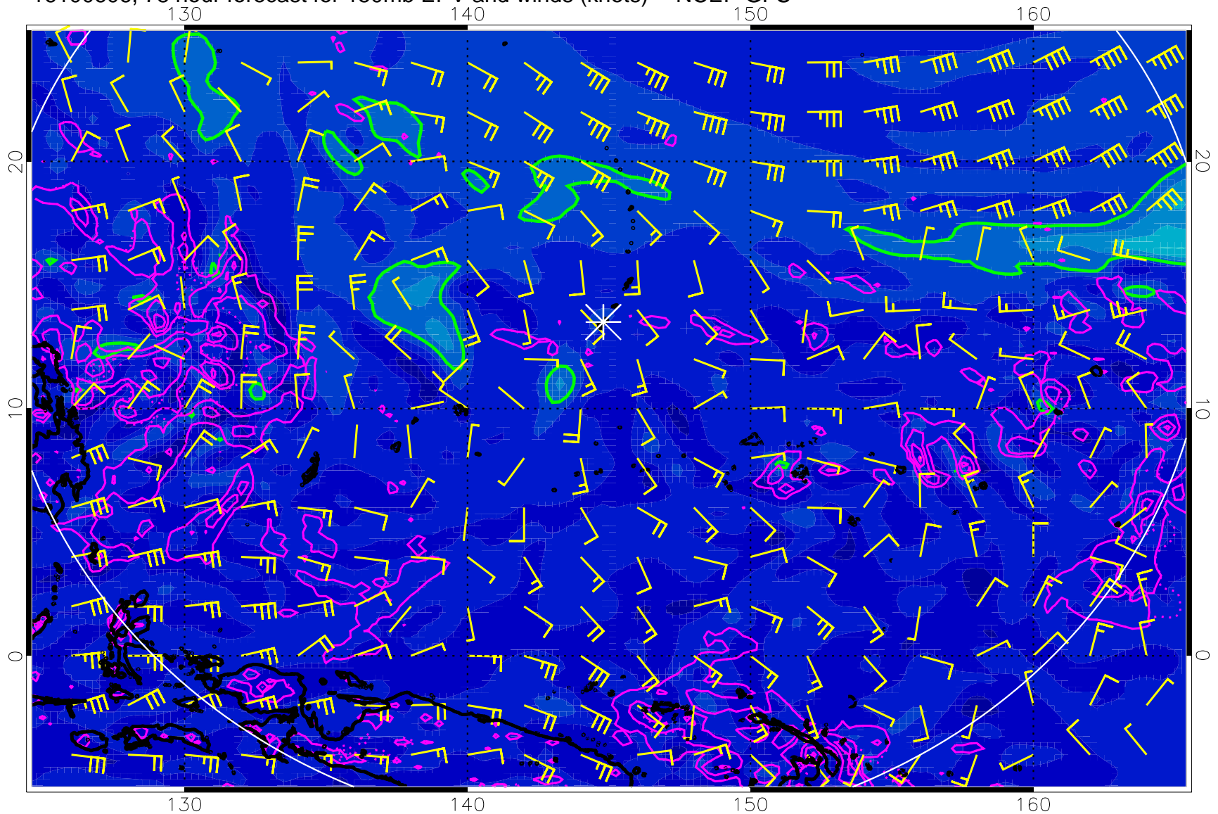
16100606, 78 hour forecast for 150mb EPV and winds (knots) -- NCEP GFS
