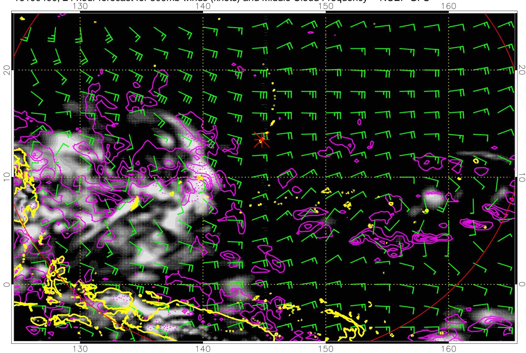
16100400, 24 hour forecast for 500mb winds (knots) and Middle Cloud Frequency -- NCEP GFS
