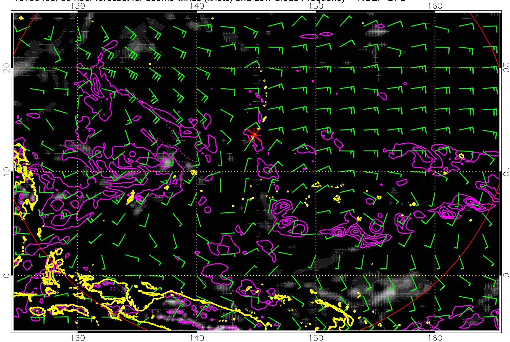
16100406, 30 hour forecast for 850mb winds (knots) and Low Cloud Frequency -- NCEP GFS
