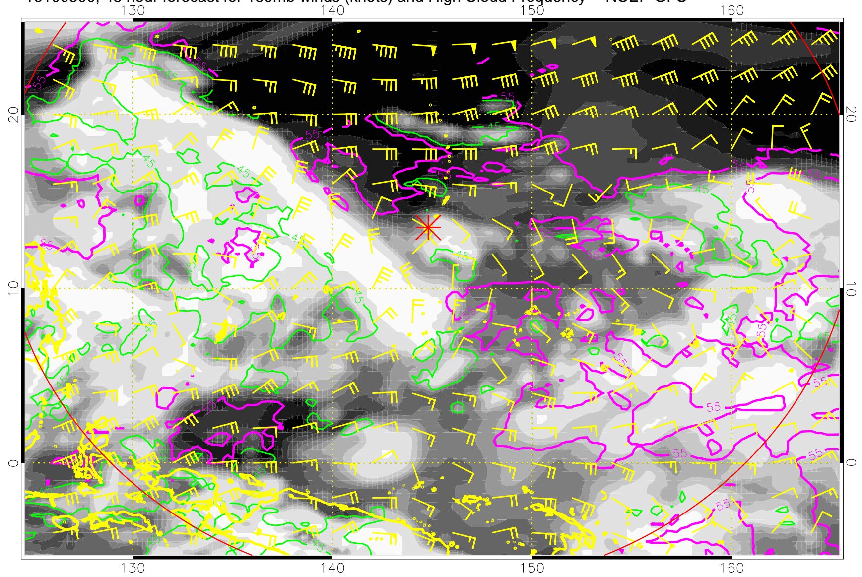
16100500, 48 hour forecast for 150mb winds (knots) and High Cloud Frequency -- NCEP GFS
