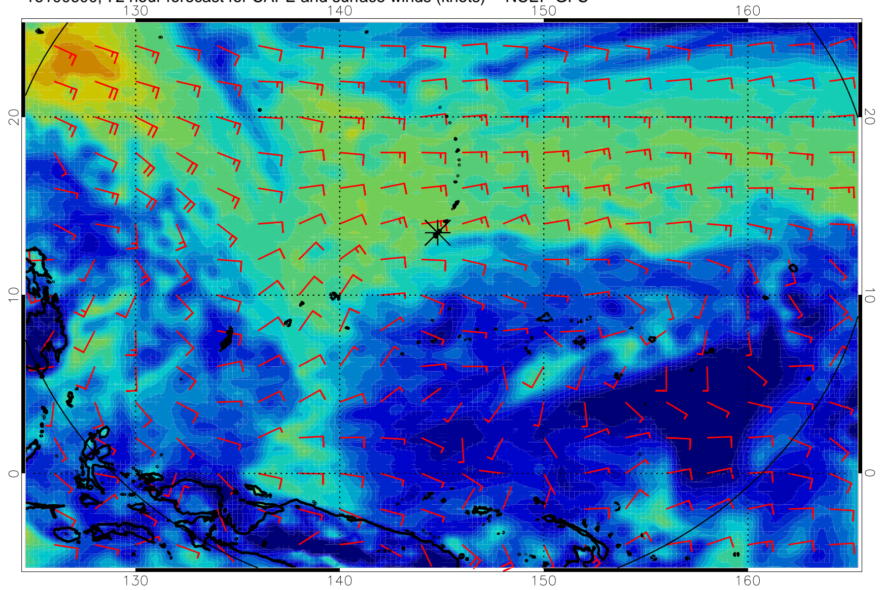
16100600, 72 hour forecast for CAPE and surface winds (knots) -- NCEP GFS
