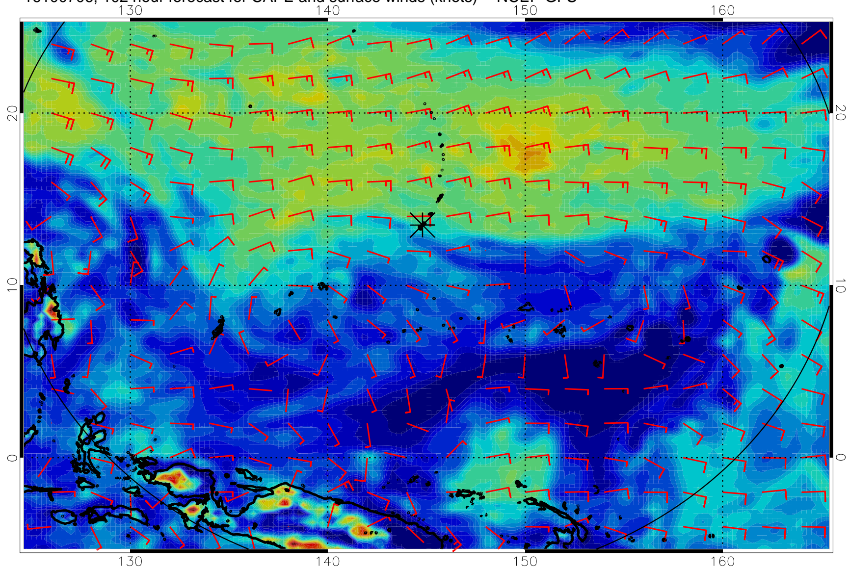
16100706, 102 hour forecast for CAPE and surface winds (knots) -- NCEP GFS
