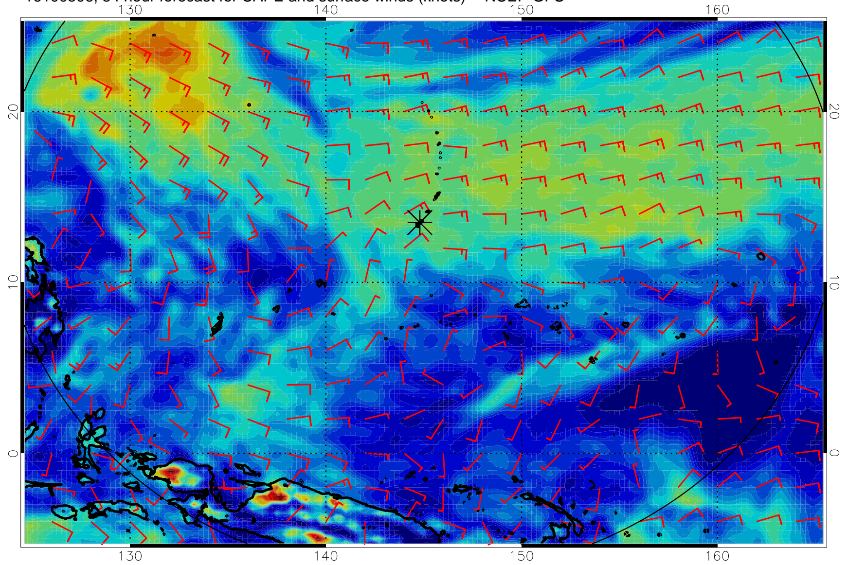
16100506, 54 hour forecast for CAPE and surface winds (knots) -- NCEP GFS
