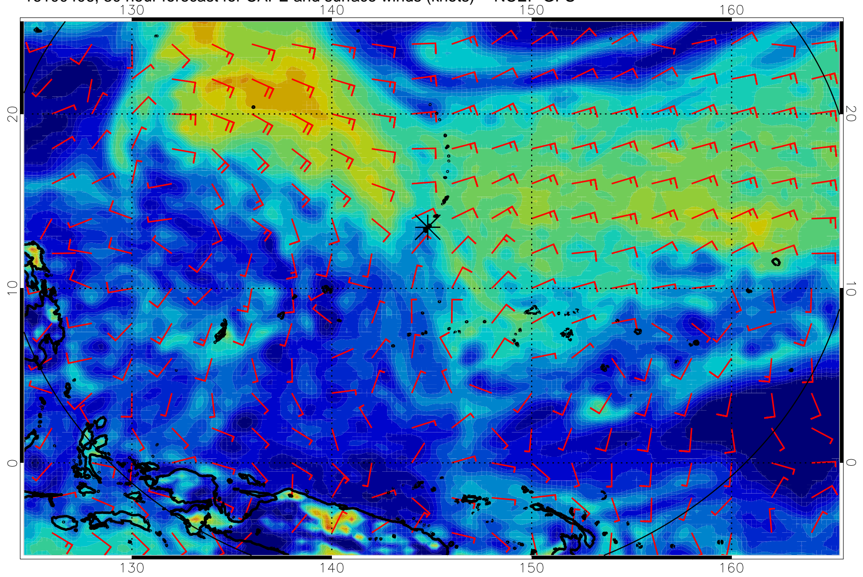
16100406, 30 hour forecast for CAPE and surface winds (knots) -- NCEP GFS
