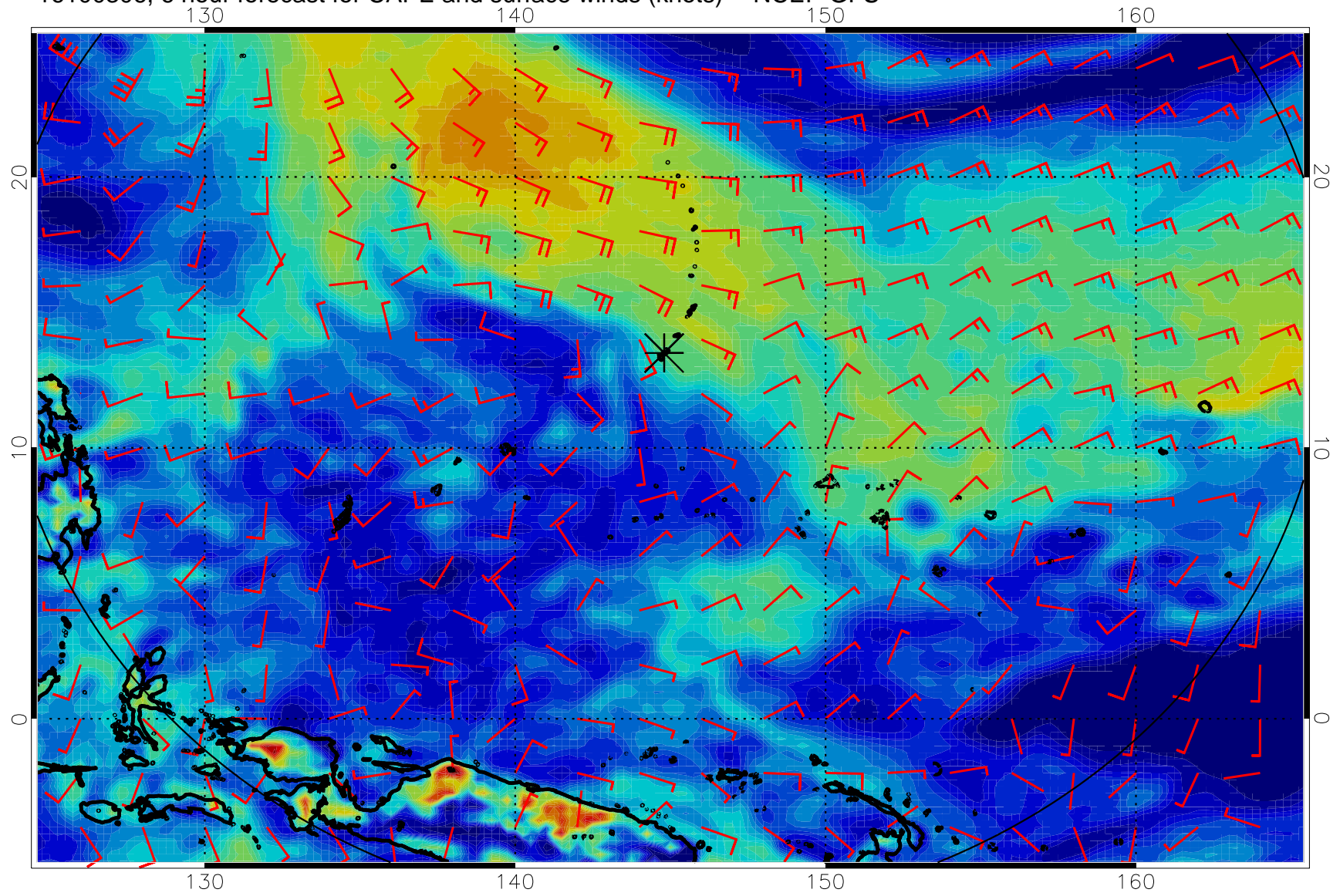
16100306, 6 hour forecast for CAPE and surface winds (knots) -- NCEP GFS
