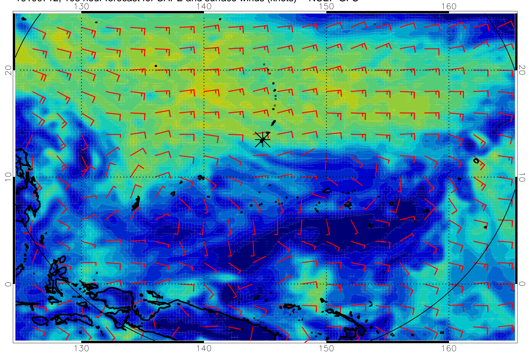
16100712, 108 hour forecast for CAPE and surface winds (knots) -- NCEP GFS
