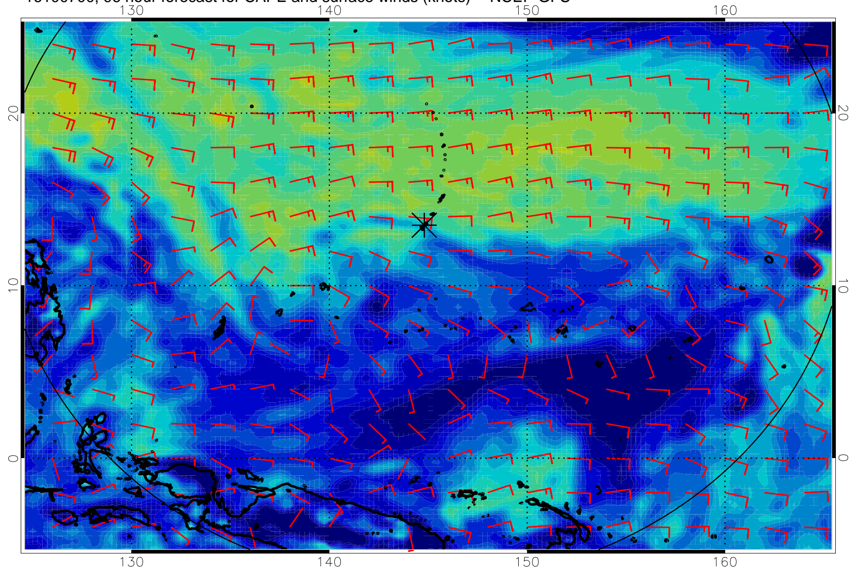
16100700, 96 hour forecast for CAPE and surface winds (knots) -- NCEP GFS
