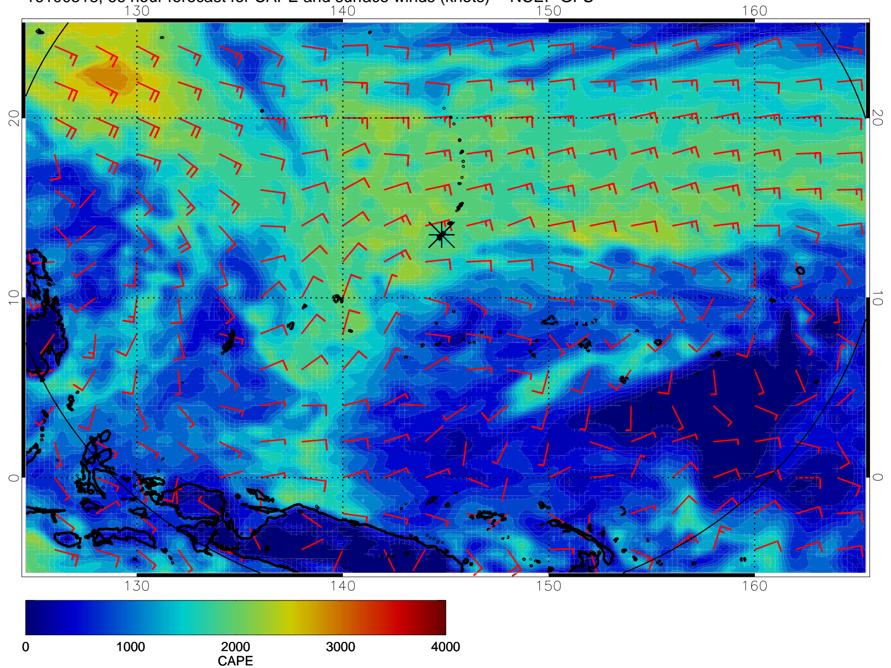
16100518, 66 hour forecast for CAPE and surface winds (knots) -- NCEP GFS
