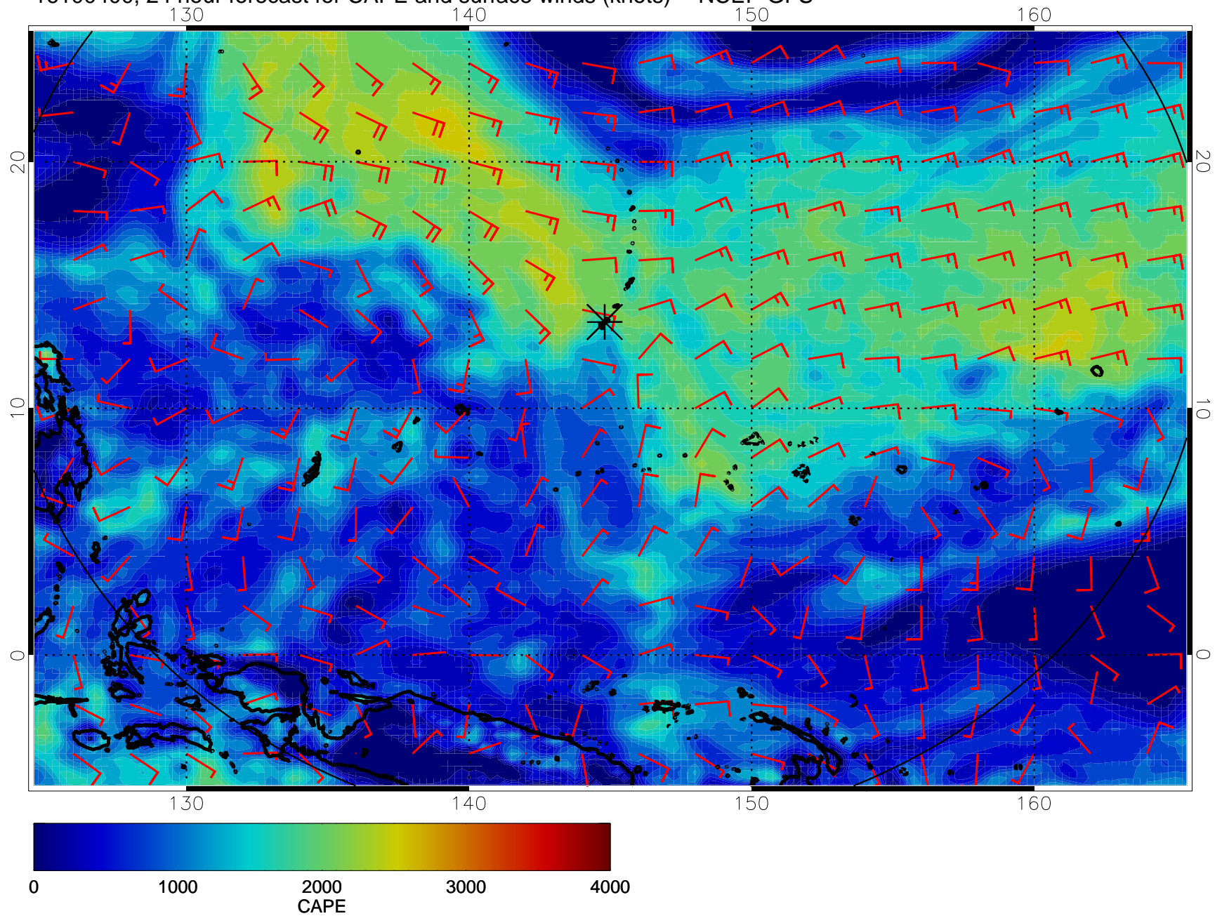
16100400, 24 hour forecast for CAPE and surface winds (knots) -- NCEP GFS
