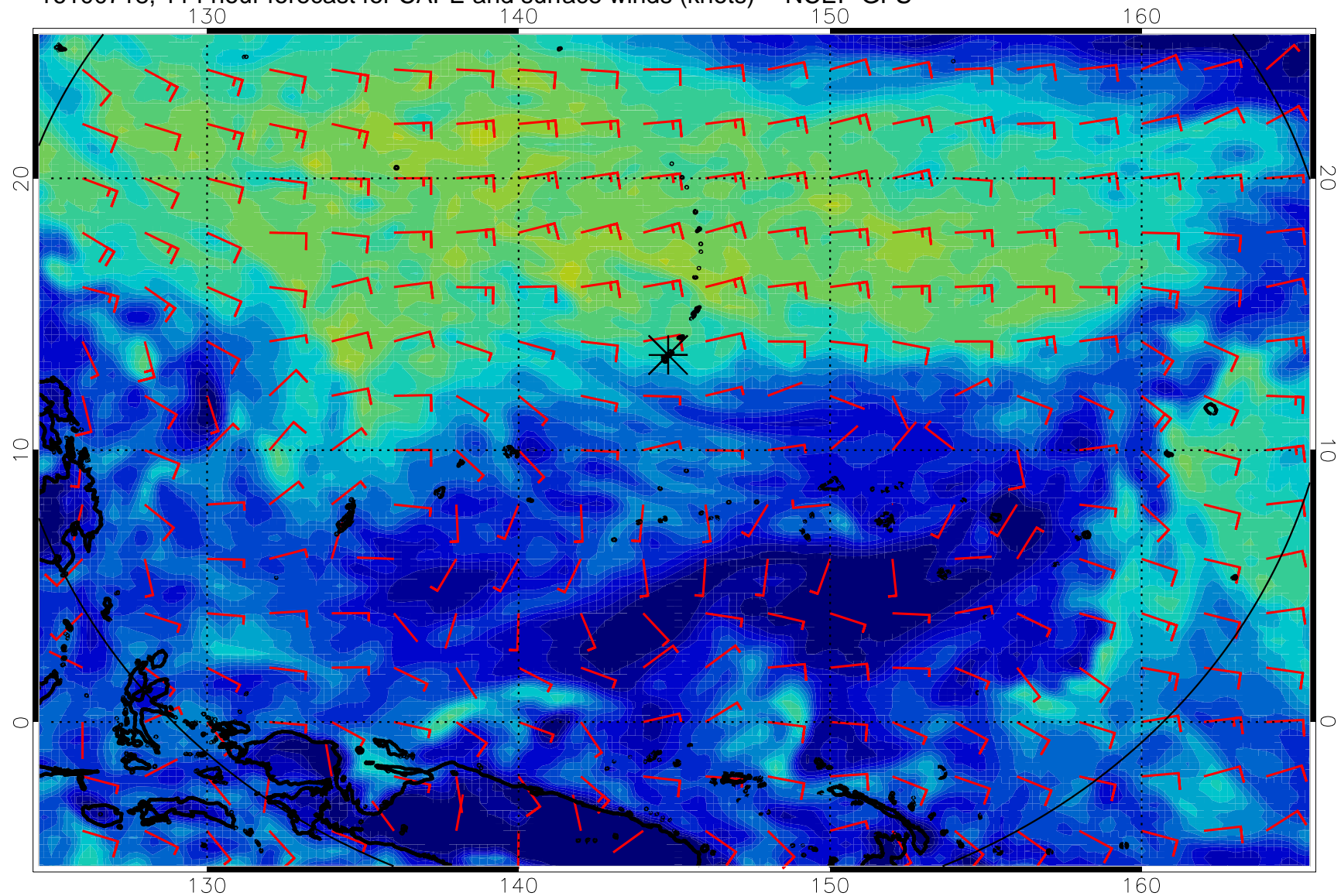
16100718, 114 hour forecast for CAPE and surface winds (knots) -- NCEP GFS
