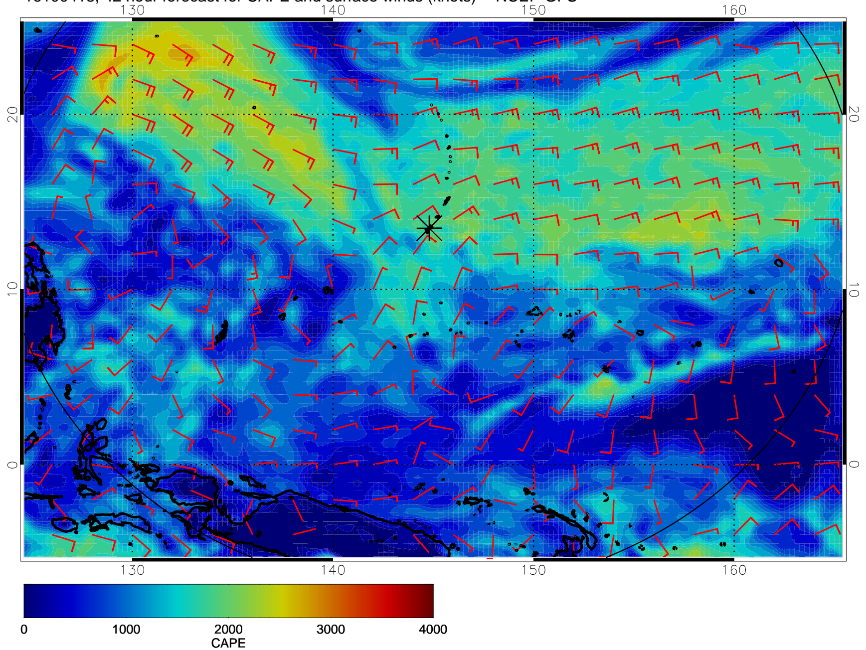
16100418, 42 hour forecast for CAPE and surface winds (knots) -- NCEP GFS
