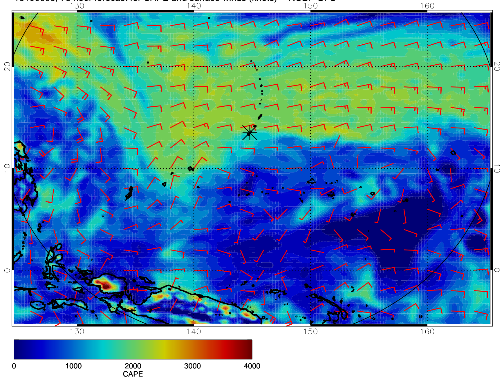
16100606, 78 hour forecast for CAPE and surface winds (knots) -- NCEP GFS
