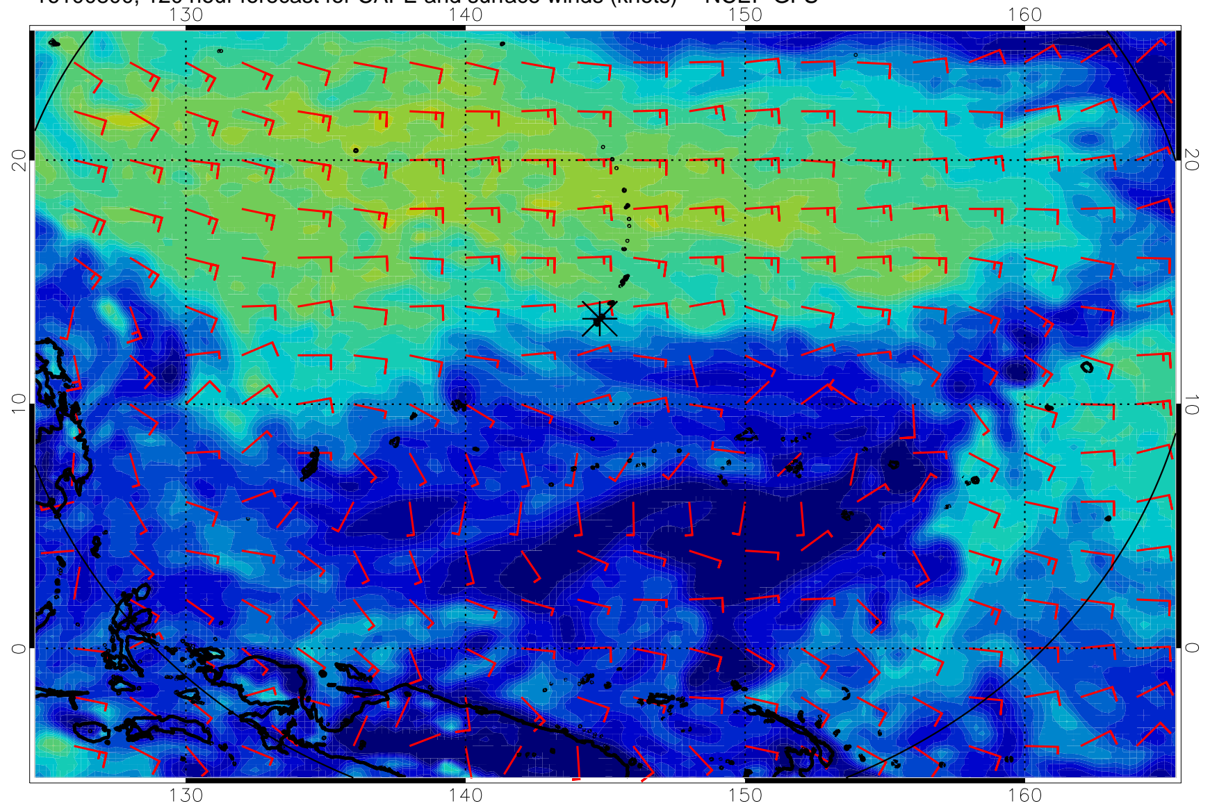
16100800, 120 hour forecast for CAPE and surface winds (knots) -- NCEP GFS
