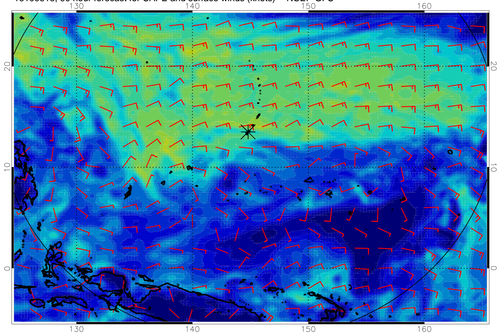
16100618, 90 hour forecast for CAPE and surface winds (knots) -- NCEP GFS
