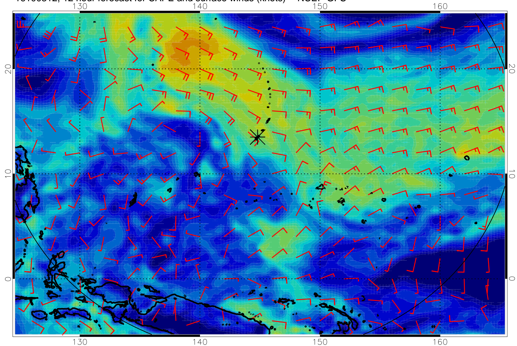
16100312, 12 hour forecast for CAPE and surface winds (knots) -- NCEP GFS
