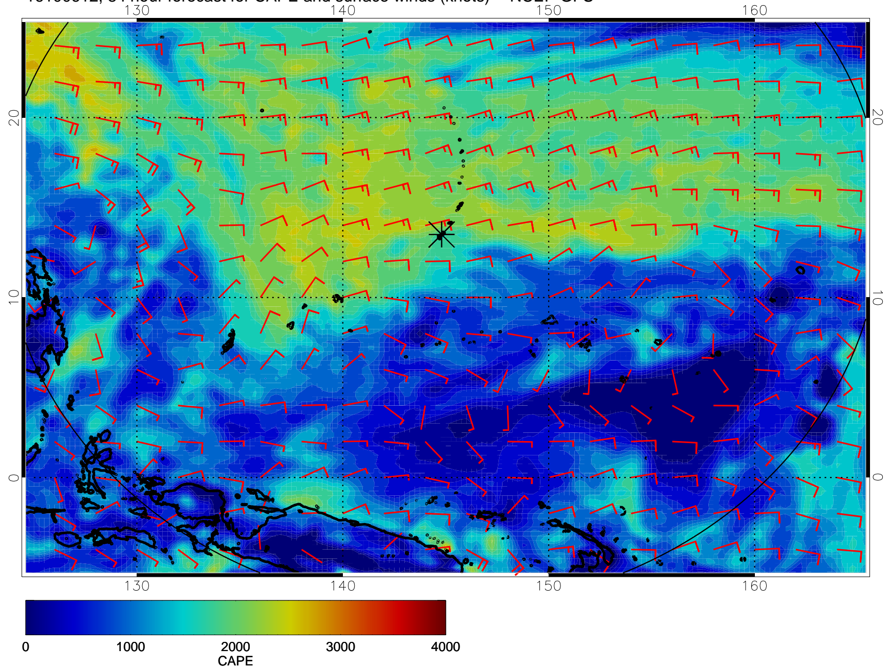
16100612, 84 hour forecast for CAPE and surface winds (knots) -- NCEP GFS
