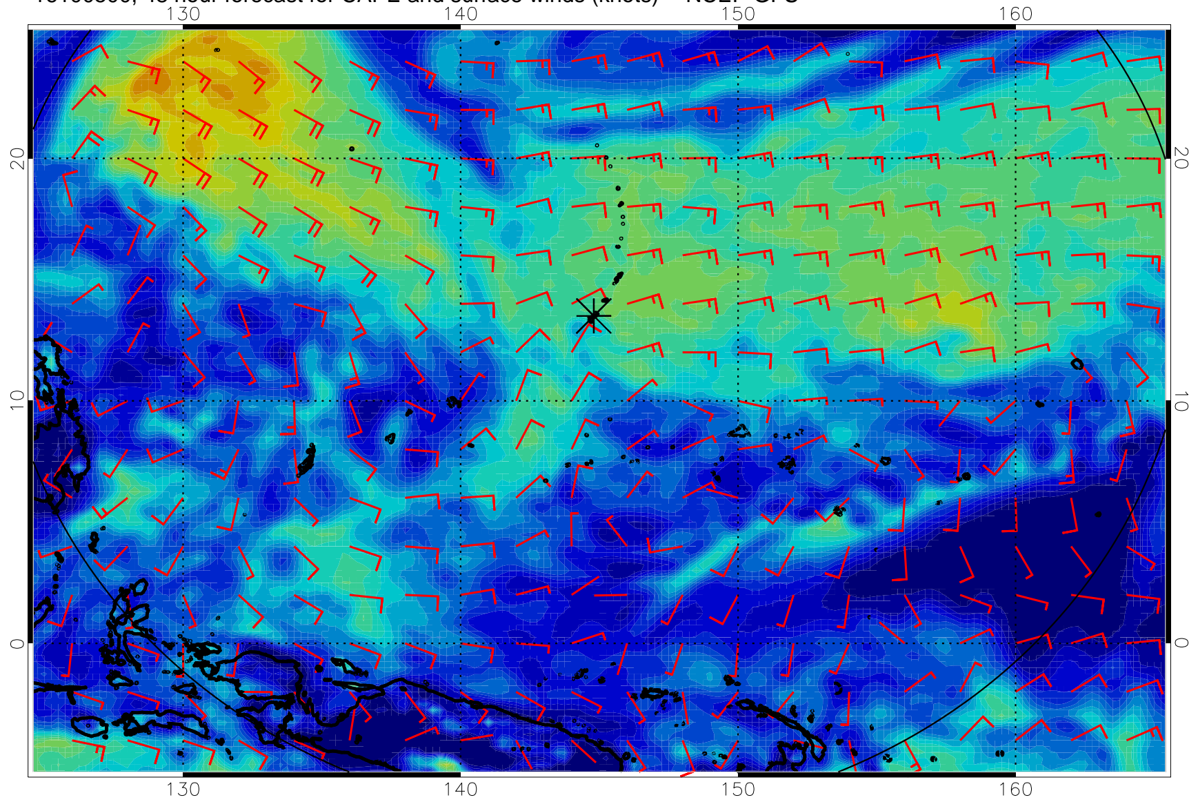
16100500, 48 hour forecast for CAPE and surface winds (knots) -- NCEP GFS
