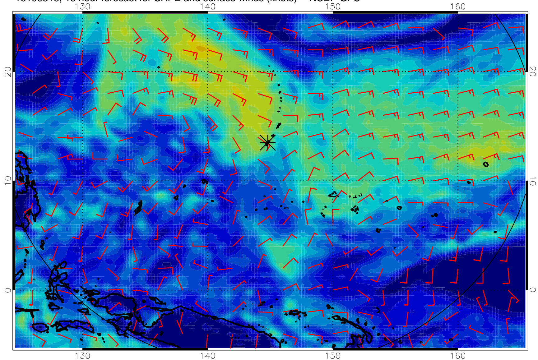
16100318, 18 hour forecast for CAPE and surface winds (knots) -- NCEP GFS
