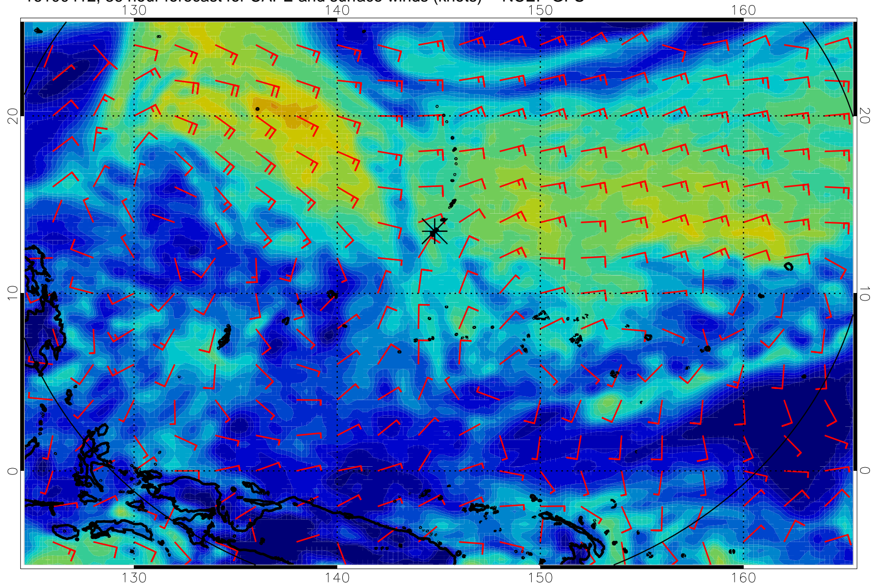
16100412, 36 hour forecast for CAPE and surface winds (knots) -- NCEP GFS
