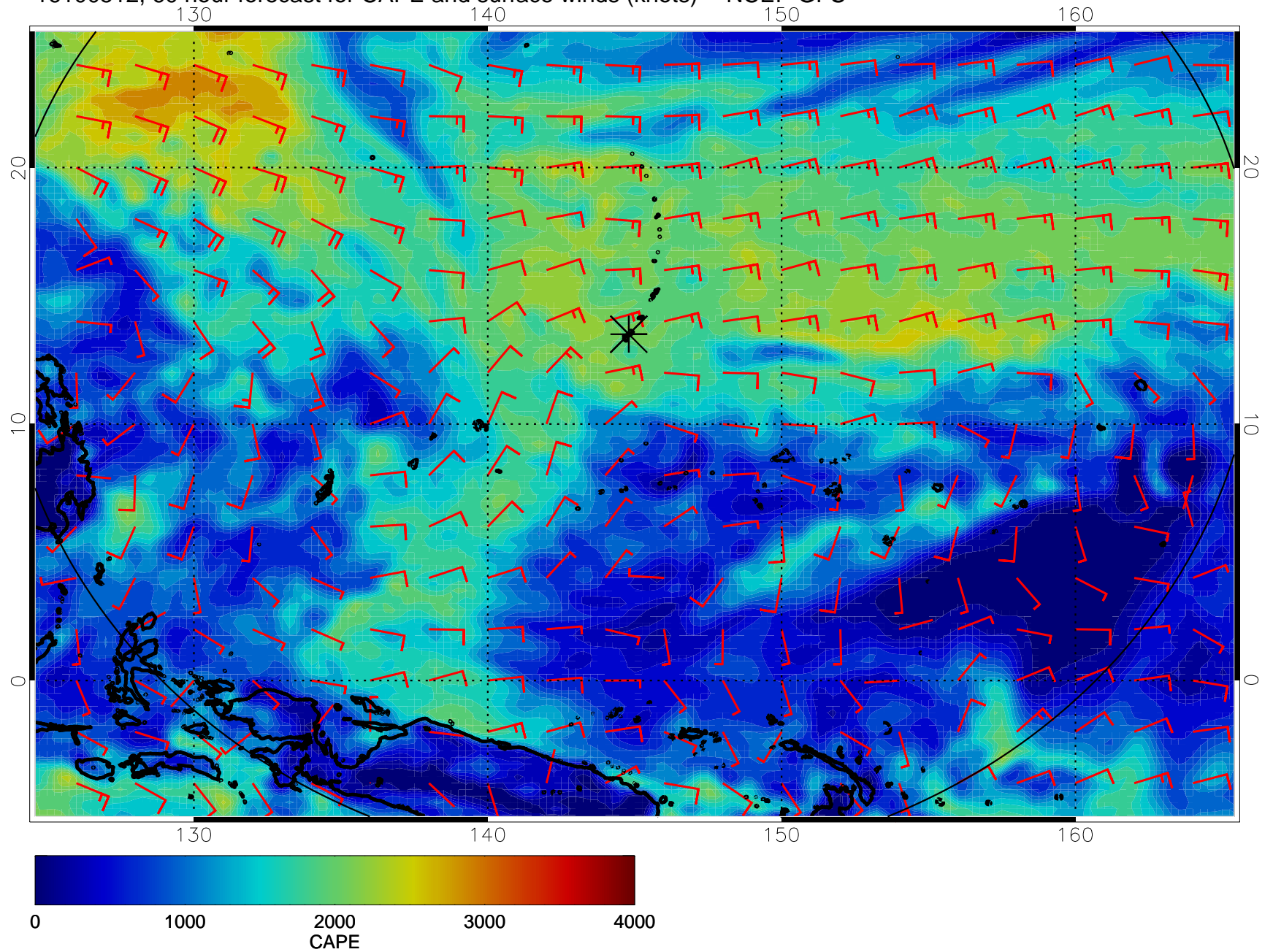
16100512, 60 hour forecast for CAPE and surface winds (knots) -- NCEP GFS
