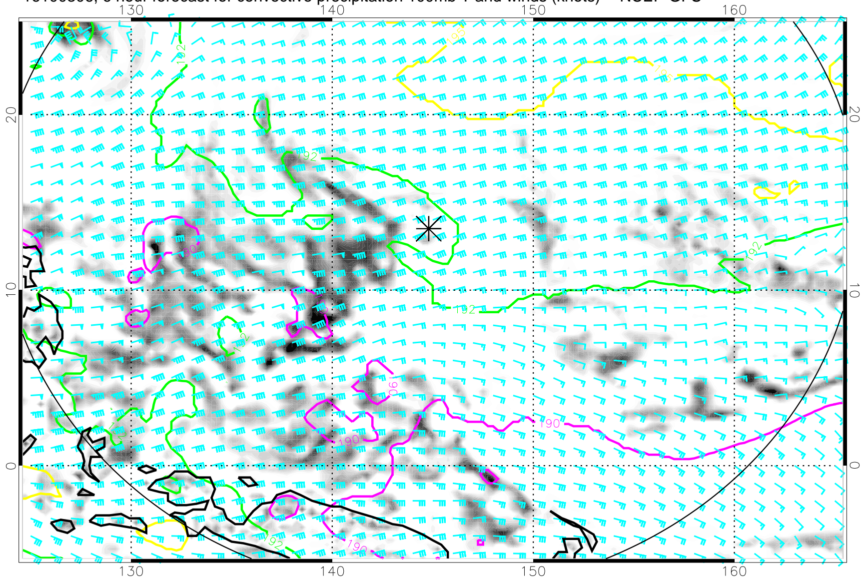
16100306, 6 hour forecast for convective precipitation 100mb T and winds (knots) -- NCEP GFS
