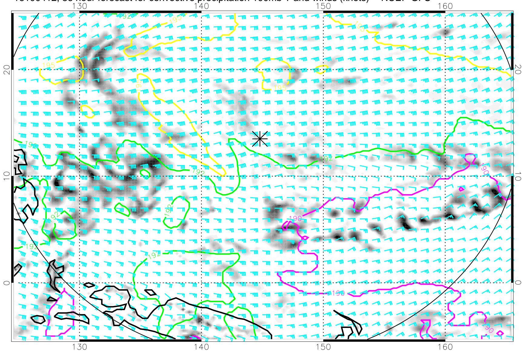
16100412, 36 hour forecast for convective precipitation 100mb T and winds (knots) -- NCEP GFS
