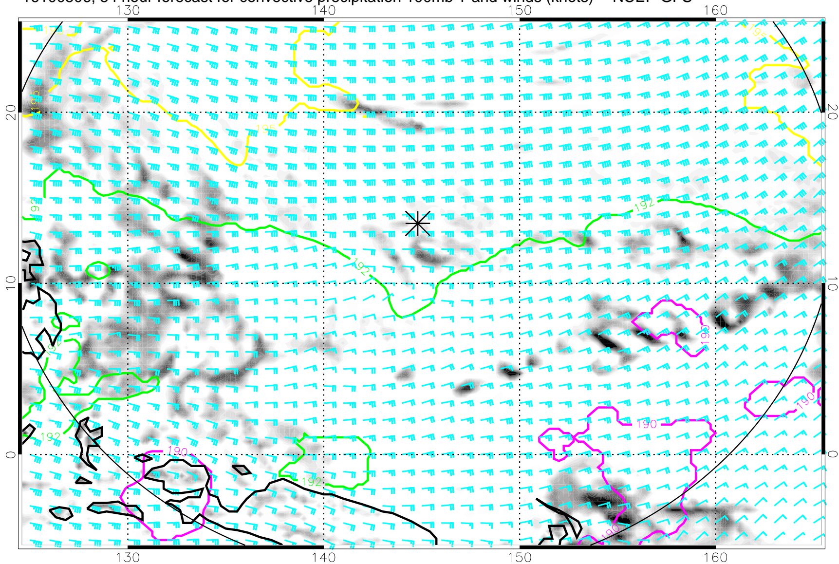
16100506, 54 hour forecast for convective precipitation 100mb T and winds (knots) -- NCEP GFS
