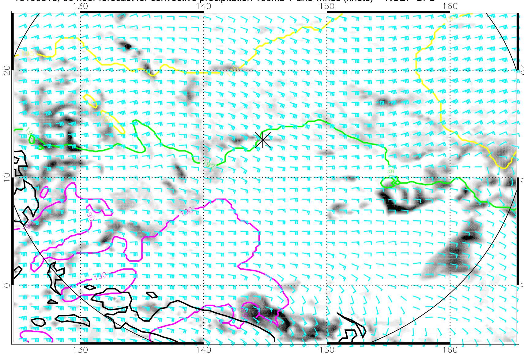
16100618, 90 hour forecast for convective precipitation 100mb T and winds (knots) -- NCEP GFS
