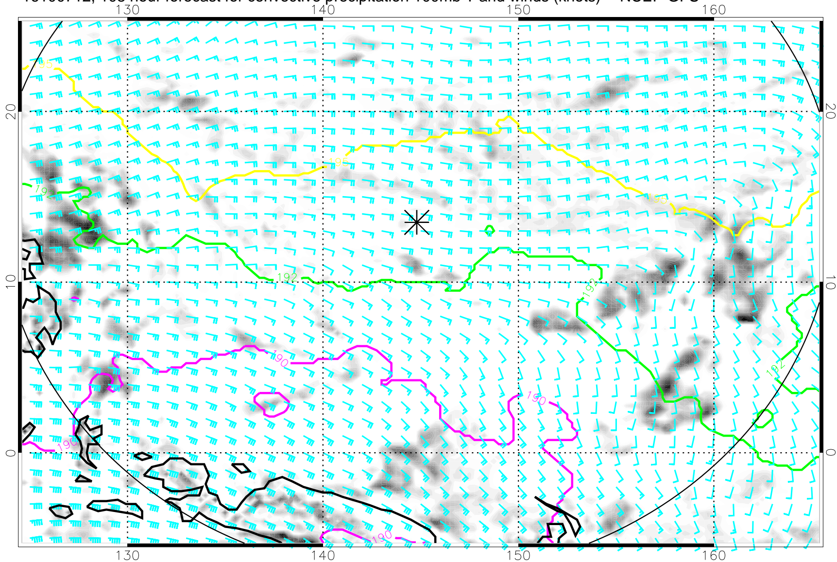
16100712, 108 hour forecast for convective precipitation 100mb T and winds (knots) -- NCEP GFS
