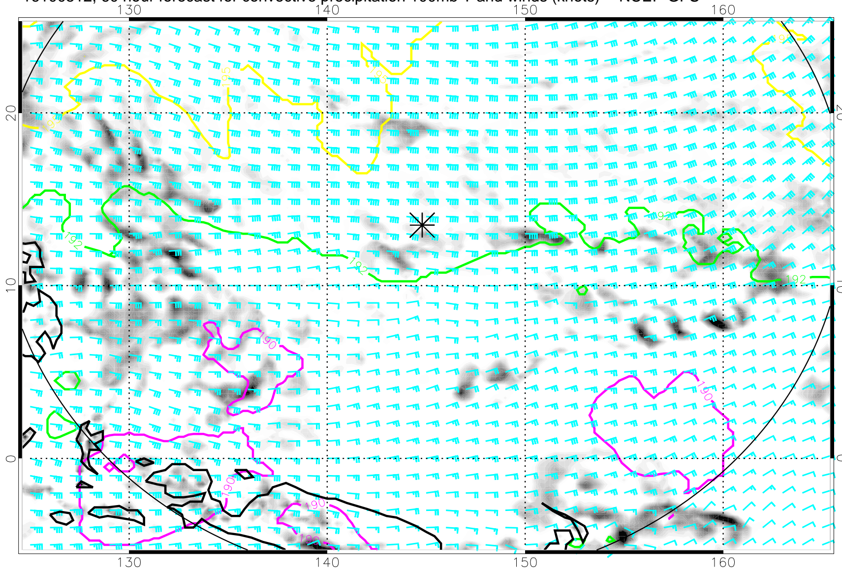
16100512, 60 hour forecast for convective precipitation 100mb T and winds (knots) -- NCEP GFS
