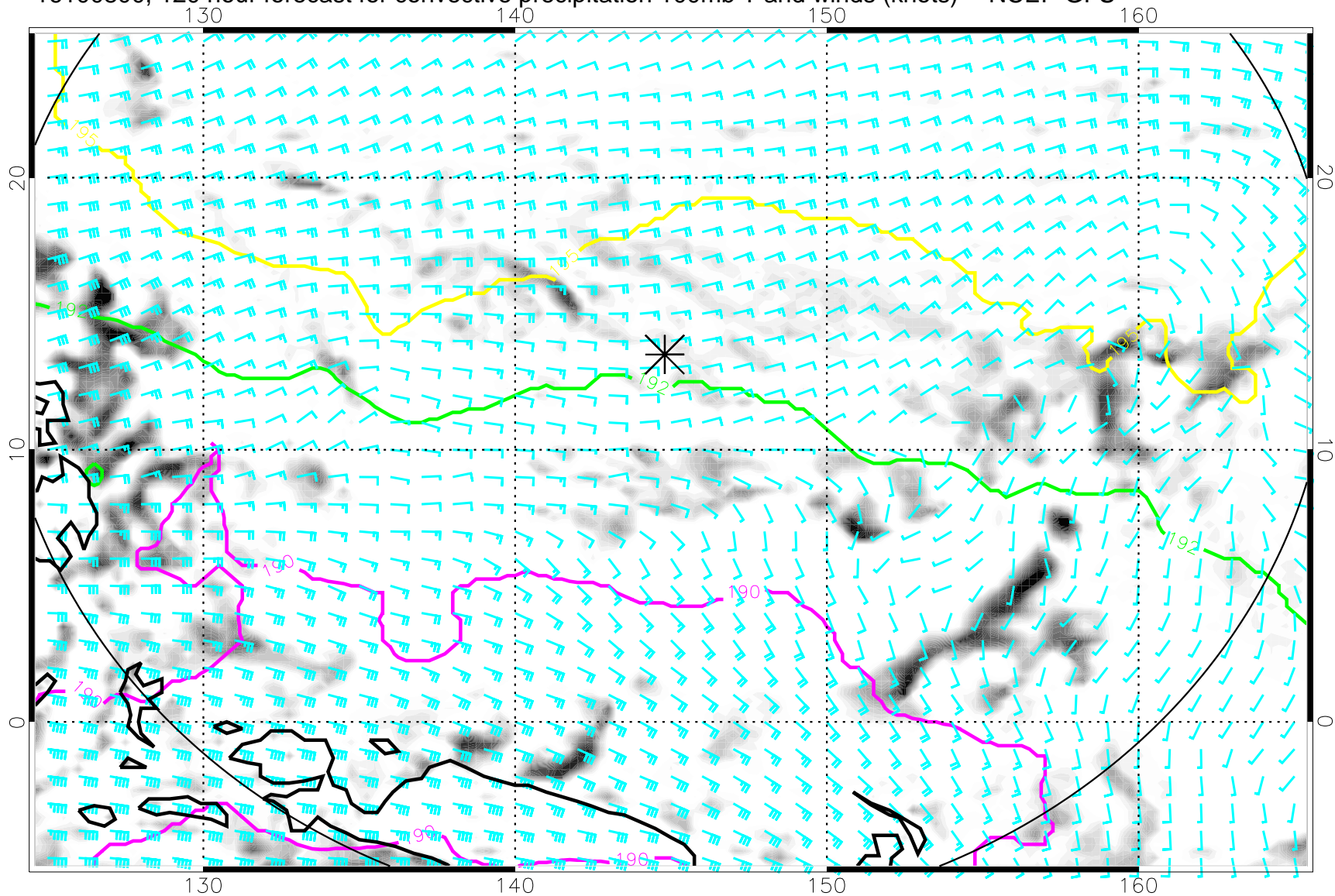
16100800, 120 hour forecast for convective precipitation 100mb T and winds (knots) -- NCEP GFS
