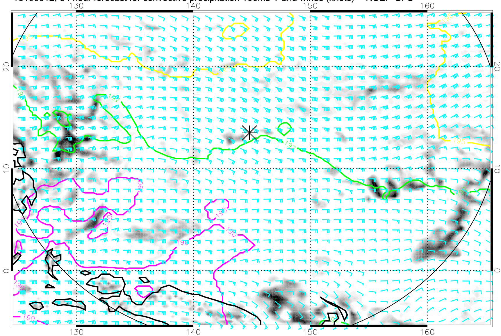
16100612, 84 hour forecast for convective precipitation 100mb T and winds (knots) -- NCEP GFS
