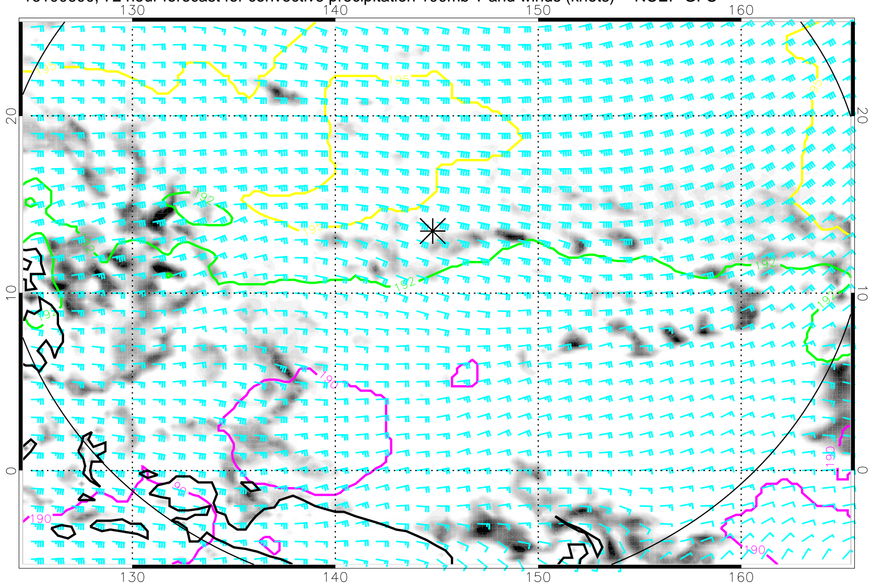
16100600, 72 hour forecast for convective precipitation 100mb T and winds (knots) -- NCEP GFS
