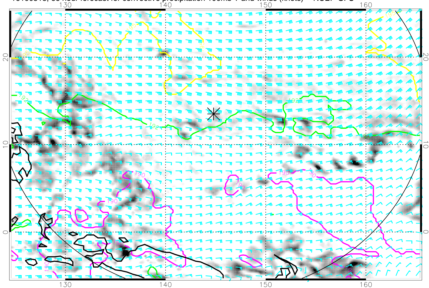
16100518, 66 hour forecast for convective precipitation 100mb T and winds (knots) -- NCEP GFS
