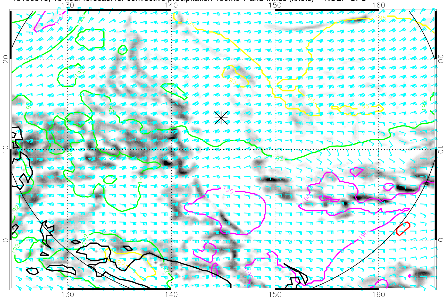
16100318, 18 hour forecast for convective precipitation 100mb T and winds (knots) -- NCEP GFS
