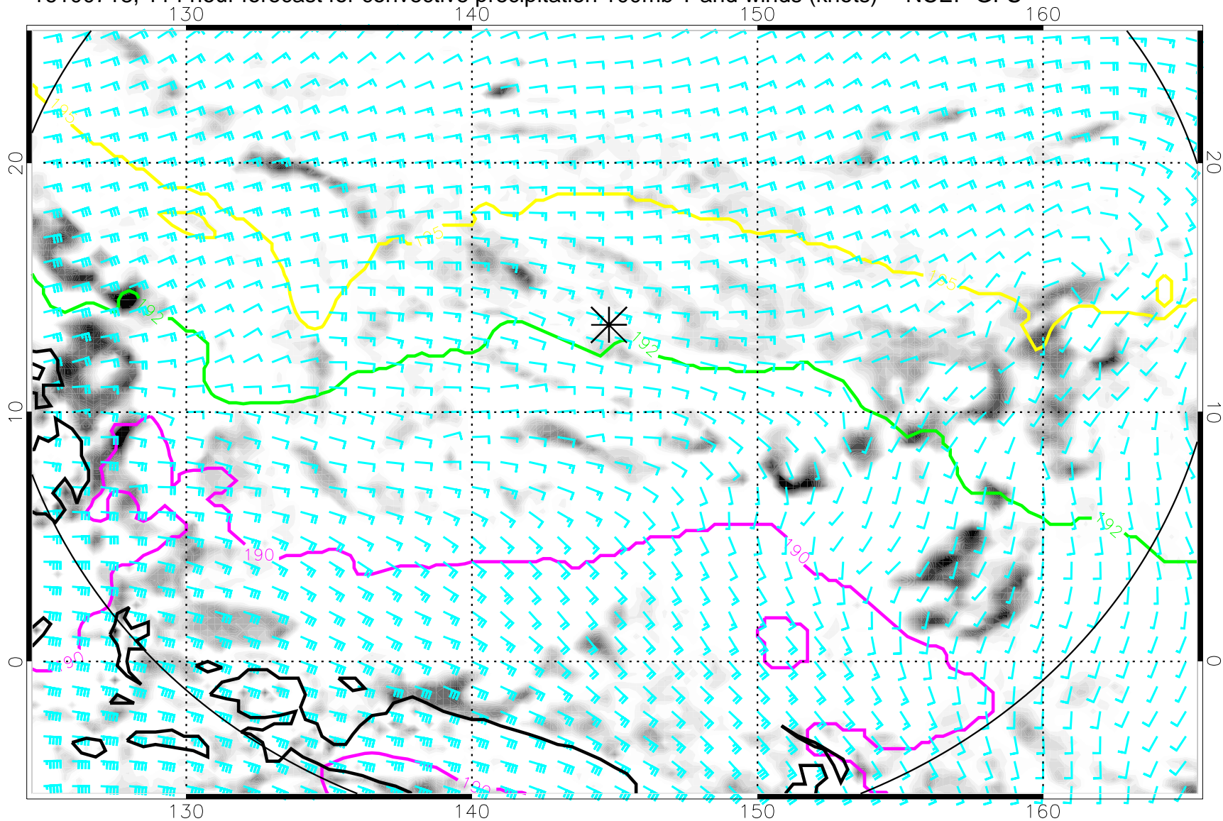
16100718, 114 hour forecast for convective precipitation 100mb T and winds (knots) -- NCEP GFS
