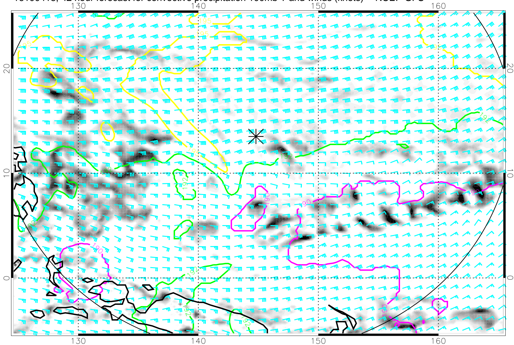
16100418, 42 hour forecast for convective precipitation 100mb T and winds (knots) -- NCEP GFS
