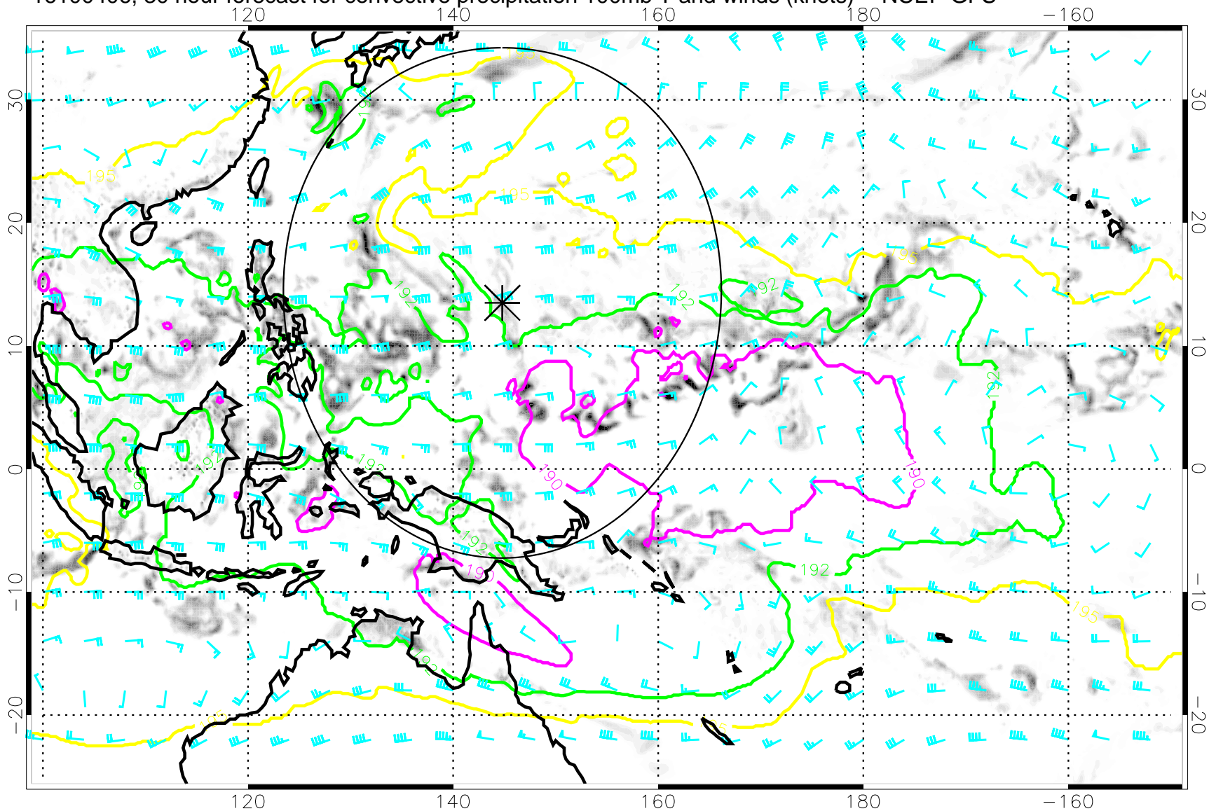
16100406, 30 hour forecast for convective precipitation 100mb T and winds (knots) -- NCEP GFS
