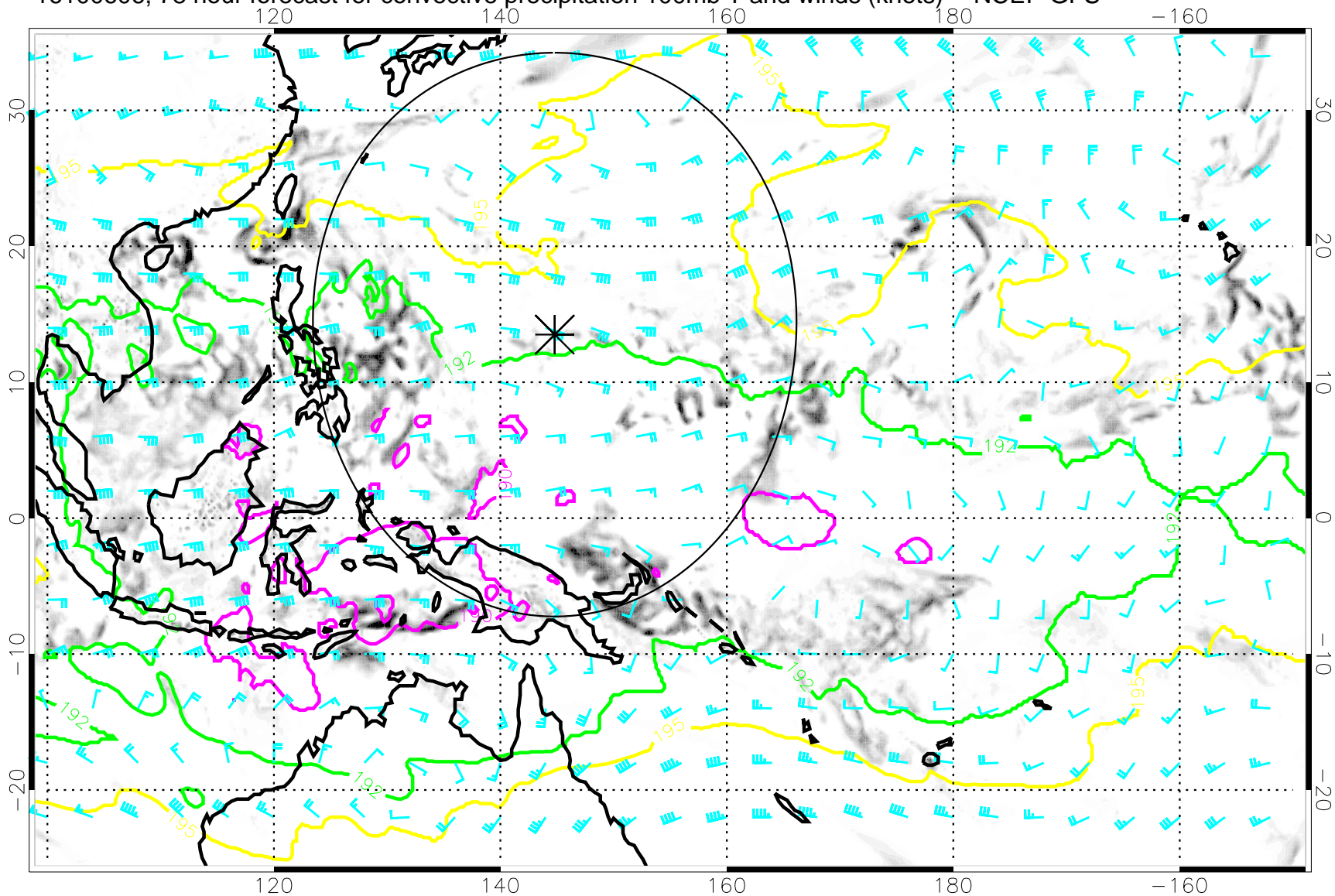
16100606, 78 hour forecast for convective precipitation 100mb T and winds (knots) -- NCEP GFS
