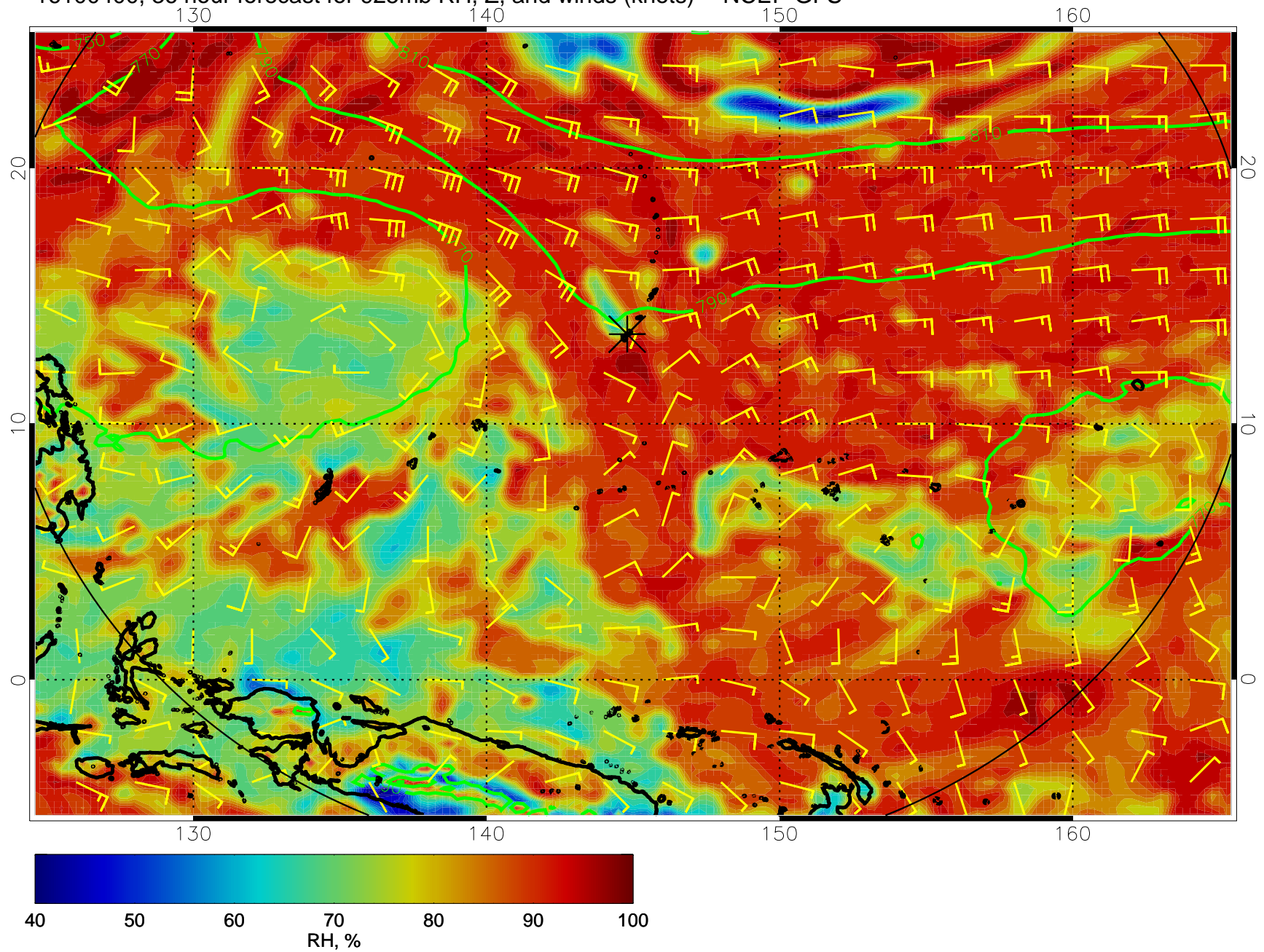
16100400, 36 hour forecast for 925mb RH, Z, and winds (knots) -- NCEP GFS
