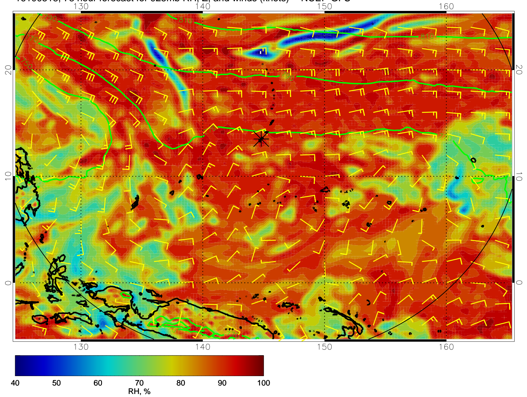
16100518, 78 hour forecast for 925mb RH, Z, and winds (knots) -- NCEP GFS
