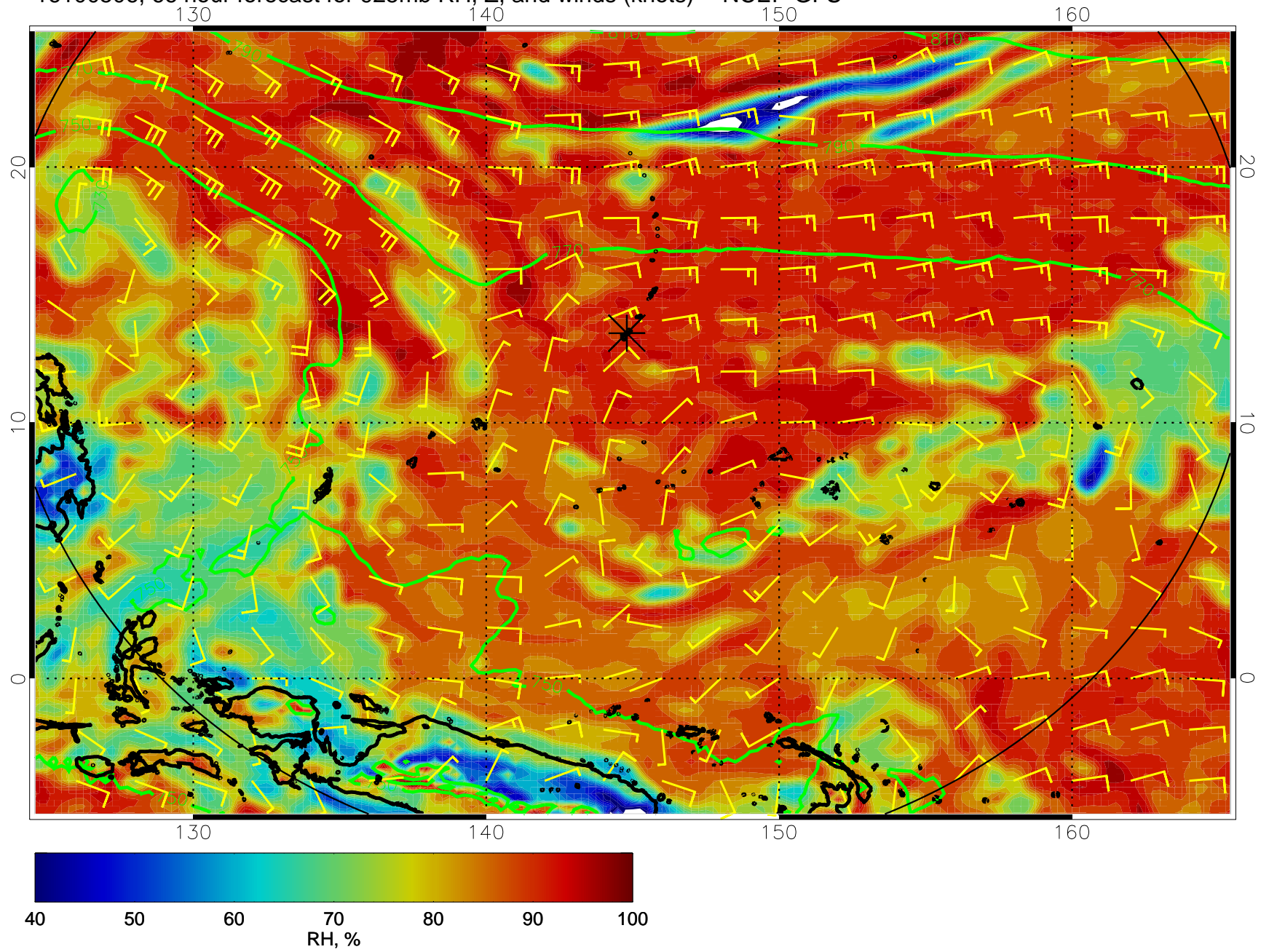
16100506, 66 hour forecast for 925mb RH, Z, and winds (knots) -- NCEP GFS
