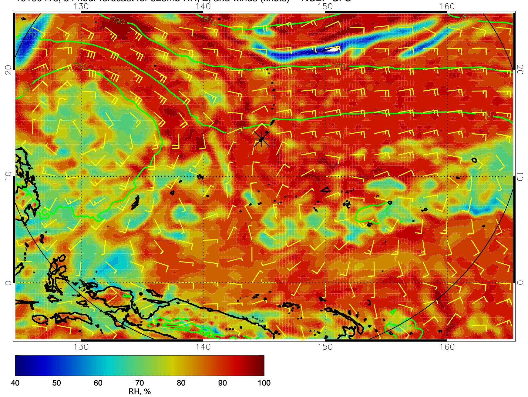
16100418, 54 hour forecast for 925mb RH, Z, and winds (knots) -- NCEP GFS
