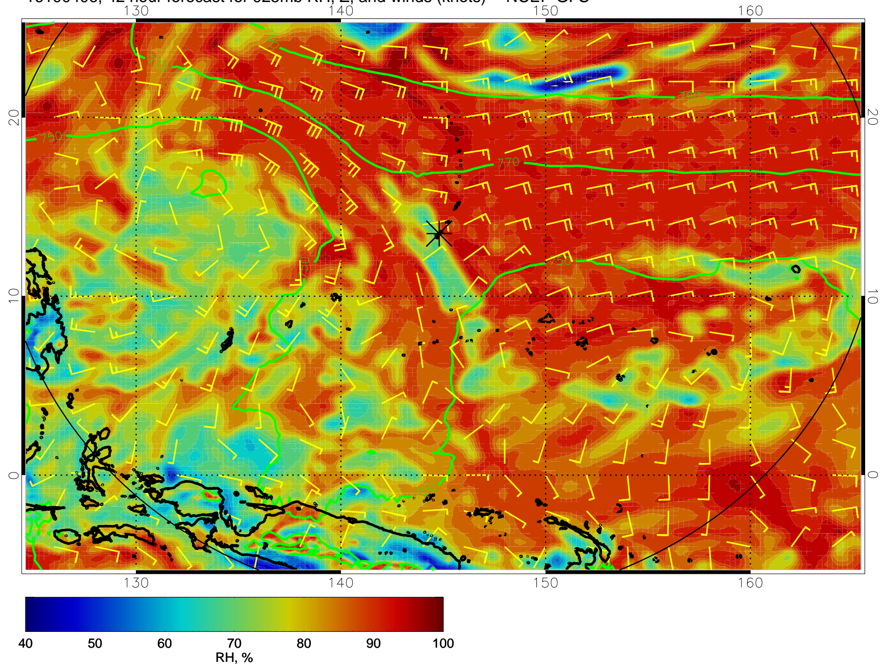
16100406, 42 hour forecast for 925mb RH, Z, and winds (knots) -- NCEP GFS
