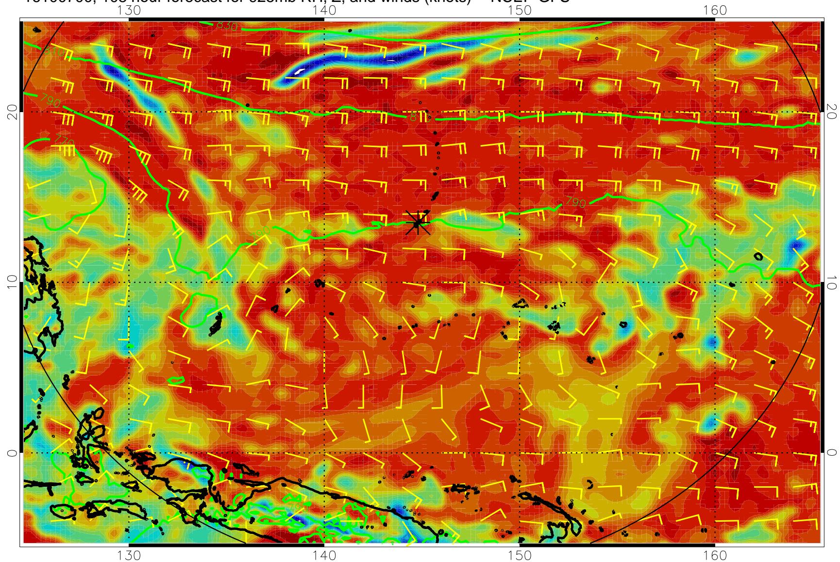
16100700, 108 hour forecast for 925mb RH, Z, and winds (knots) -- NCEP GFS
