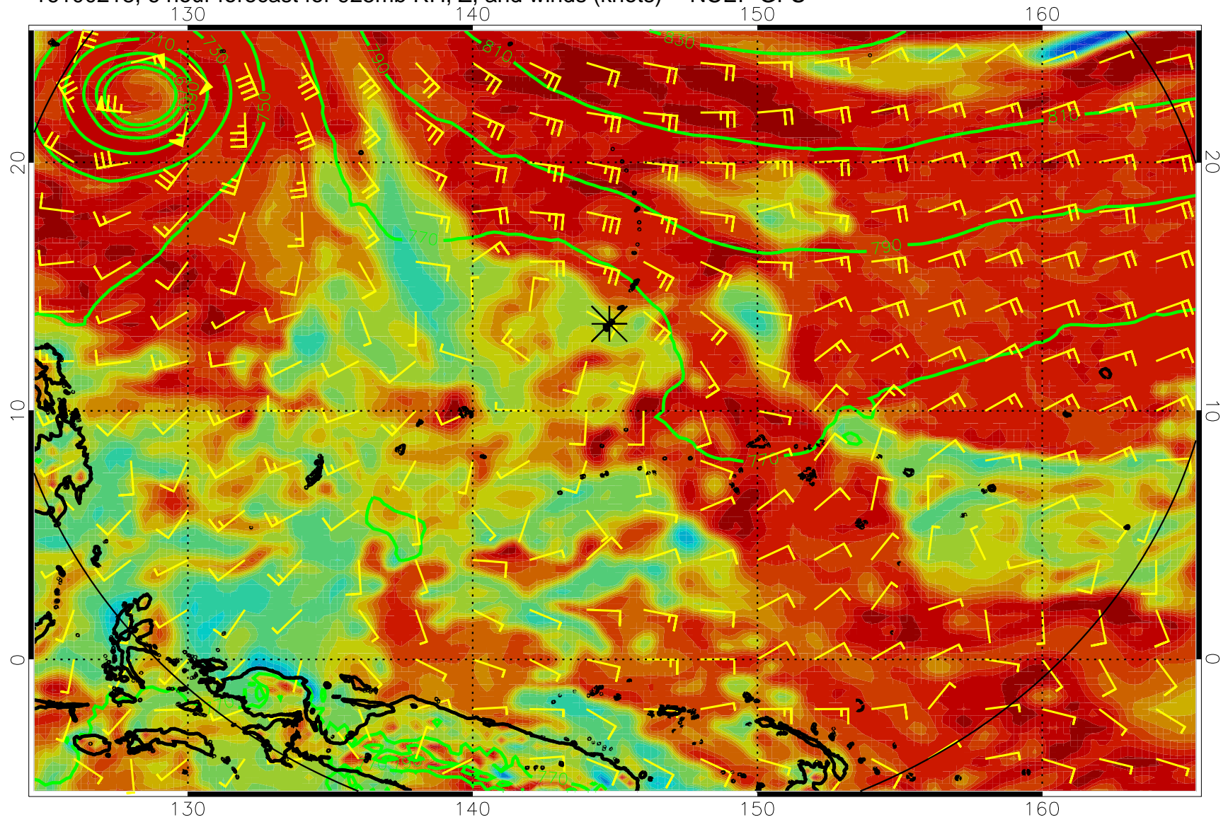
16100218, 6 hour forecast for 925mb RH, Z, and winds (knots) -- NCEP GFS
