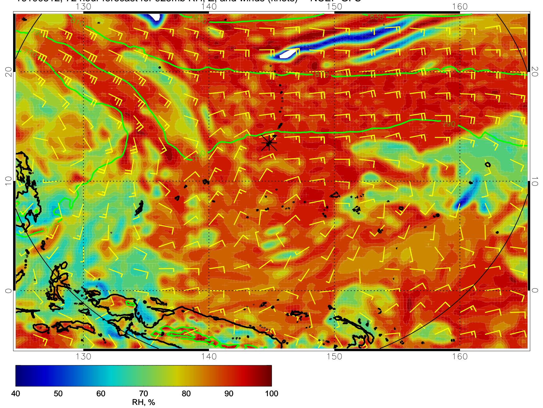
16100512, 72 hour forecast for 925mb RH, Z, and winds (knots) -- NCEP GFS
