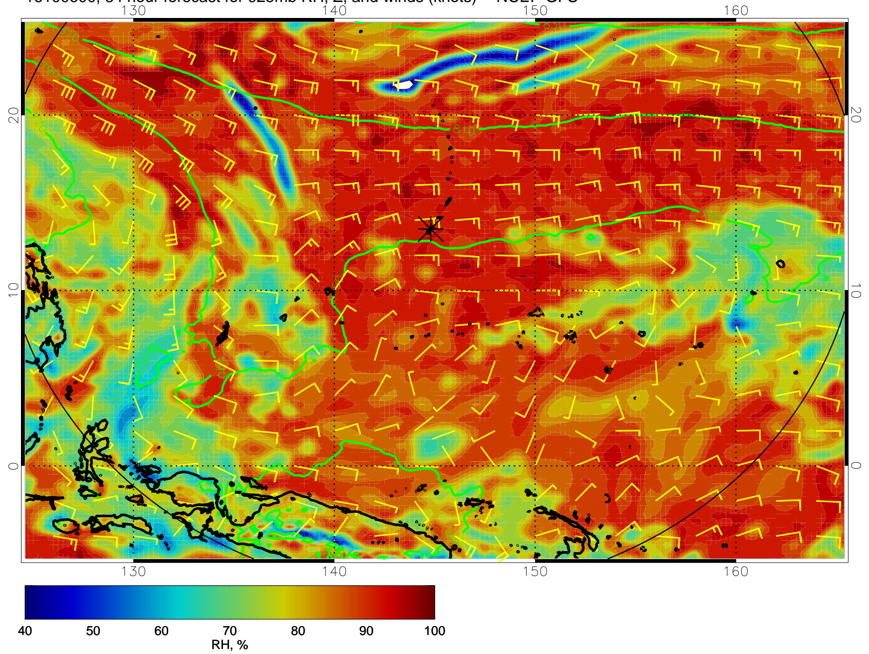
16100600, 84 hour forecast for 925mb RH, Z, and winds (knots) -- NCEP GFS
