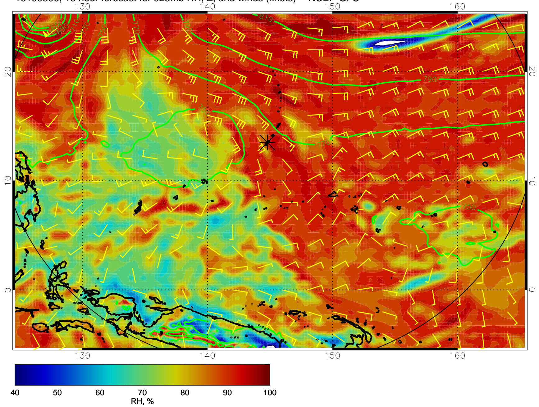
16100306, 18 hour forecast for 925mb RH, Z, and winds (knots) -- NCEP GFS
