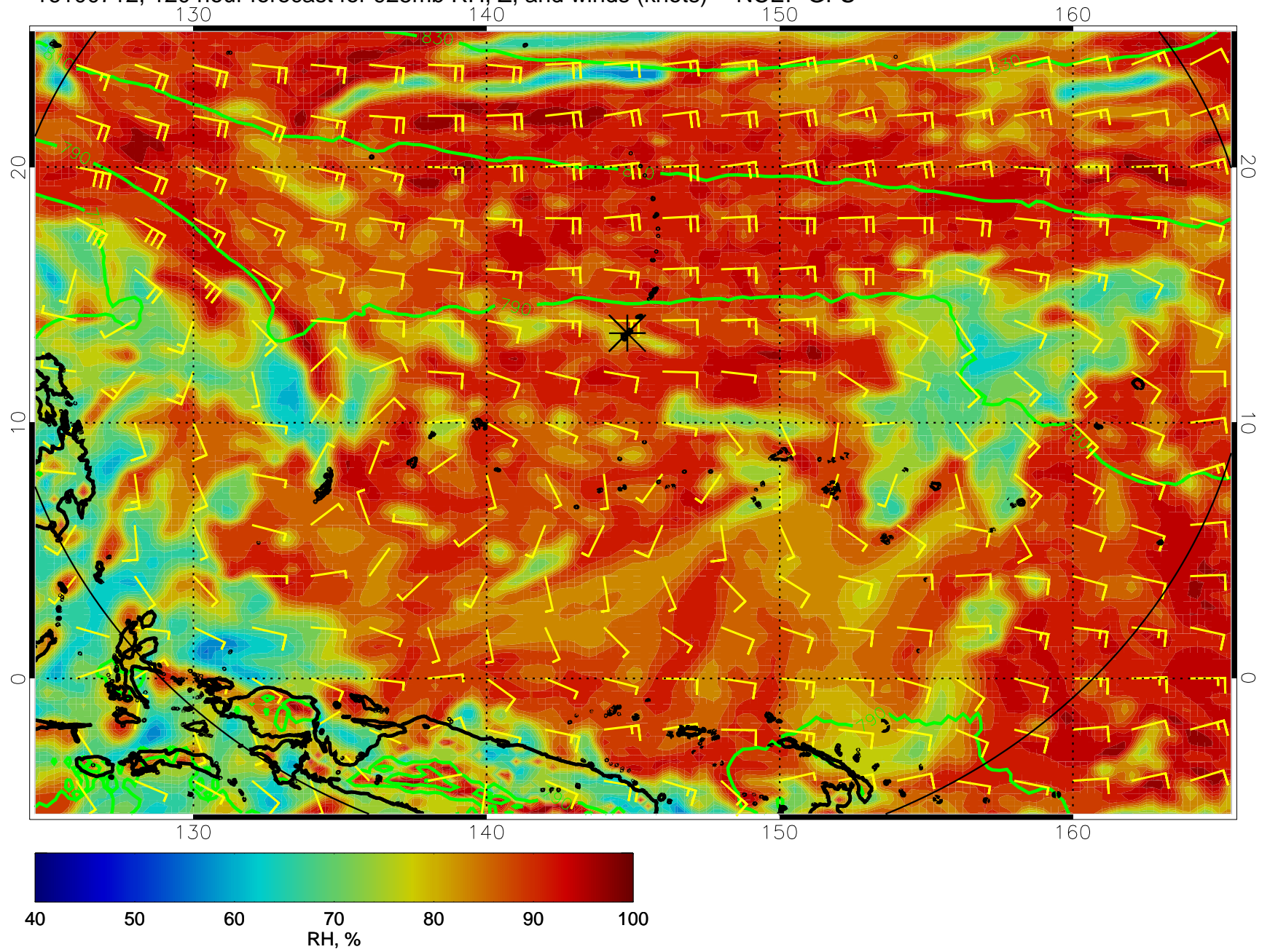
16100712, 120 hour forecast for 925mb RH, Z, and winds (knots) -- NCEP GFS
