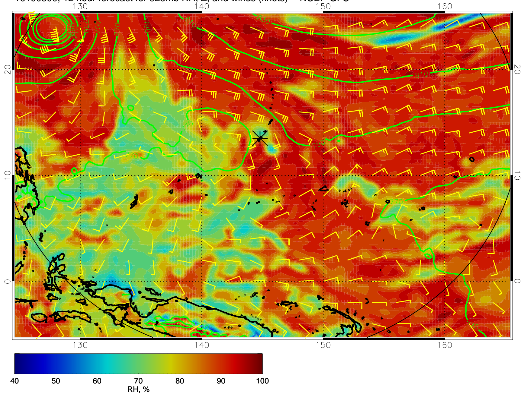
16100300, 12 hour forecast for 925mb RH, Z, and winds (knots) -- NCEP GFS
