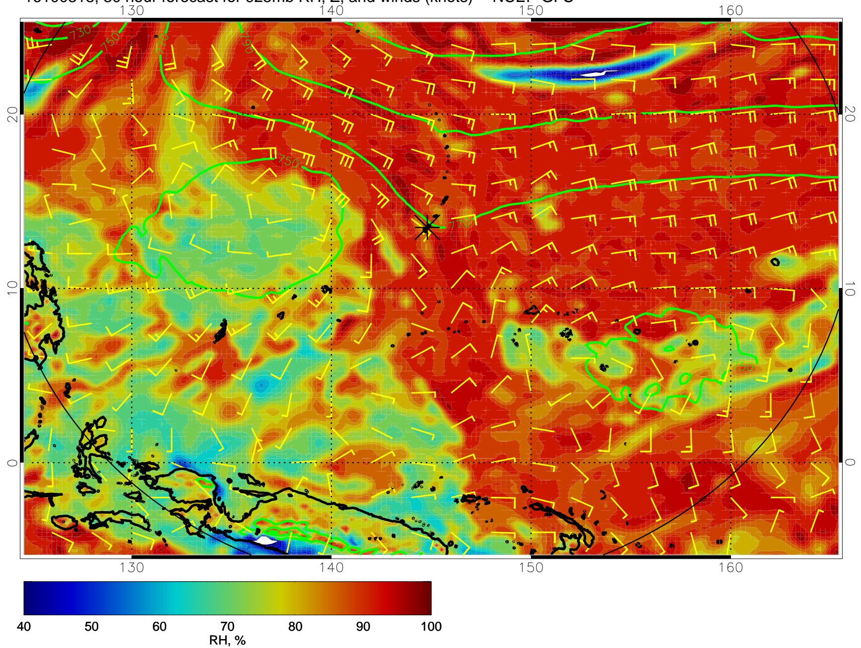
16100318, 30 hour forecast for 925mb RH, Z, and winds (knots) -- NCEP GFS
