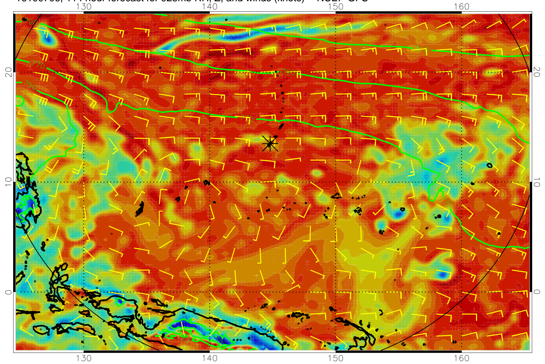
16100706, 114 hour forecast for 925mb RH, Z, and winds (knots) -- NCEP GFS
