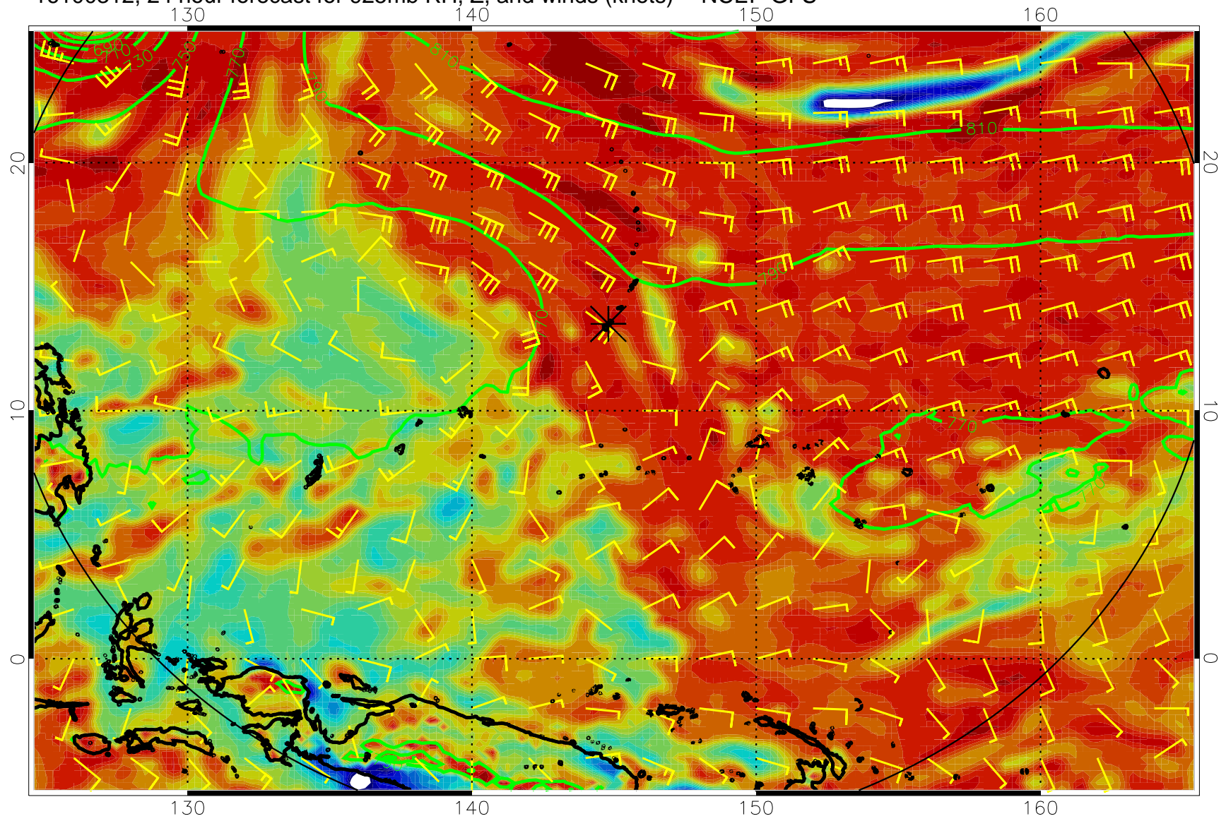
16100312, 24 hour forecast for 925mb RH, Z, and winds (knots) -- NCEP GFS
