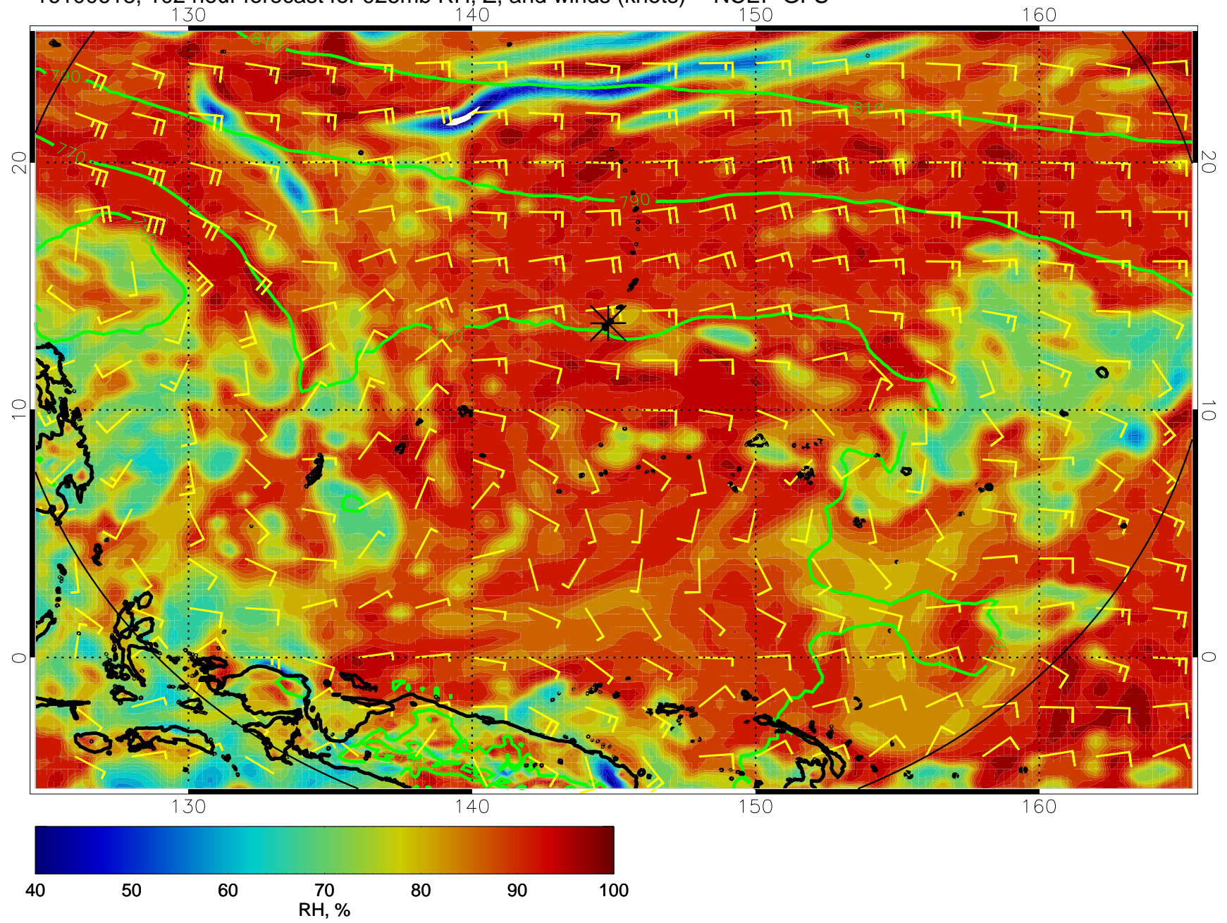
16100618, 102 hour forecast for 925mb RH, Z, and winds (knots) -- NCEP GFS
