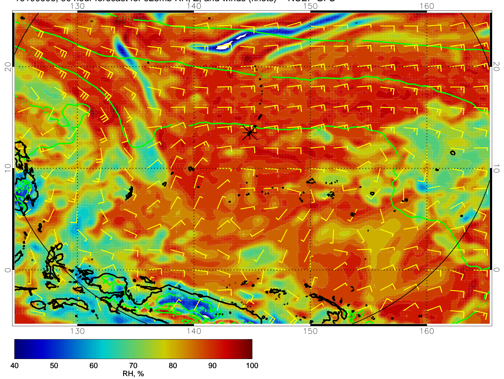
16100606, 90 hour forecast for 925mb RH, Z, and winds (knots) -- NCEP GFS
