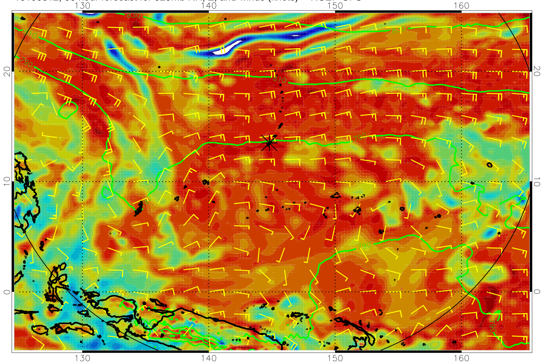
16100612, 96 hour forecast for 925mb RH, Z, and winds (knots) -- NCEP GFS
