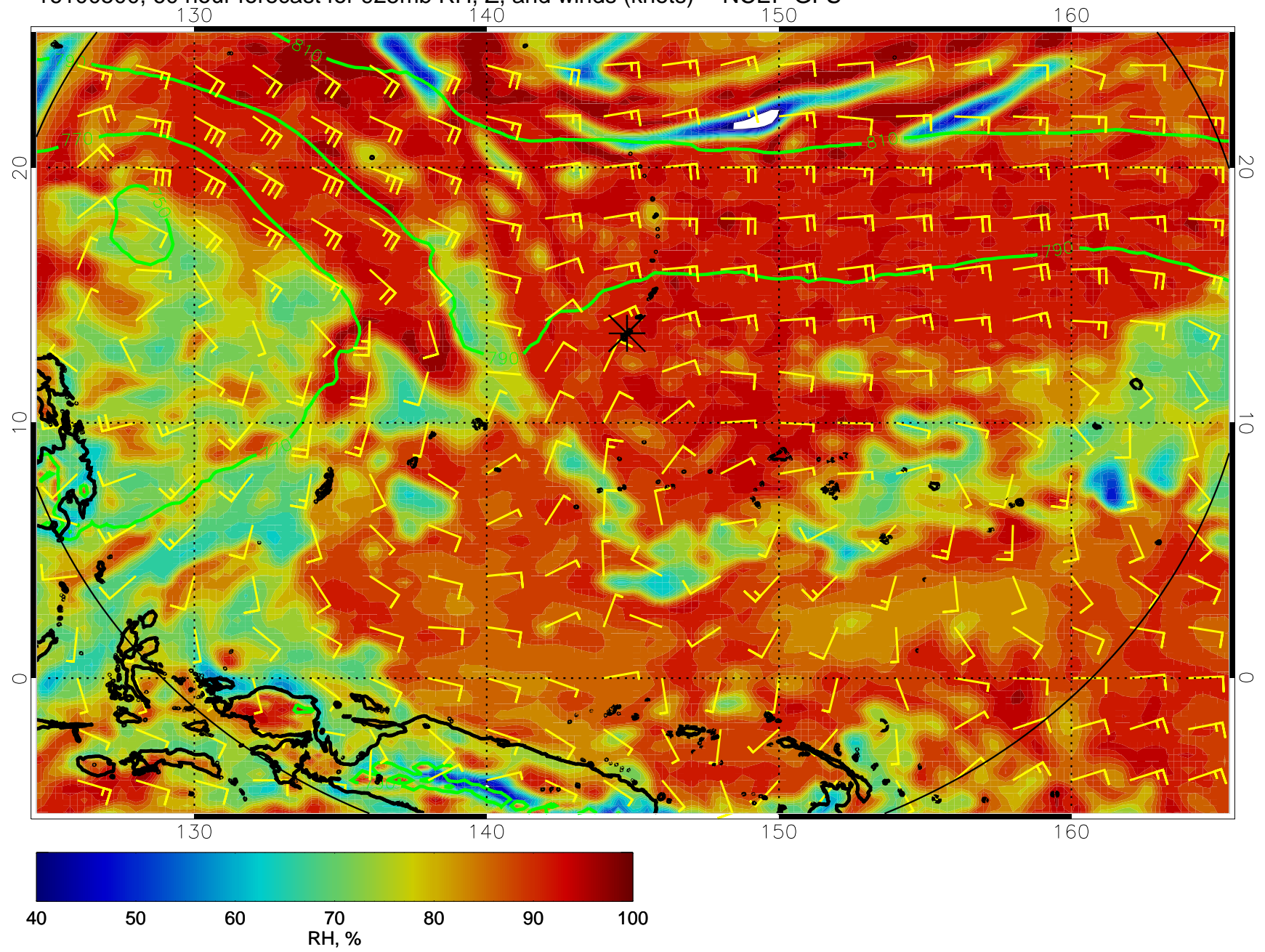
16100500, 60 hour forecast for 925mb RH, Z, and winds (knots) -- NCEP GFS
