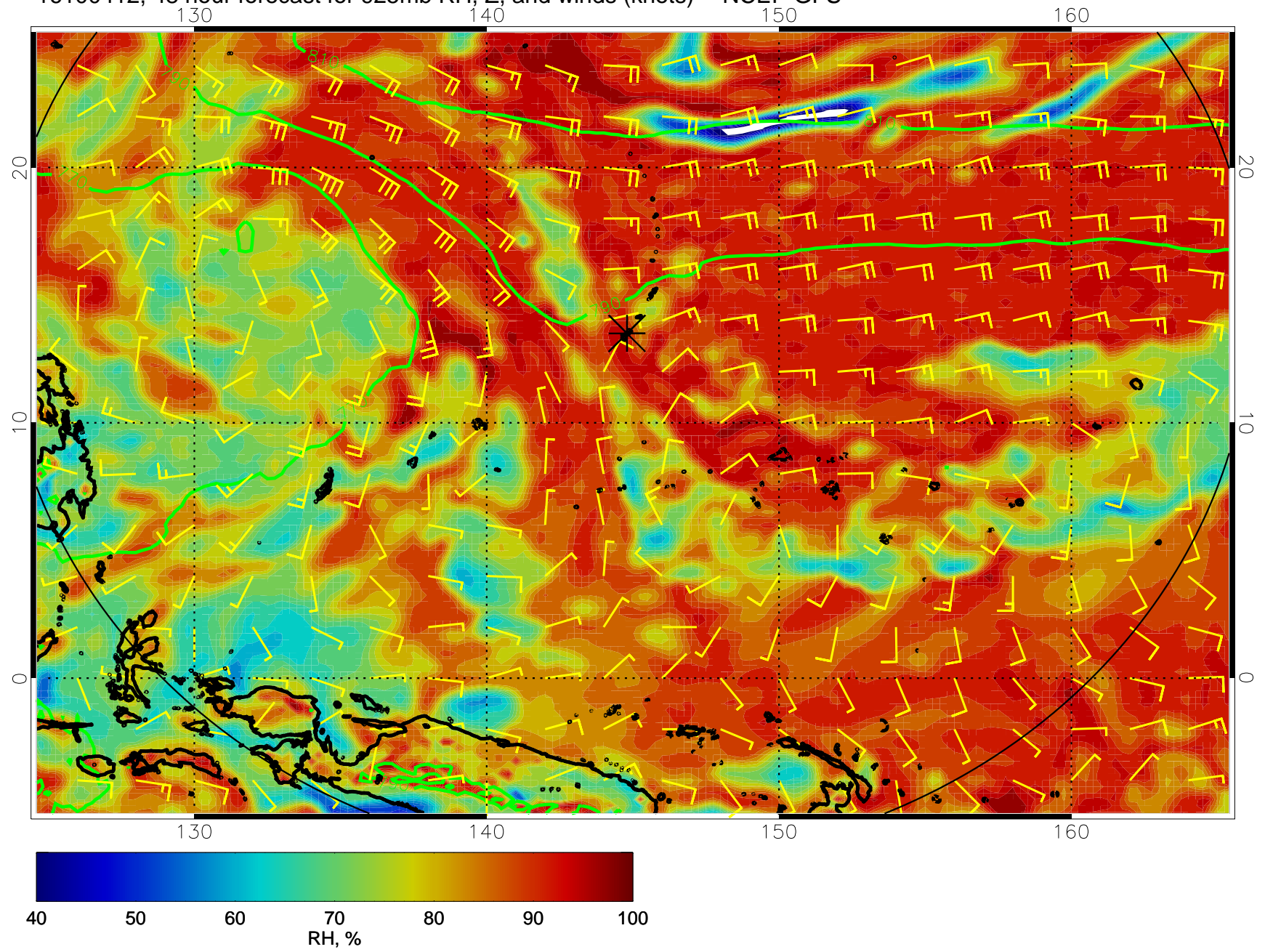
16100412, 48 hour forecast for 925mb RH, Z, and winds (knots) -- NCEP GFS
