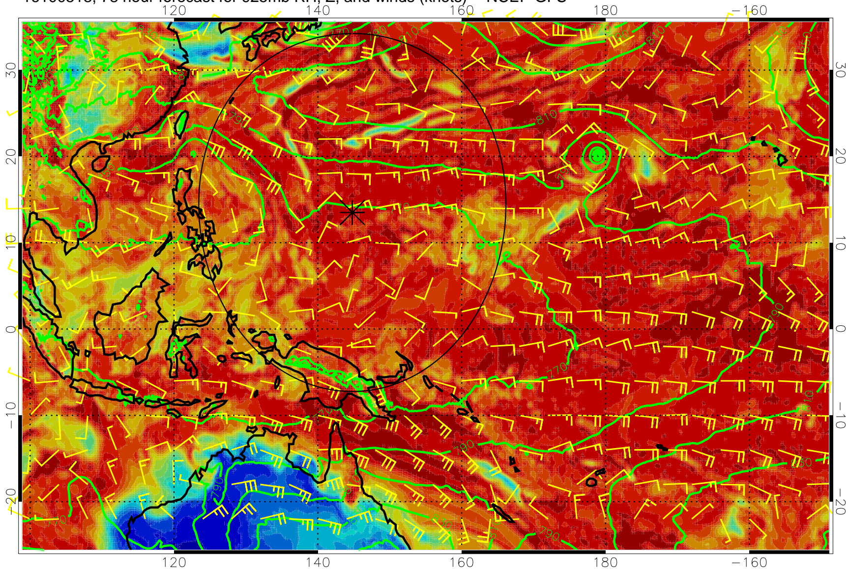
16100518, 78 hour forecast for 925mb RH, Z, and winds (knots) -- NCEP GFS
