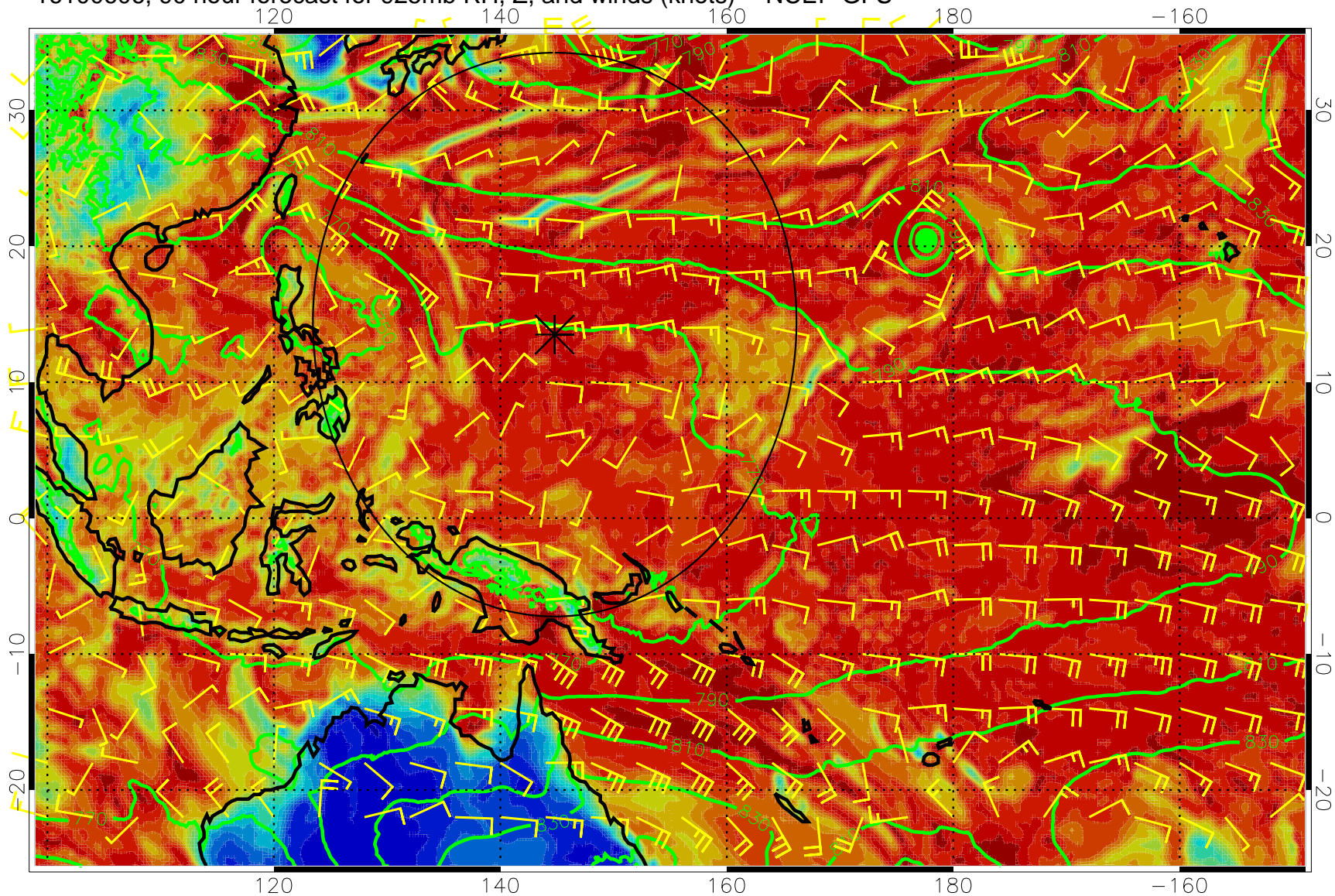
16100606, 90 hour forecast for 925mb RH, Z, and winds (knots) -- NCEP GFS
