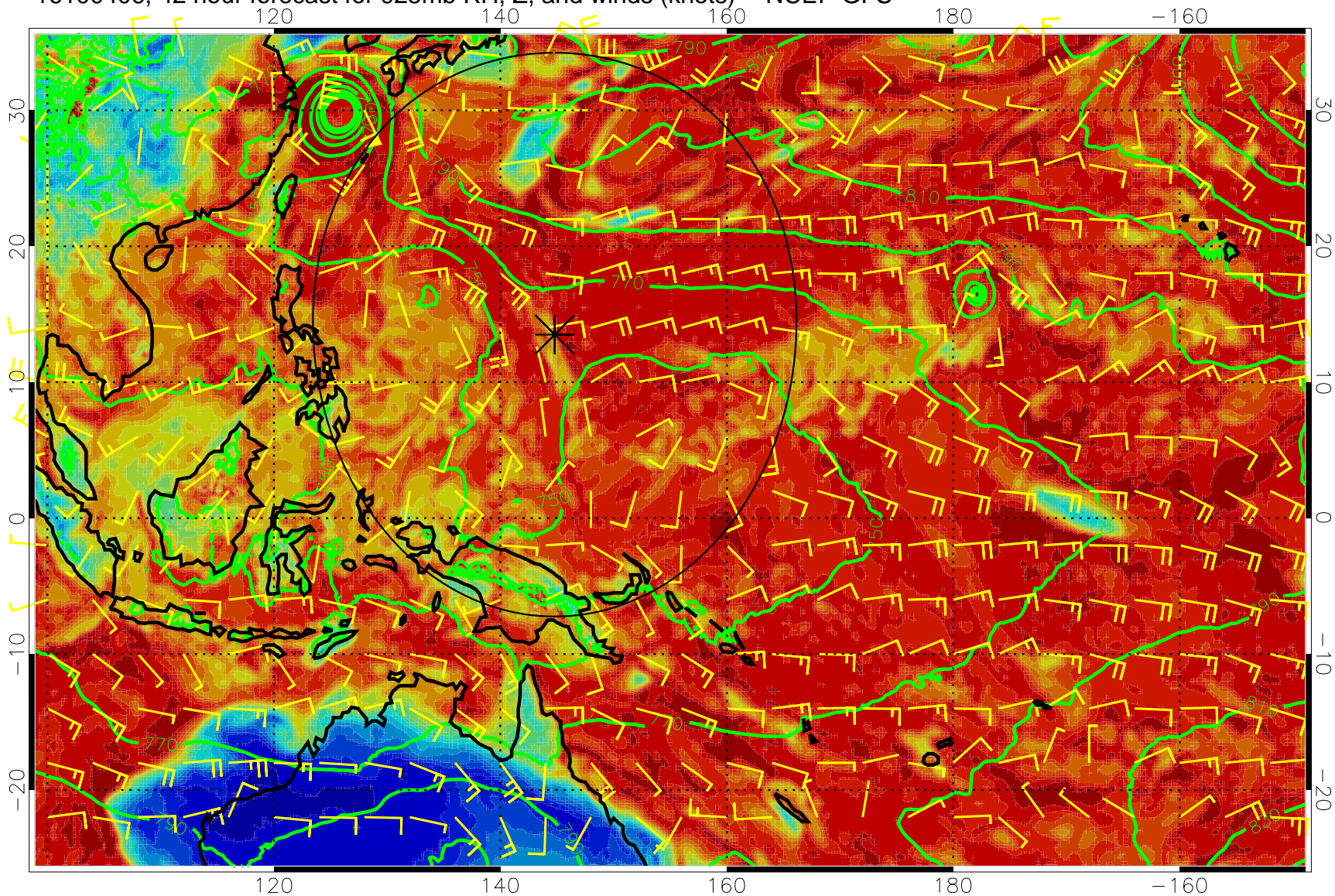
16100406, 42 hour forecast for 925mb RH, Z, and winds (knots) -- NCEP GFS
