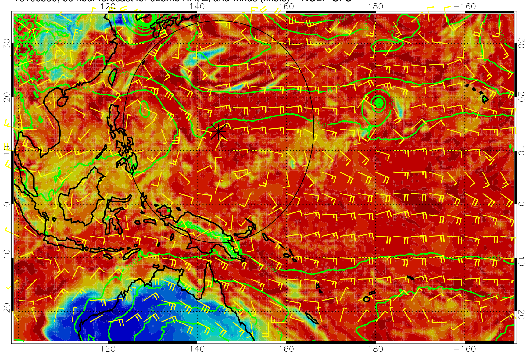
16100500, 60 hour forecast for 925mb RH, Z, and winds (knots) -- NCEP GFS
