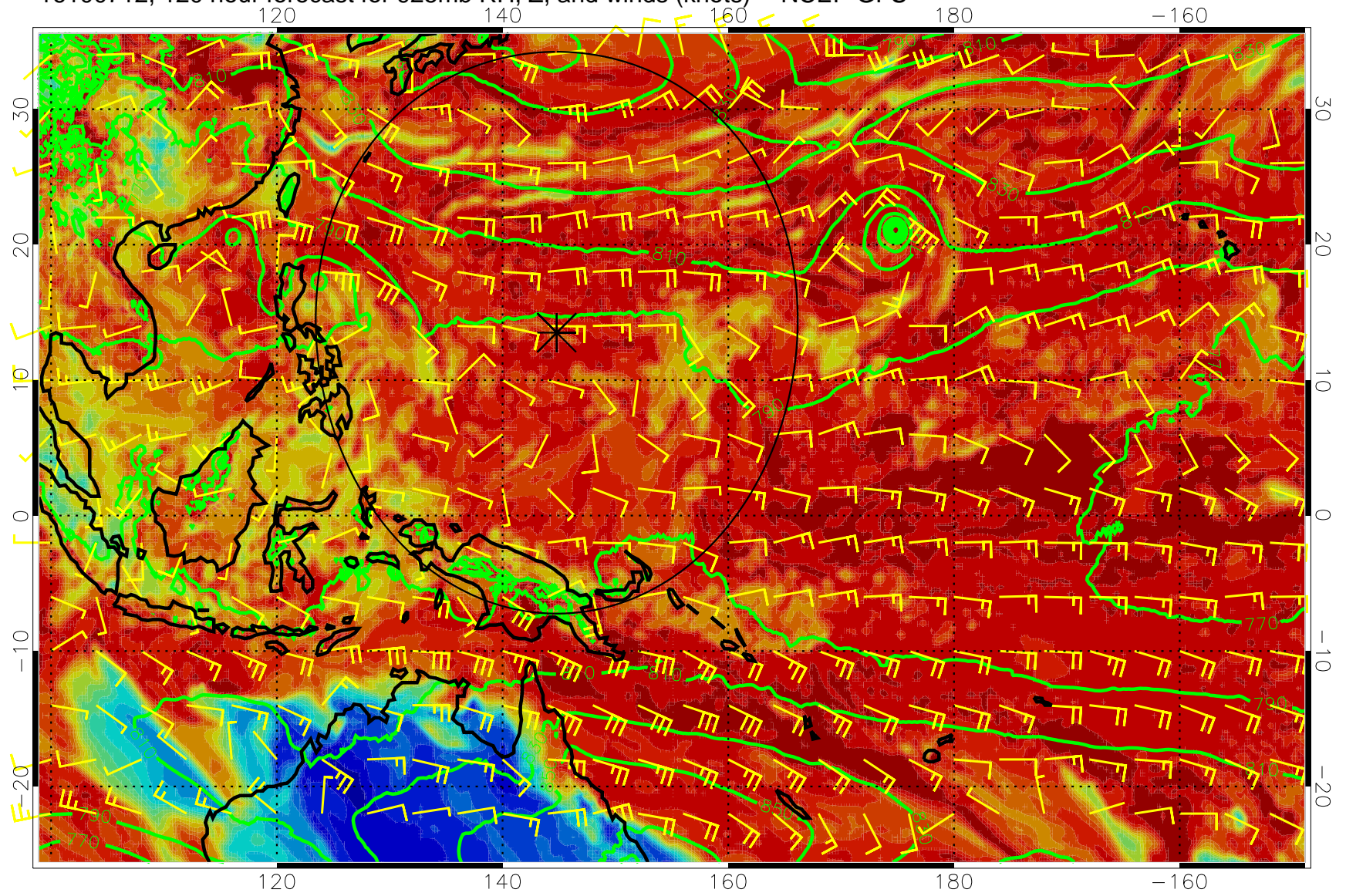
16100712, 120 hour forecast for 925mb RH, Z, and winds (knots) -- NCEP GFS
