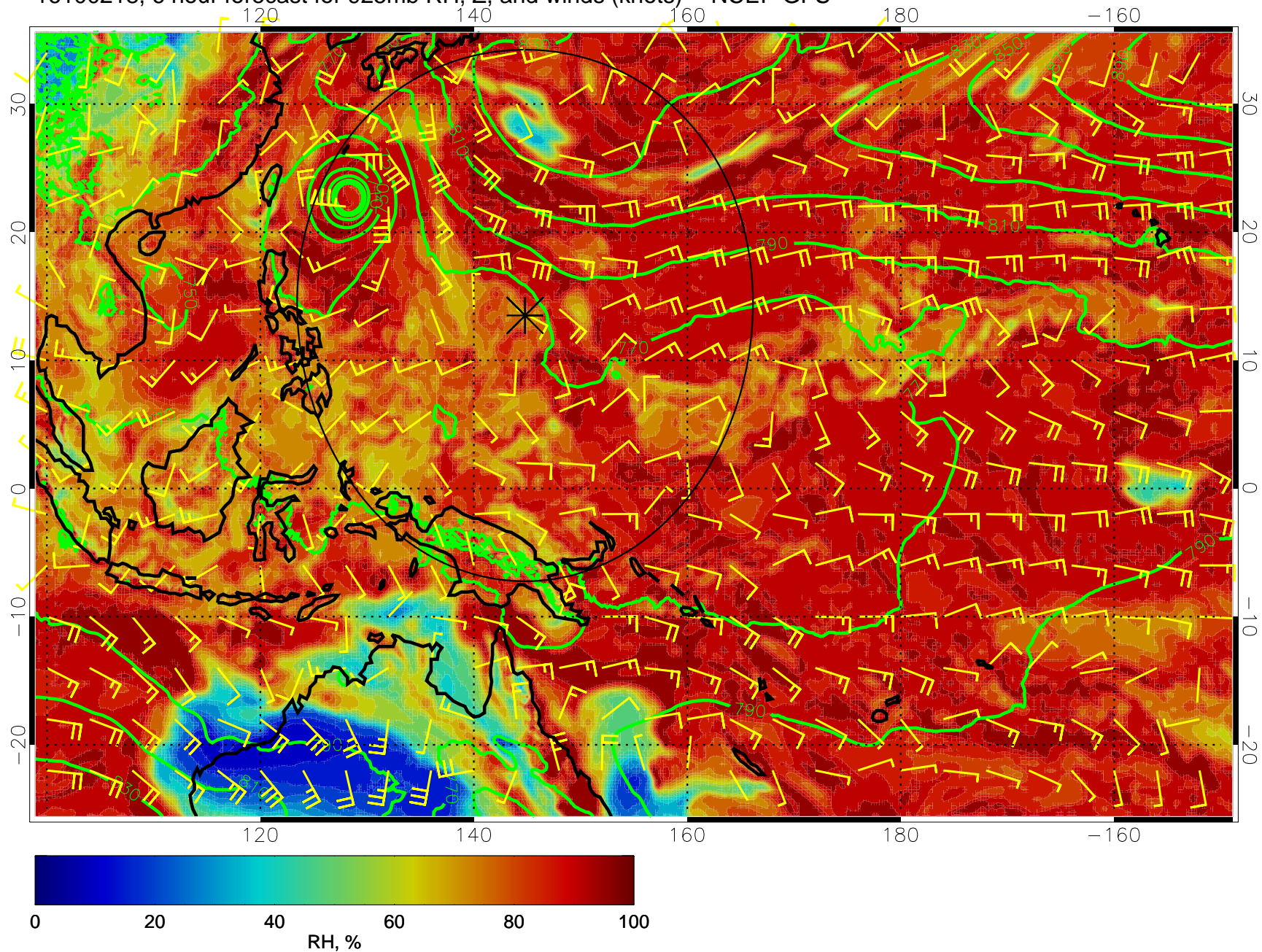
16100218, 6 hour forecast for 925mb RH, Z, and winds (knots) -- NCEP GFS
