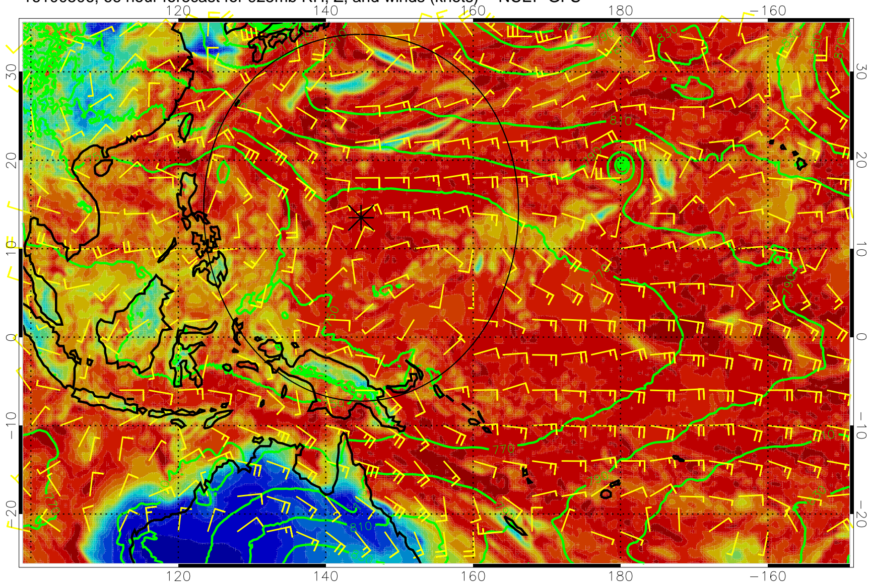
16100506, 66 hour forecast for 925mb RH, Z, and winds (knots) -- NCEP GFS
