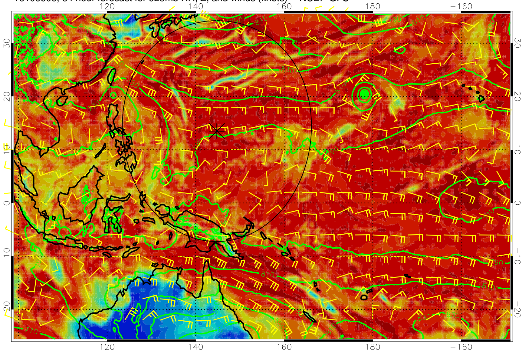
16100600, 84 hour forecast for 925mb RH, Z, and winds (knots) -- NCEP GFS
