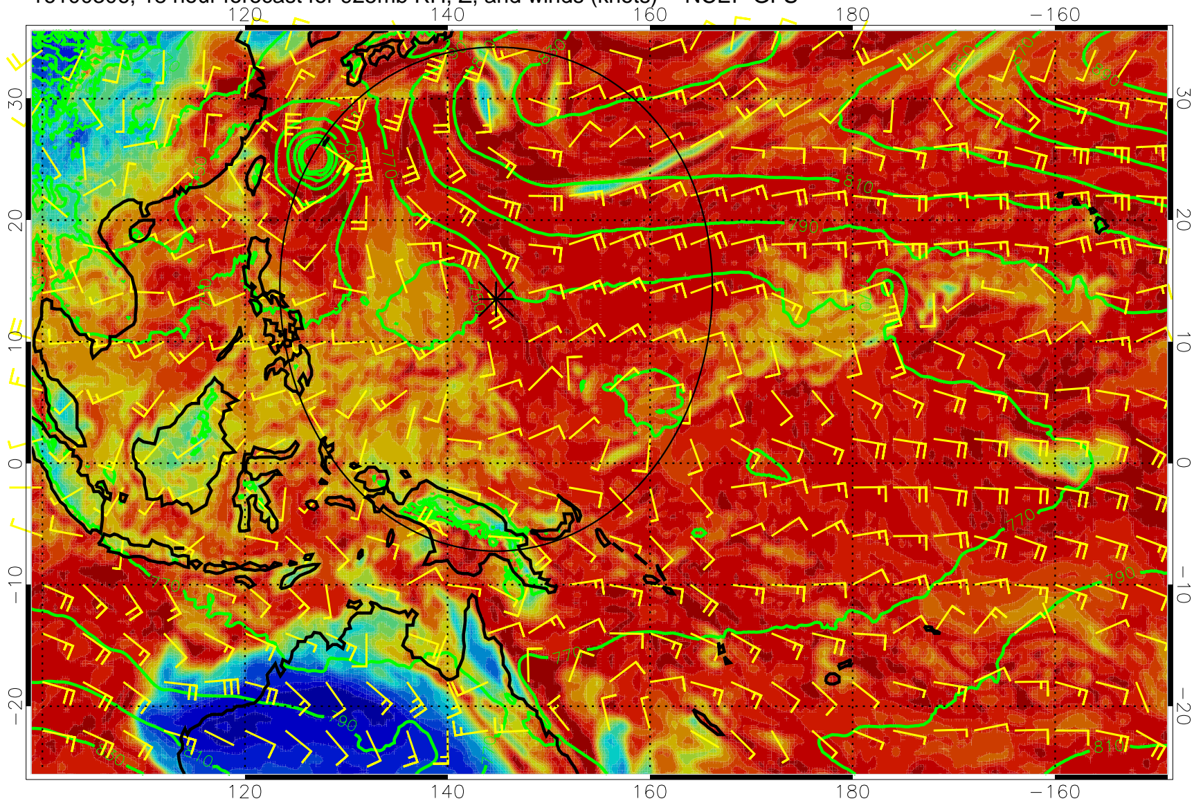
16100306, 18 hour forecast for 925mb RH, Z, and winds (knots) -- NCEP GFS
