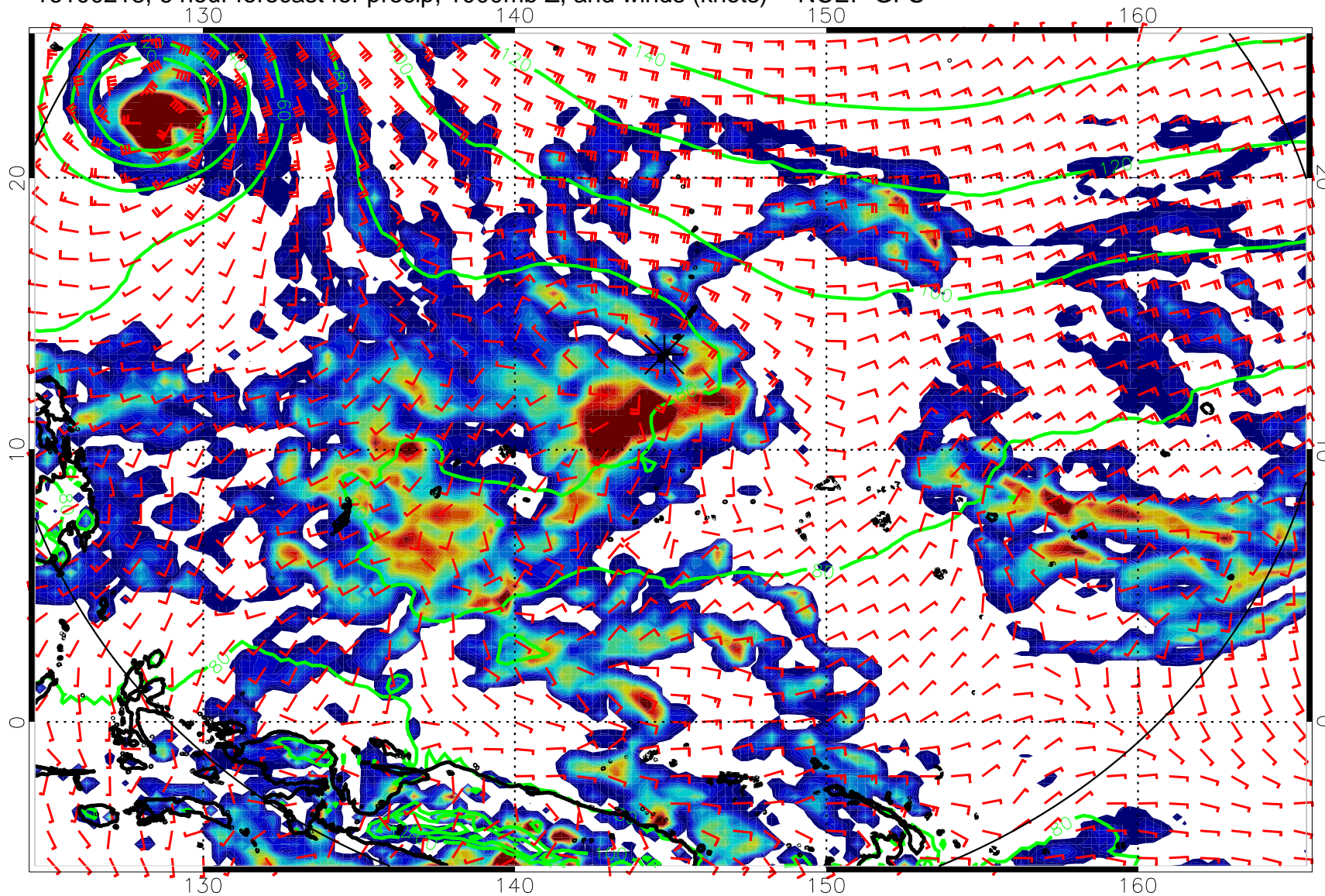
16100218, 6 hour forecast for precip, 1000mb Z, and winds (knots) -- NCEP GFS
