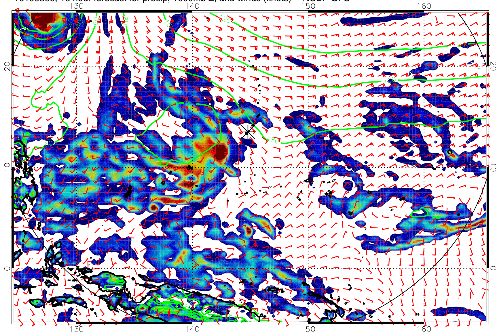
16100306, 18 hour forecast for precip, 1000mb Z, and winds (knots) -- NCEP GFS
