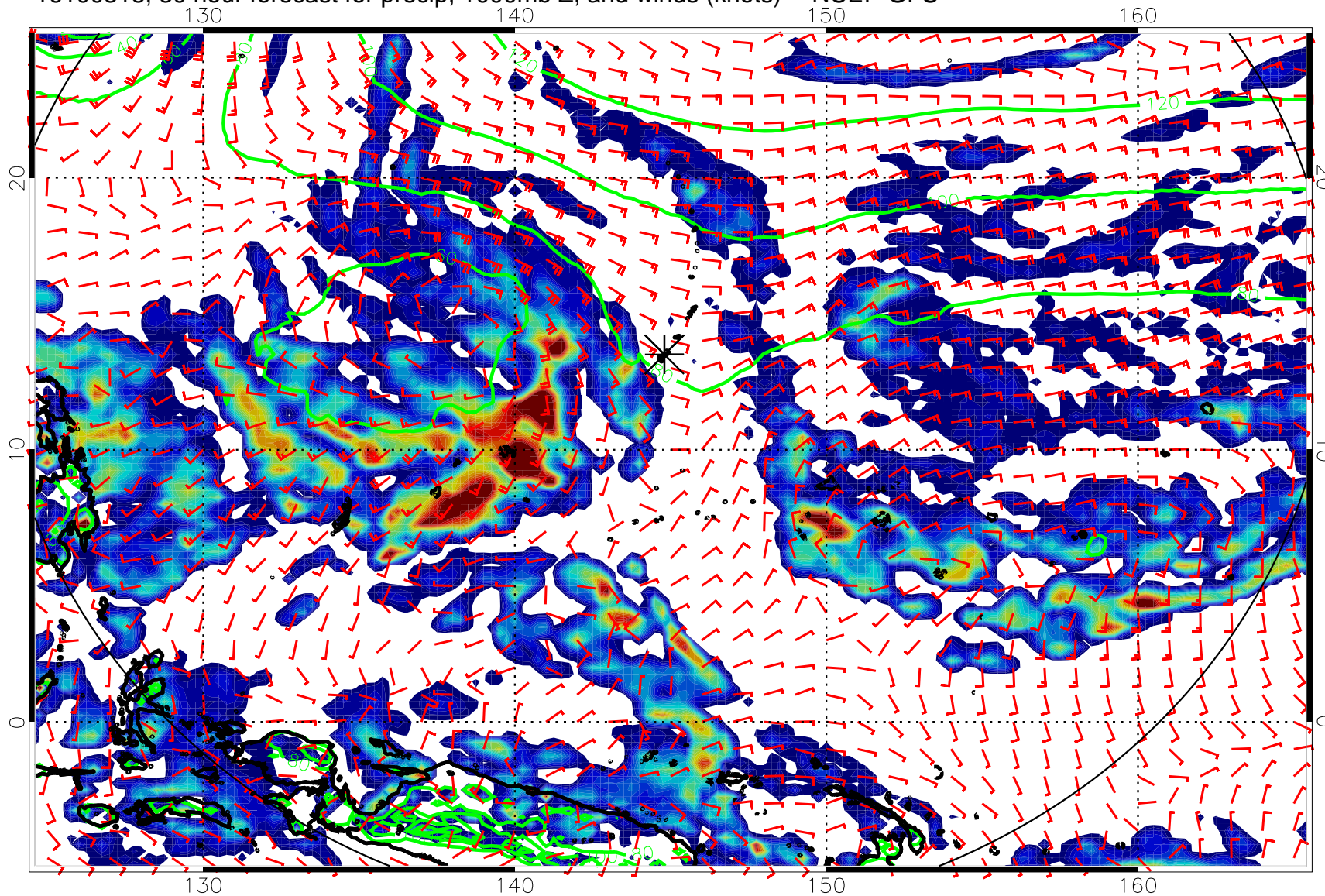
16100318, 30 hour forecast for precip, 1000mb Z, and winds (knots) -- NCEP GFS
