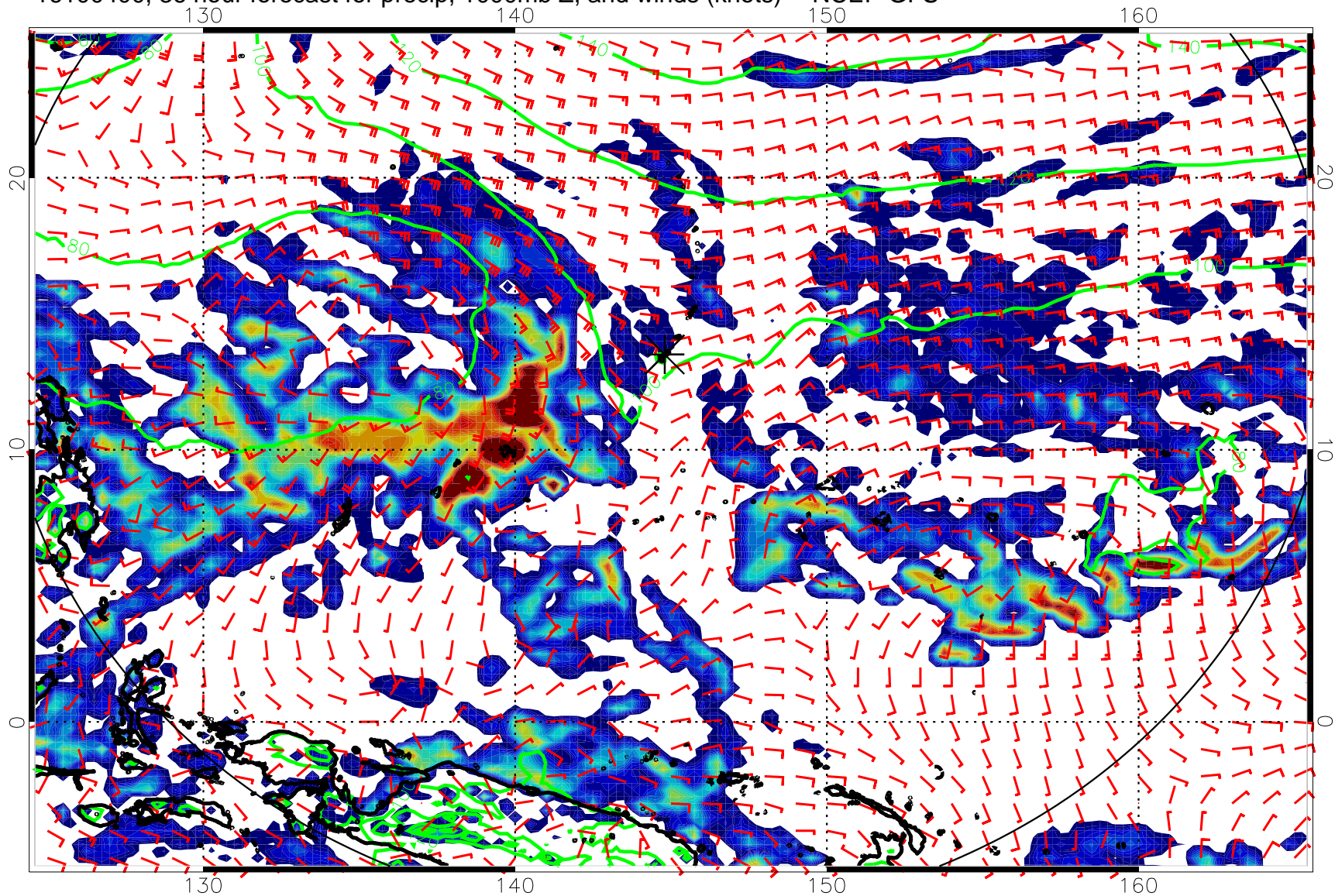
16100400, 36 hour forecast for precip, 1000mb Z, and winds (knots) -- NCEP GFS
