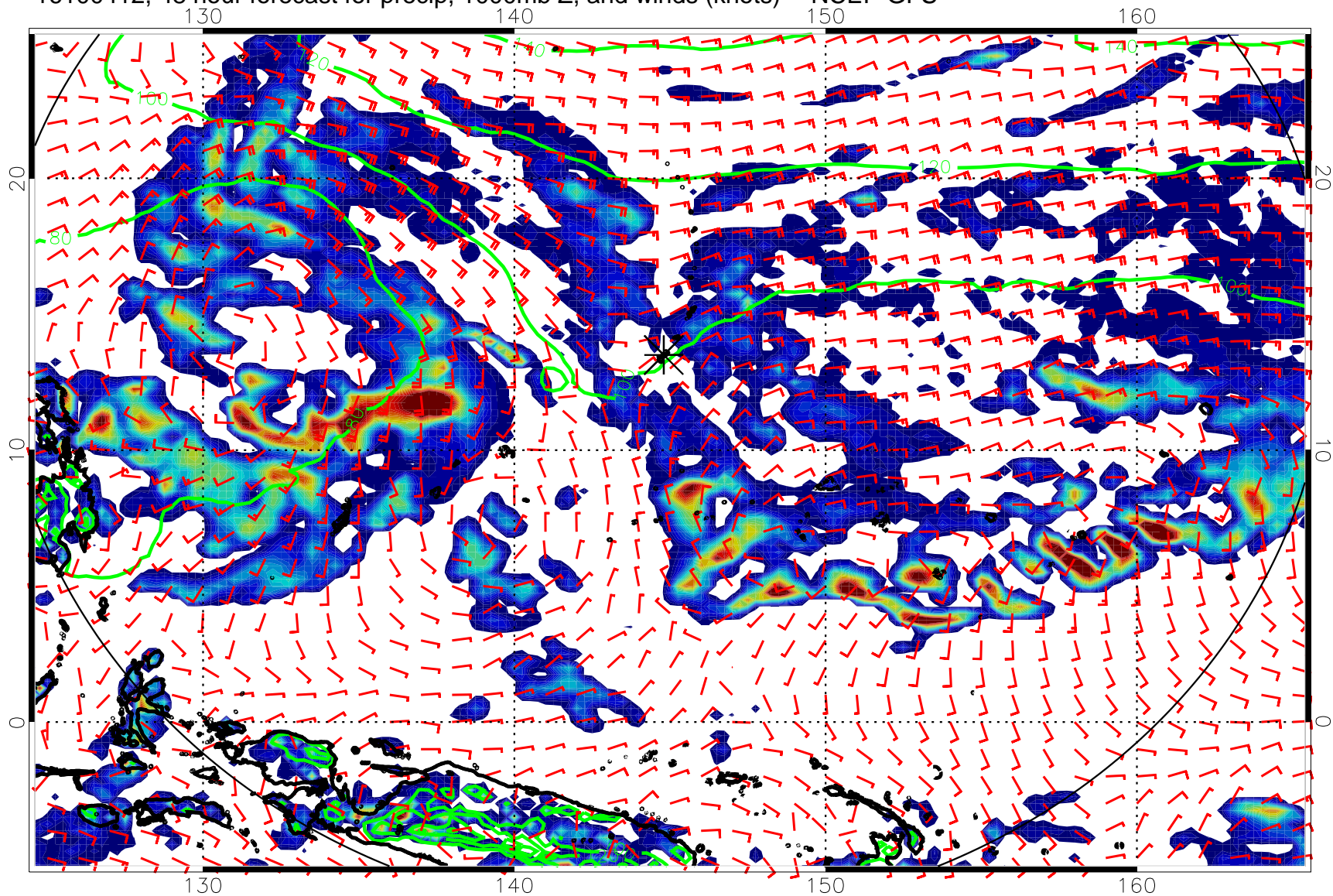
16100412, 48 hour forecast for precip, 1000mb Z, and winds (knots) -- NCEP GFS
