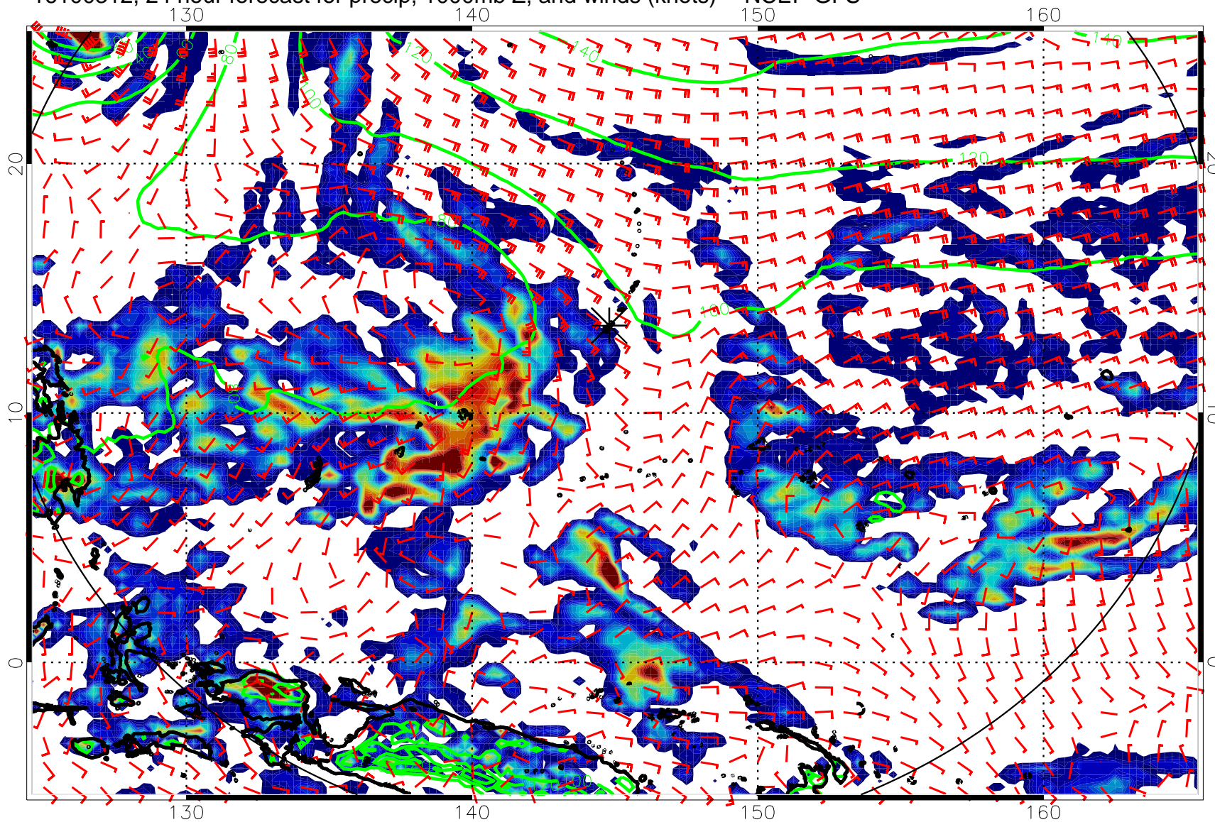
16100312, 24 hour forecast for precip, 1000mb Z, and winds (knots) -- NCEP GFS
