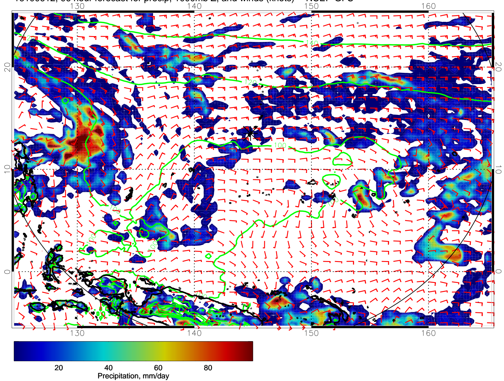
16100612, 96 hour forecast for precip, 1000mb Z, and winds (knots) -- NCEP GFS
