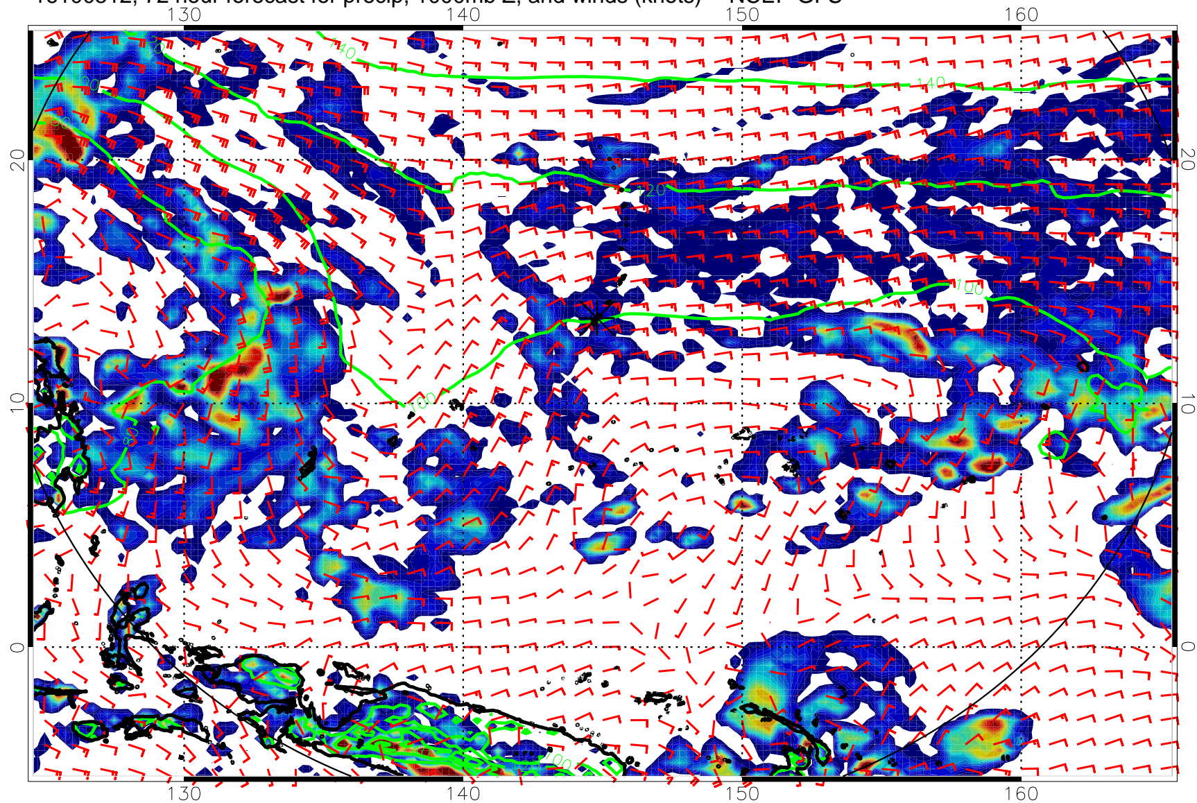
16100512, 72 hour forecast for precip, 1000mb Z, and winds (knots) -- NCEP GFS
