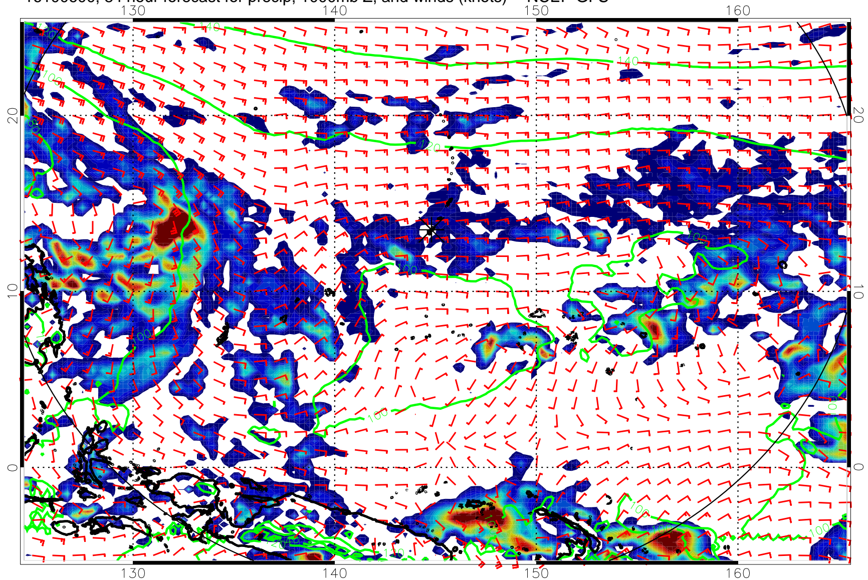
16100600, 84 hour forecast for precip, 1000mb Z, and winds (knots) -- NCEP GFS
