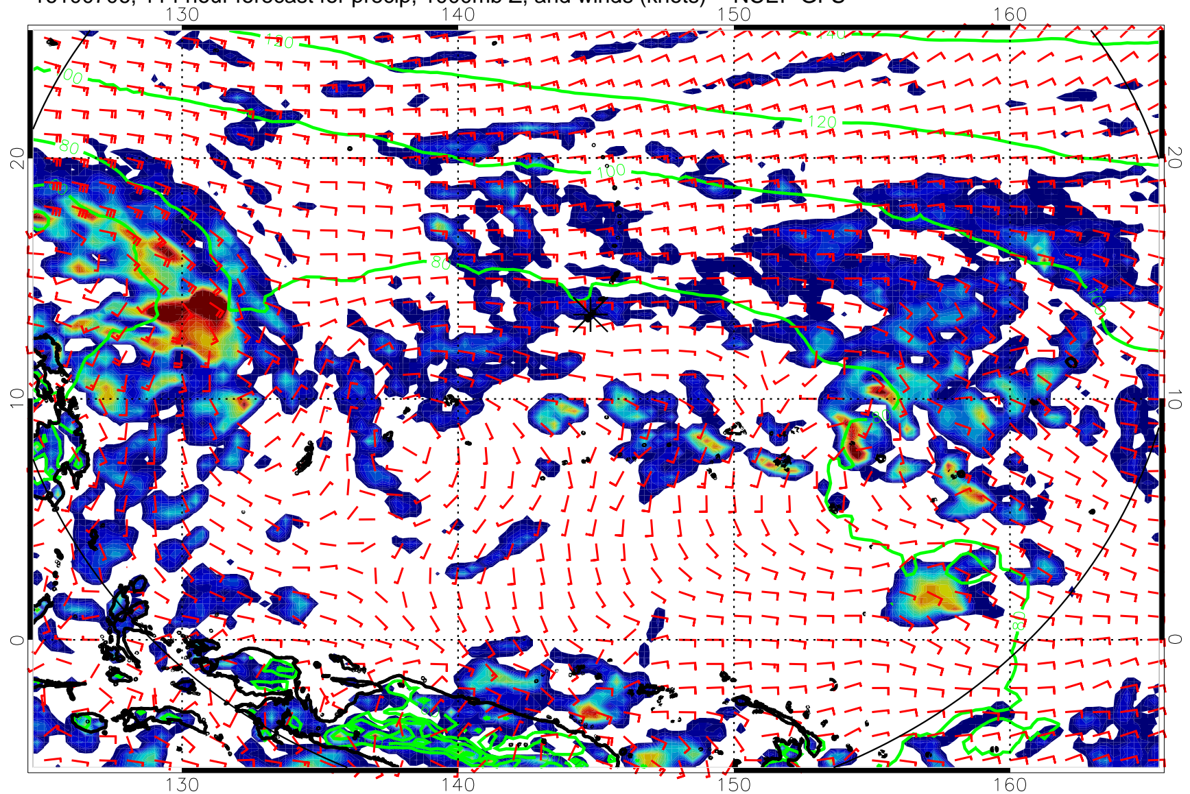
16100706, 114 hour forecast for precip, 1000mb Z, and winds (knots) -- NCEP GFS
