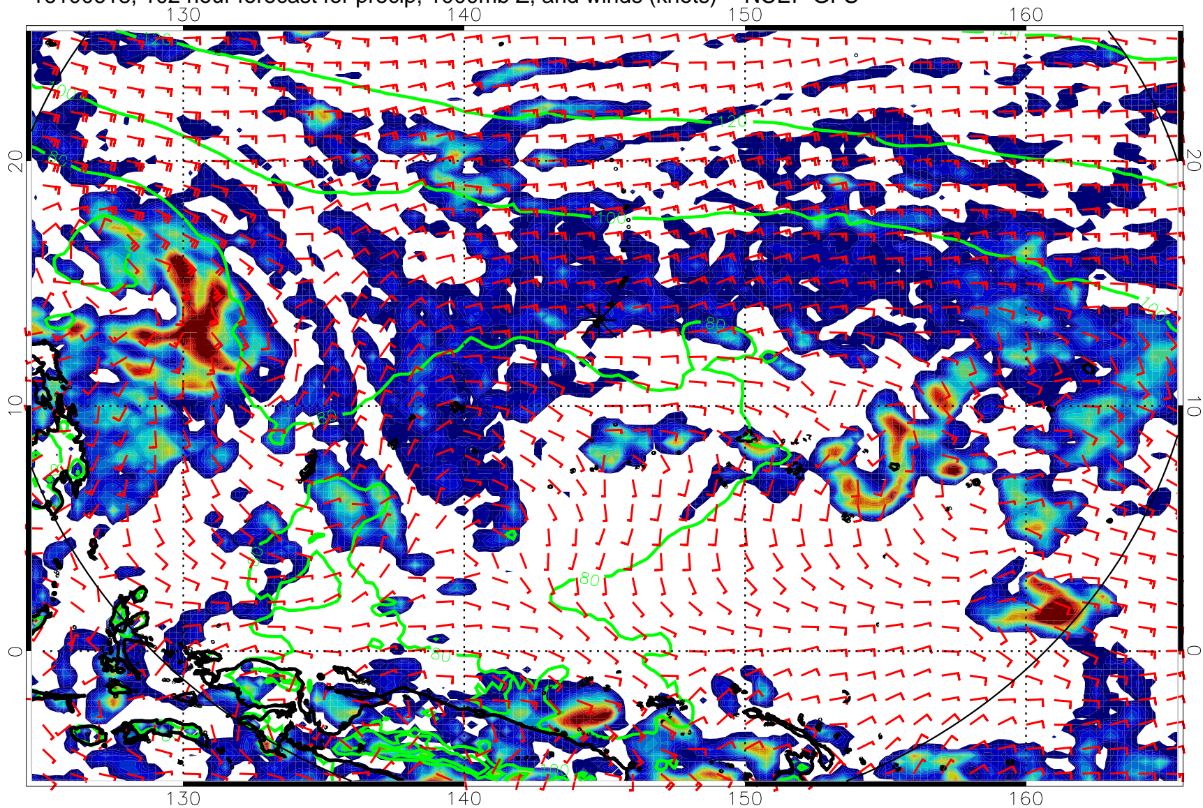
16100618, 102 hour forecast for precip, 1000mb Z, and winds (knots) -- NCEP GFS
