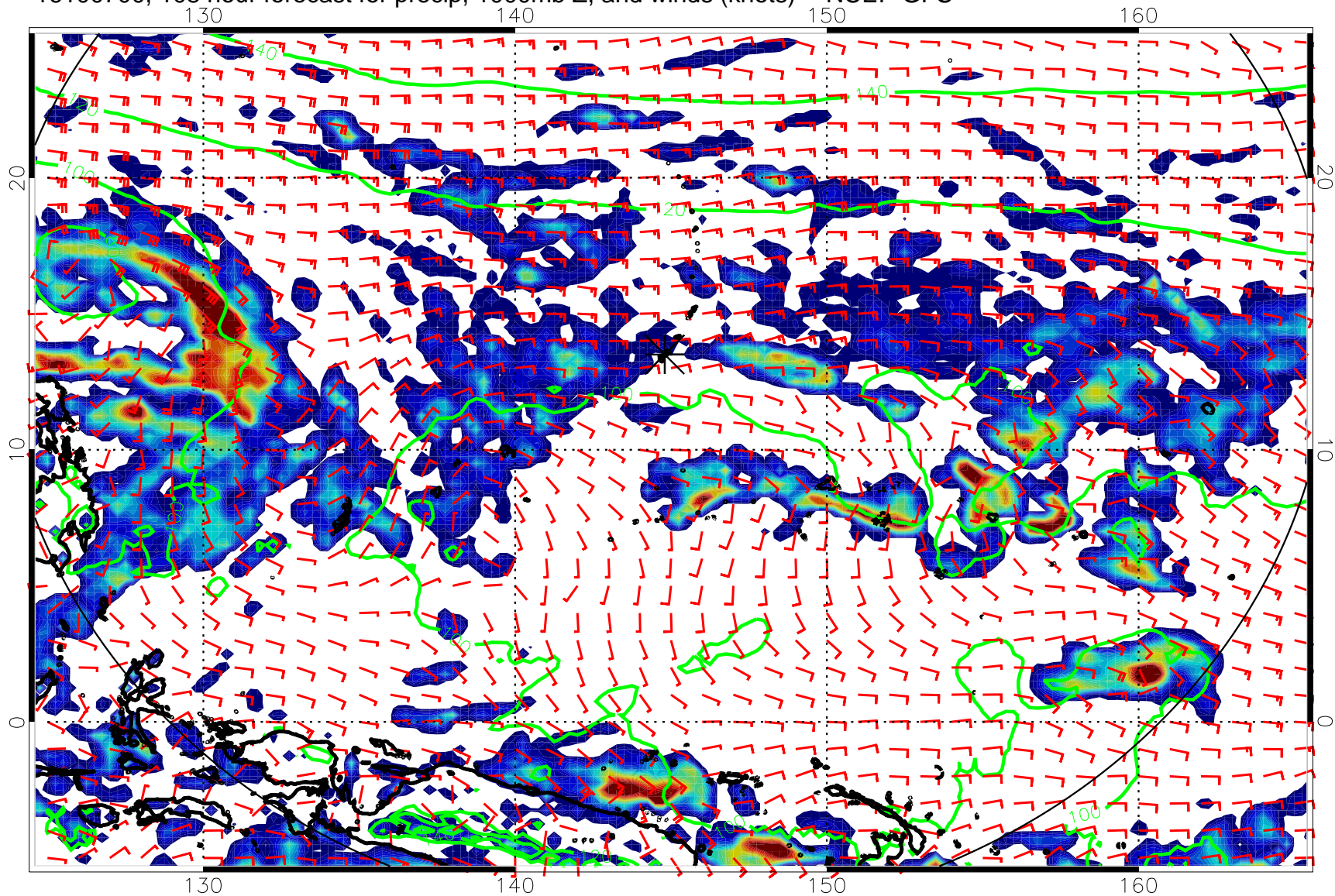
16100700, 108 hour forecast for precip, 1000mb Z, and winds (knots) -- NCEP GFS
