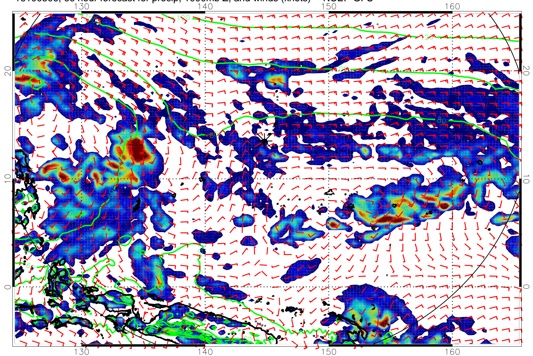
16100506, 66 hour forecast for precip, 1000mb Z, and winds (knots) -- NCEP GFS
