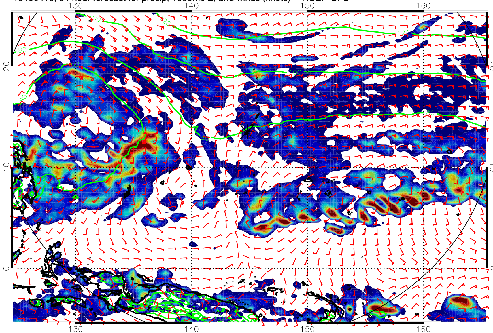
16100418, 54 hour forecast for precip, 1000mb Z, and winds (knots) -- NCEP GFS
