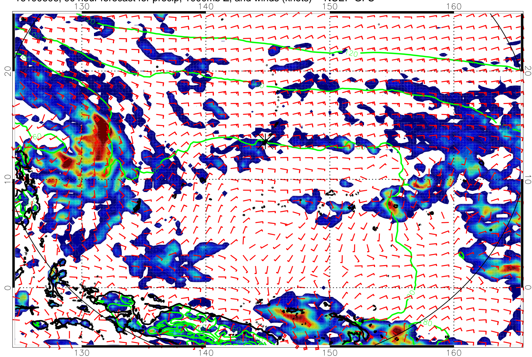
16100606, 90 hour forecast for precip, 1000mb Z, and winds (knots) -- NCEP GFS
