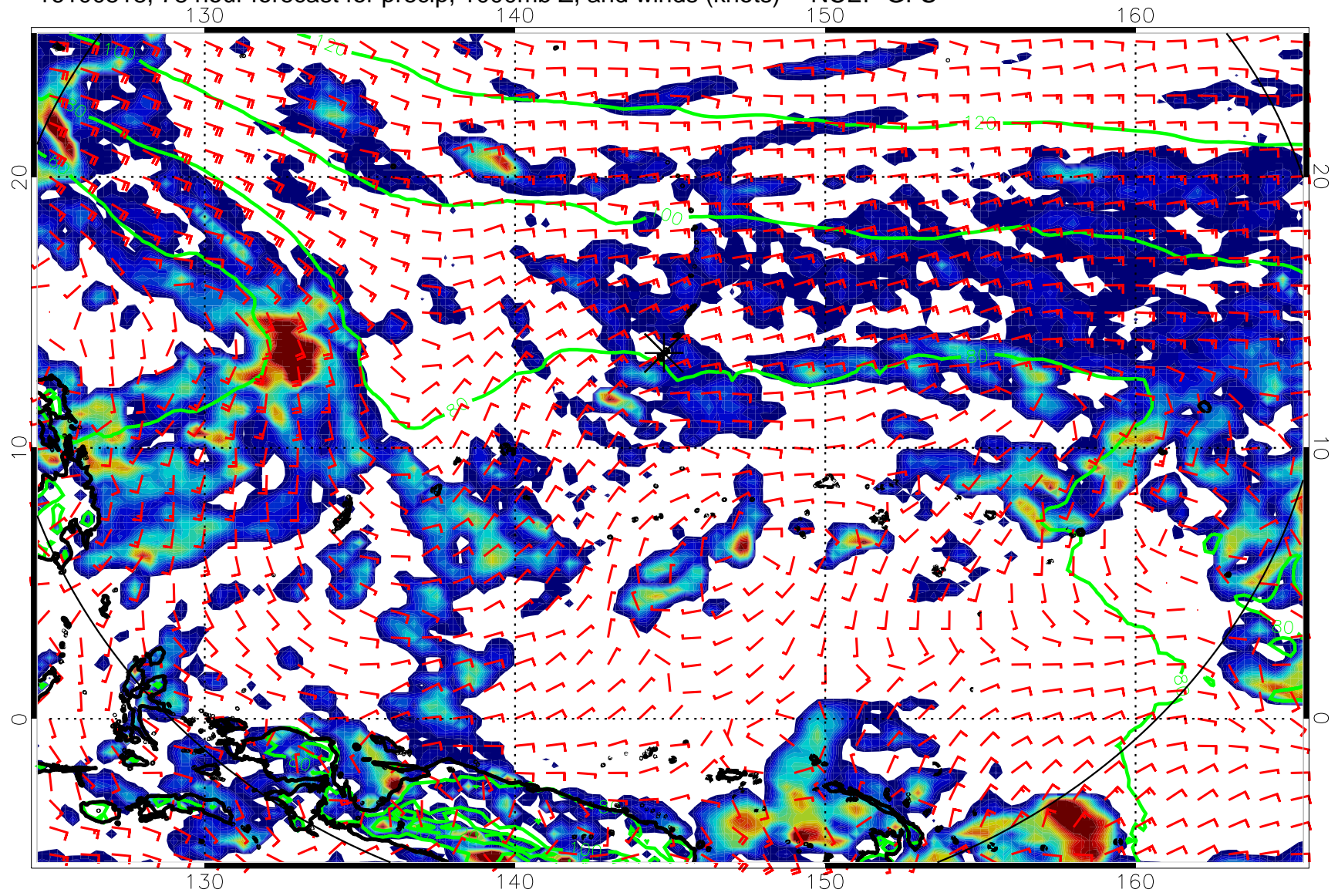
16100518, 78 hour forecast for precip, 1000mb Z, and winds (knots) -- NCEP GFS
