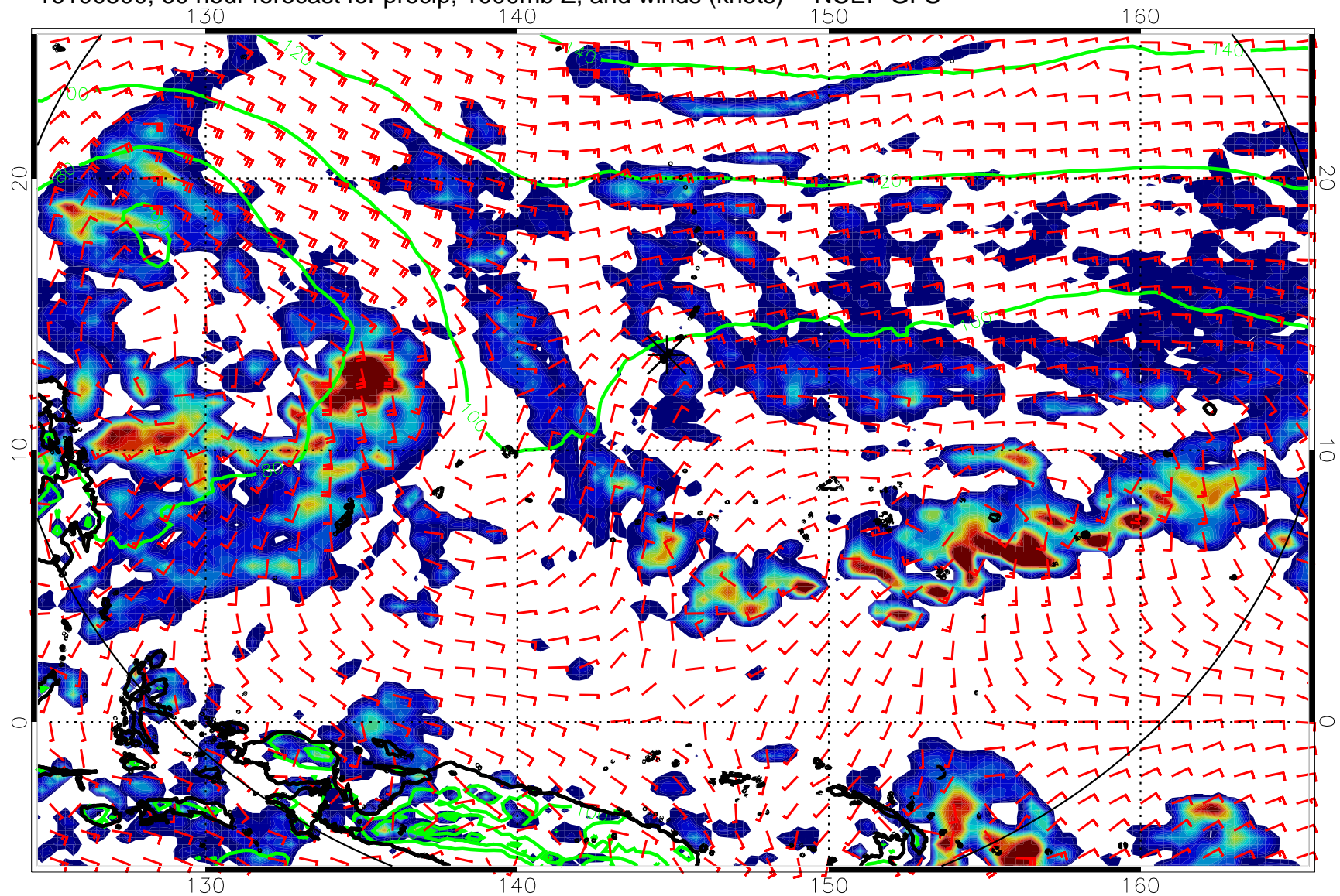
16100500, 60 hour forecast for precip, 1000mb Z, and winds (knots) -- NCEP GFS
