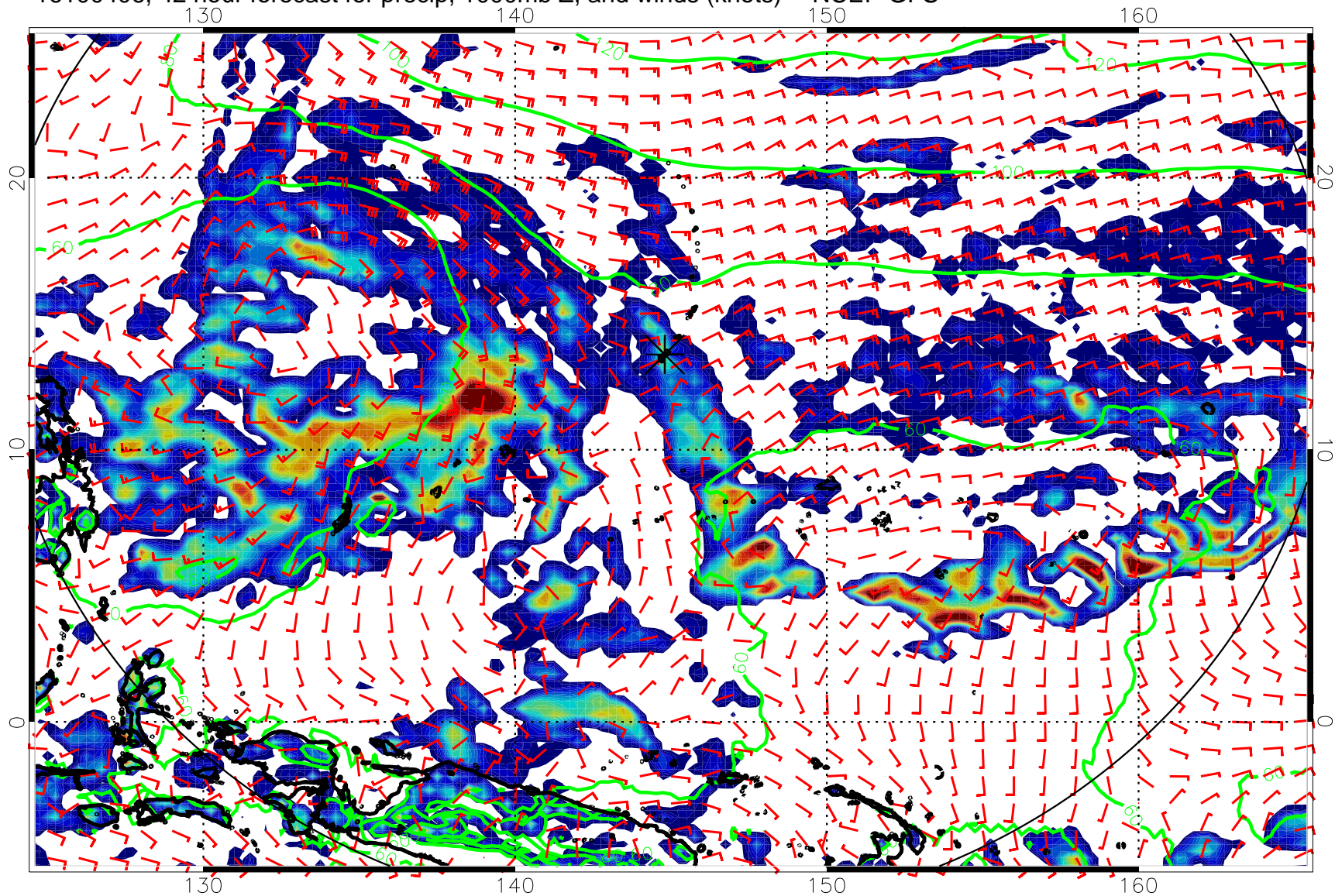
16100406, 42 hour forecast for precip, 1000mb Z, and winds (knots) -- NCEP GFS
