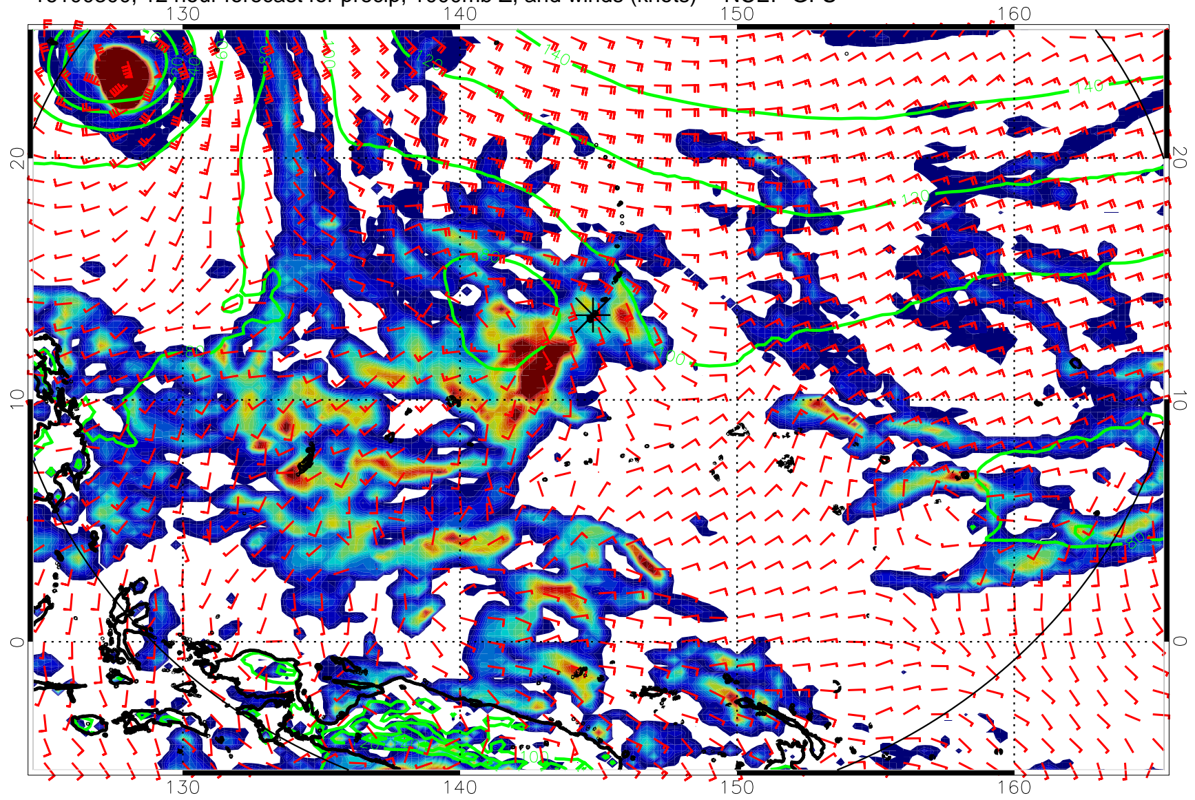
16100300, 12 hour forecast for precip, 1000mb Z, and winds (knots) -- NCEP GFS
