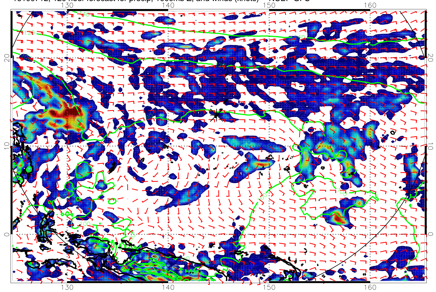
16100712, 120 hour forecast for precip, 1000mb Z, and winds (knots) -- NCEP GFS
