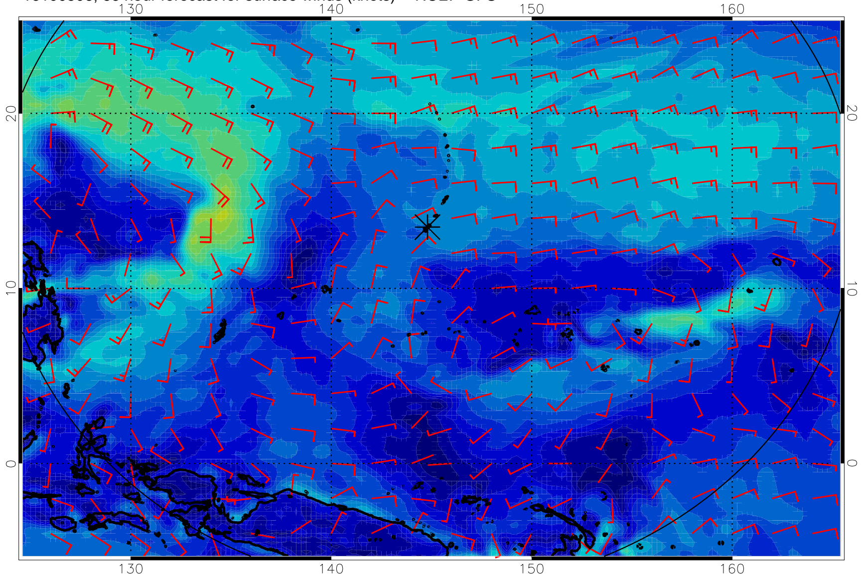
16100506, 66 hour forecast for surface winds (knots) -- NCEP GFS
