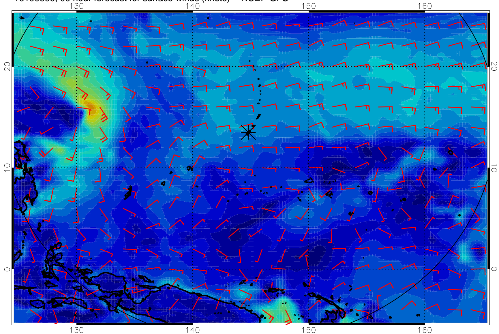
16100606, 90 hour forecast for surface winds (knots) -- NCEP GFS
