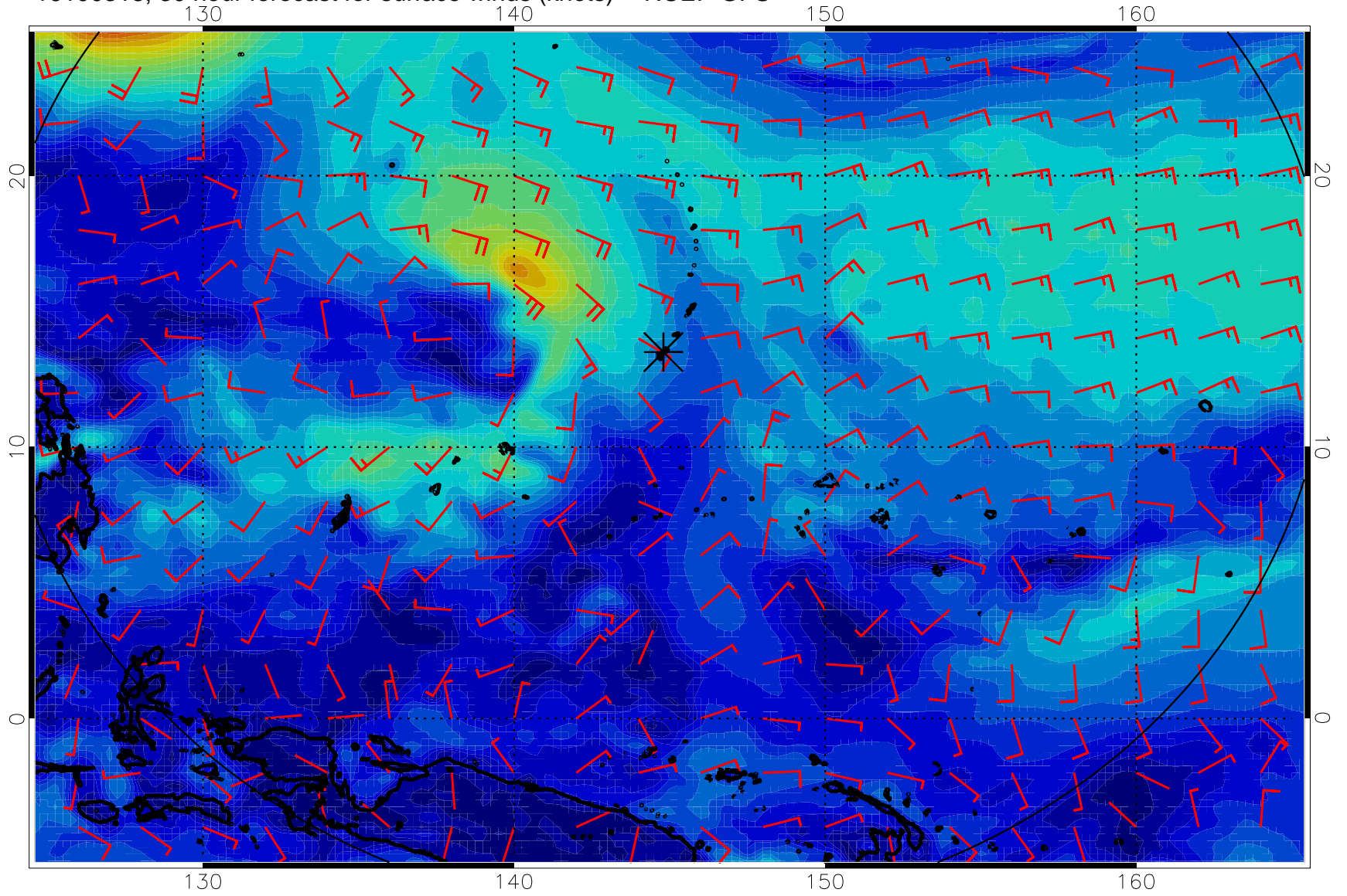
16100318, 30 hour forecast for surface winds (knots) -- NCEP GFS
