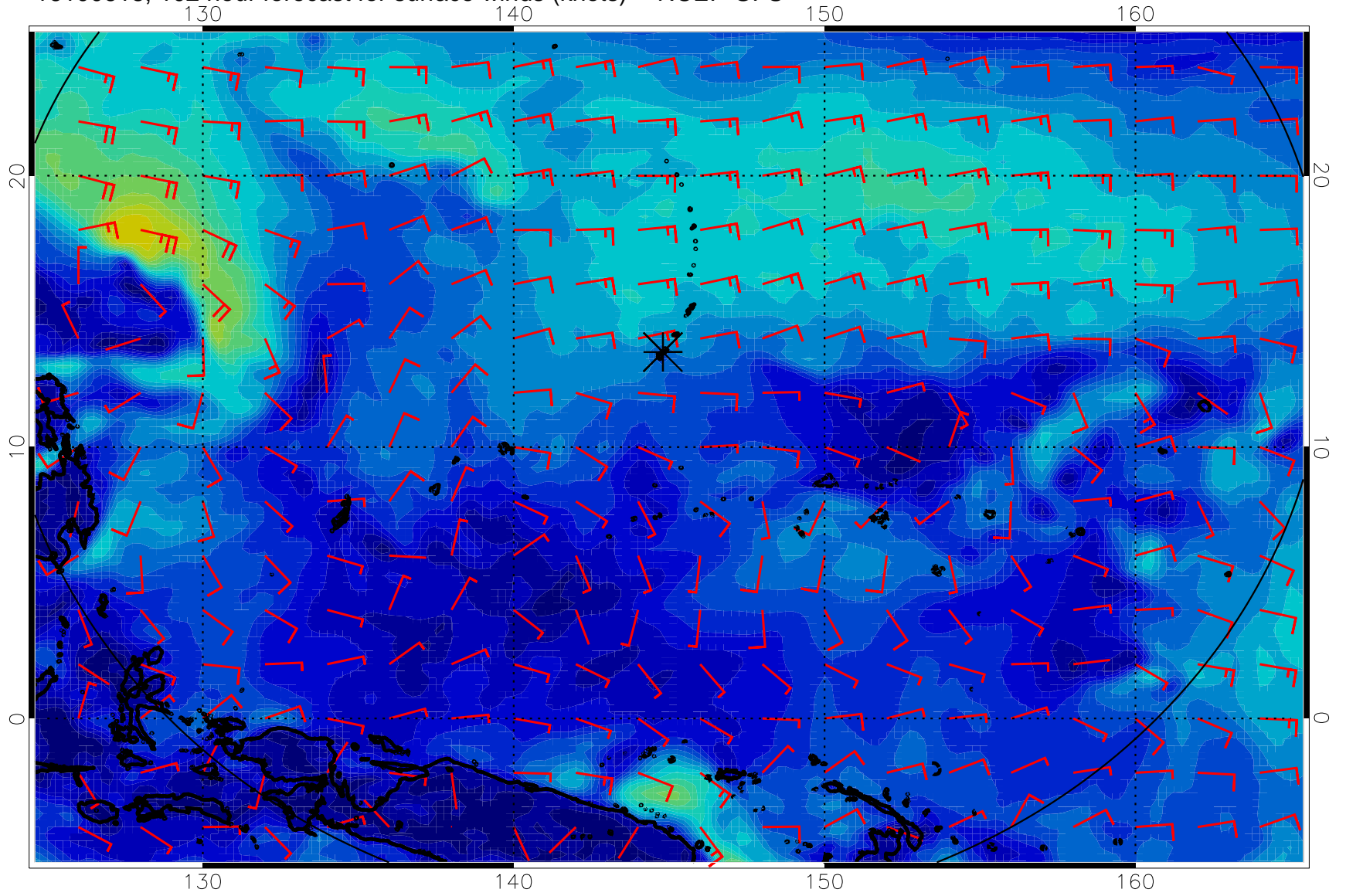
16100618, 102 hour forecast for surface winds (knots) -- NCEP GFS
