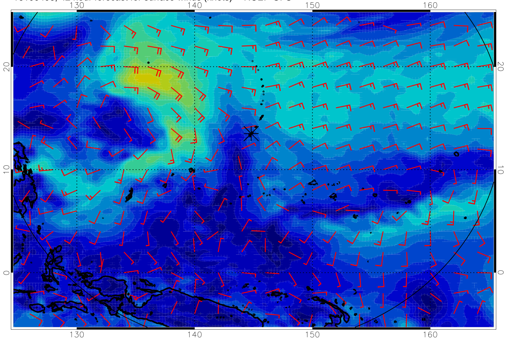
16100406, 42 hour forecast for surface winds (knots) -- NCEP GFS
