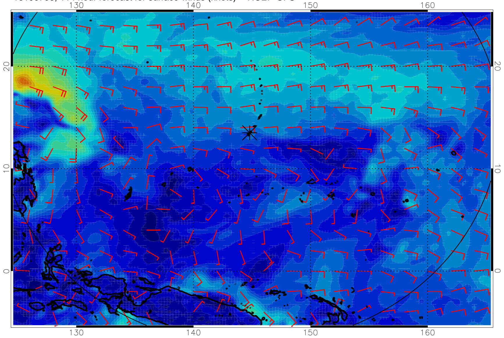
16100706, 114 hour forecast for surface winds (knots) -- NCEP GFS
