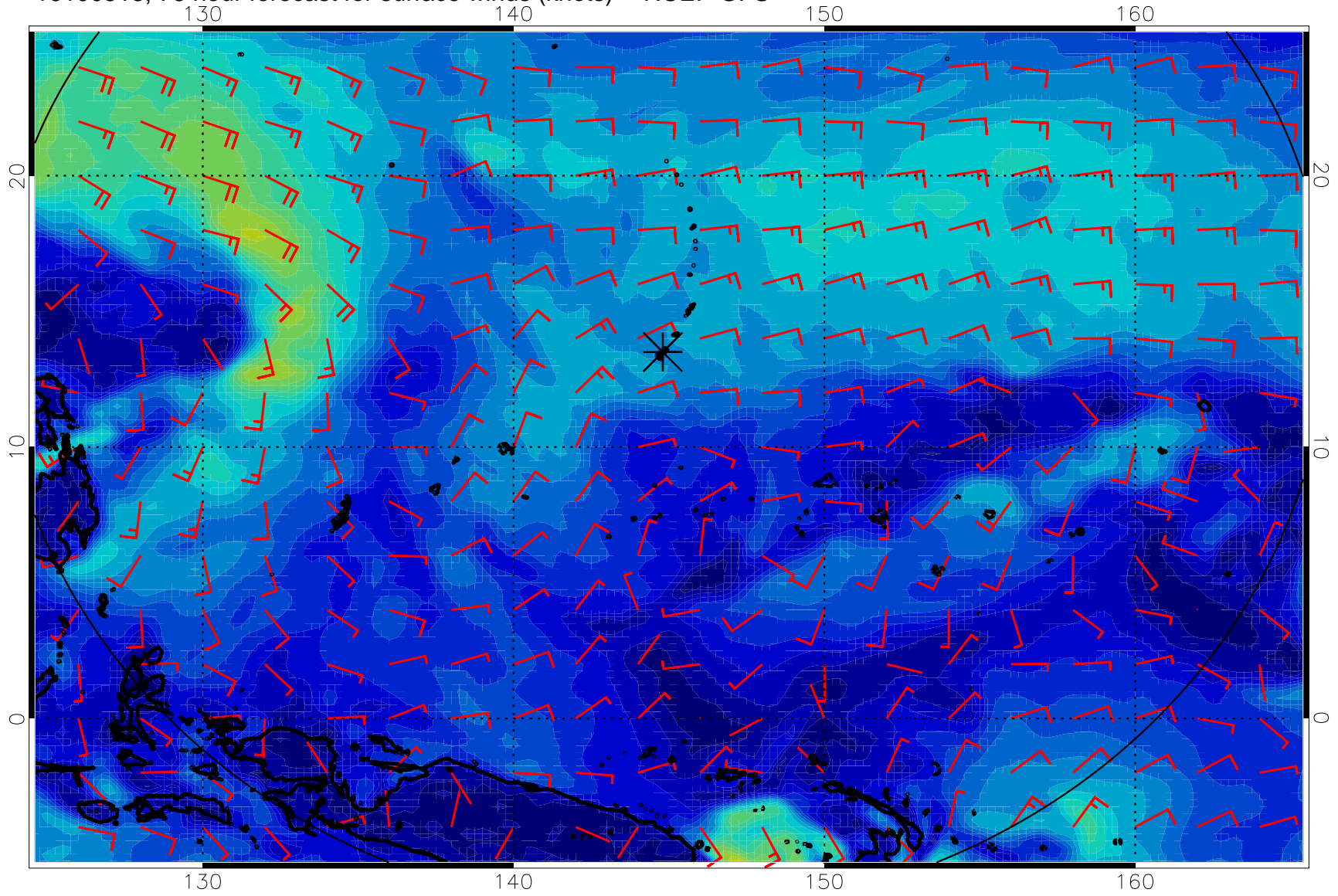
16100518, 78 hour forecast for surface winds (knots) -- NCEP GFS
