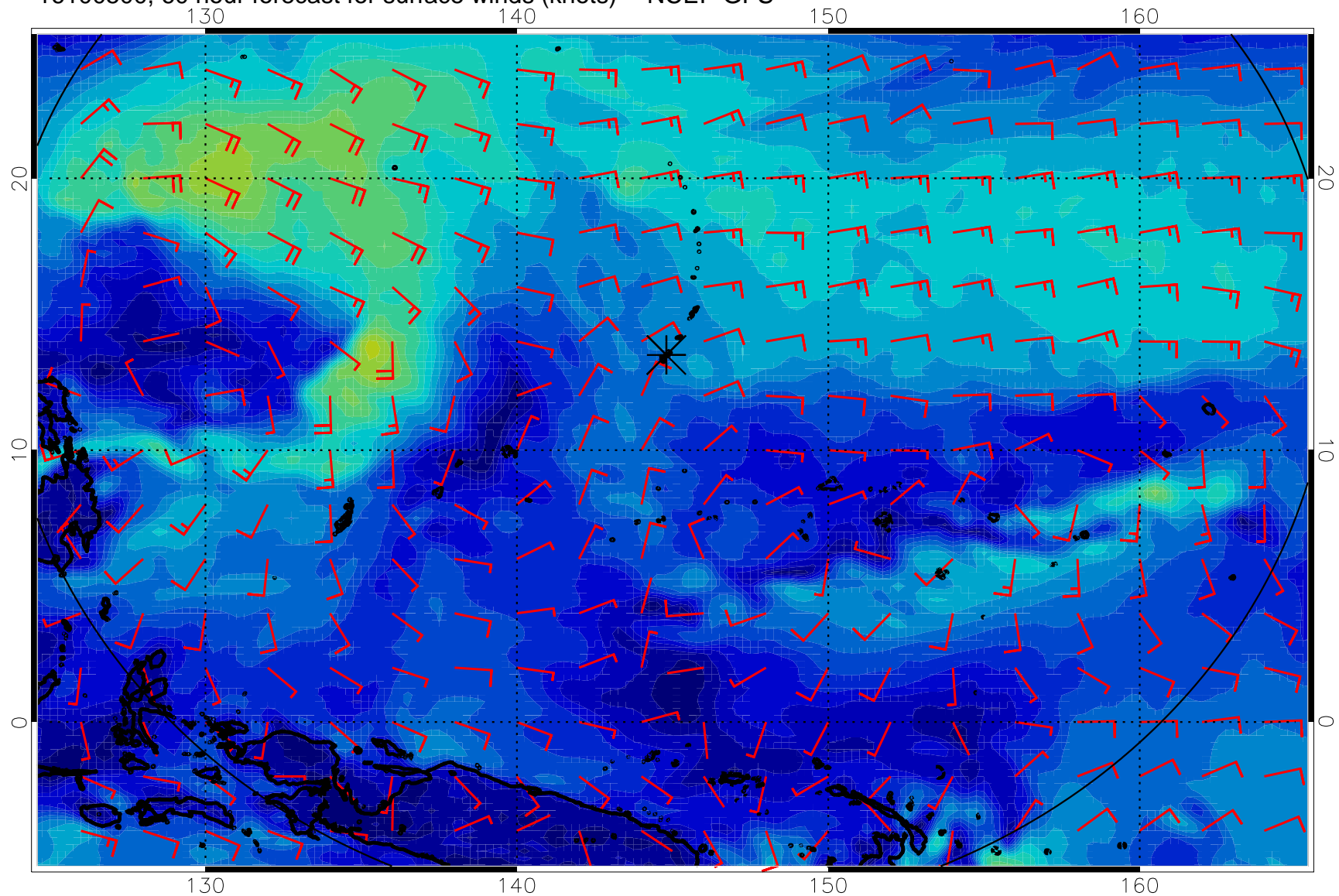
16100500, 60 hour forecast for surface winds (knots) -- NCEP GFS
