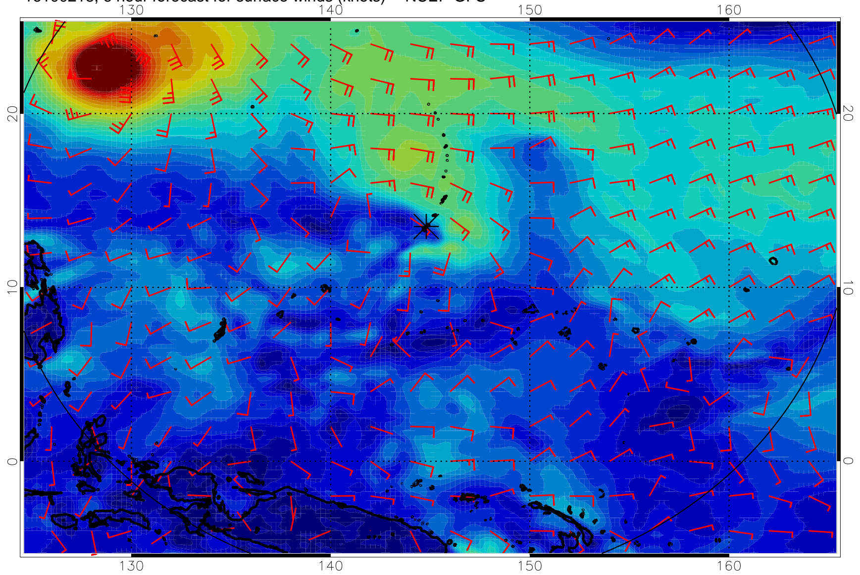
16100218, 6 hour forecast for surface winds (knots) -- NCEP GFS
