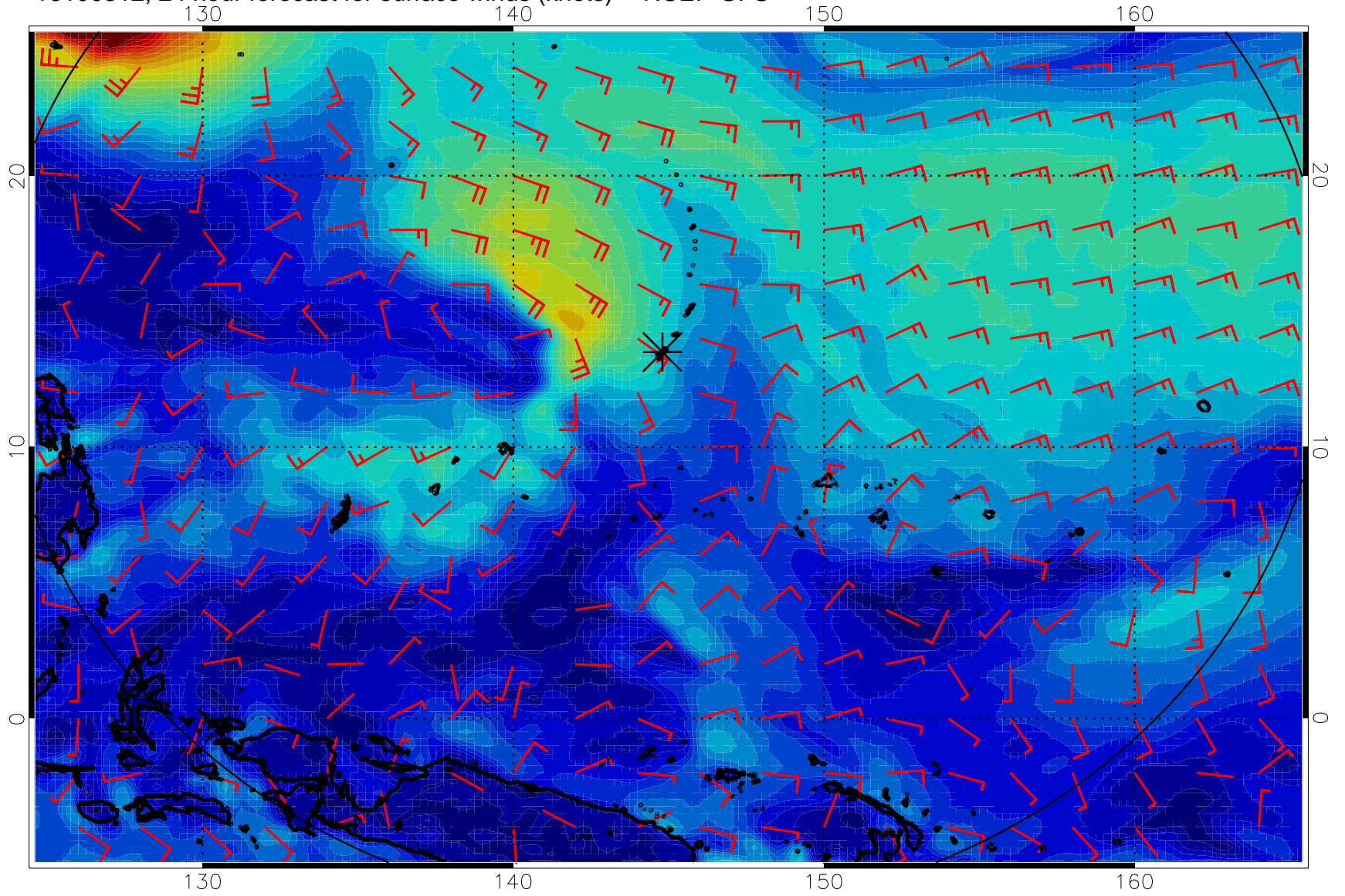
16100312, 24 hour forecast for surface winds (knots) -- NCEP GFS
