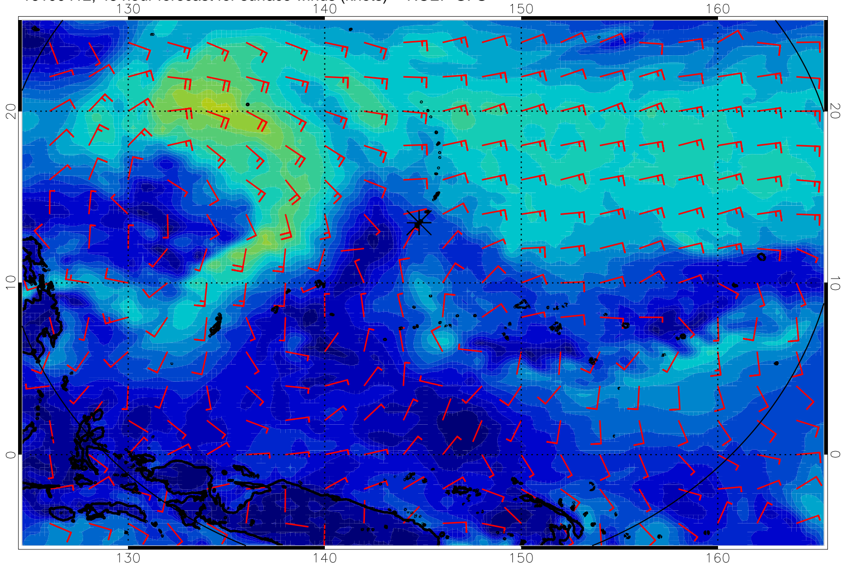
16100412, 48 hour forecast for surface winds (knots) -- NCEP GFS
