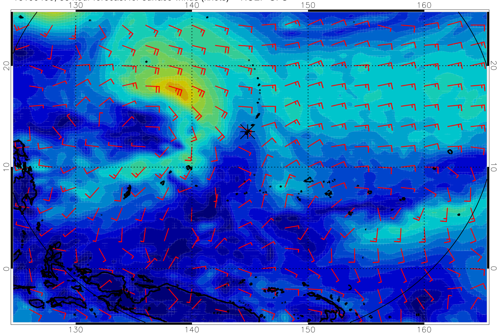
16100400, 36 hour forecast for surface winds (knots) -- NCEP GFS
