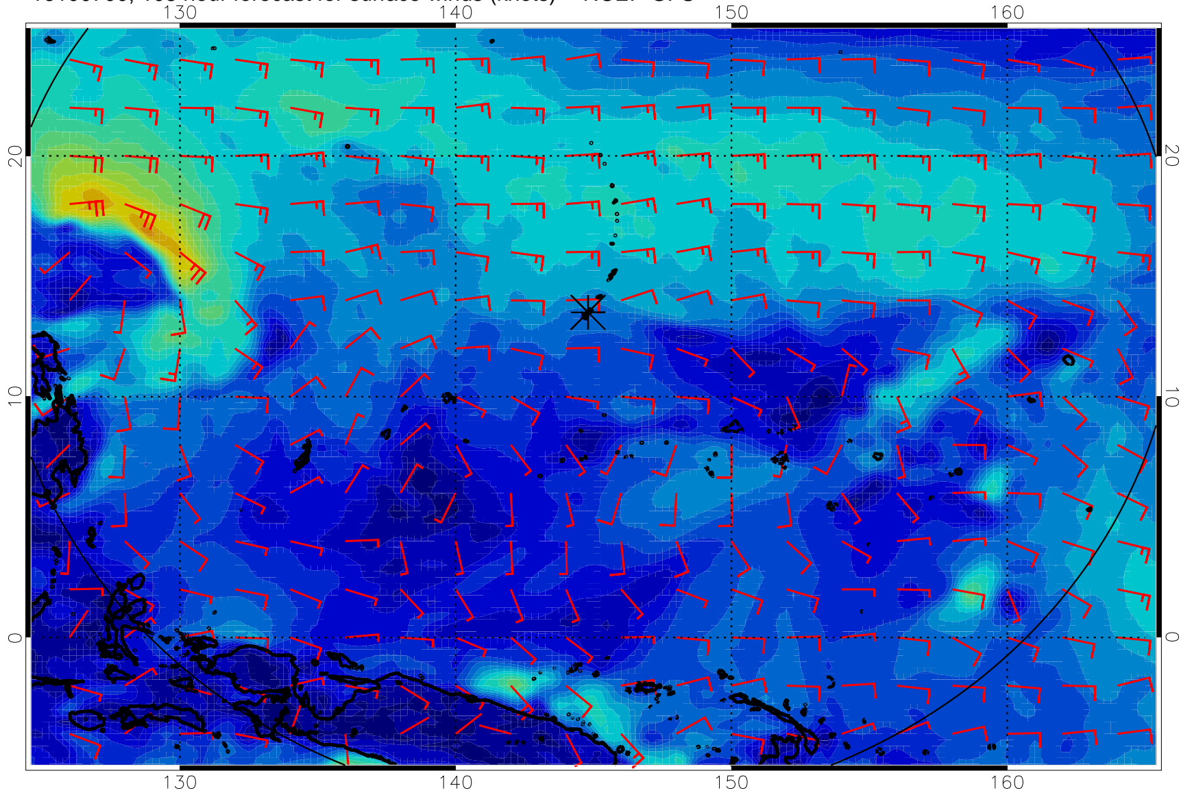
16100700, 108 hour forecast for surface winds (knots) -- NCEP GFS
