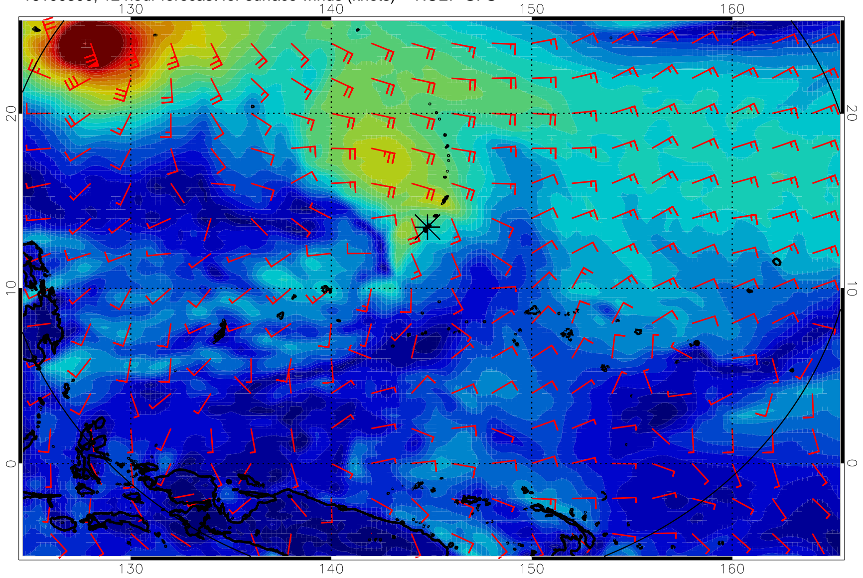
16100300, 12 hour forecast for surface winds (knots) -- NCEP GFS
