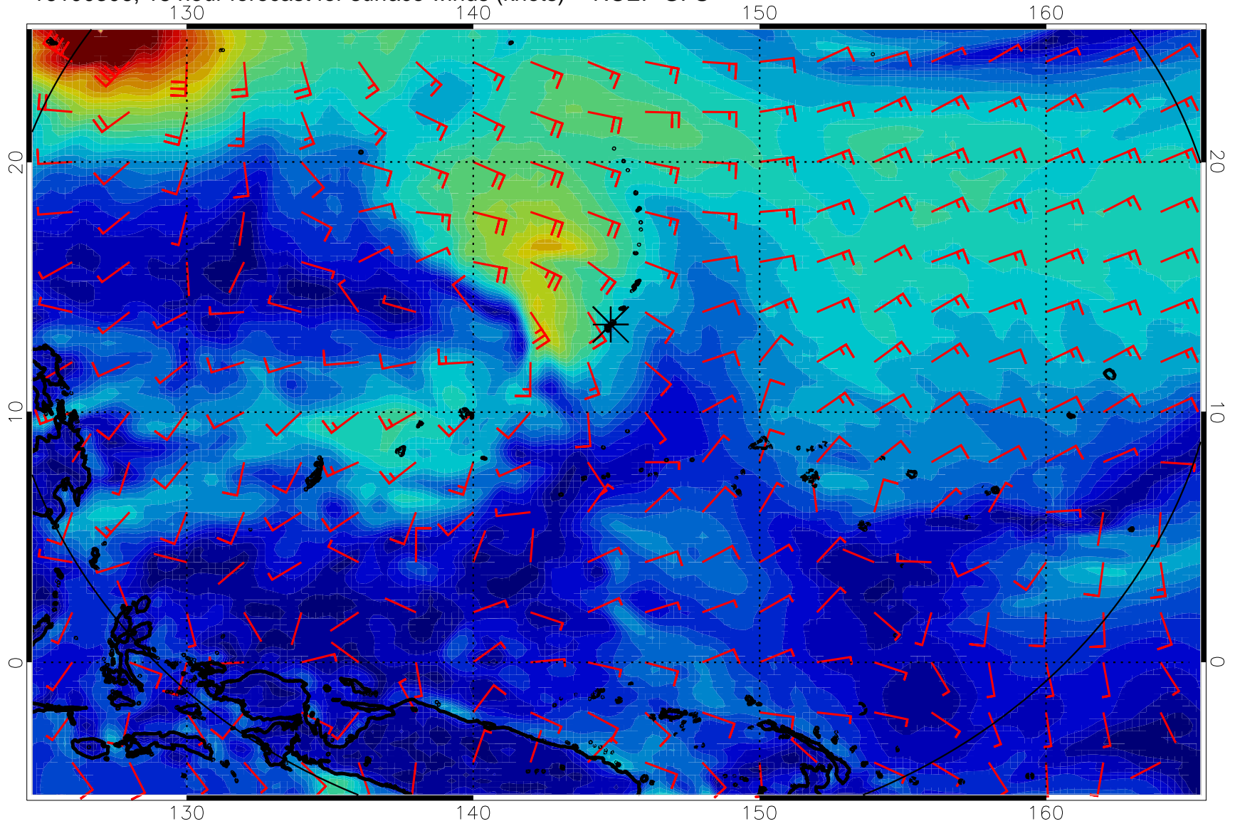
16100306, 18 hour forecast for surface winds (knots) -- NCEP GFS
