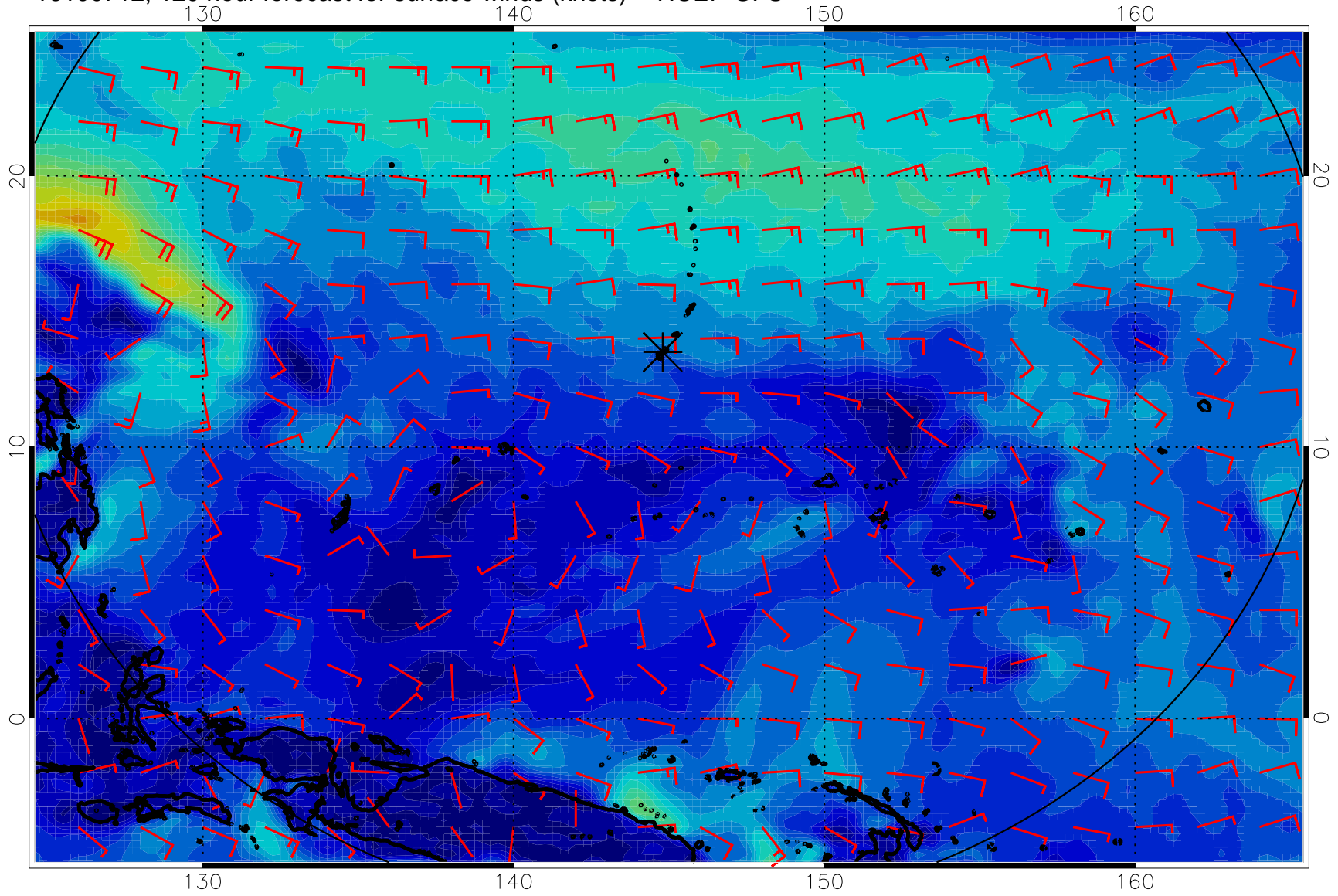
16100712, 120 hour forecast for surface winds (knots) -- NCEP GFS
