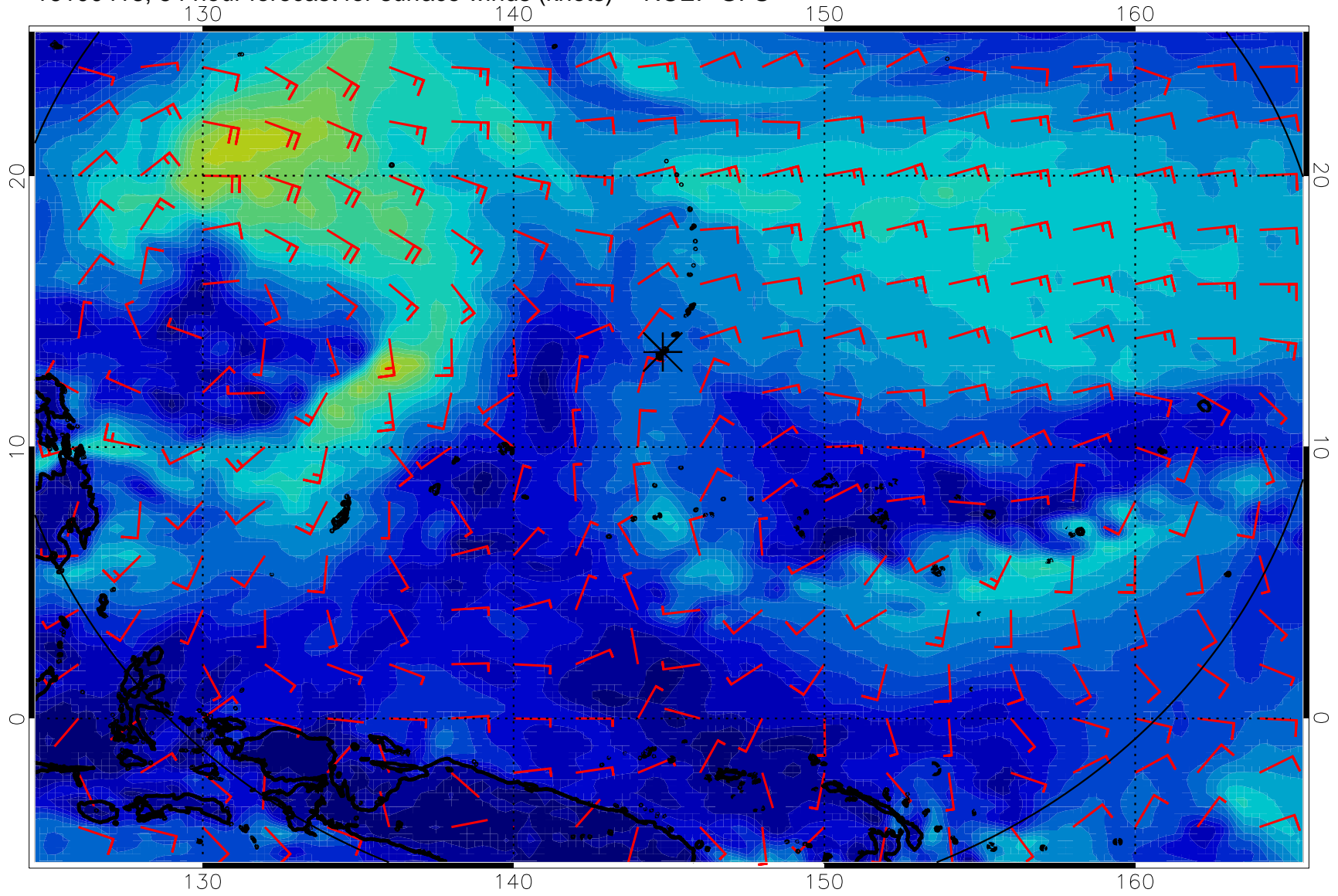
16100418, 54 hour forecast for surface winds (knots) -- NCEP GFS
