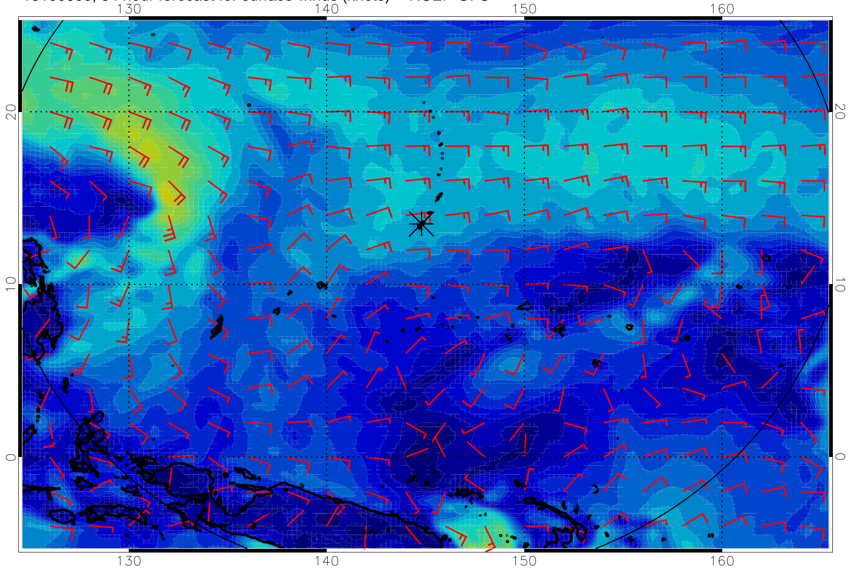
16100600, 84 hour forecast for surface winds (knots) -- NCEP GFS
