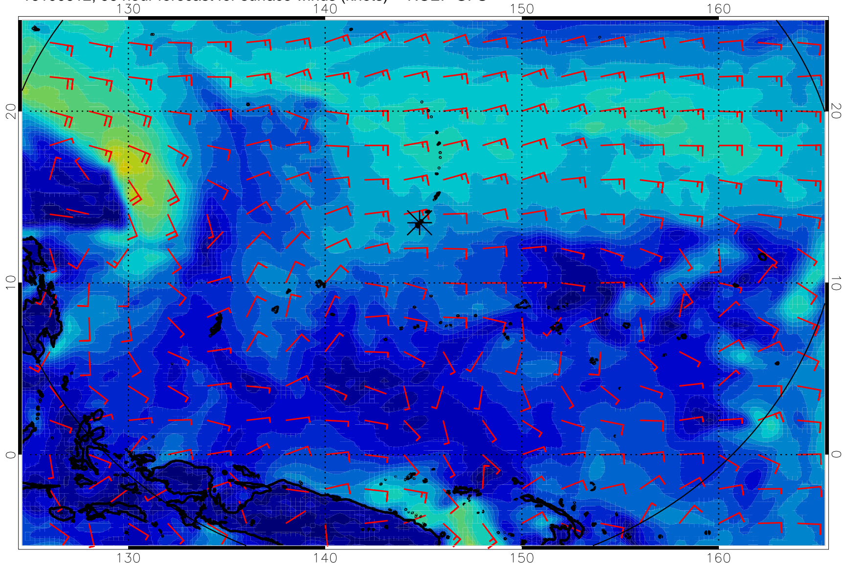
16100612, 96 hour forecast for surface winds (knots) -- NCEP GFS
