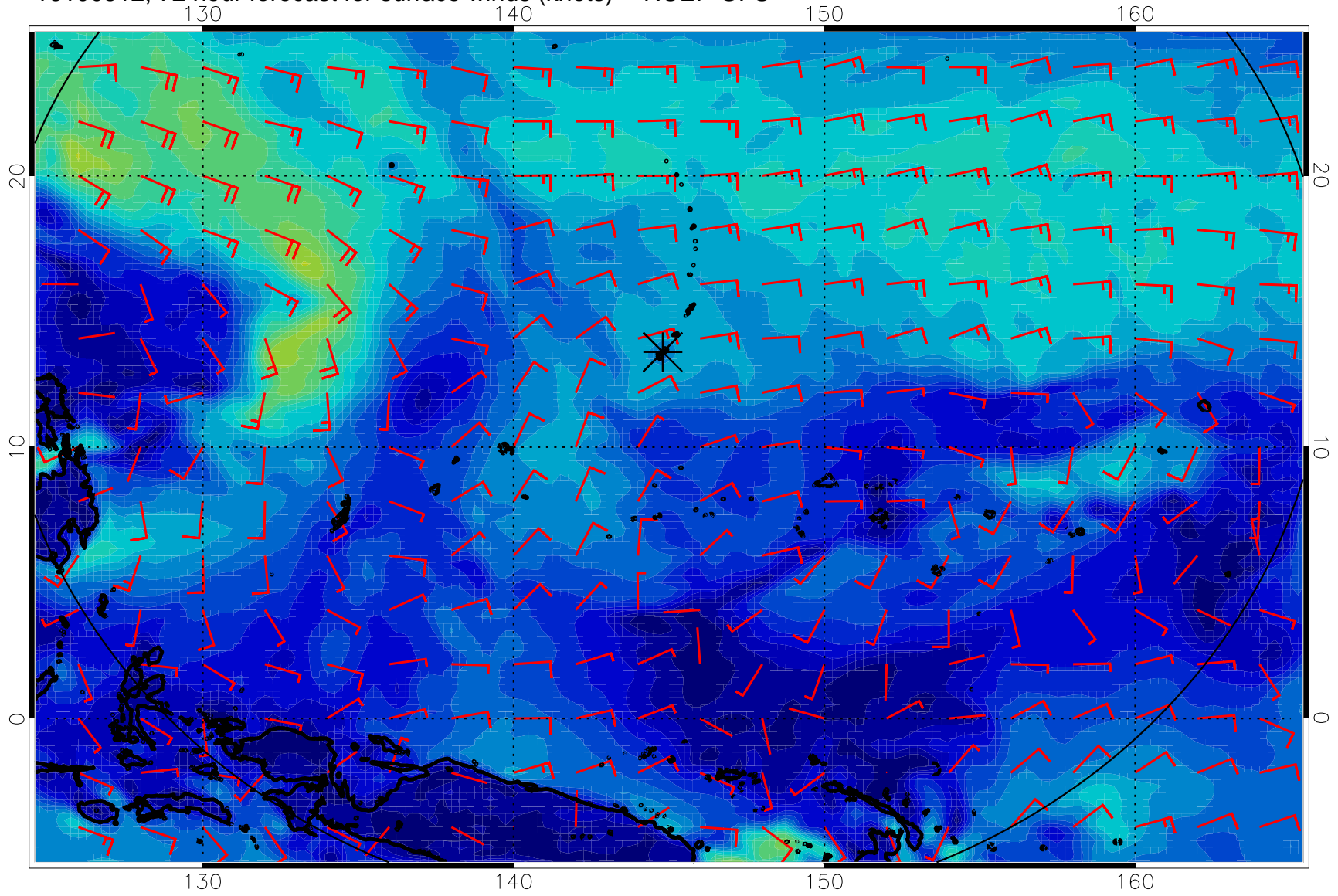
16100512, 72 hour forecast for surface winds (knots) -- NCEP GFS
