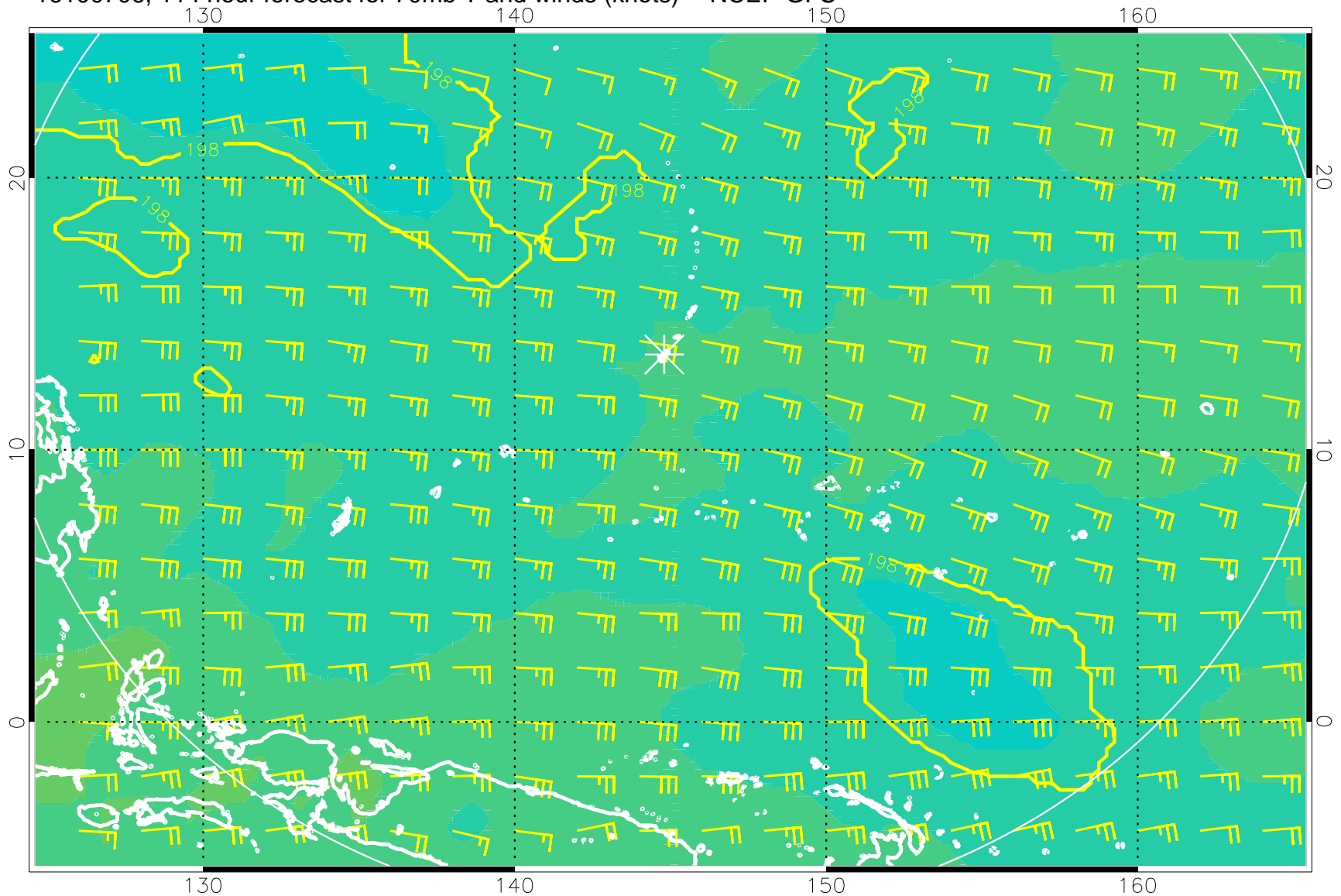
16100706, 114 hour forecast for 70mb T and winds (knots) -- NCEP GFS
