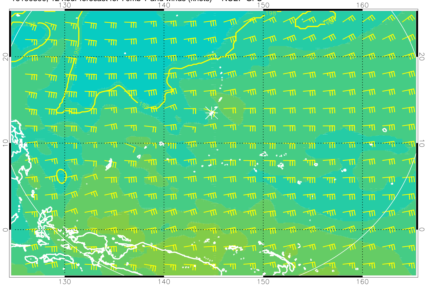
16100300, 12 hour forecast for 70mb T and winds (knots) -- NCEP GFS
