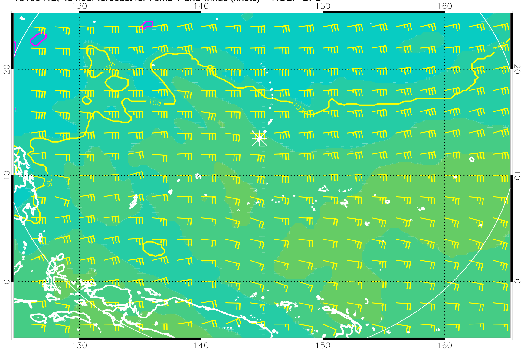
16100412, 48 hour forecast for 70mb T and winds (knots) -- NCEP GFS
