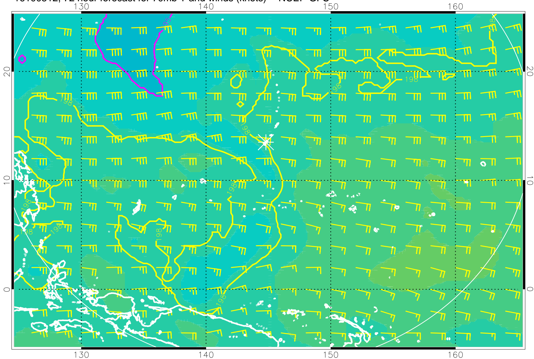
16100512, 72 hour forecast for 70mb T and winds (knots) -- NCEP GFS
