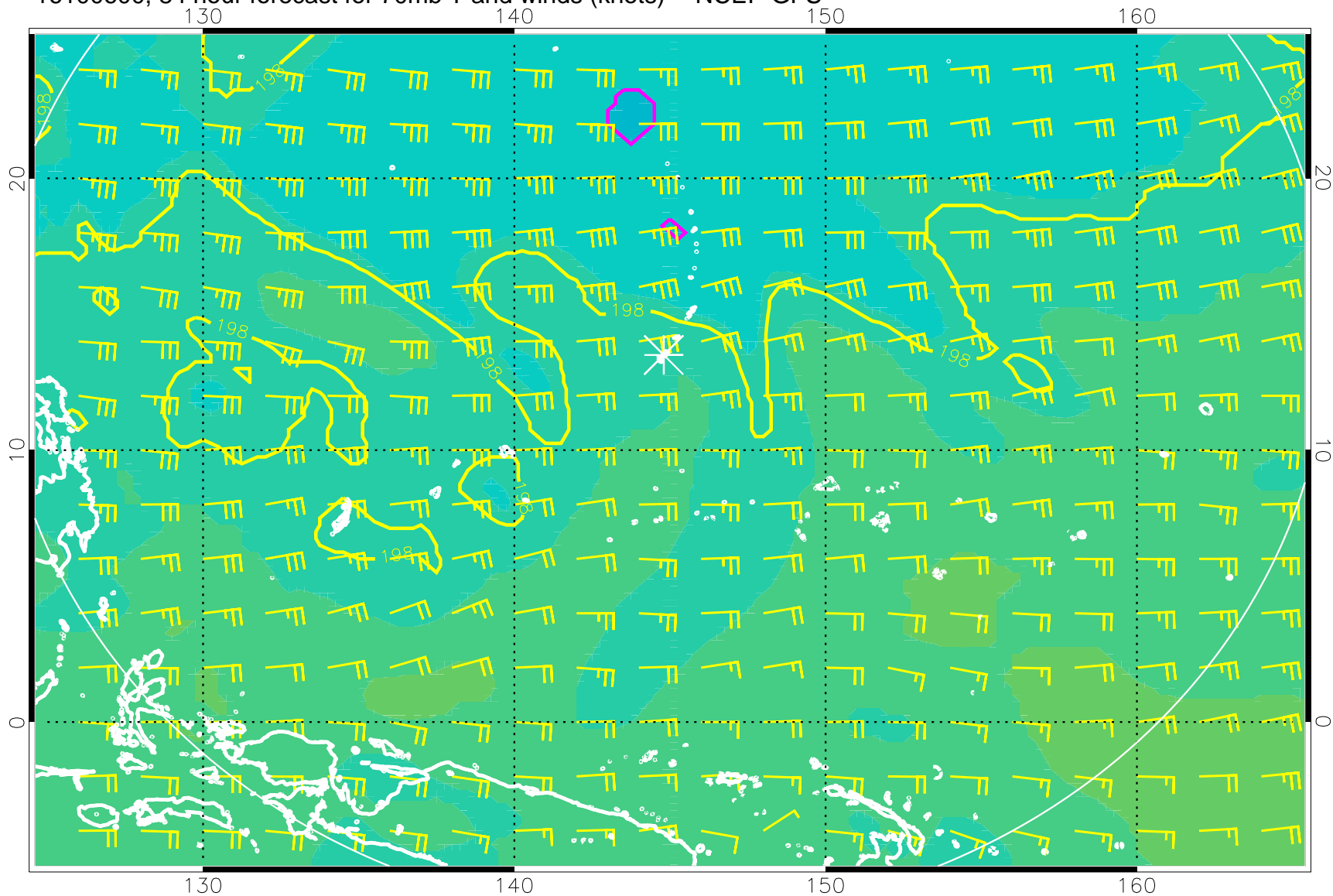
16100600, 84 hour forecast for 70mb T and winds (knots) -- NCEP GFS
