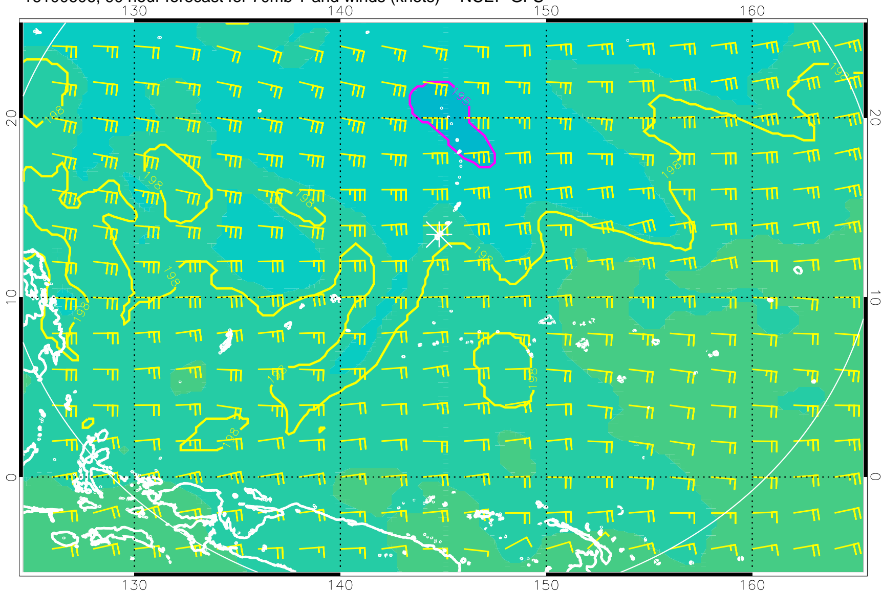
16100606, 90 hour forecast for 70mb T and winds (knots) -- NCEP GFS
