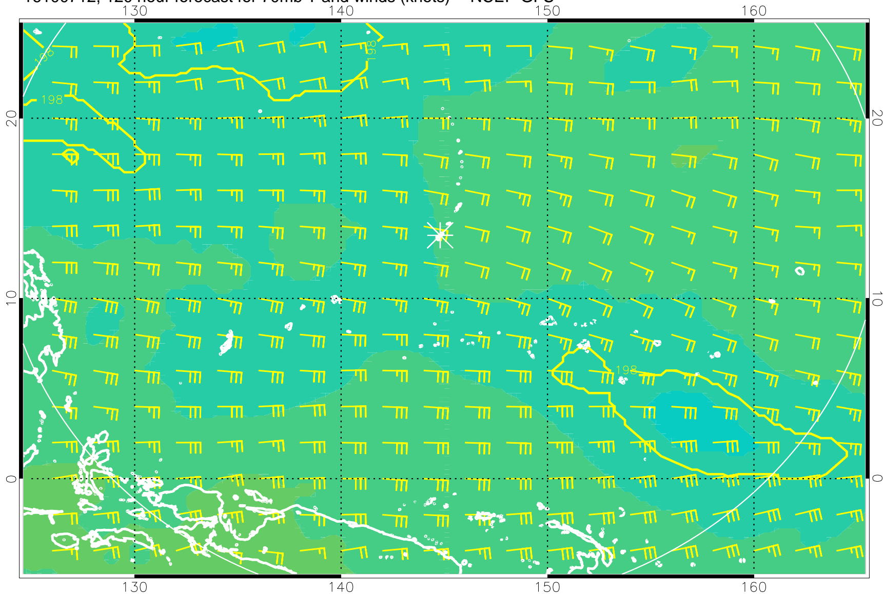
16100712, 120 hour forecast for 70mb T and winds (knots) -- NCEP GFS
