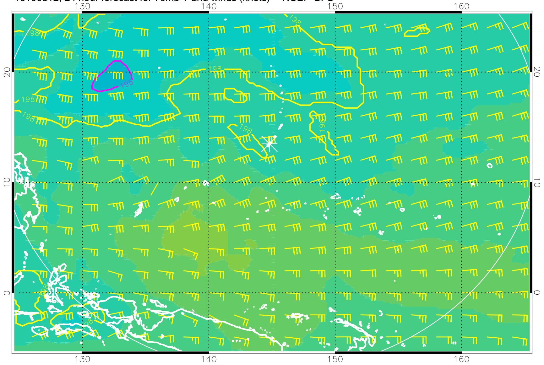
16100312, 24 hour forecast for 70mb T and winds (knots) -- NCEP GFS
