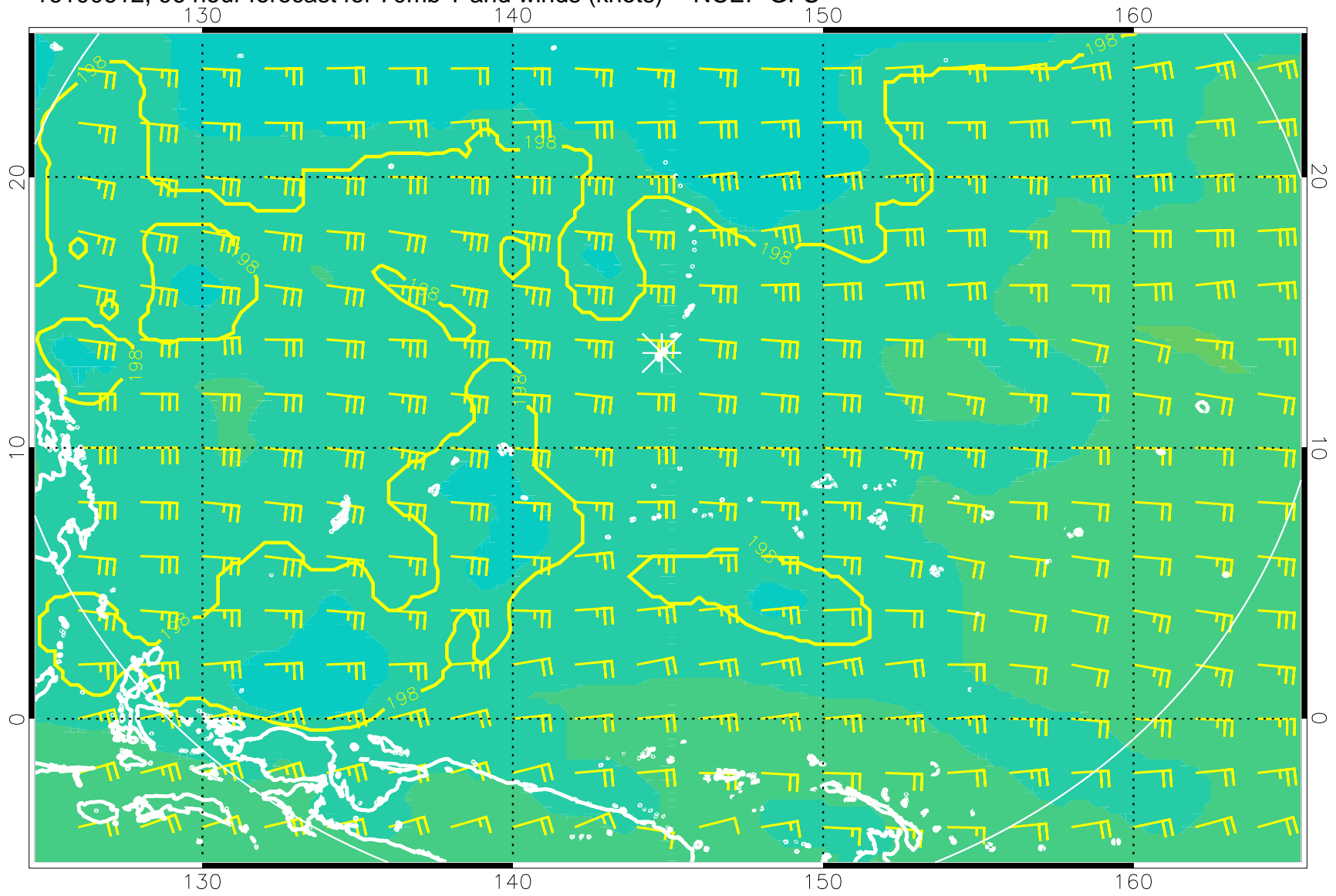
16100612, 96 hour forecast for 70mb T and winds (knots) -- NCEP GFS
