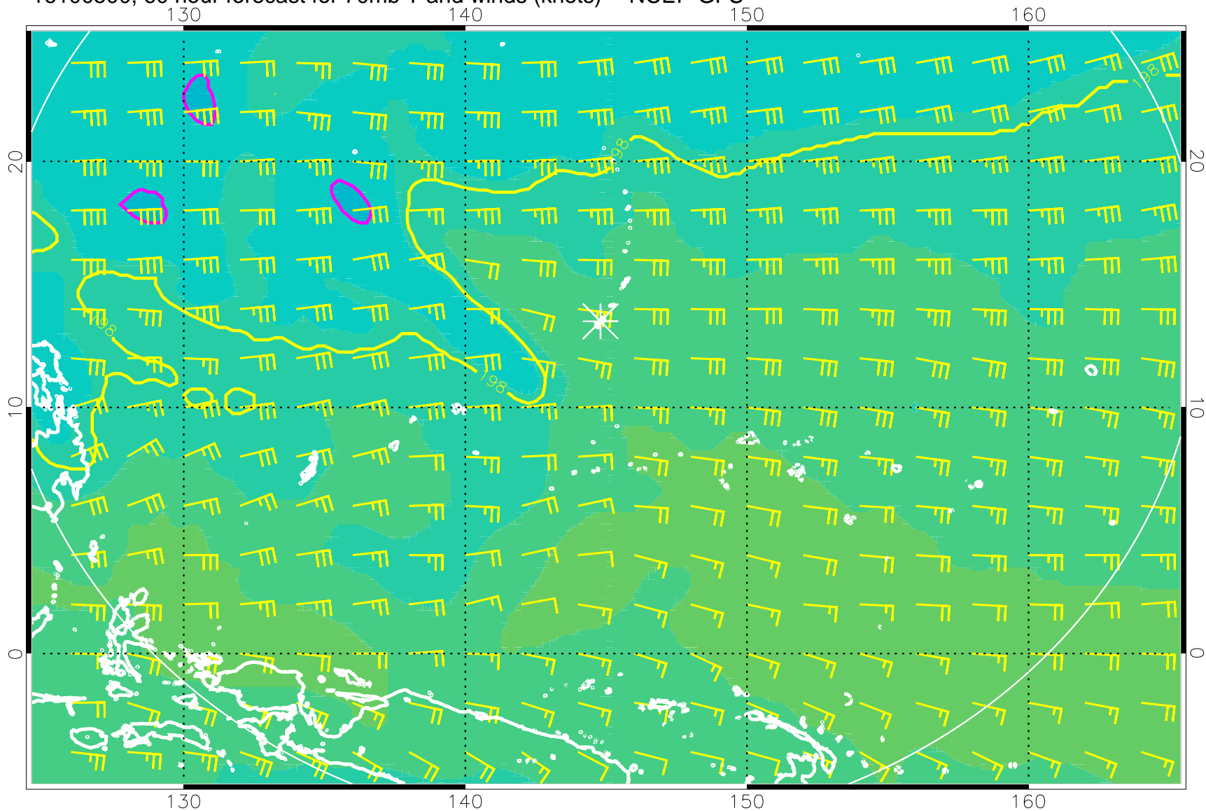
16100500, 60 hour forecast for 70mb T and winds (knots) -- NCEP GFS
