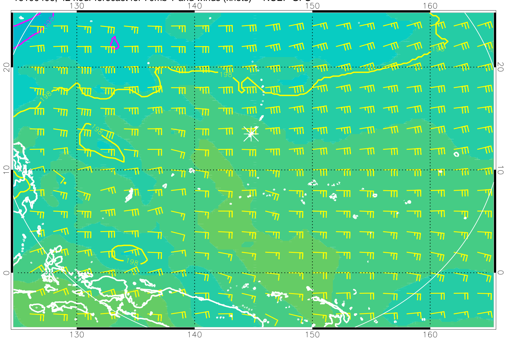
16100406, 42 hour forecast for 70mb T and winds (knots) -- NCEP GFS
