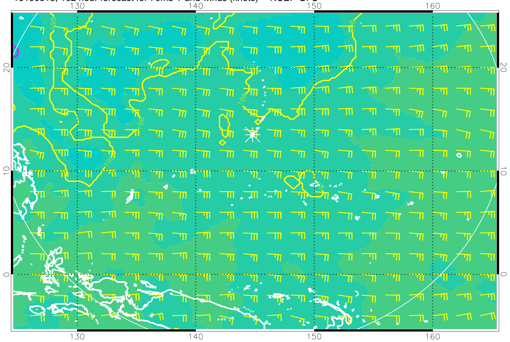
16100618, 102 hour forecast for 70mb T and winds (knots) -- NCEP GFS
