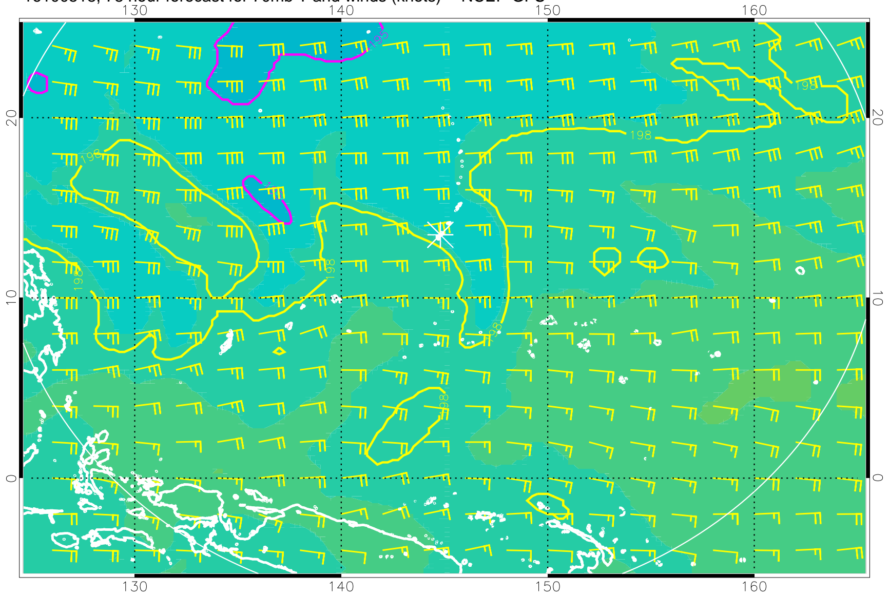
16100518, 78 hour forecast for 70mb T and winds (knots) -- NCEP GFS
