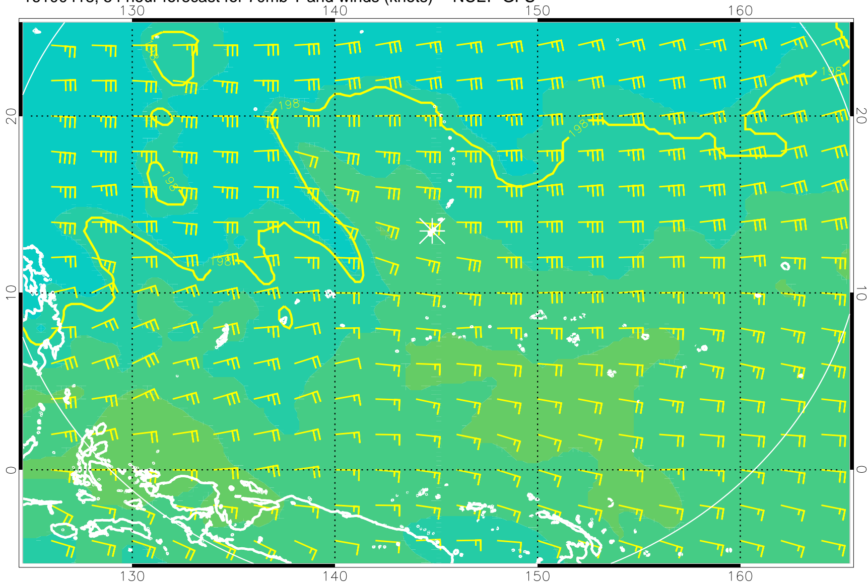
16100418, 54 hour forecast for 70mb T and winds (knots) -- NCEP GFS
