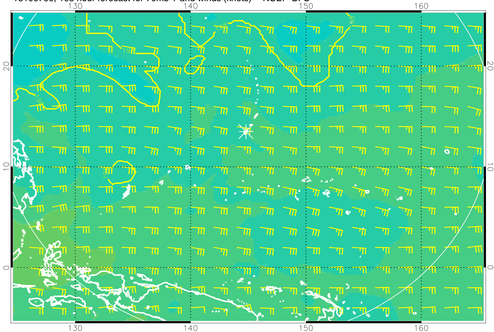
16100700, 108 hour forecast for 70mb T and winds (knots) -- NCEP GFS
