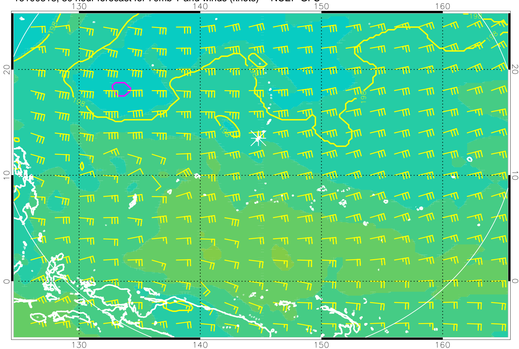
16100318, 30 hour forecast for 70mb T and winds (knots) -- NCEP GFS
