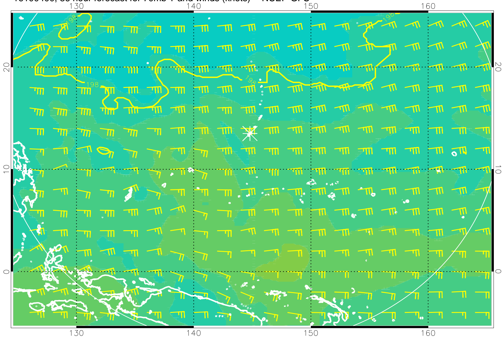
16100400, 36 hour forecast for 70mb T and winds (knots) -- NCEP GFS
