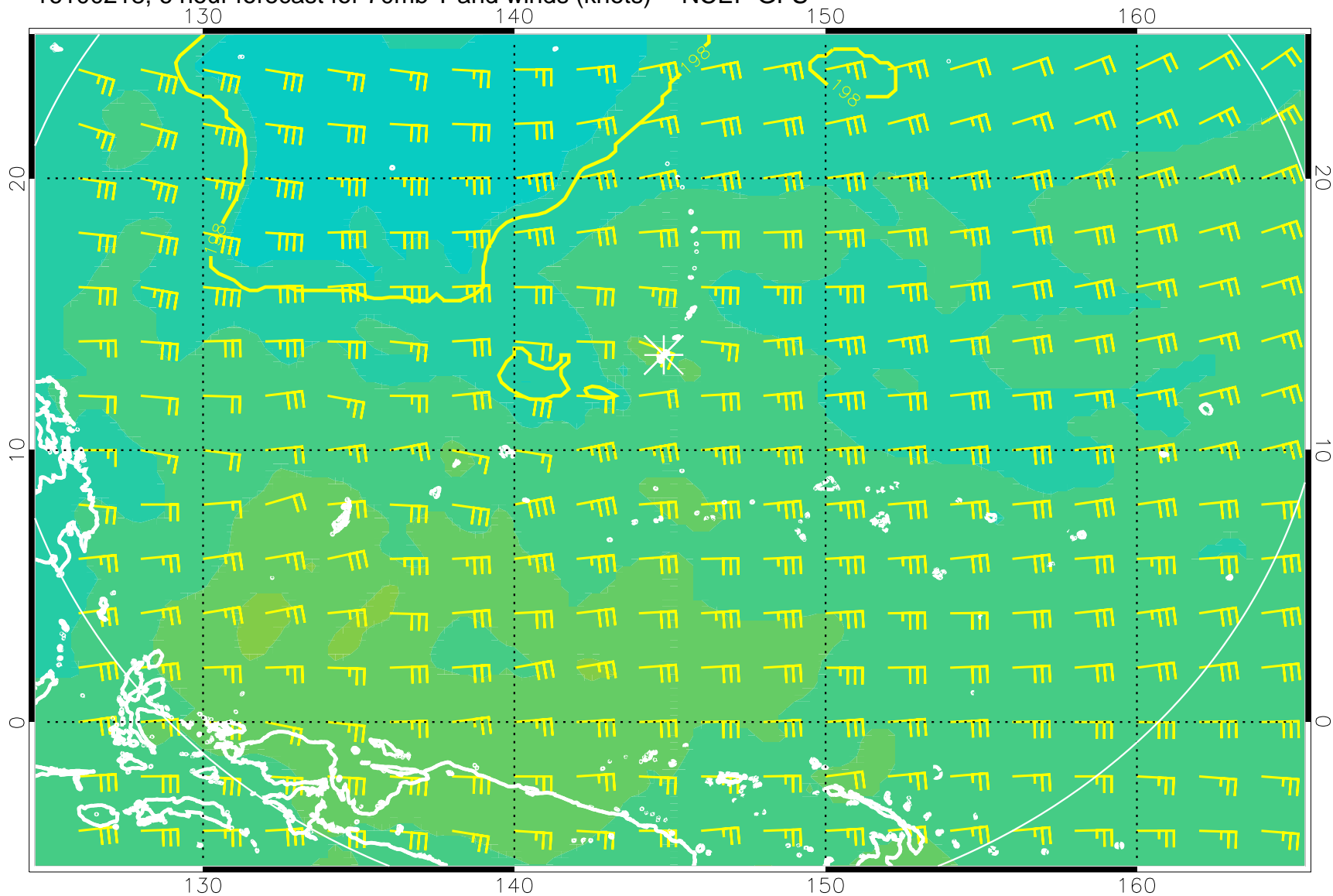
16100218, 6 hour forecast for 70mb T and winds (knots) -- NCEP GFS
