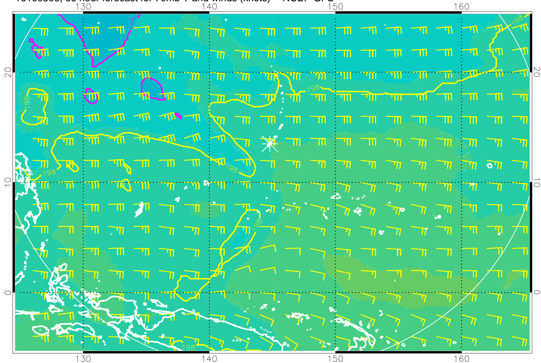
16100506, 66 hour forecast for 70mb T and winds (knots) -- NCEP GFS
