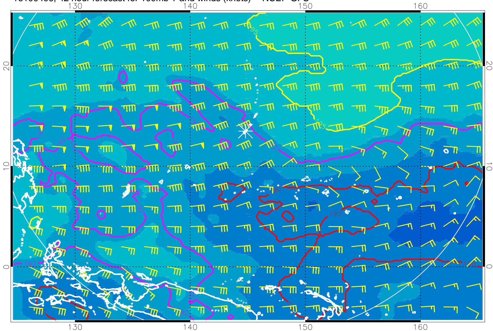
16100406, 42 hour forecast for 100mb T and winds (knots) -- NCEP GFS
