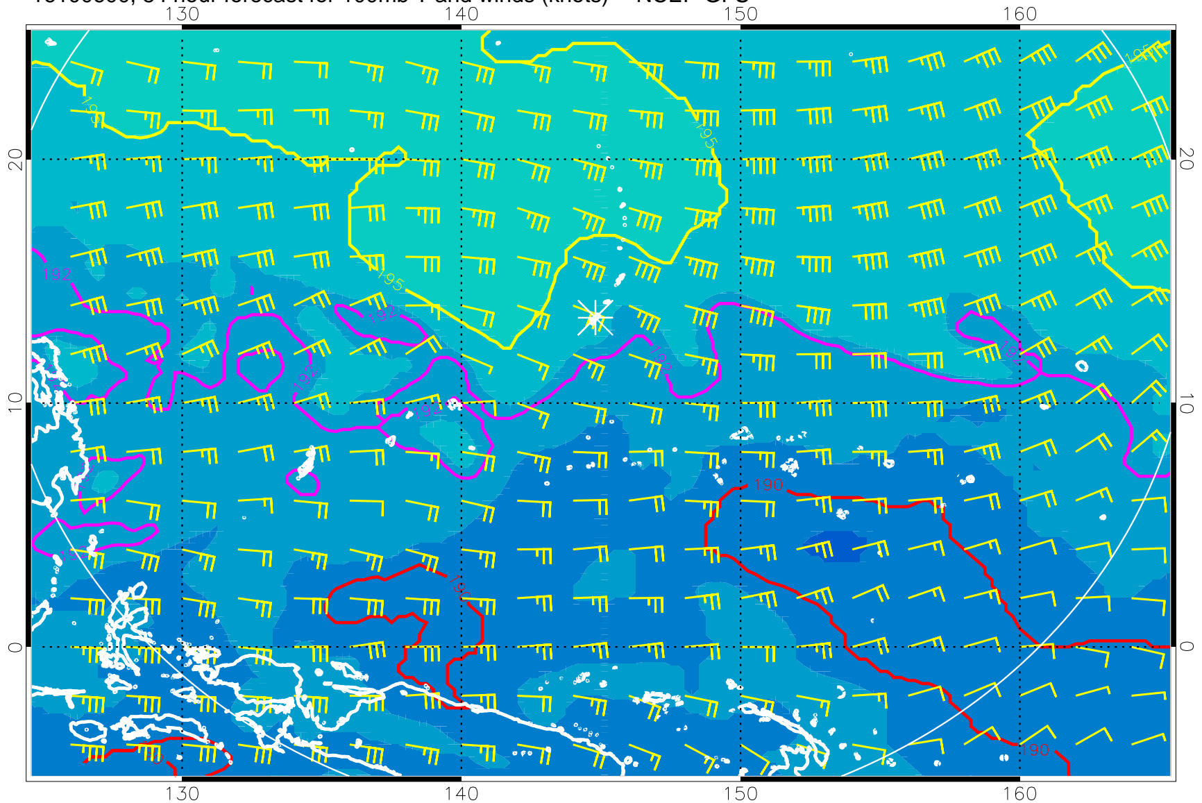
16100600, 84 hour forecast for 100mb T and winds (knots) -- NCEP GFS
