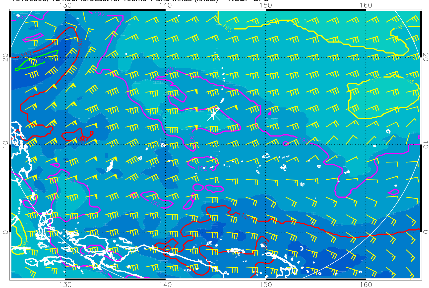
16100300, 12 hour forecast for 100mb T and winds (knots) -- NCEP GFS
