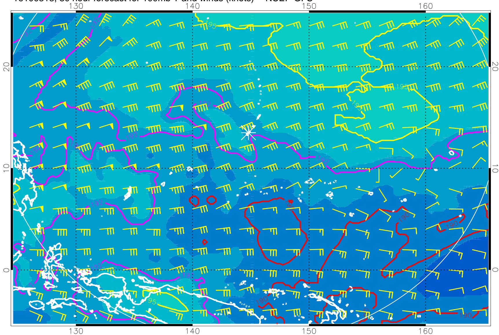
16100318, 30 hour forecast for 100mb T and winds (knots) -- NCEP GFS
