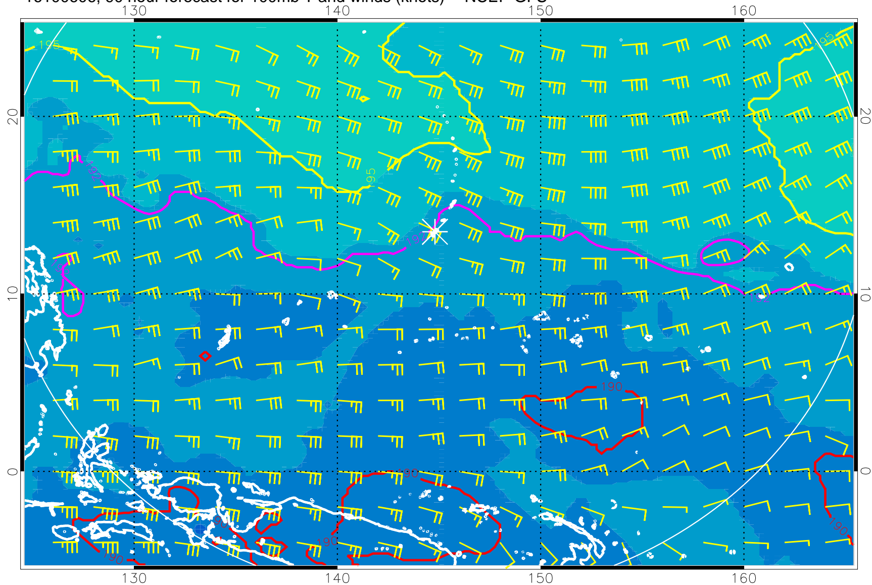
16100606, 90 hour forecast for 100mb T and winds (knots) -- NCEP GFS
