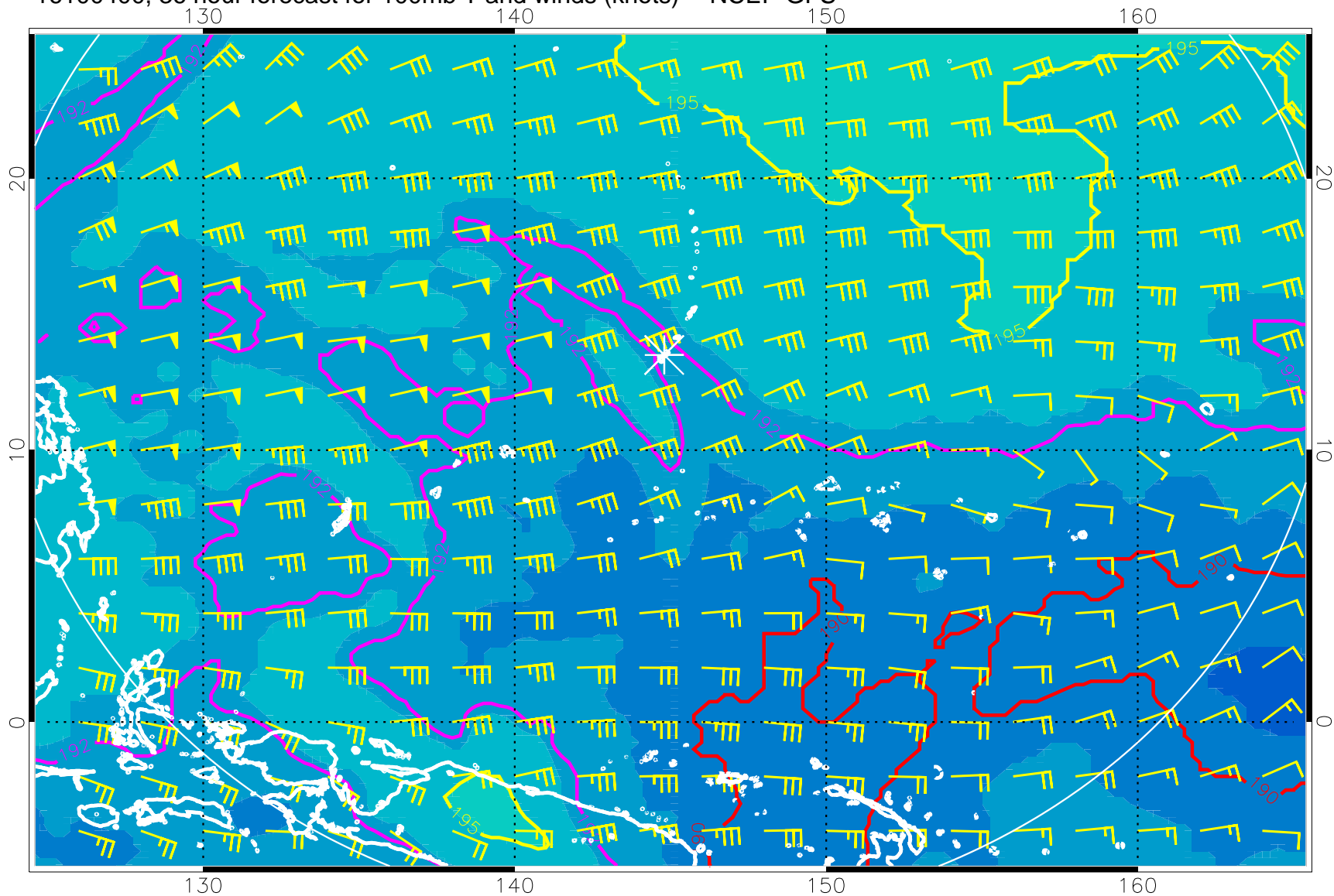
16100400, 36 hour forecast for 100mb T and winds (knots) -- NCEP GFS
