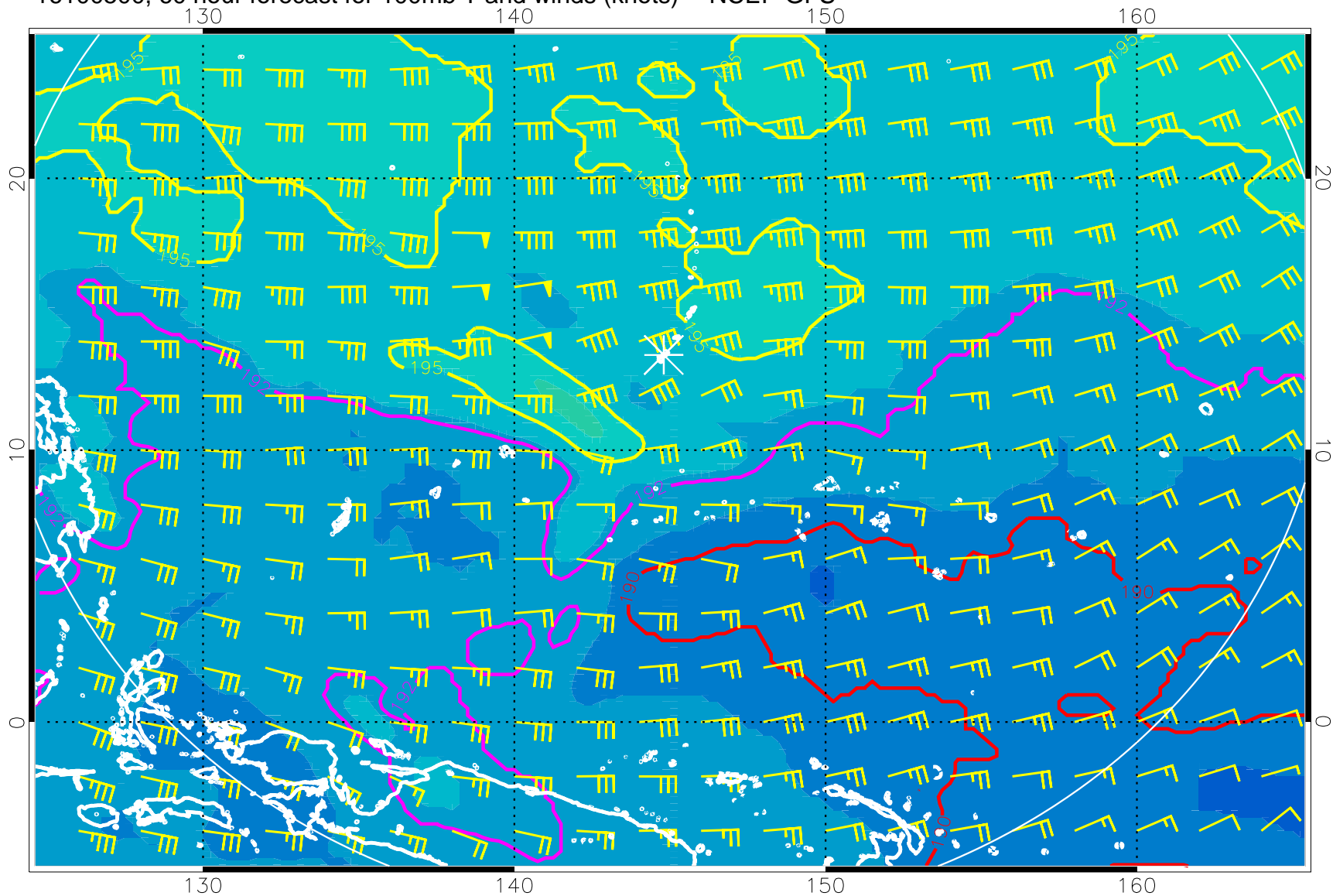
16100500, 60 hour forecast for 100mb T and winds (knots) -- NCEP GFS
