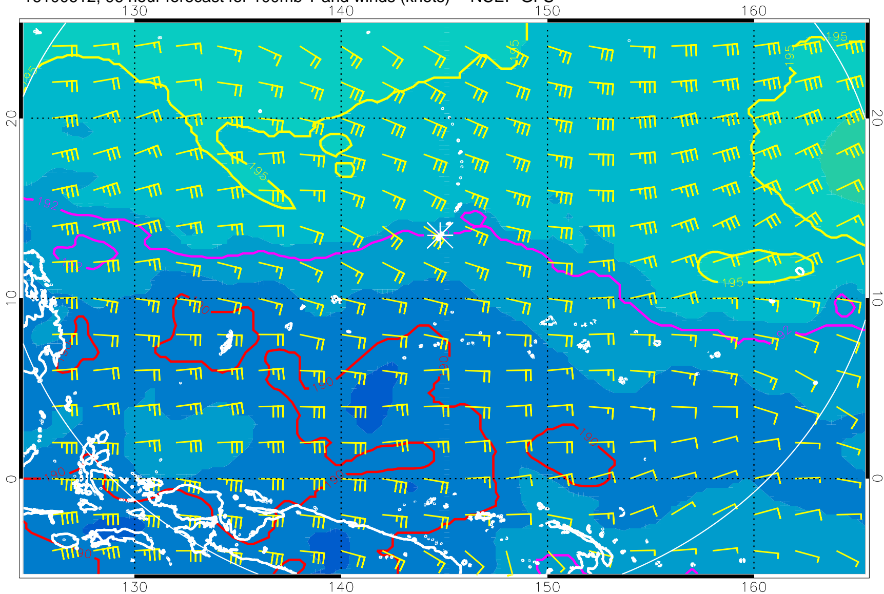
16100612, 96 hour forecast for 100mb T and winds (knots) -- NCEP GFS
