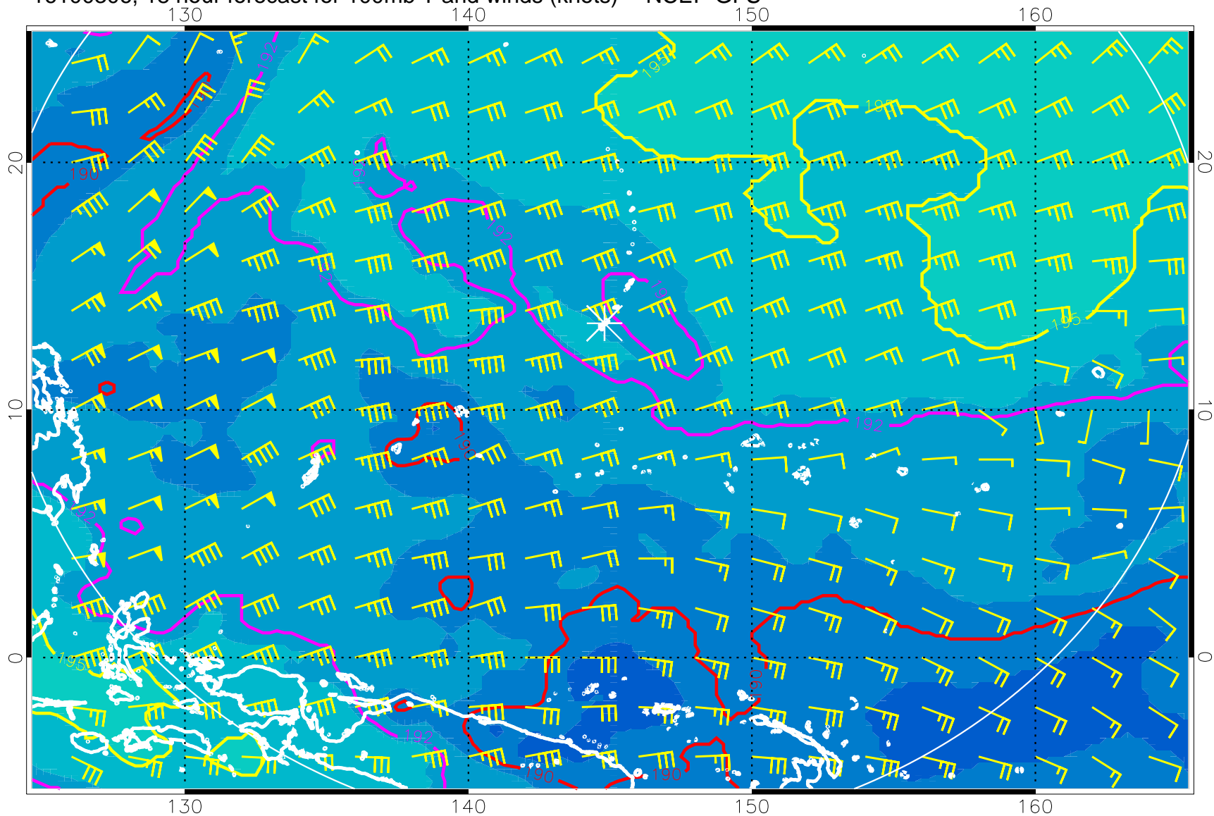
16100306, 18 hour forecast for 100mb T and winds (knots) -- NCEP GFS
