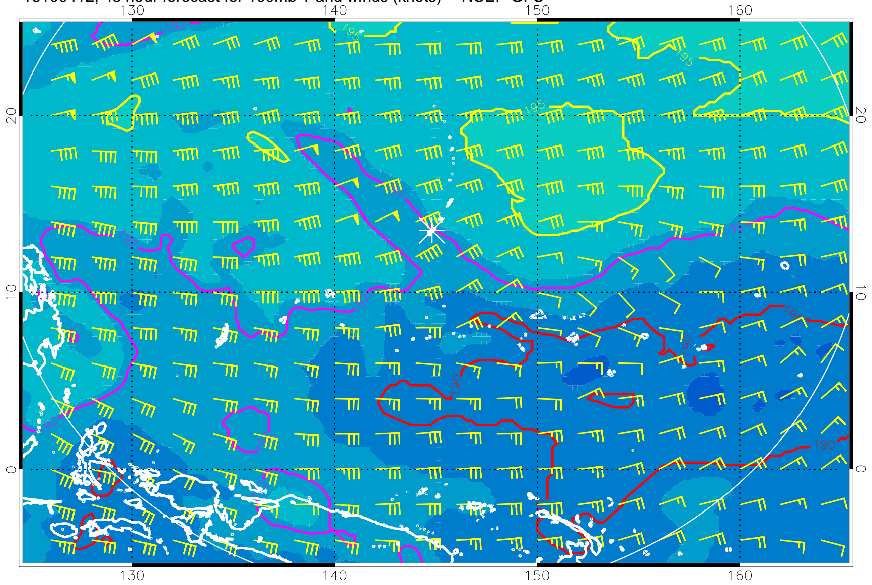
16100412, 48 hour forecast for 100mb T and winds (knots) -- NCEP GFS
