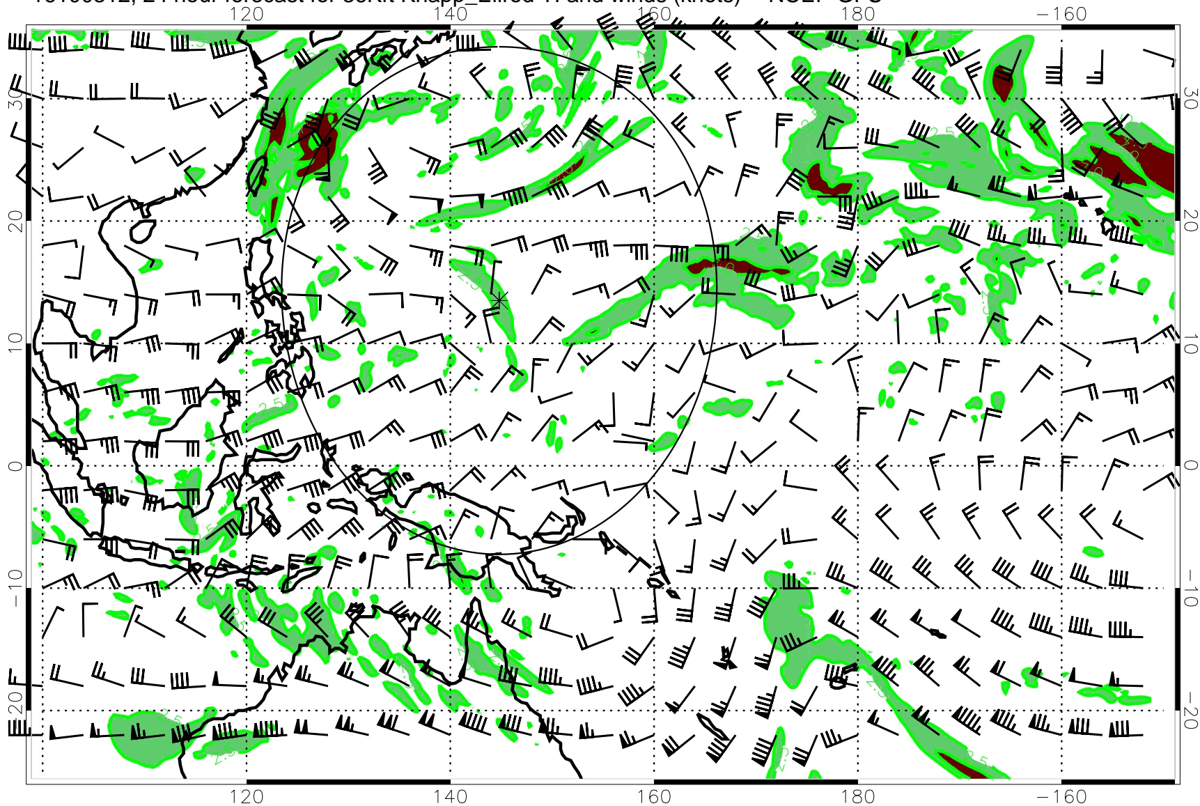
16100312, 24 hour forecast for 36Kft Knapp_Ellrod TI and winds (knots) -- NCEP GFS
