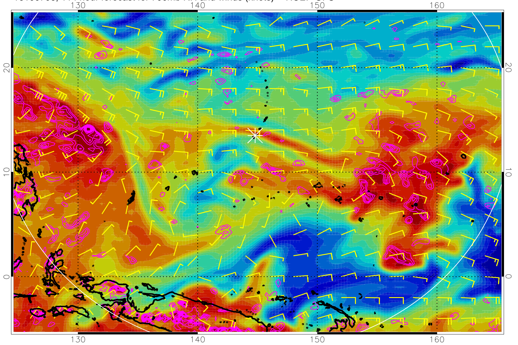
16100706, 114 hour forecast for 700mb RH and winds (knots) -- NCEP GFS
