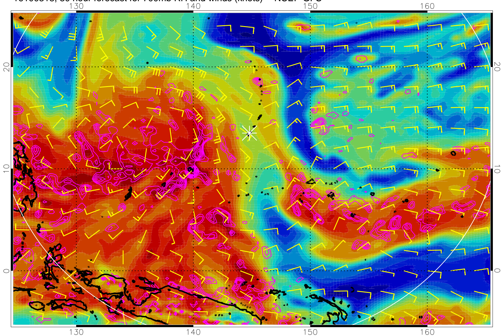
16100318, 30 hour forecast for 700mb RH and winds (knots) -- NCEP GFS
