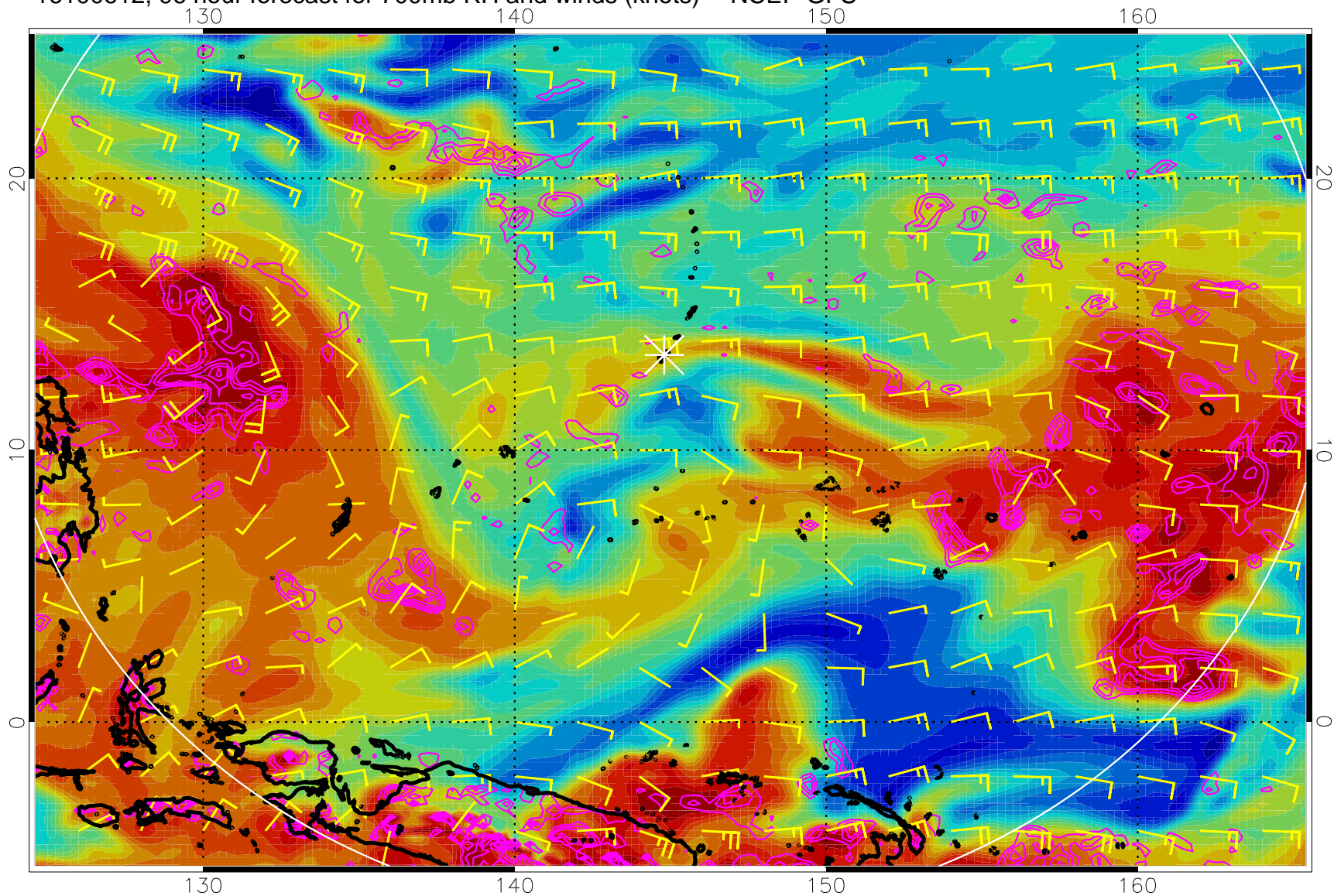
16100612, 96 hour forecast for 700mb RH and winds (knots) -- NCEP GFS
