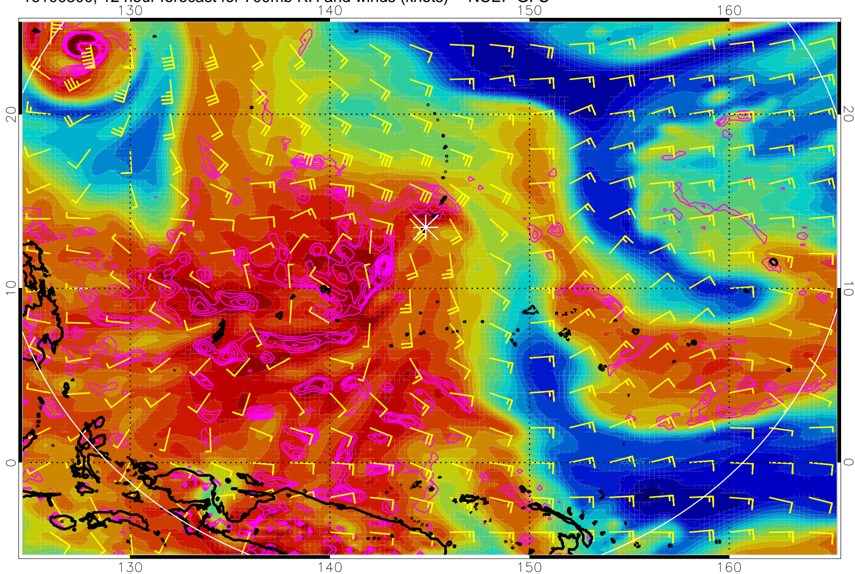
16100300, 12 hour forecast for 700mb RH and winds (knots) -- NCEP GFS
