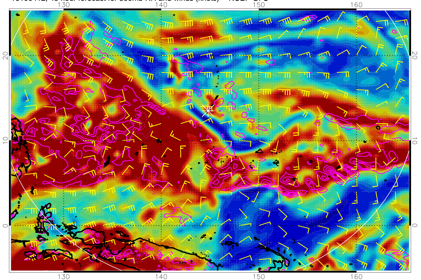
16100412, 48 hour forecast for 300mb RH and winds (knots) -- NCEP GFS
