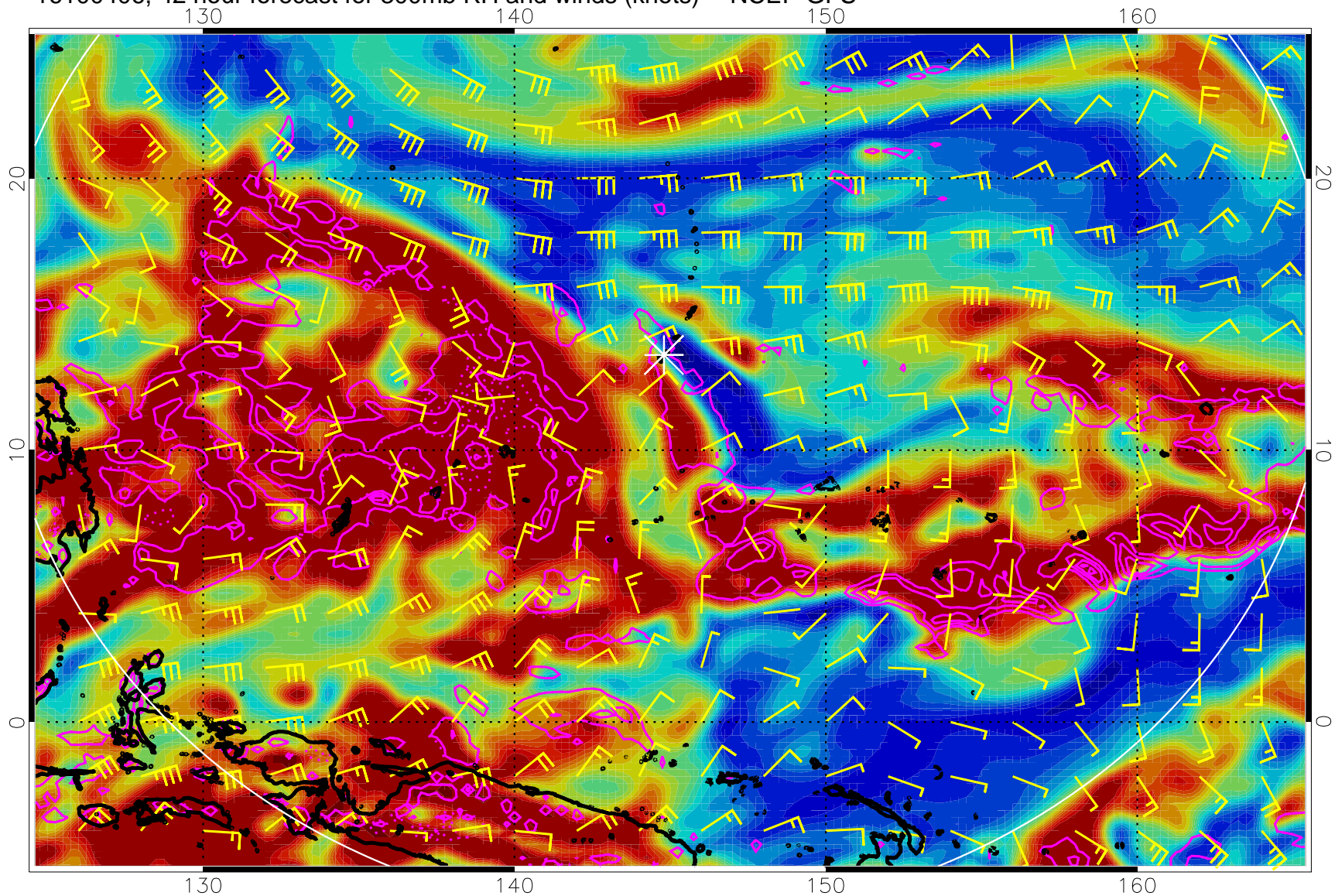
16100406, 42 hour forecast for 300mb RH and winds (knots) -- NCEP GFS
