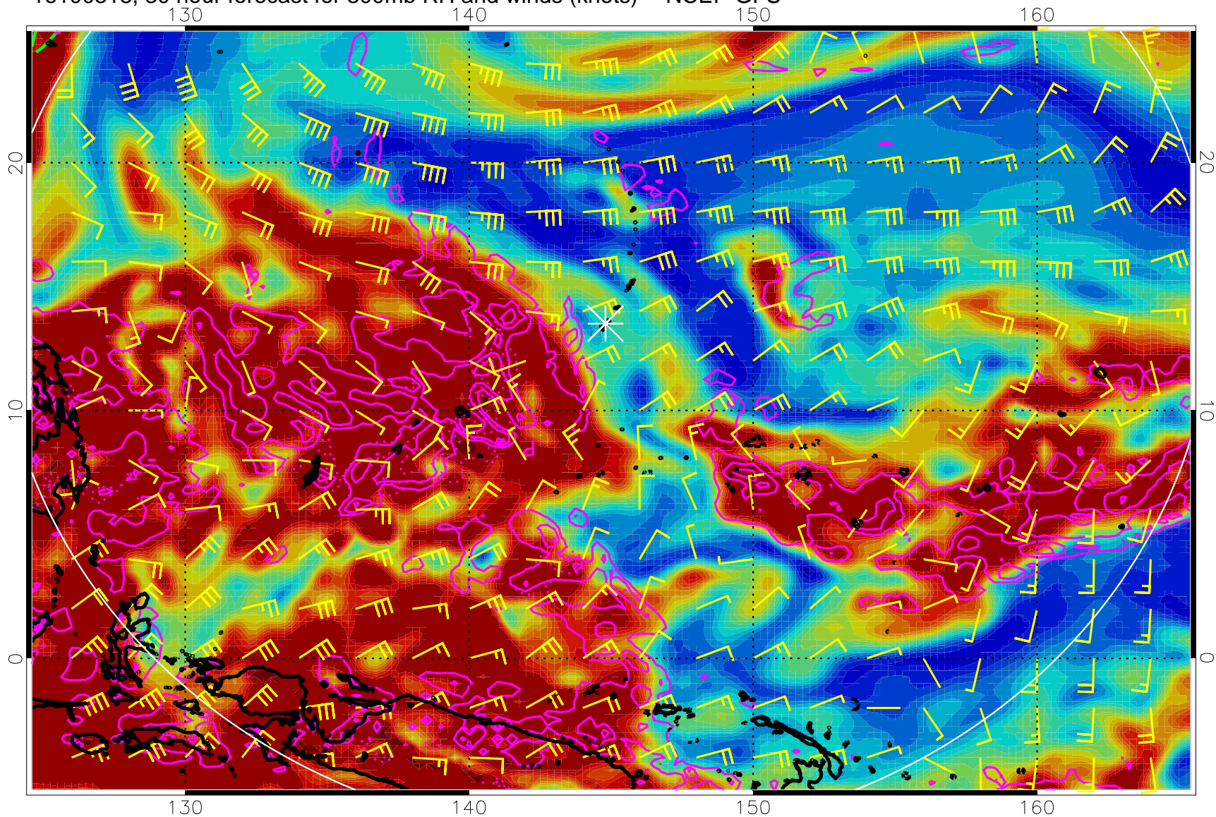
16100318, 30 hour forecast for 300mb RH and winds (knots) -- NCEP GFS
