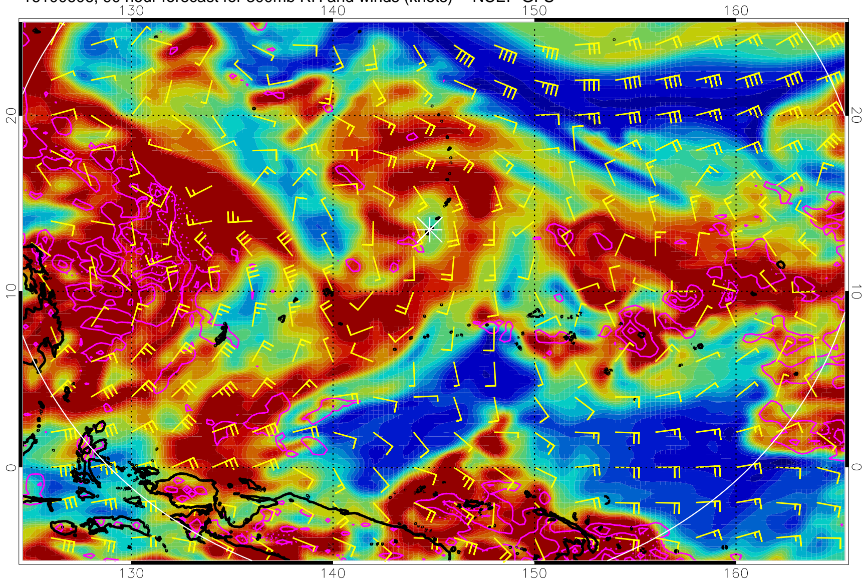
16100606, 90 hour forecast for 300mb RH and winds (knots) -- NCEP GFS
