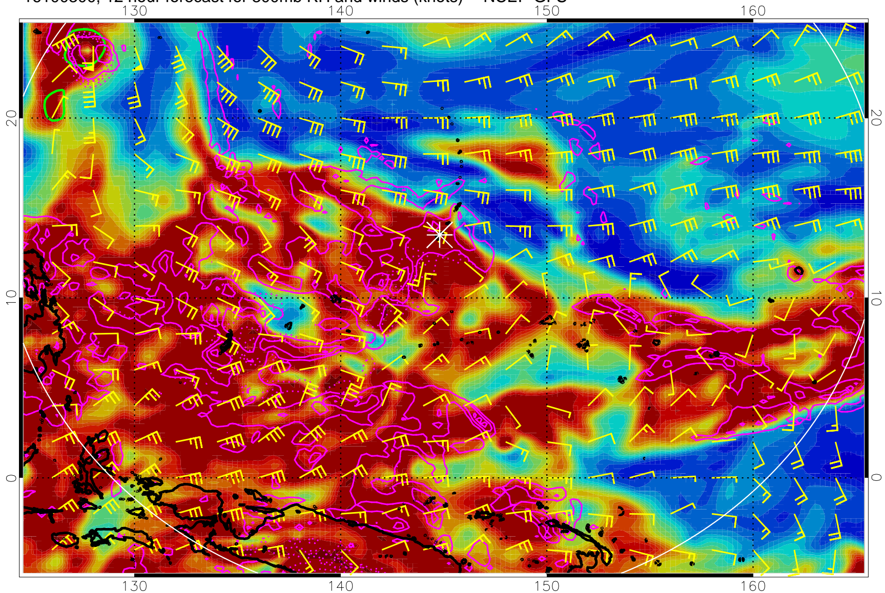
16100300, 12 hour forecast for 300mb RH and winds (knots) -- NCEP GFS
