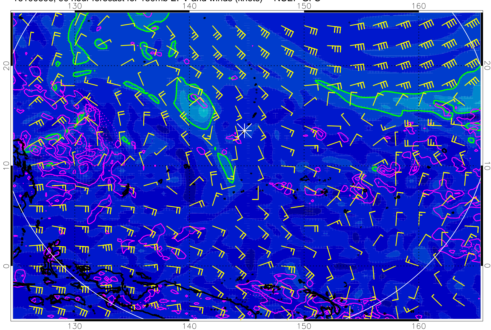
16100606, 90 hour forecast for 150mb EPV and winds (knots) -- NCEP GFS
