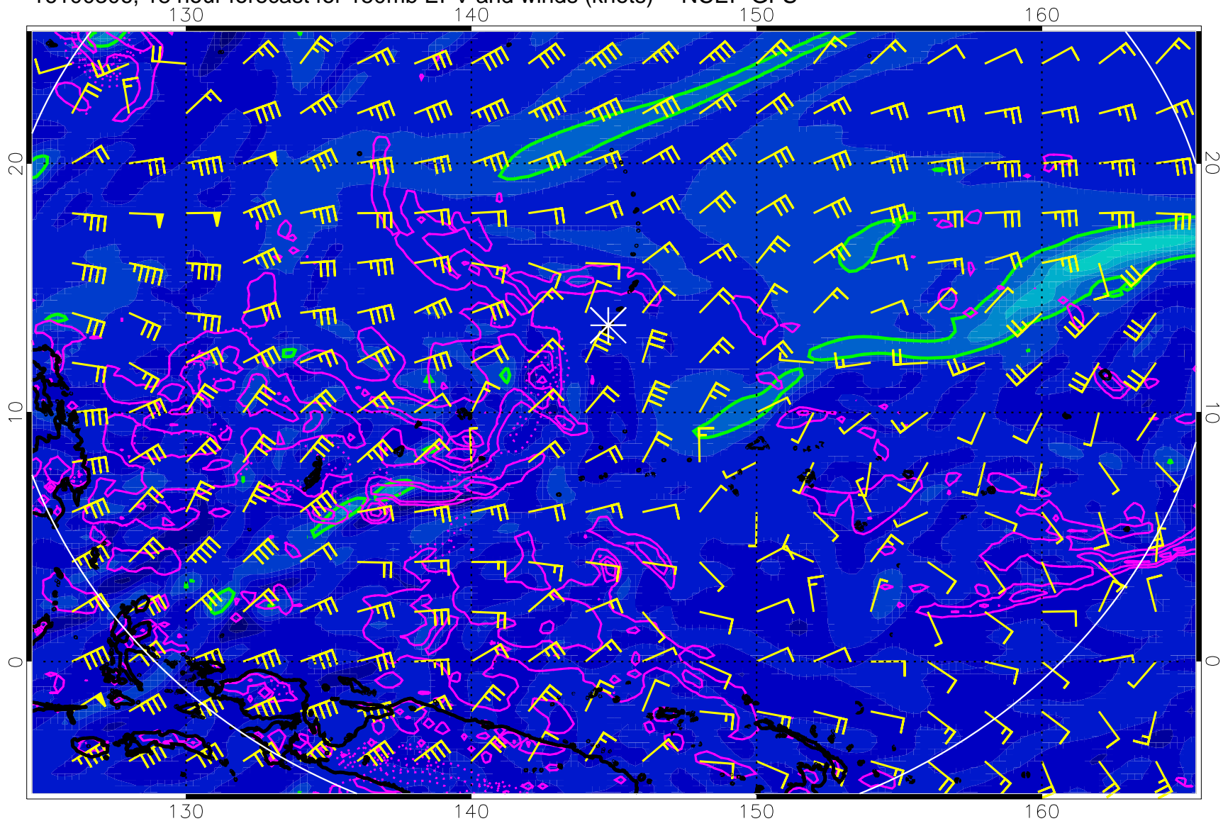
16100306, 18 hour forecast for 150mb EPV and winds (knots) -- NCEP GFS
