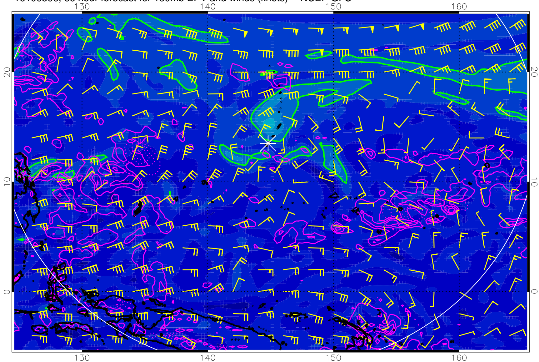
16100506, 66 hour forecast for 150mb EPV and winds (knots) -- NCEP GFS
