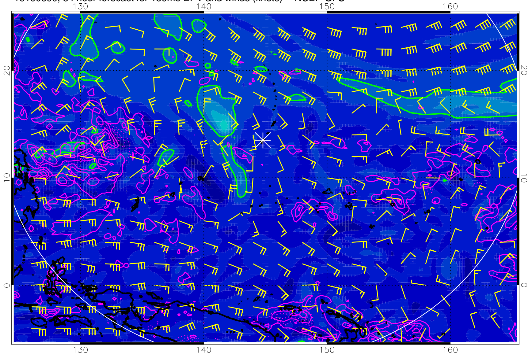
16100600, 84 hour forecast for 150mb EPV and winds (knots) -- NCEP GFS
