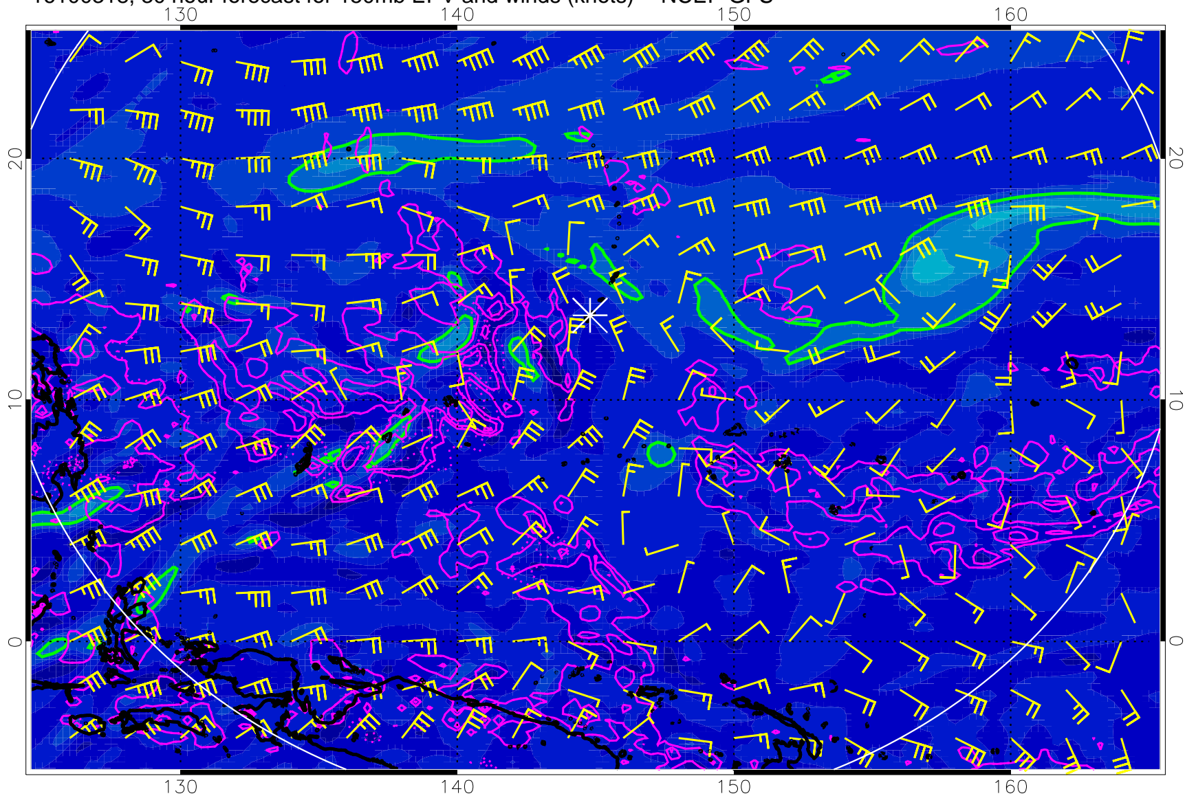
16100318, 30 hour forecast for 150mb EPV and winds (knots) -- NCEP GFS
