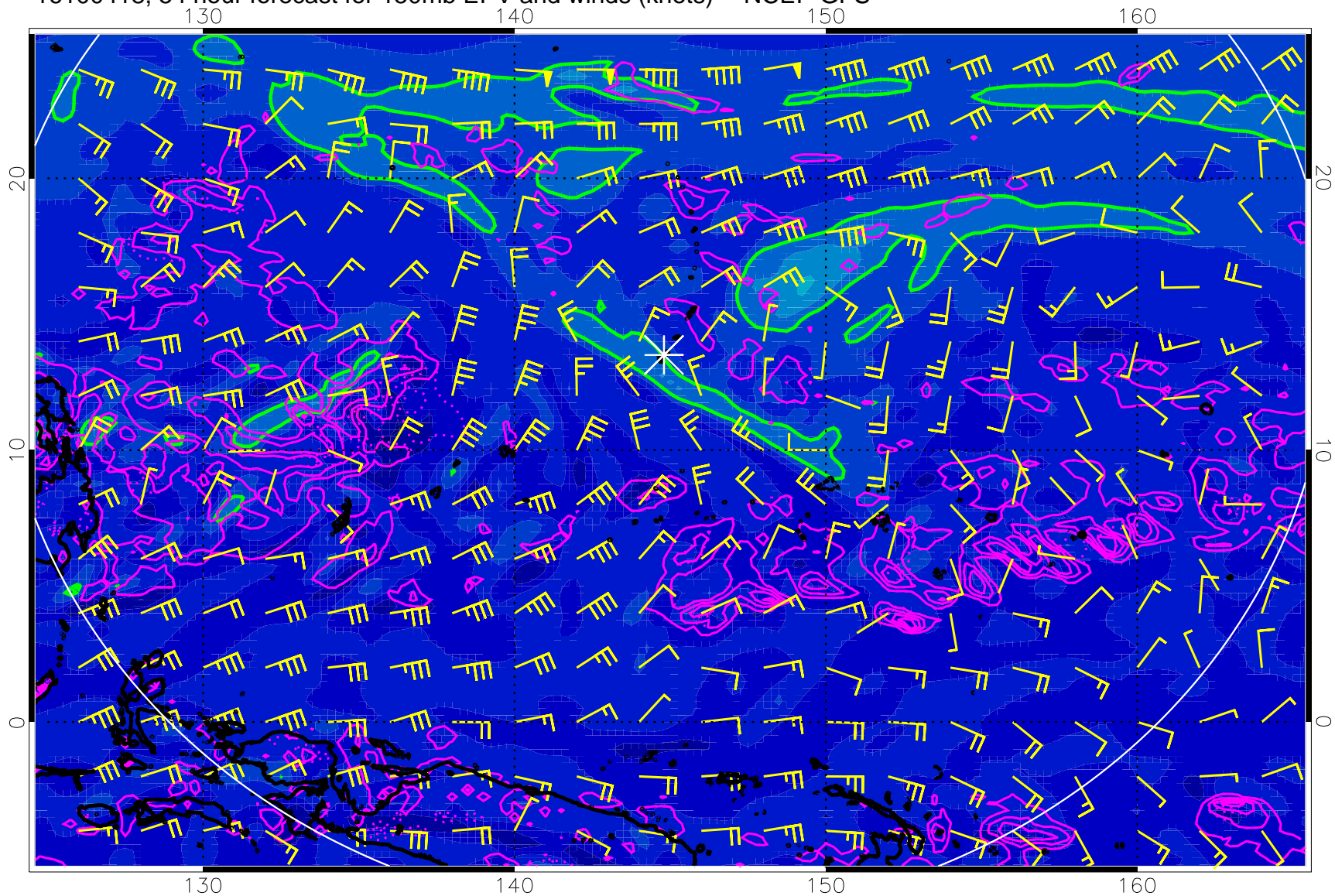
16100418, 54 hour forecast for 150mb EPV and winds (knots) -- NCEP GFS
