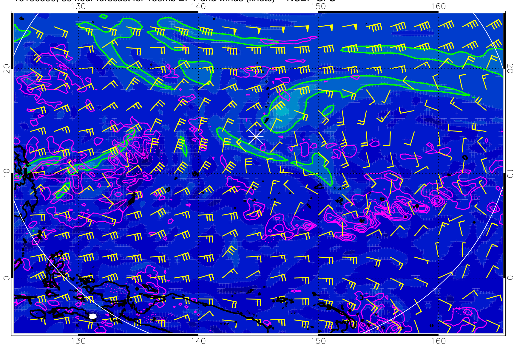
16100500, 60 hour forecast for 150mb EPV and winds (knots) -- NCEP GFS
