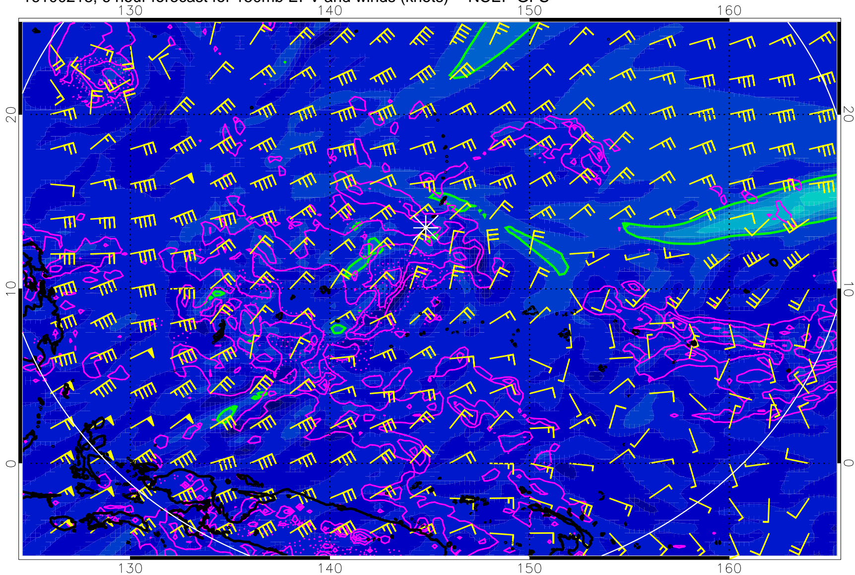
16100218, 6 hour forecast for 150mb EPV and winds (knots) -- NCEP GFS
