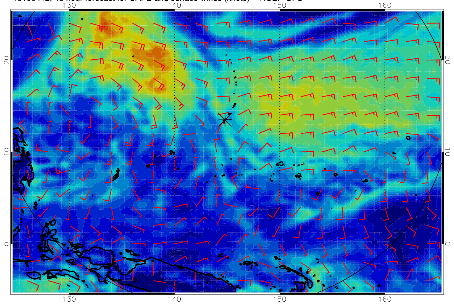
16100412, 48 hour forecast for CAPE and surface winds (knots) -- NCEP GFS
