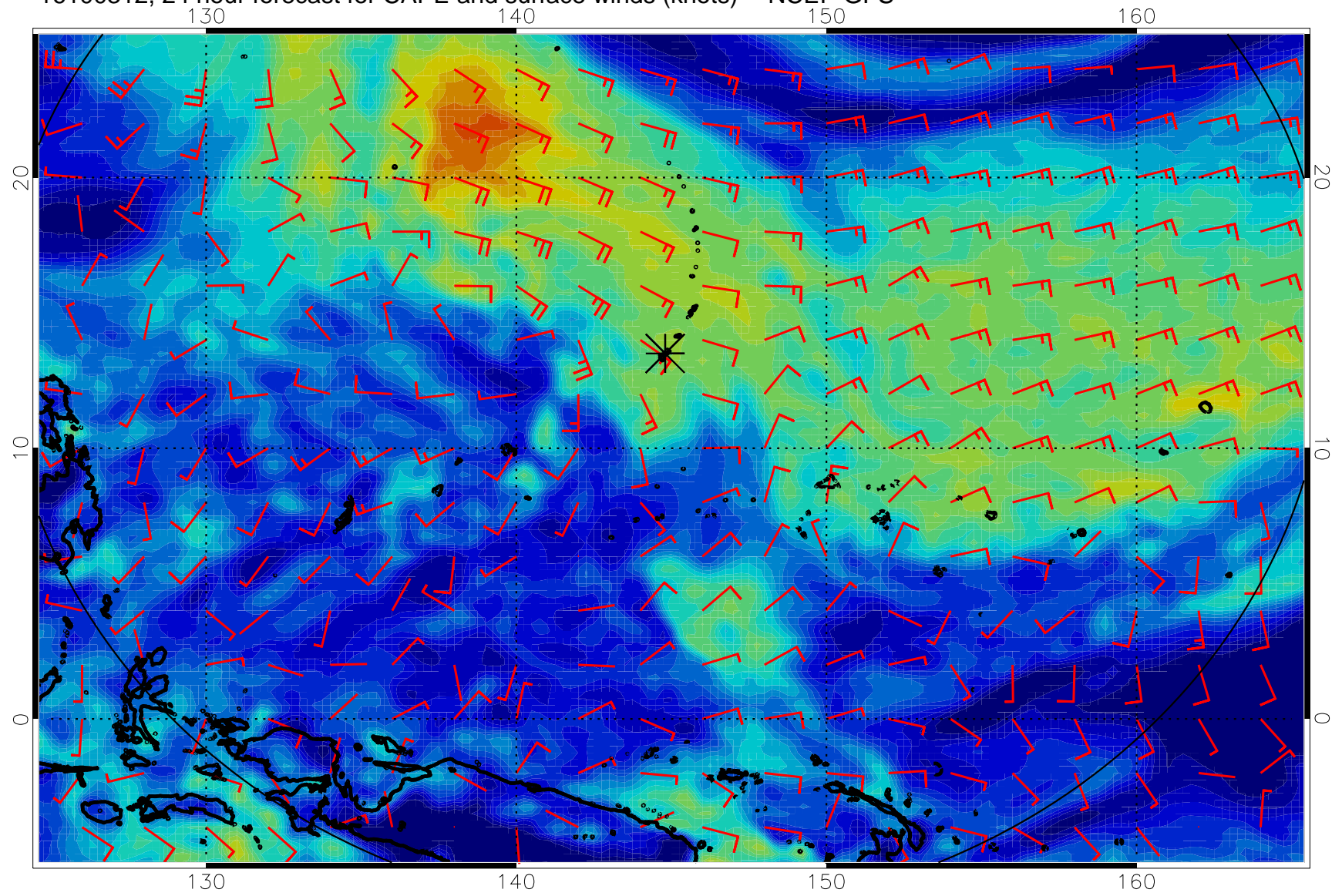
16100312, 24 hour forecast for CAPE and surface winds (knots) -- NCEP GFS
