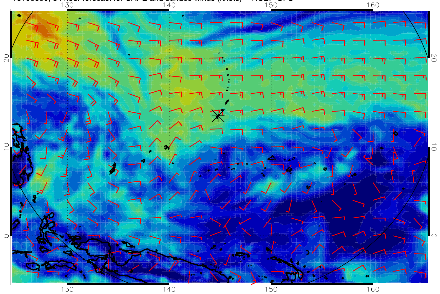
16100600, 84 hour forecast for CAPE and surface winds (knots) -- NCEP GFS
