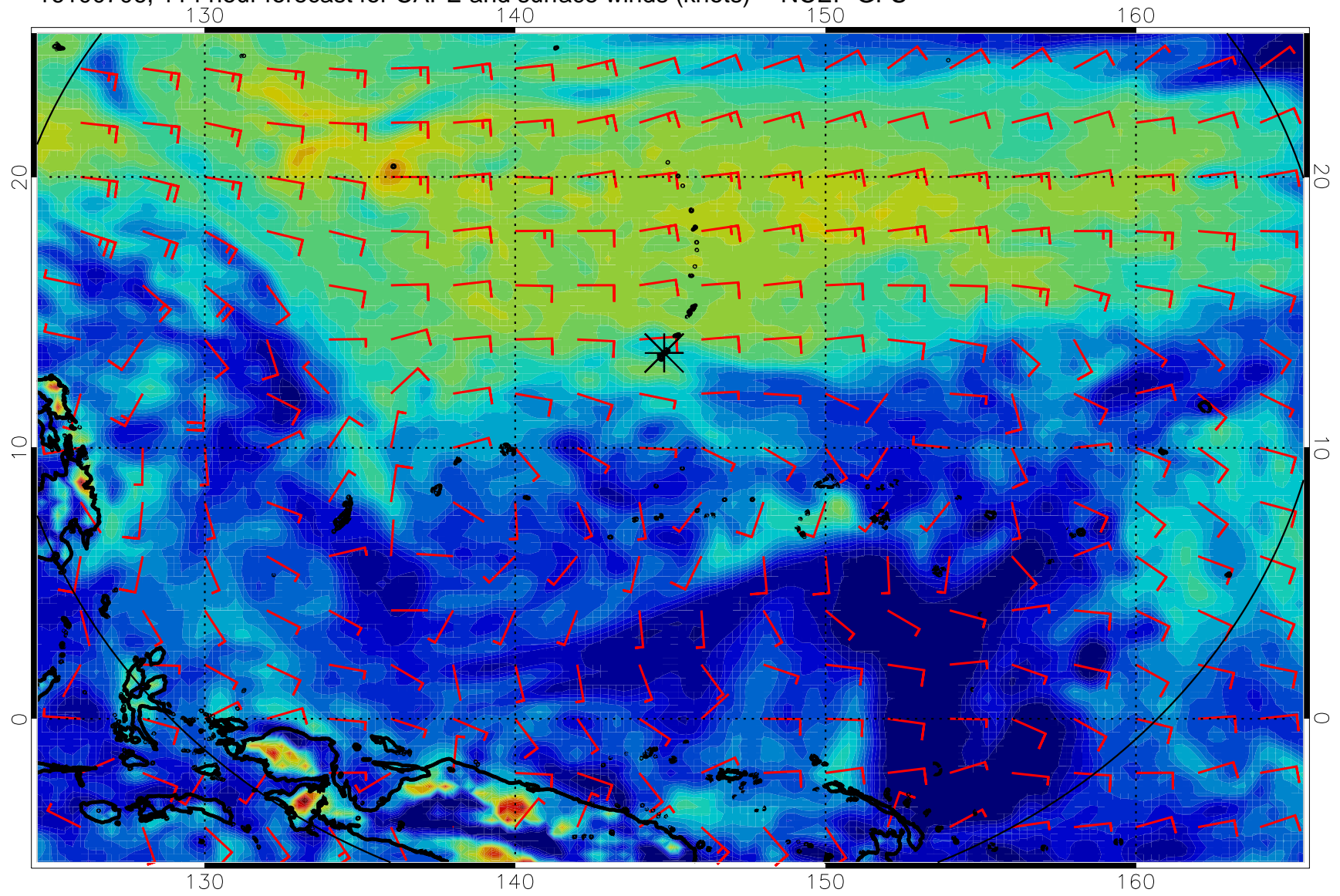
16100706, 114 hour forecast for CAPE and surface winds (knots) -- NCEP GFS
