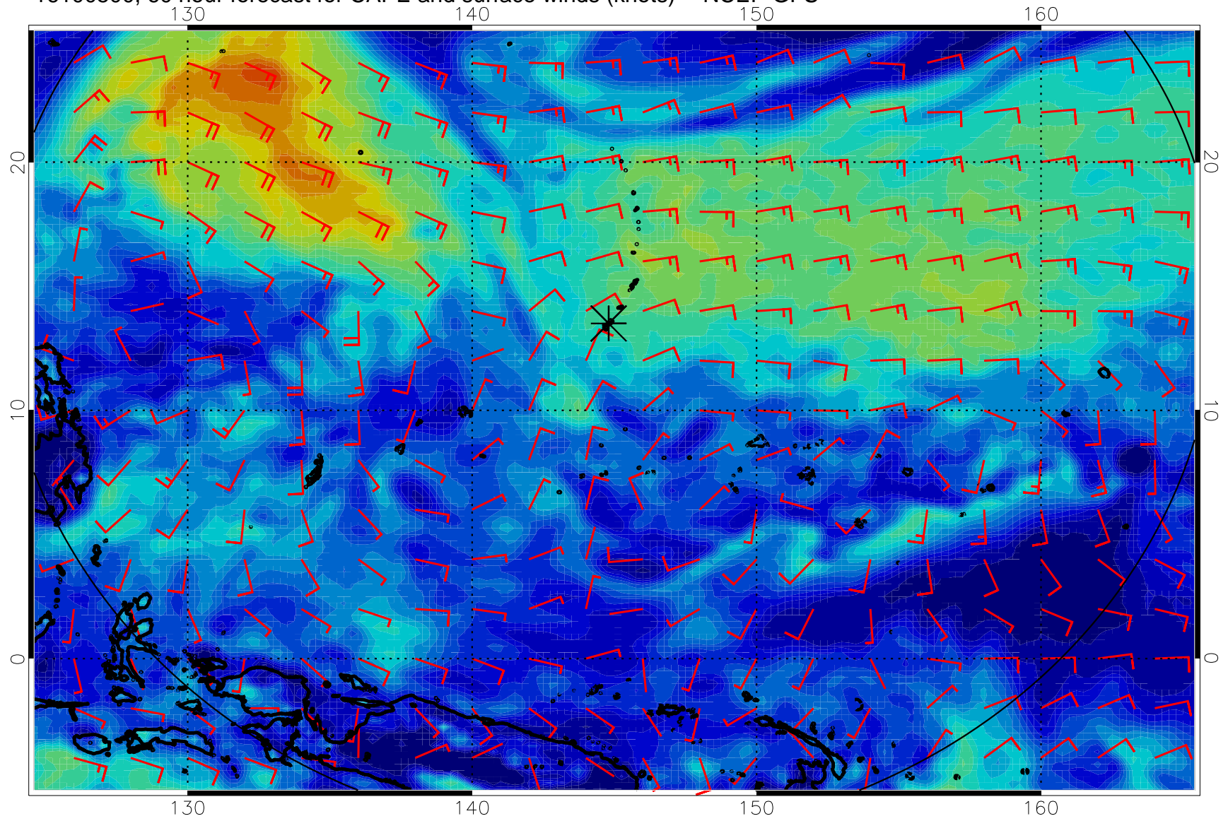
16100500, 60 hour forecast for CAPE and surface winds (knots) -- NCEP GFS
