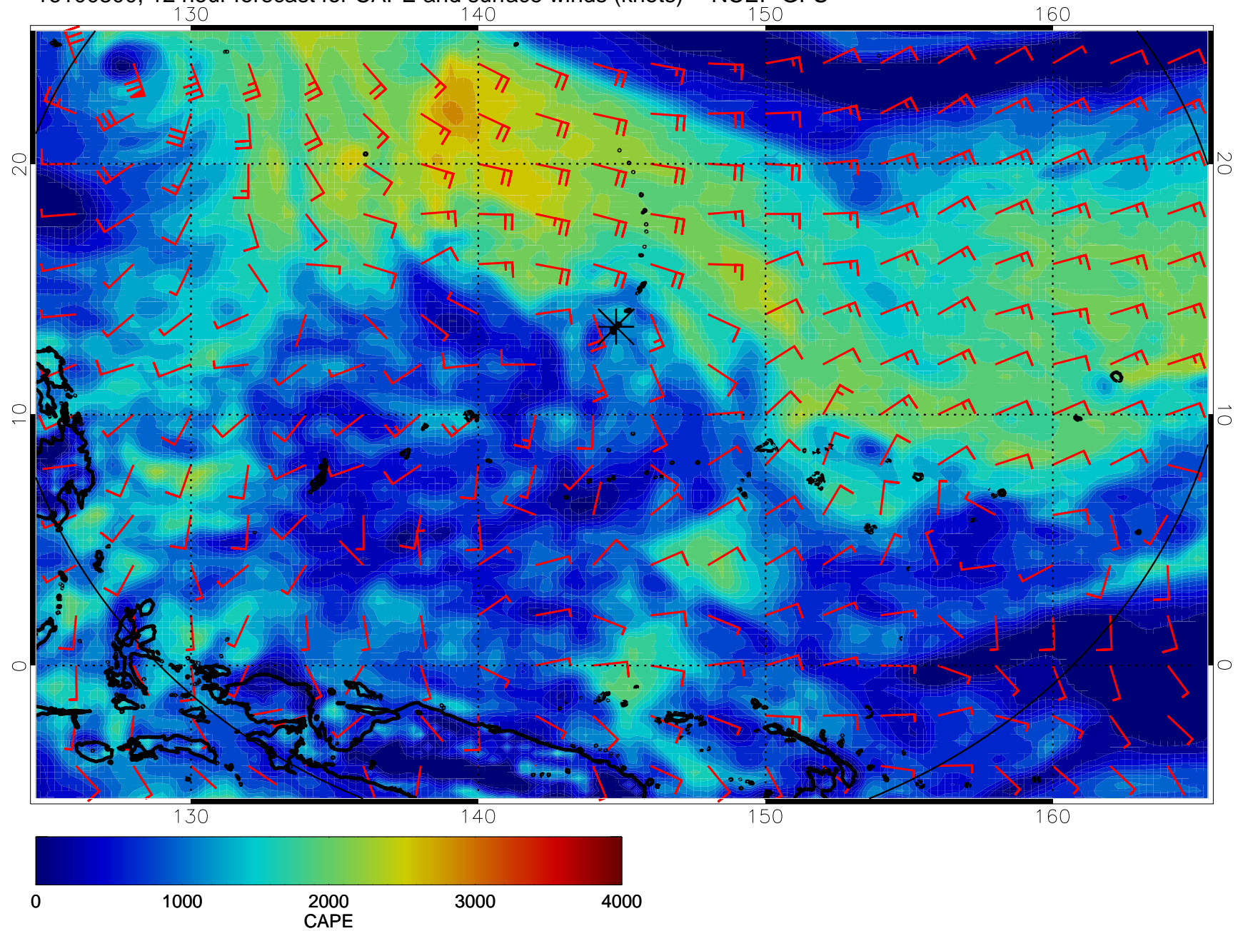
16100300, 12 hour forecast for CAPE and surface winds (knots) -- NCEP GFS
