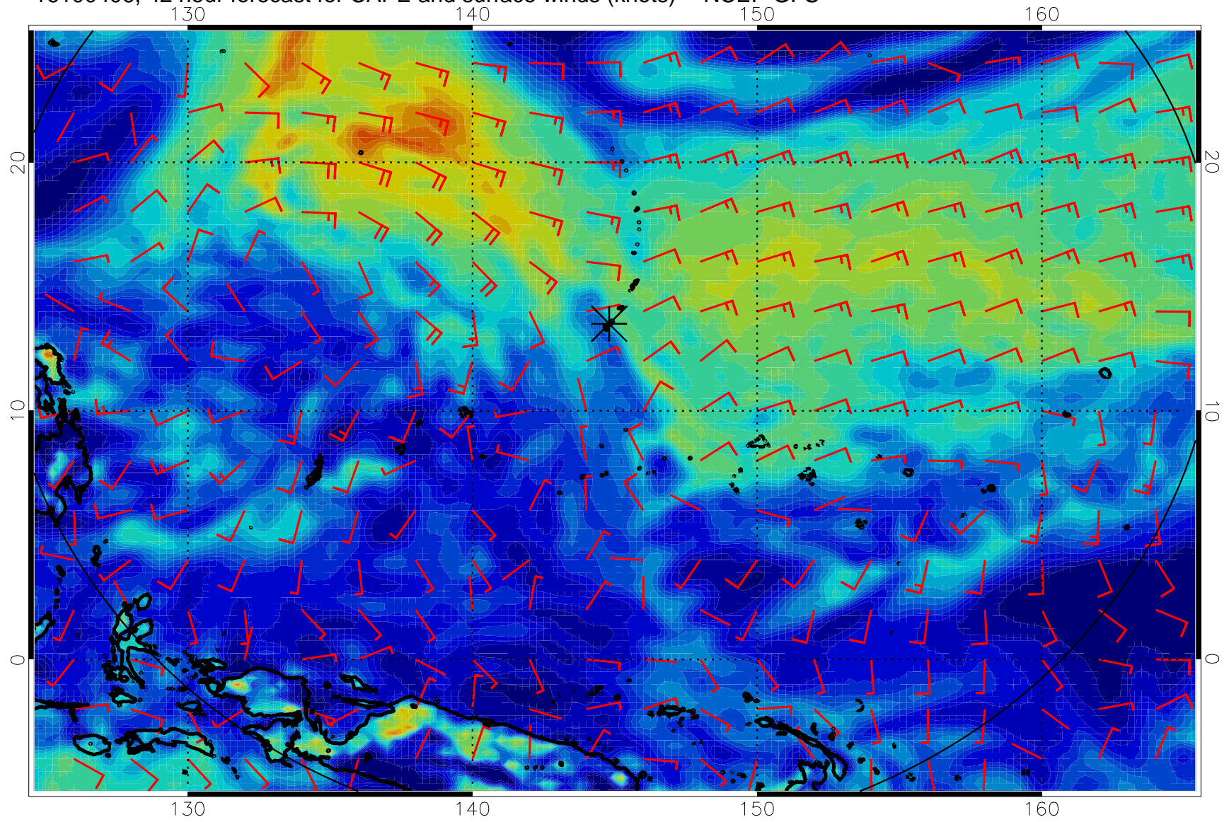
16100406, 42 hour forecast for CAPE and surface winds (knots) -- NCEP GFS
