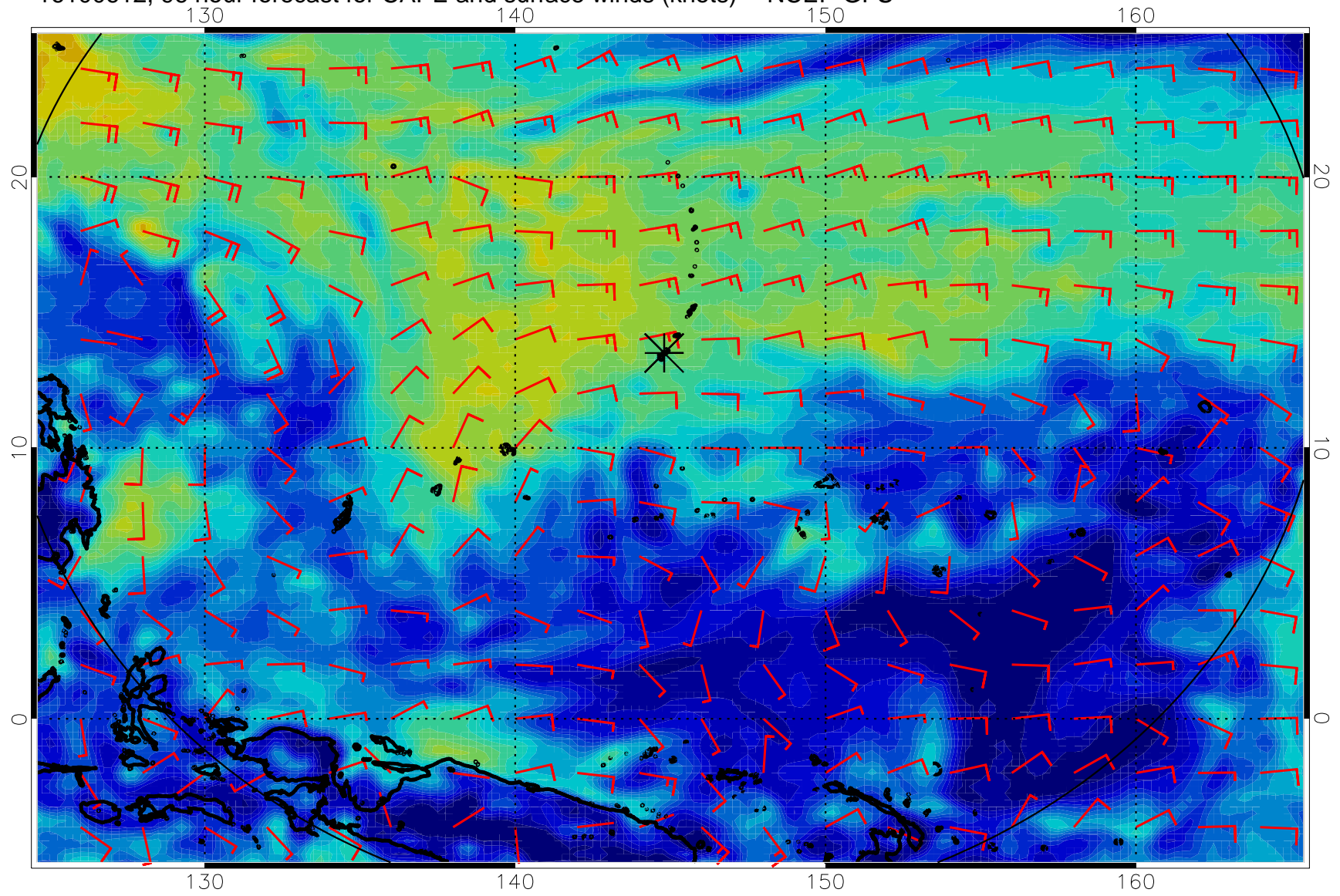
16100612, 96 hour forecast for CAPE and surface winds (knots) -- NCEP GFS
