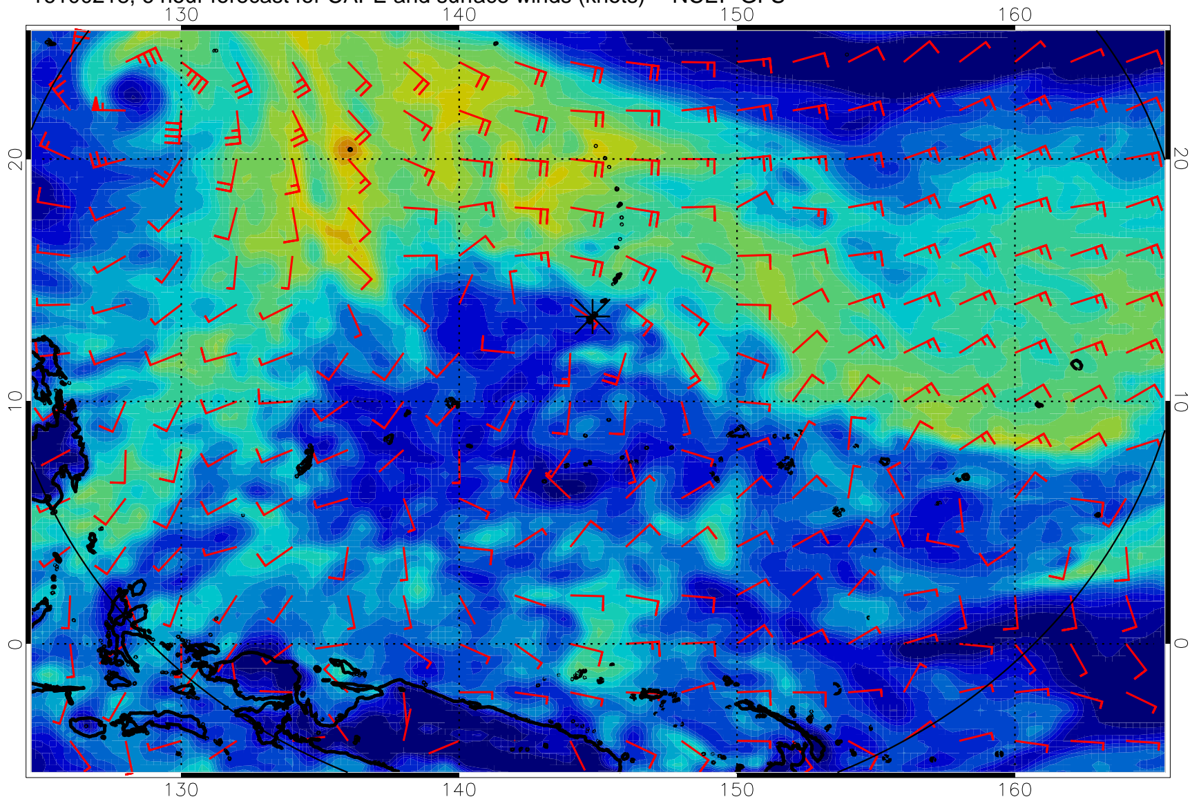
16100218, 6 hour forecast for CAPE and surface winds (knots) -- NCEP GFS
