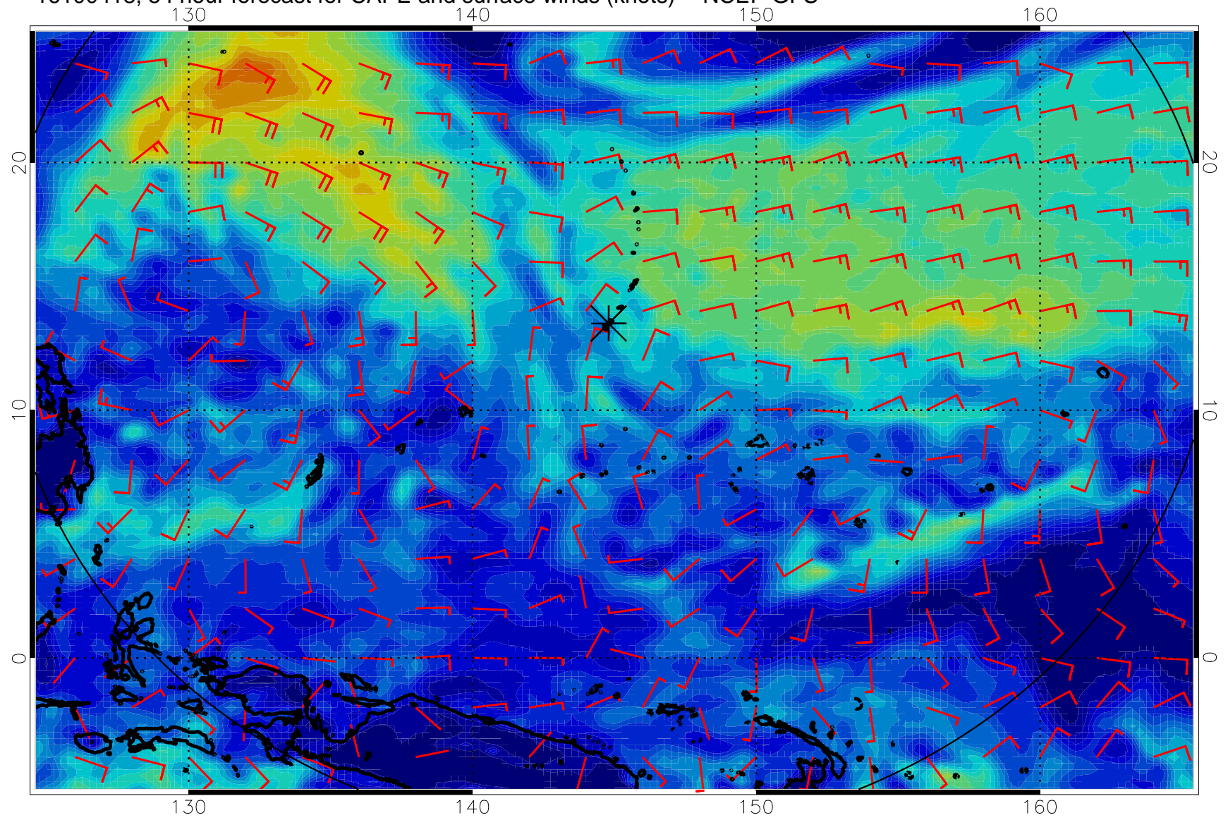
16100418, 54 hour forecast for CAPE and surface winds (knots) -- NCEP GFS
