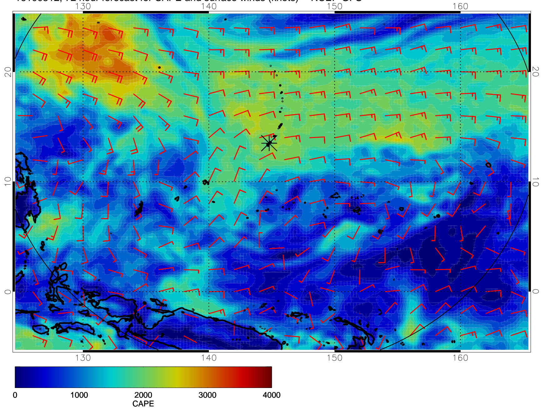
16100512, 72 hour forecast for CAPE and surface winds (knots) -- NCEP GFS
