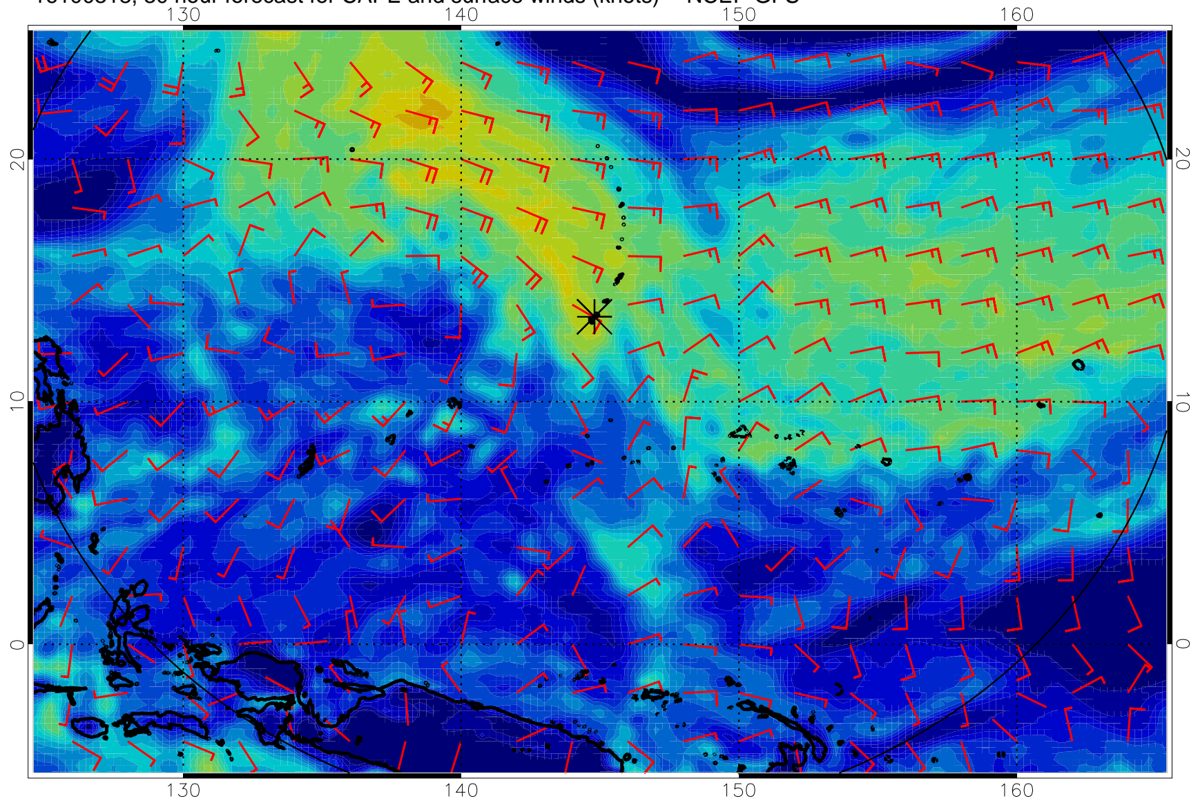
16100318, 30 hour forecast for CAPE and surface winds (knots) -- NCEP GFS
