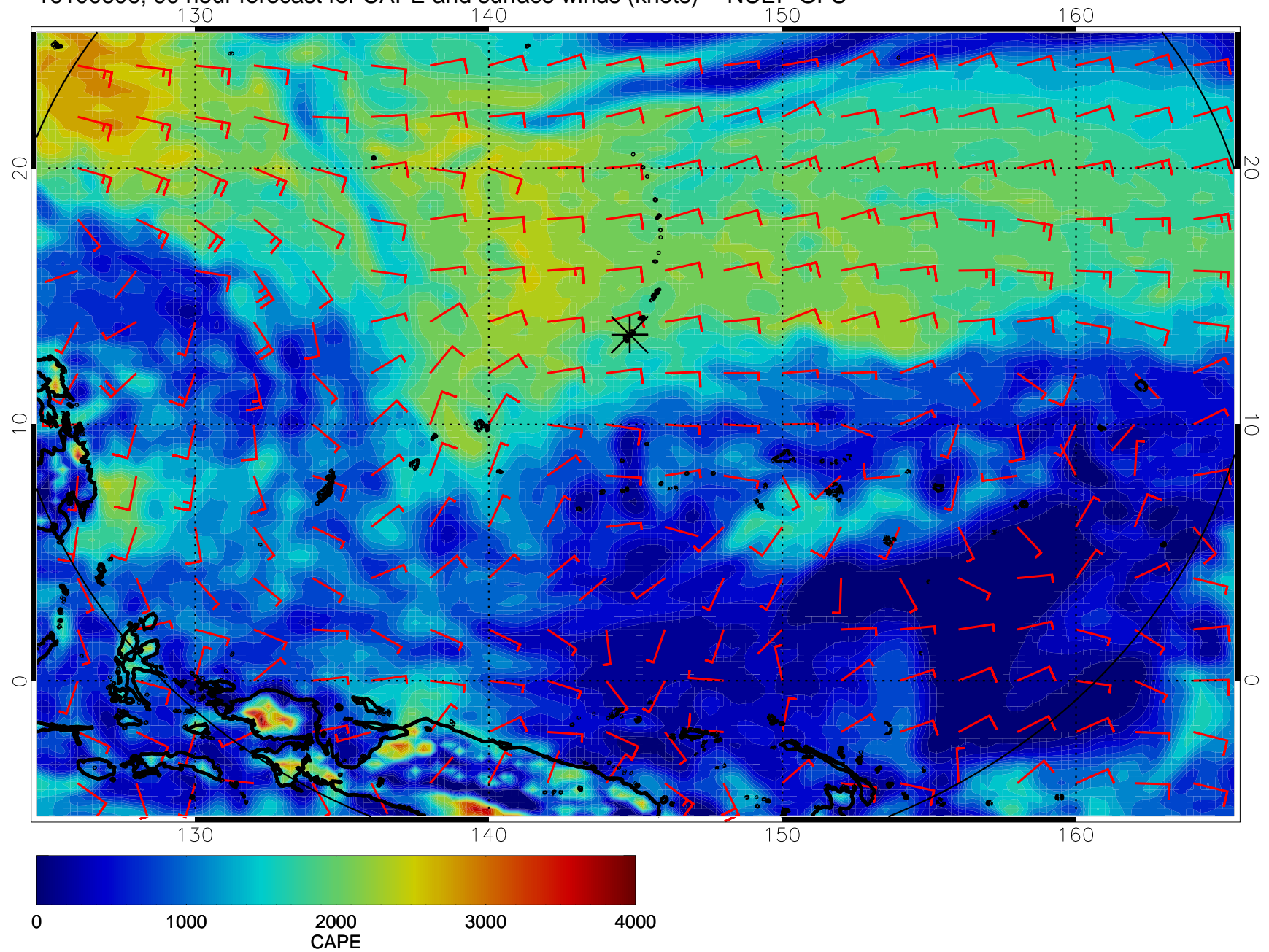
16100606, 90 hour forecast for CAPE and surface winds (knots) -- NCEP GFS
