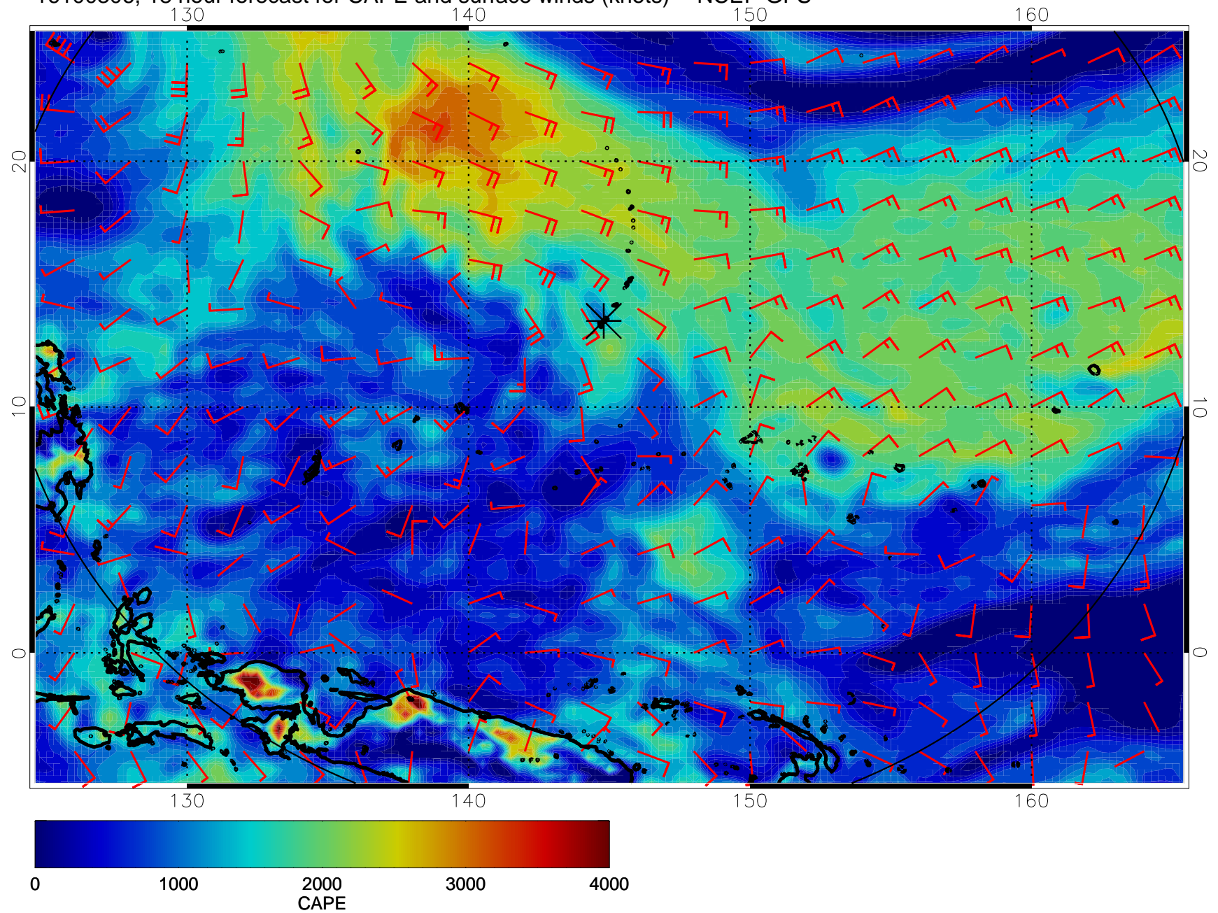
16100306, 18 hour forecast for CAPE and surface winds (knots) -- NCEP GFS
