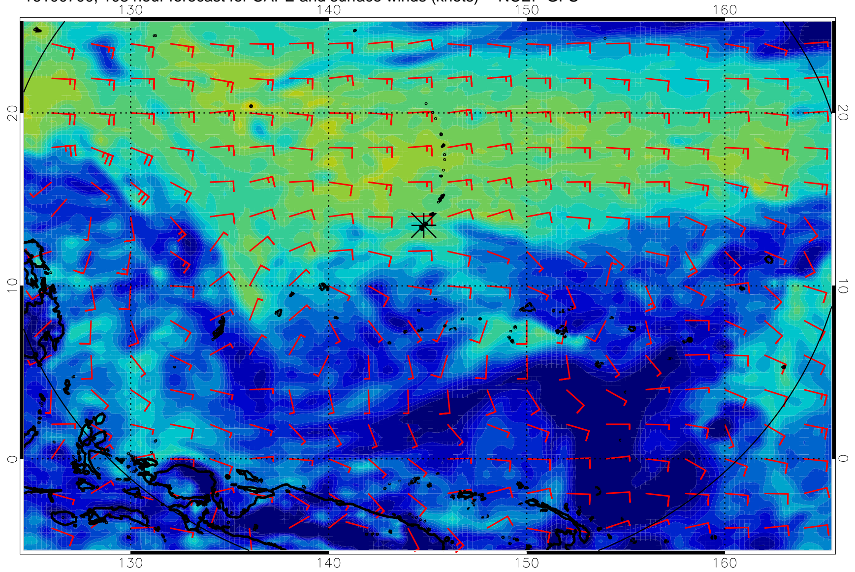
16100700, 108 hour forecast for CAPE and surface winds (knots) -- NCEP GFS
