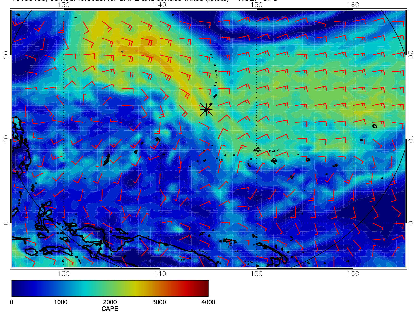
16100400, 36 hour forecast for CAPE and surface winds (knots) -- NCEP GFS
