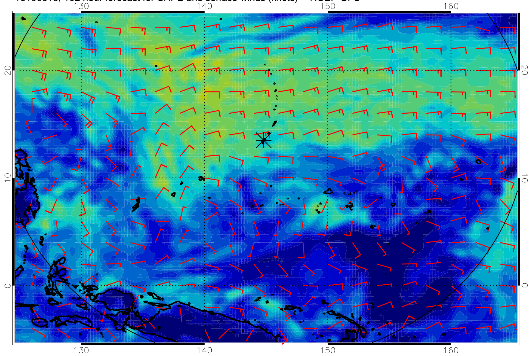
16100618, 102 hour forecast for CAPE and surface winds (knots) -- NCEP GFS
