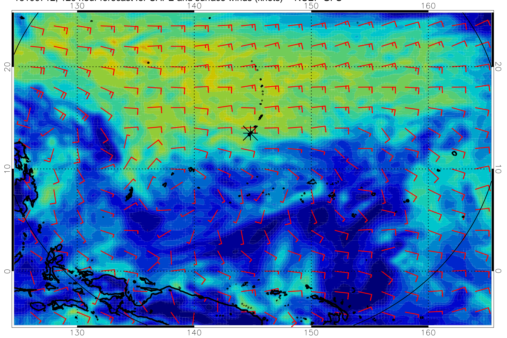
16100712, 120 hour forecast for CAPE and surface winds (knots) -- NCEP GFS
