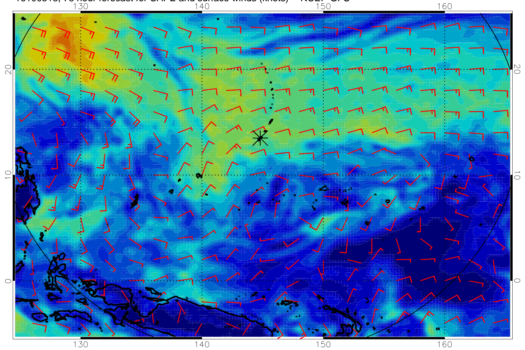
16100518, 78 hour forecast for CAPE and surface winds (knots) -- NCEP GFS
