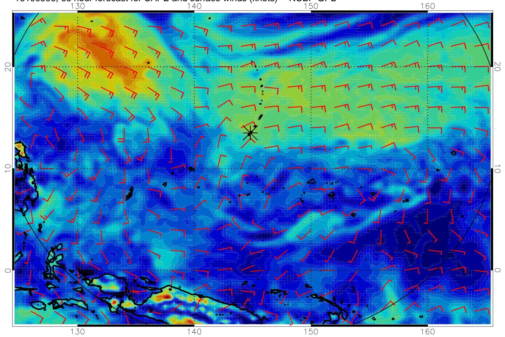
16100506, 66 hour forecast for CAPE and surface winds (knots) -- NCEP GFS
