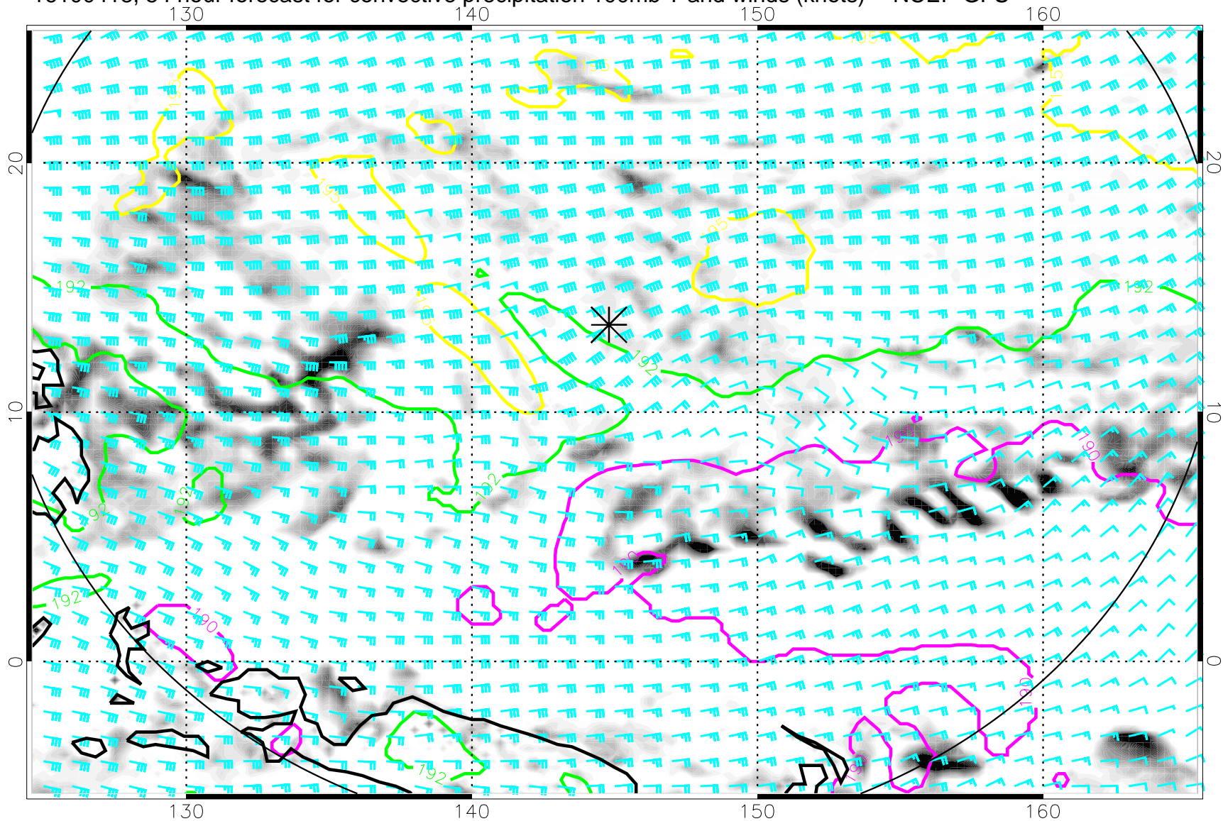
16100418, 54 hour forecast for convective precipitation 100mb T and winds (knots) -- NCEP GFS
