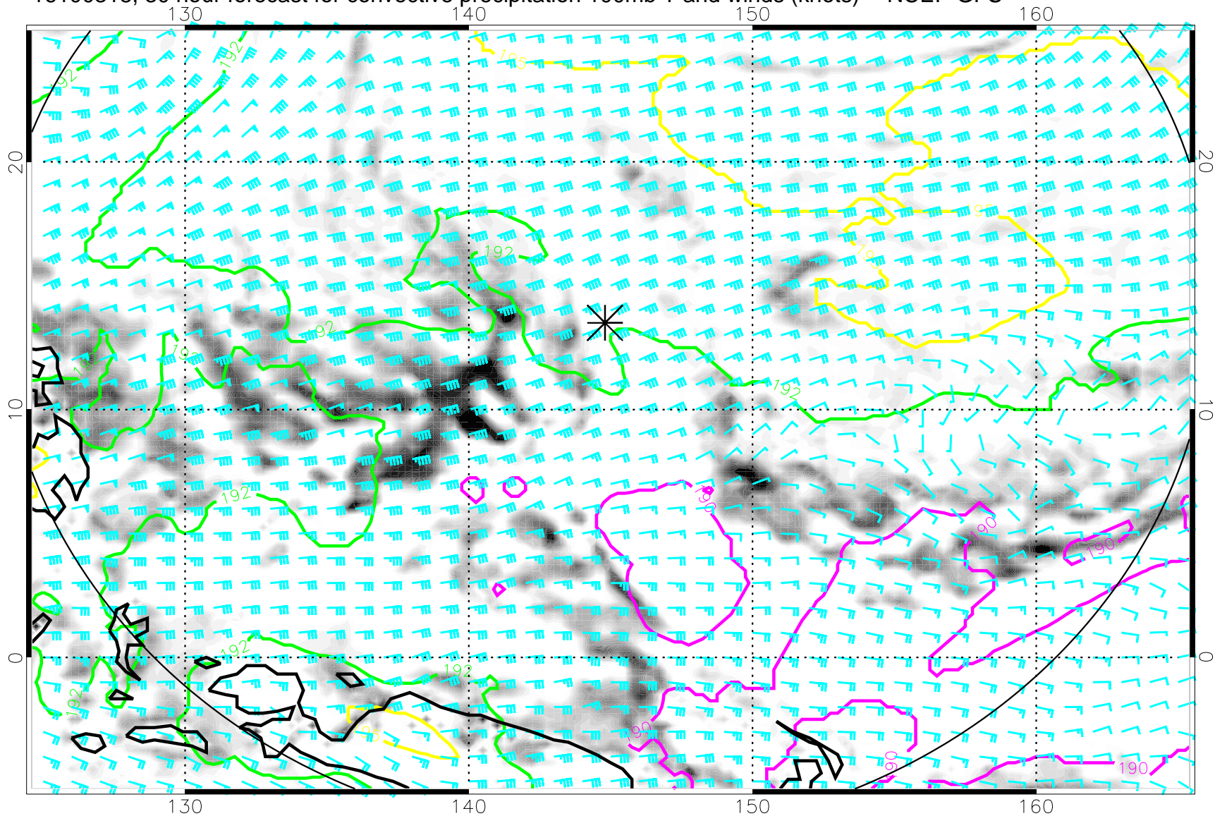
16100318, 30 hour forecast for convective precipitation 100mb T and winds (knots) -- NCEP GFS
