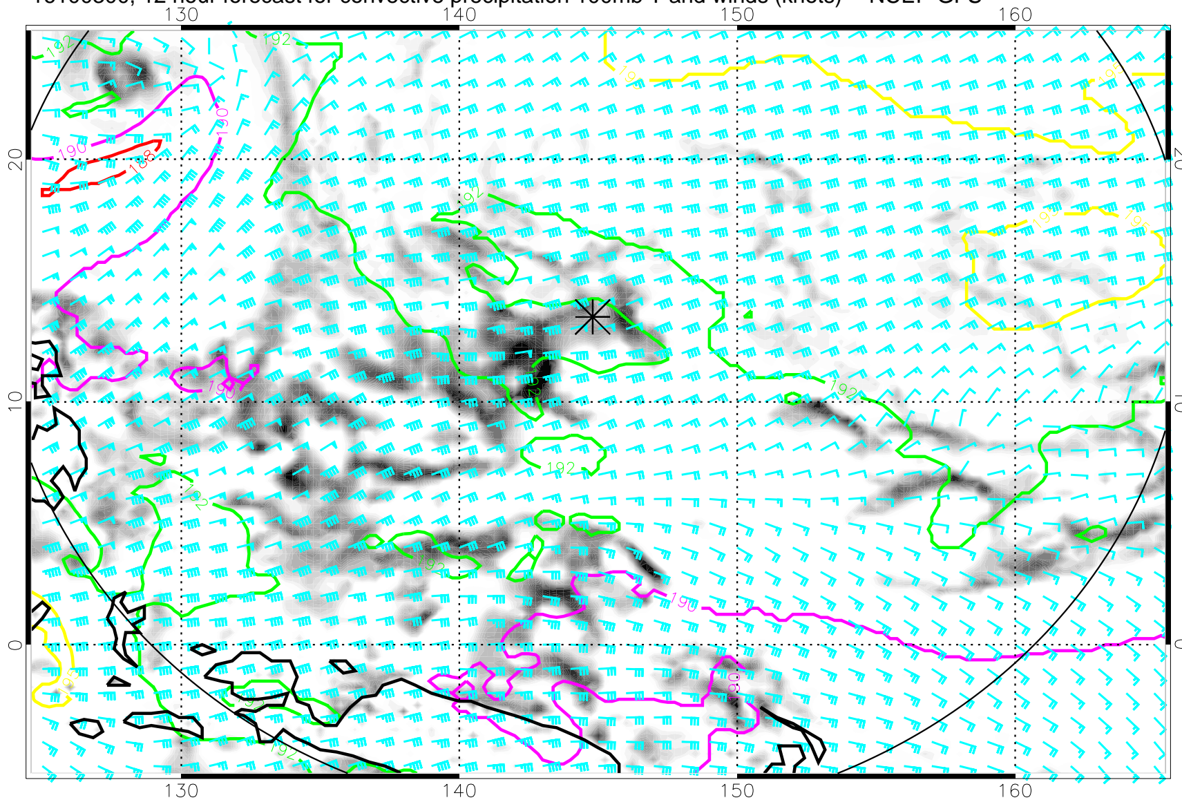
16100300, 12 hour forecast for convective precipitation 100mb T and winds (knots) -- NCEP GFS
