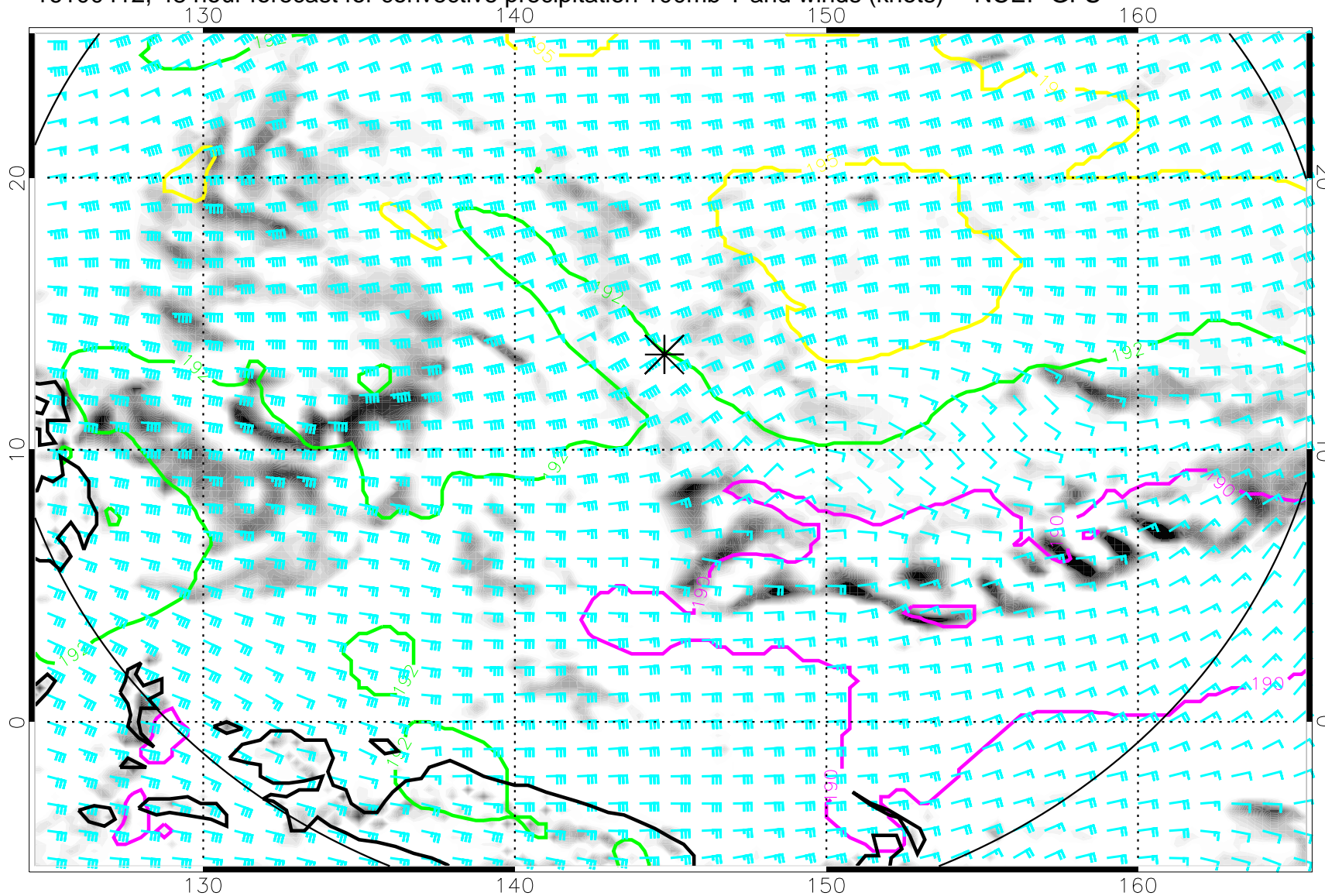
16100412, 48 hour forecast for convective precipitation 100mb T and winds (knots) -- NCEP GFS
