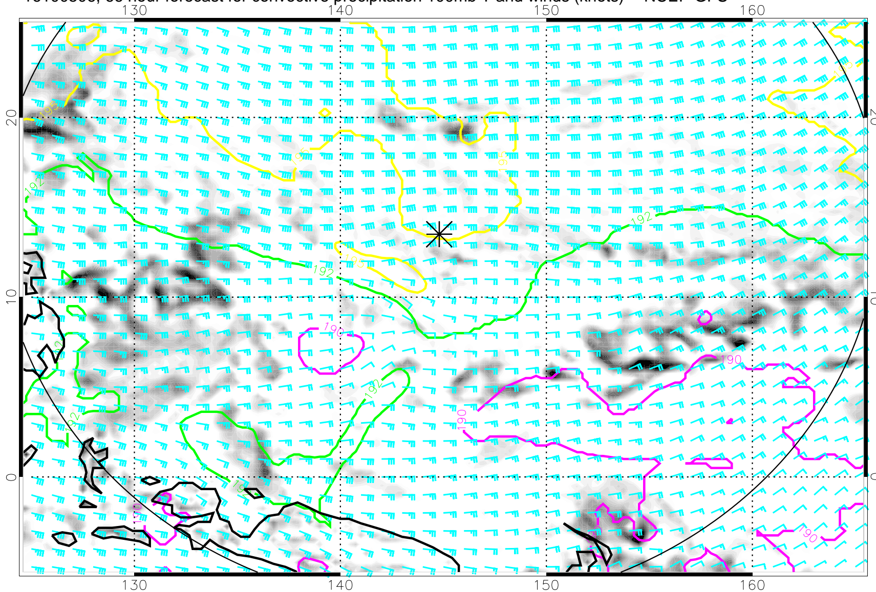
16100506, 66 hour forecast for convective precipitation 100mb T and winds (knots) -- NCEP GFS
