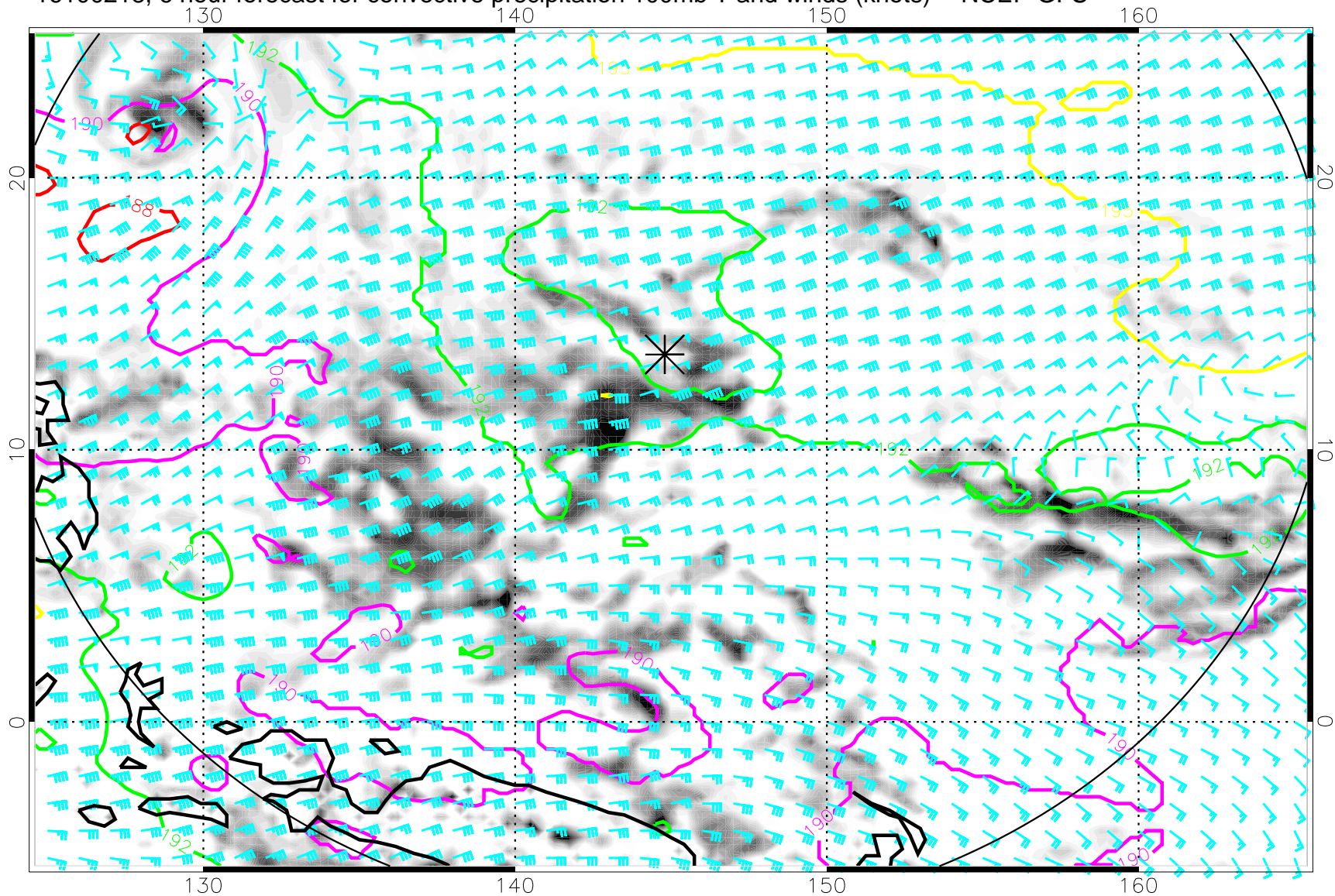
16100218, 6 hour forecast for convective precipitation 100mb T and winds (knots) -- NCEP GFS
