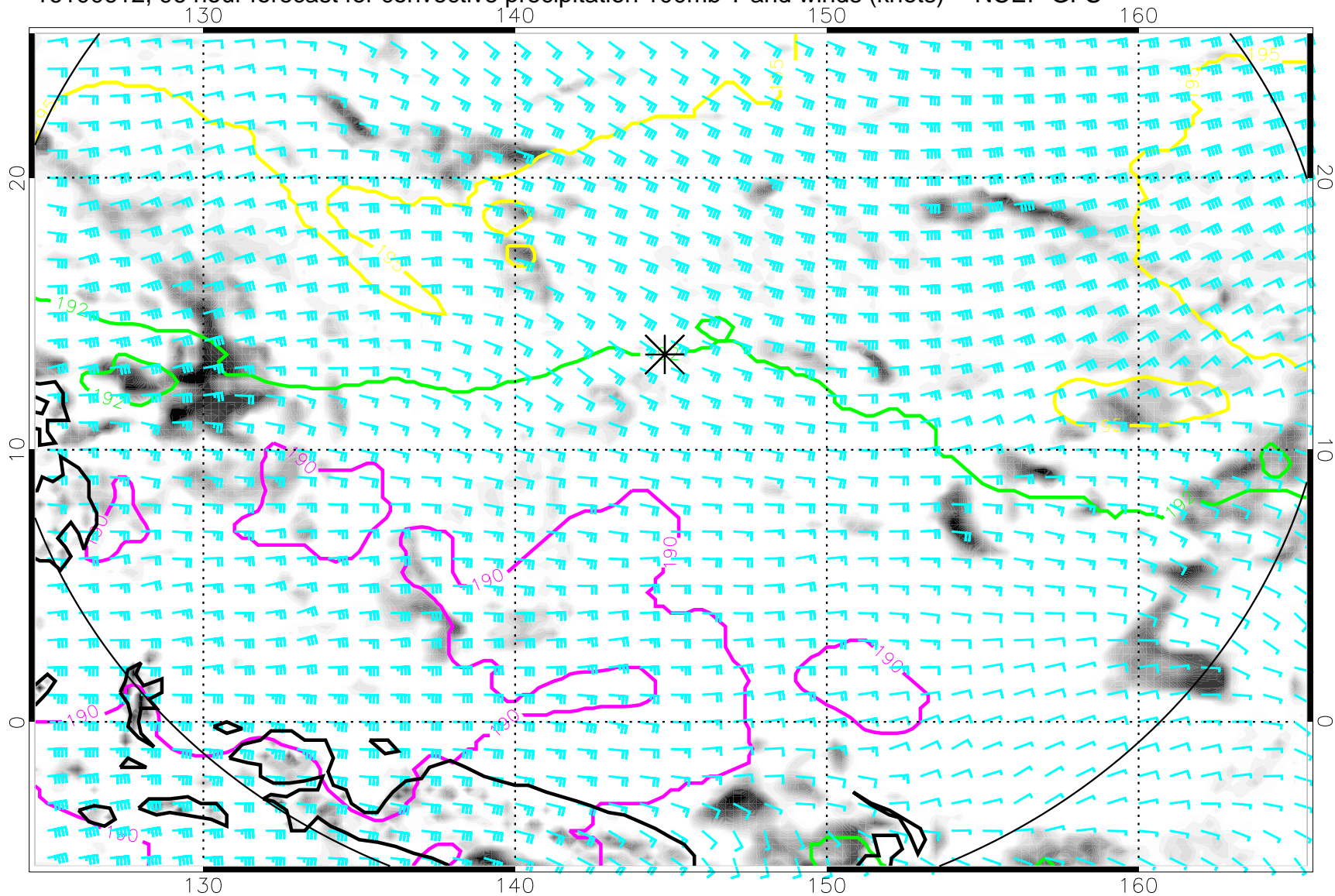
16100612, 96 hour forecast for convective precipitation 100mb T and winds (knots) -- NCEP GFS
