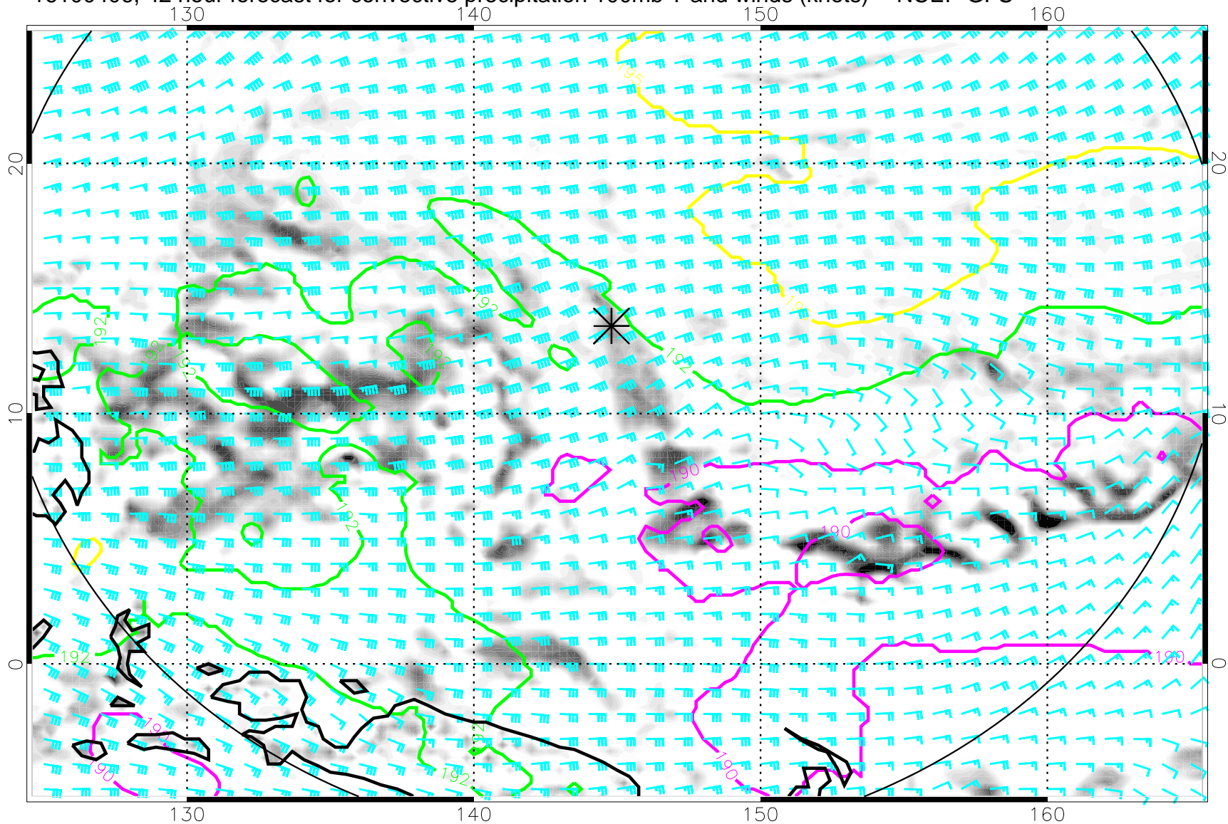
16100406, 42 hour forecast for convective precipitation 100mb T and winds (knots) -- NCEP GFS
