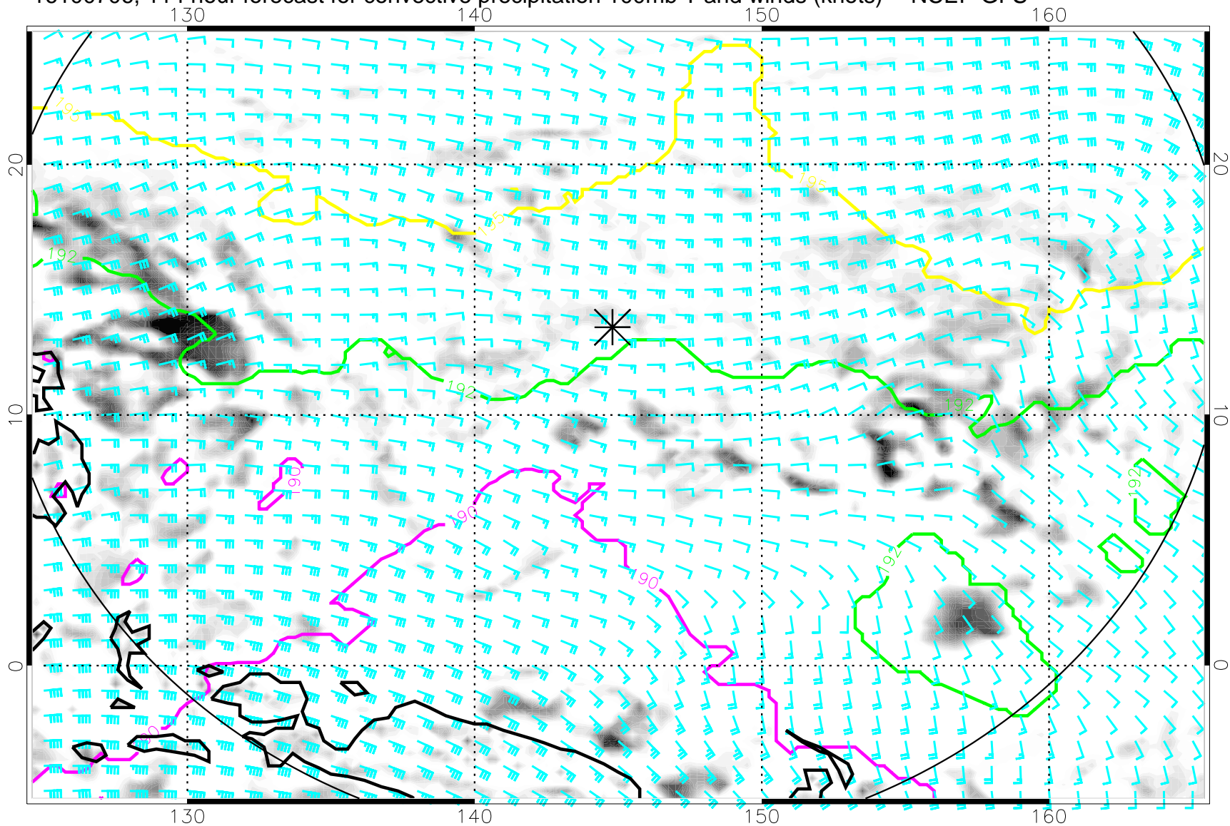
16100706, 114 hour forecast for convective precipitation 100mb T and winds (knots) -- NCEP GFS
