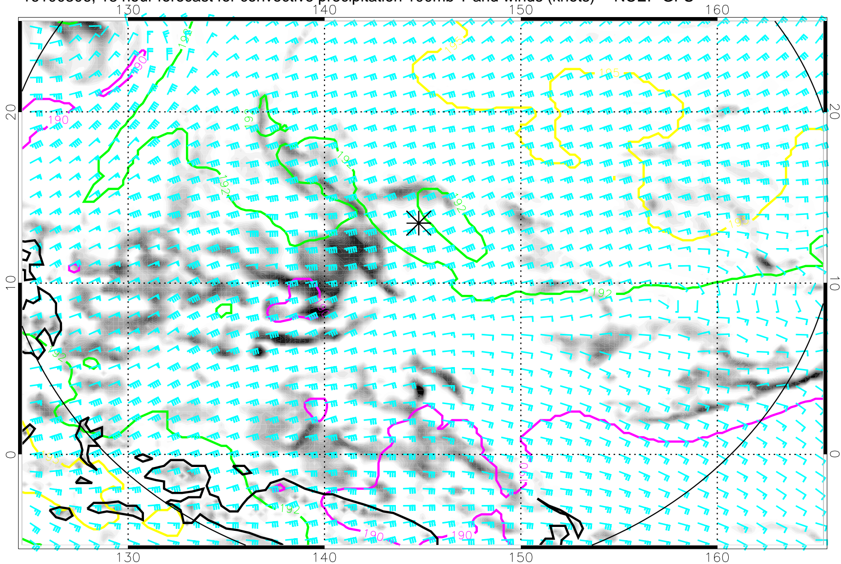
16100306, 18 hour forecast for convective precipitation 100mb T and winds (knots) -- NCEP GFS
