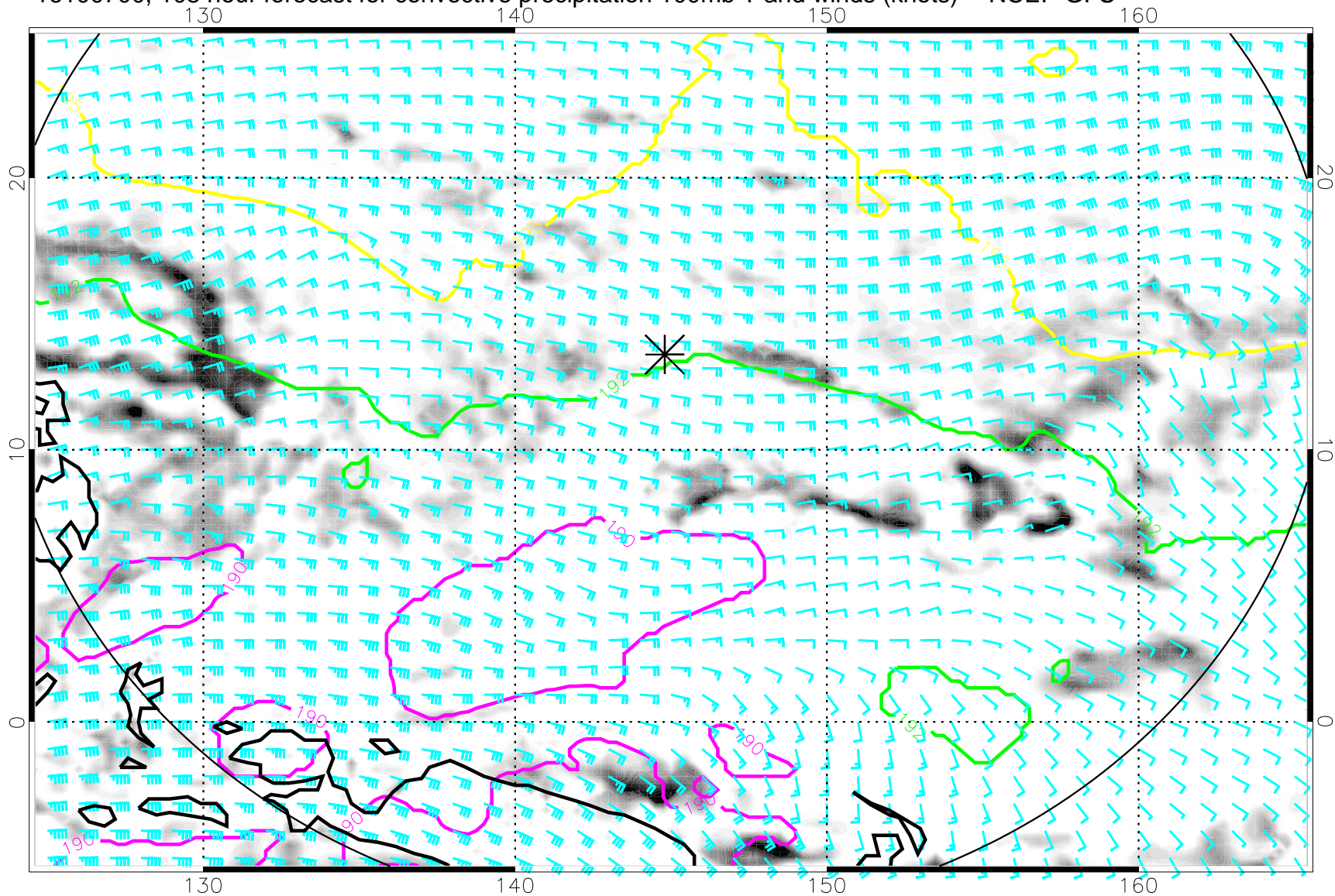
16100700, 108 hour forecast for convective precipitation 100mb T and winds (knots) -- NCEP GFS
