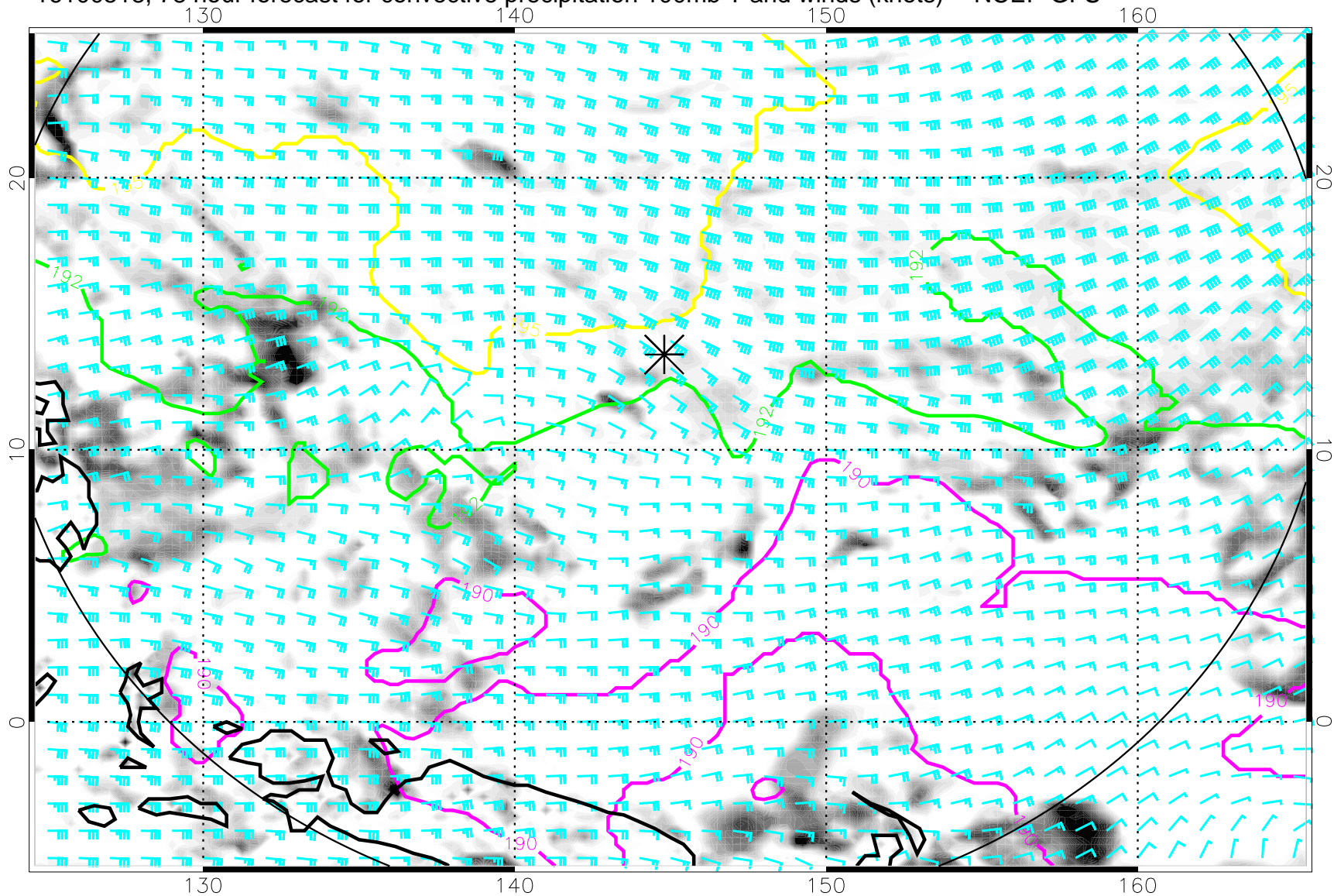
16100518, 78 hour forecast for convective precipitation 100mb T and winds (knots) -- NCEP GFS
