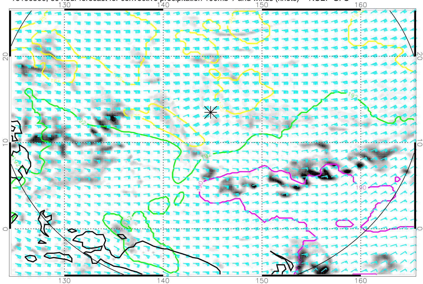
16100500, 60 hour forecast for convective precipitation 100mb T and winds (knots) -- NCEP GFS
