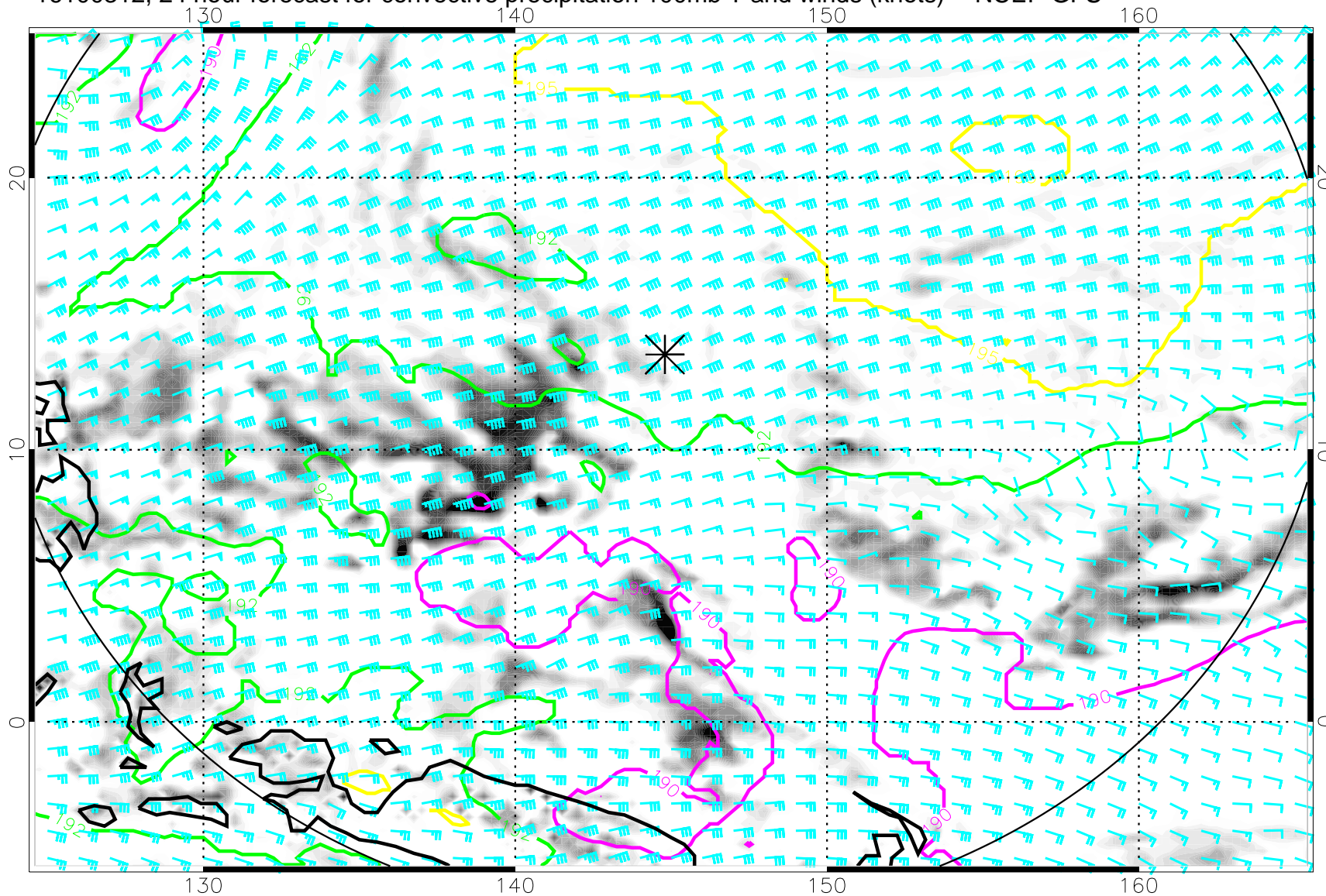
16100312, 24 hour forecast for convective precipitation 100mb T and winds (knots) -- NCEP GFS
