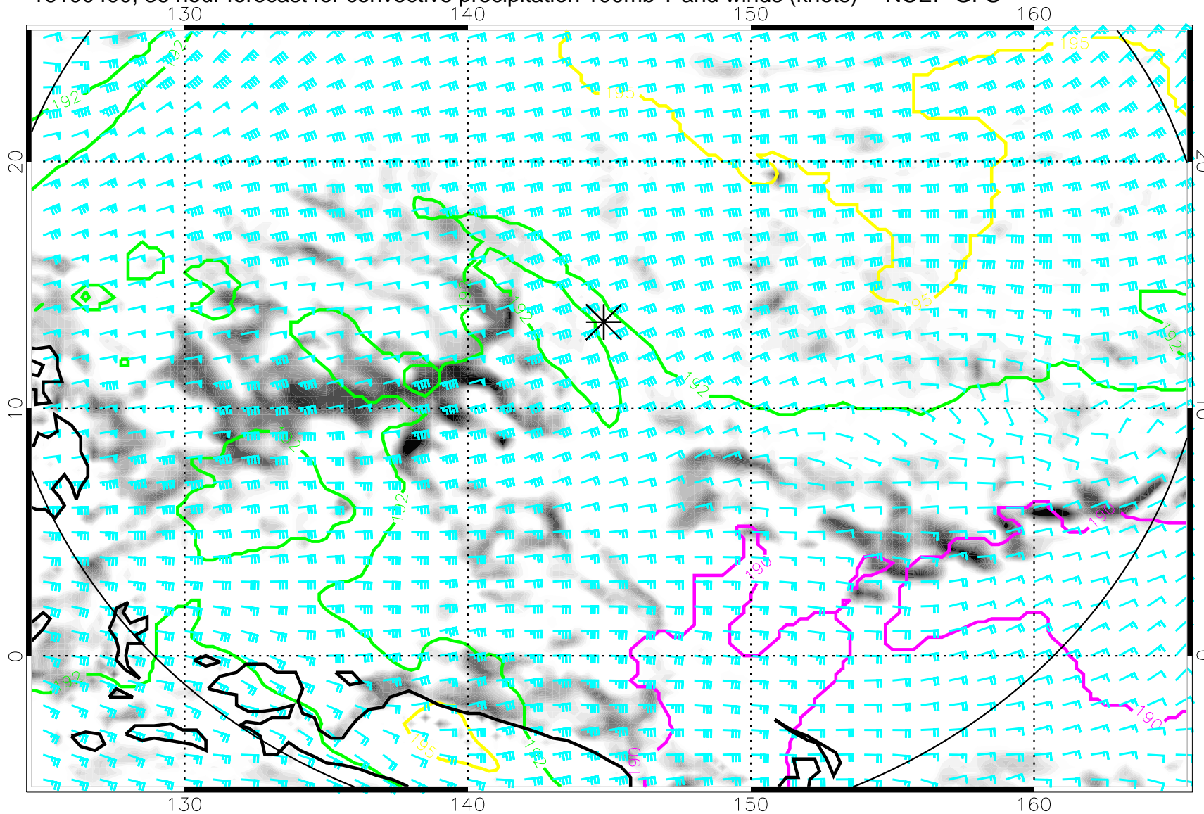
16100400, 36 hour forecast for convective precipitation 100mb T and winds (knots) -- NCEP GFS
