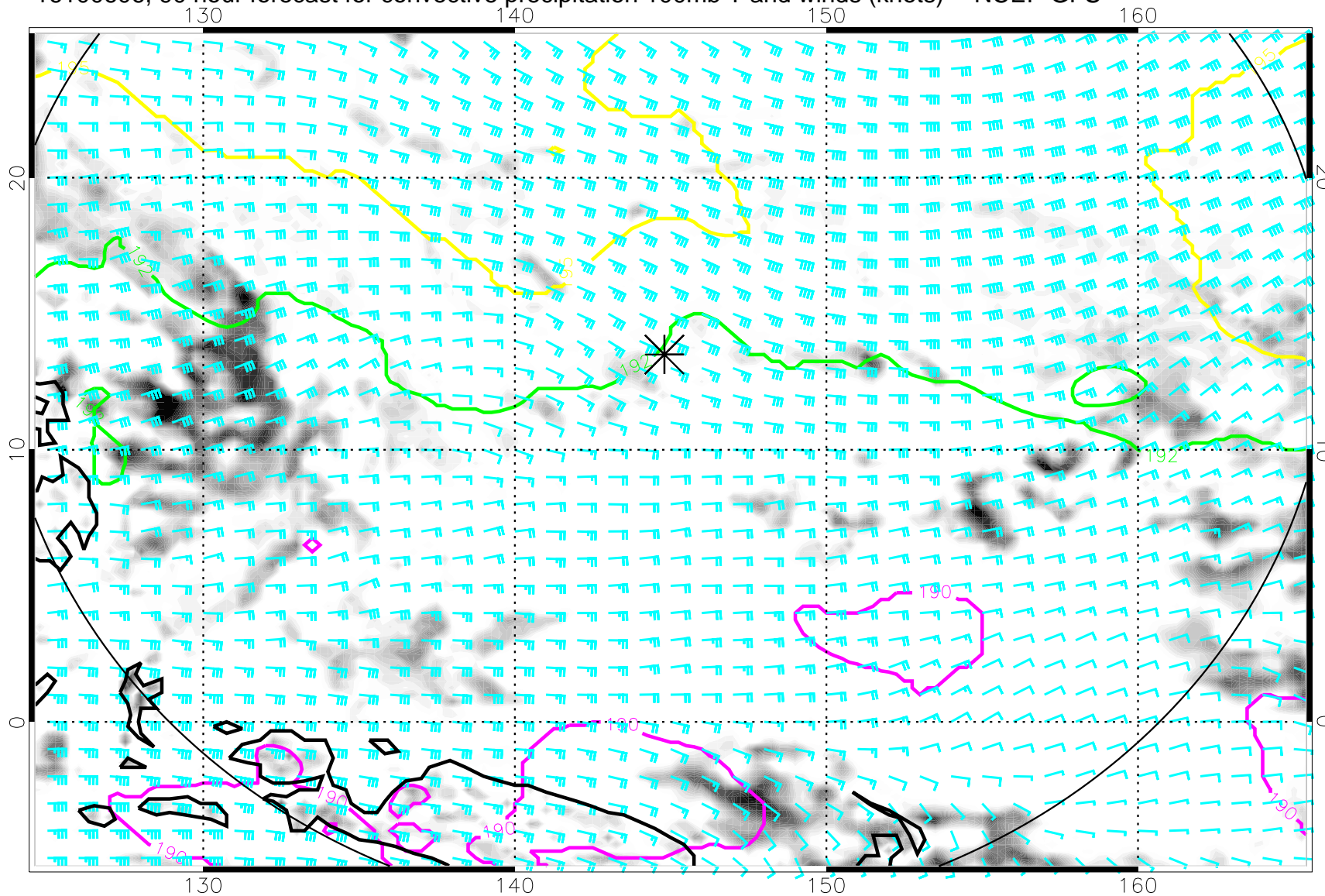
16100606, 90 hour forecast for convective precipitation 100mb T and winds (knots) -- NCEP GFS
