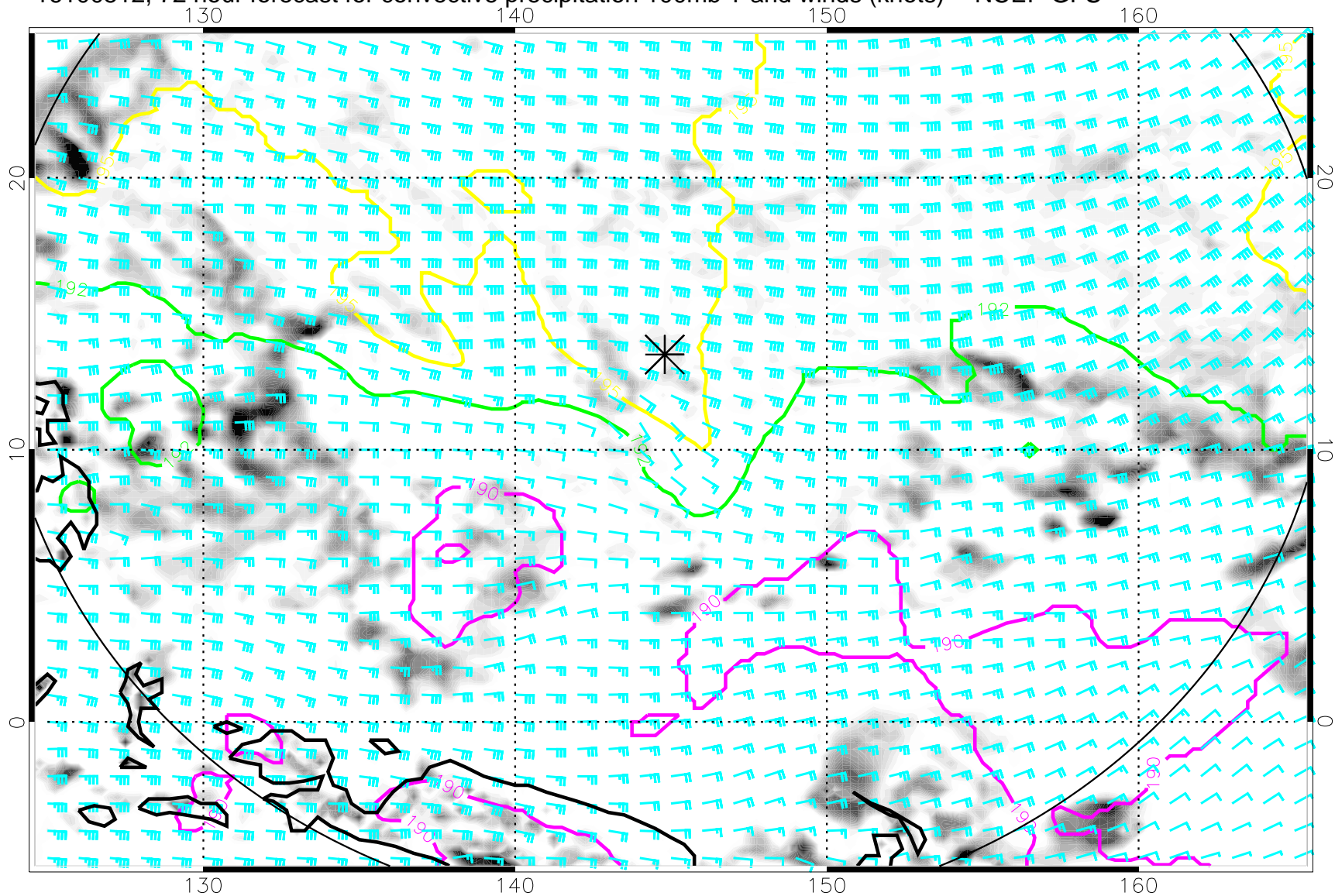
16100512, 72 hour forecast for convective precipitation 100mb T and winds (knots) -- NCEP GFS
